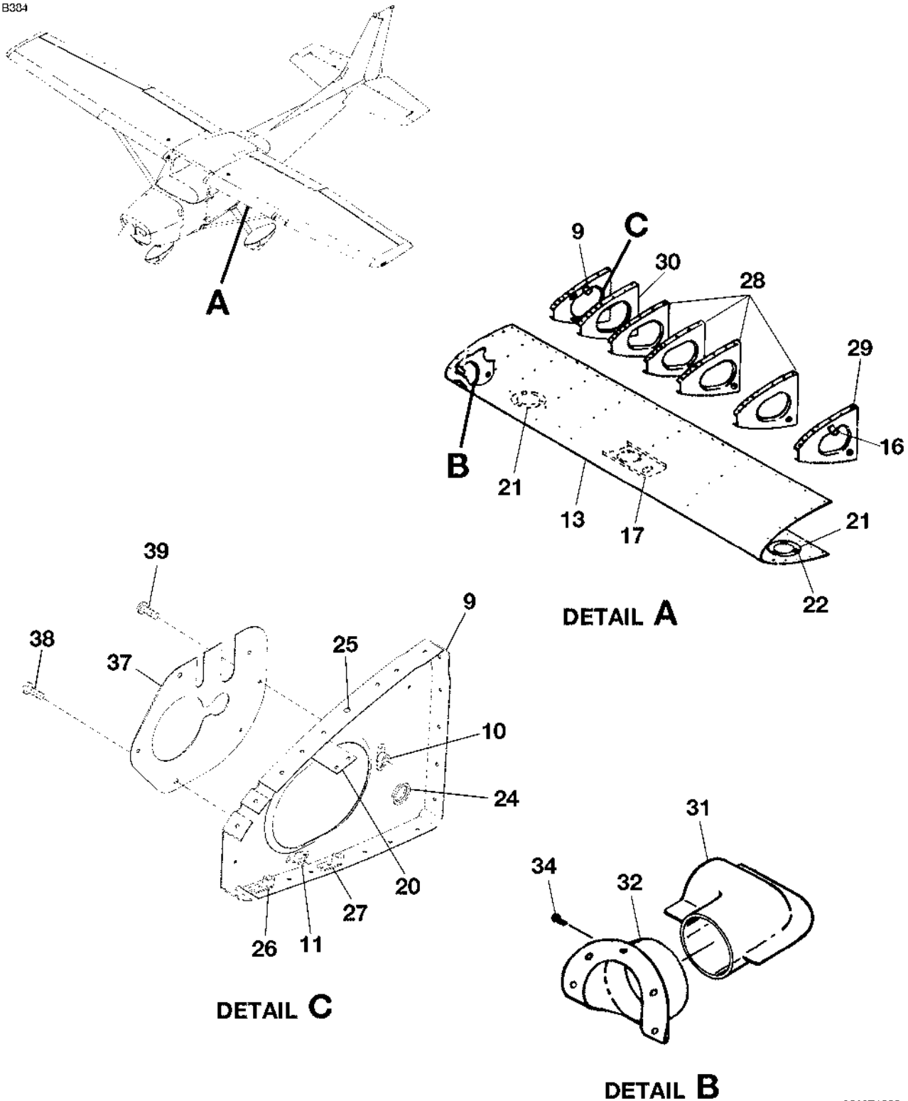
LEADING EDGE ASSEMBLY - INBOARD WING FIGURE 01 (SHEET 1)
