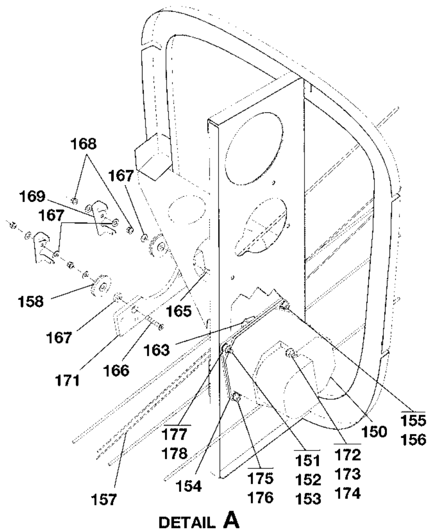
AUTOPILOT INSTALLATION KAP & KC-140 FIGURE 01 (SHEET 3)
