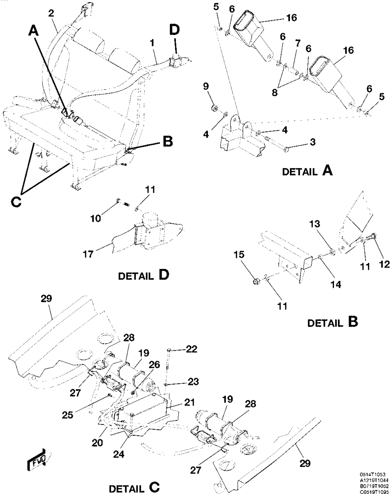
AMSAFE INFLATABLE RESTRAINT SYSTEM FIGURE 01A (SHEET 1)
