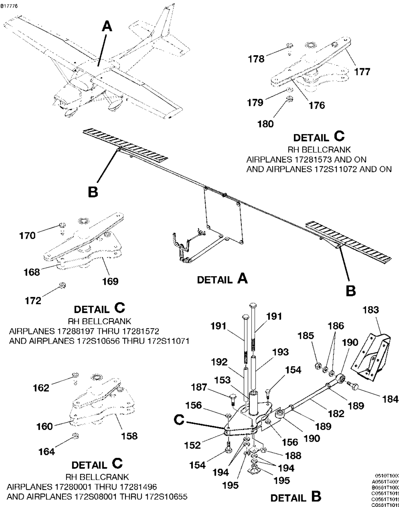
AILERON CONTROL SYSTEM FIGURE 03 (SHEET 3)
