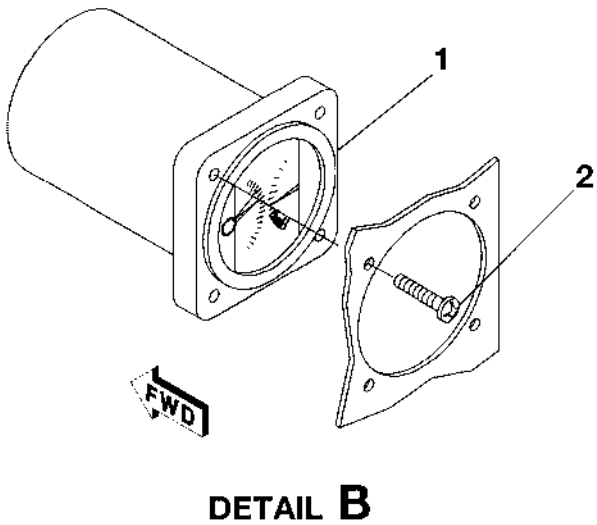
EXHAUST TEMPERATURE GAUGE INSTALLATION FIGURE 01 (SHEET 1)
