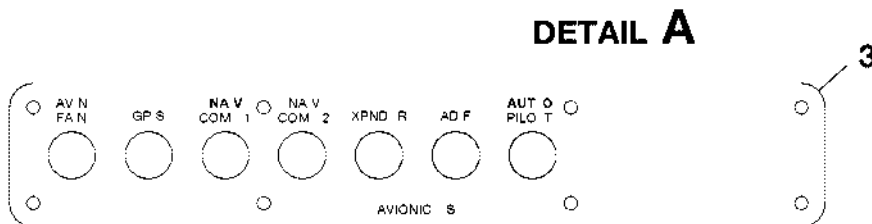
BEZEL PANEL SILKSCREENS FIGURE 03 (SHEET 1)
