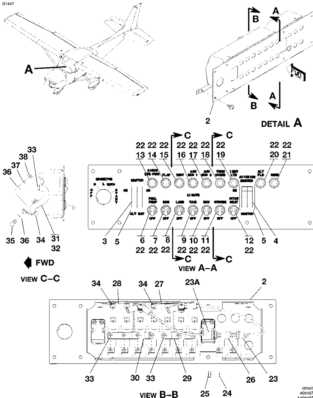
CIRCUIT BREAKER PANEL ASSEMBLY FIGURE 01A (SHEET 1)
