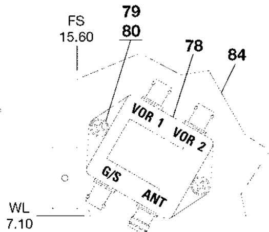
VIEW A-A LOOKING OUTBD AT LH SIDE
