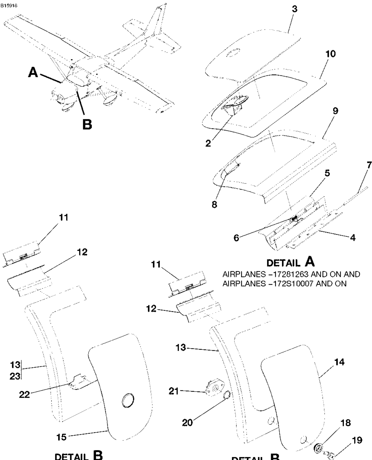
SERVICE DOORS FIGURE 02 (SHEET 1)
