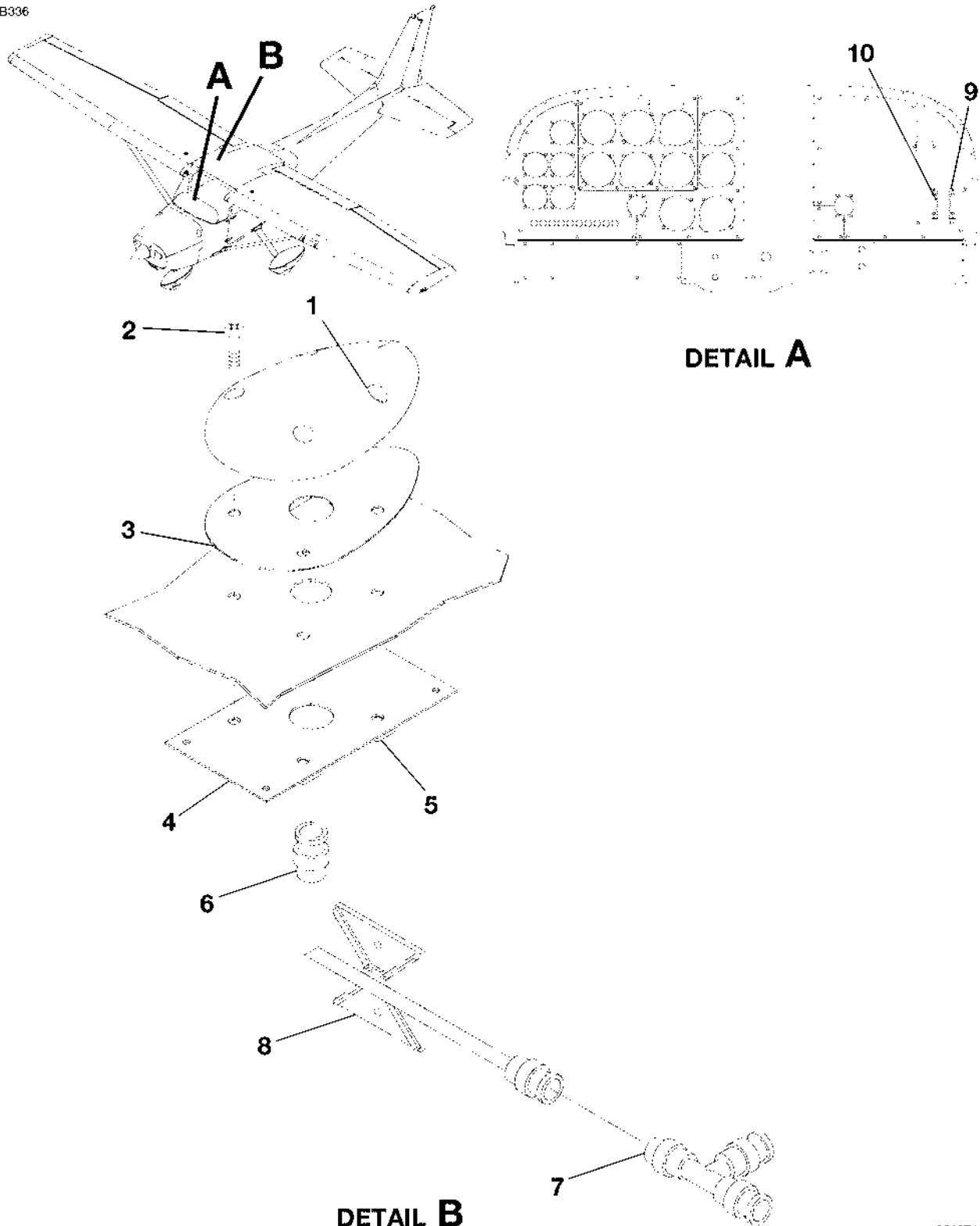
GLOBAL POSITIONING SYSTEM (GPS) INSTALLATION FIGURE 01 (SHEET 1)
