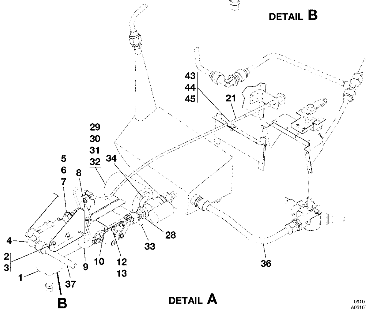
FUEL SYSTEM FIGURE 01 (SHEET 1)
