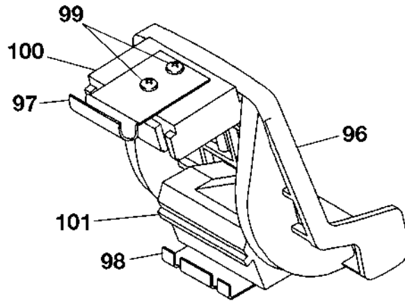
RUDDER PEDAL EXTENSION
