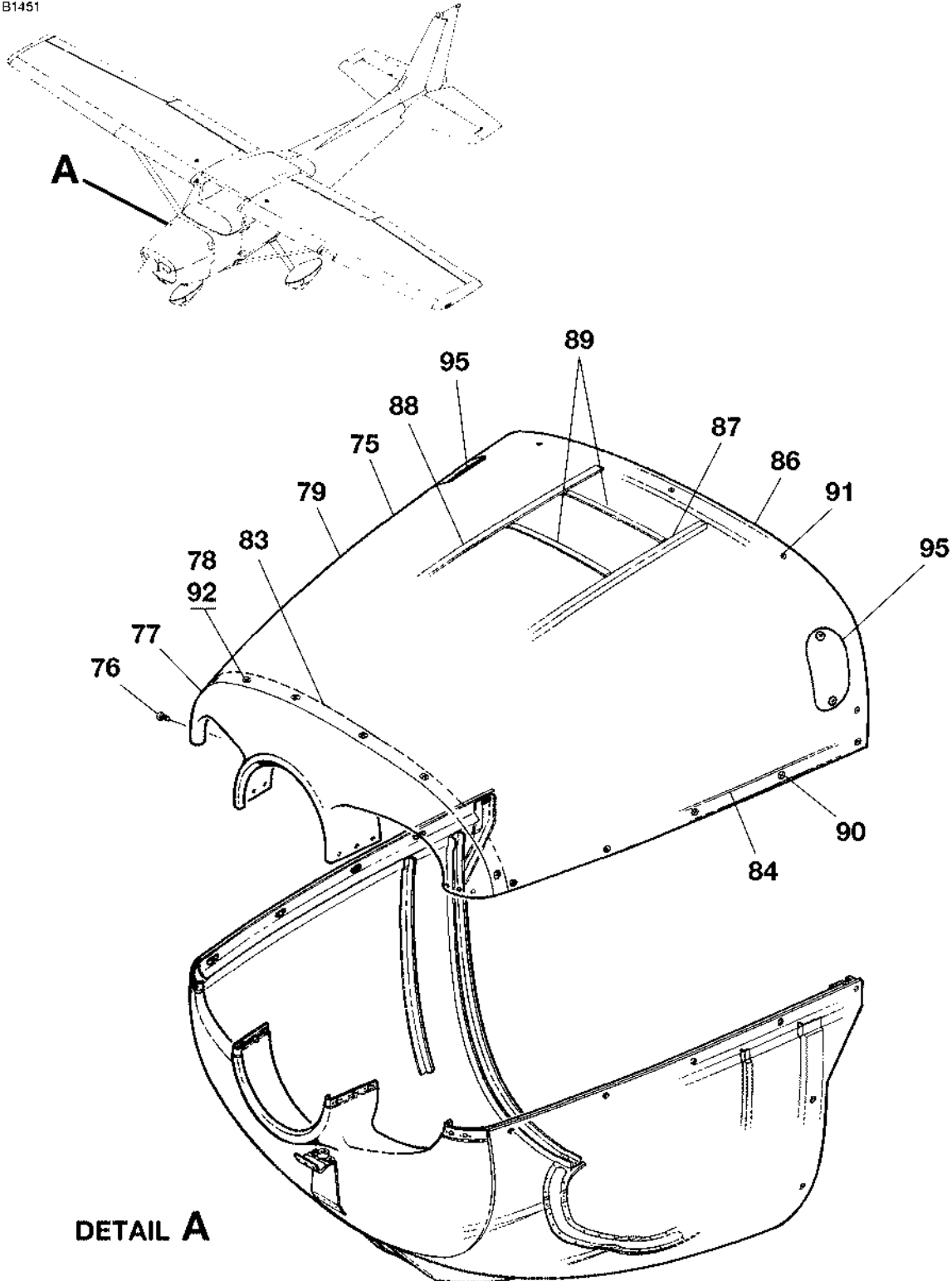
ENGINE COWL ASSEMBLY FIGURE 01 (SHEET 2)
