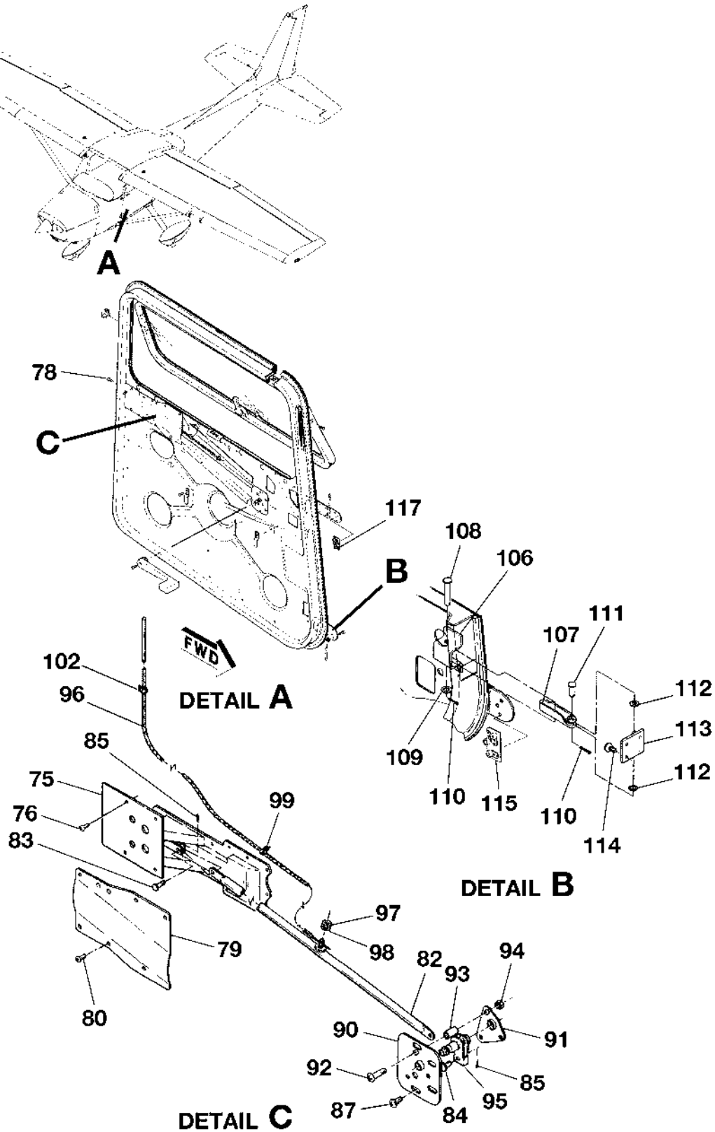
CABIN DOOR INSTALLATION - LH FIGURE 01 (SHEET 2)
