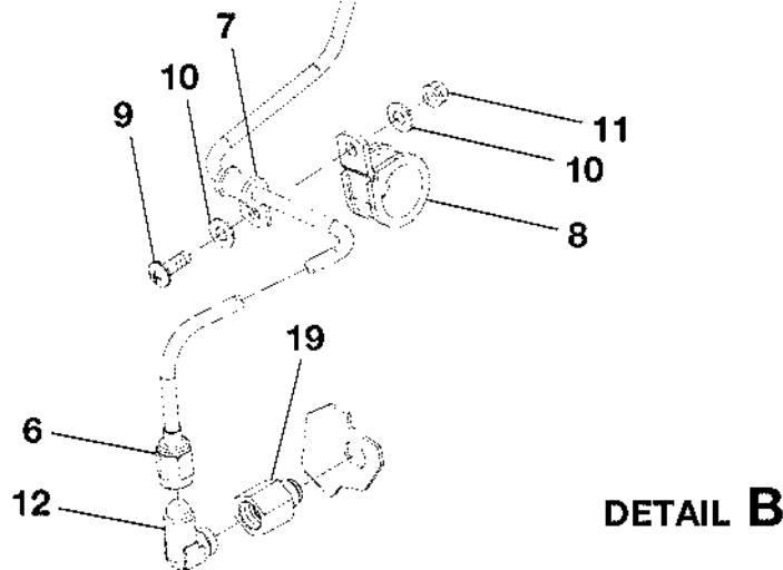
OIL INDICATING SYSTEM FIGURE 01 (SHEET 1)
