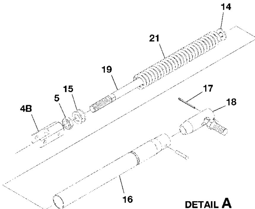
NOSE GEAR STEERING TUBE ASSEMBLY FIGURE 01 (SHEET 1)
