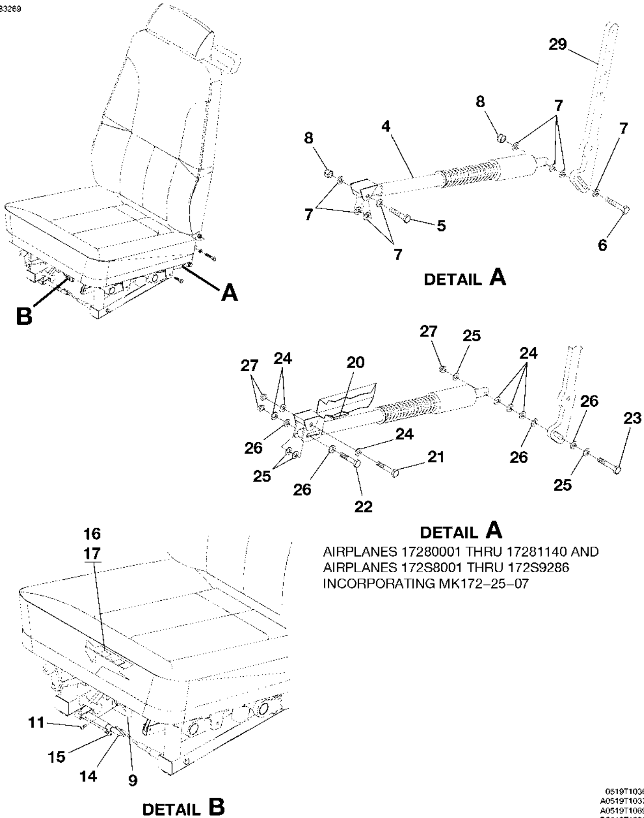
SEAT ASSEMBLY - PILOT AND COPILOT FIGURE 02 (SHEET 1)
