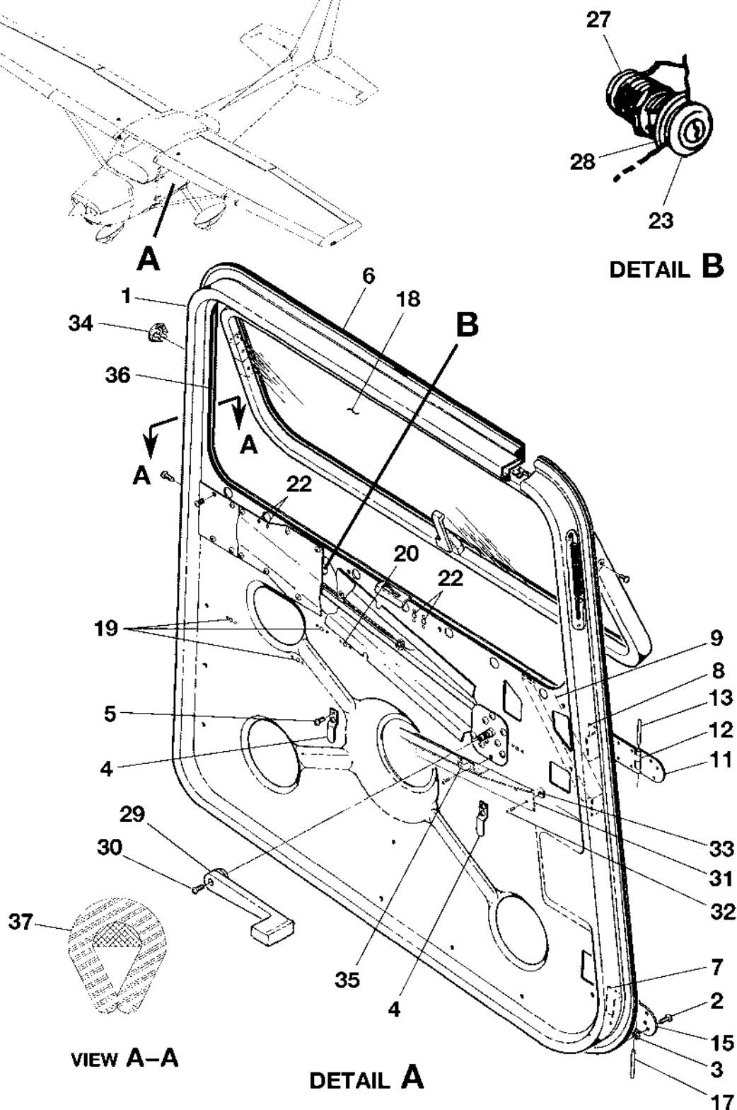
CABIN DOOR INSTALLATION - LH FIGURE 01 (SHEET 1)
