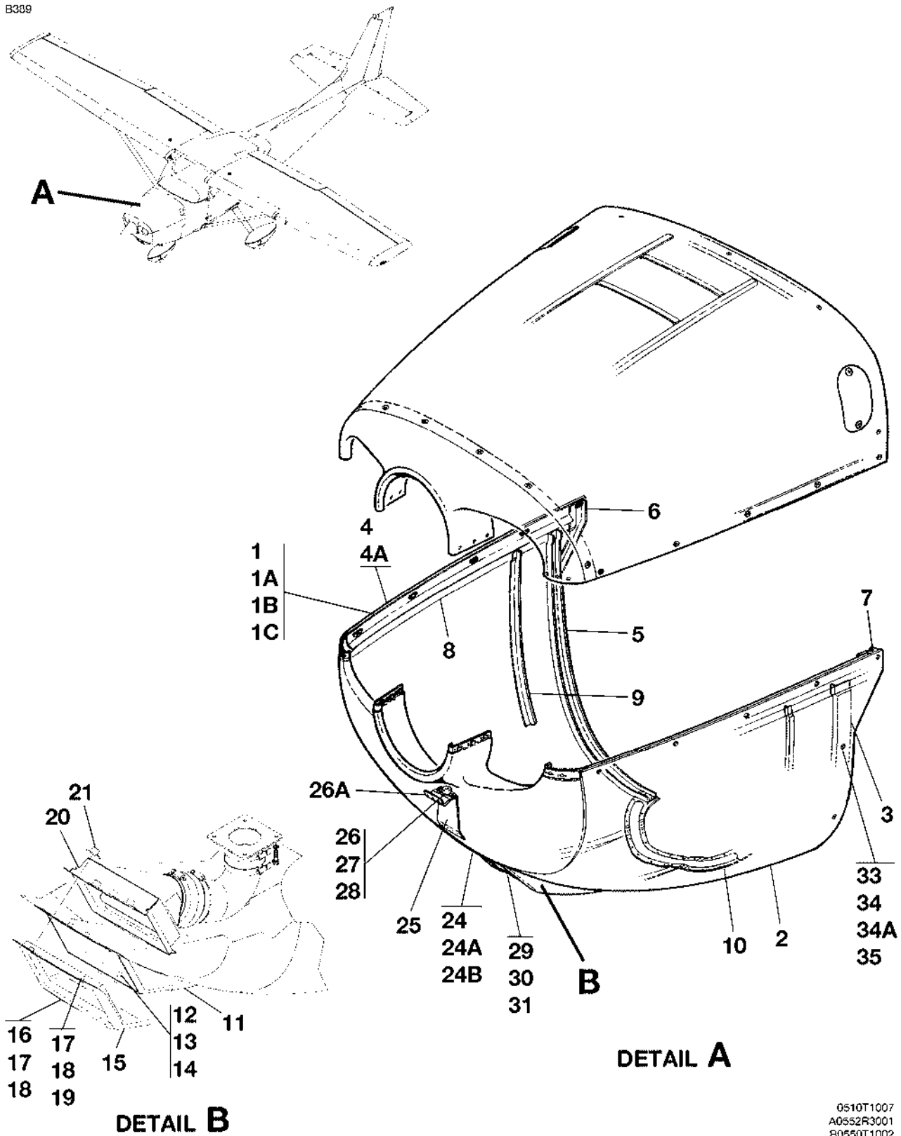
ENGINE COWL ASSEMBLY FIGURE 01 (SHEET 1)
