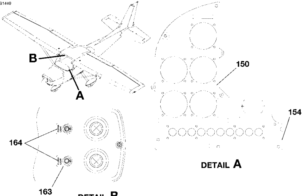
NAV III OVERHEAD CONSOLE SILKSCREEN
