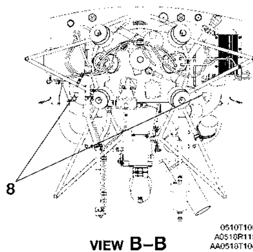
EXHAUST TEMPERATURE GAUGE INSTALLATION FIGURE 01 (SHEET 1)
