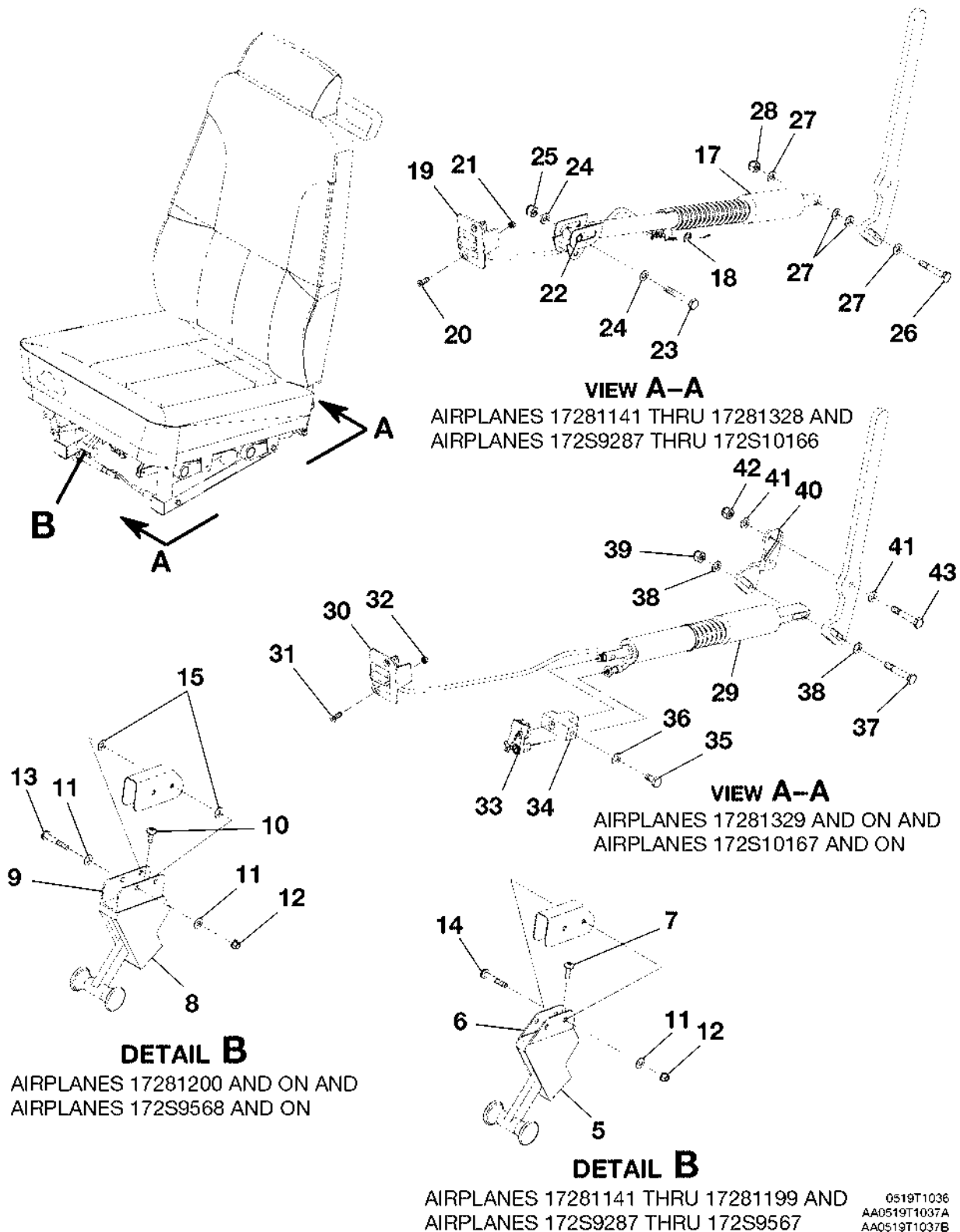
SEAT ASSEMBLY-PILOT AND COPILOT FIGURE 03 (SHEET 1)
