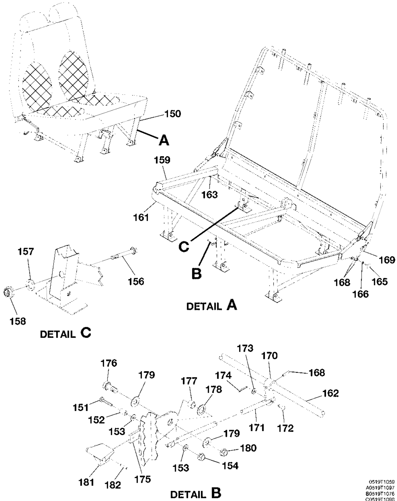
AFT BENCH SEAT INSTALLATION FIGURE 01 (SHEET 3)
