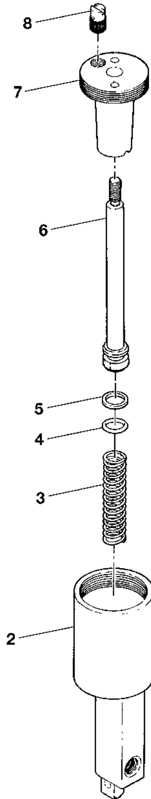
MASTER BRAKE CYLINDER ASSEMBLY FIGURE 01 (SHEET 1)
