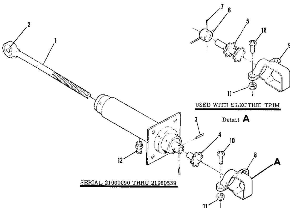
Figure 102C. Elevator Trim Tab Actuator Assembly
