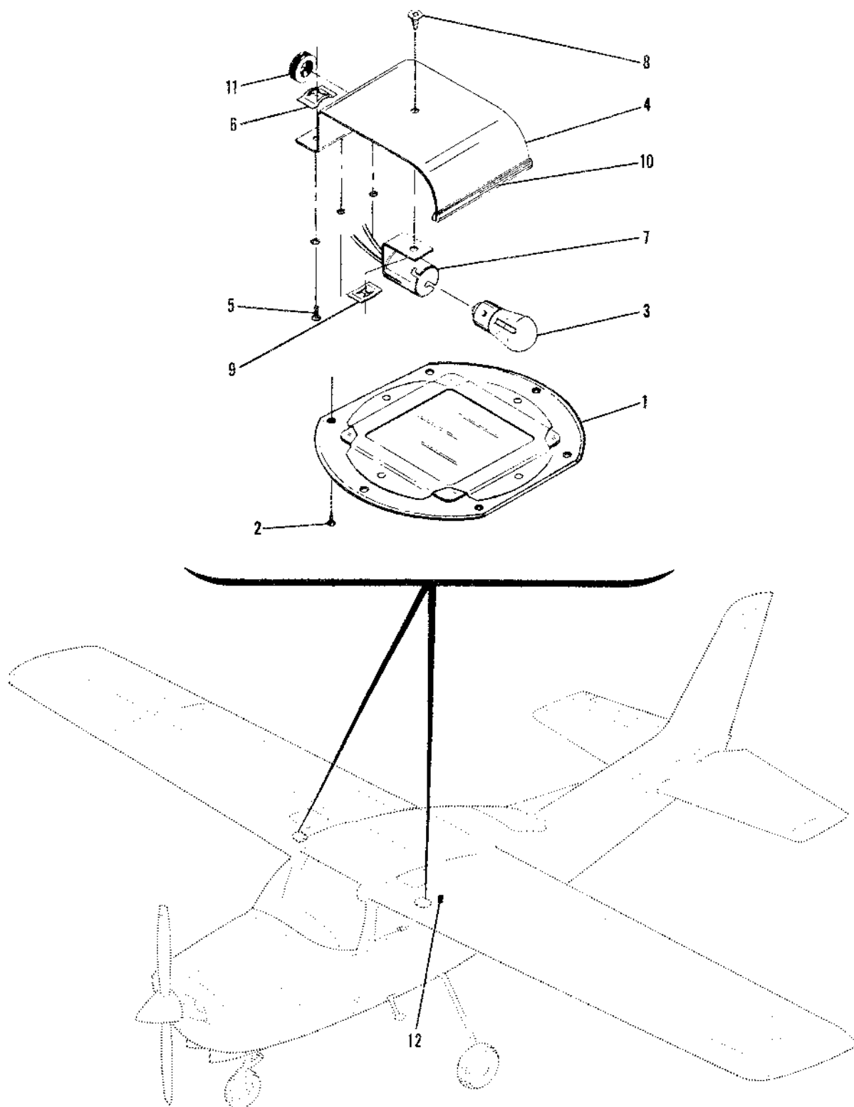
Figure 139. Courtesy Light Installation
