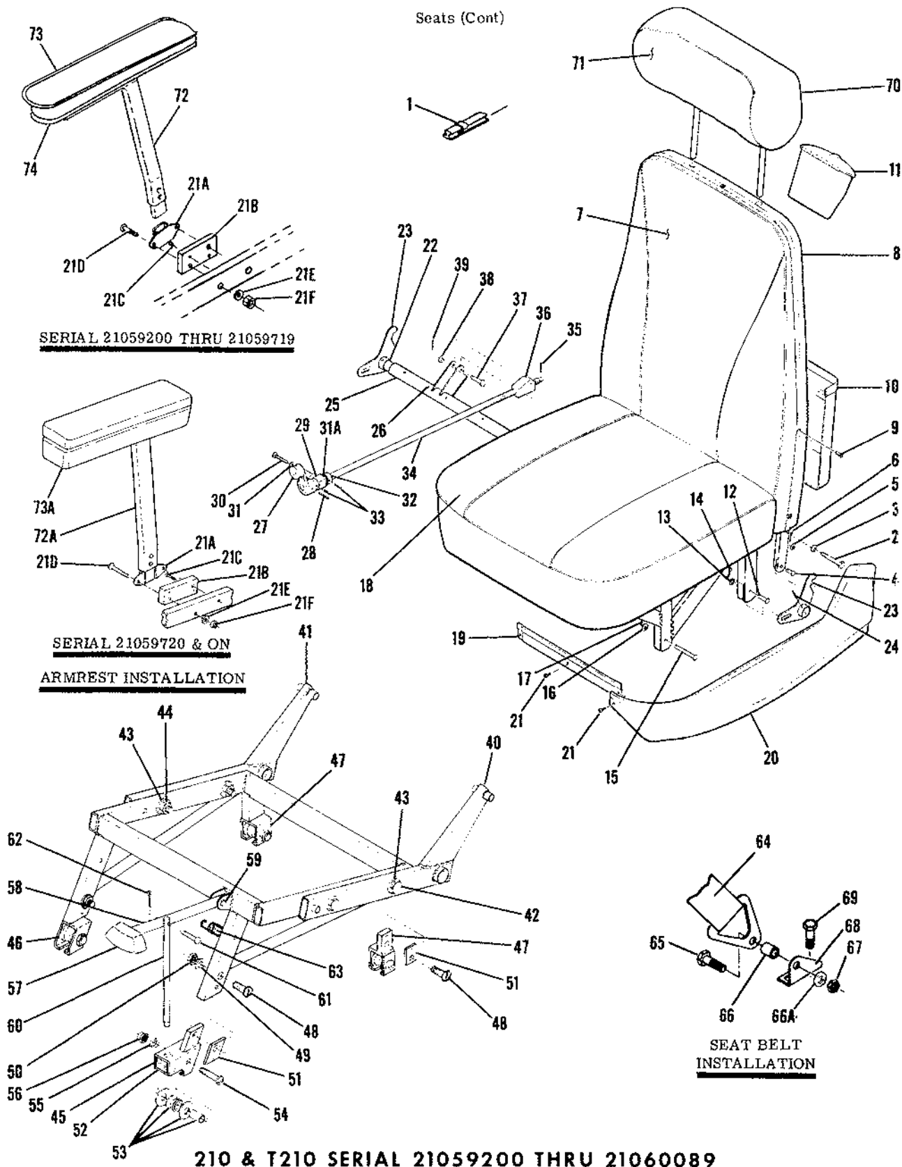
Figure 56. Articulating Recline Middle Seats Installation
