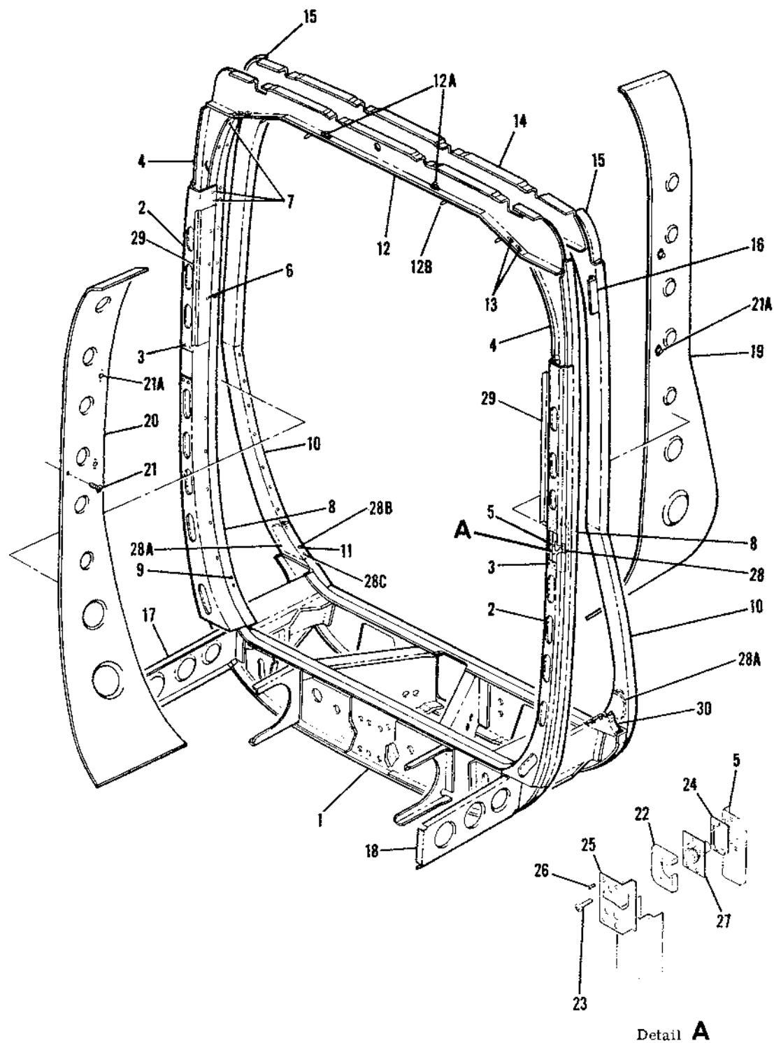
Figure 19. Rear Doorpost & Main Landing Gear Bulkhead Assembly
