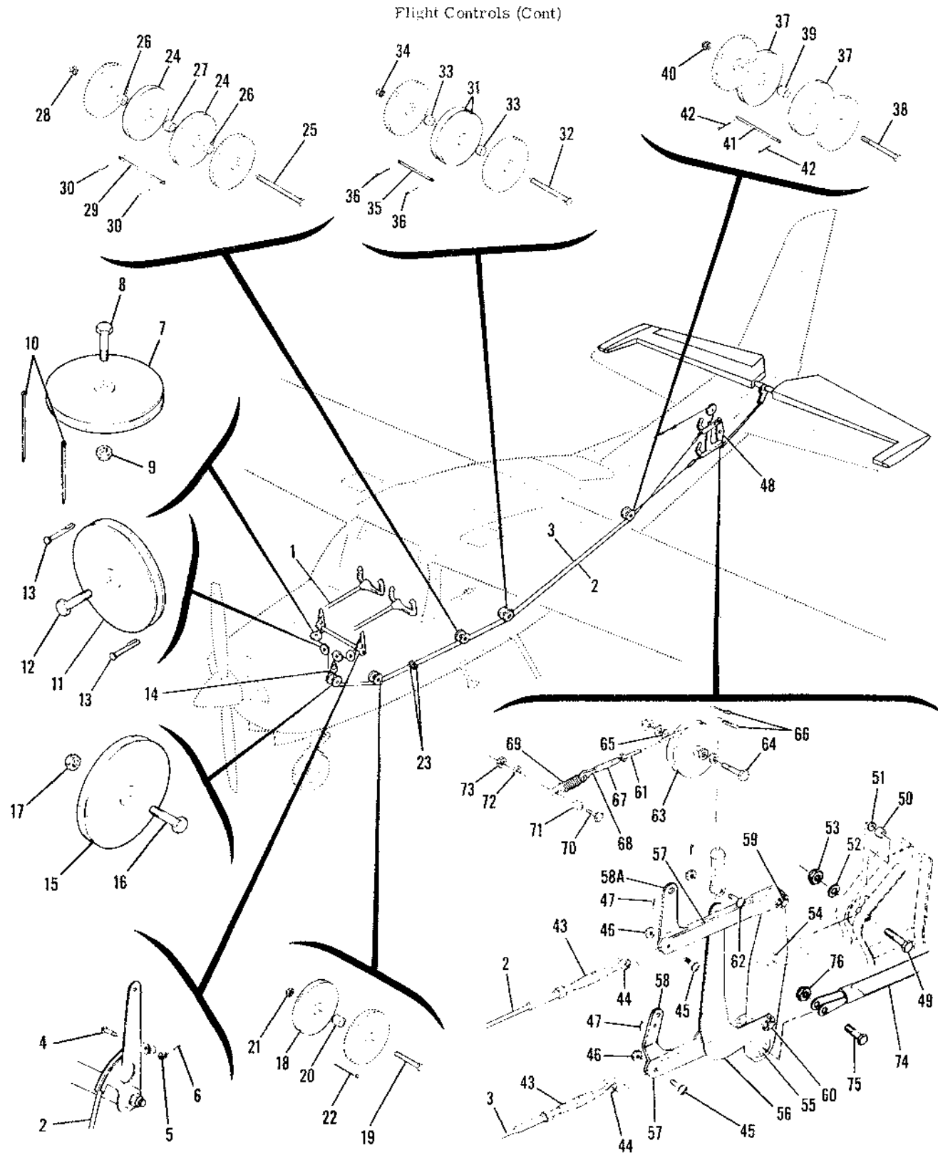
Figure 100. Elevator Control System Installation
