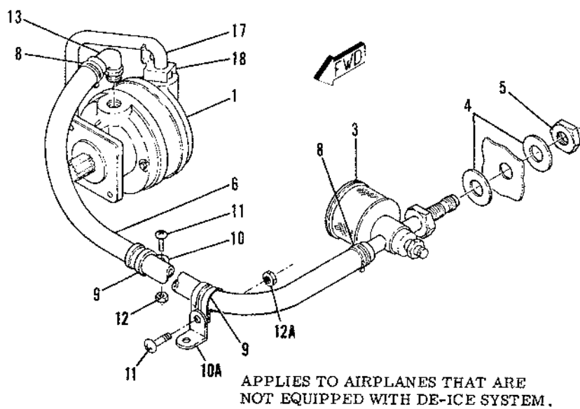
Figure 115A. Vacuum System Installation - Engine Driven
