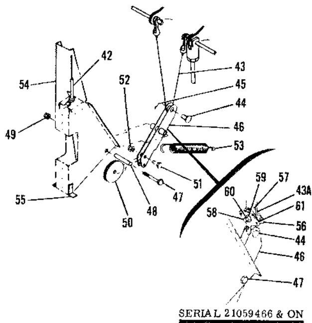
Figure 92. Brake System Installation
