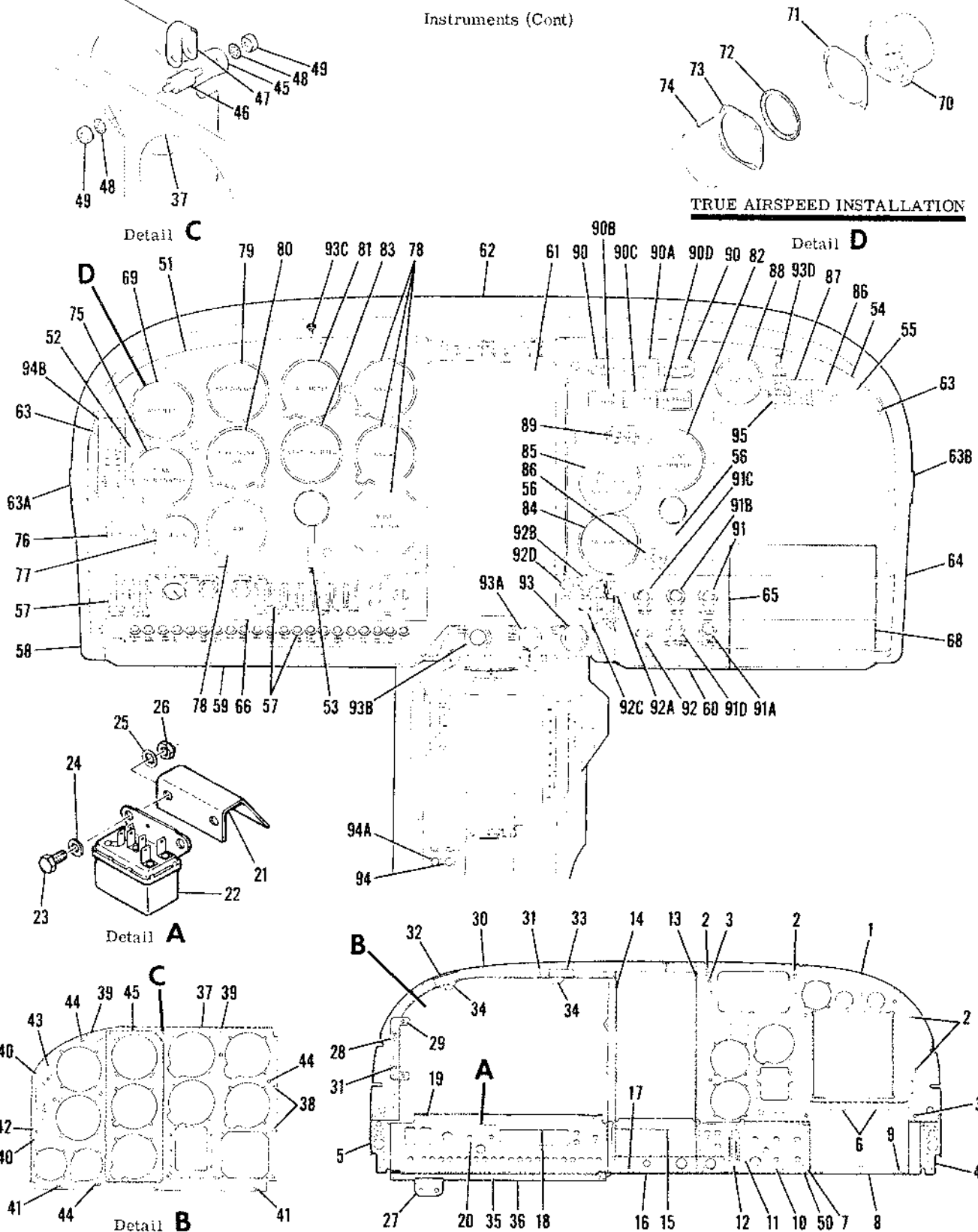
210 & T210 SERIAL 21061040 & ON Figure 58E, Instrument Panel Equipment Installation
