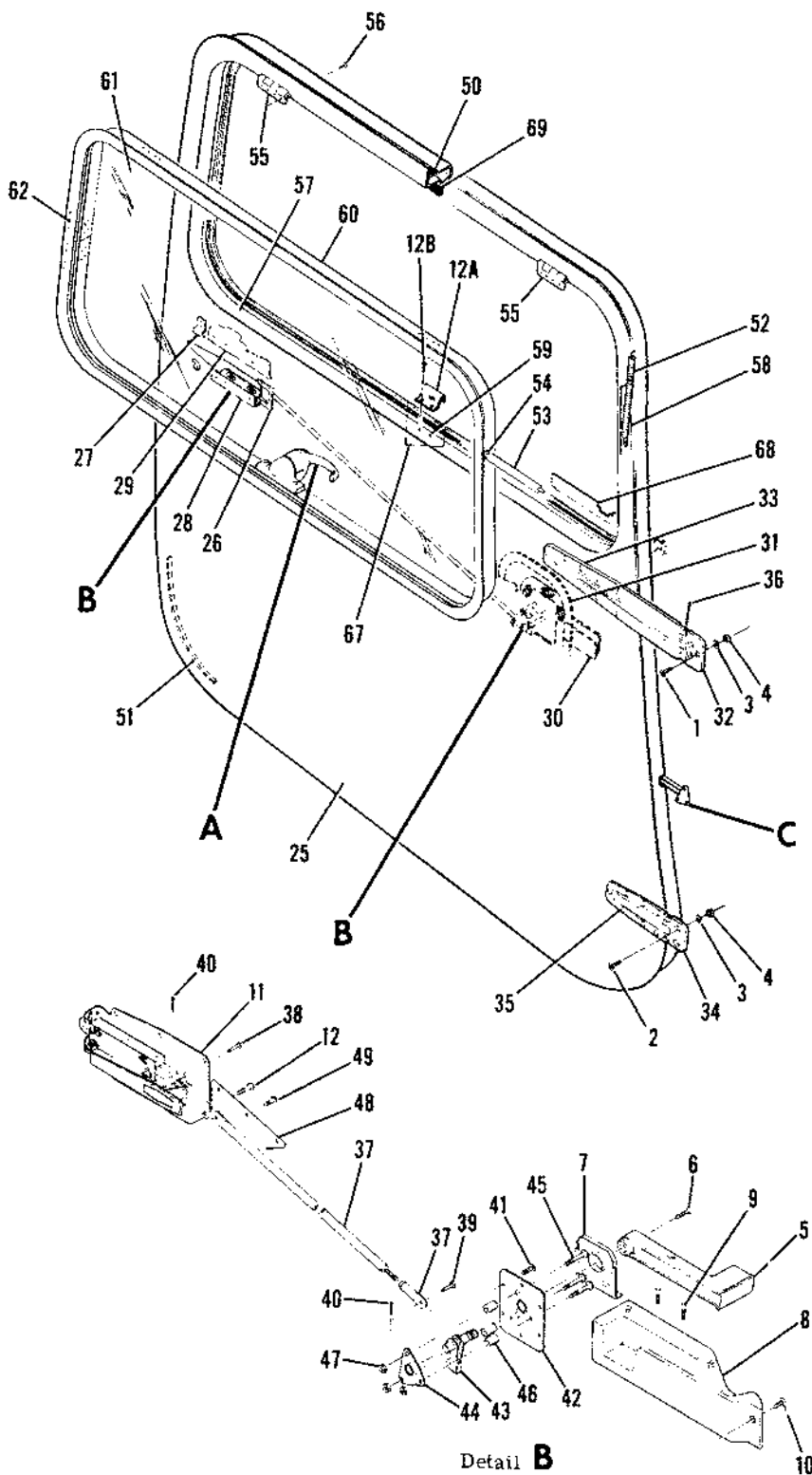
Figure 45B. Right Cabin Door Installation - Openable Window
