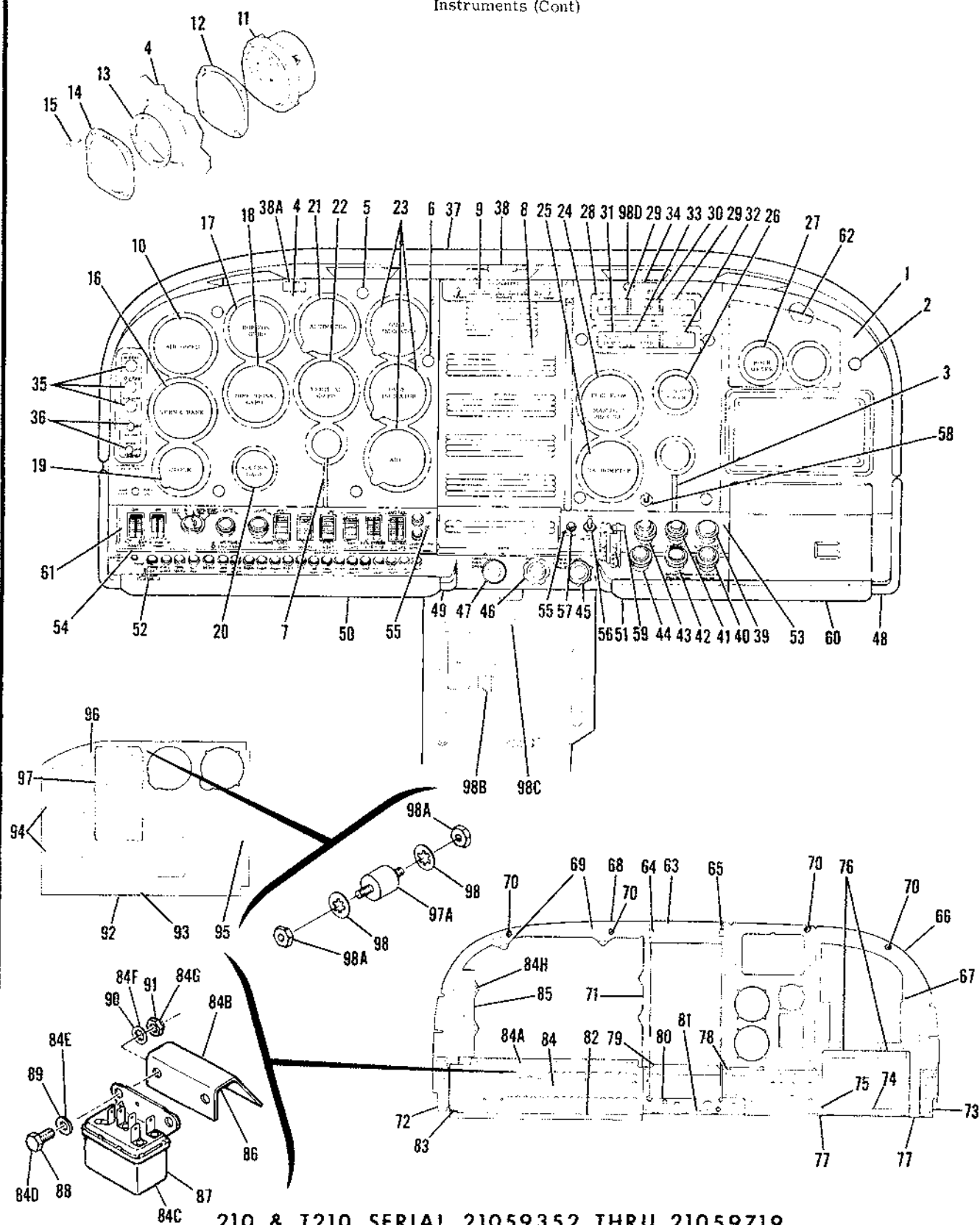
Figure 58A. Instrument Panel Equipment Installation
