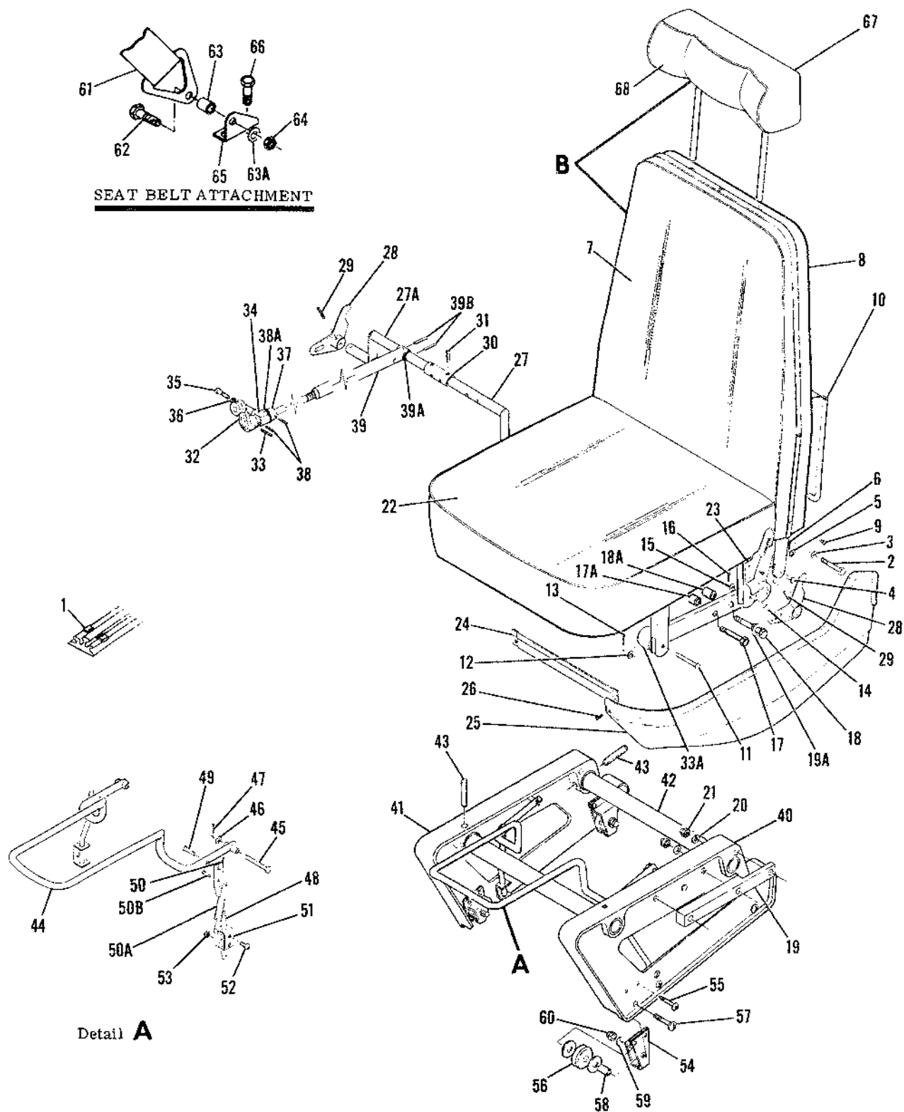
Figure 53A. Articulating Recline Copilot Seat Installation (Sheet 1 of 2)
