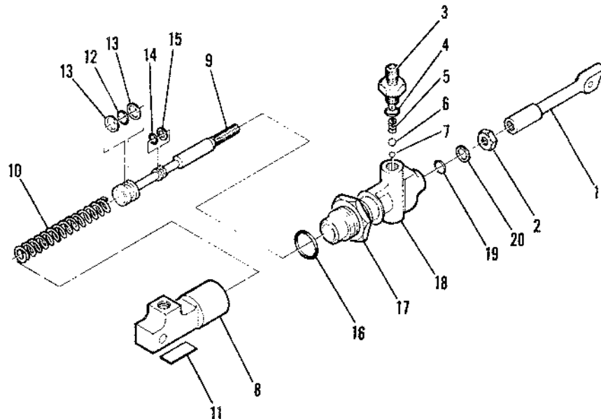
Figure 130A. Downlock Actuator Assembly
