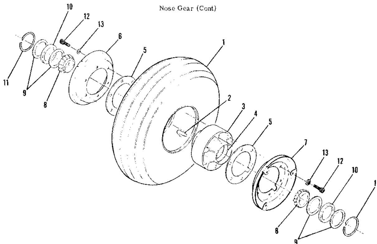
Figure 35B. Nose Gear Wheel & Tire Assembly - McCauley
