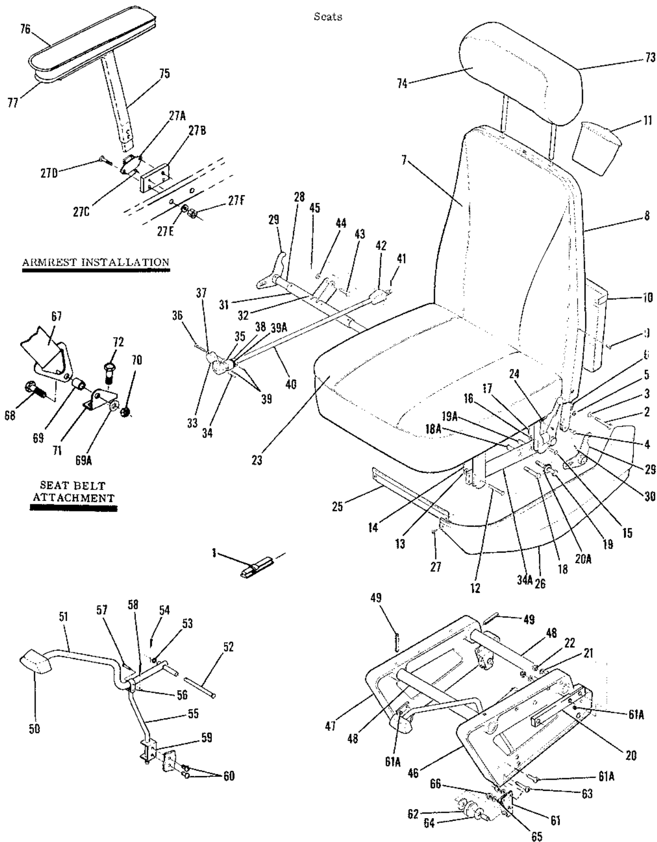
Figure 53. Articulating Recline Co-pilot Seat Installation
