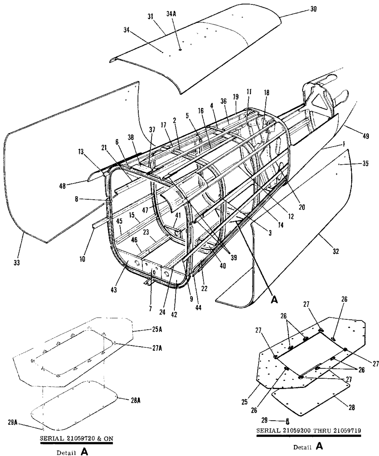
Figure 29. Tailcone Installation
