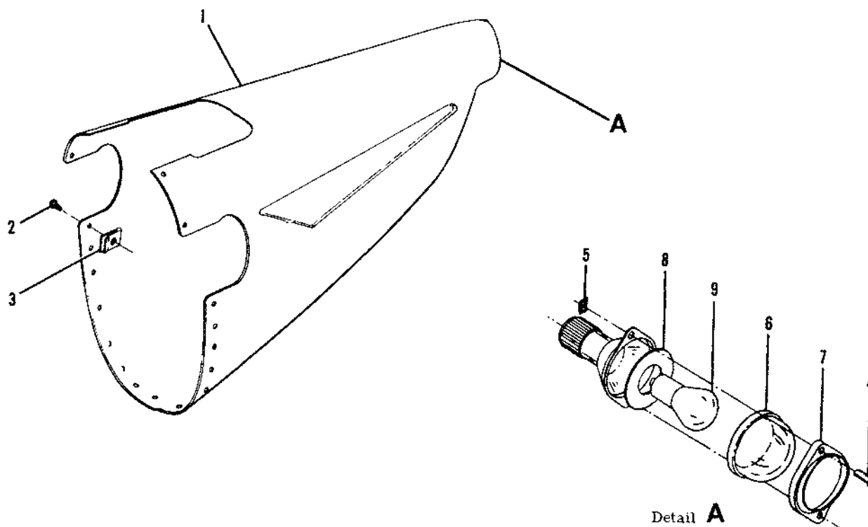
Fuselage (Cont)
