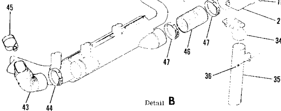
Figure 91. Heater & Defroster Installation
