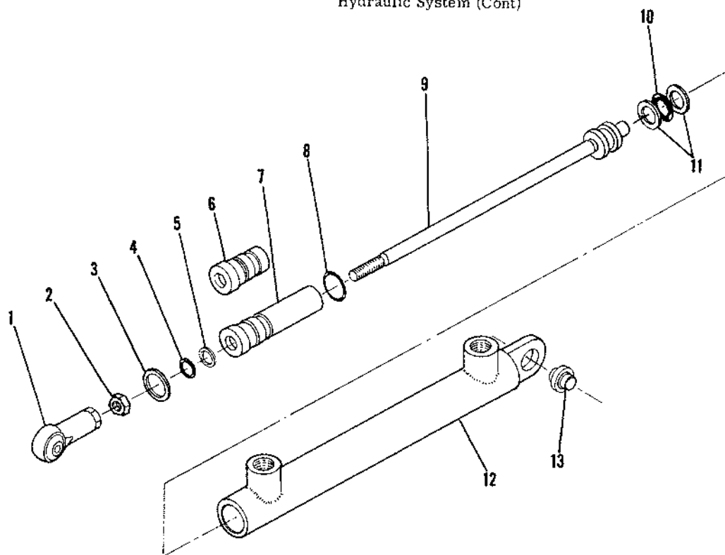
Figure 128. Main Gear Doors &amp; Nose Gear Doors Actuator Assembly
