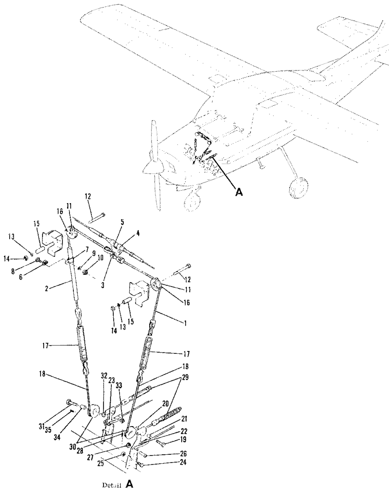
Figure 106. Alleron, Rudder Interconnect System
