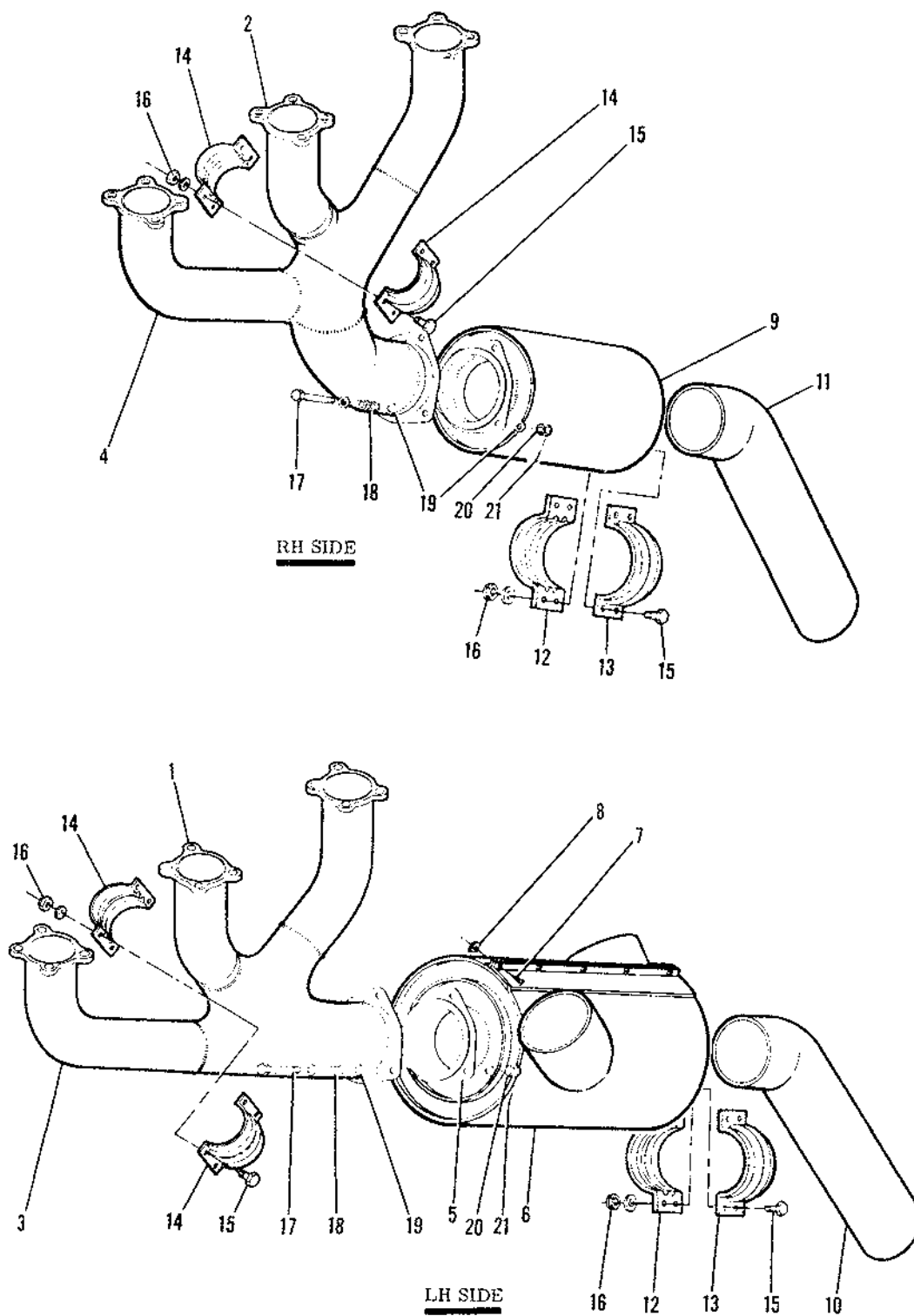
210 SERIAL 21059200 & ON Figure 83. Exhaust Stack Assembly
