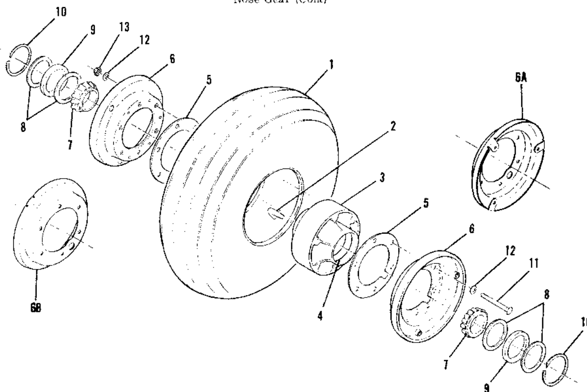
Figure 35A. Nose Gear Wheel &amp; Tire Assembly - McCauley
