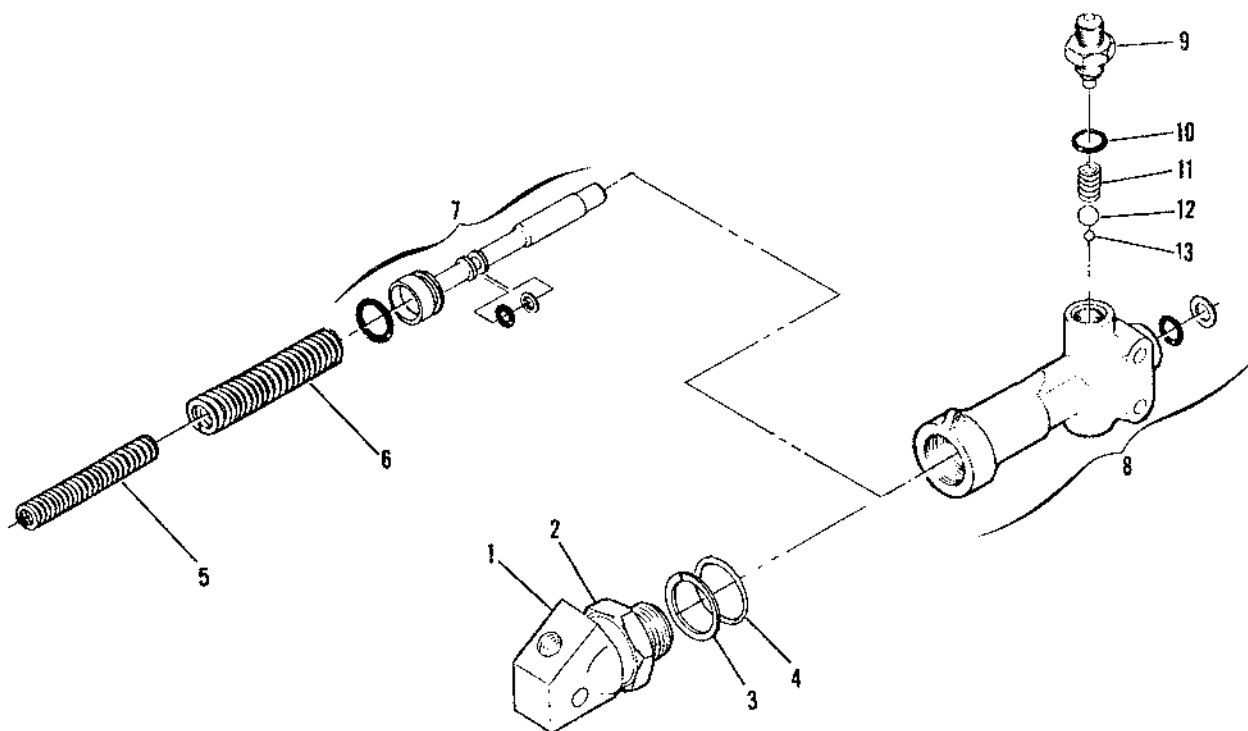
Figure 130. Downlock Actuator Assembly
