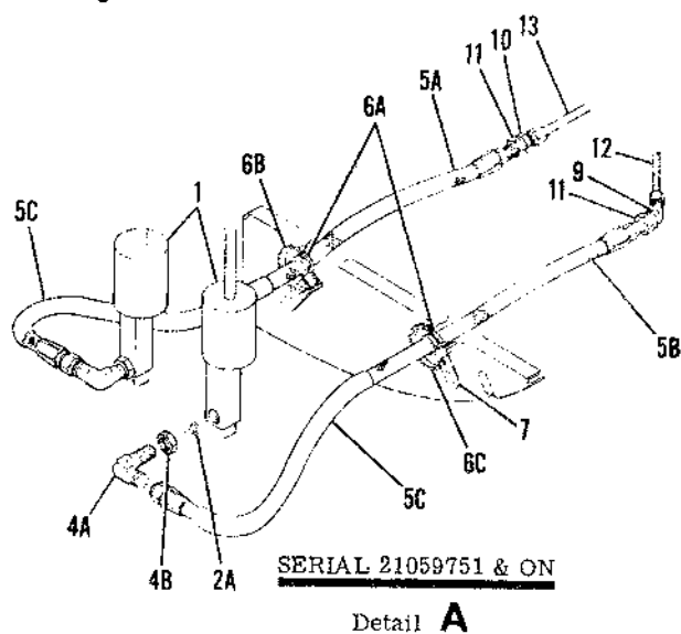
Figure 92. Brake System Installation
