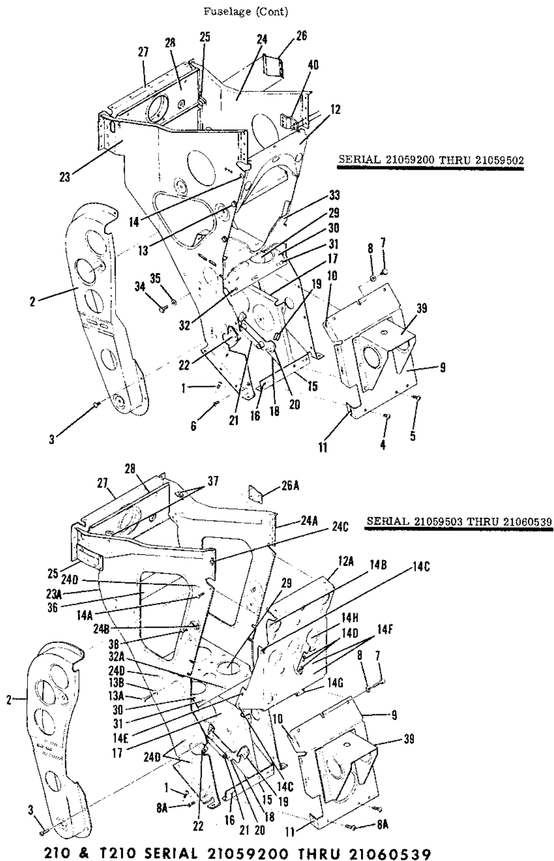
Figure 20. Pedestal Installation
