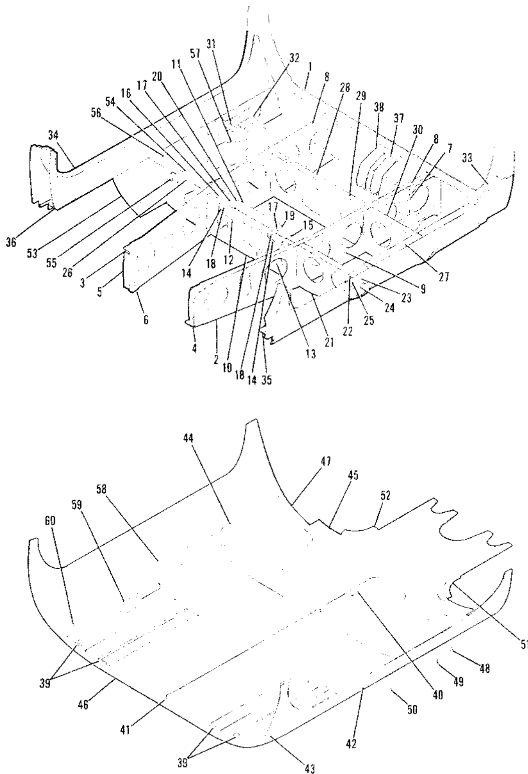
Figure 21B. Fuselage Belly Section Components
