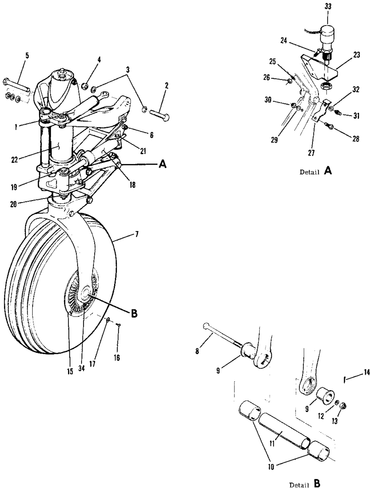
Figure 32. Nose Gear Installation
