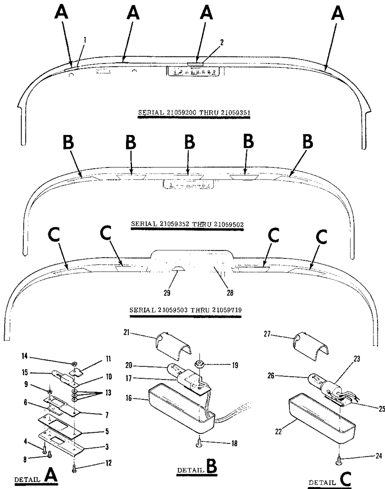
Figure 137. Instrument Panel Brow Lights Installation
