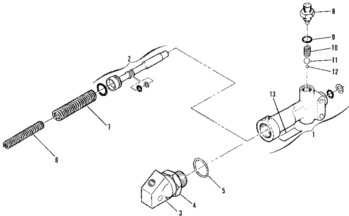
Figure 131A. Nose Gear Unlock &amp; Sequence Actuator Assembly
