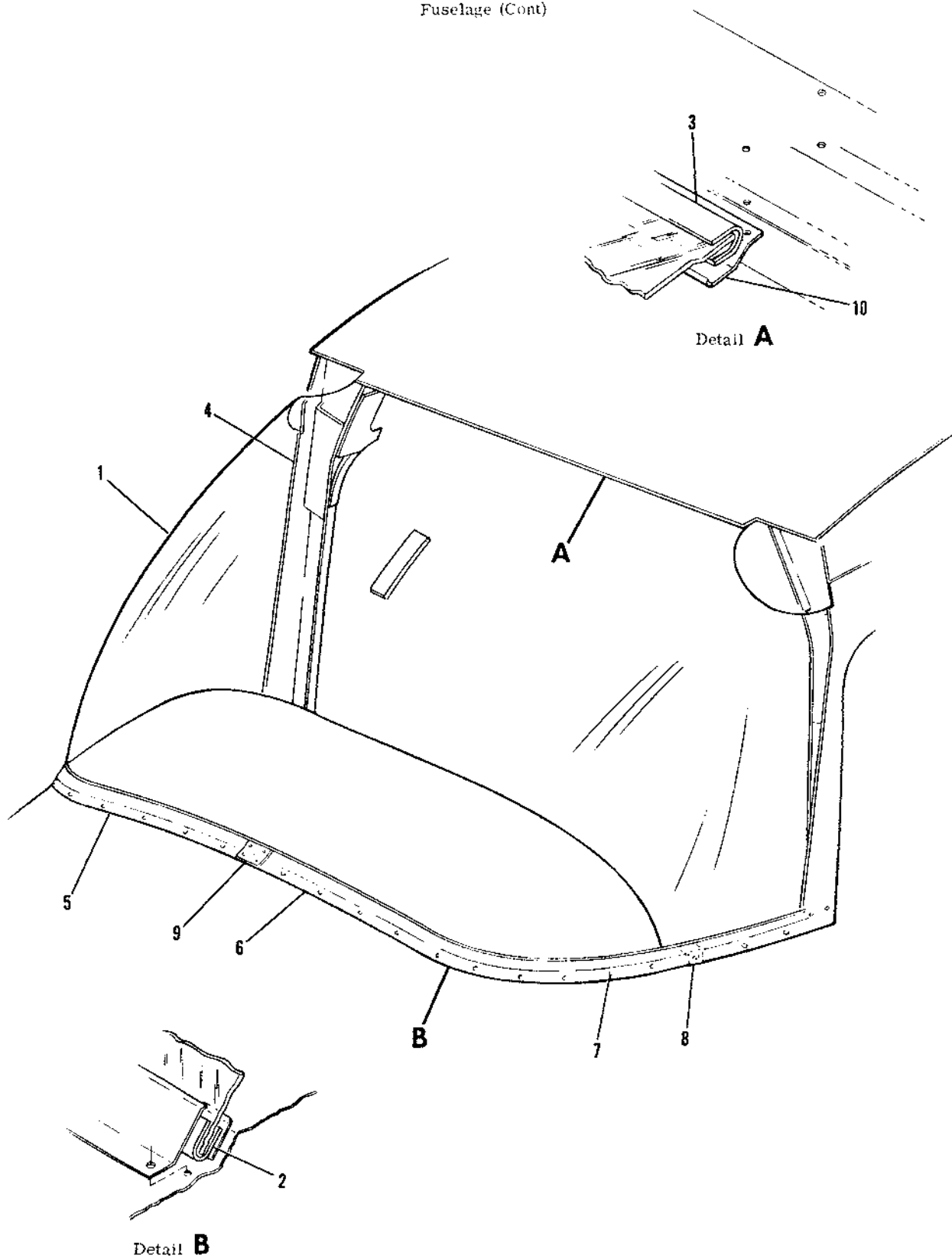
Figure 28. Windshield Installation
