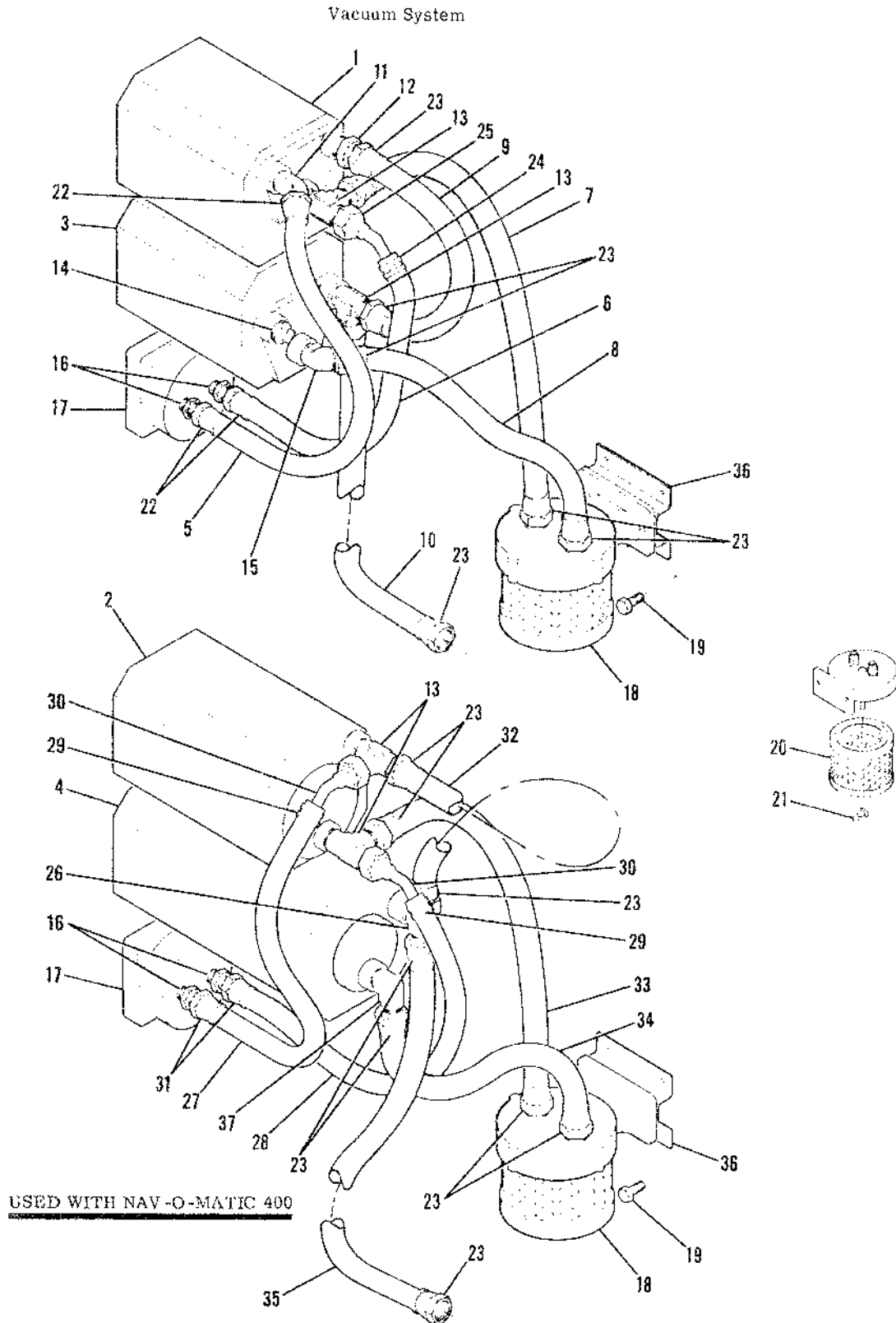
Figure 114. Gyros Installation - Engine Driven
