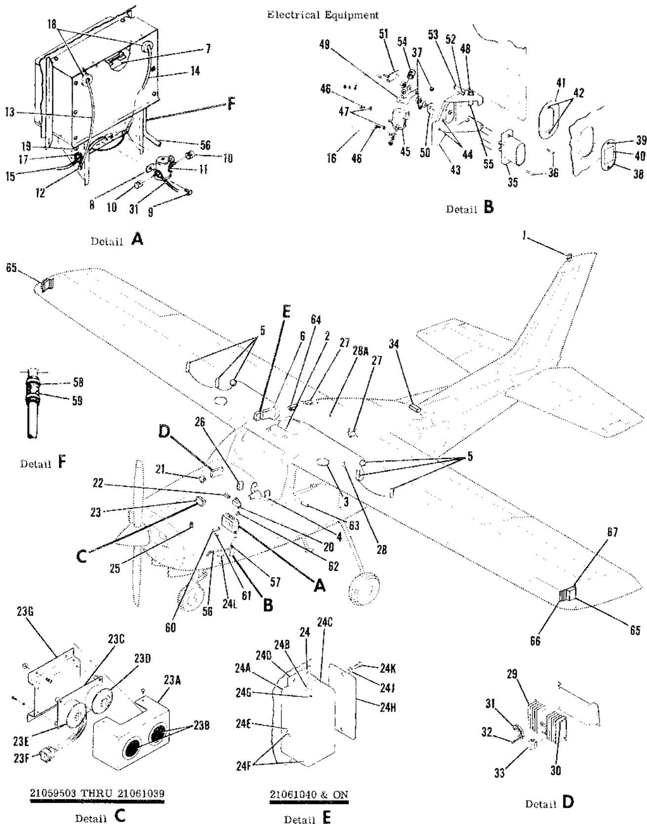
Figure 135. Electrical Equipment Installation
