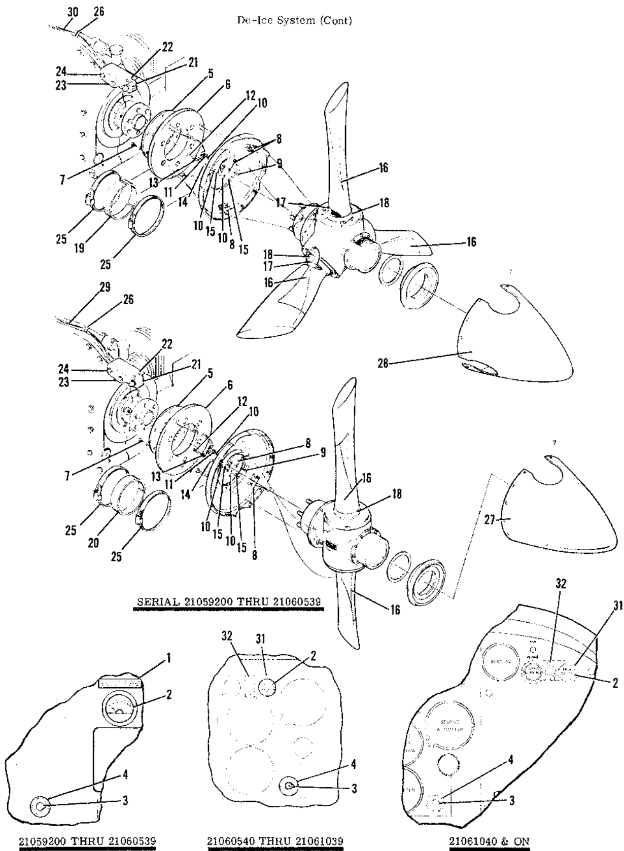
Figure 133. Propeller De-Ice System Installation
