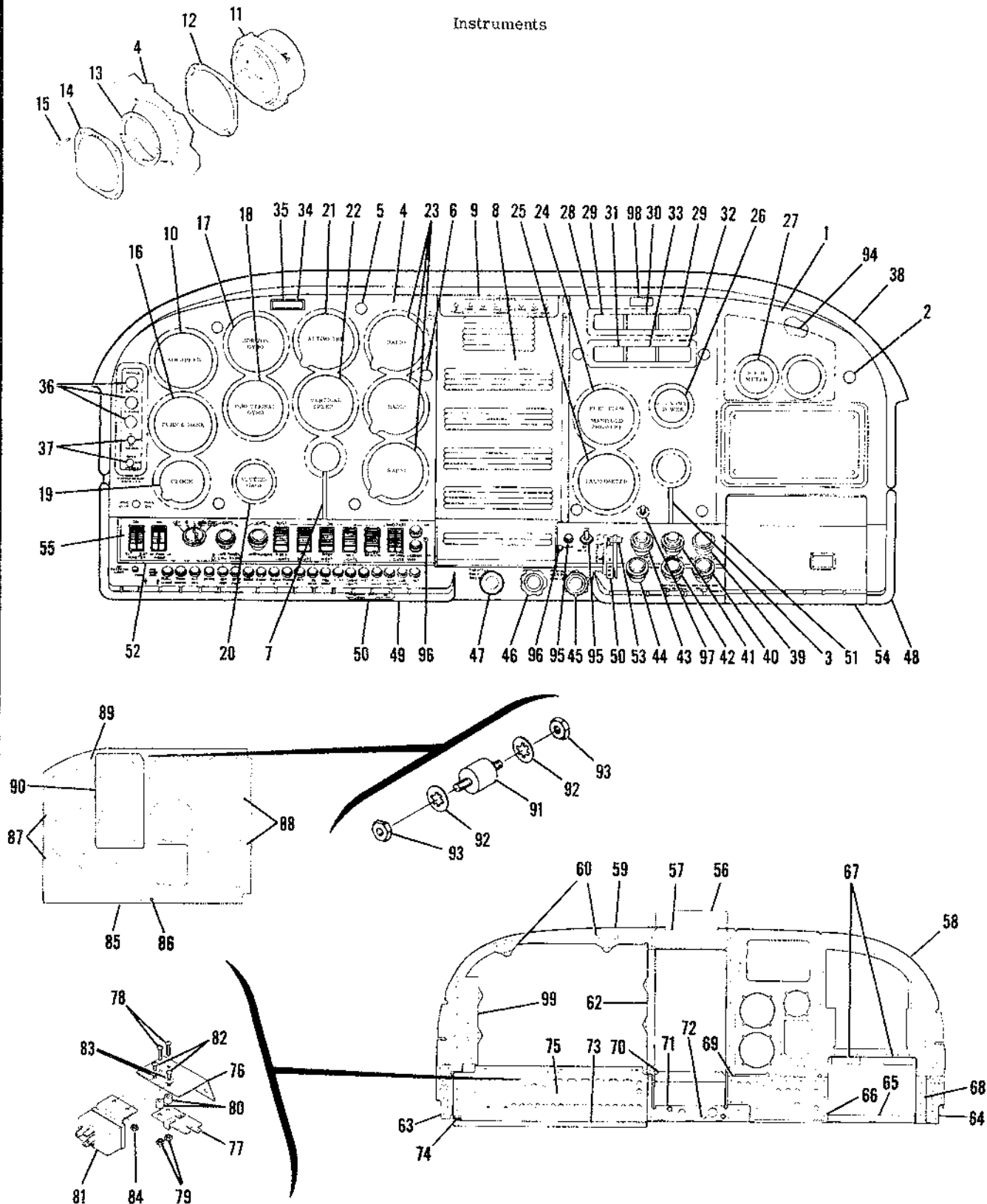
Figure 58. Instrument Panel Equipment Installation
