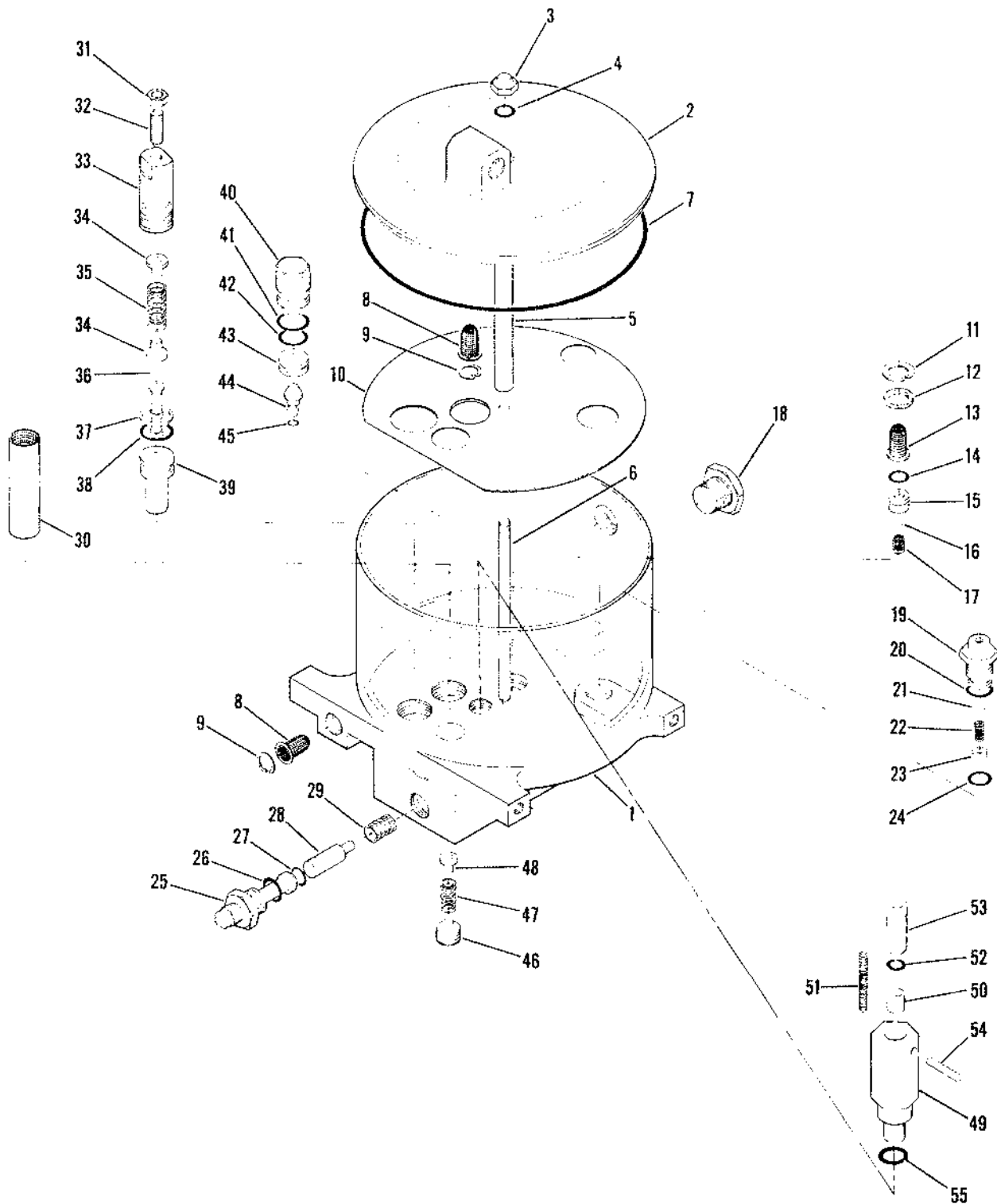
Figure 118. Hydraulic Power Pack Body Assembly
