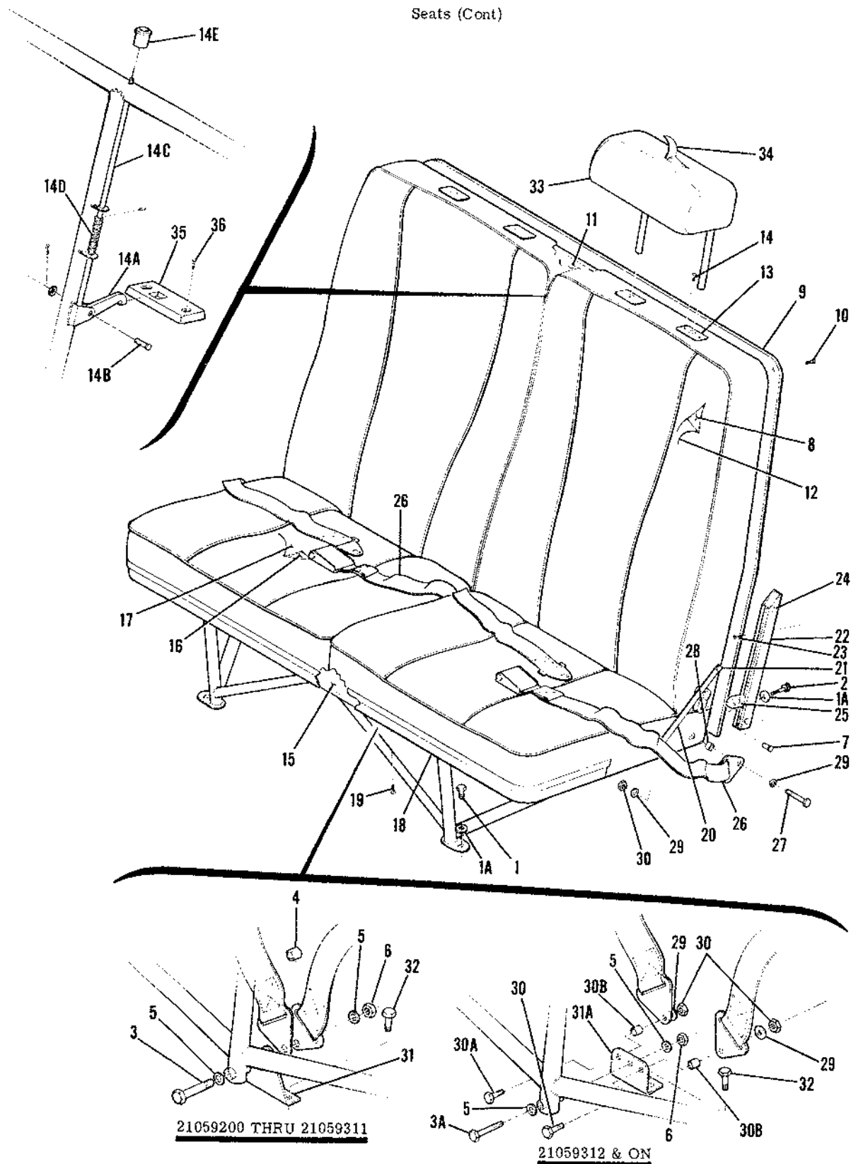
Figure 57. Bench Seat Installation - 5th & 6th Place
