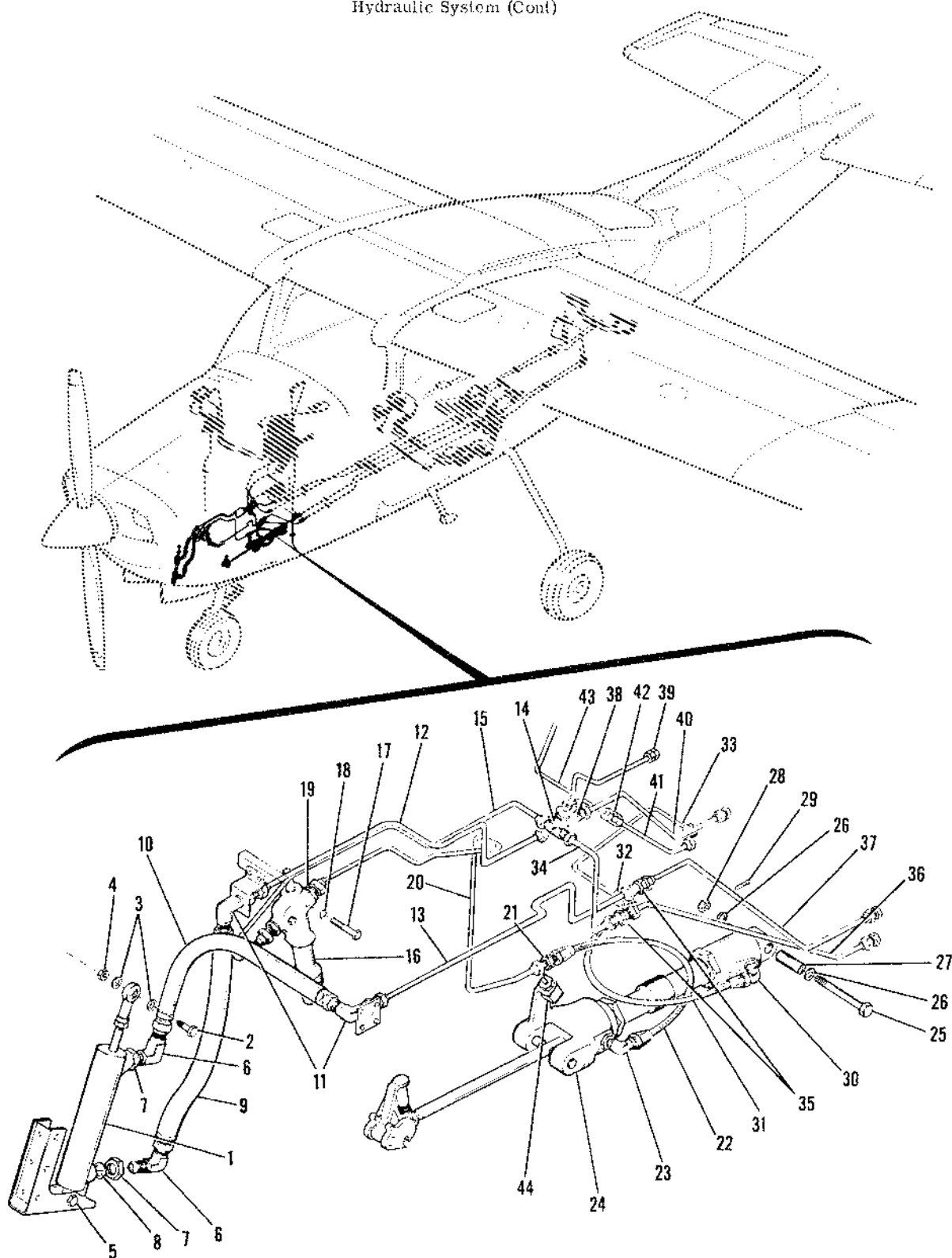
Figure 122. Nose Gear & Nose Gear Doors Hydraulic System Installation
