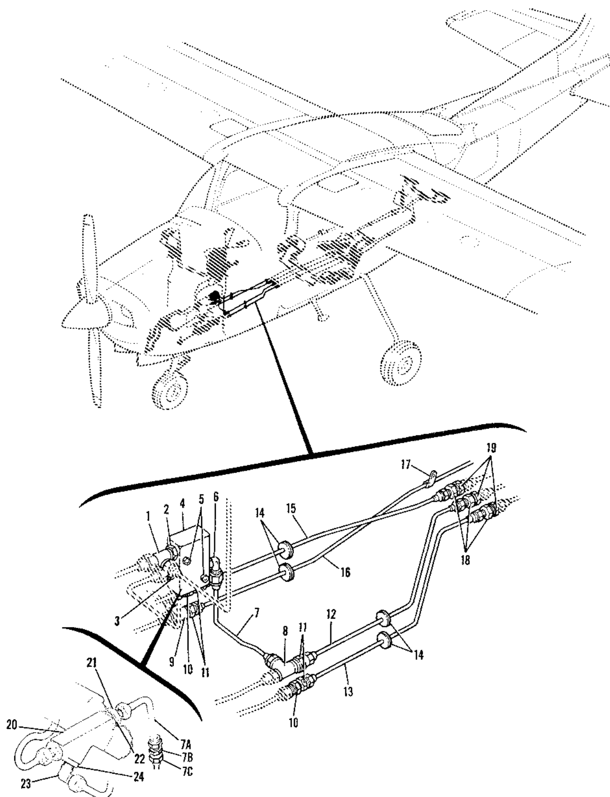
Figure 123. Hydraulic System Installation - Lock Out Valve to Sta. 44.00
