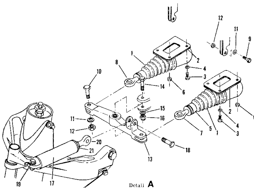
Figure 33. Nose Gear Steering System Installation
