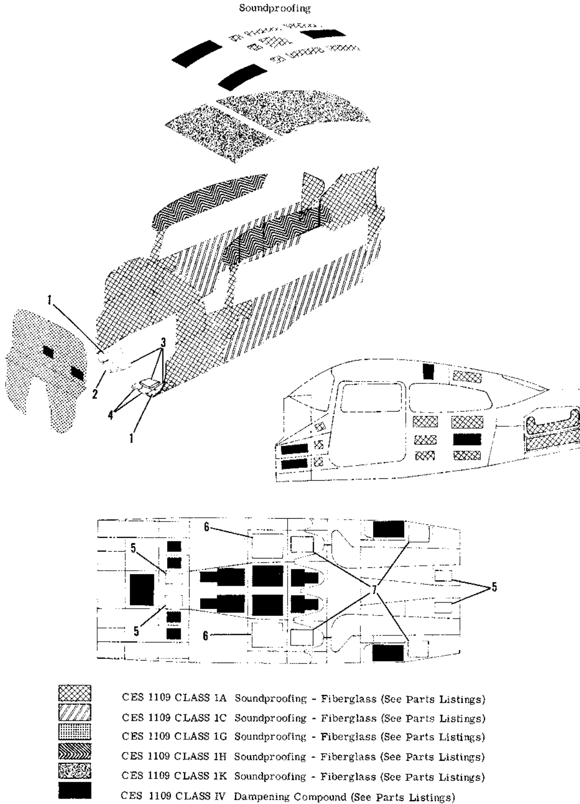
Figure 52. Cabin Soundproofing Installation
