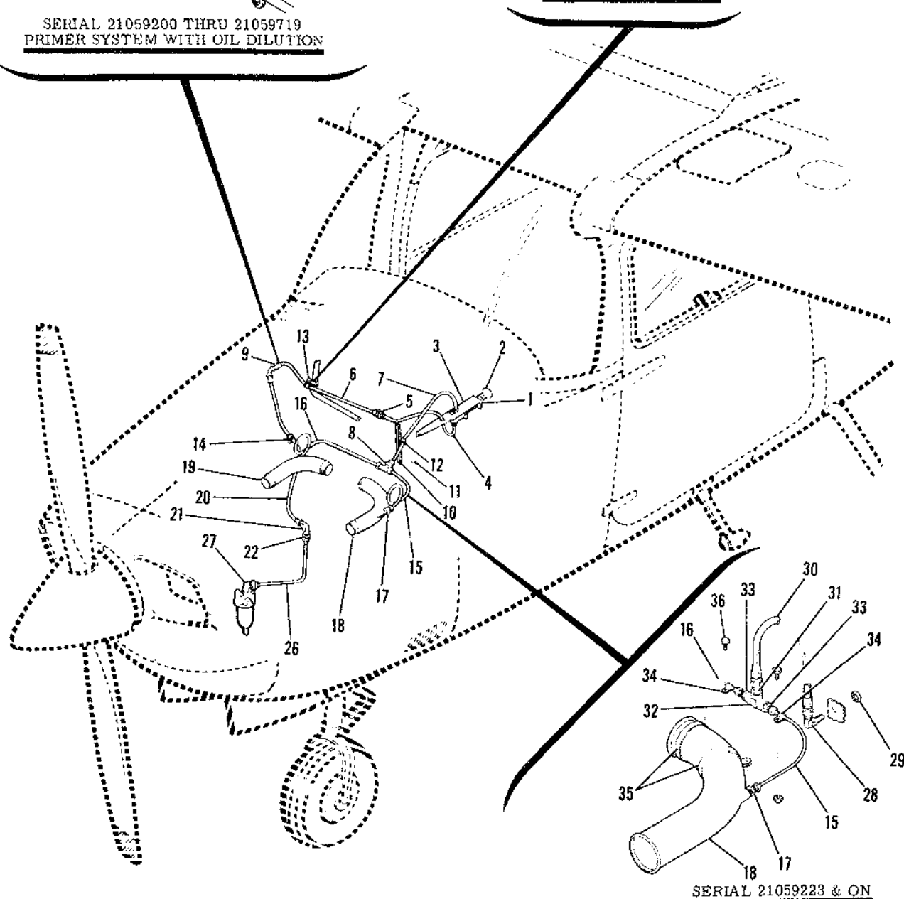
Figure 112. Engine Primer System Installation
