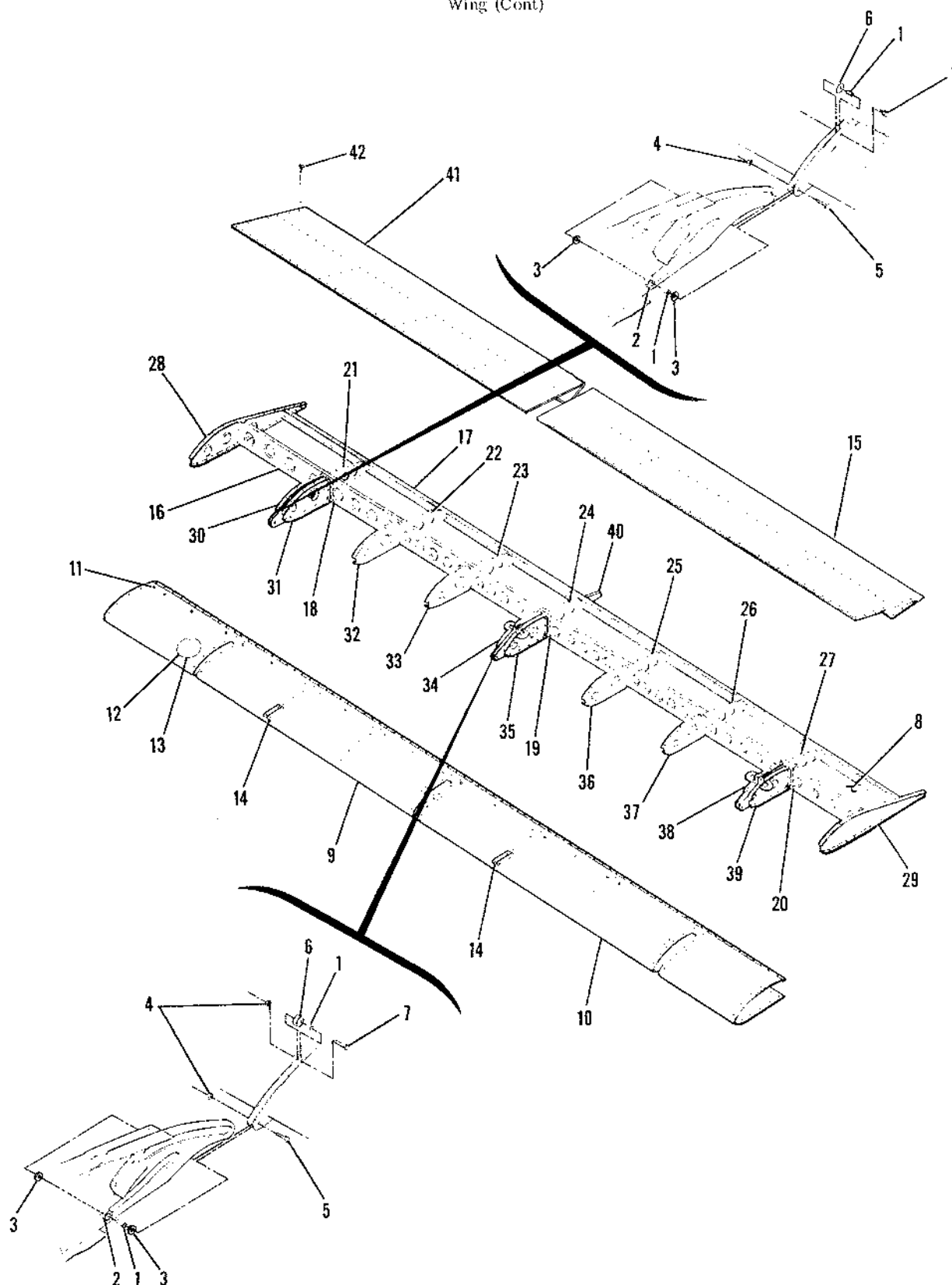
Figure 10. Flap Installation
