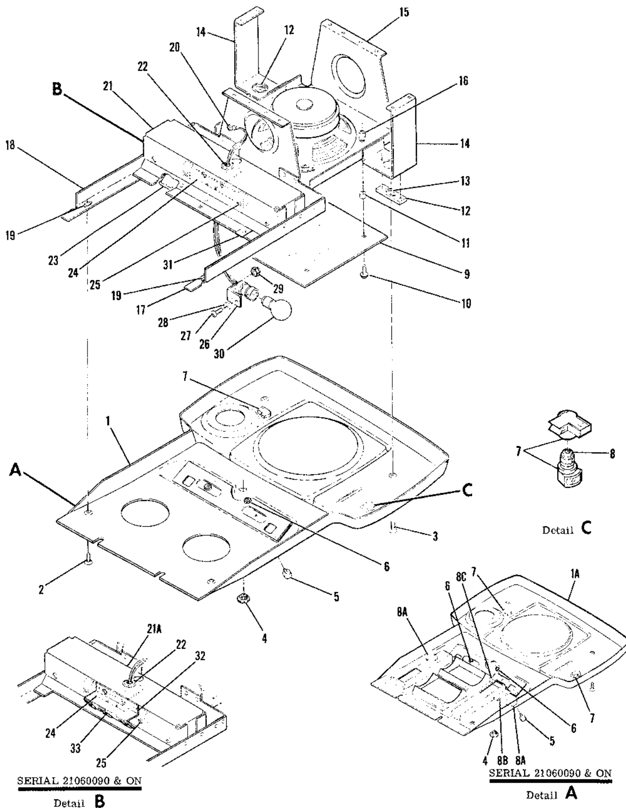
Figure 136. Instrument Panel Lights & Overhead Console Installation
