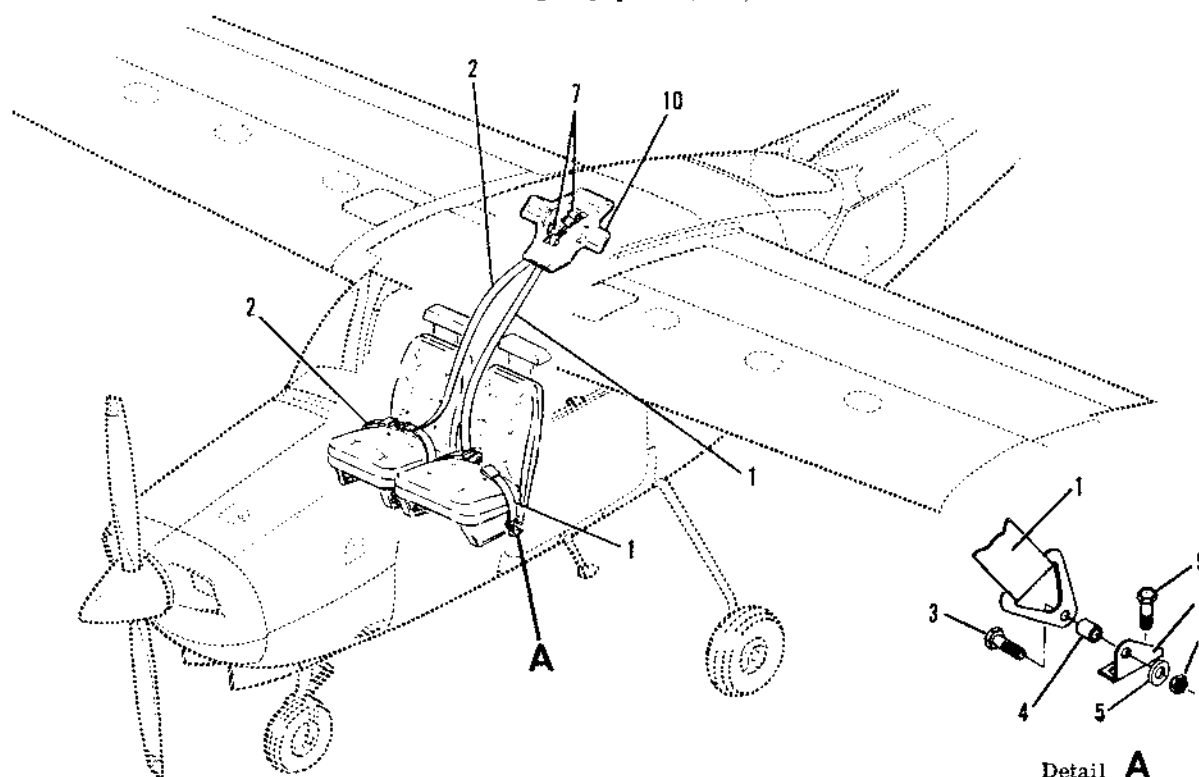
Figure 62B. Inertia Reel Seat Belt &amp; Shoulder Harness Installation
