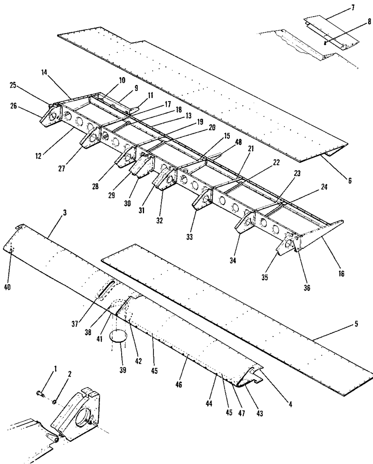
Figure 9. Aileron Installation
