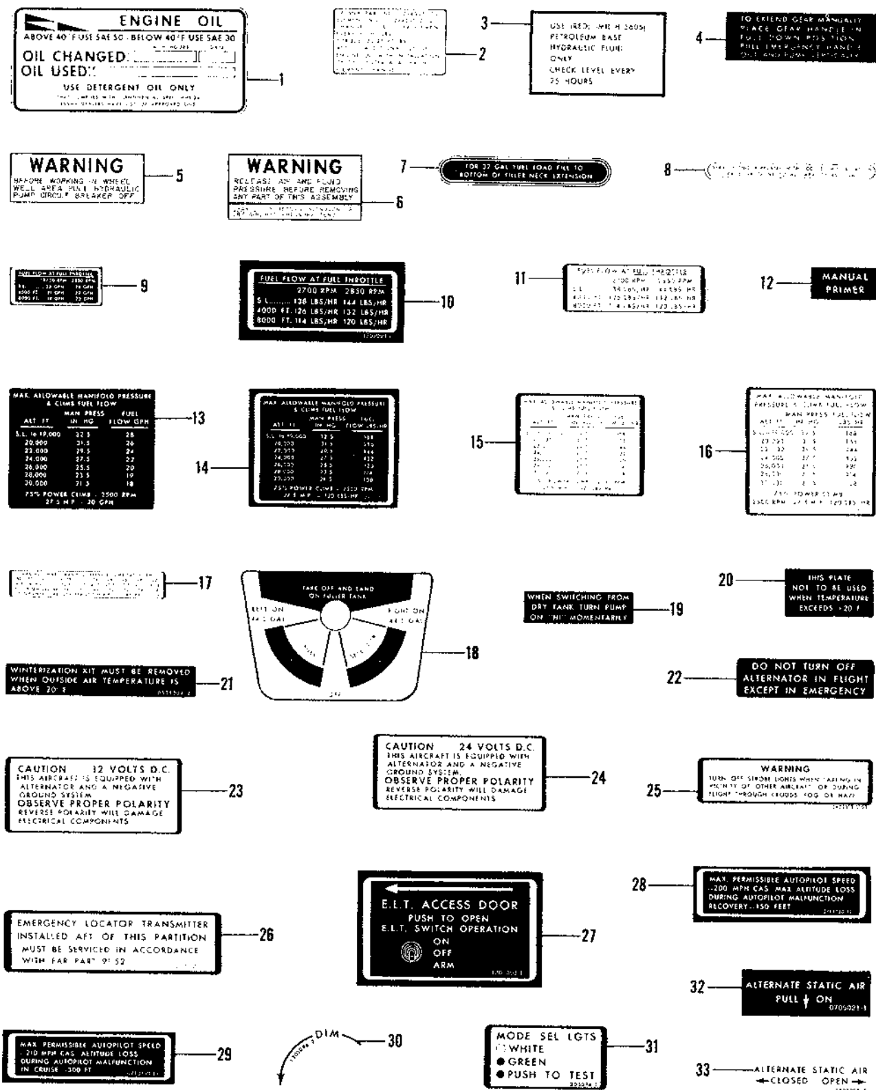
Figure 2. (Sheet 3) Nameplates, Placards & Exterior Markings Installation
