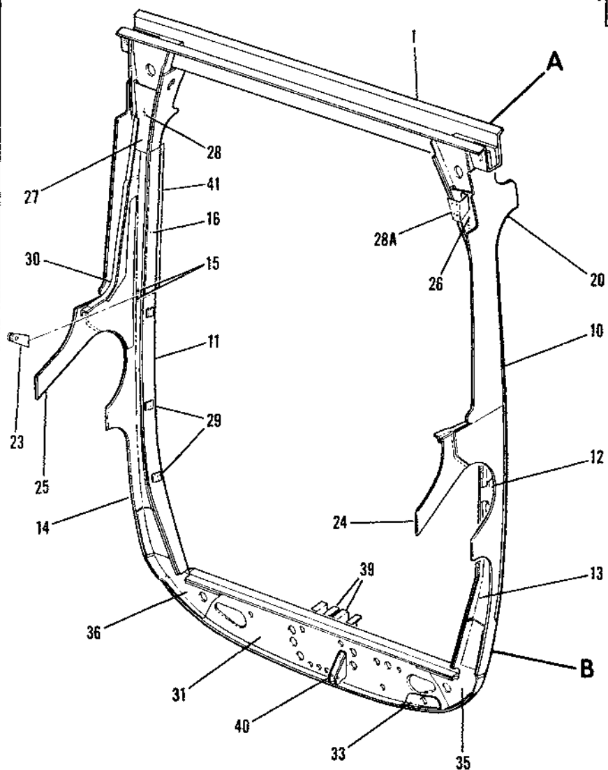
Figure 18. Front Door Post & Bulkhead Assembly
