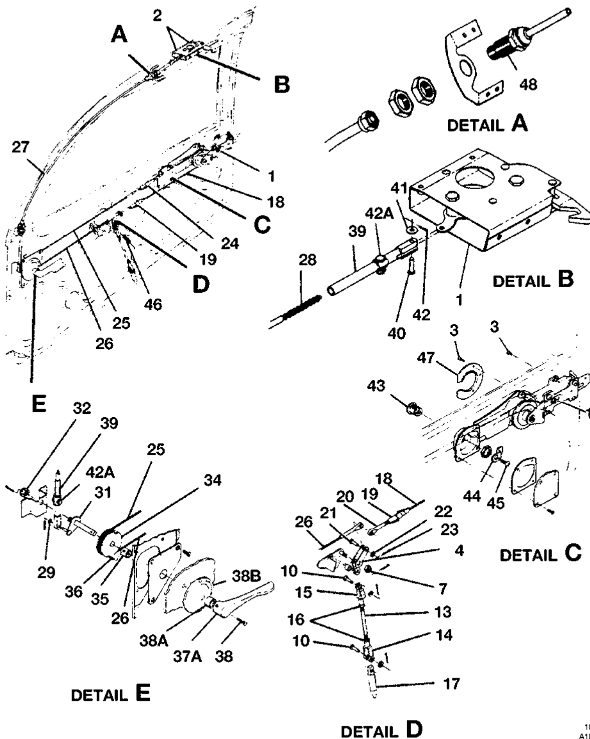
CABIN DOOR LATCH MECHANISM INSTALLATION FIGURE 02 (SHEET 1)
