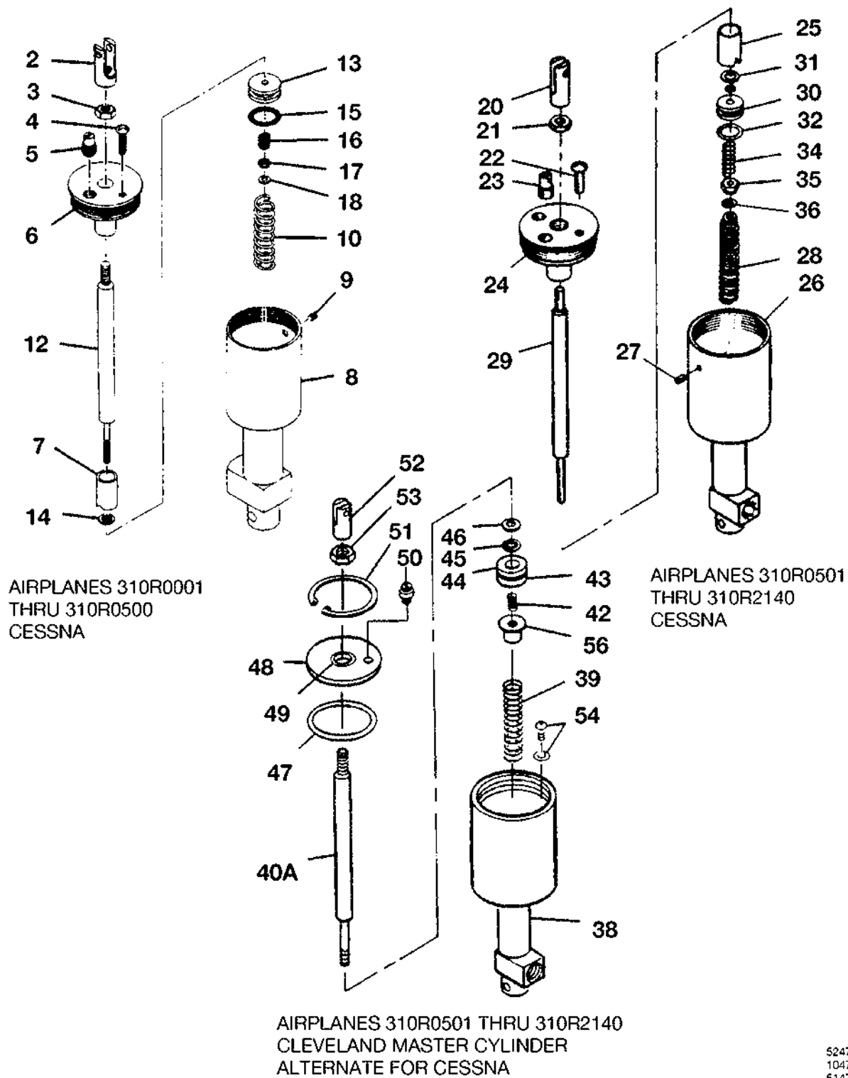
MASTER CYLINDER - BRAKE FIGURE 02 (SHEET 1)
