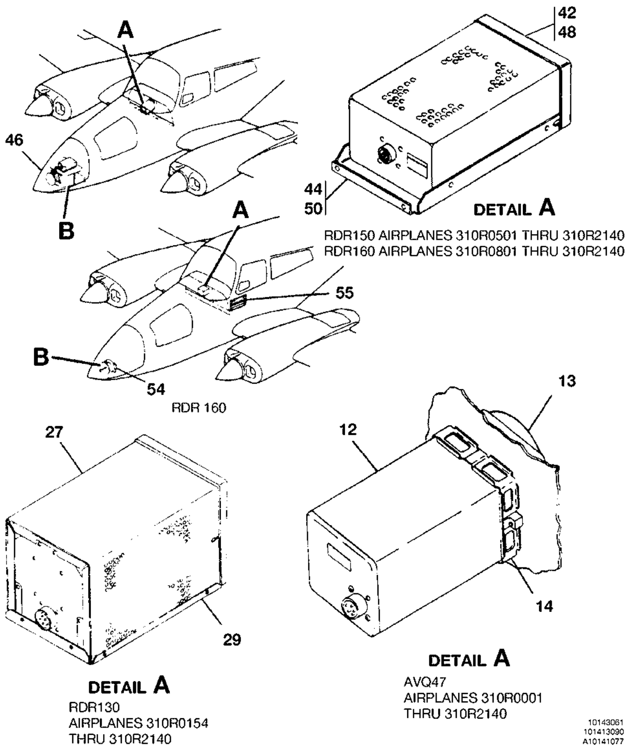
WEATHER RADAR FIGURE 01 (SHEET 1)
