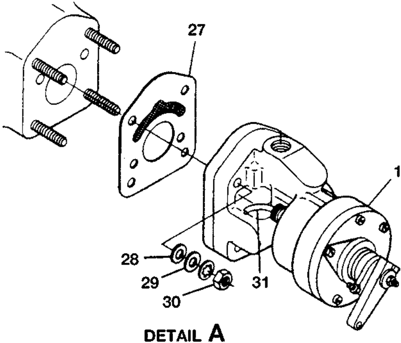
PROPELLER GOVERNOR INSTALLATION FIGURE 01 (SHEET 1)
