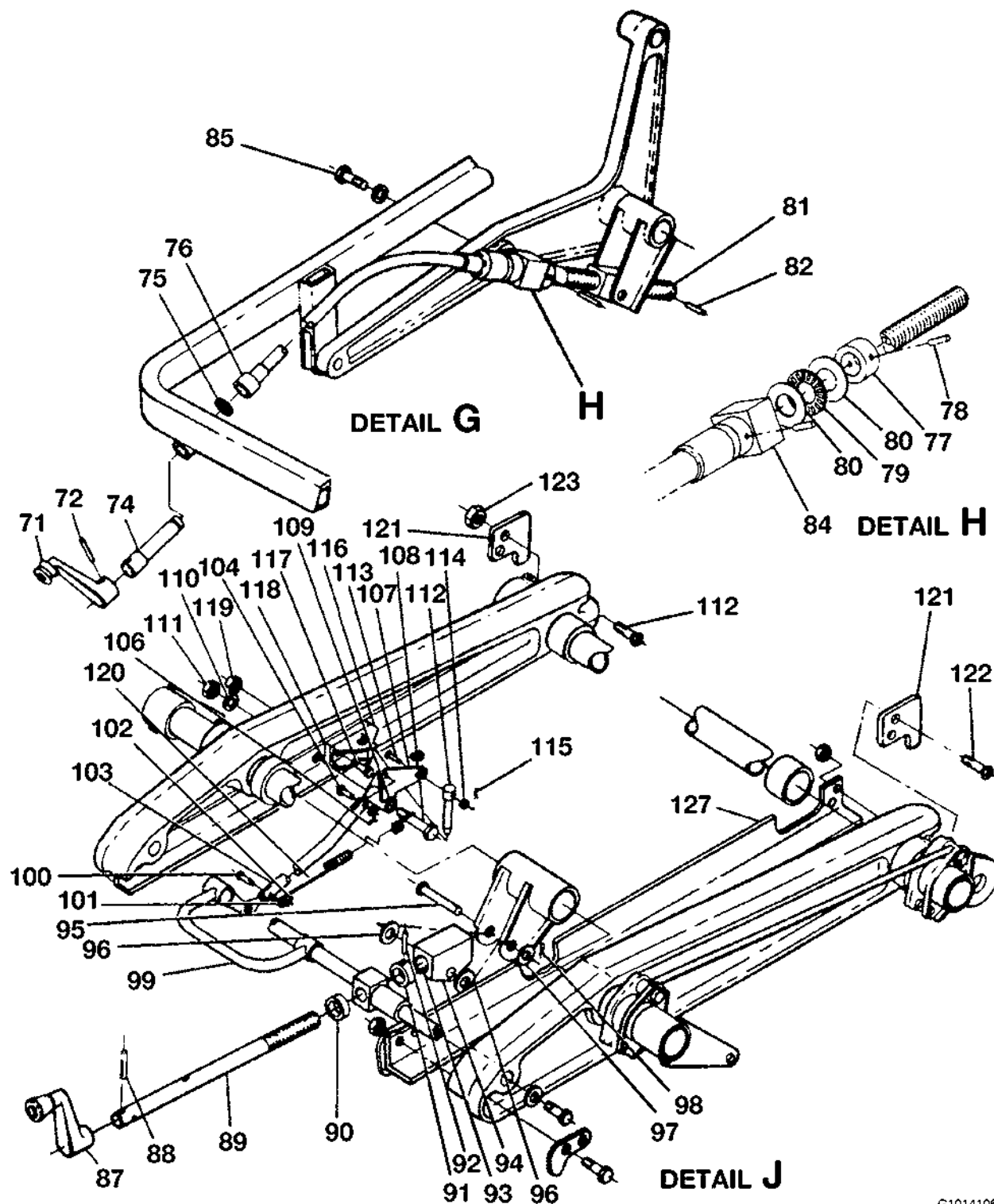
PILOT AND COPILOT MANUALLY ADJUSTABLE SEAT INSTALLATION FIGURE 02 (SHEET 3)
