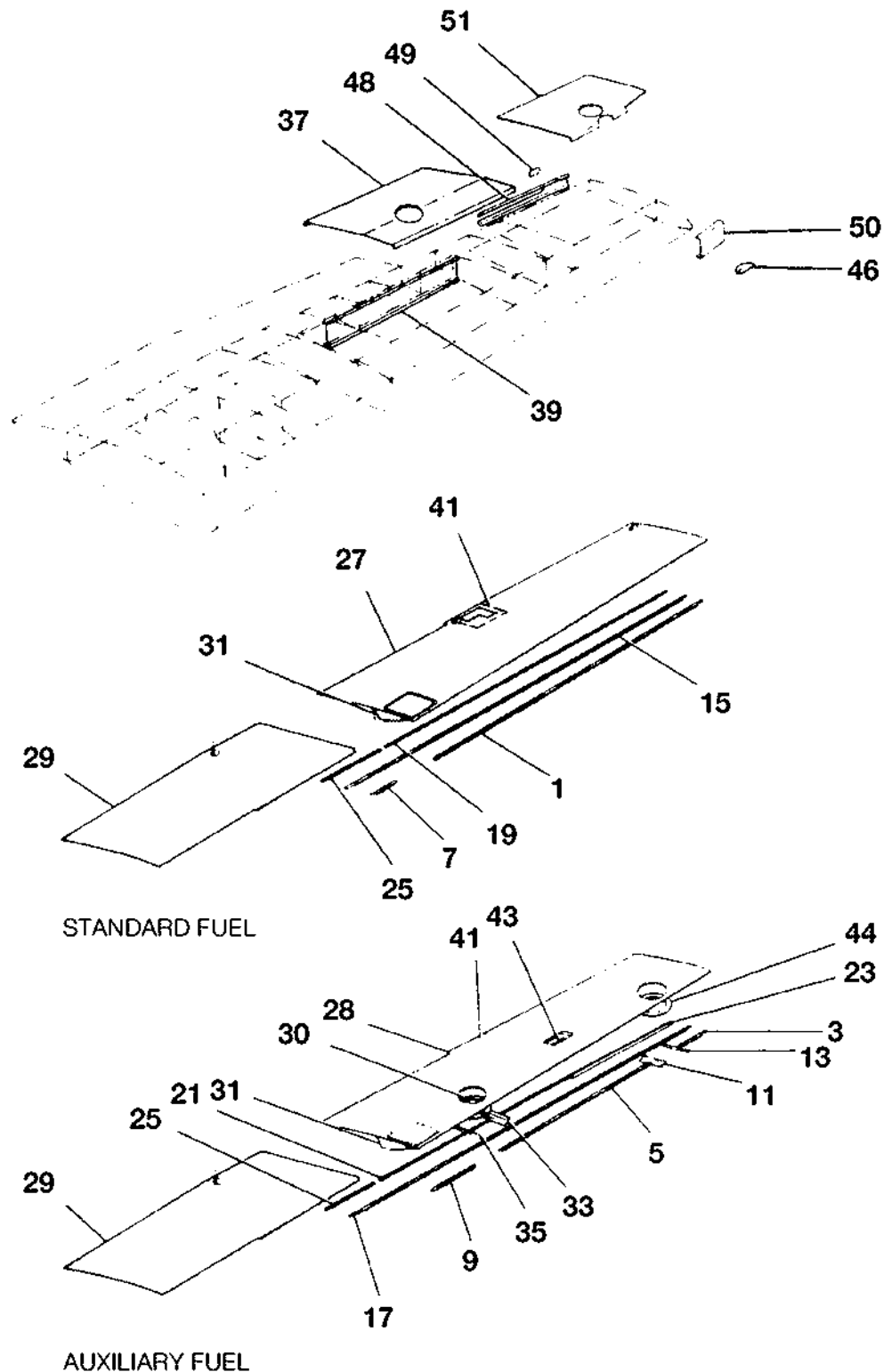
WING UPPER INTERSPAR SKINS AND STRINGERS INSTALLATION FIGURE 04 (SHEET 1)
