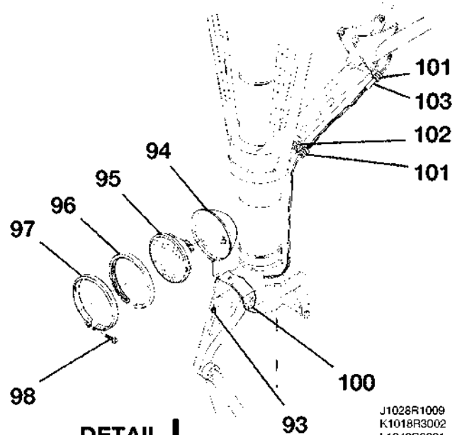
EXTERIOR LIGHTING INSTALLATION FIGURE 01 (SHEET 3)
