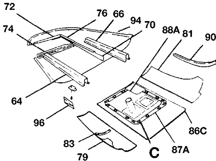
DETAIL B AIRPLANES 310R0501 THRU 310R2140
