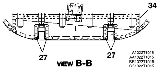
WING SPAR STRAP FIGURE 08 (SHEET 1)
