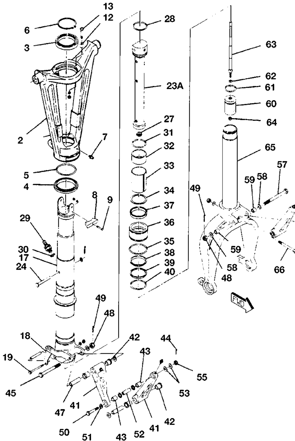
NOSE GEAR STRUT ASSEMBLY FIGURE 02 (SHEET 1)
