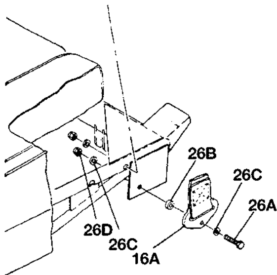
DETAIL B AIRPLANES 310R0501 THRU 310R2140
