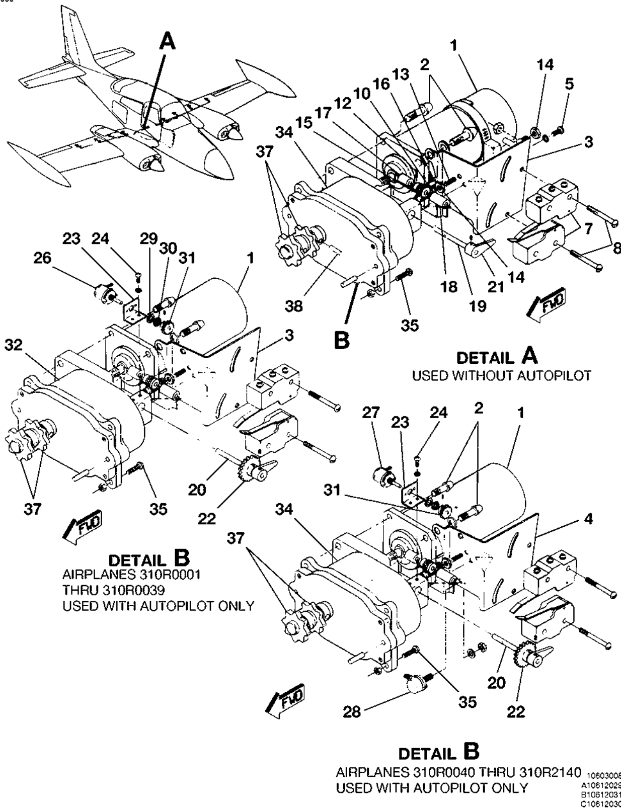
FLAP ACTUATOR AND REDUCTION UNIT INSTALLATION FIGURE 04 (SHEET 1)
