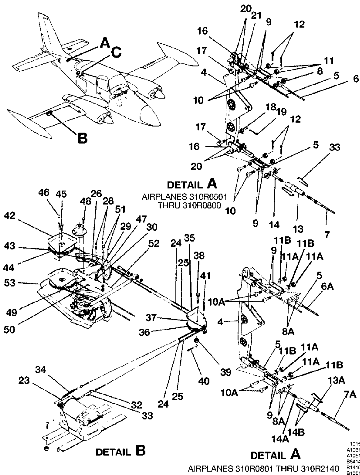
400B NAV-O-MATIC ACTUATOR CABLES INSTALLATION FIGURE 02 (SHEET 1)
