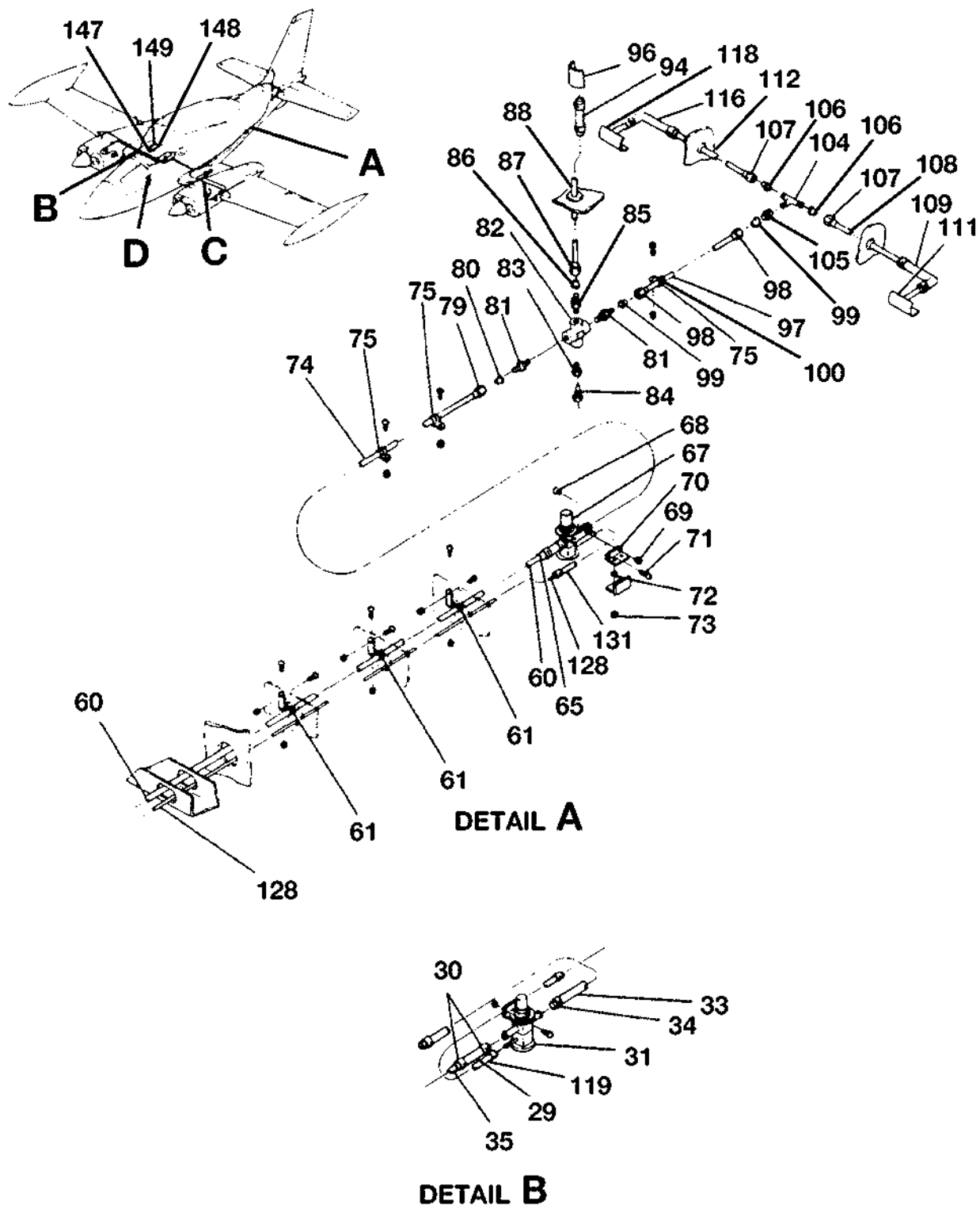
SURFACE DEICE SYSTEM FIGURE 02 (SHEET 1)
