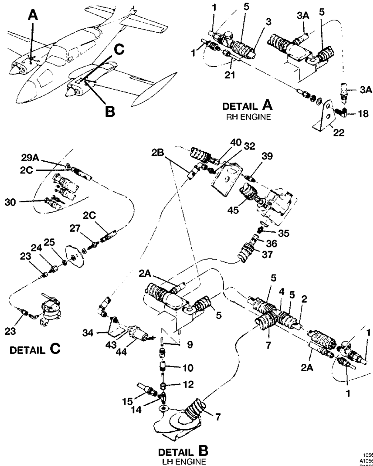
ENGINE COMPARTMENT FUEL SYSTEM COMPONENTS TURBO SYSTEM FIGURE 02 (SHEET 1)
