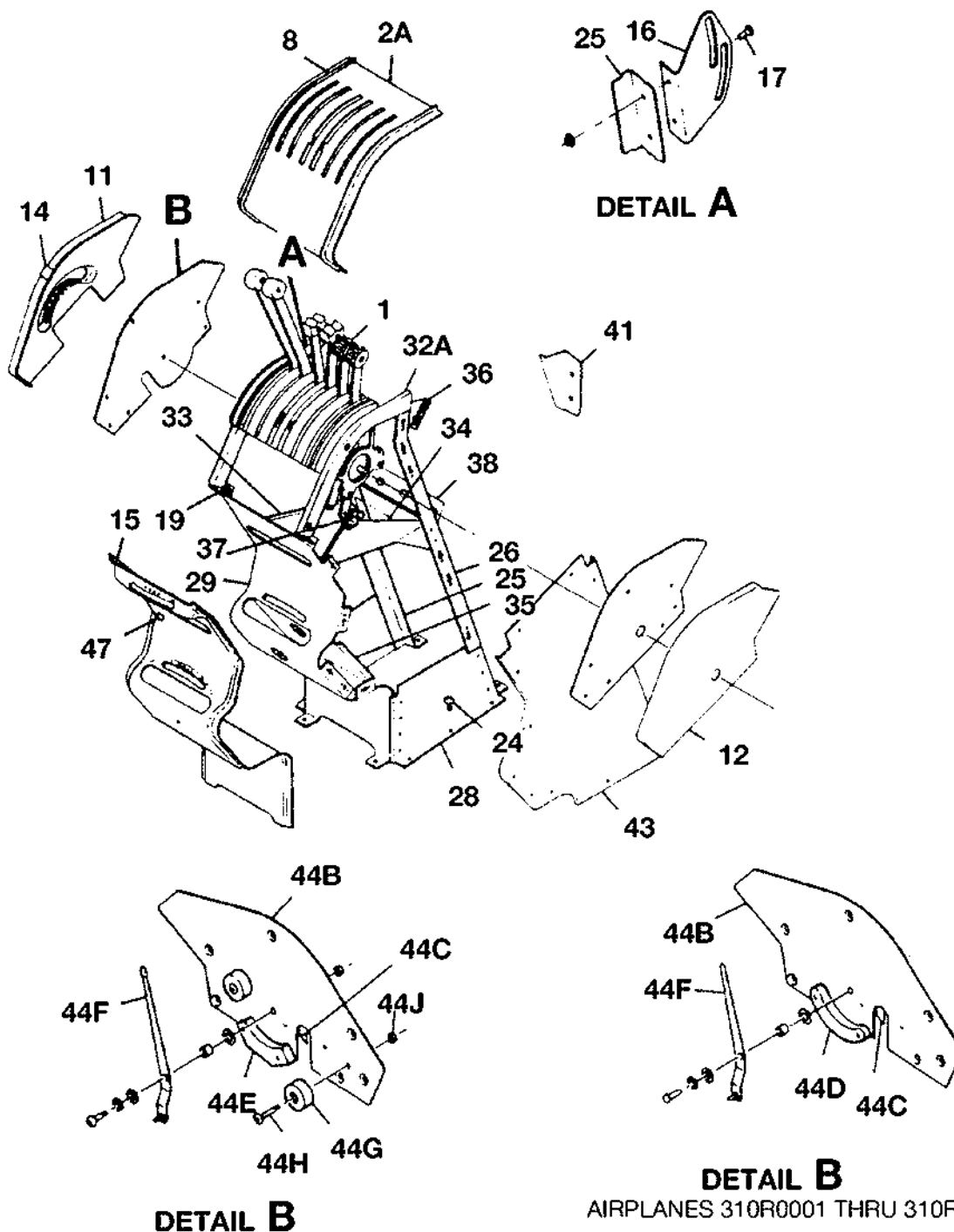
CONTROL PEDESTAL STRUCTURE INSTALLATION FIGURE 01 (SHEET 1)
