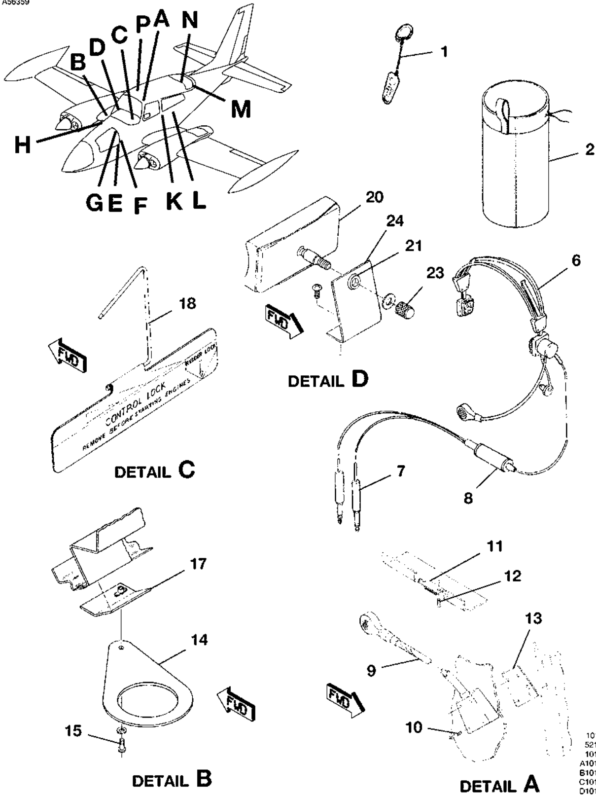
MISCELLANEOUS EQUIPMENT FIGURE 01 (SHEET 1)
