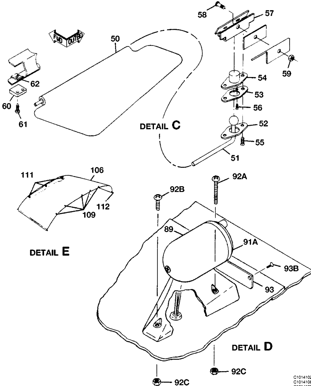
UPHOLSTERY TRIM INSTALLATION FIGURE 01 (SHEET 2)
