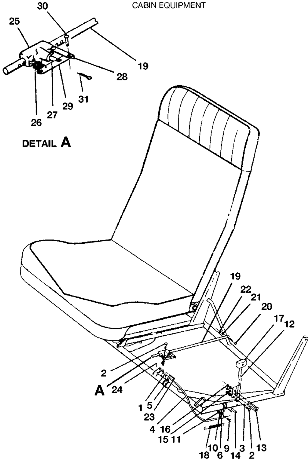
RECLINING ADJUSTMENT MECHANISM INSTALLATION FIGURE 02 (SHEET 1)
