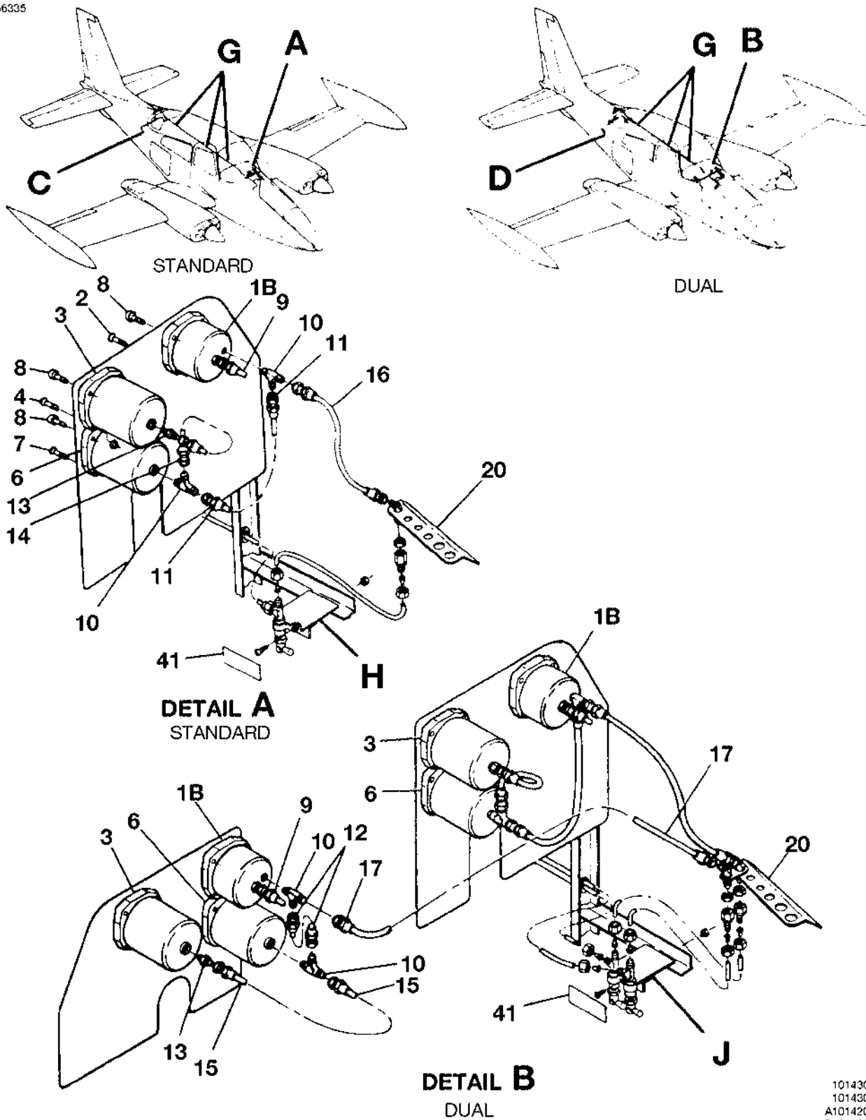
STATIC SYSTEM FIGURE 01 (SHEET 1)
