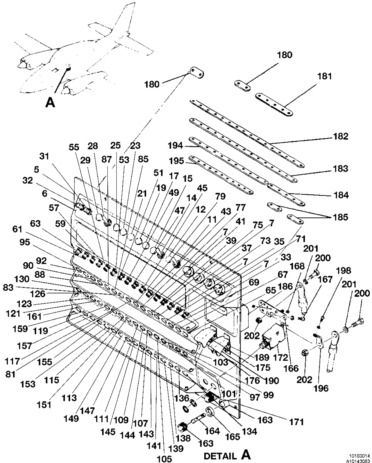
CIRCUIT BREAKER PANEL INSTALLATION FIGURE 03 (SHEET 1)
