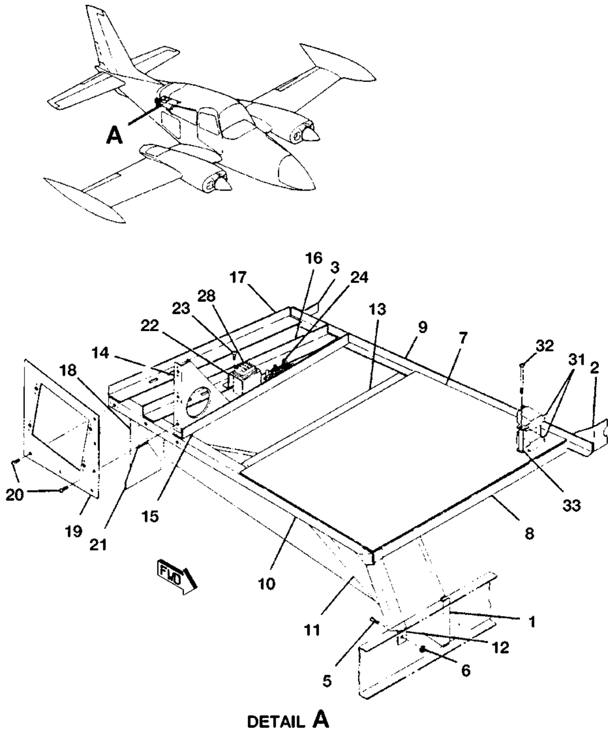
400A NAV-O-MATIC ACTUATOR SHELF INSTALLATION FIGURE 03 (SHEET 1)
