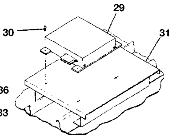
DETAIL C EXTERIOR LIGHTING INSTALLATION FIGURE 01 (SHEET 1)
