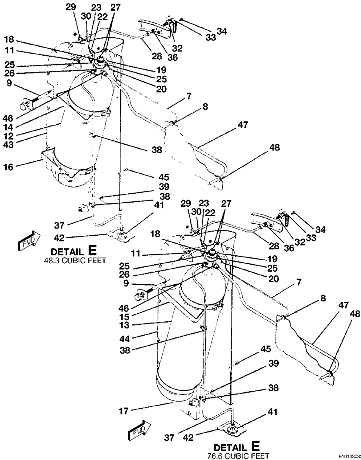
OXYGEN SYSTEM FIGURE 01 (SHEET 3)
