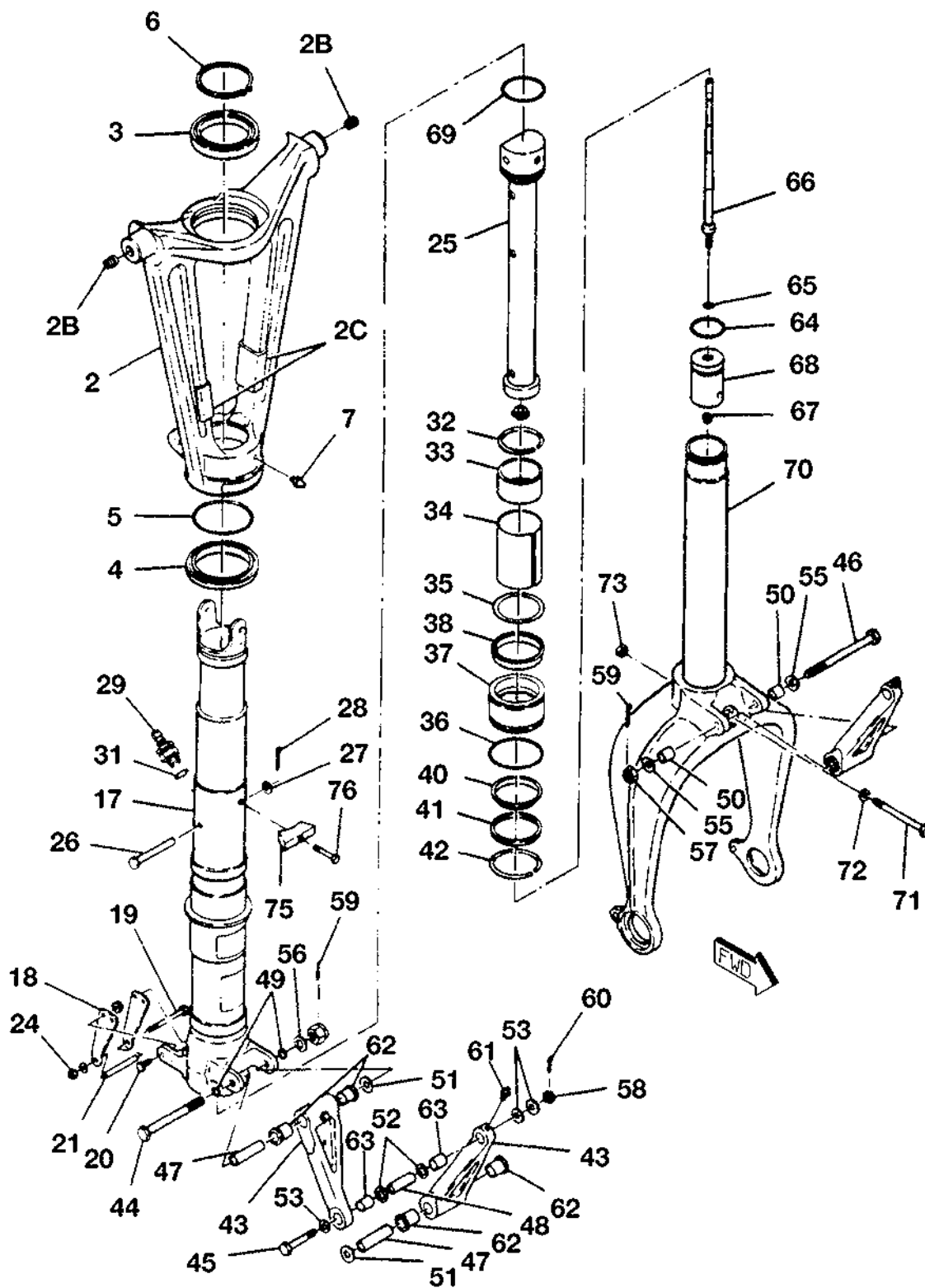
NOSE GEAR STRUT ASSEMBLY FIGURE 03 (SHEET 1)
