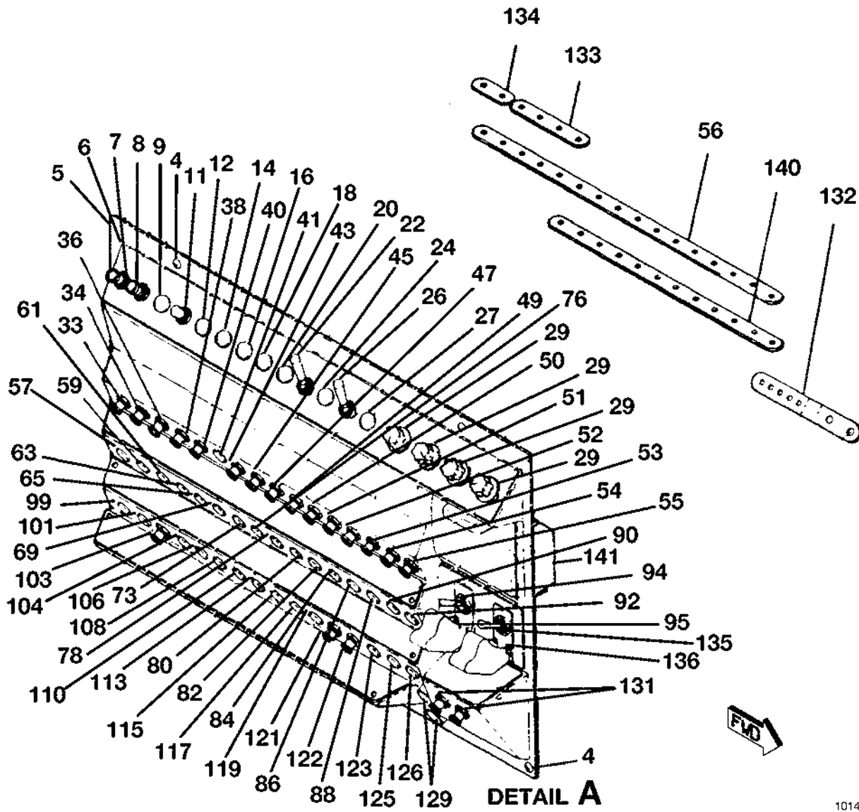
CIRCUIT BREAKER PANEL INSTALLATION FIGURE 02 (SHEET 1)
