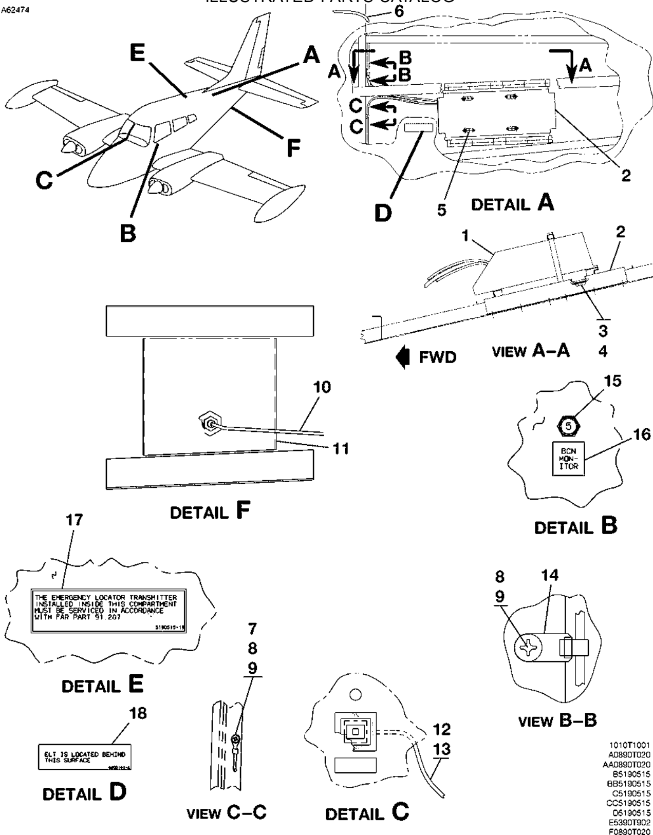
POINTER 3000-11 ELT INSTALLATION FIGURE 02 (SHEET 1)
