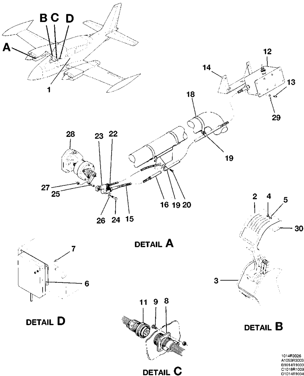
PROPELLER SYNCHRONIZER COMPONENTS FIGURE 03 (SHEET 1)
