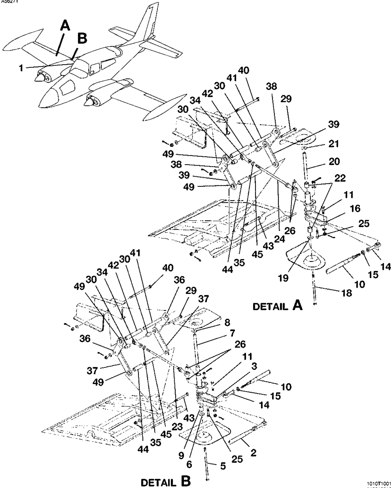
OUTBOARD FLAP CONTROL SYSTEM FIGURE 02 (SHEET 1)
