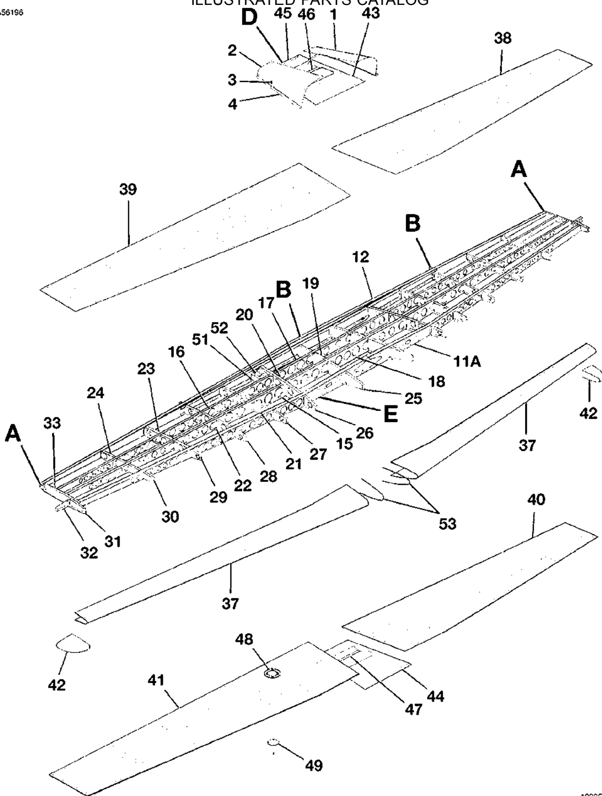
HORIZONTAL STABILIZER STRUCTURE INSTALLATION FIGURE 01 (SHEET 1)
