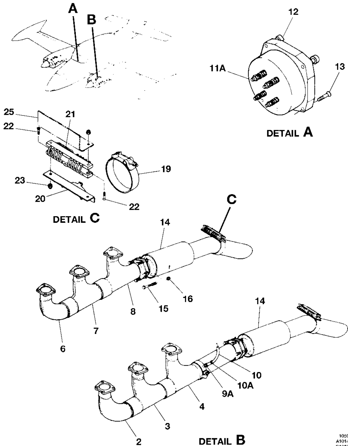
ENGINE EXHAUST SYSTEM FIGURE 01 (SHEET 1)
