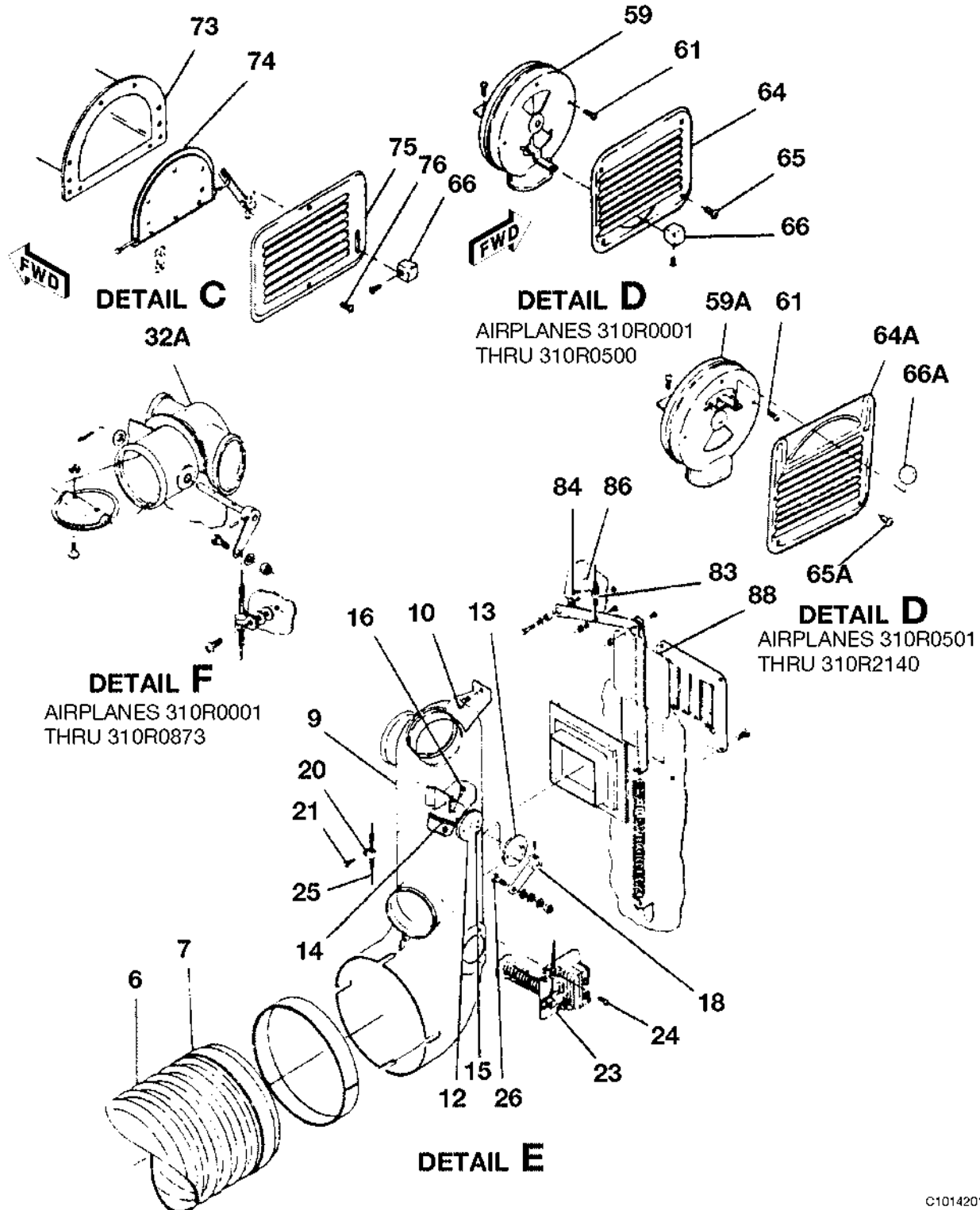
CABIN HEAT AND DEFROST SYSTEM FIGURE 01 (SHEET 2)
