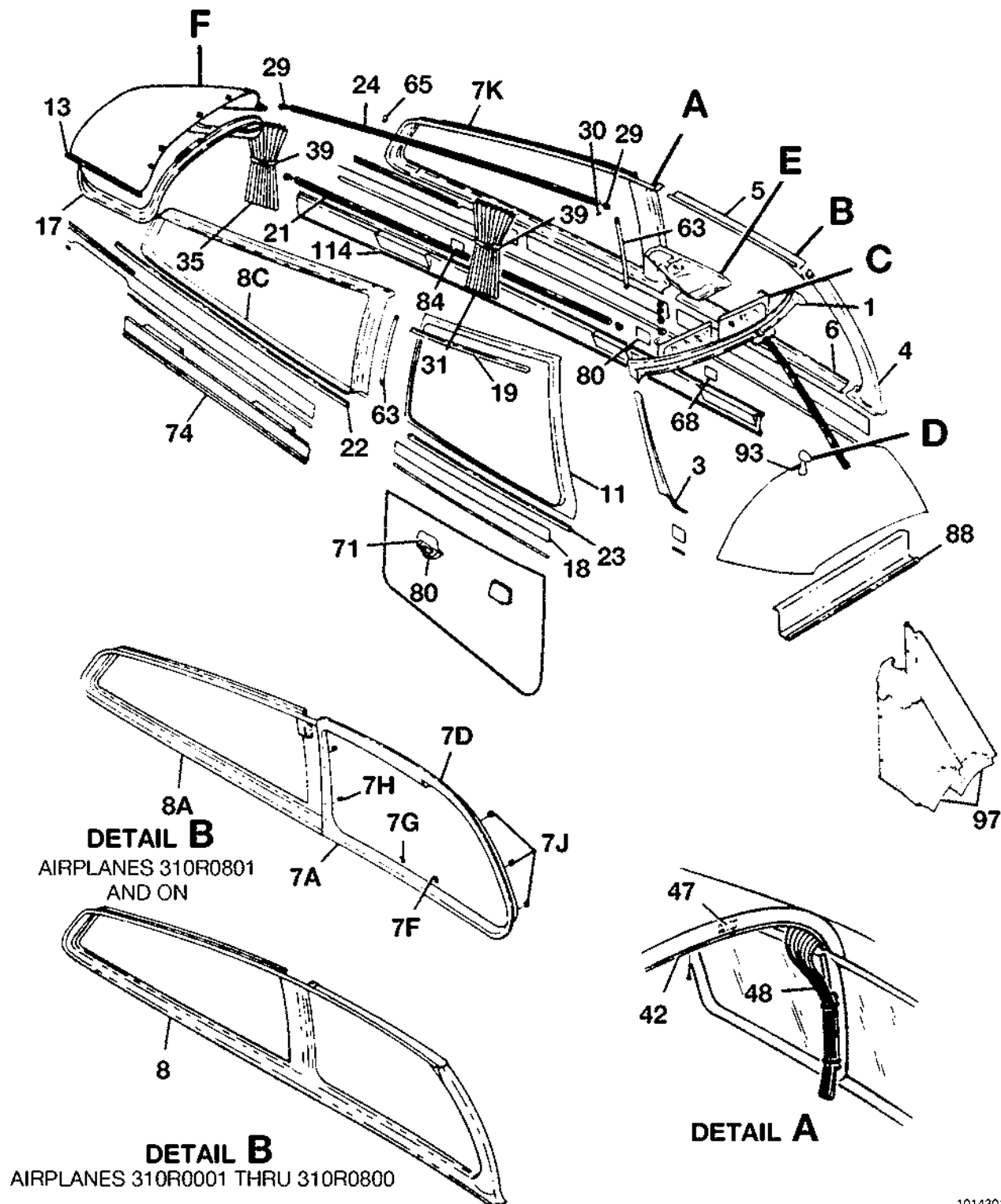
UPHOLSTERY TRIM INSTALLATION FIGURE 01 (SHEET 1)
