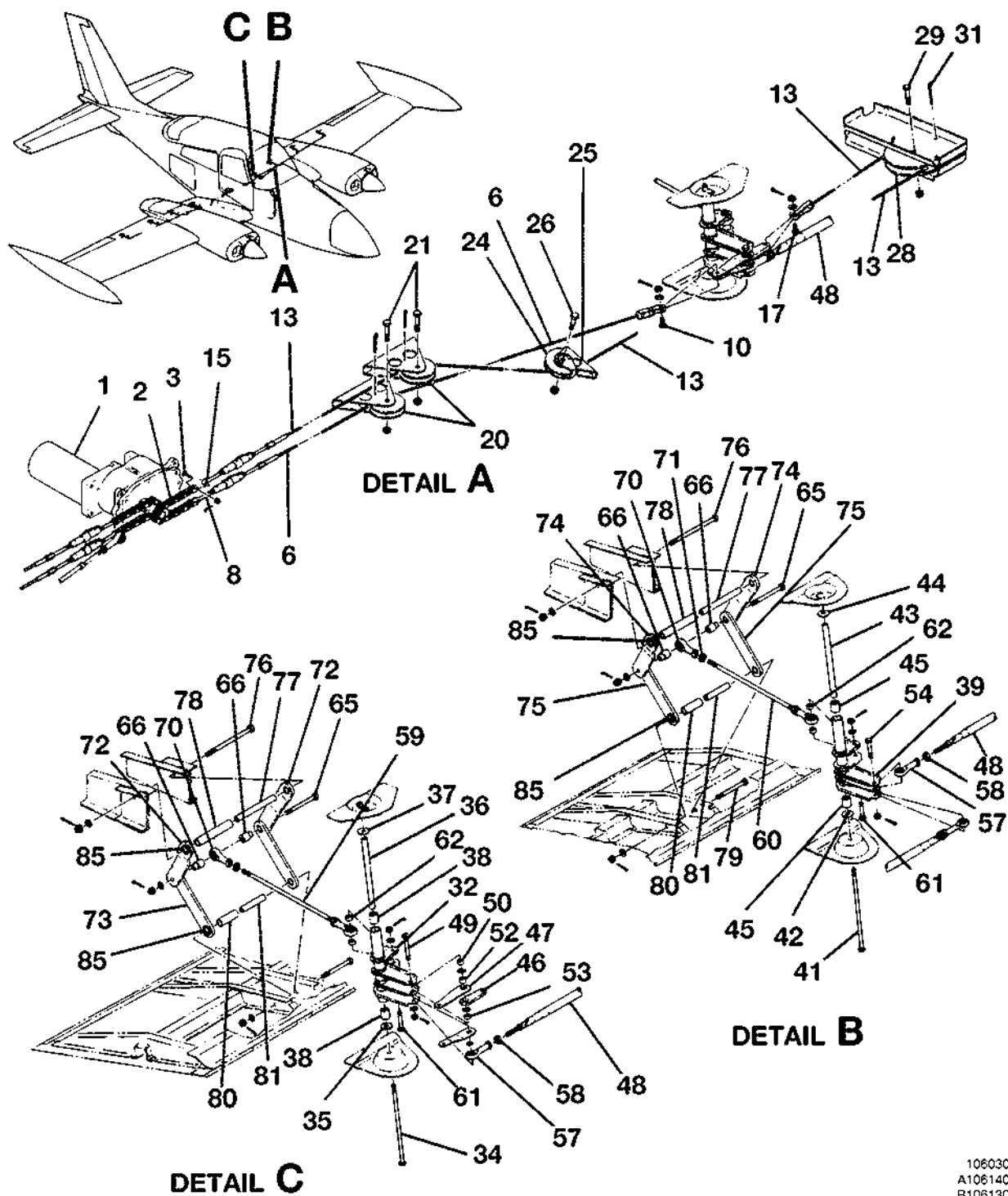
INBOARD FLAP CONTROL SYSTEM FIGURE 01 (SHEET 1)
