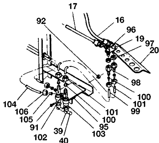
DETAIL J DUAL AIRPLANES 310R0801 THRU 310R2140
