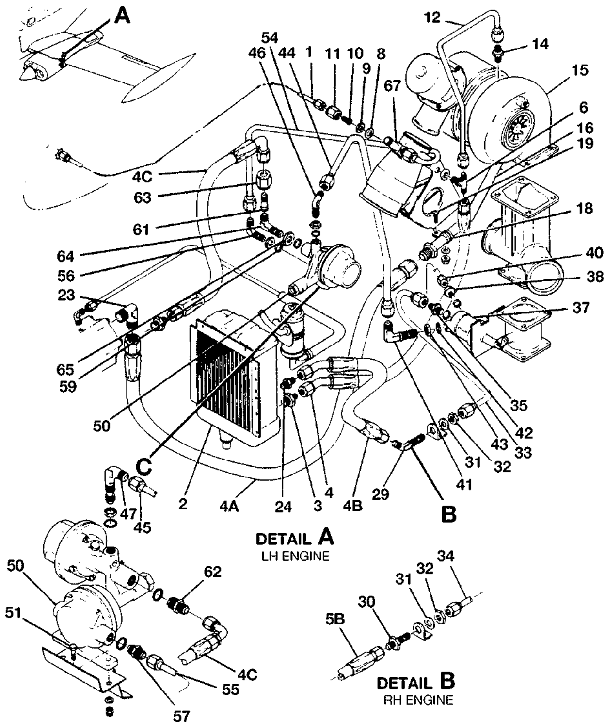
TURBOCHARGER AND CONTROL OIL SYSTEM FIGURE 01 (SHEET 1)
