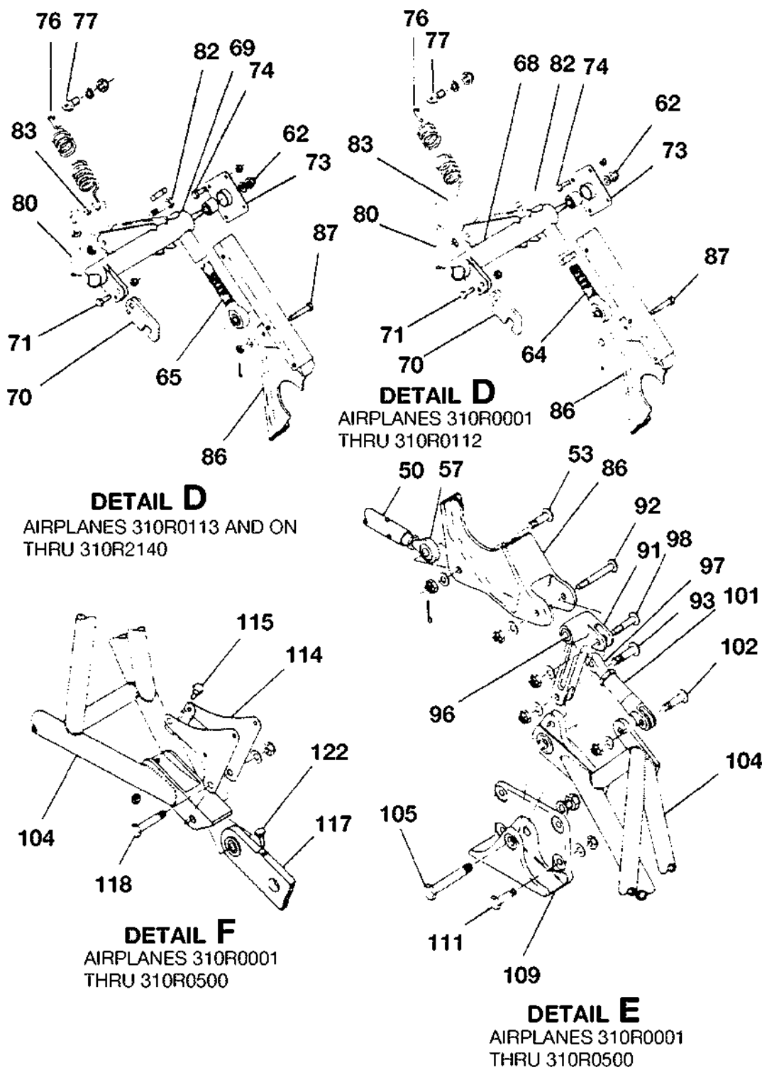
NOSE GEAR RETRACTION LINKAGE INSTALLATION FIGURE 03 (SHEET 2)
