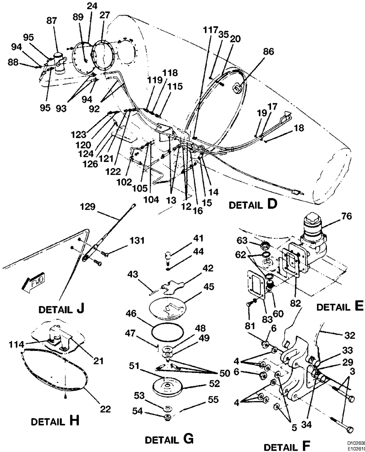
WING TIP FUEL TANKS INSTALLATION FIGURE 01 (SHEET 2)
