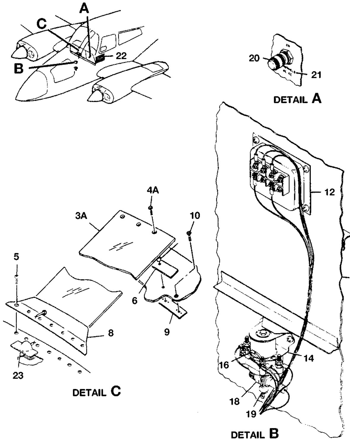
WINDSHIELD ANTI-ICE INSTALLATION-ELECTRICAL FIGURE 02 (SHEET 1)
