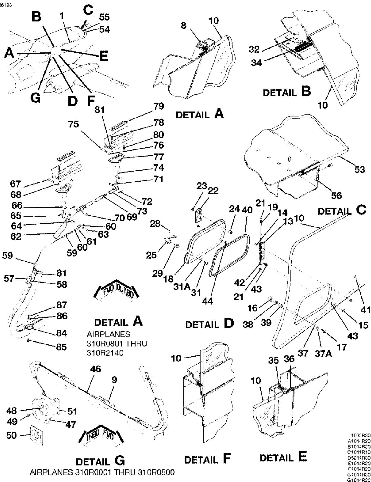
CABIN WINDOWS INSTALLATION FIGURE 02 (SHEET 1)
