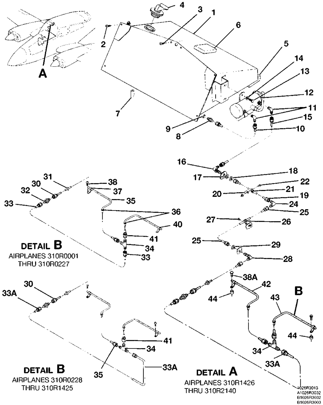
WINDSHIELD ANTI-ICE SYSTEM-ALCOHOL FIGURE 01 (SHEET 1)
