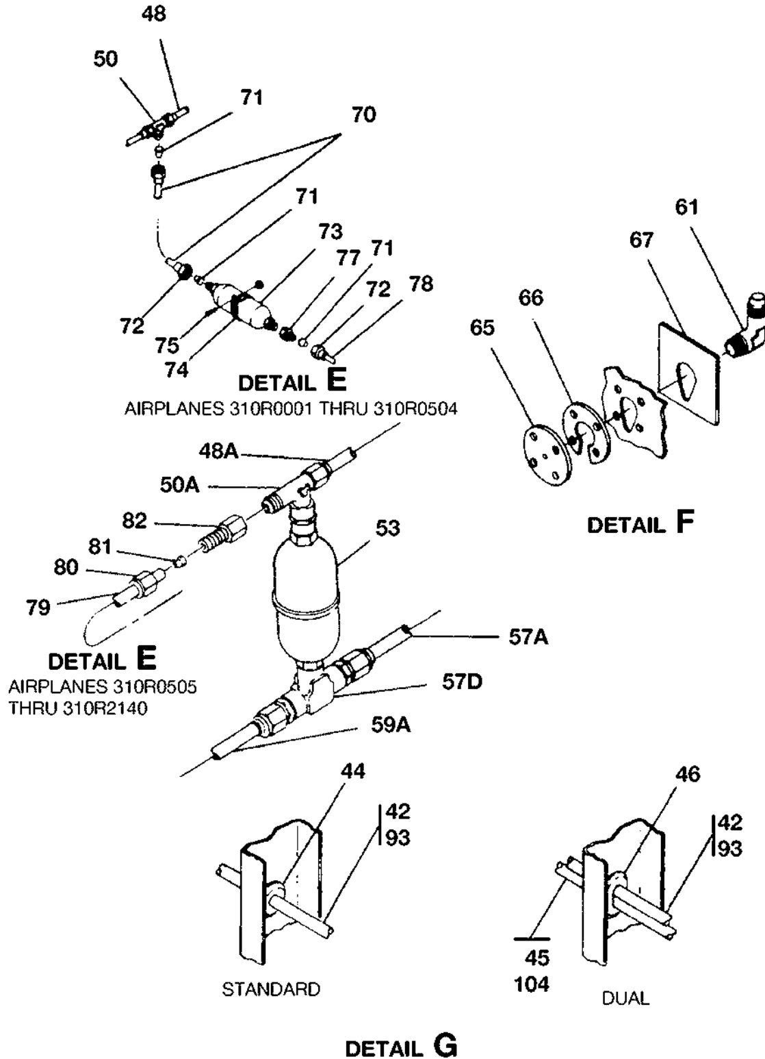
STATIC SYSTEM FIGURE 01 (SHEET 4)
