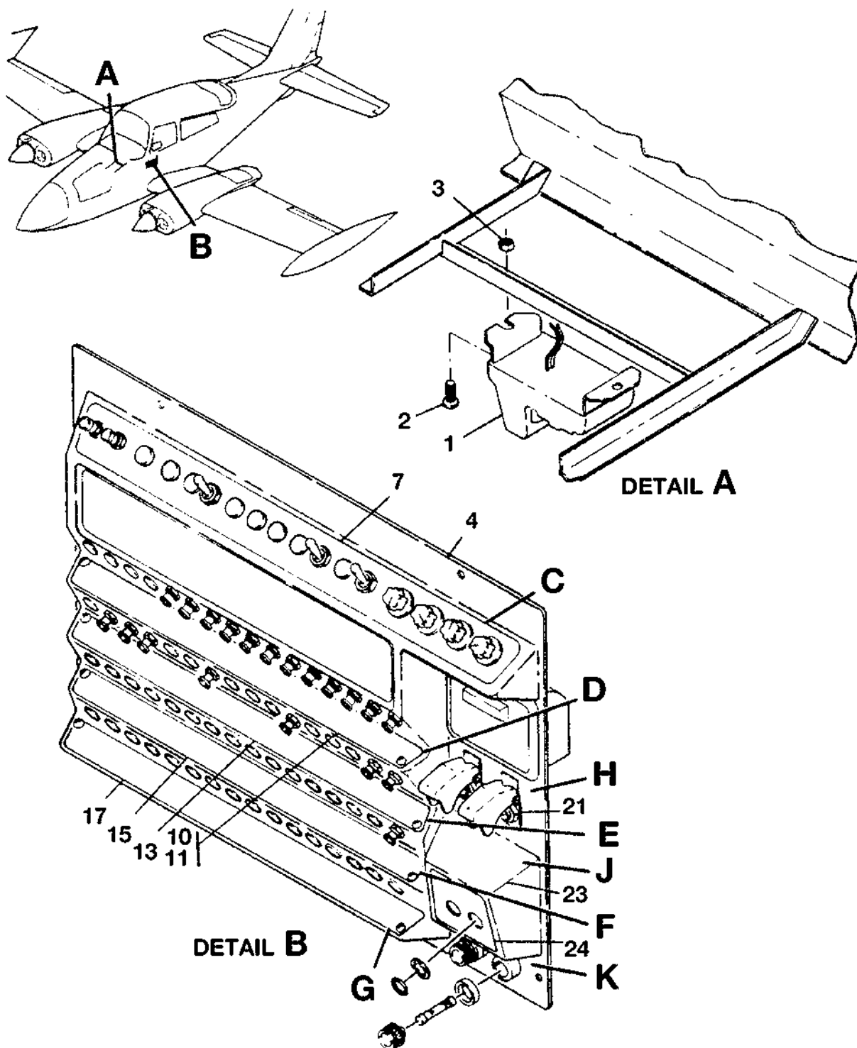
CIRCUIT BREAKER ELECTROLUMINESCENT AND SILKSCREEN PANELS INSTALLATION FIGURE 05 (SHEET 1)
