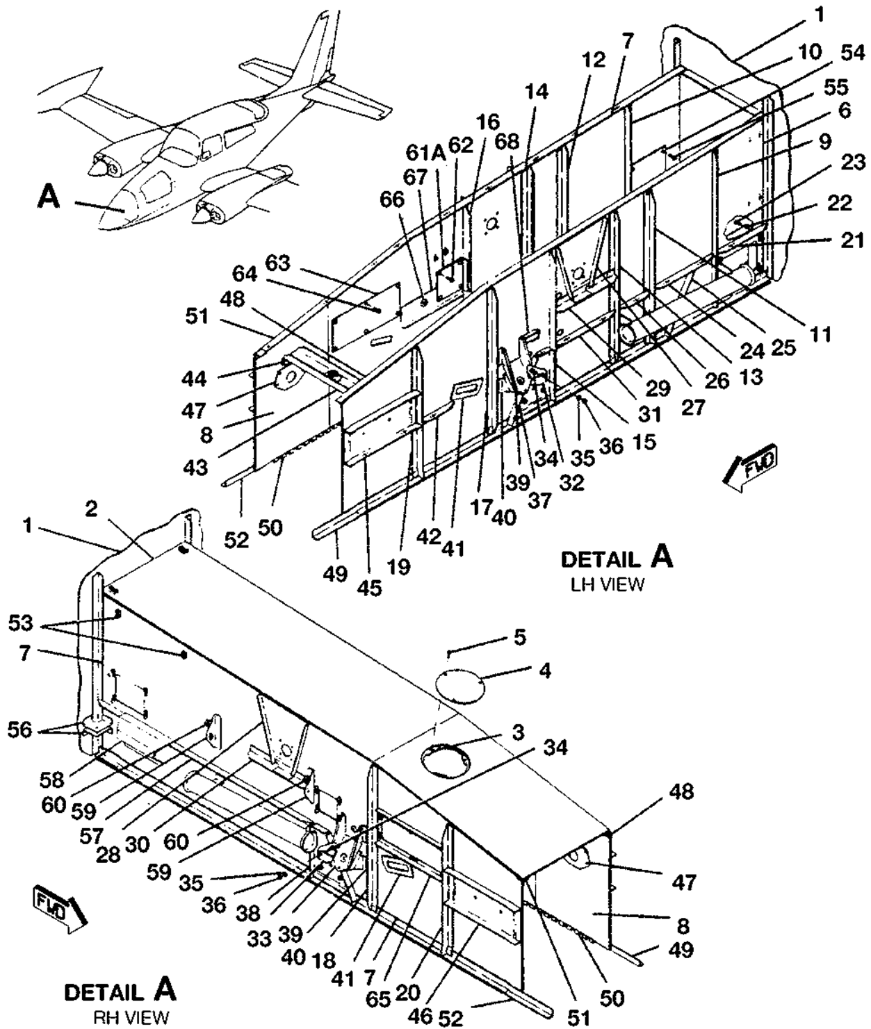
NOSE WHEEL WELL STRUCTURE INSTALLATION FIGURE 03 (SHEET 1)
