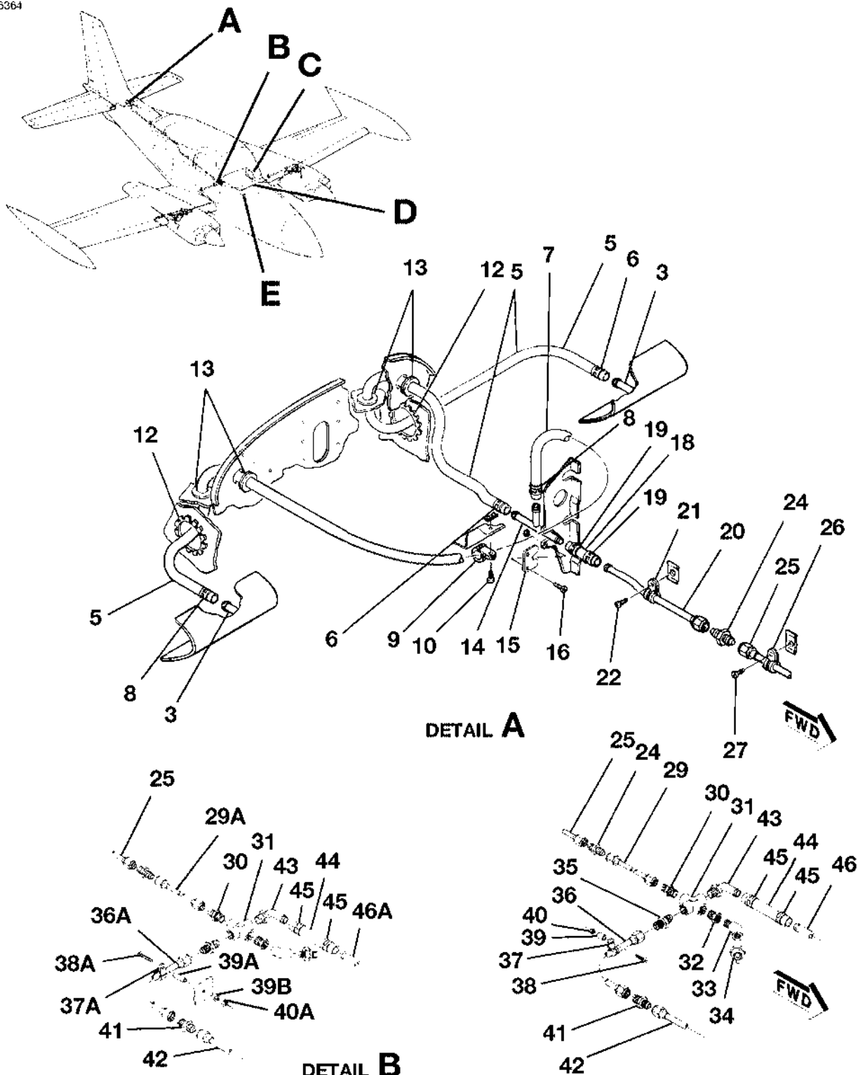
SURFACE DEICE SYSTEM FIGURE 01 (SHEET 1)
