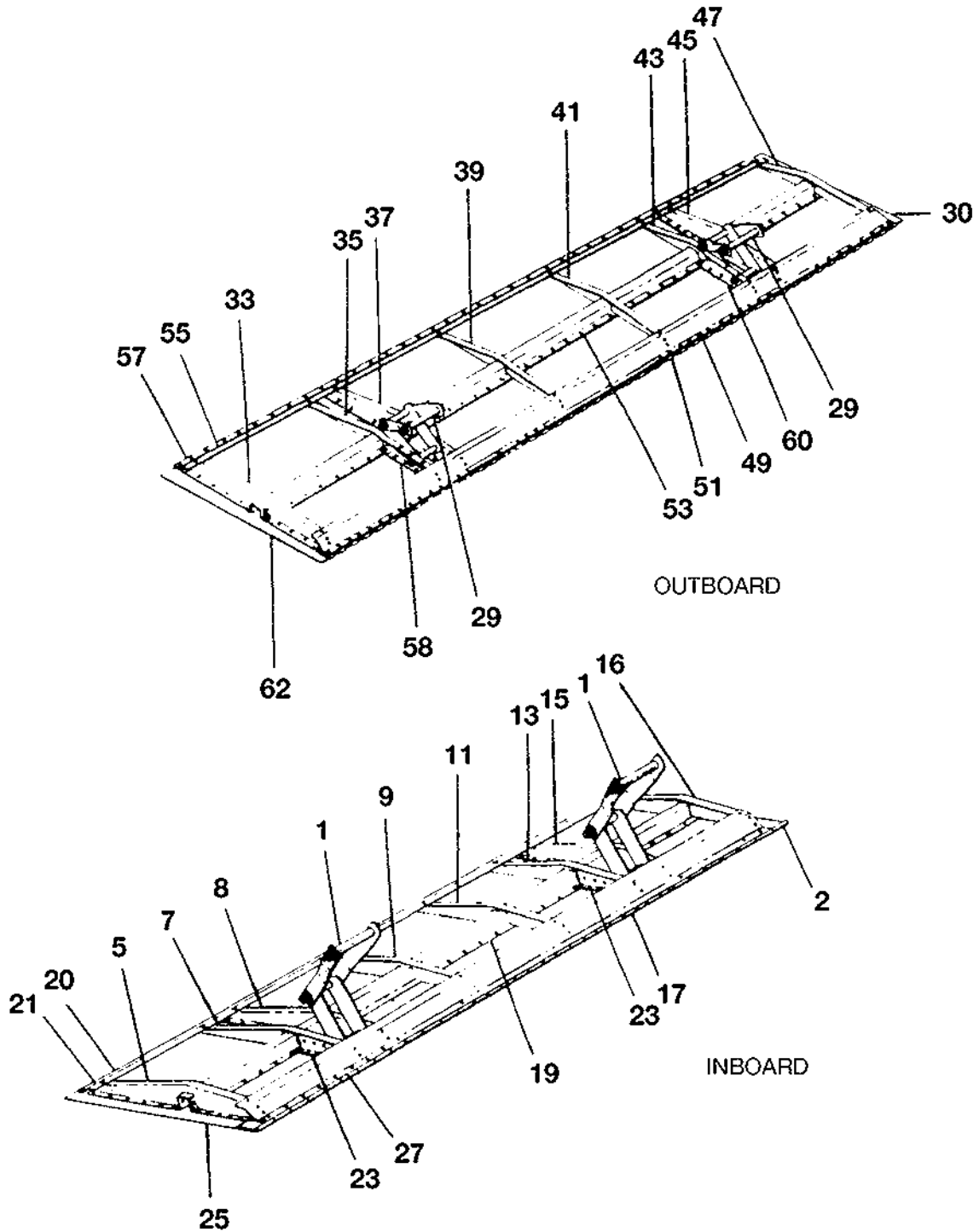
WING FLAP STRUCTURE INSTALLATION FIGURE 03 (SHEET 1)
