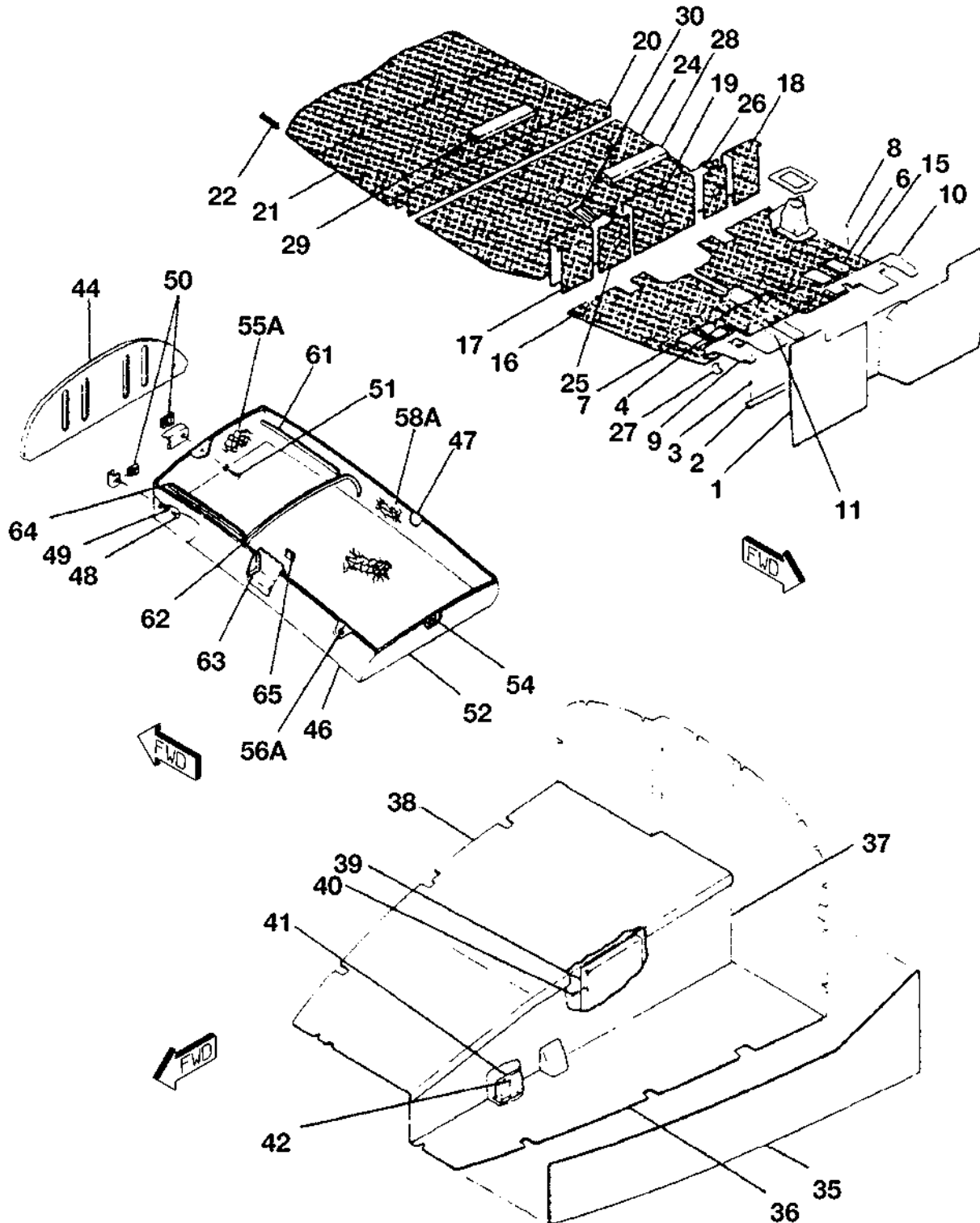
CARPET INSTALLATION FIGURE 01 (SHEET 1)
