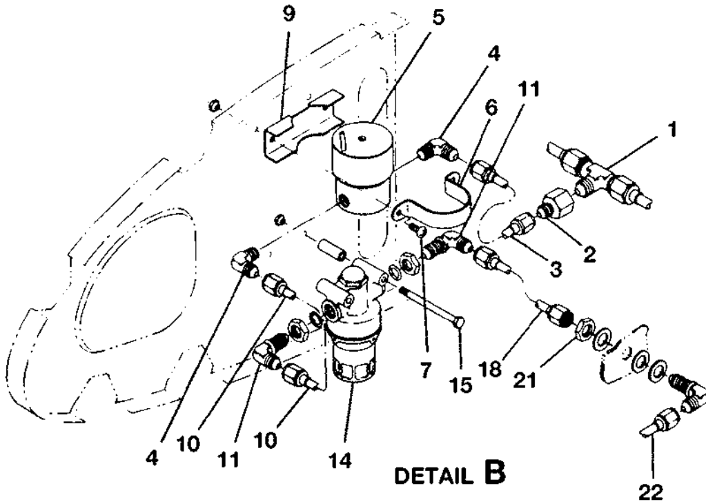
CABIN HEATER FUEL SYSTEM COMPONENTS FIGURE 03 (SHEET 1)
