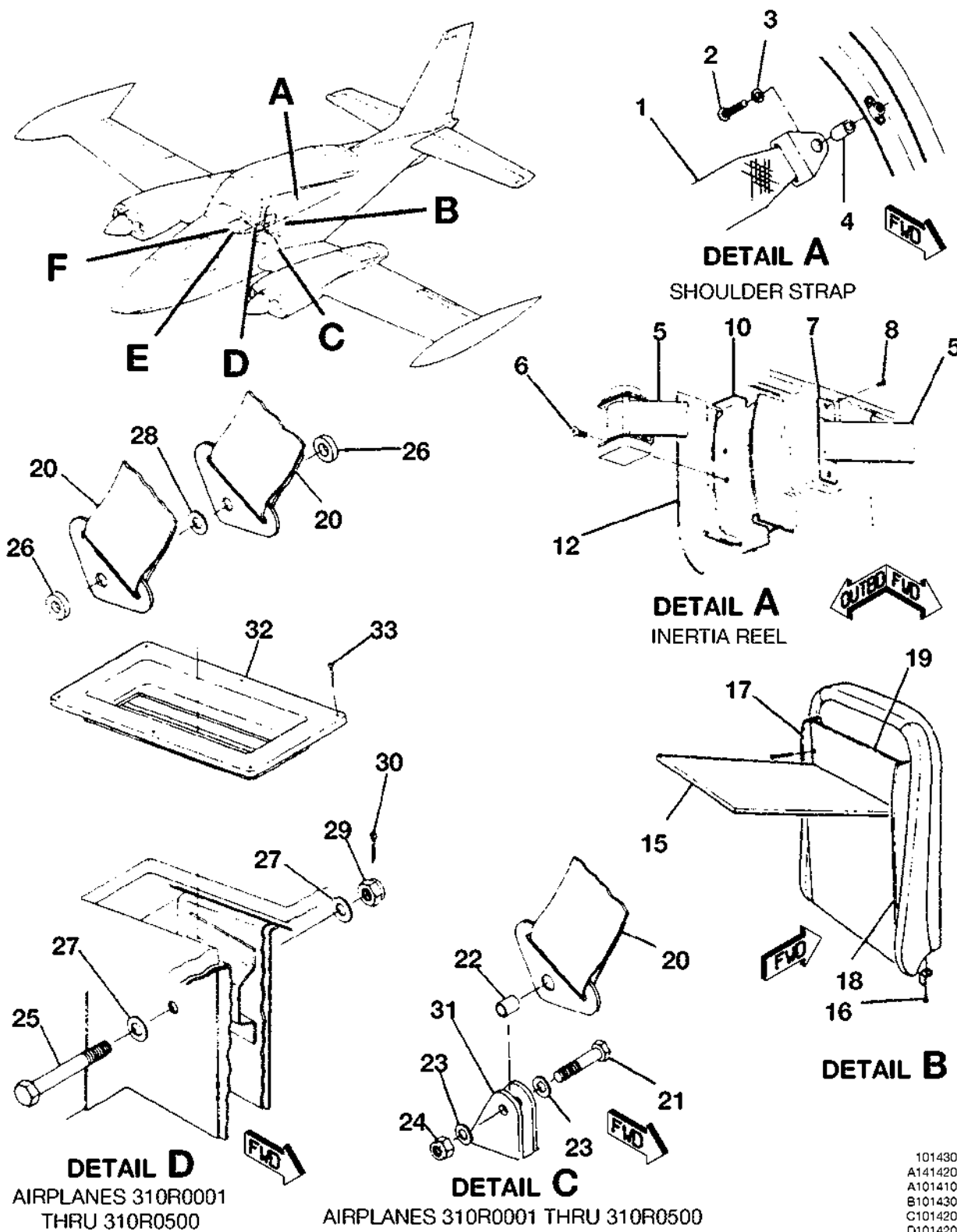
PILOT AND COPILOT ELECTRICALLY ADJUSTABLE SEAT INSTALLATION FIGURE 03 (SHEET 1)
