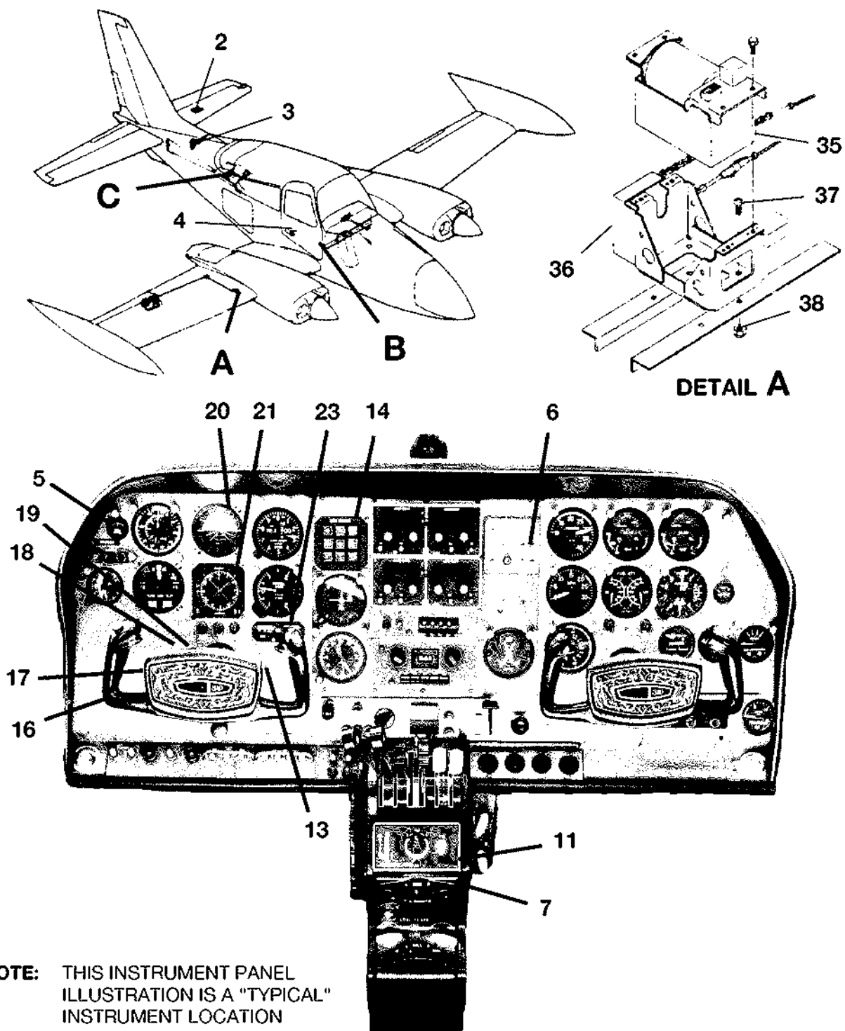
INTEGRATED FLIGHT CONTROL SYSTEM FIGURE 04 (SHEET 1)
