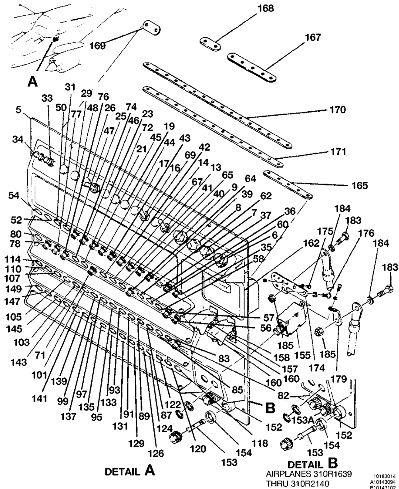
CIRCUIT BREAKER PANEL INSTALLATION FIGURE 04 (SHEET 1)
