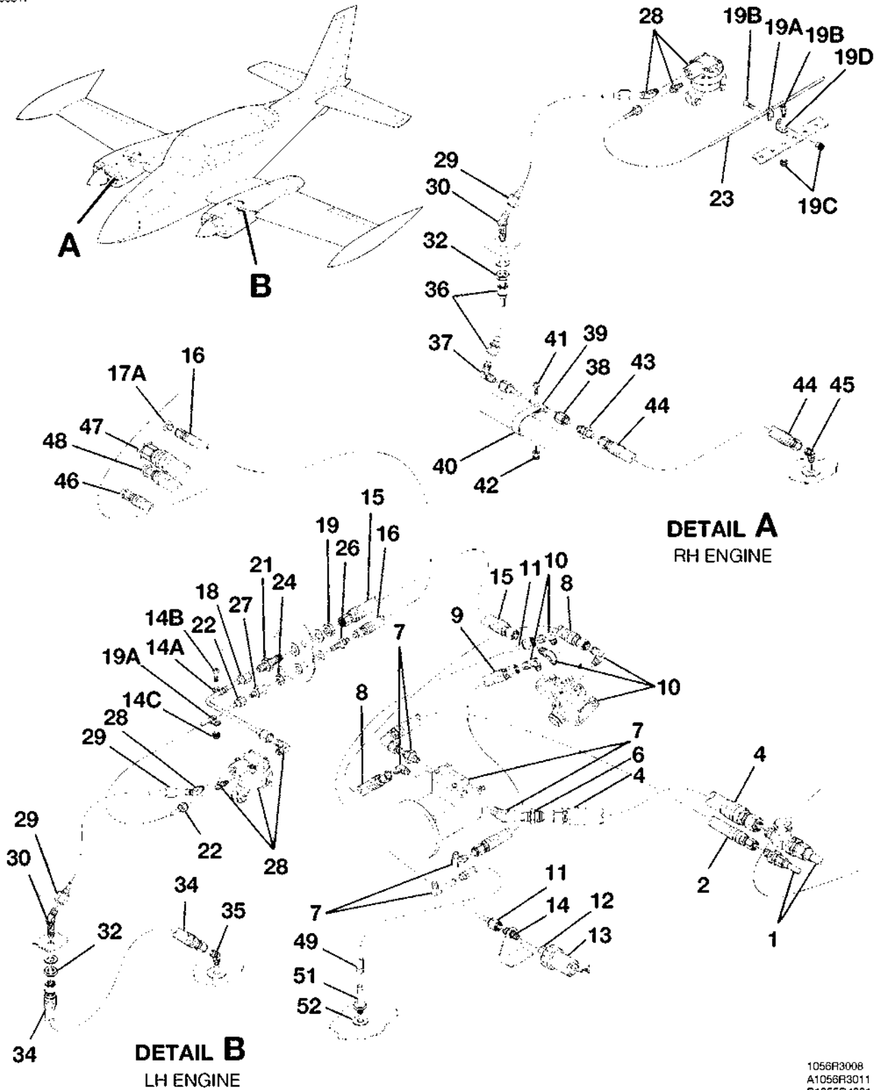
ENGINE COMPARTMENT FUEL SYSTEM COMPONENTS FIGURE 01 (SHEET 1)
