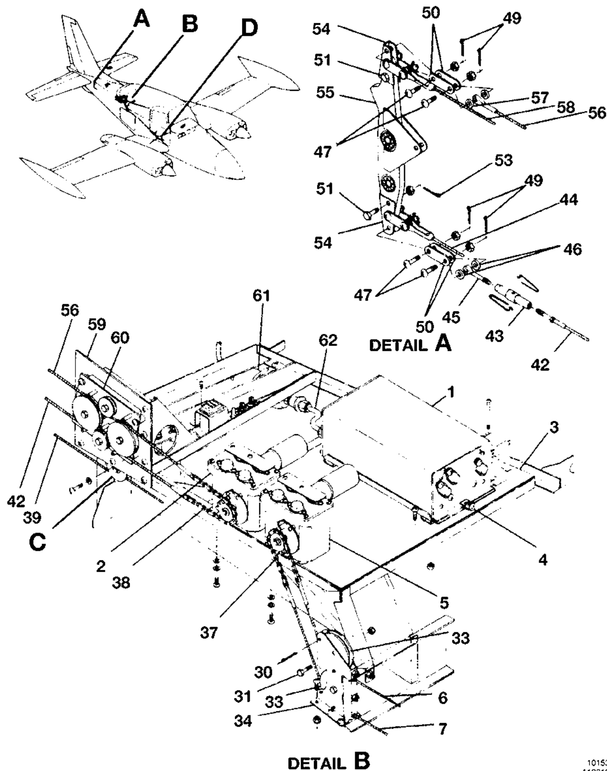
400A NAV-O-MATIC ACTUATOR CABLES INSTALLATION FIGURE 01 (SHEET 1)
