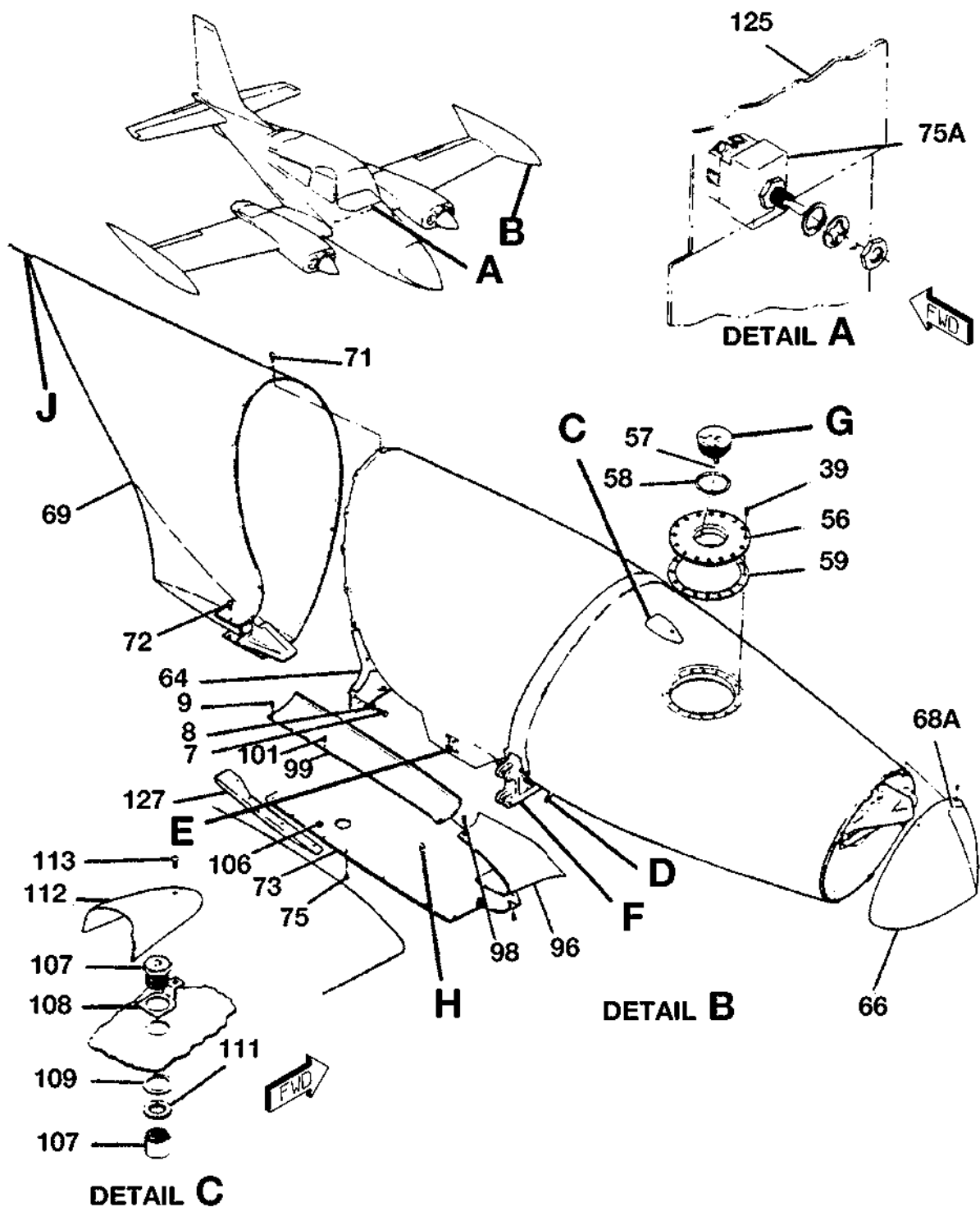
WING TIP FUEL TANKS INSTALLATION FIGURE 01 (SHEET 1)
