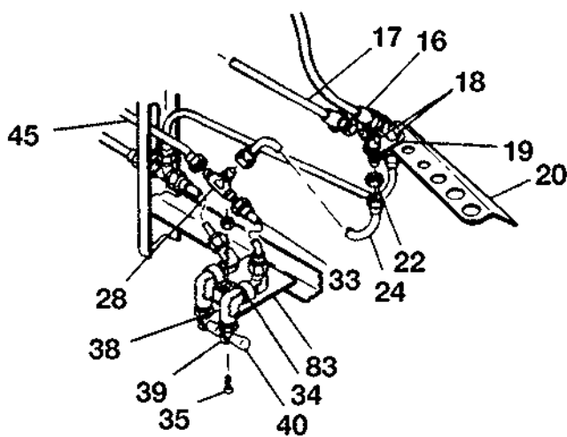
DETAIL J DUAL AIRPLANES 310R0001 THRU 310R0800
