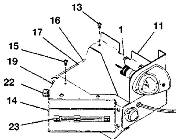
DETAIL A STROBE LIGHT INSTL.
