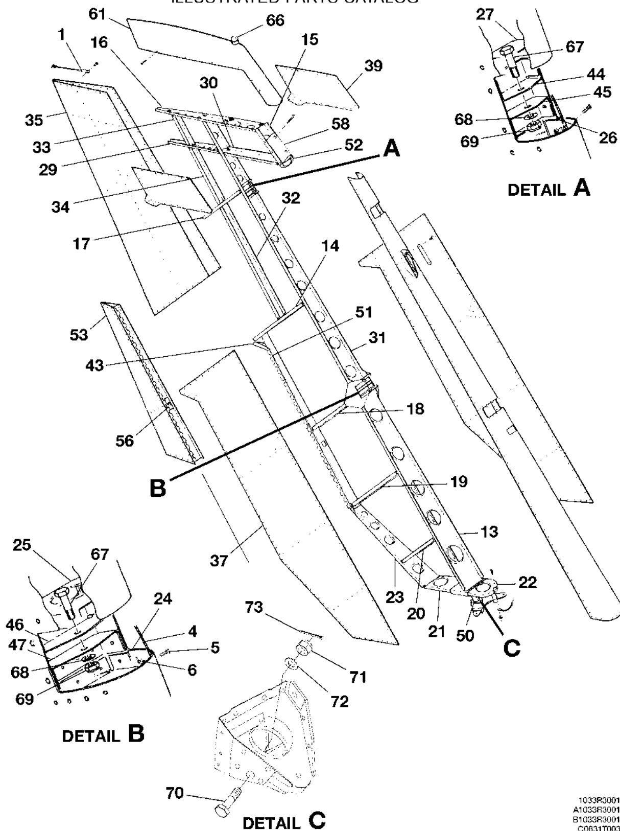
RUDDER STRUCTURE INSTALLATION FIGURE 01 (SHEET 1)
