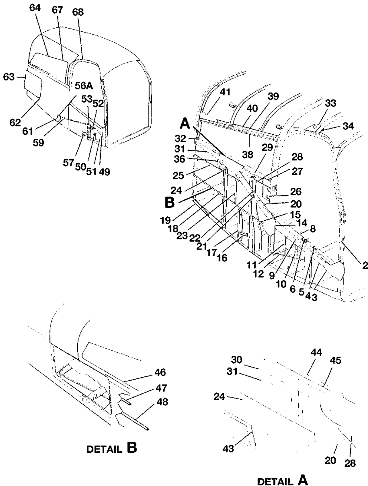
RIGHT CABIN SIDE STRUCTURE ASSEMBLY FIGURE 01 (SHEET 1)
