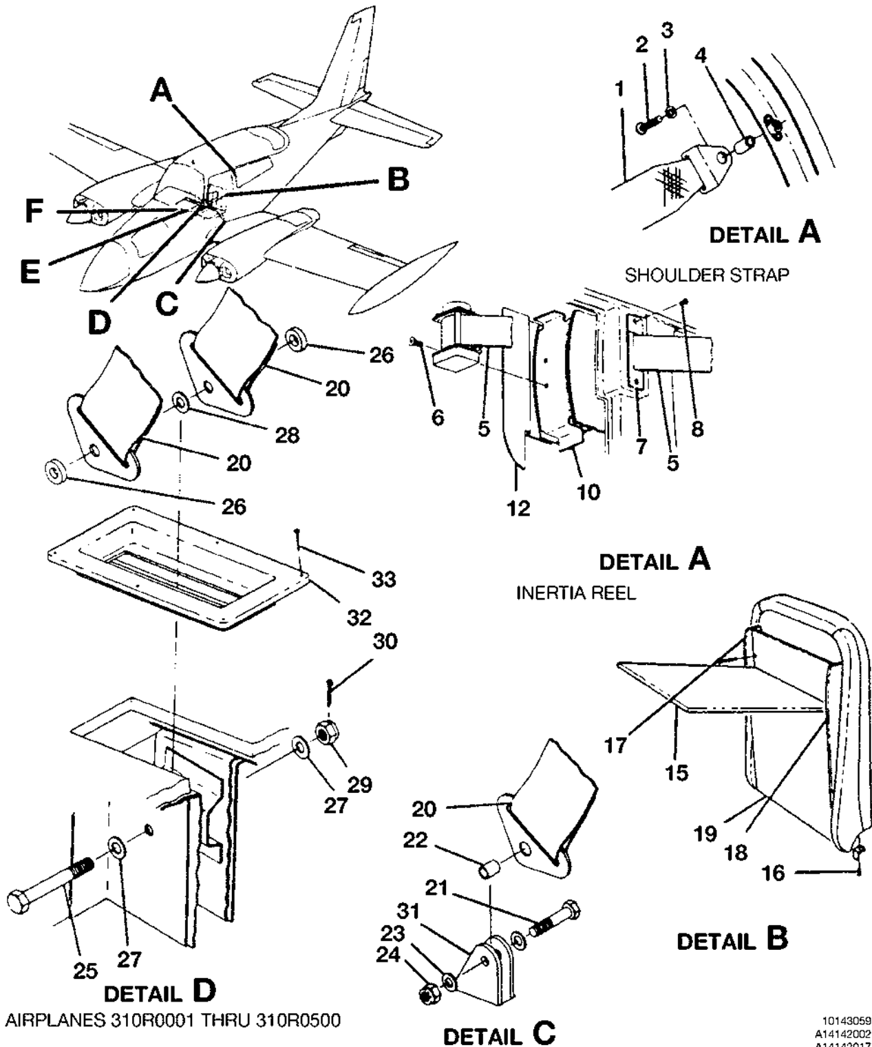
PILOT AND COPILOT MANUALLY ADJUSTABLE SEAT INSTALLATION FIGURE 02 (SHEET 1)
