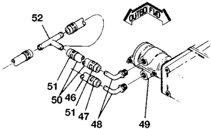
DETAIL B RH ENGINE
