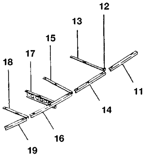
DETAIL B AIRPLANES 310R0001 THRU 310R0500
