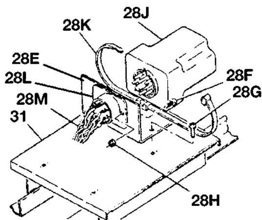
DETAIL C AIRPLANES 310R1201 THRU 310R2140
