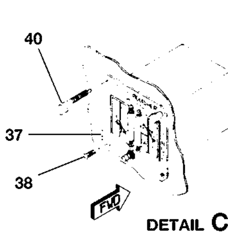
ENGINE COMPARTMENT FIRE EXTINGUISHER FIGURE 01 (SHEET 1)
