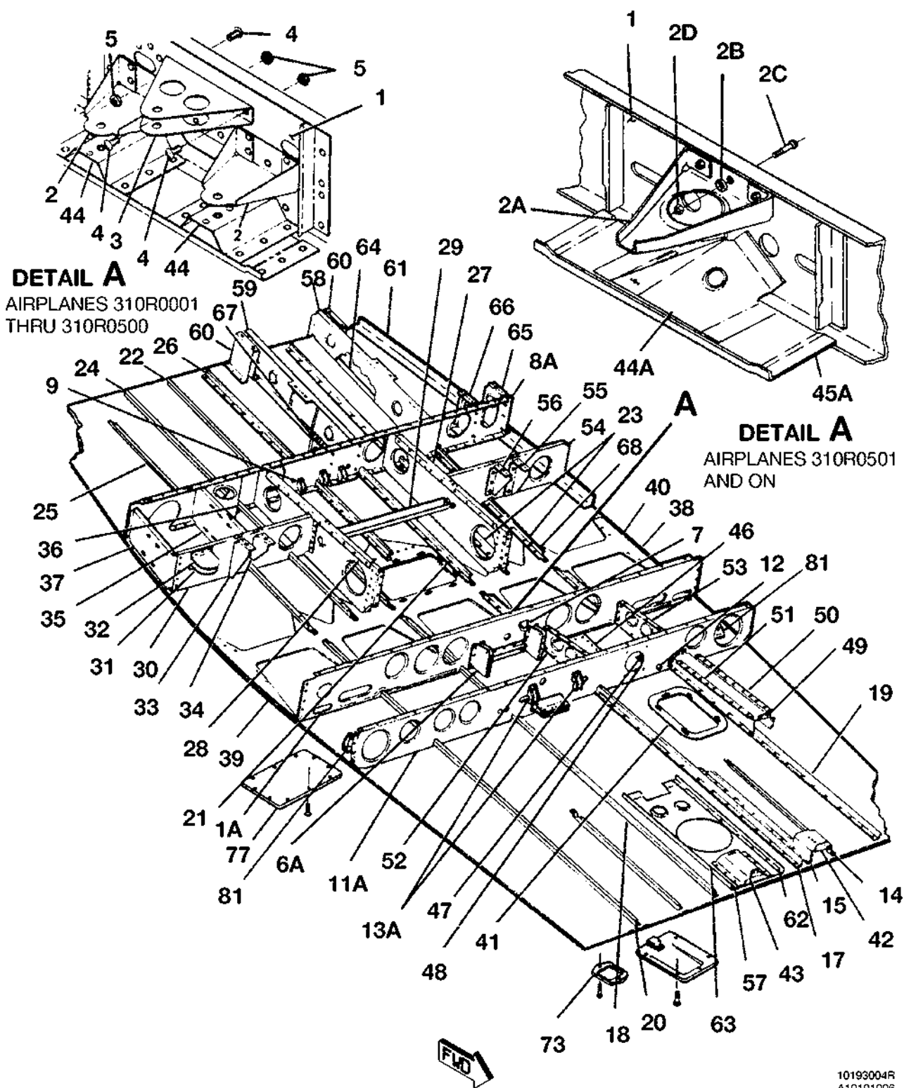
CABIN BOTTOM SECTION STRUCTURE ASSEMBLY FIGURE 01 (SHEET 1)
