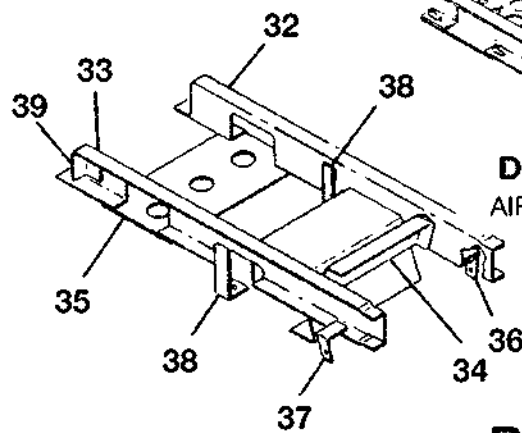
CABIN TOP SECTION STRUCTURE ASSEMBLY FIGURE 01 (SHEET 1)
