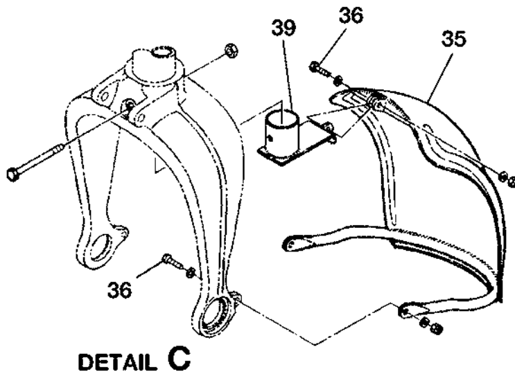
NOSE LANDING GEAR INSTALLATION FIGURE 01 (SHEET 1)
