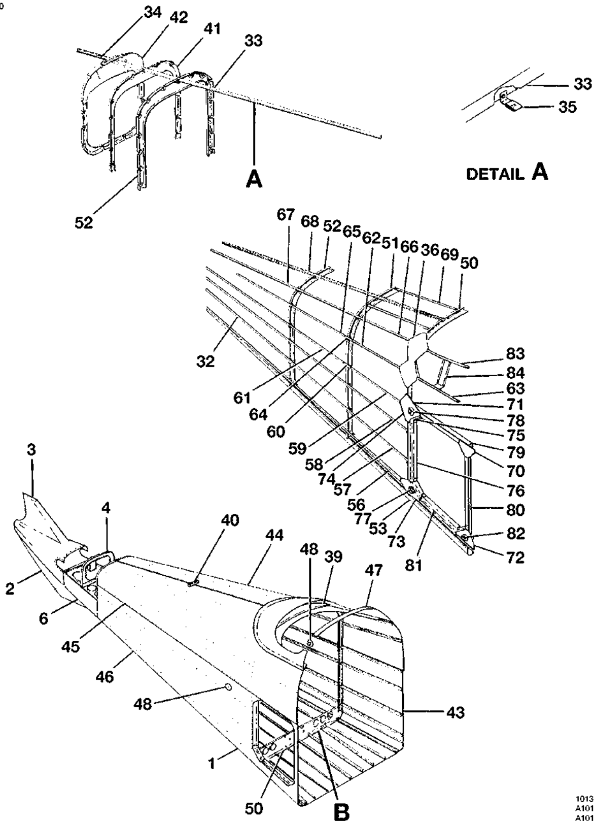
FUSELAGE AFT SECTION STRUCTURE ASSEMBLY FIGURE 01 (SHEET 1)
