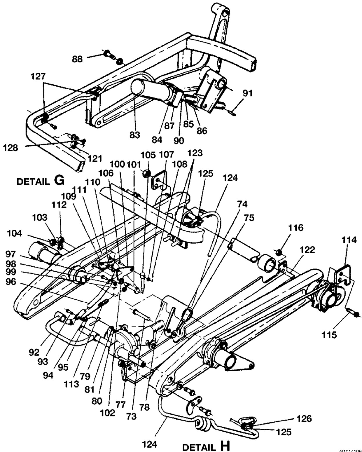
PILOT AND COPILOT ELECTRICALLY ADJUSTABLE SEAT INSTALLATION FIGURE 03 (SHEET 3)
