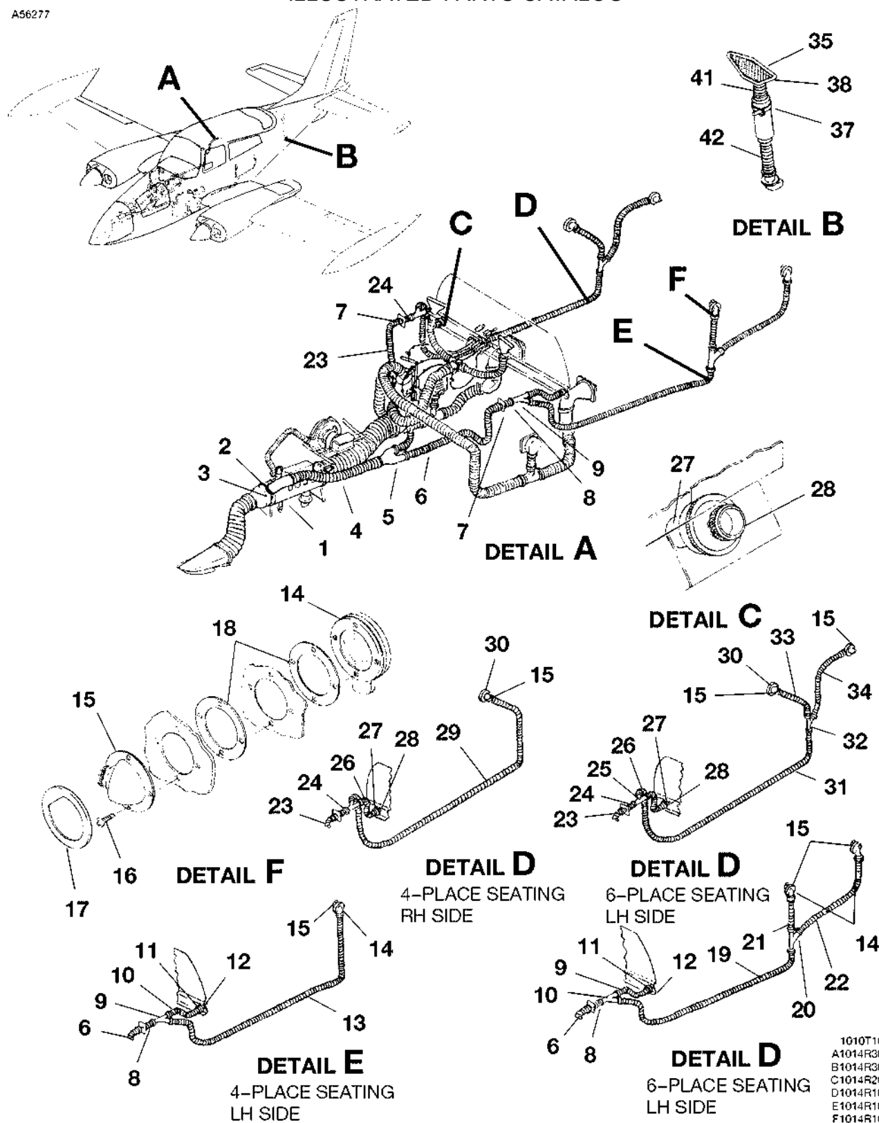
CABIN VENTILATION SYSTEM FIGURE 02 (SHEET 1)
