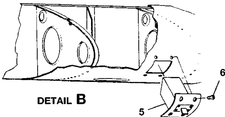
ANGLE OF ATTACK SYSTEM FIGURE 01 (SHEET 1)
