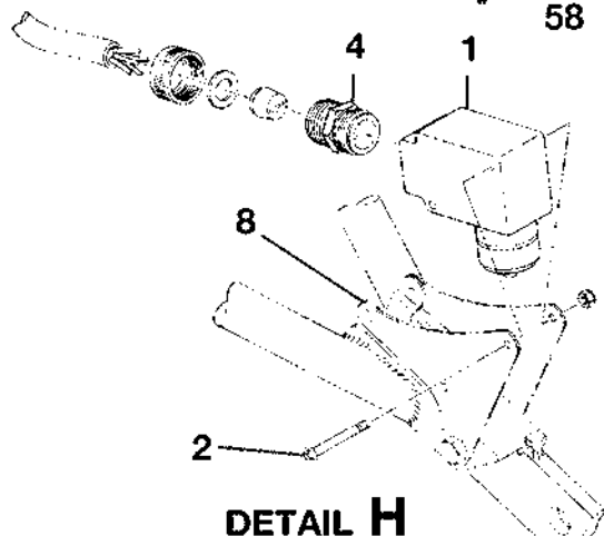
LANDING GEAR ELECTRICAL COMPONENTS FIGURE 01 (SHEET 2)
