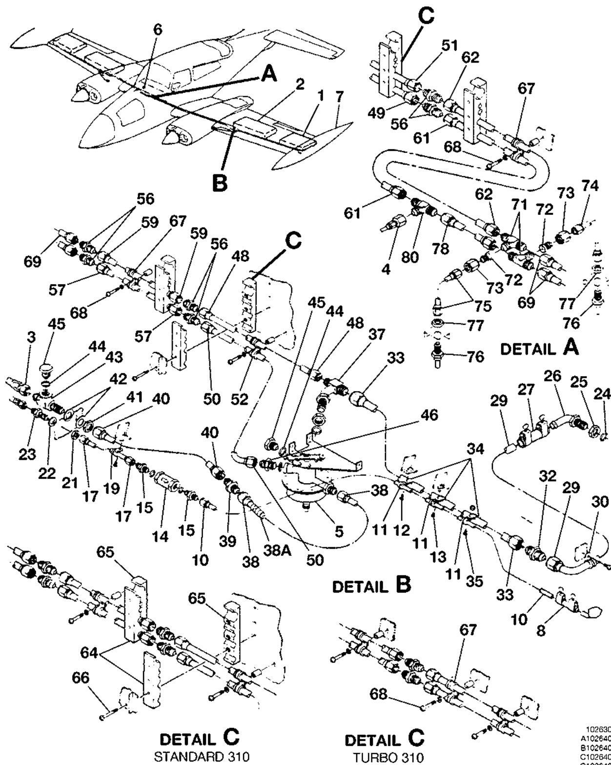
MAIN FUEL SYSTEM INSTALLATION FIGURE 01 (SHEET 1)
