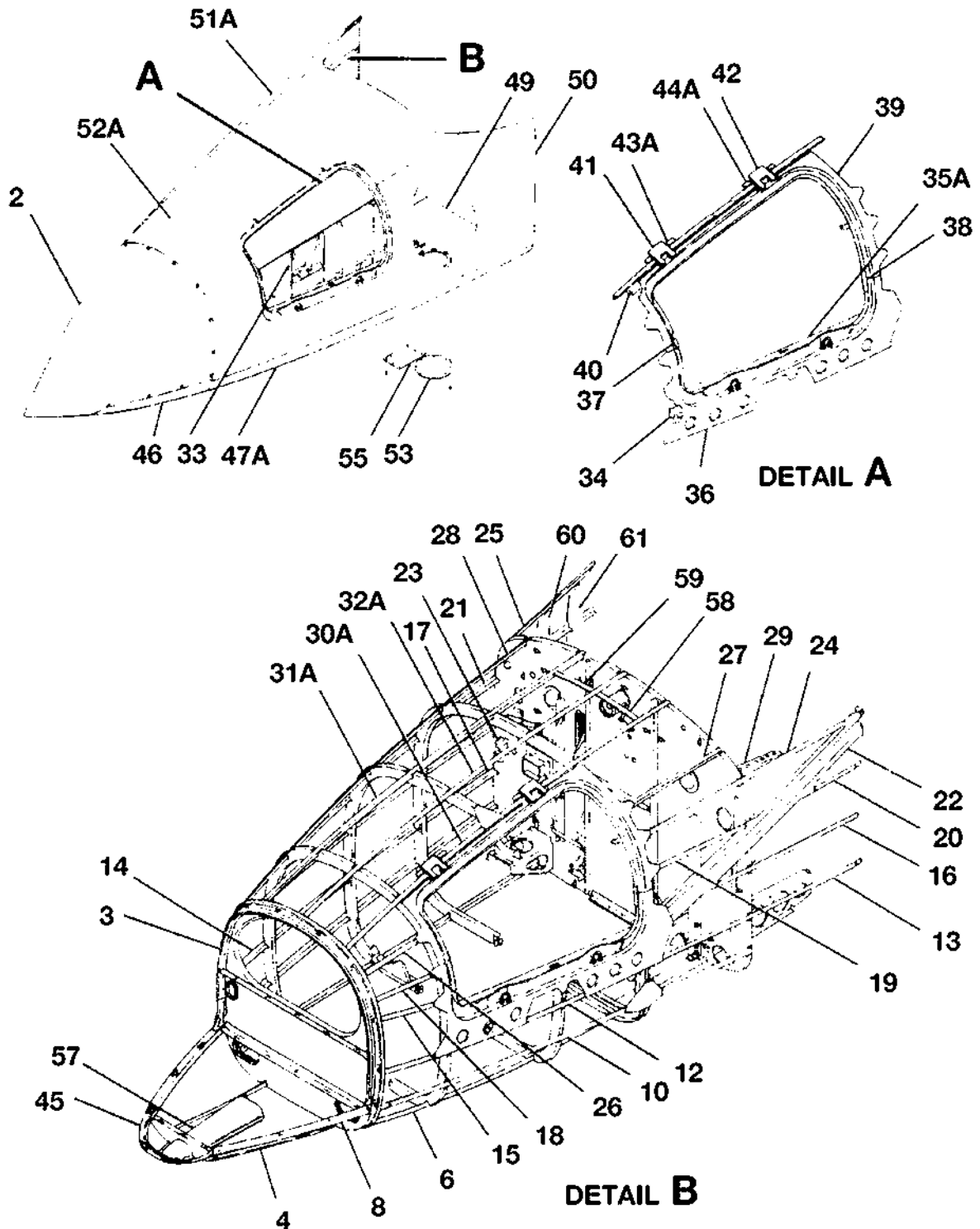
NOSE STRUCTURE ASSEMBLY FIGURE 01 (SHEET 1)
