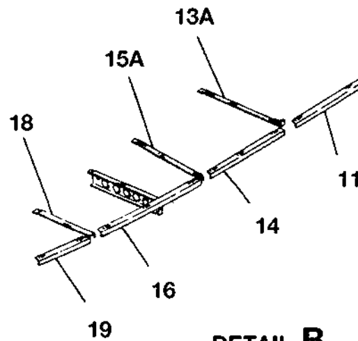
DETAIL B AIRPLANES 310R0501 THRU 310R2140
