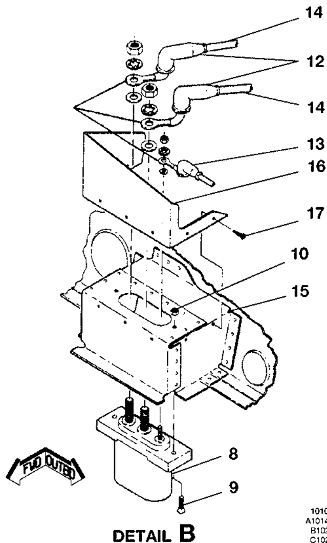
DC POWER SYSTEM INSTALLATION FIGURE 02 (SHEET 1)
