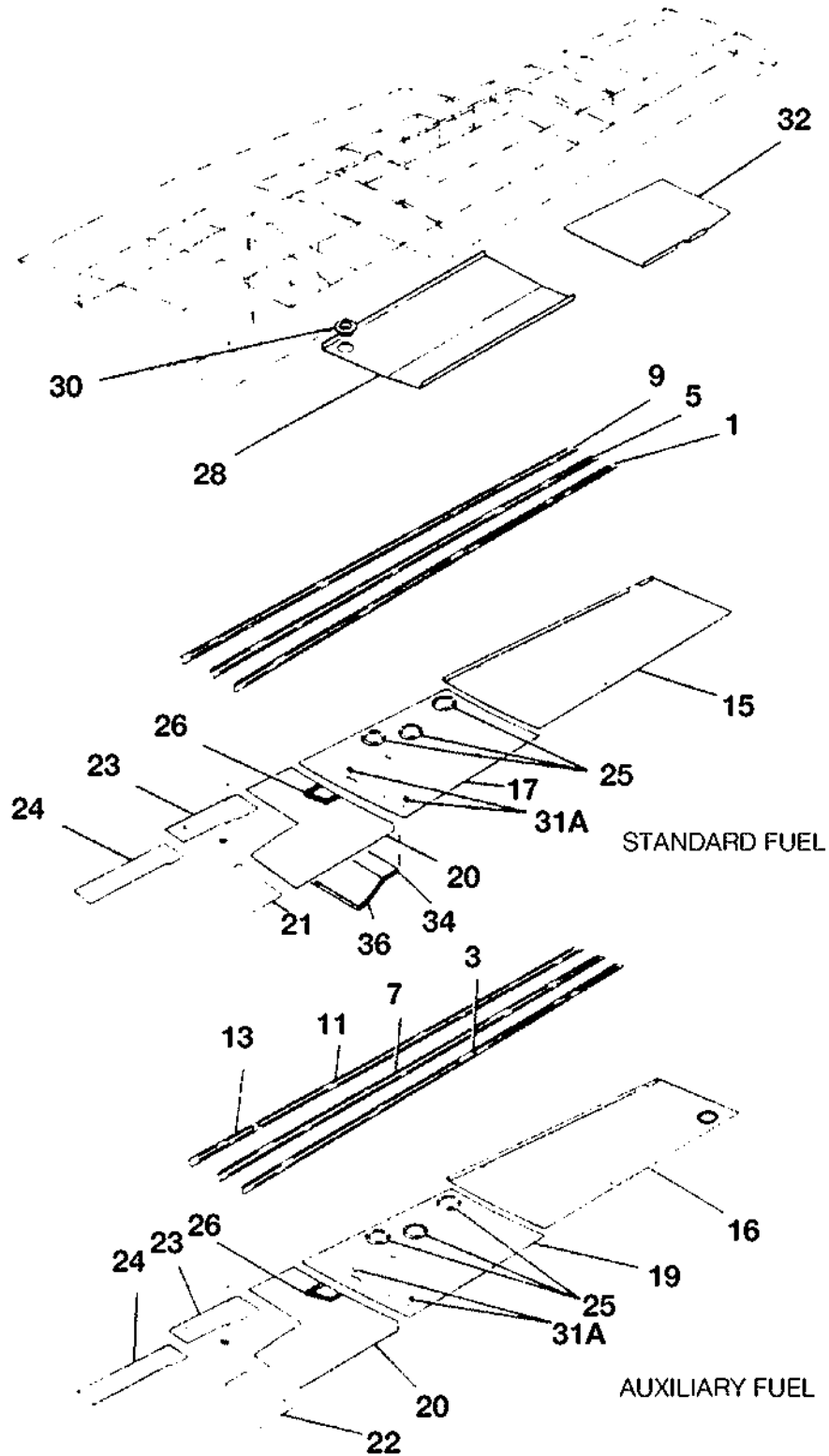
WING LOWER INTERSPAR SKINS AND STRINGERS INSTALLATION FIGURE 05 (SHEET 1)
