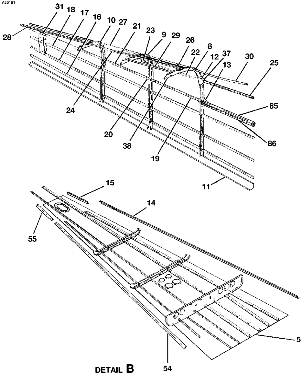
FUSELAGE AFT SECTION STRUCTURE ASSEMBLY FIGURE 01 (SHEET 2)
