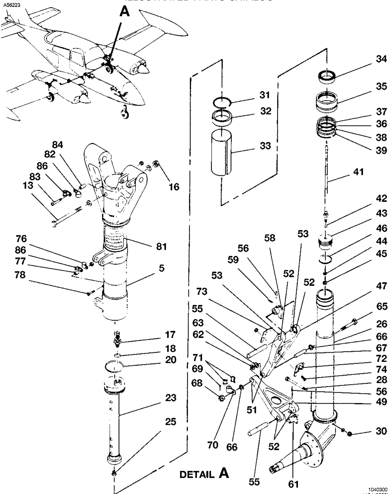
MAIN LANDING GEAR STRUT ASSEMBLY FIGURE 02 (SHEET 1)
