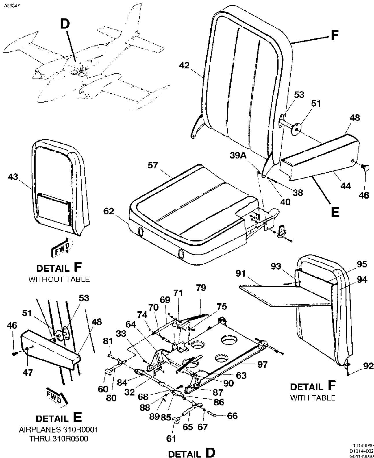
PILOT AND COPILOT SEAT INSTALLATION FIGURE 01 (SHEET 2)
