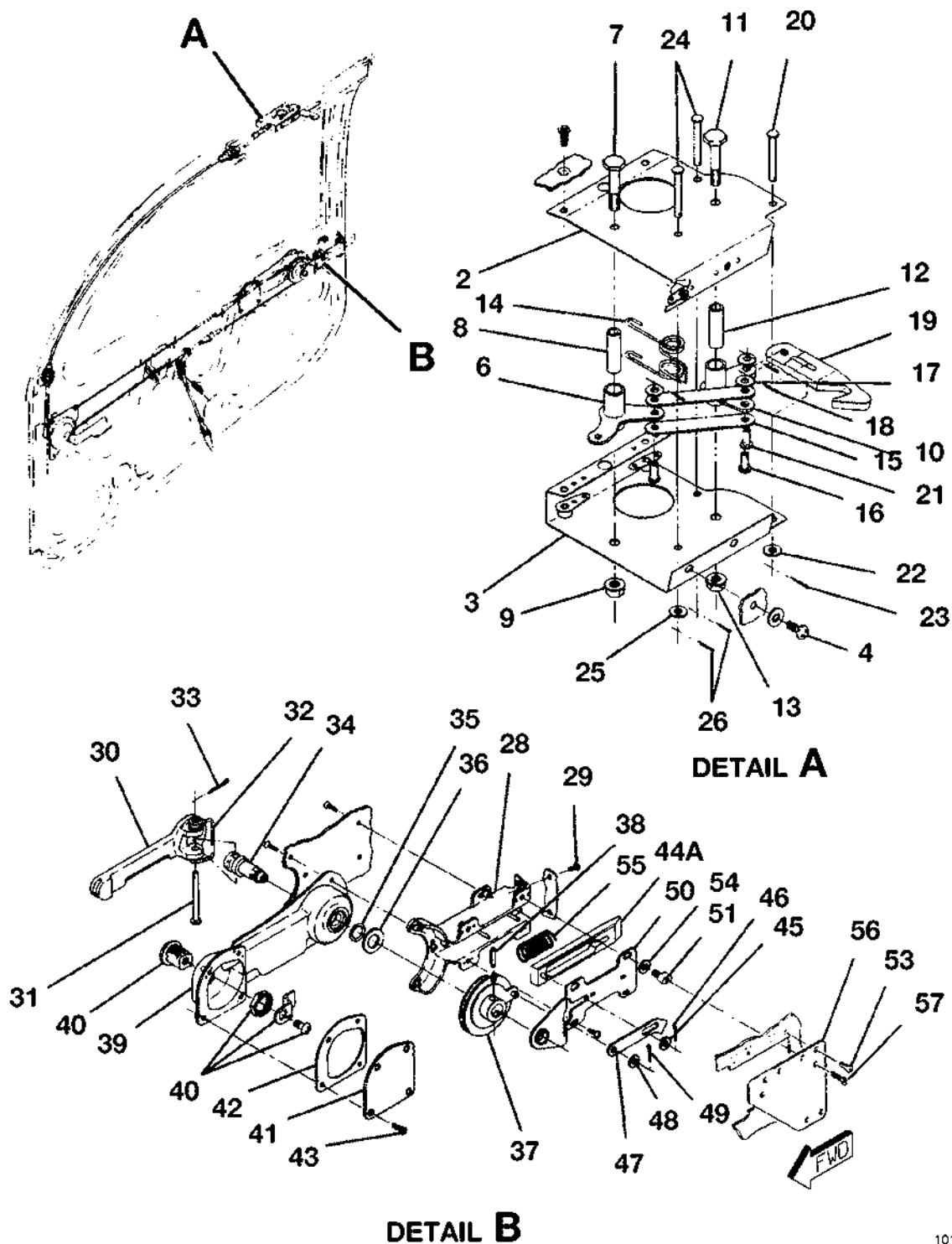
CABIN DOOR LATCH INSTALLATION FIGURE 03 (SHEET 1)
