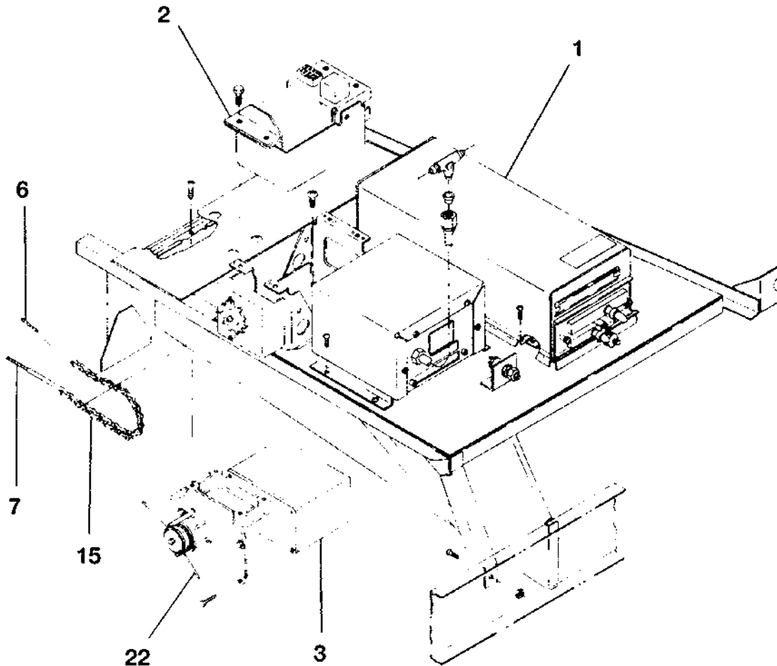
DETAIL C AIRPLANES 310R0501 THRU 310R0800
