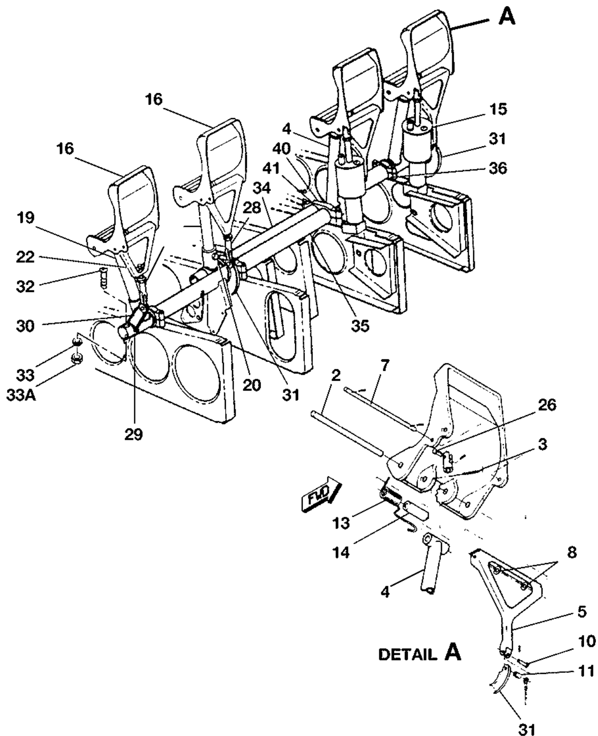
RUDDER AND BRAKE PEDAL INSTALLATION FIGURE 01 (SHEET 1)
