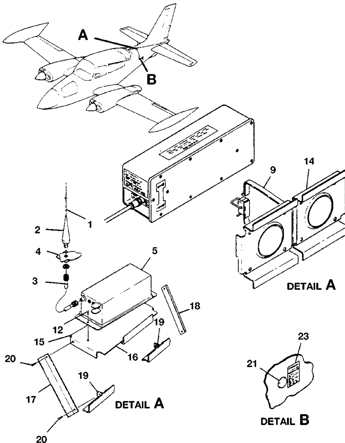
LOCATOR BEACON INSTALLATION FIGURE 01 (SHEET 1)
