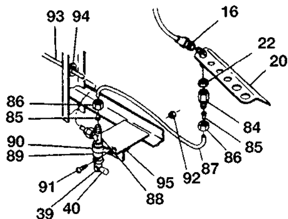
DETAIL H STANDARD AIRPLANES 310R0801 THRU 310R2140
