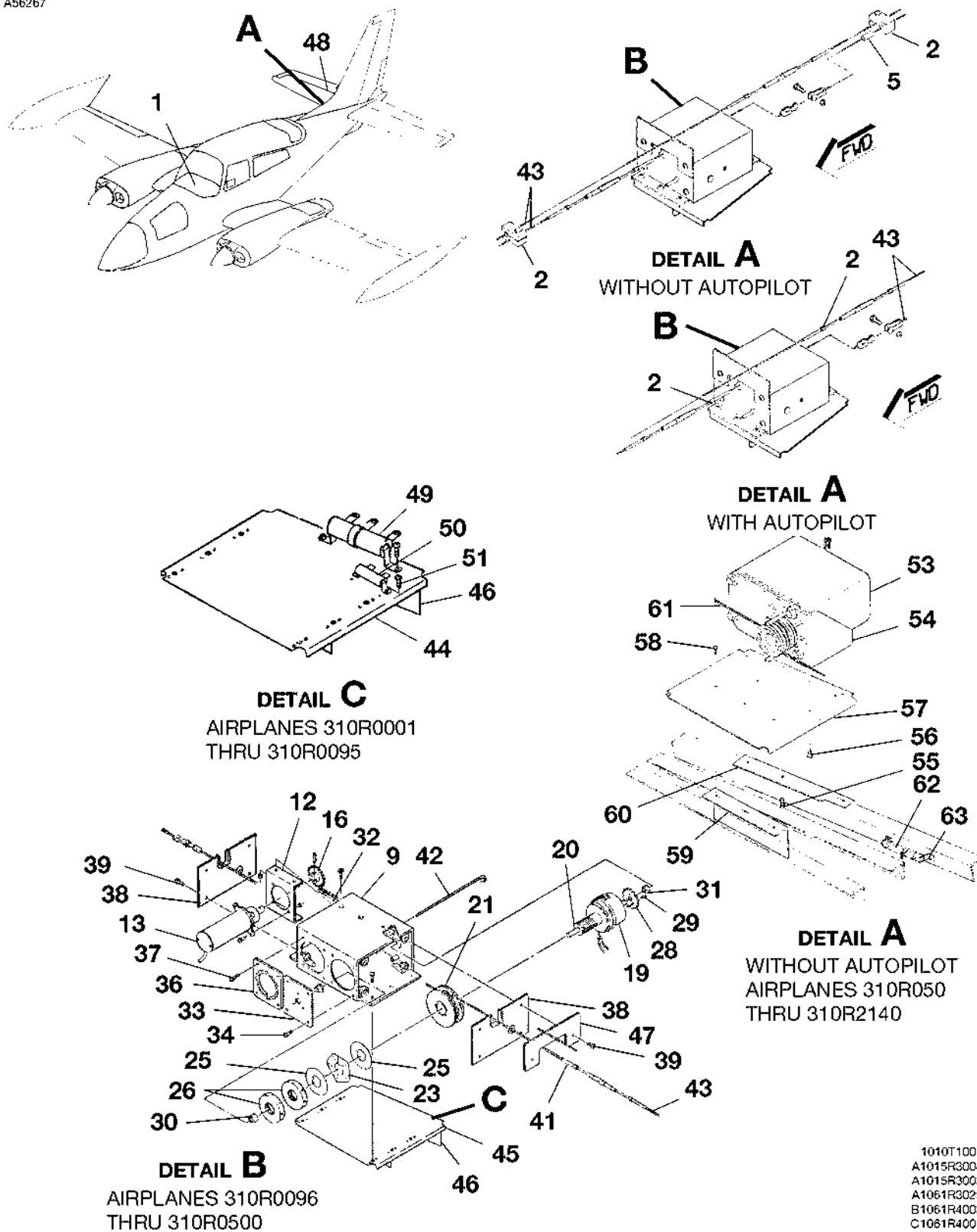
ELECTRIC ELEVATOR TRIM CONTROL SYSTEM FIGURE 03 (SHEET 1)
