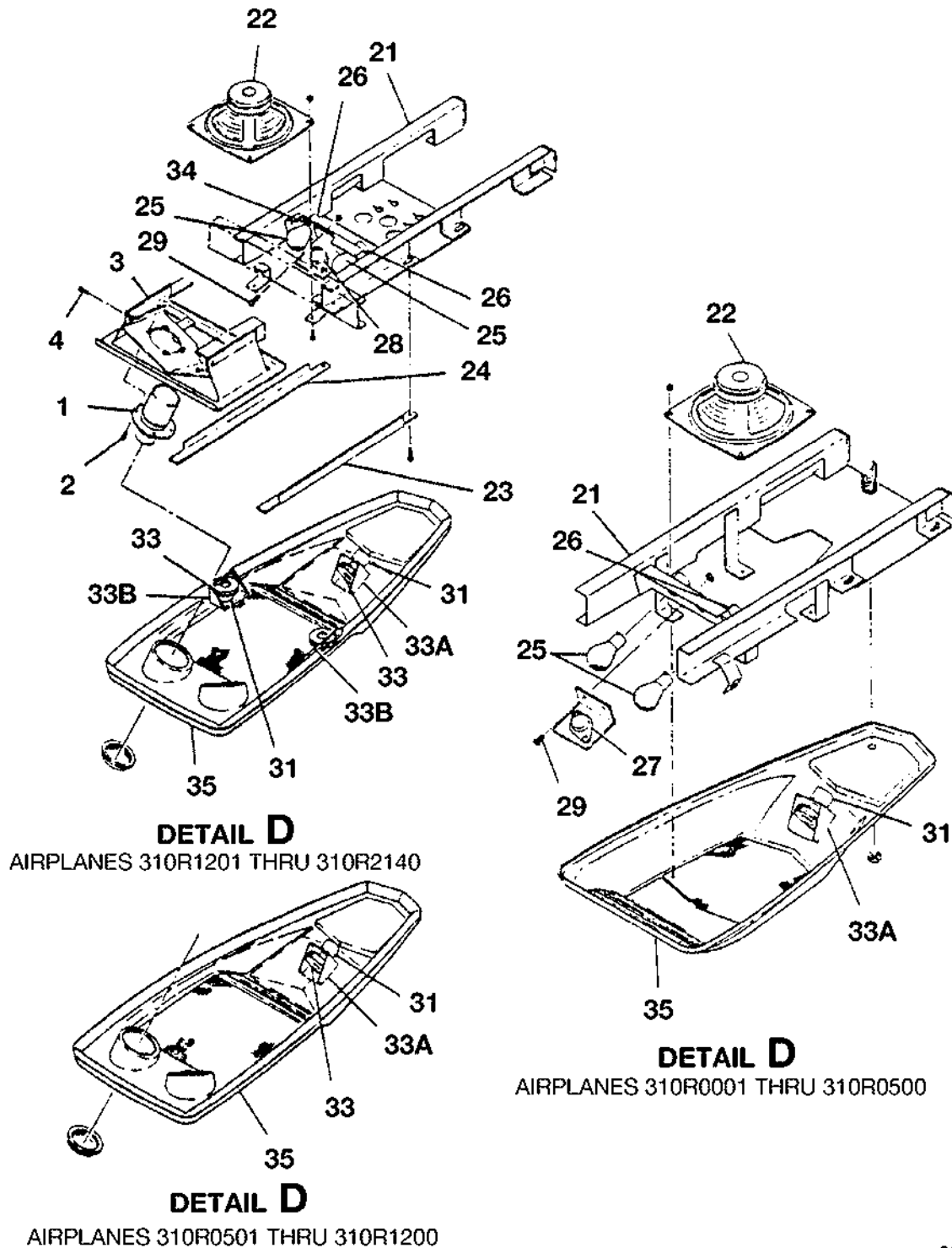
INTERIOR LIGHTING INSTALLATION FIGURE 01 (SHEET 2)
