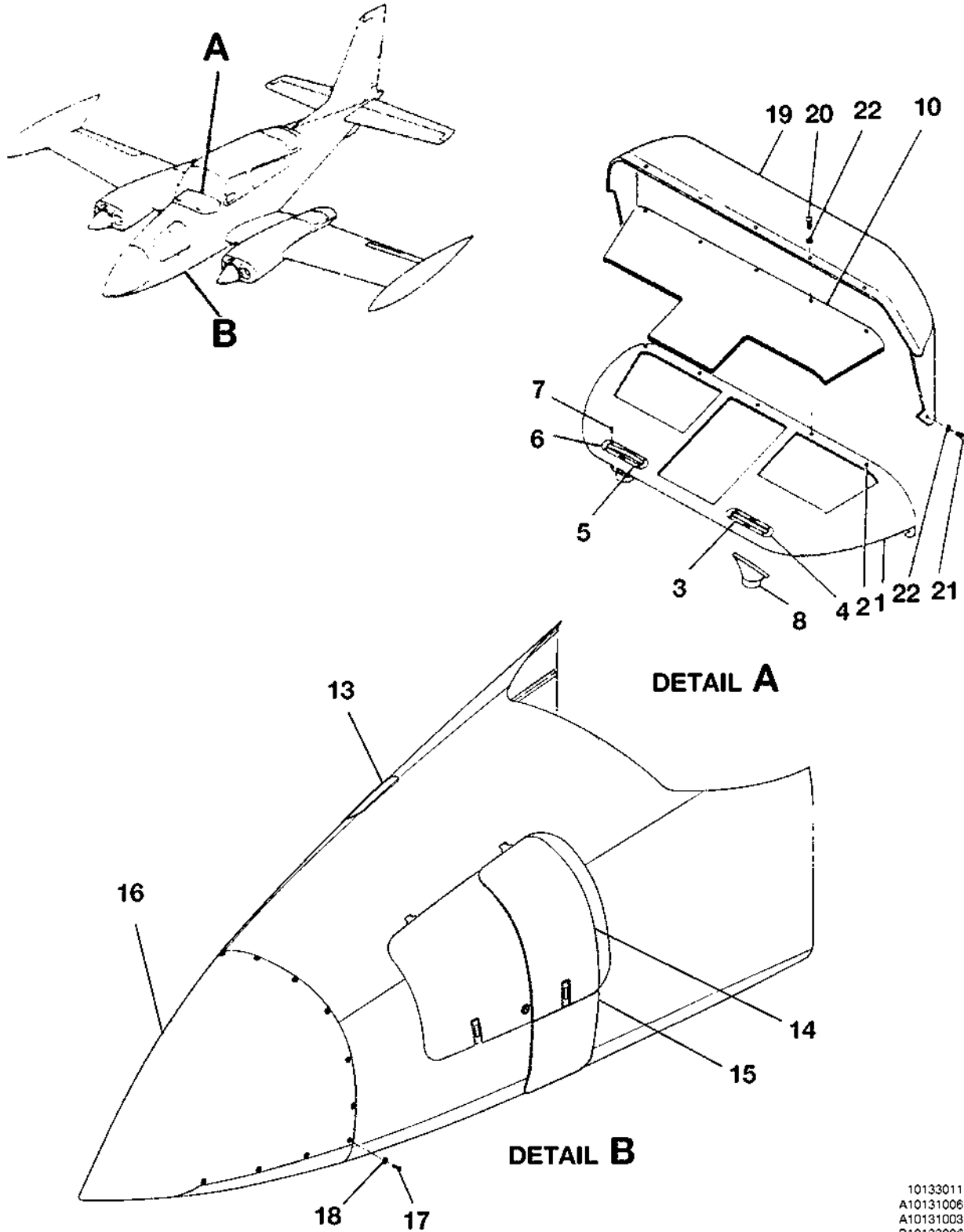
NOSE STRUCTURE COMPONENTS INSTALLATION FIGURE 05 (SHEET 1)
