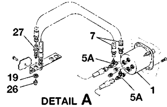
DETAIL A AIRPLANES 310R0558 THRU 310R2140
