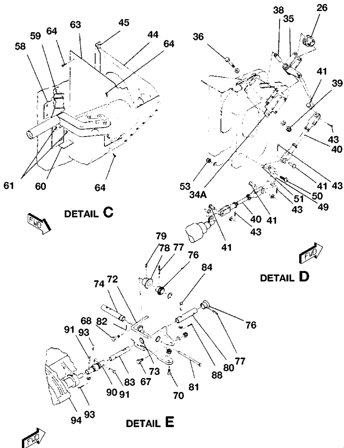
LANDING GEAR MANUAL EXTENSION MECHANISM INSTALLATION FIGURE 05 (SHEET 2)
