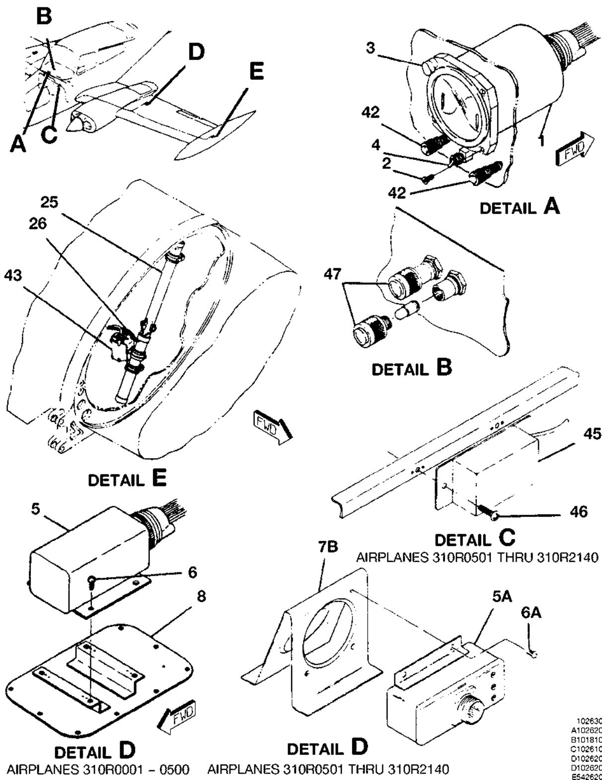
CAPACITANCE FUEL INDICATING SYSTEM COMPONENTS FIGURE 01 (SHEET 1)
