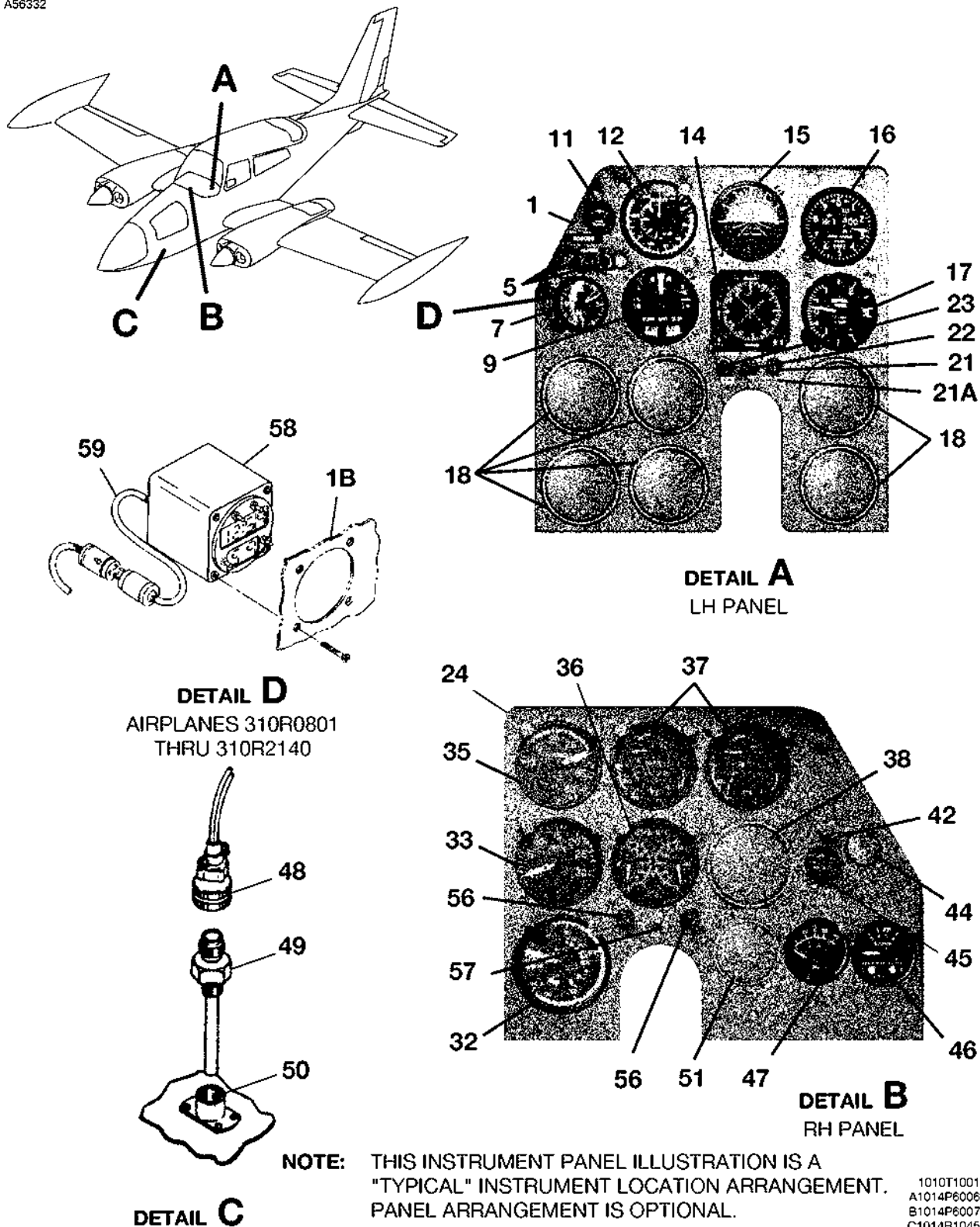
FLIGHT INSTRUMENT PANEL INSTALLATION FIGURE 02 (SHEET 1)
