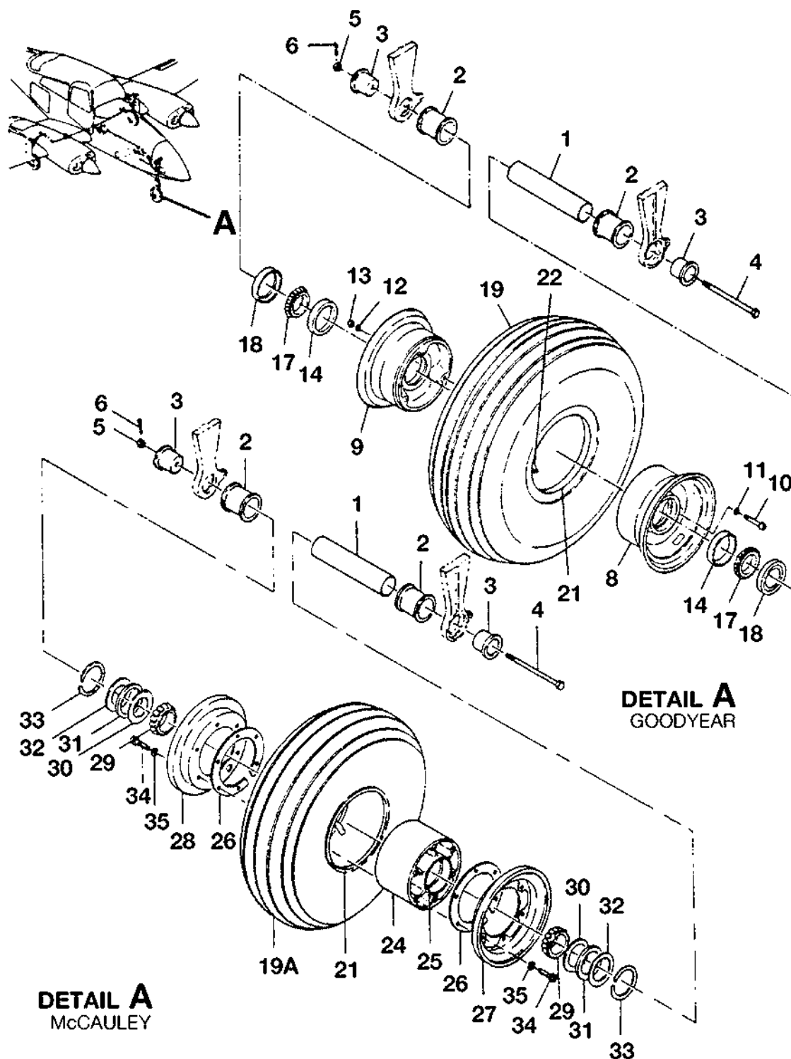
NOSE GEAR WHEEL AND TIRE INSTALLATION FIGURE 01 (SHEET 1)
