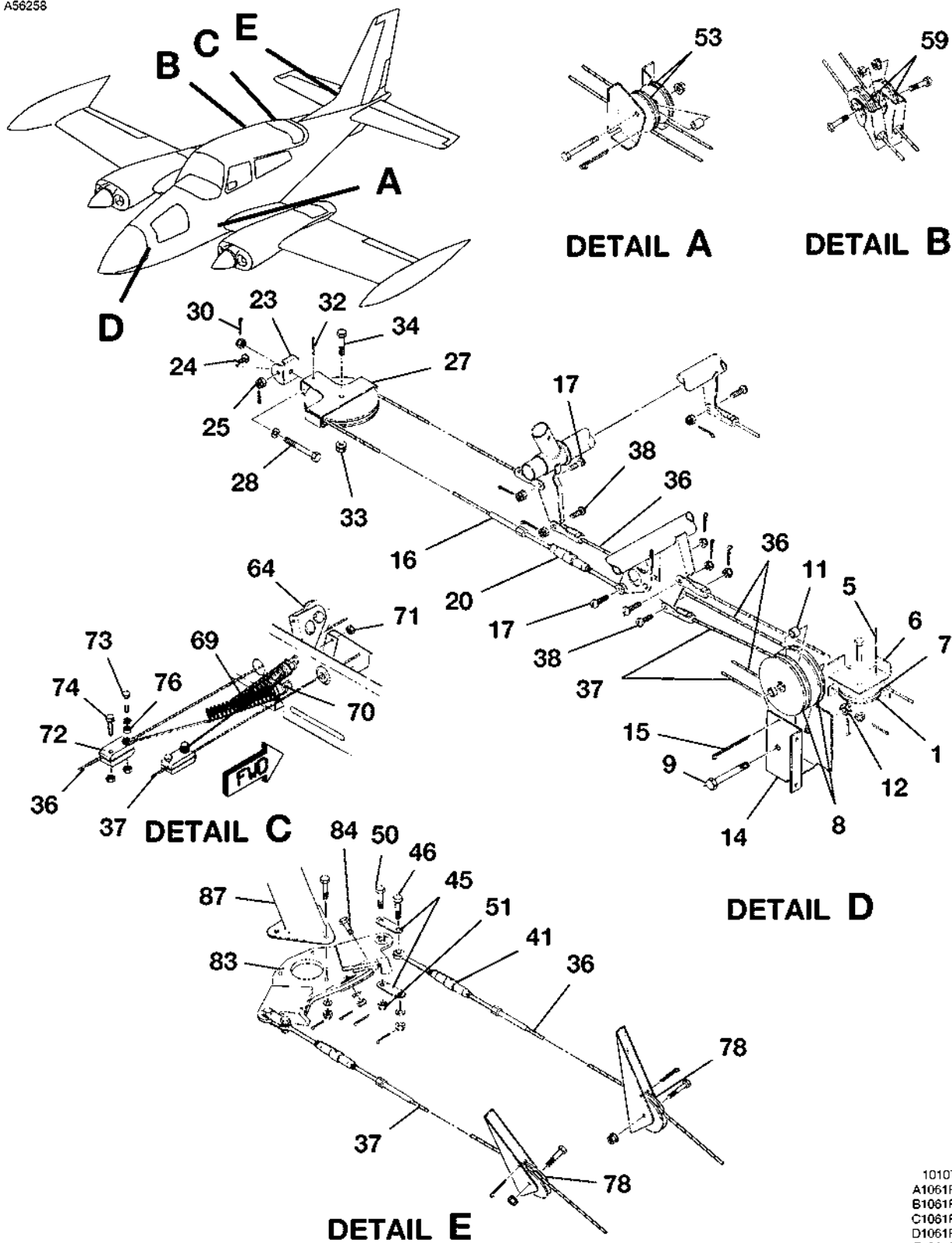
RUDDER CONTROL INSTALLATION FIGURE 01 (SHEET 1)
