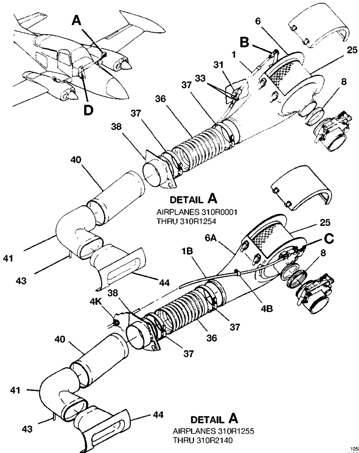
ENGINE INDUCTION AIR SYSTEM FIGURE 01 (SHEET 1)
