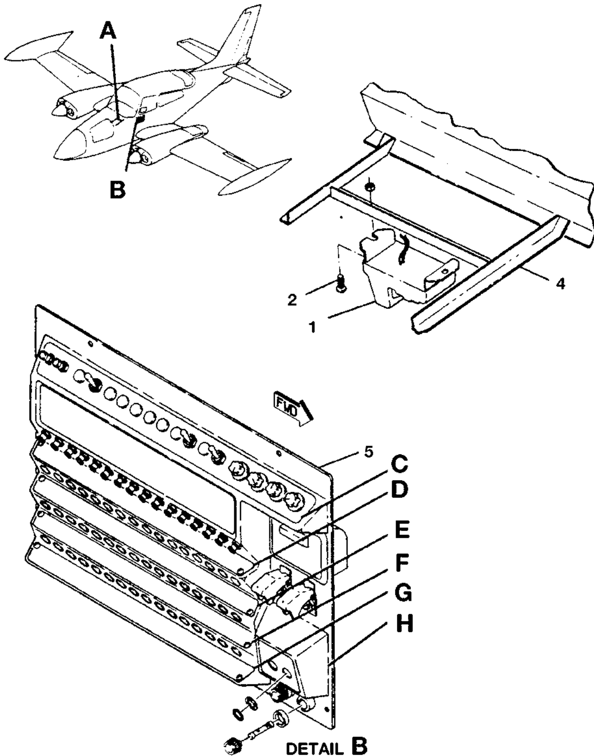
CIRCUIT BREAKER ELECTROLUMINESCENT AND SILKSCREEN FIGURE 04 (SHEET 1)
