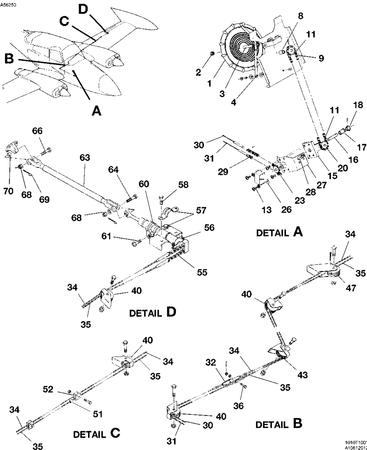
AILERON TRIM CONTROL SYSTEM FIGURE 02 (SHEET 1)
