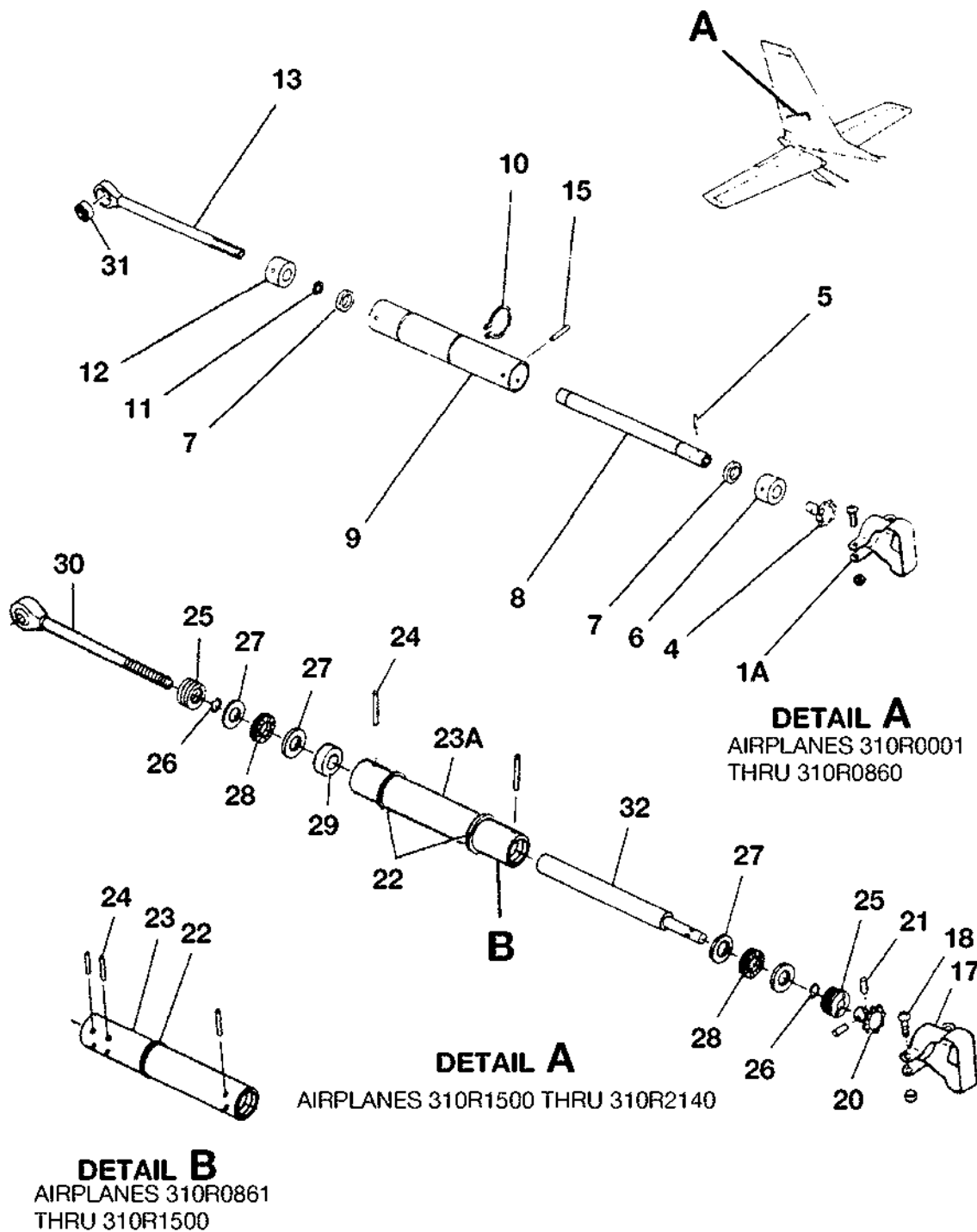
RUDDER TRIM TAB ACTUATOR ASSEMBLY FIGURE 02 (SHEET 1)
