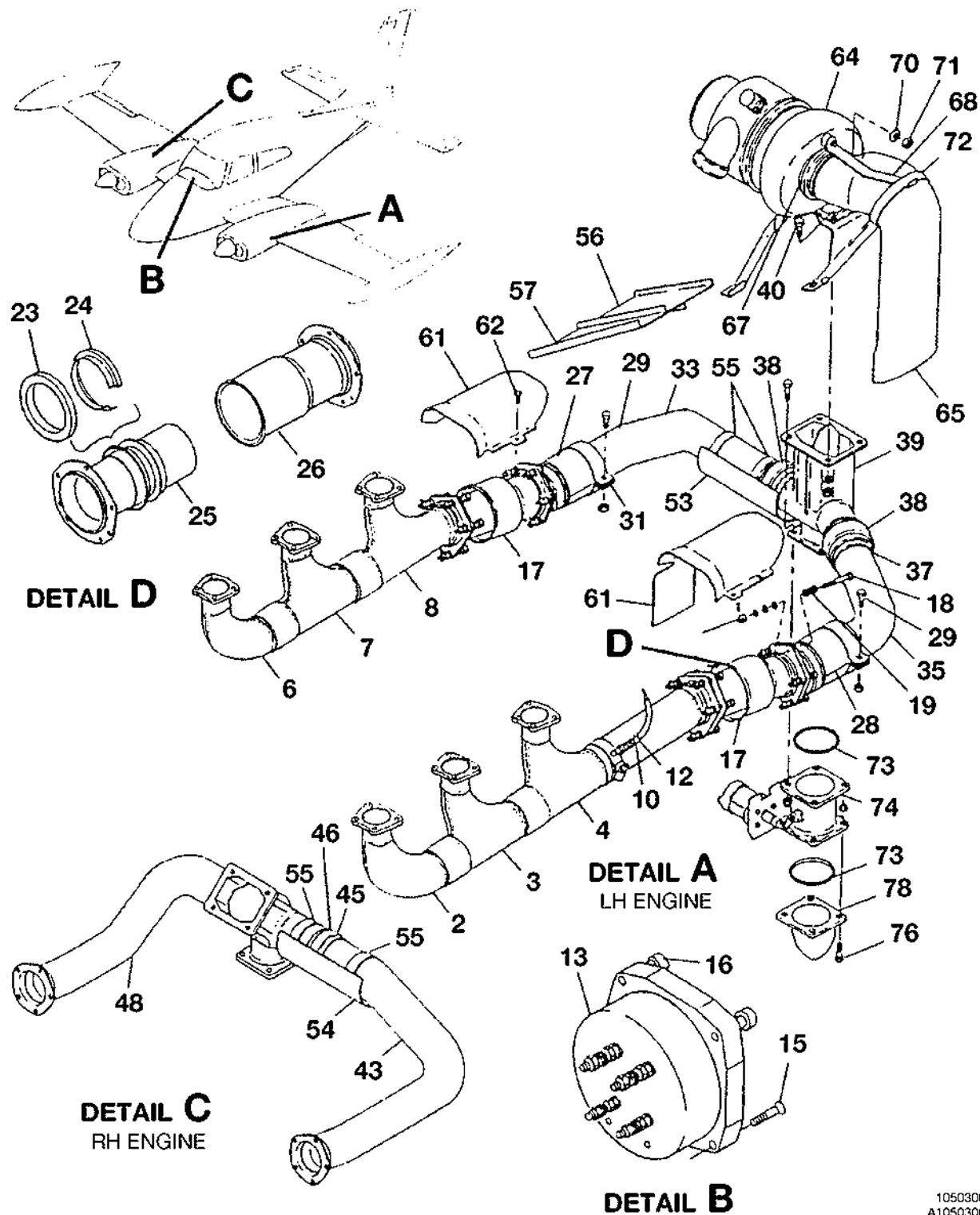
ENGINE EXHAUST SYSTEM-TURBOCHARGED FIGURE 02 (SHEET 1)
