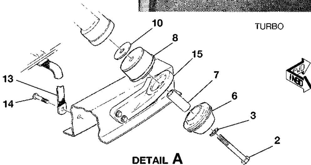
ENGINE INSTALLATION FIGURE 01 (SHEET 1)
