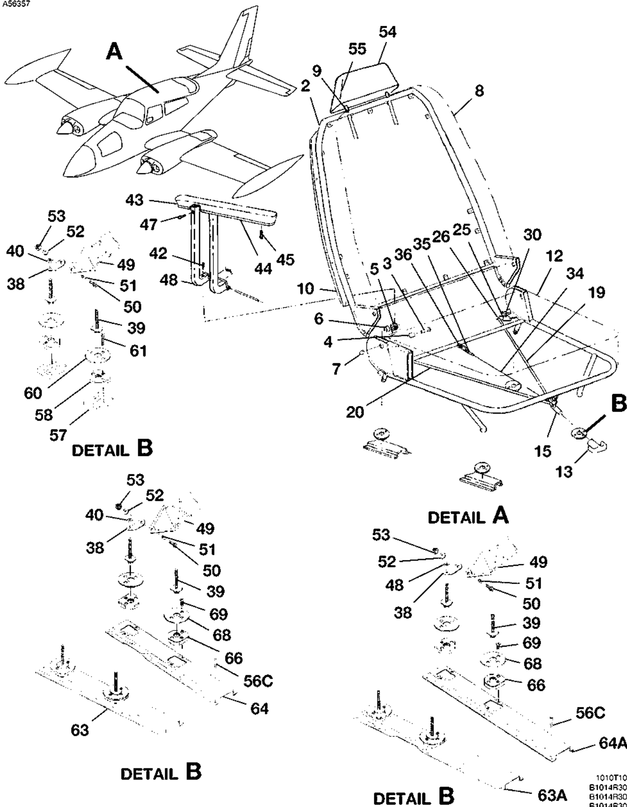
AFT SINGLE SEAT INSTALLATION FIGURE 03 (SHEET 1)
