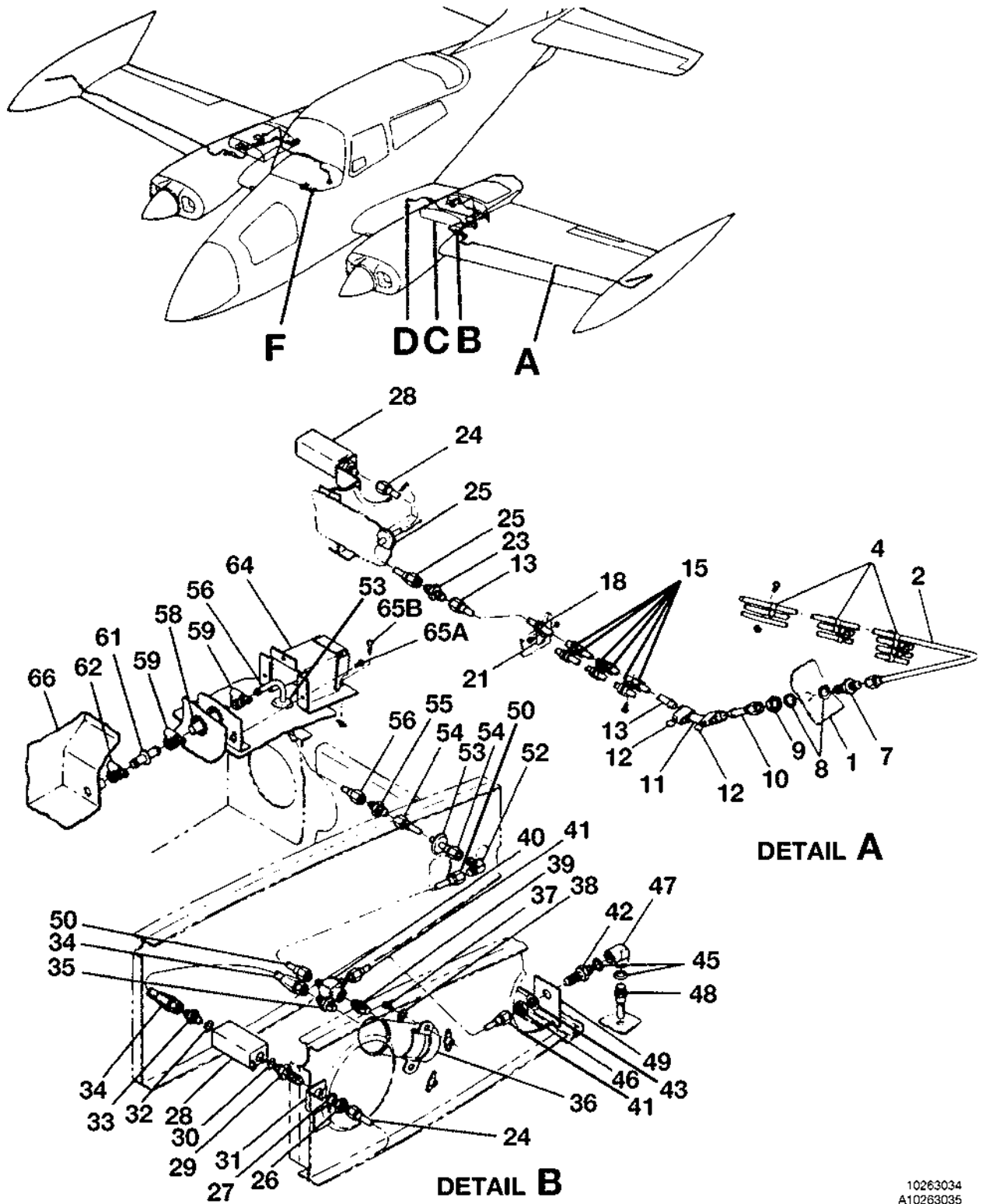
WING LOCKER FUEL SYSTEM FIGURE 02 (SHEET 1)
