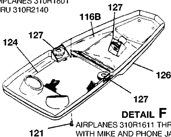
UPHOLSTERY TRIM INSTALLATION FIGURE 01 (SHEET 3)
