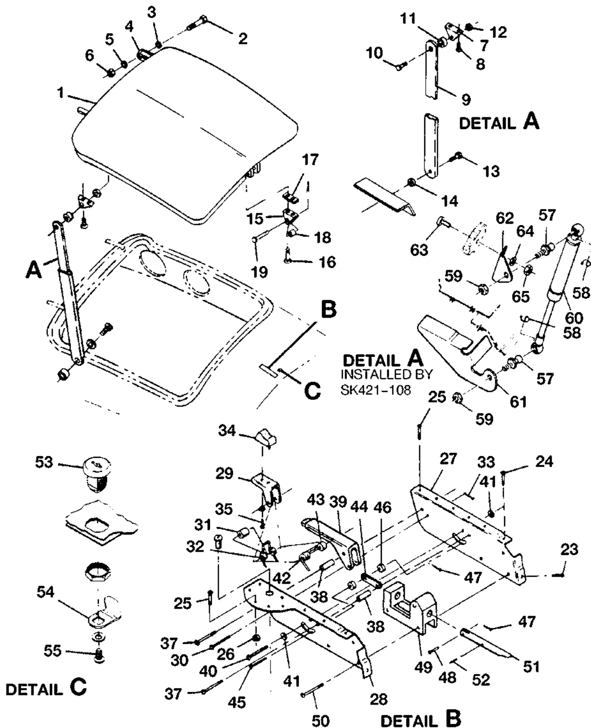
NACELLE BAGGAGE DOOR AND LATCH INSTALLATION FIGURE 03 (SHEET 1)
