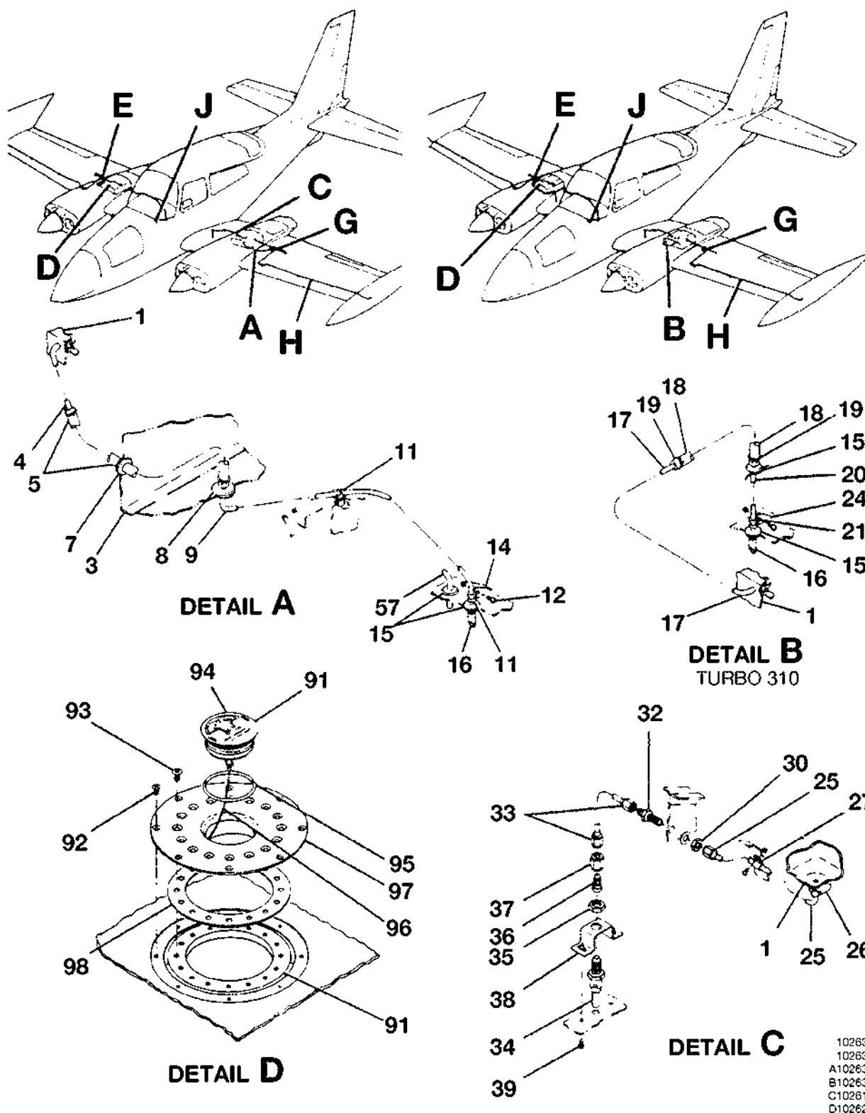
WING LOCKER FUEL SYSTEM FIGURE 01 (SHEET 1)
