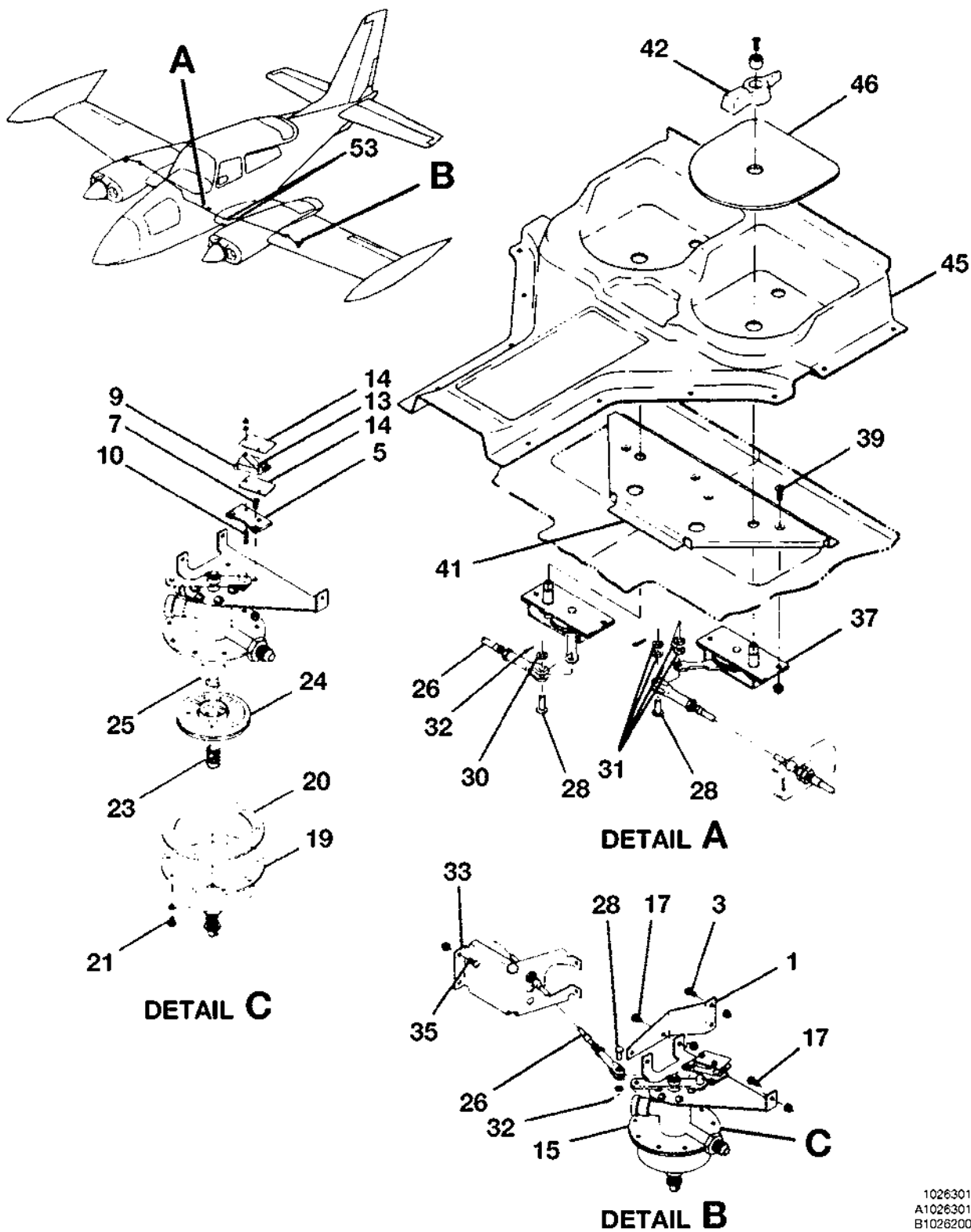
FUEL SELECTOR VALVE AND CONTROLS INSTALLATION FIGURE 02 (SHEET 1)
