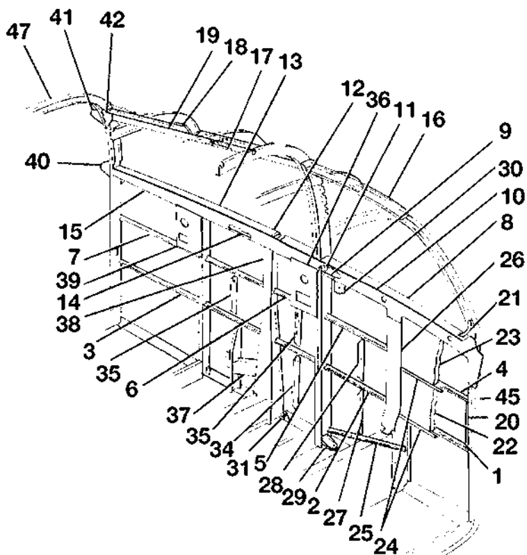
LEFT CABIN SIDE STRUCTURE ASSY FIGURE 01 (SHEET 1)
