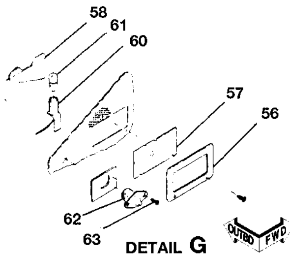
EXTERIOR LIGHTING INSTALLATION FIGURE 01 (SHEET 2)
