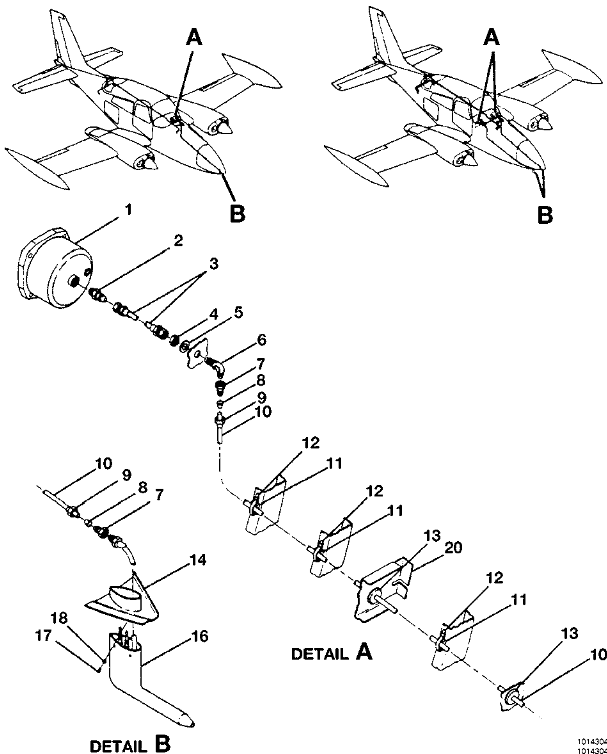
PITOT SYSTEM FIGURE 02 (SHEET 1)
