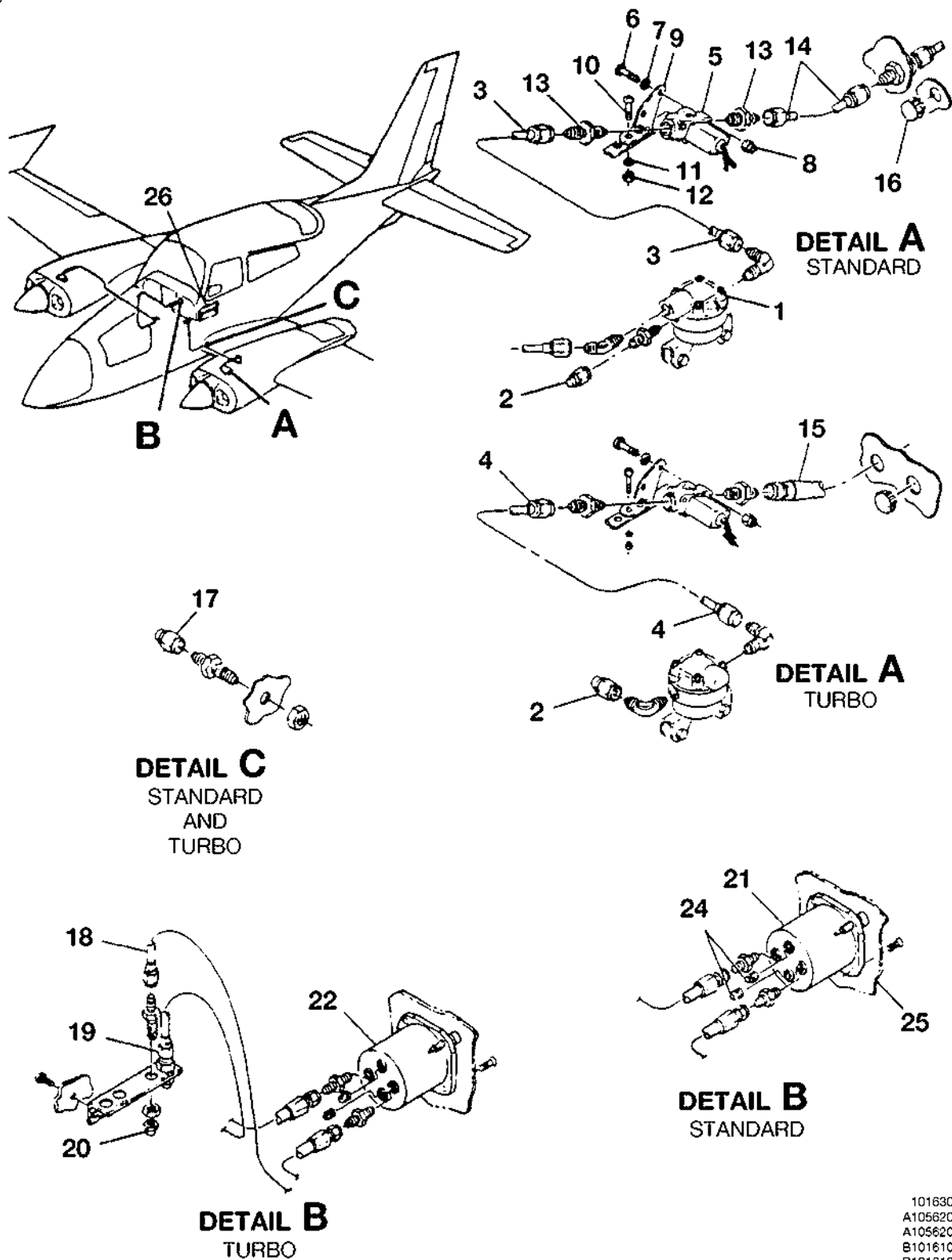
ELECTRONIC FUEL FLOW INDICATING SYSTEM - 310 AND T310 FIGURE 02 (SHEET 1)
