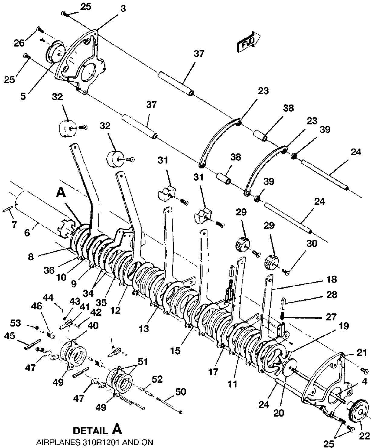
ENGINE CONTROL QUADRANT FIGURE 01 (SHEET 1)
