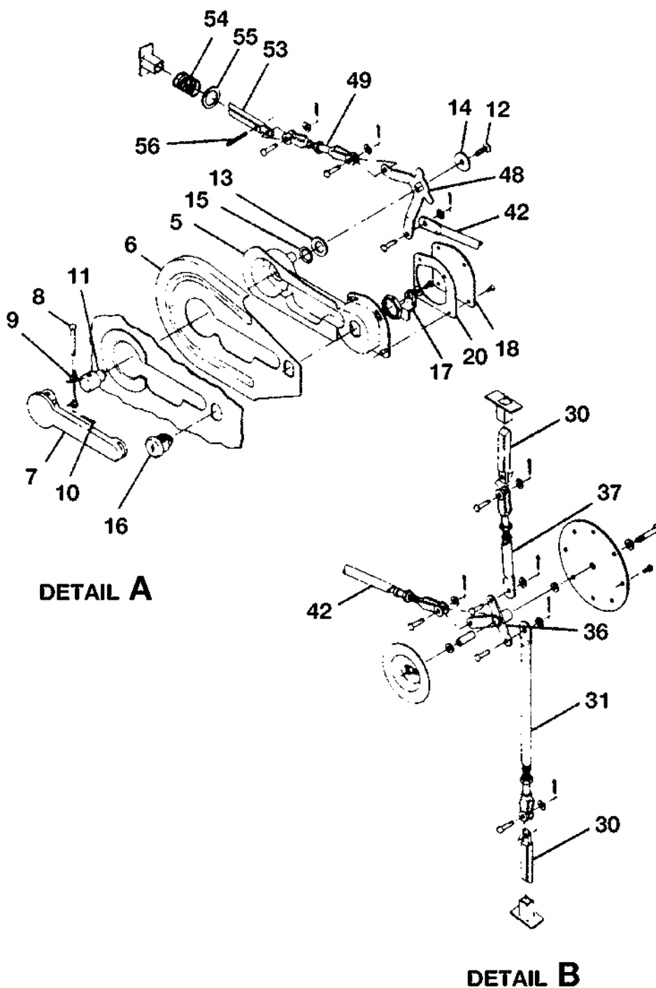
BAGGAGE DOOR INSTALLATION - LARGE FIGURE 02 (SHEET 2)
