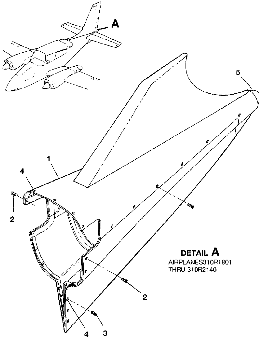
STINGER INSTALLATION FIGURE 06 (SHEET 1)
