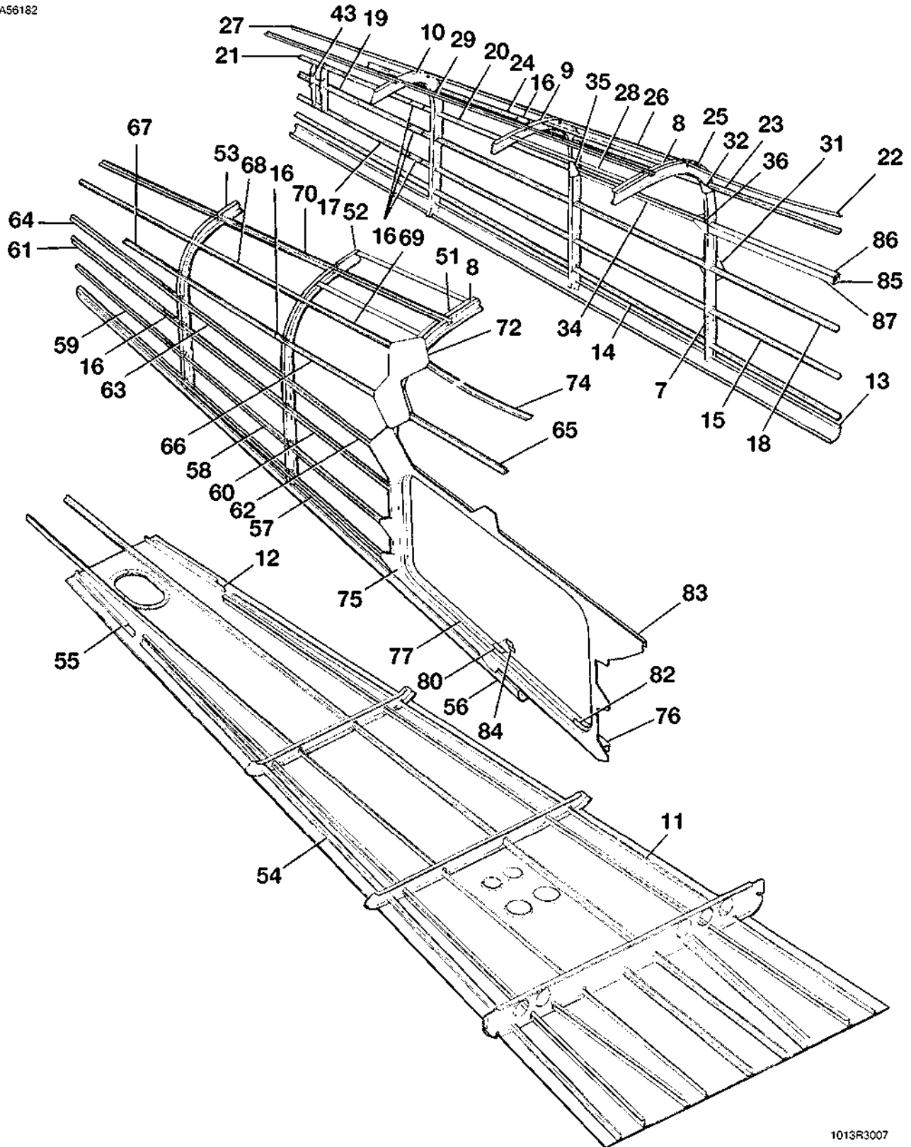
FUSELAGE AFT SECTION STRUCTURE ASSEMBLY WITH LARGE BAGGAGE DOOR FIGURE 02 (SHEET 1)
