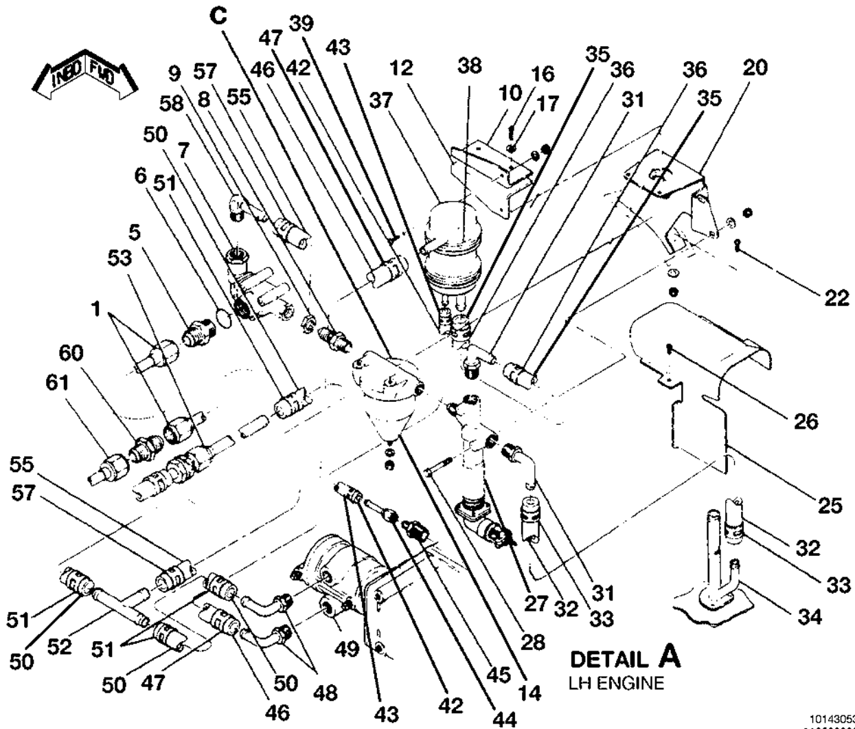
ENGINE COMPARTMENT DEICE COMPONENTS FIGURE 03 (SHEET 1)
