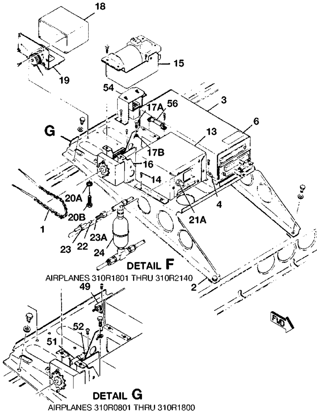
400B NAV-O-MATIC AUTOPILOT SYSTEM FIGURE 02 (SHEET 3)
