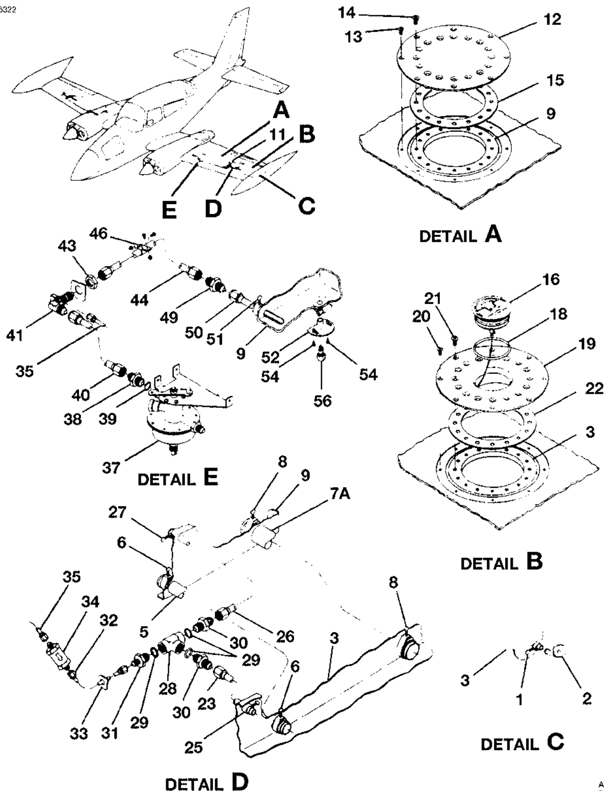
AUXILIARY FUEL SYSTEM COMPONENTS 63 GALLON CAPACITY FIGURE 02 (SHEET 1)
