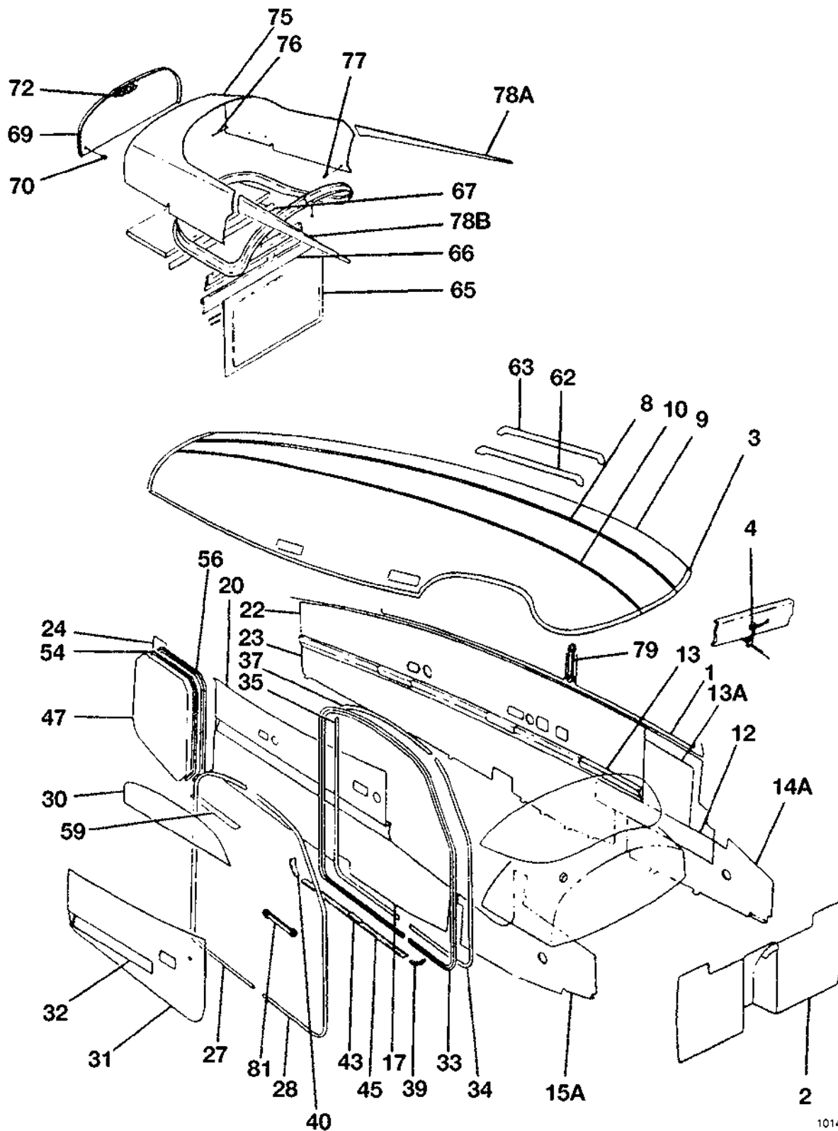
UPHOLSTERY INSTALLATION FIGURE 01 (SHEET 1)
