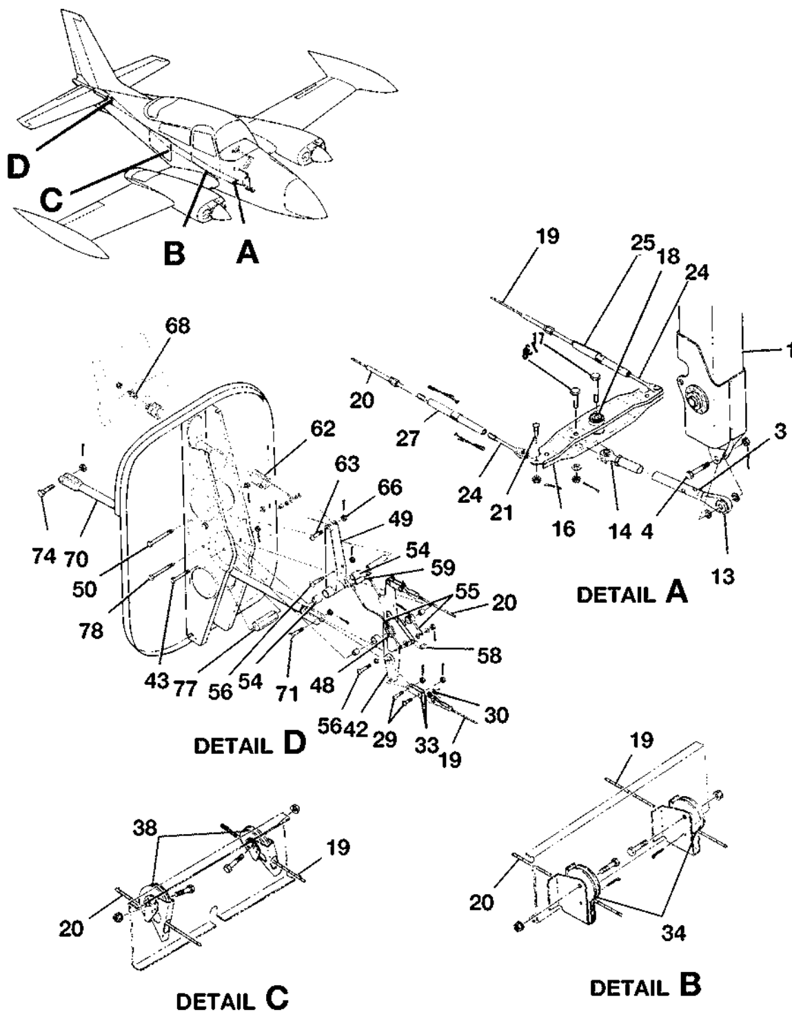
ELEVATOR CONTROL SYSTEM FIGURE 01 (SHEET 1)
