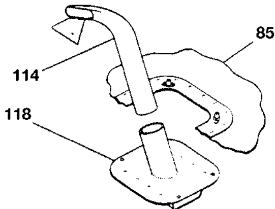
DETAIL C AIRPLANES 310R0001 THRU 310R0500
