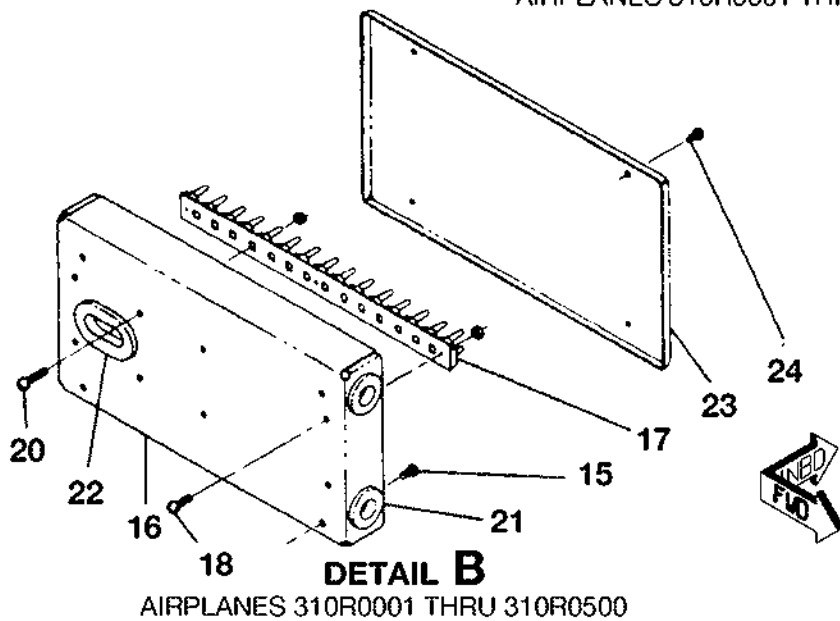
JUNCTION BOX AND WING TO FUSELAGE ELECTRICAL CONNECTORS INSTALLATION FIGURE 01 (SHEET 1)
