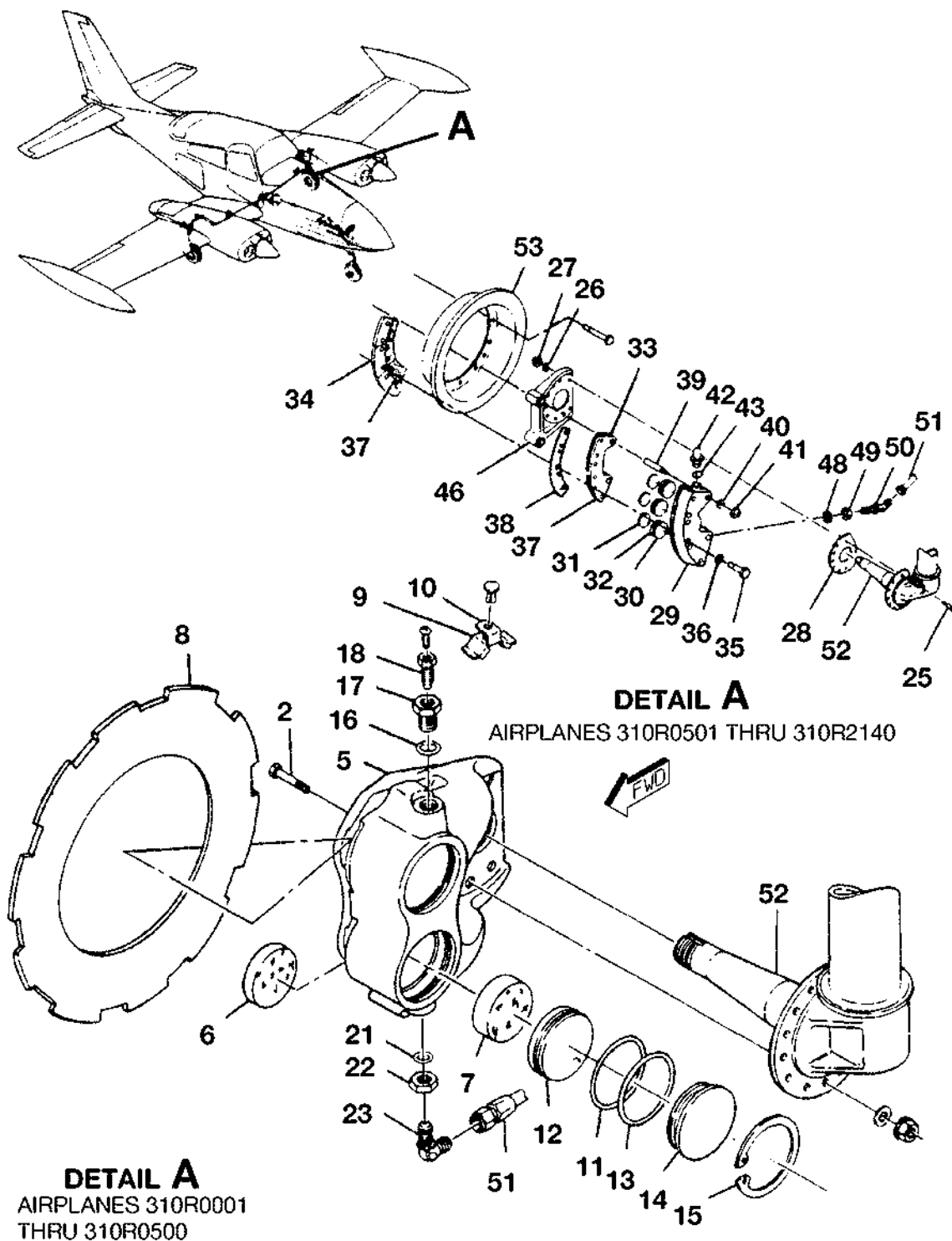
MAIN GEAR BRAKE INSTALLATION FIGURE 03 (SHEET 1)
