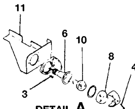
DETAIL A NAVIGATION LIGHT INSTL.
