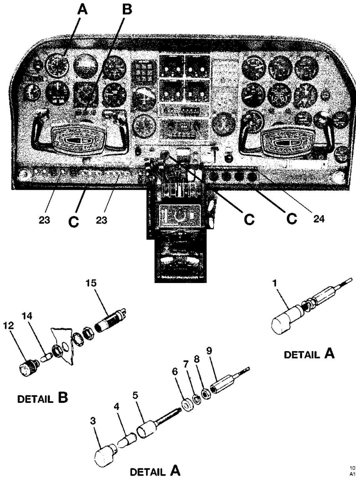
INSTRUMENT PANEL LIGHTING FIXTURES FIGURE 02 (SHEET 1)
