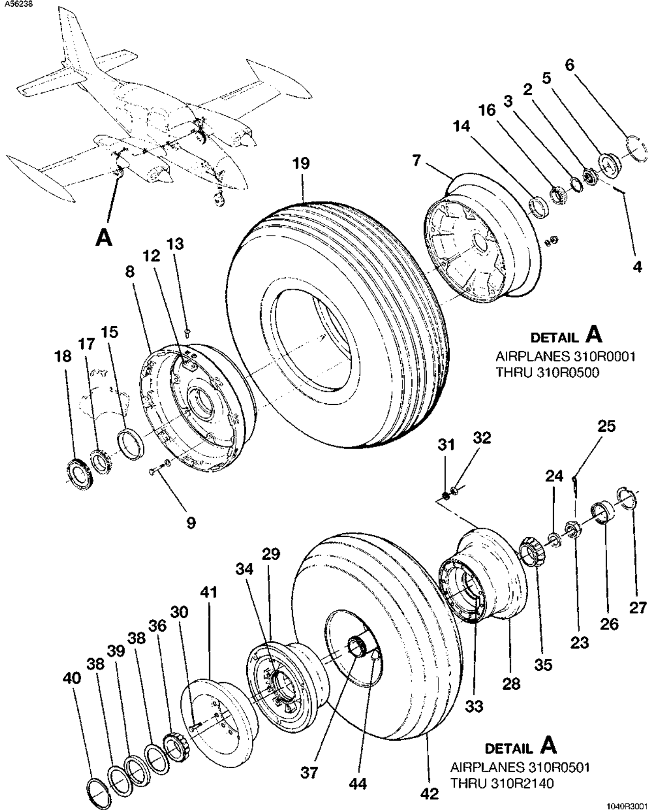
MAIN GEAR WHEEL AND TIRE INSTALLATION FIGURE 01 (SHEET 1)
