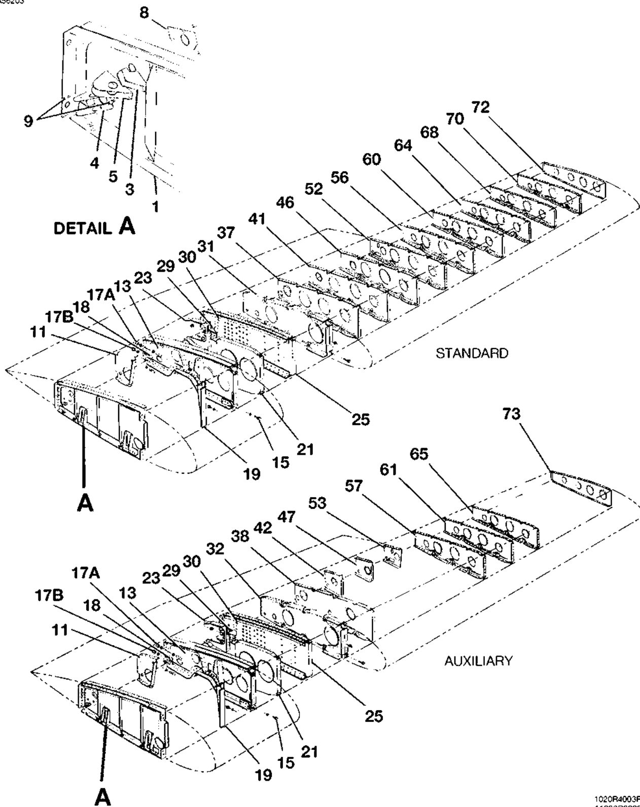
WING INTERSPAR RIBS INSTALLATION FIGURE 03 (SHEET 1)
