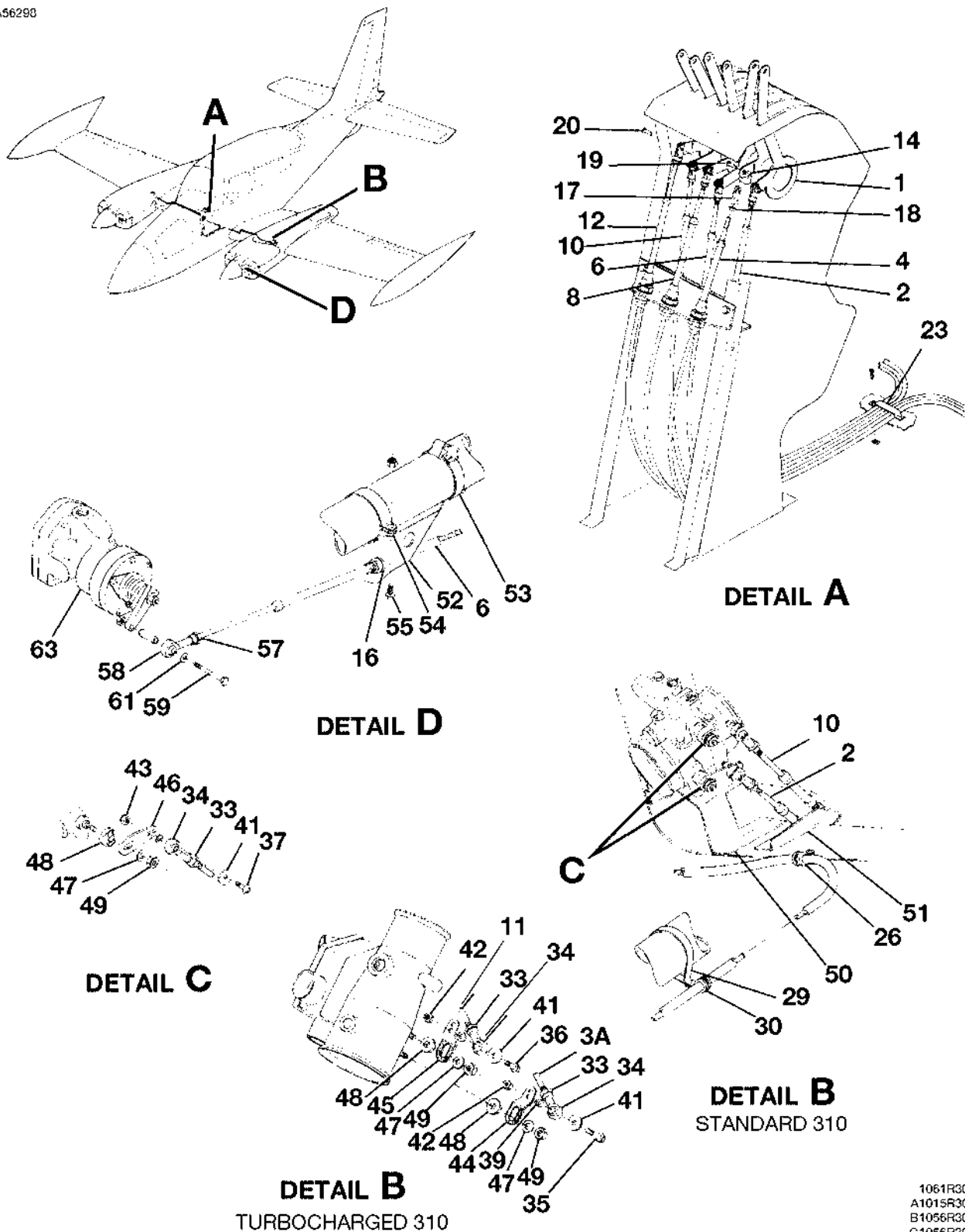
ENGINE CONTROL SYSTEM FIGURE 01 (SHEET 1)
