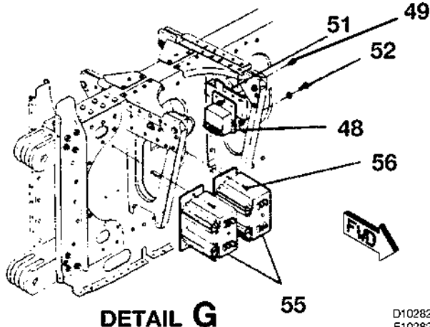
DC POWER SYSTEM INSTALLATION FIGURE 02 (SHEET 2)
