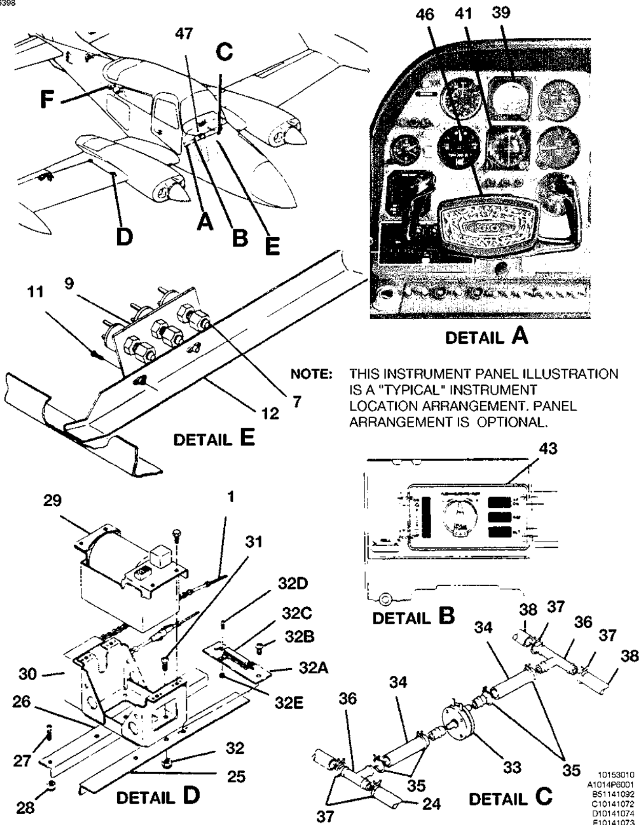
400B NAV-O-MATIC AUTOPILOT SYSTEM FIGURE 02 (SHEET 1)
