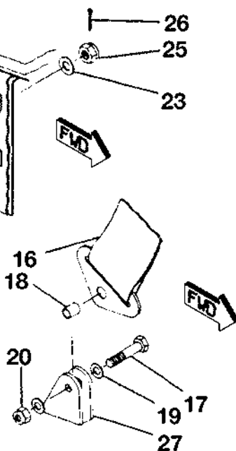
DETAIL B AIRPLANES 310R0001 THRU 310R0500
