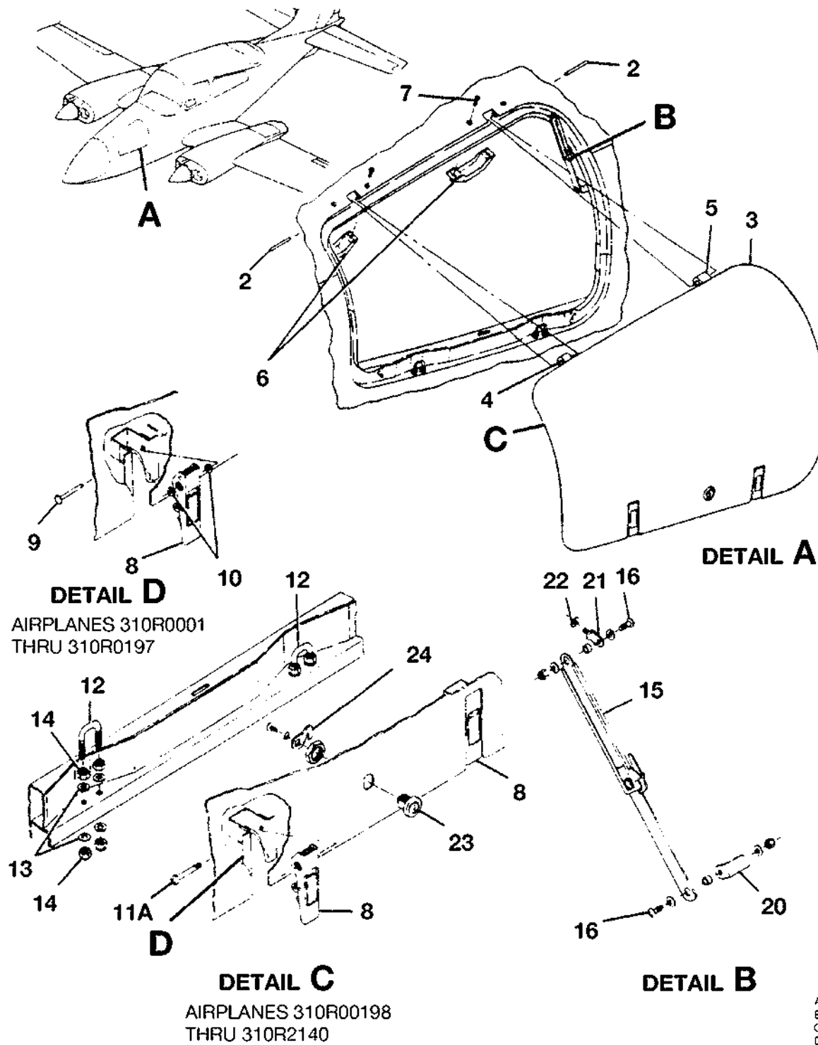
NOSE BAGGAGE DOOR INSTALLATION FIGURE 03 (SHEET 1)
