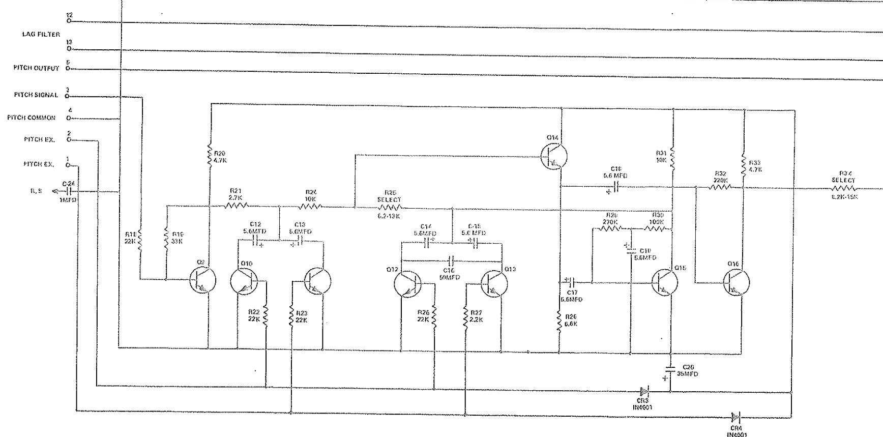
FIGURE 4-5A Cont: 1C515 AMPLIFIER
