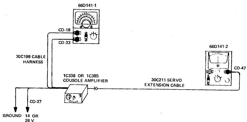
FIGURE 4-2 CENTURY II TEST SET-UP
