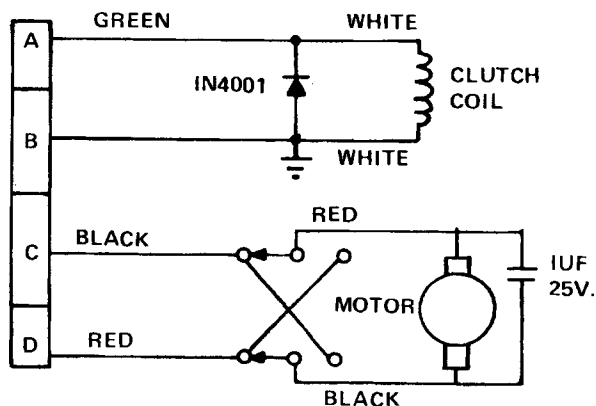
SCHEMATIC - A
