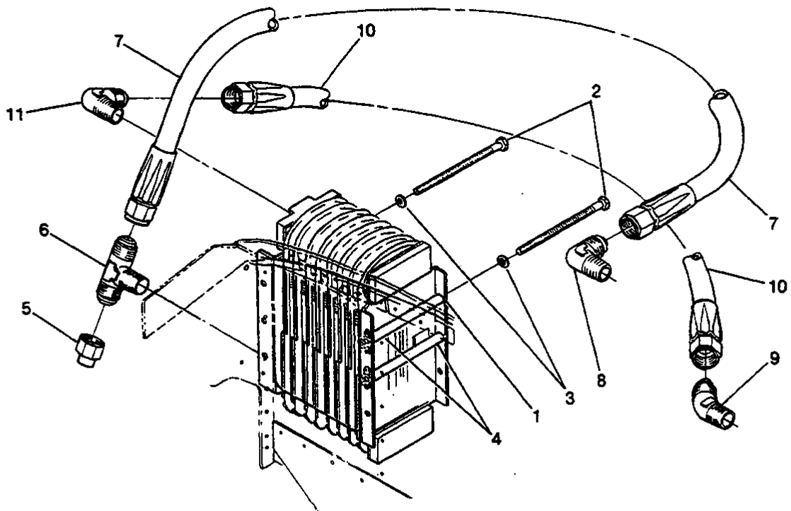
Figure 68B. Oil Cooler Installation
