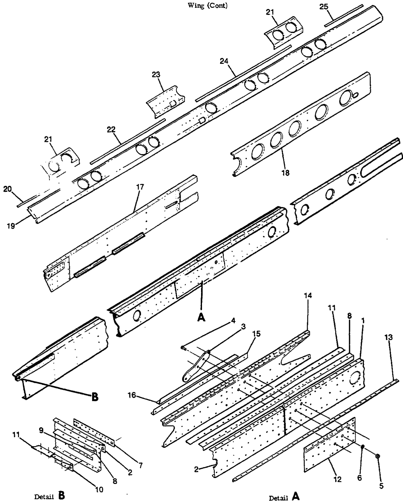
Figure 8A. Wing Spar Assembly - Integral Fuel Cell
