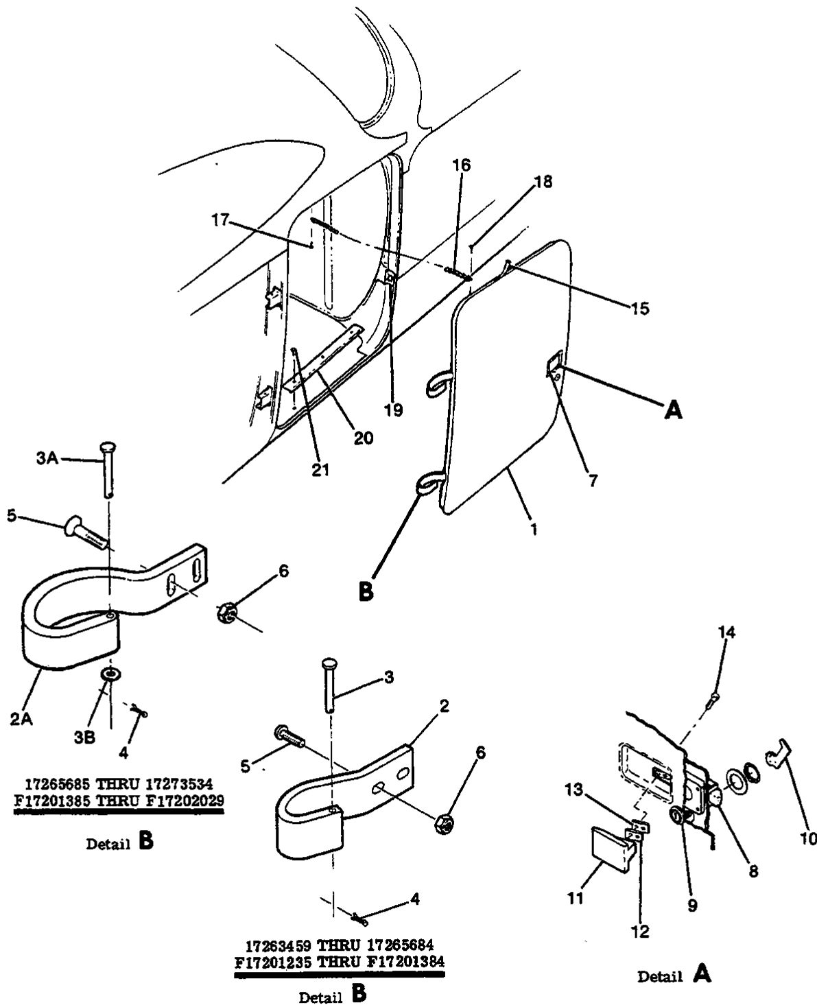
Figure 49. Baggage Door Installation
