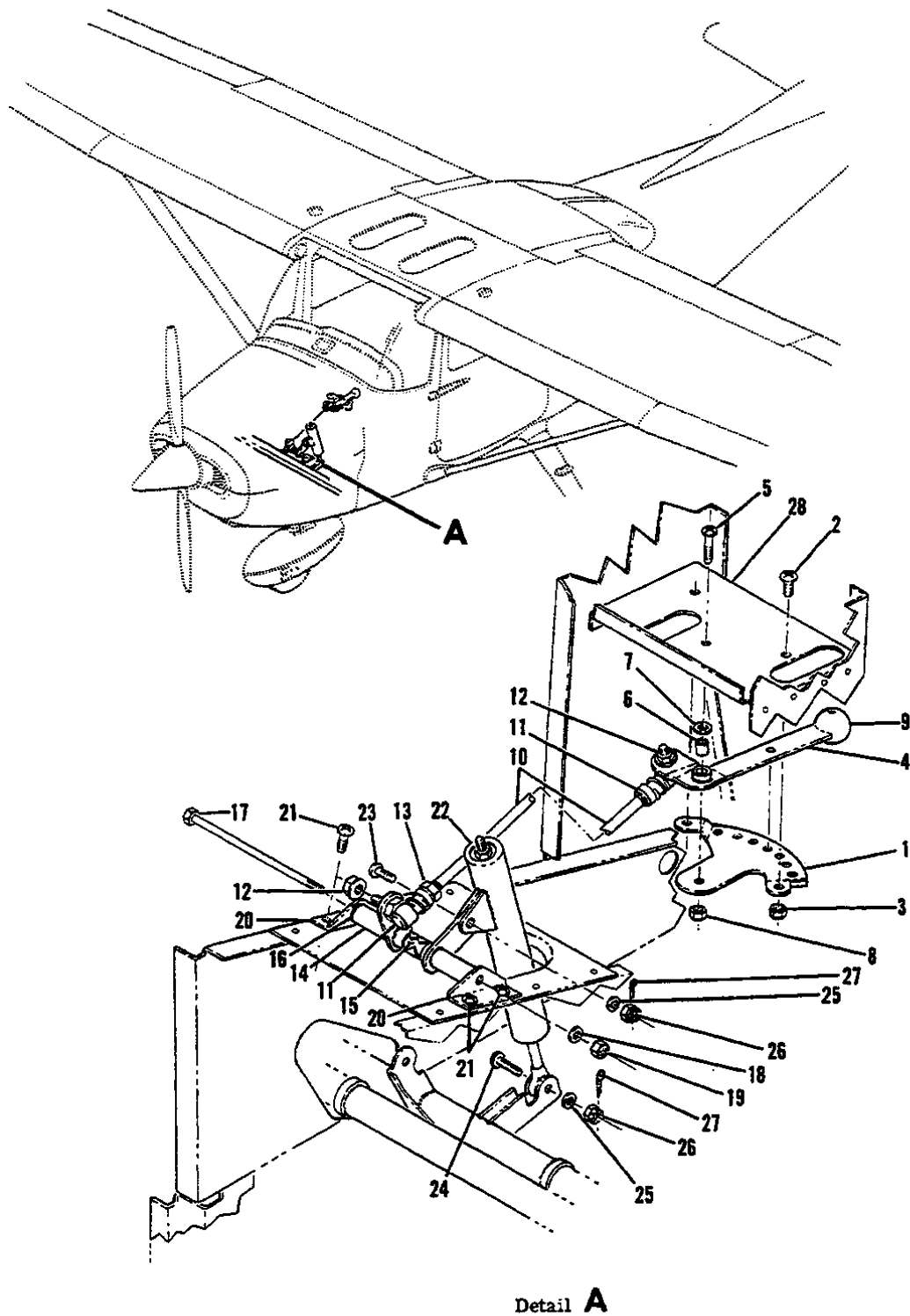
172 SERIAL 17267585 & ON F172 SERIAL F17201515 & ON Figure 83B. Rudder Trim System
