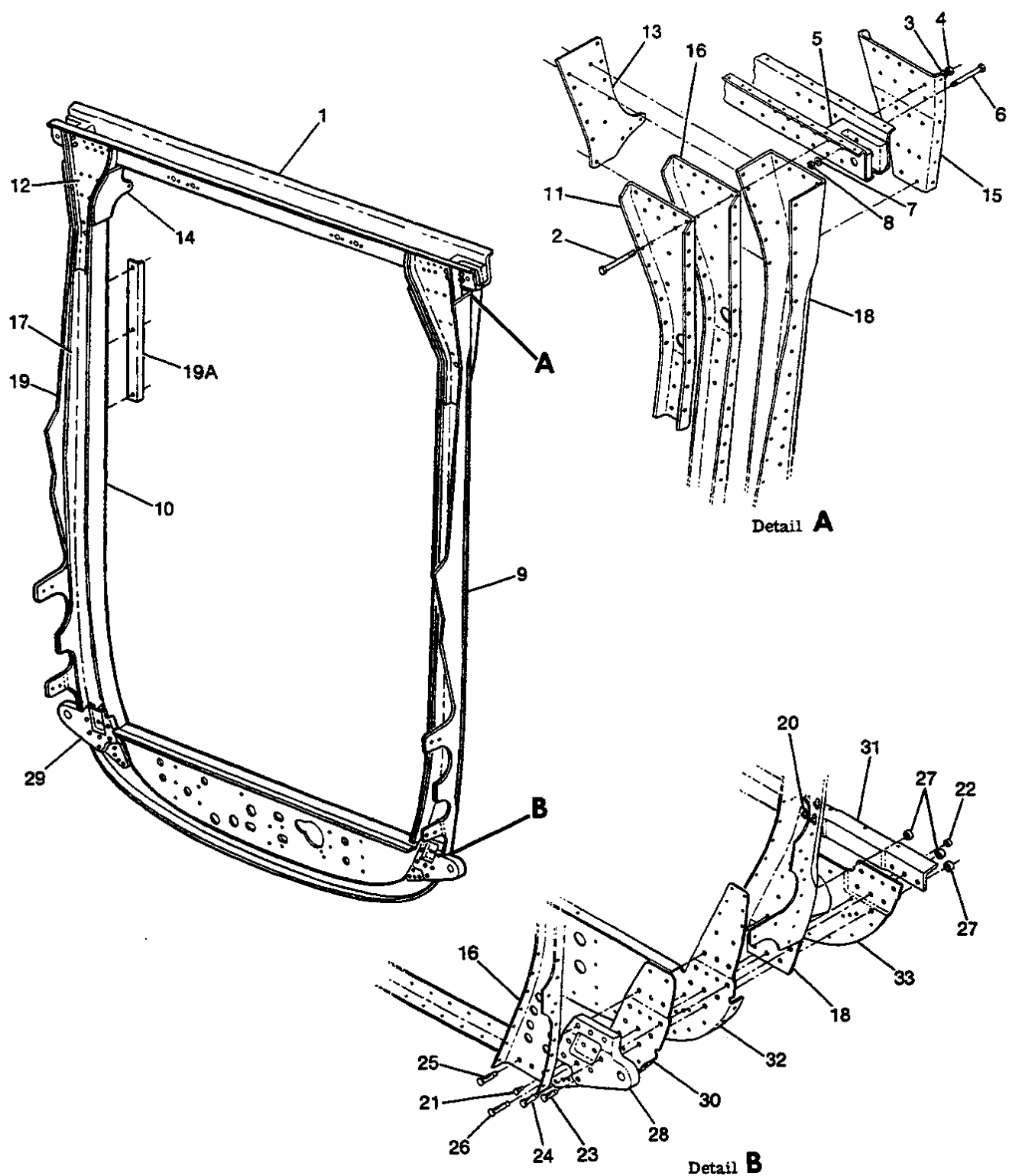
172 SERIAL 17272885 & ON F172 SERIAL F17201910 & ON Figure 24B. Front Doorpost Bulkhead Assembly
