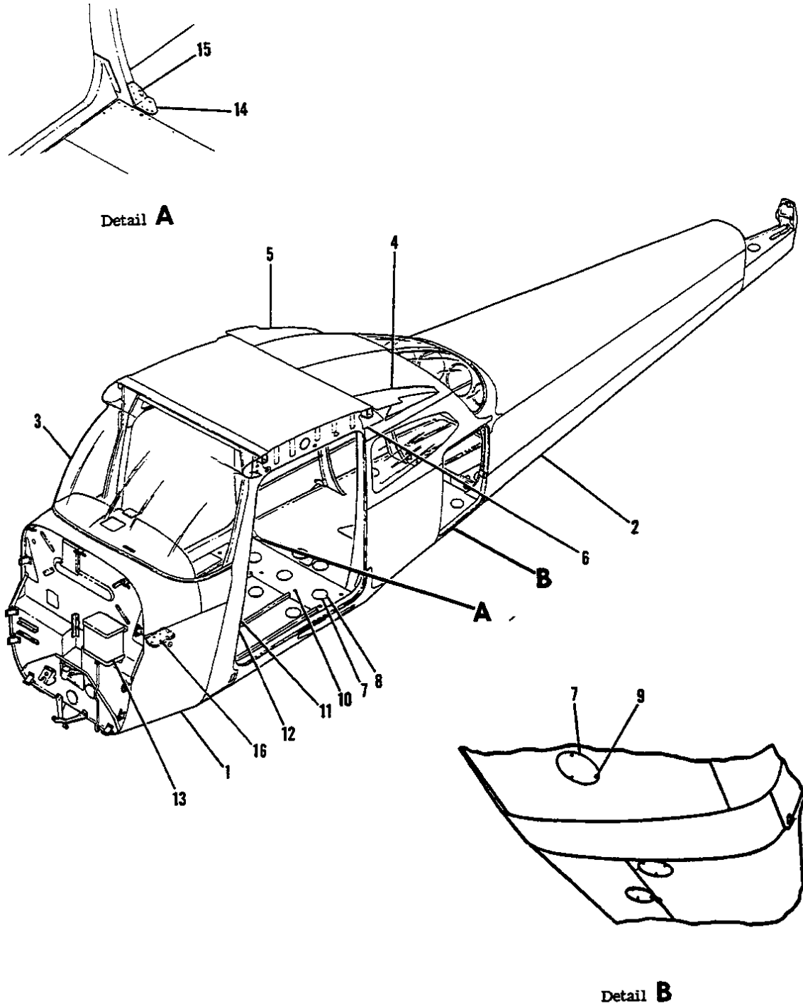
Figure 21. Fuselage Assembly
