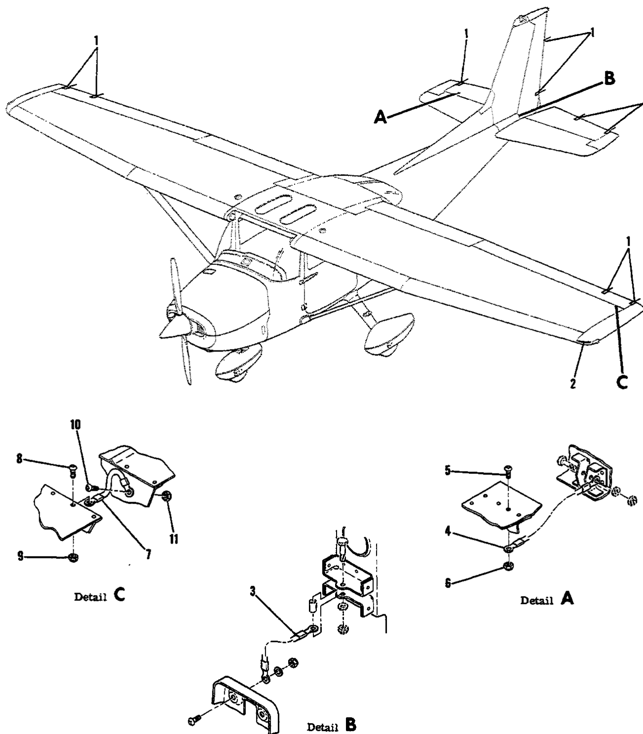
172 SERIAL 17265685 & ON F172 SERIAL F17201385 & ON Figure 63A. Static Discharger Installation
