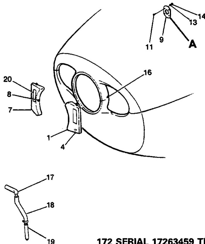
Figure 72. Winterization Equipment
