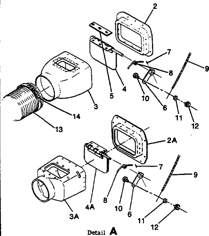
Figure 74. Cabin Heating & Defrosting Installation
