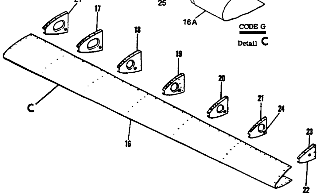
Figure 7. Wing Leading Edge Assembly
