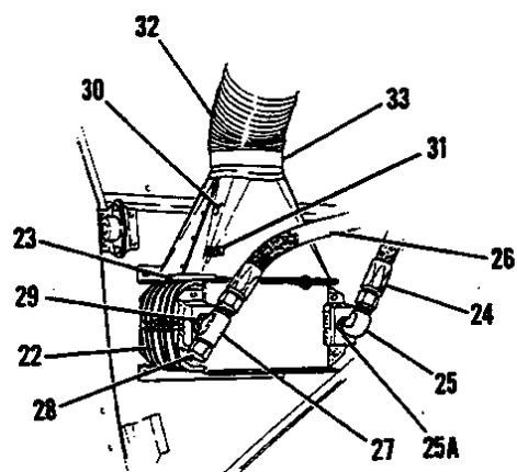
OIL COOLER
