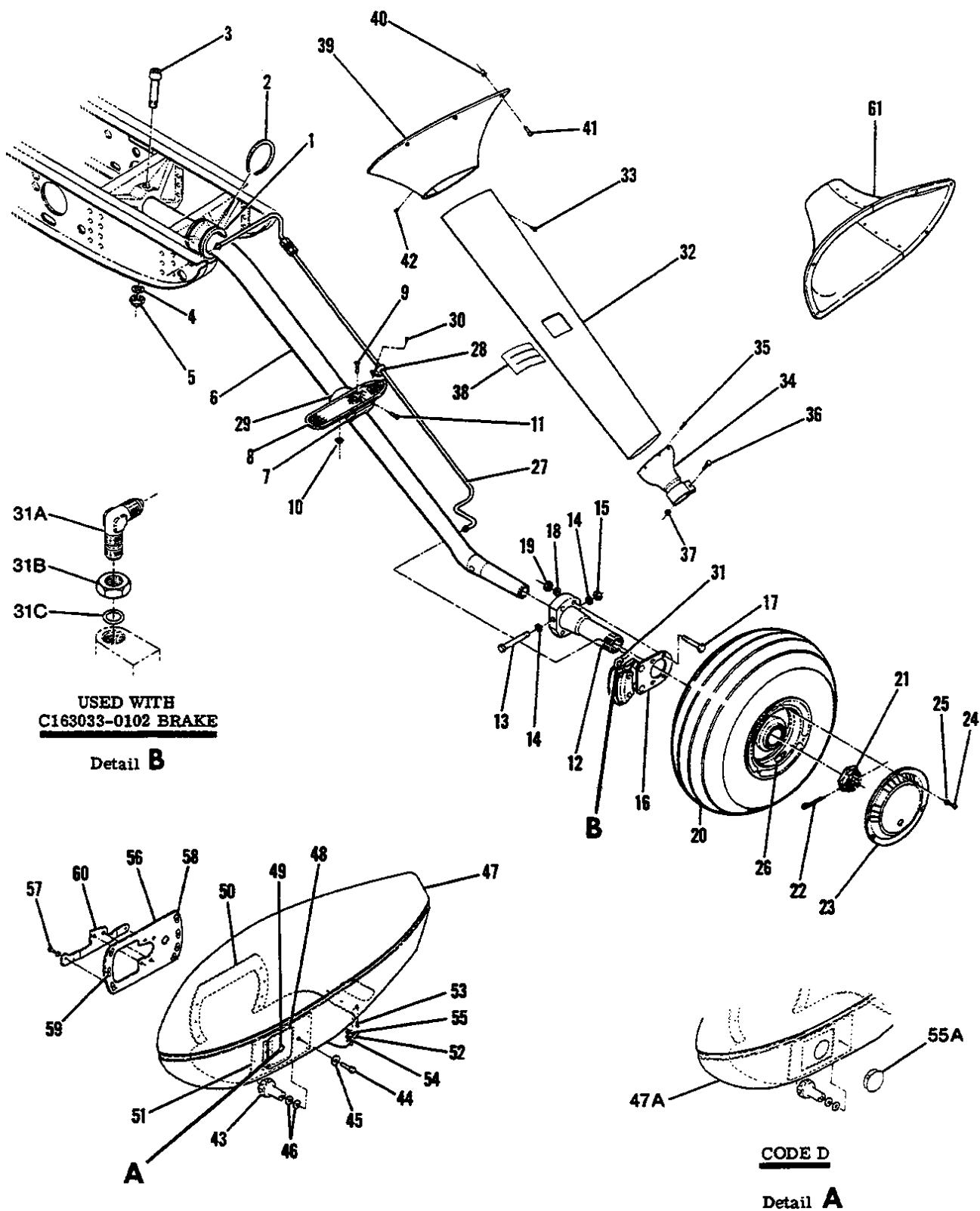
Figure 42. Main Landing Gear Installation
