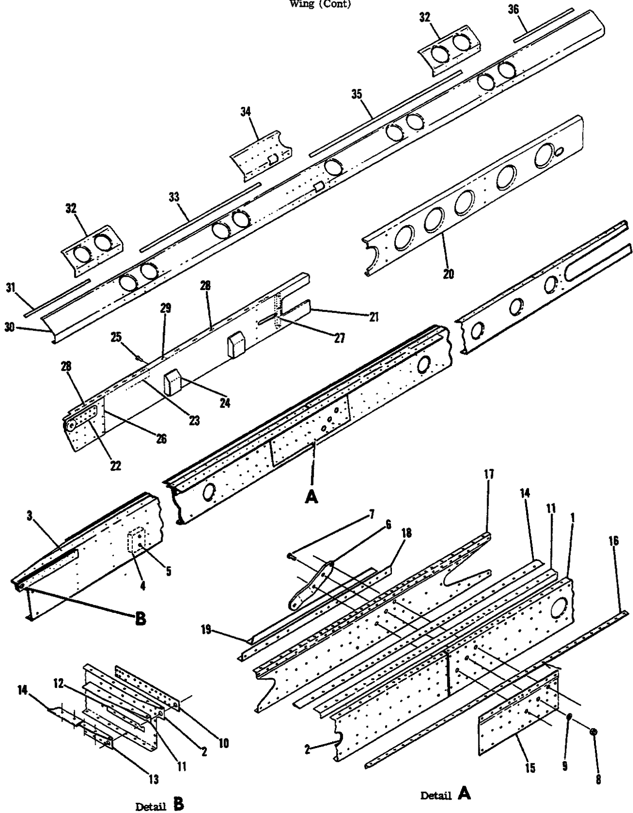
Figure 8. Wing Spar Assemblies
