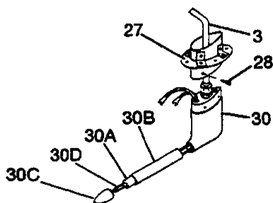
HEATED PITOT
