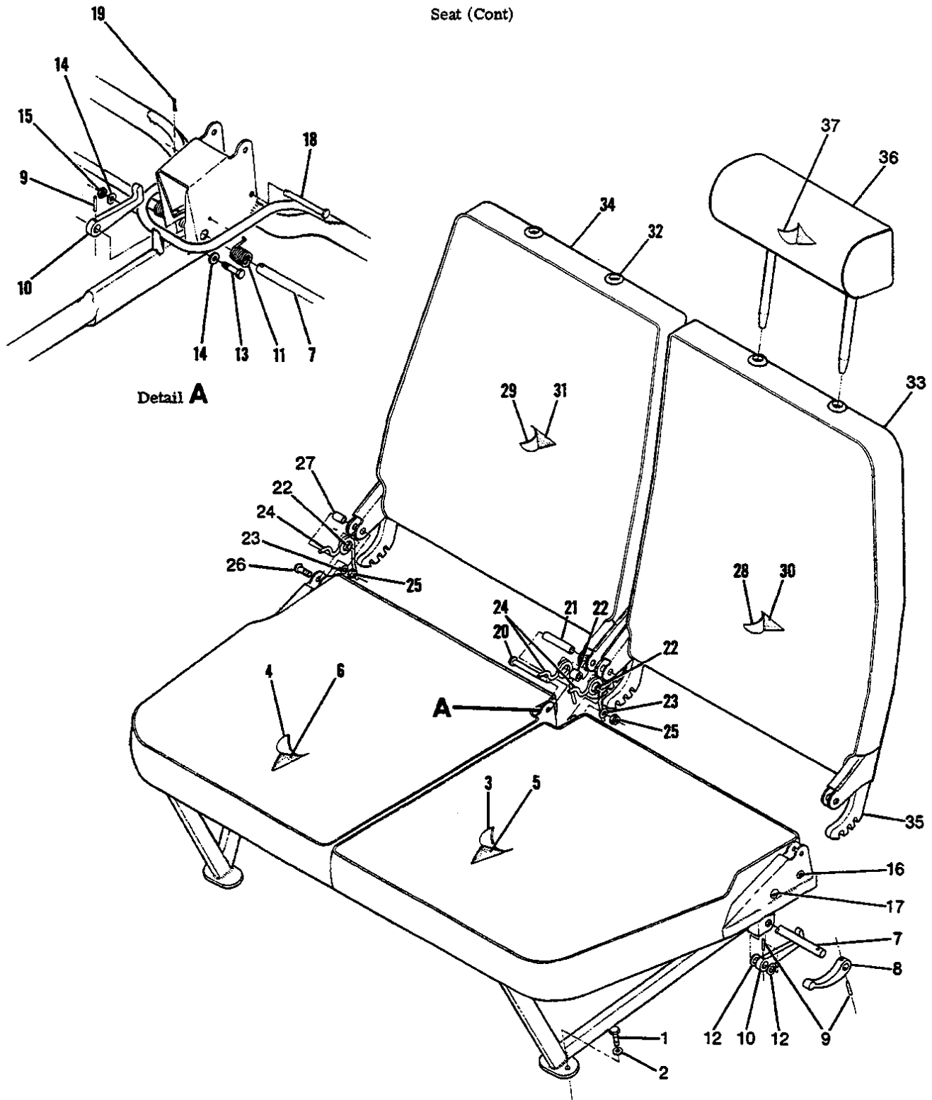
172 SERIAL 17263459 THRU 17272884 F172 SERIAL F17201235 THRU F17201909 Figure 55. Rear Seat Installation - Individually Reclining Back
