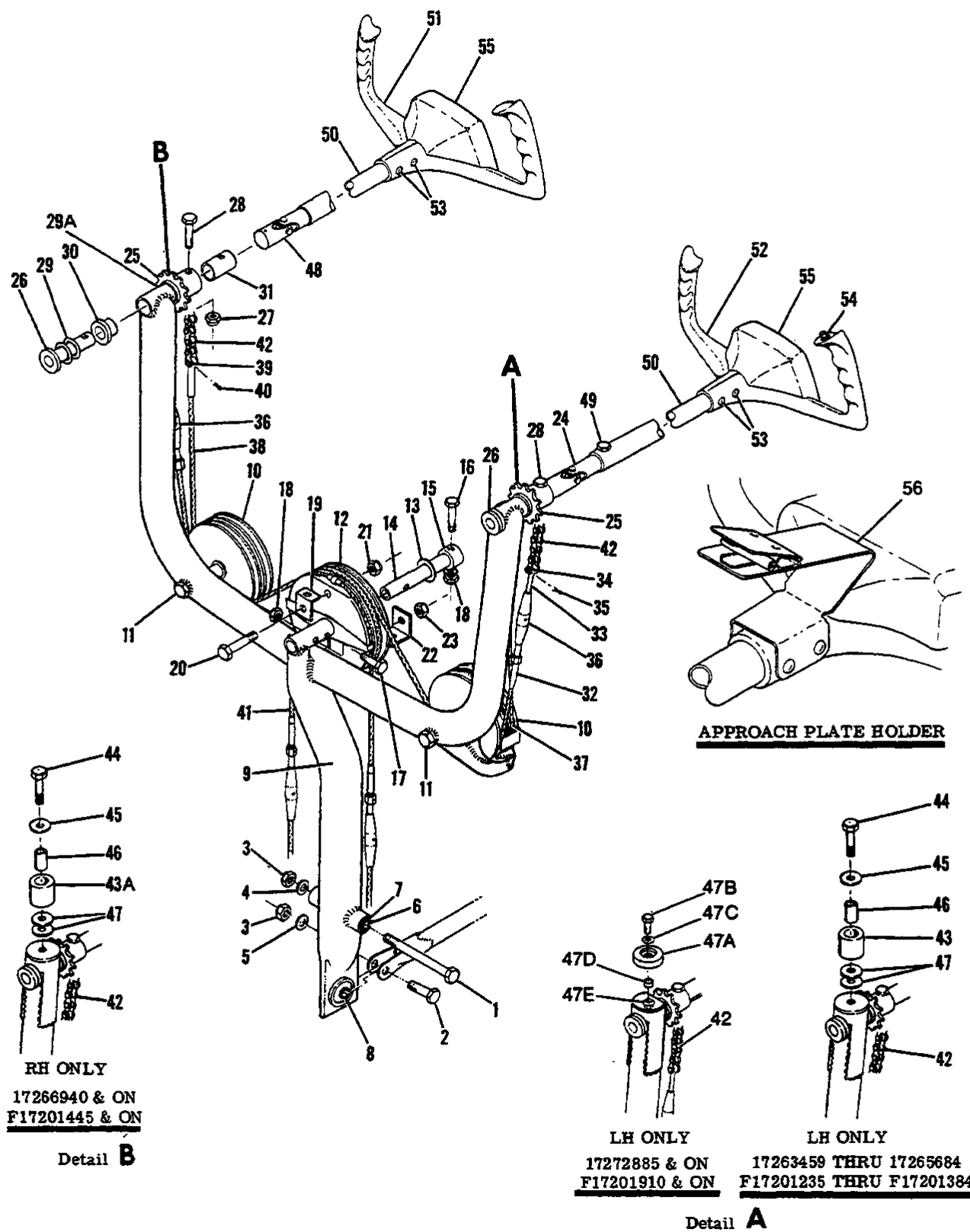
Figure 78. Control Yoke Installation.
