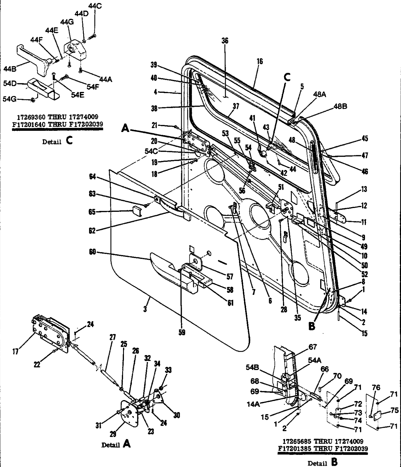
Figure 45. LH Cabin Door Installation
