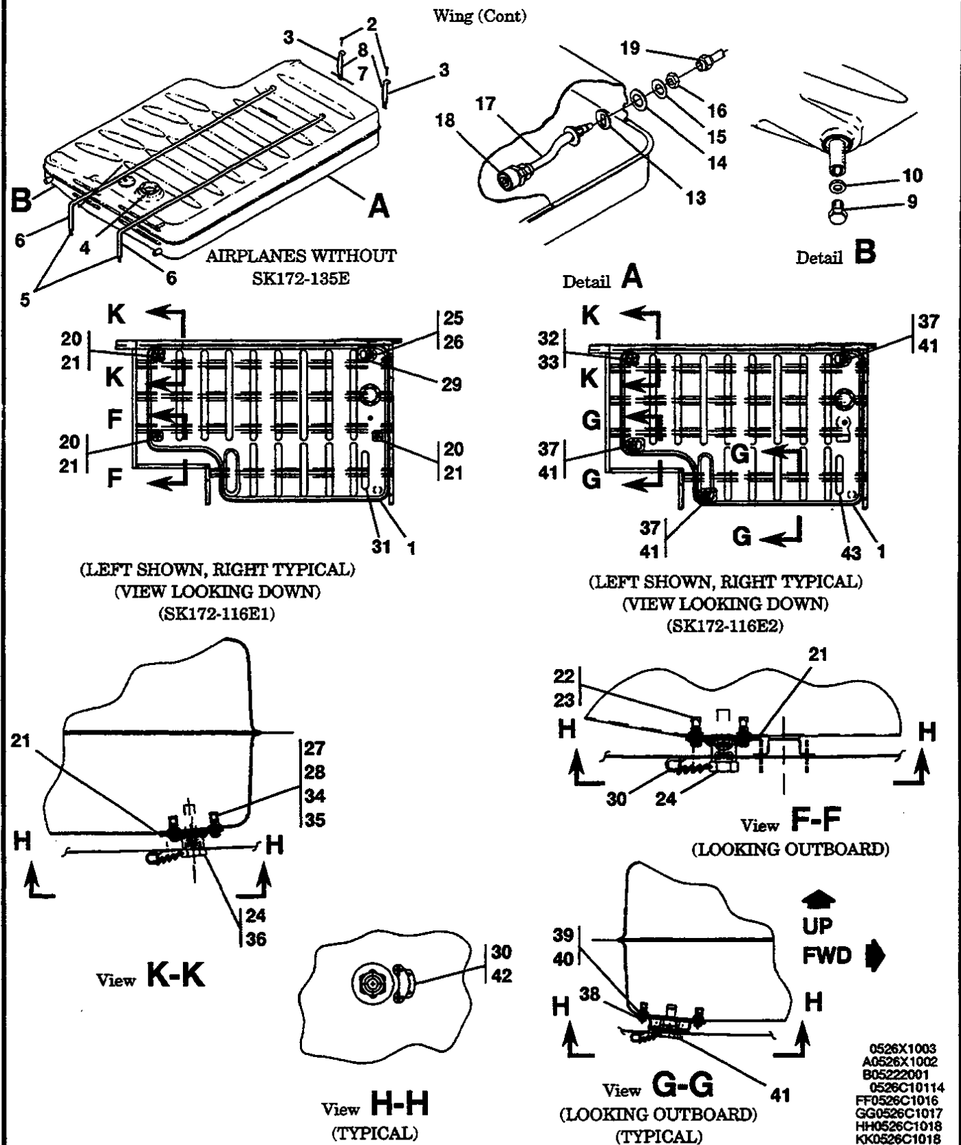
Figure 11. Fuel Tank Installation - Long Range
