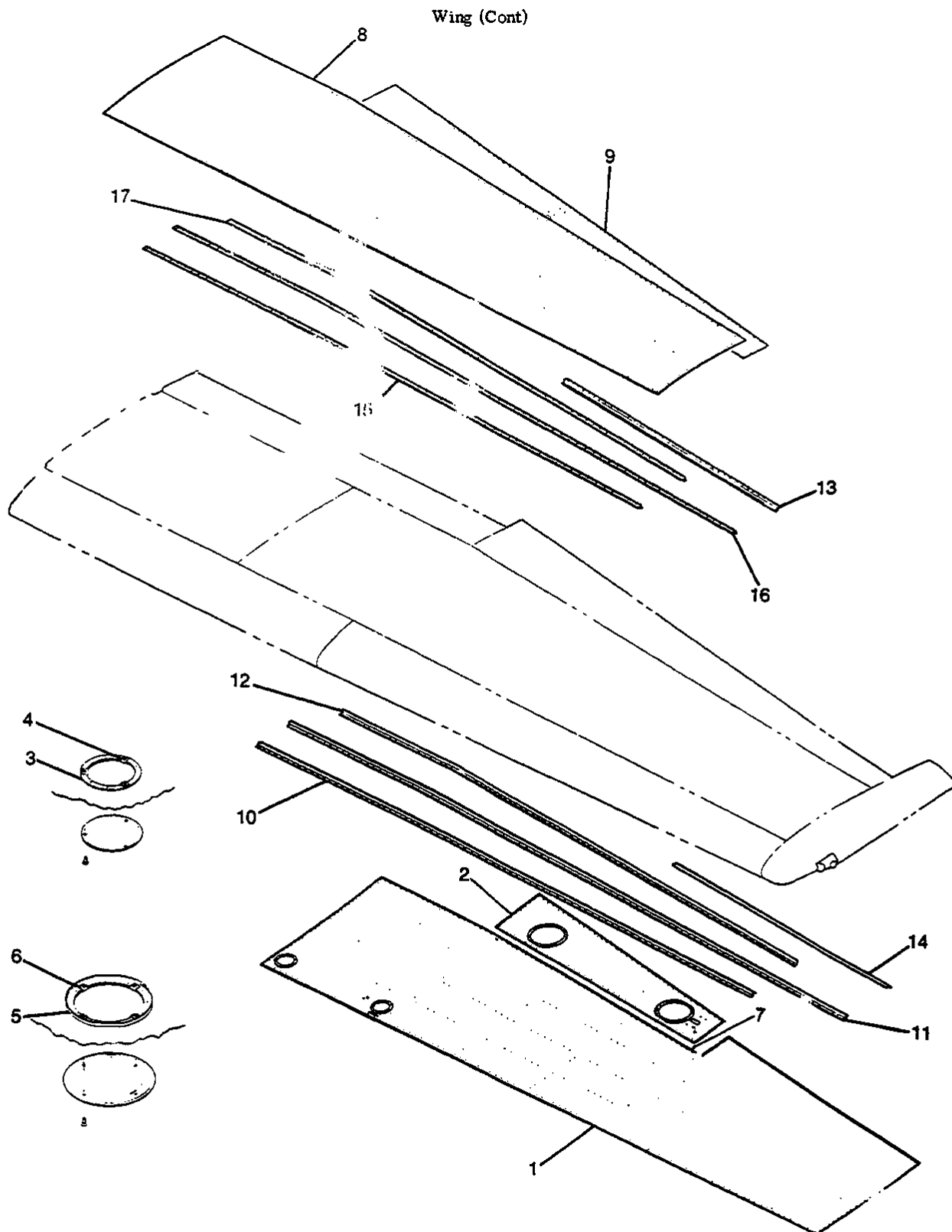
Figure 9A. Skins & Stringers Installation - Integral Fuel Cell
