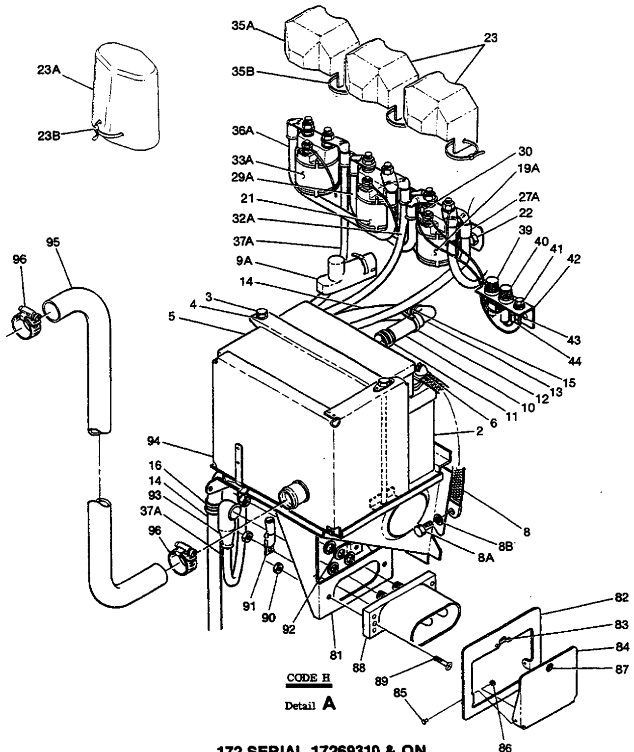
Figure 96A. (Sheet 3 of 3) Electrical Equipment Installation - 24 Volt
