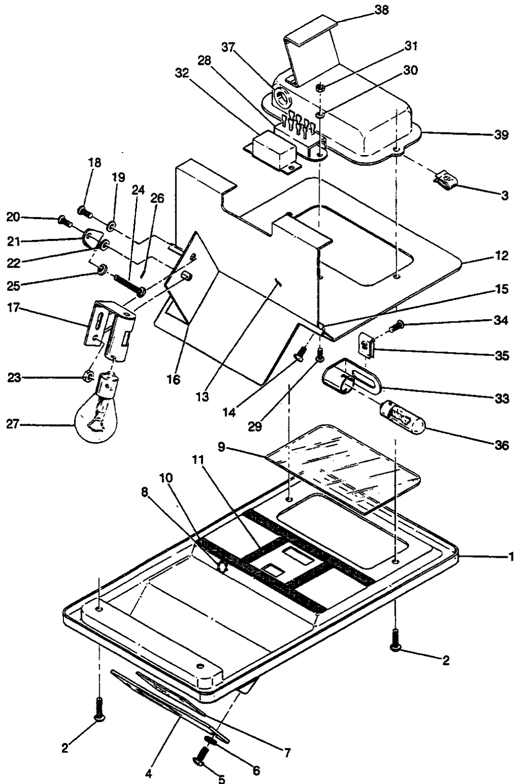
Figure 97B. Instrument Panel Light Installation
