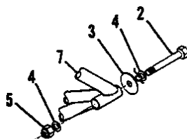
ENGINE MOUNT
