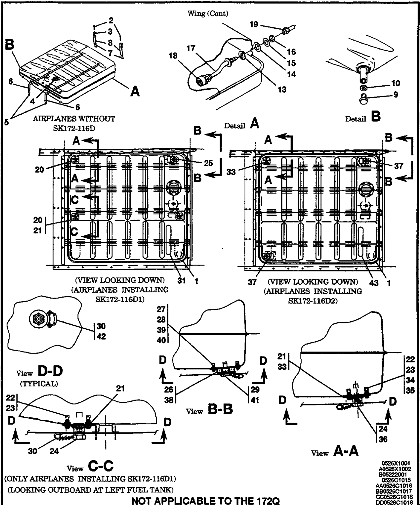
Figure 10. Fuel Tank Installation
