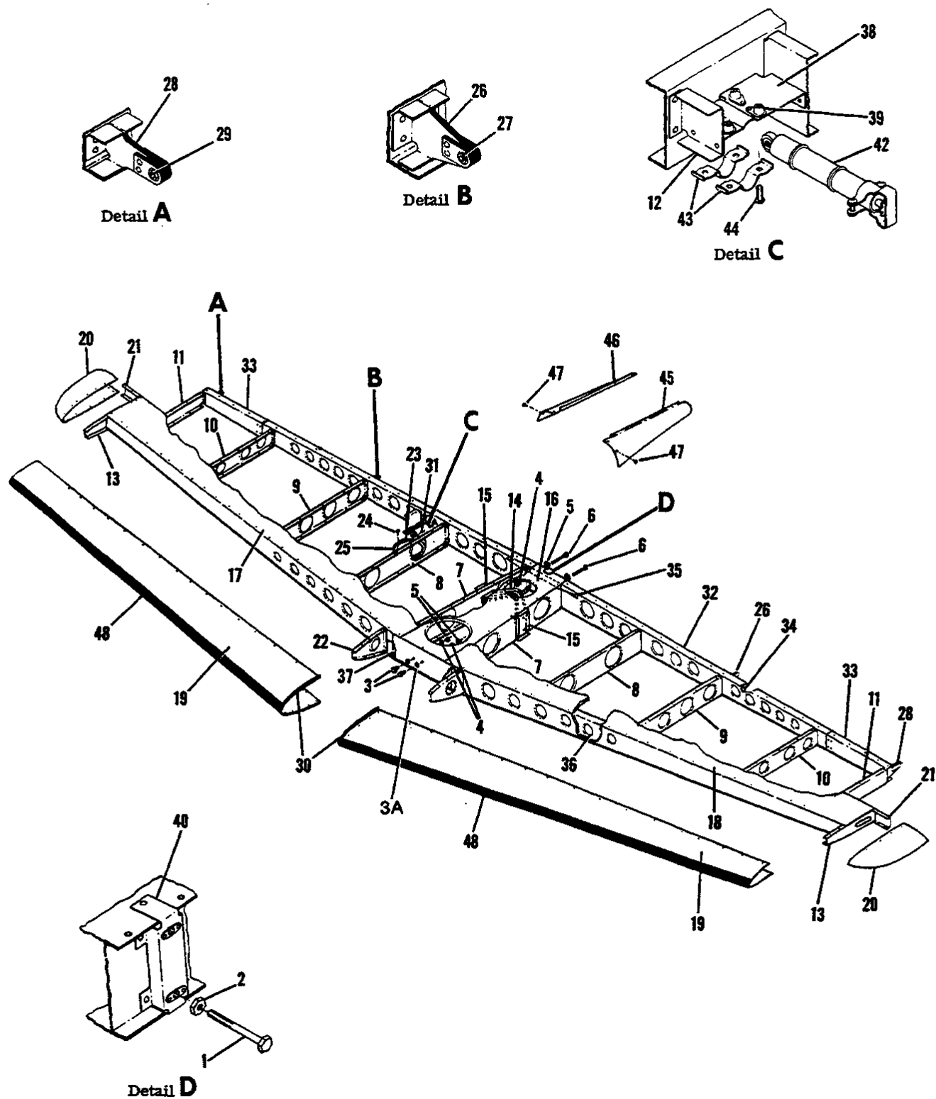
Figure 18. Stabilizer Installation
