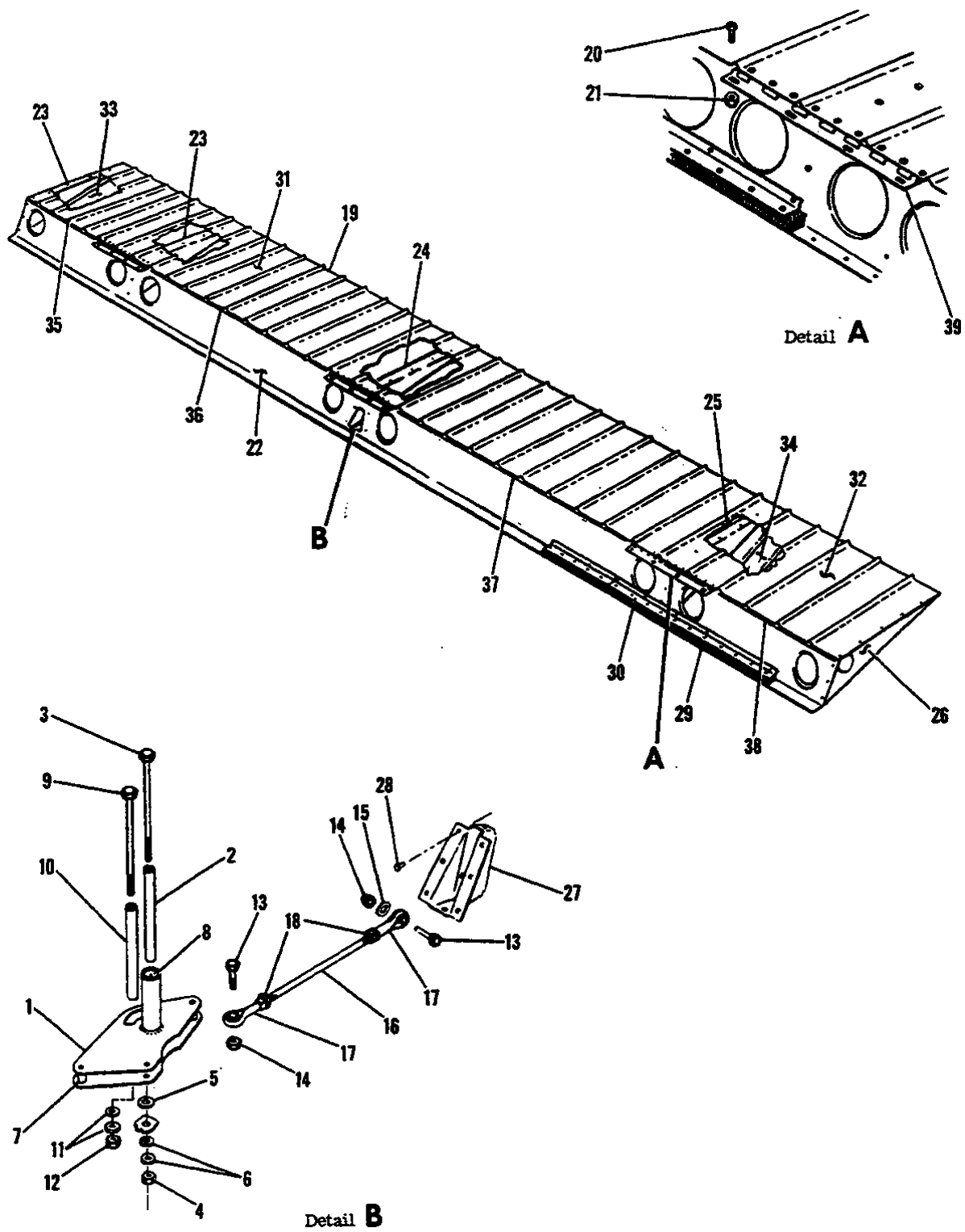
Figure 13. Aileron Installation
