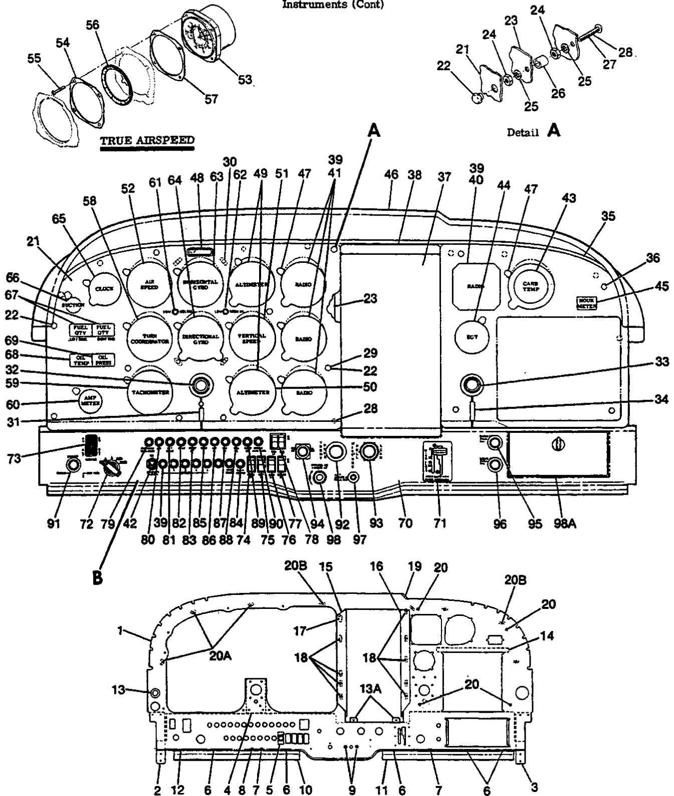
Figure 58D. (Sheet 1 of 2) Instrument Panel Equipment Installation
