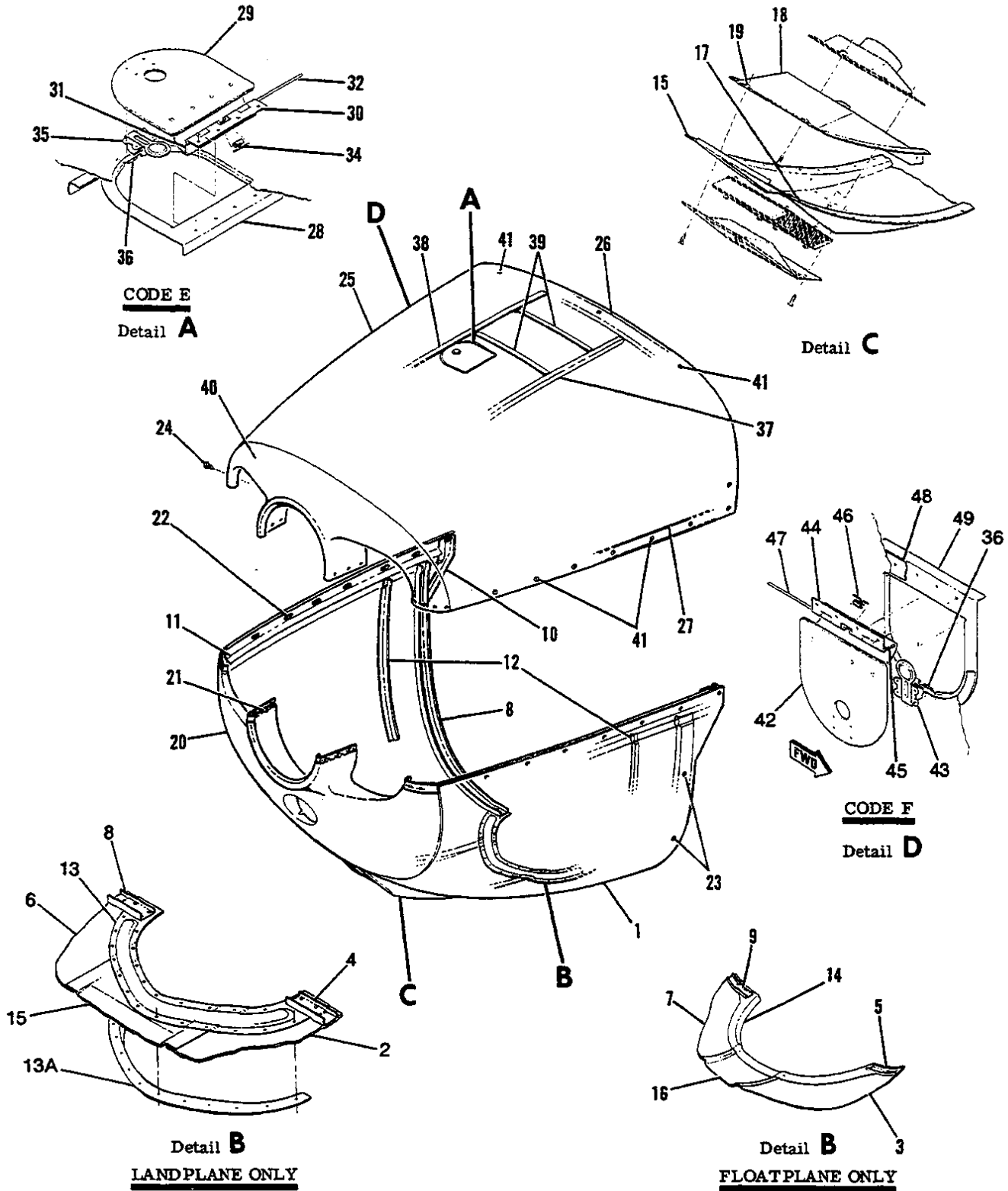
Figure 66A. Engine Cowl Assembly - Single Landing Light
