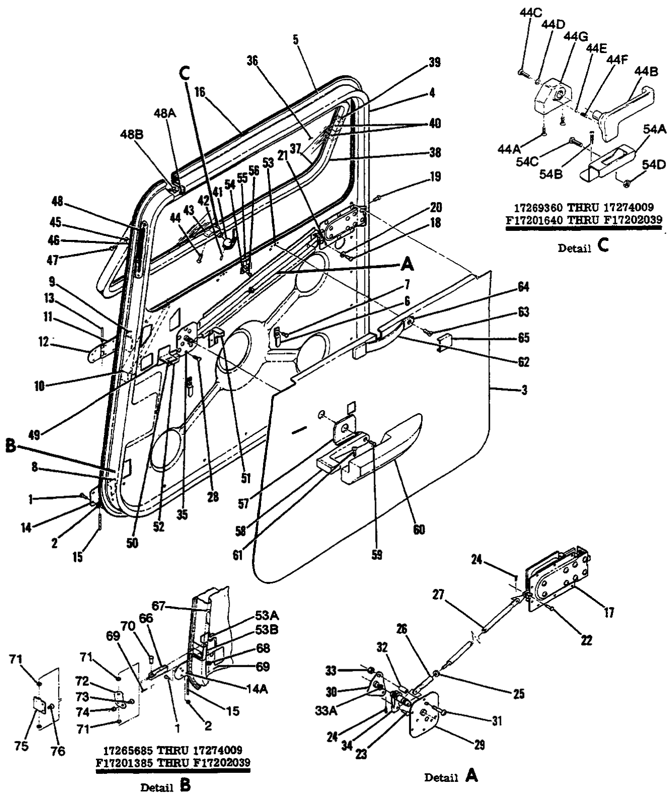
Figure 47. RH Cabin Door Installation (Openable Window)
