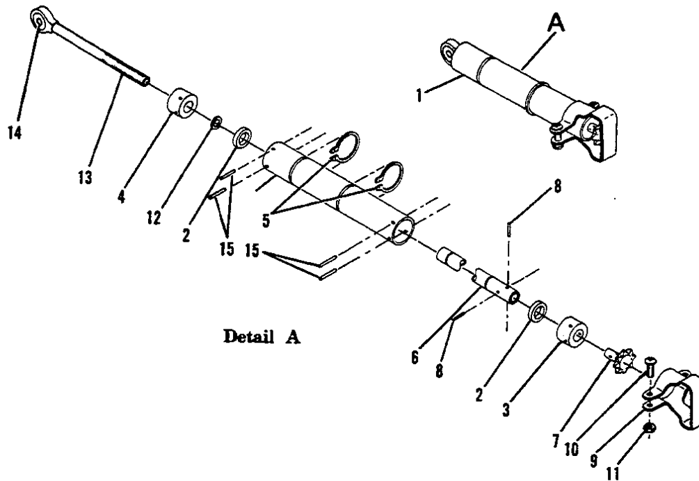
Figure 19. Elevator Trim Tab Actuator Assembly
