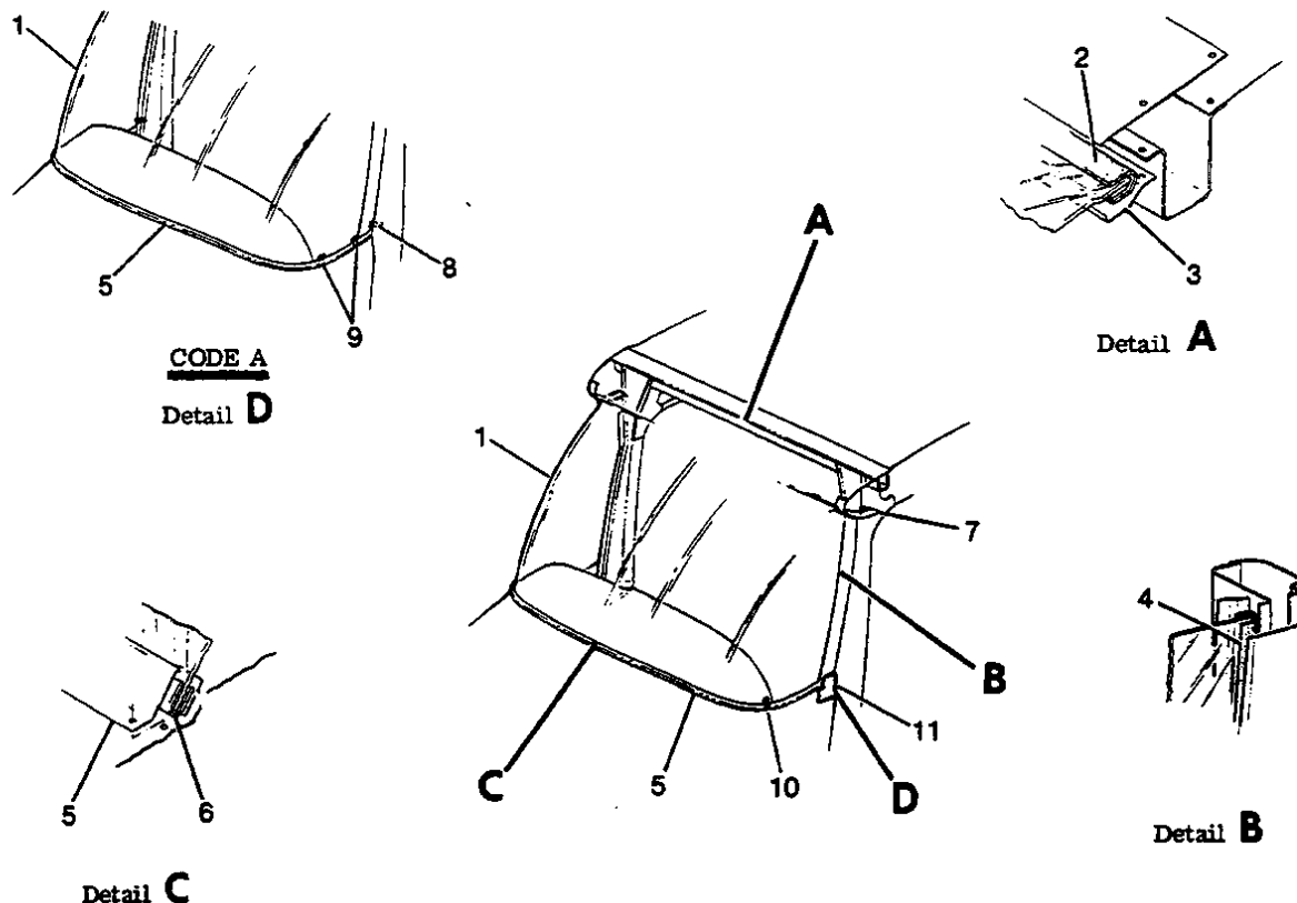
Figure 31. Windshield Installation
