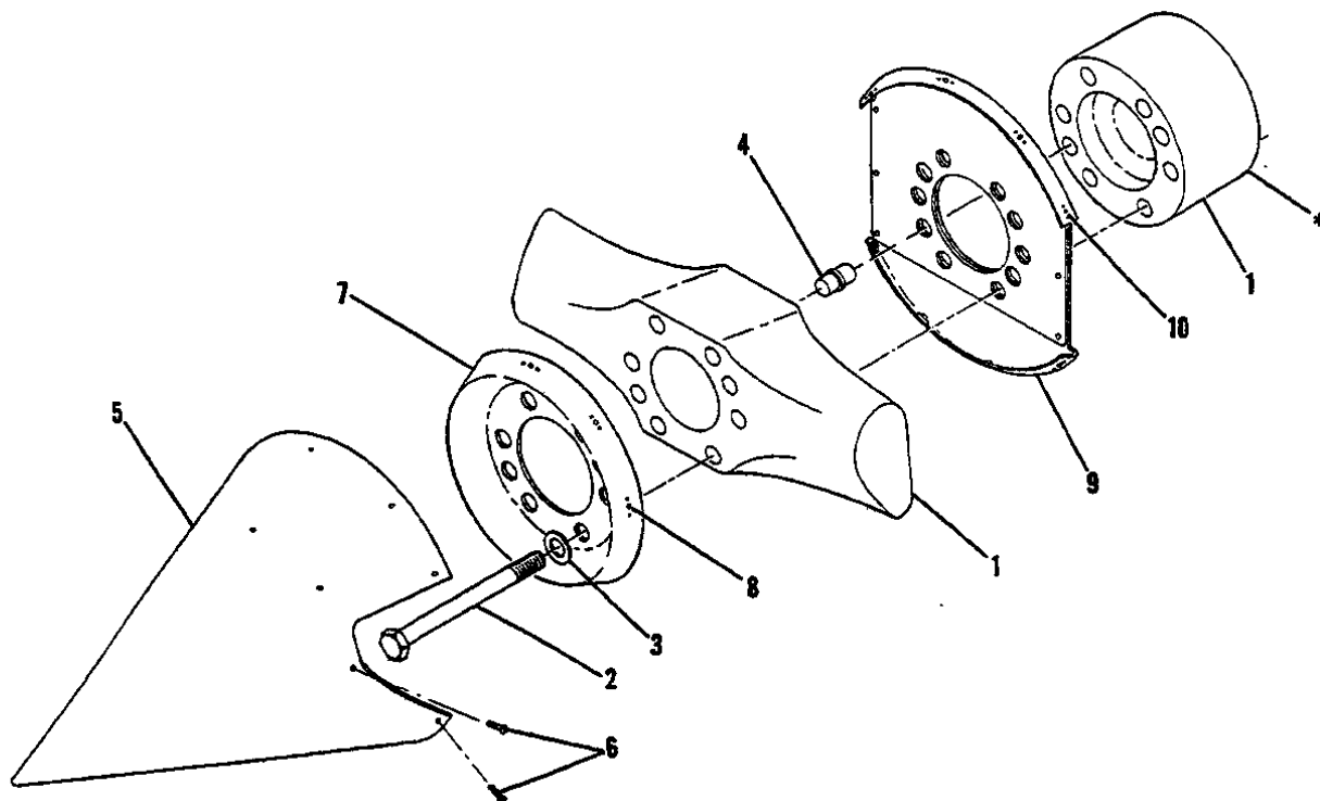
Propeller
