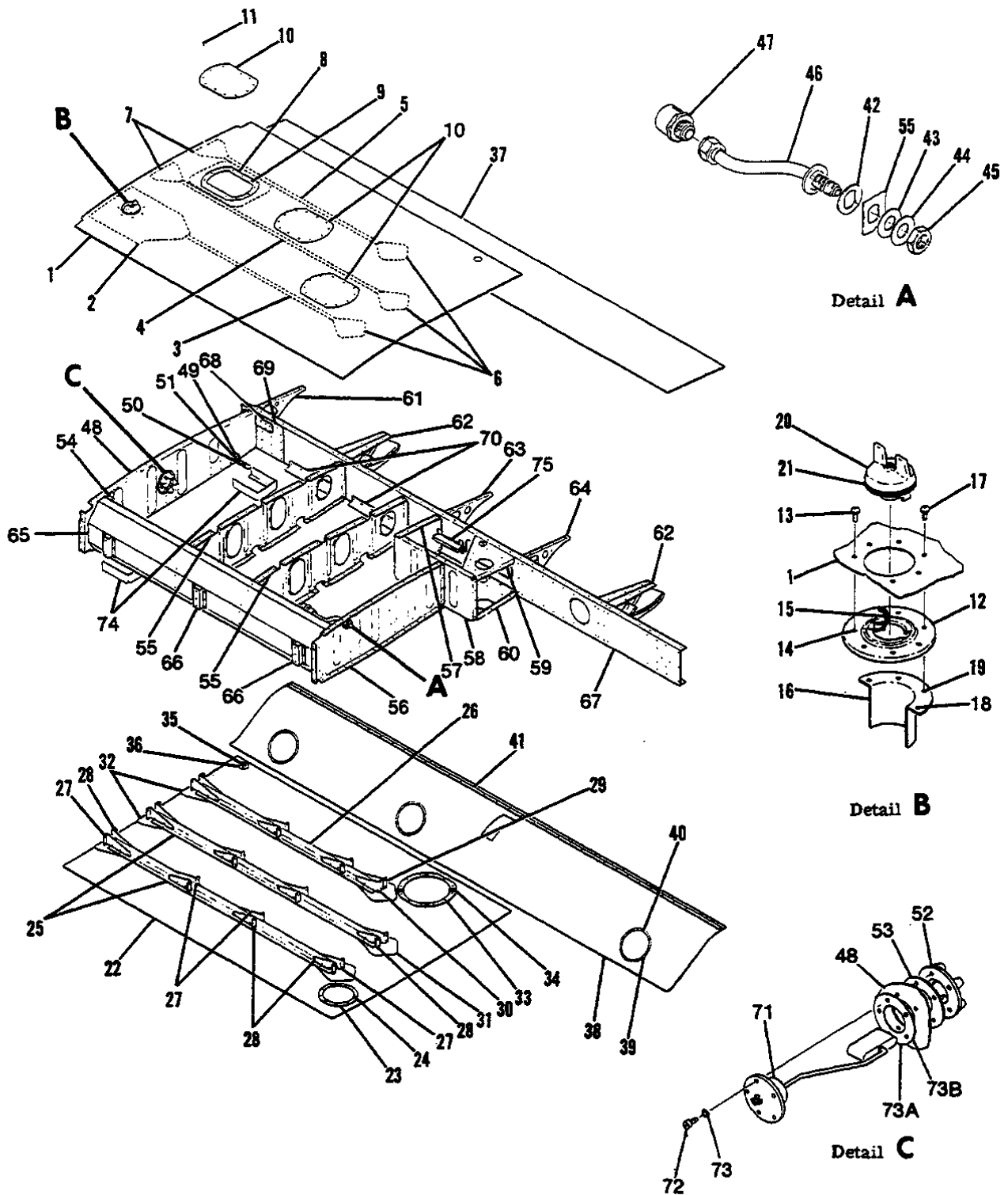
172 SERIAL 17274010 & ON F172 SERIAL F17202040 & ON Figure 6B. Integral Fuel Cell Structure Assembly
