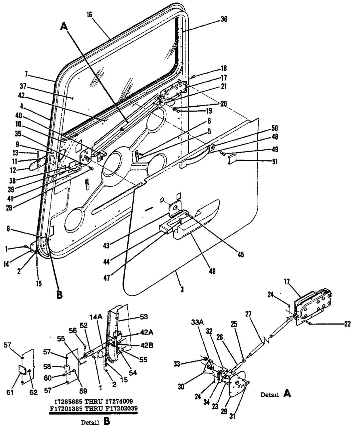
Figure 46. RH Cabin Door Installation
