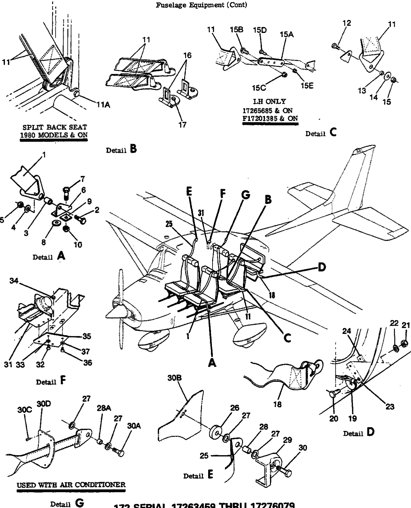
Figure 61. Seat Belts & Shoulder Harness Installation
