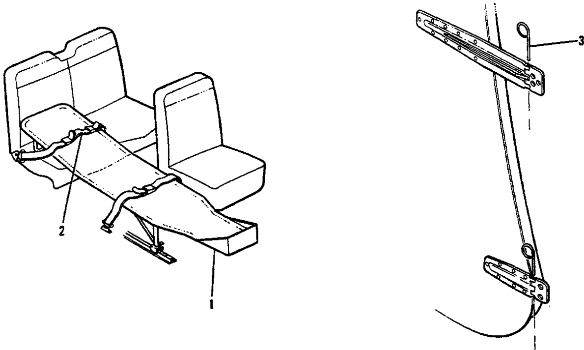
Figure 62. Portable Stretcher Installation
