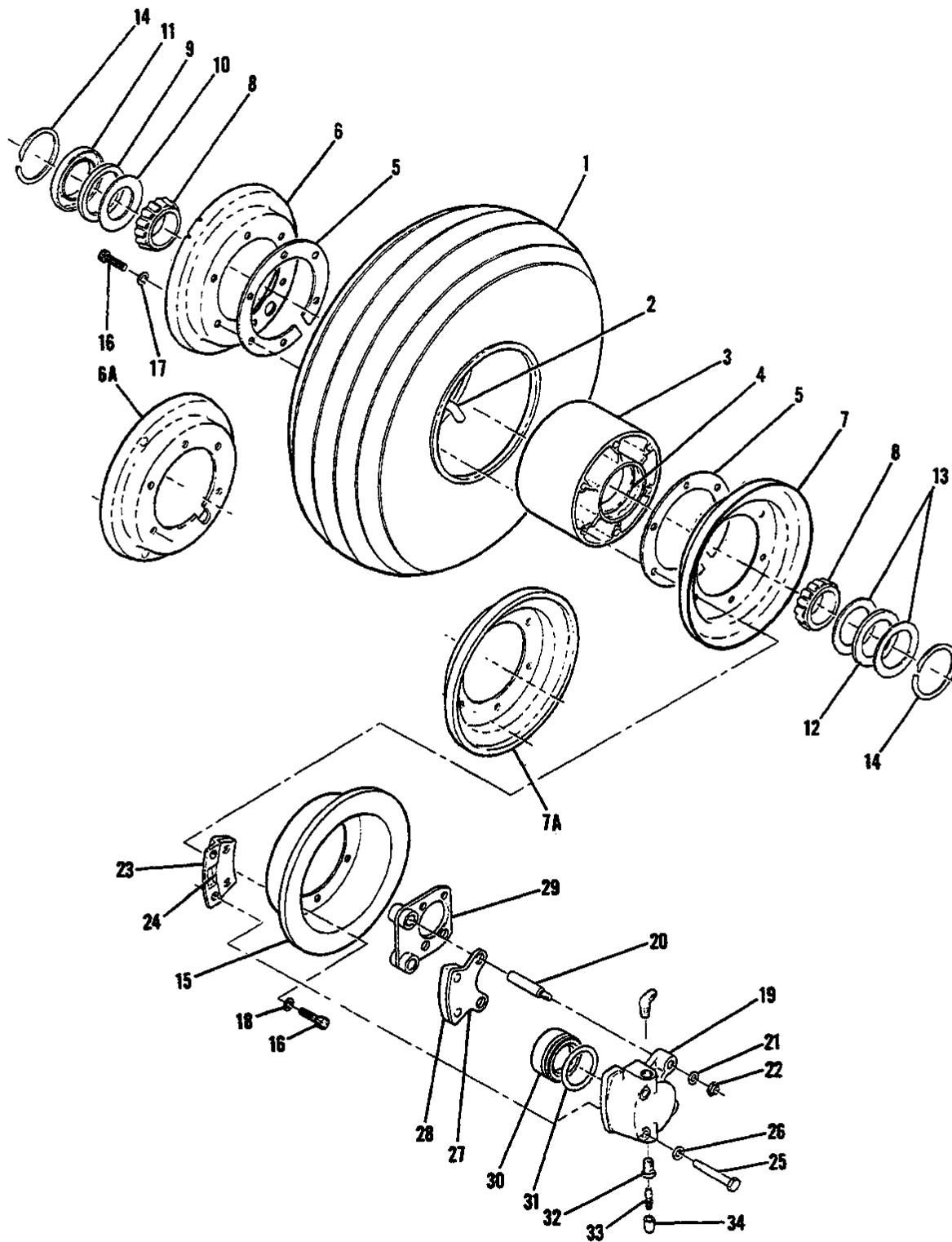
172 SERIAL 17263459 THRU 17268399 F172 SERIAL F17201235 THRU F17201633 Figure 44. Main Landing Gear Wheel & Brake Assembly
