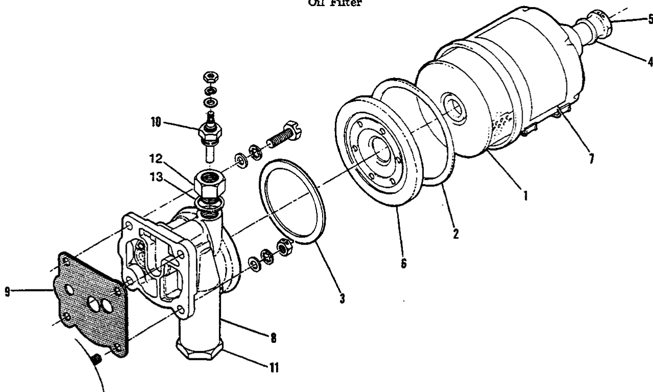
Oil Filter
