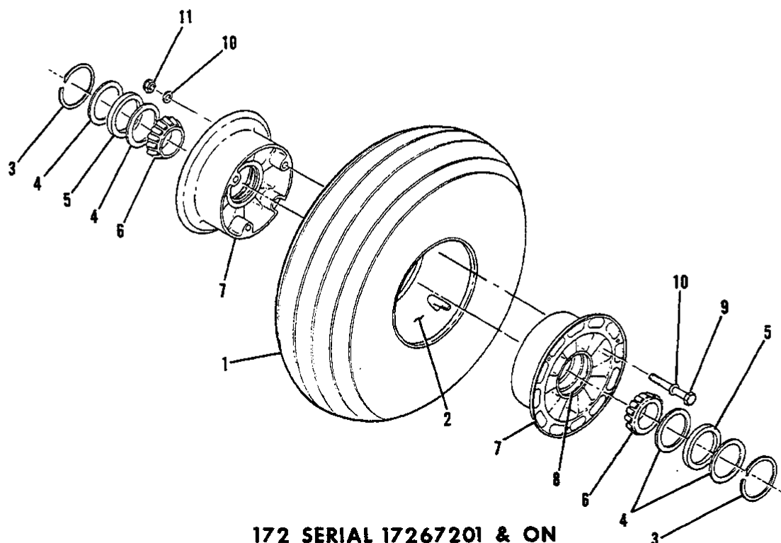
Figure 40A. Nose Gear Wheel & Tire Assembly - McCauley
