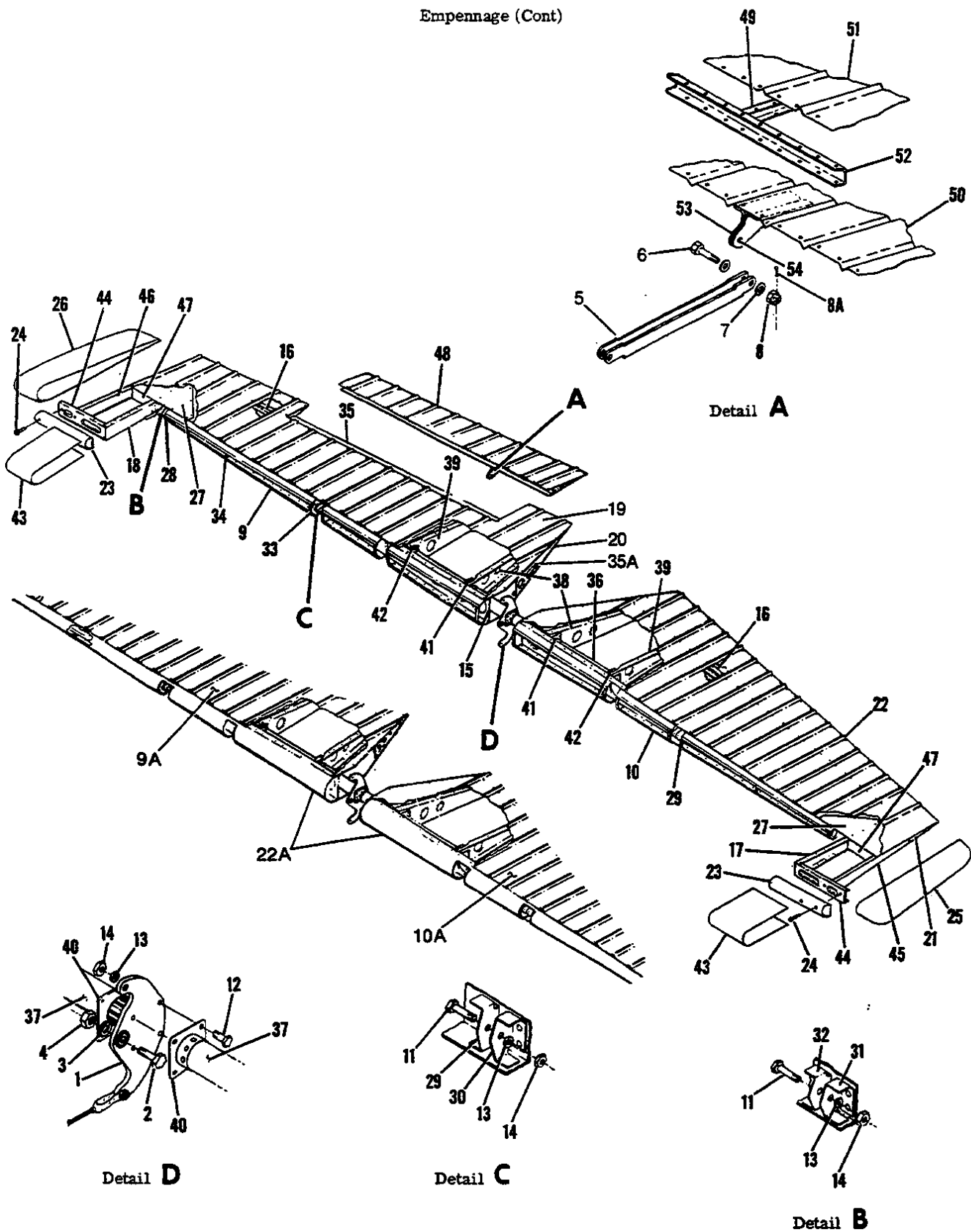
Figure 20. Elevator Installation
