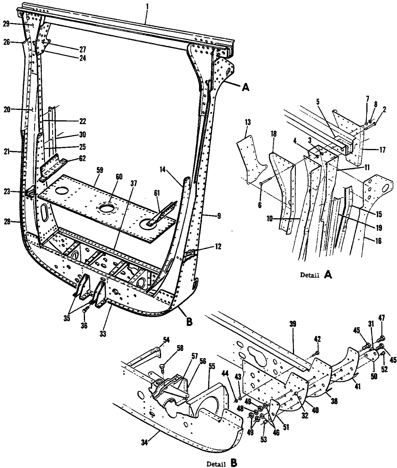
Figure 24A. Front Doorpost Bulkhead Assembly
