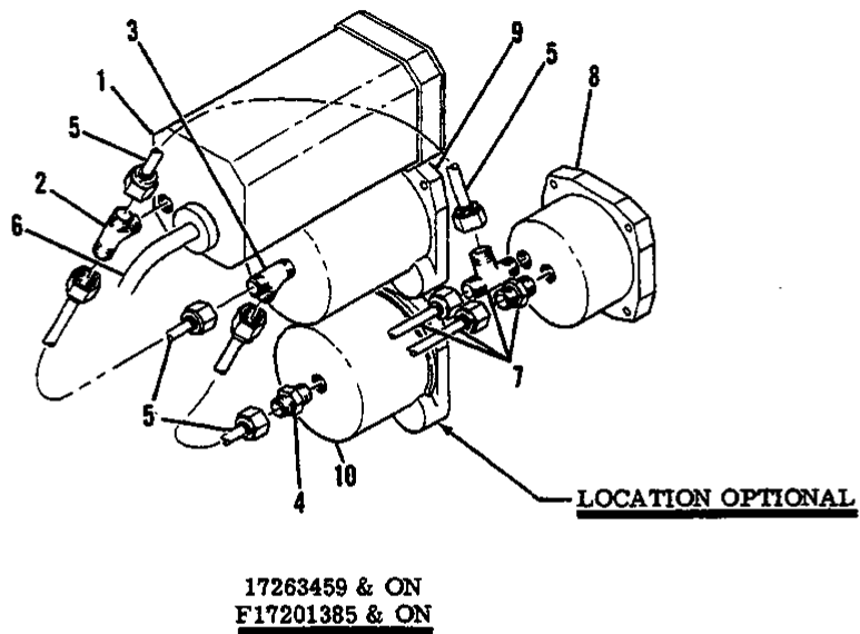
172 SERIAL 17263459 & ON F172 SERIAL F17201385 & ON Figure 84A. Encoding Altimeters Installation
