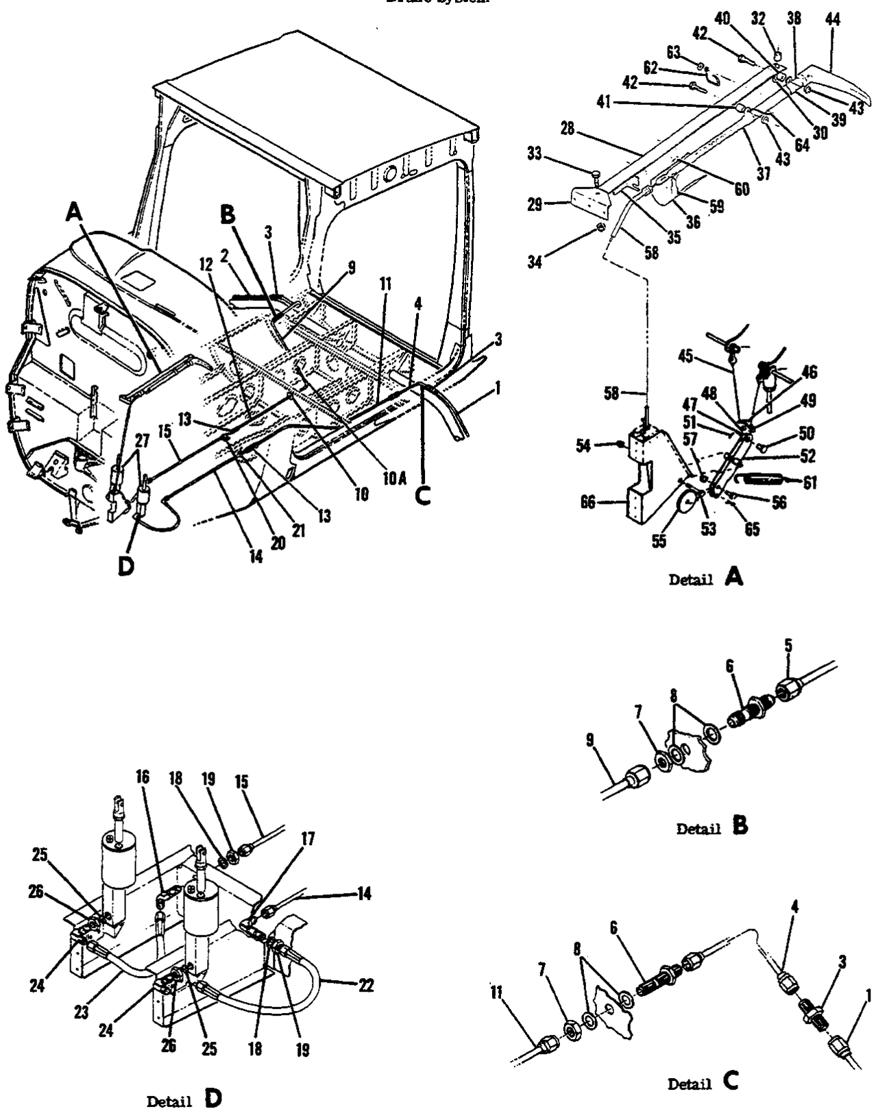
Figure 75. Brake System
