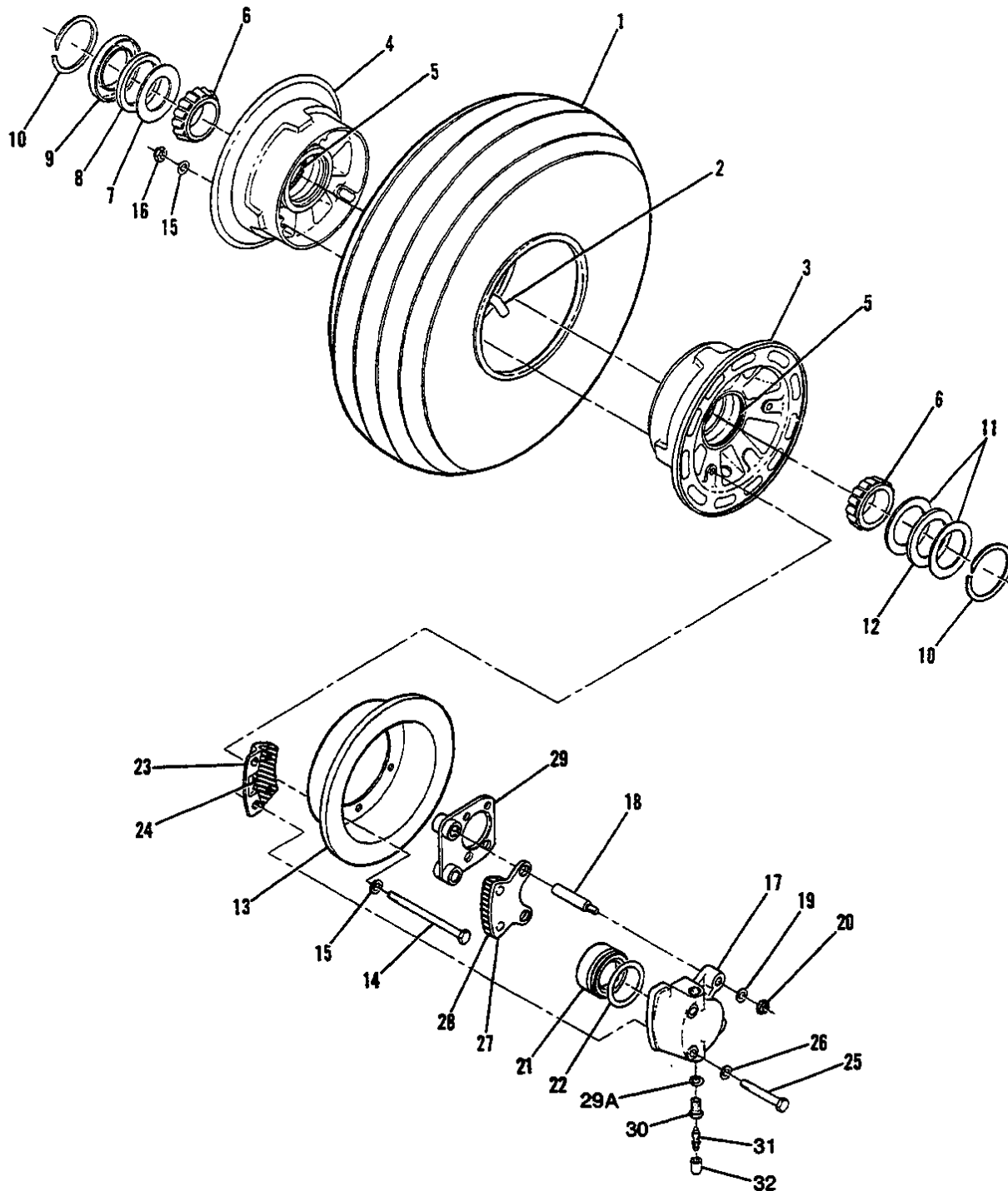
172 SERIAL 17268400 & ON F172 SERIAL F17201634 & ON Figure 44A. Main Landing Gear Wheel & Brake Assembly
