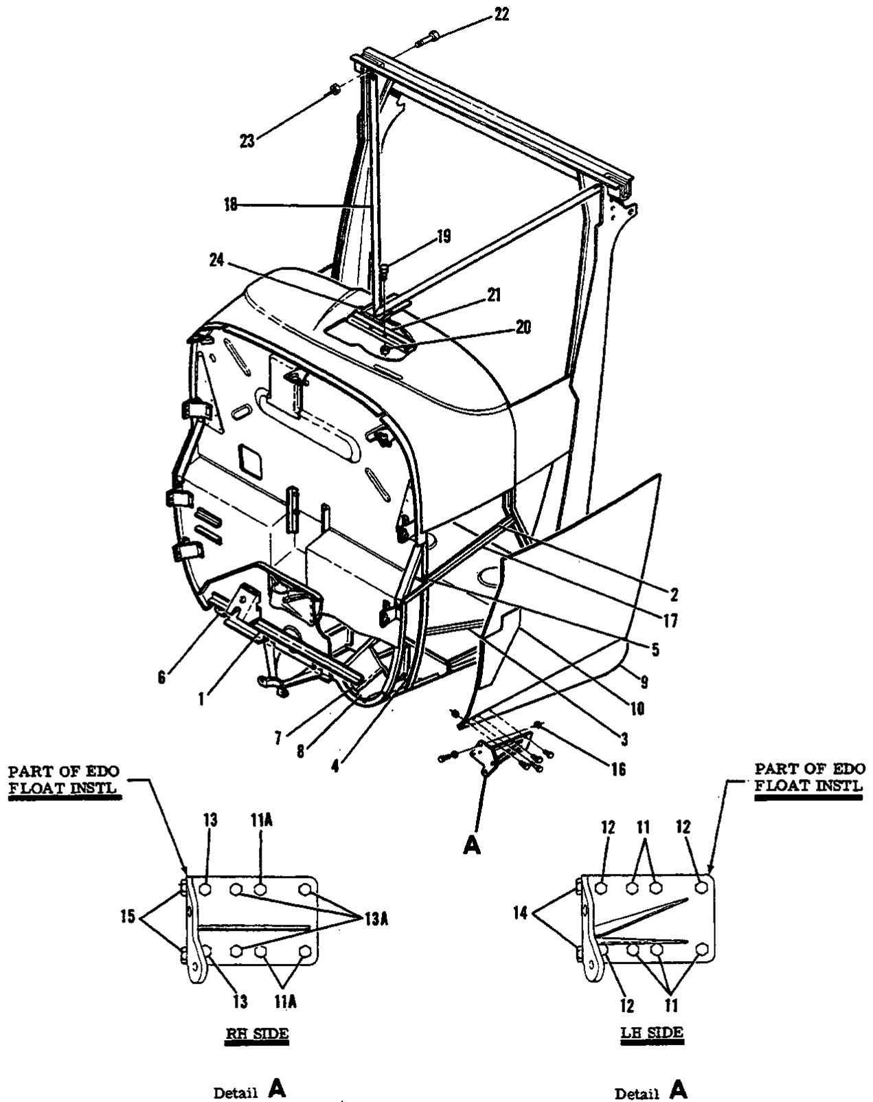
Figure 95. Floatplane Fuselage Structure Details
