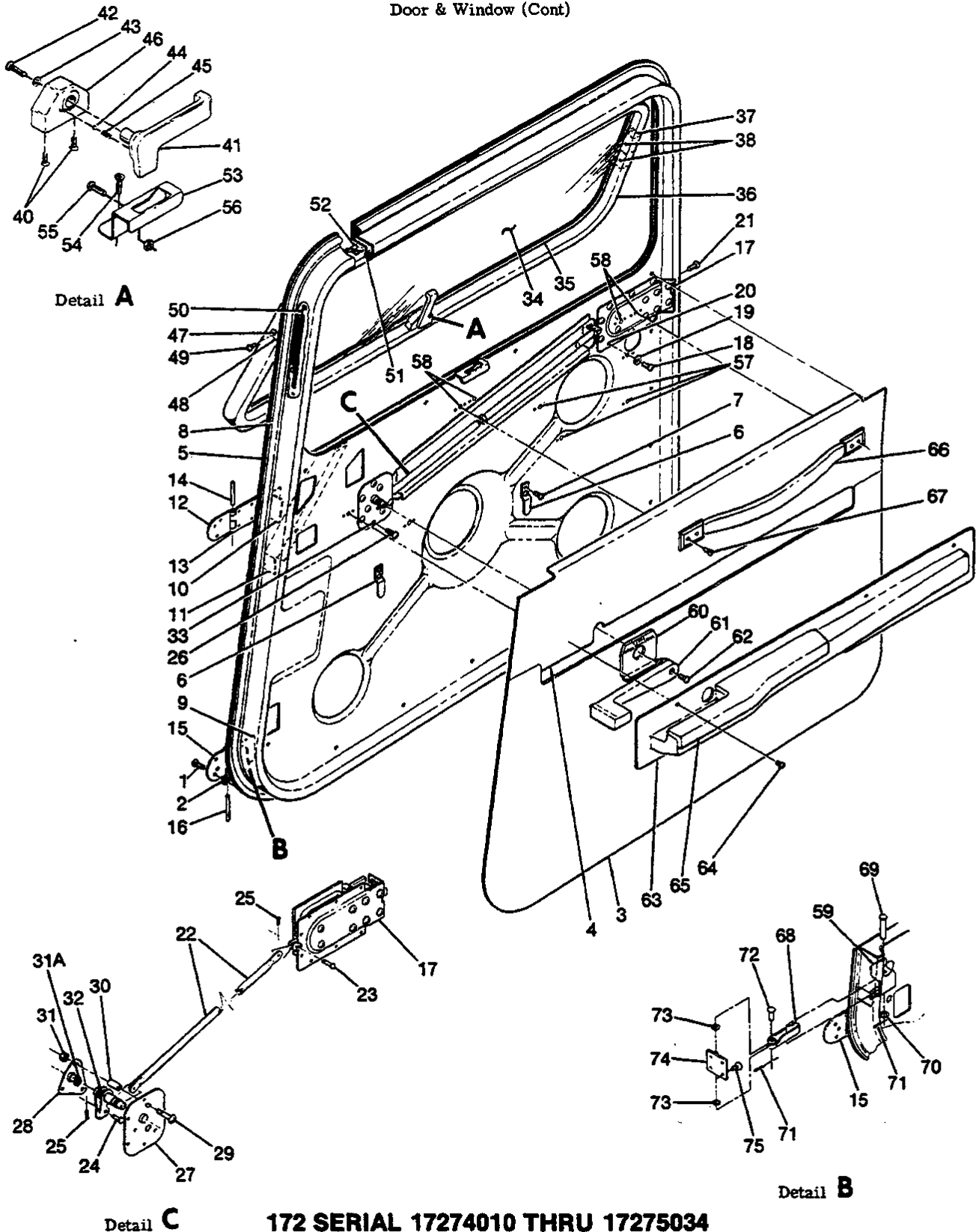
Figure 47A. RH Cabin Door Installation (Openable Window)
