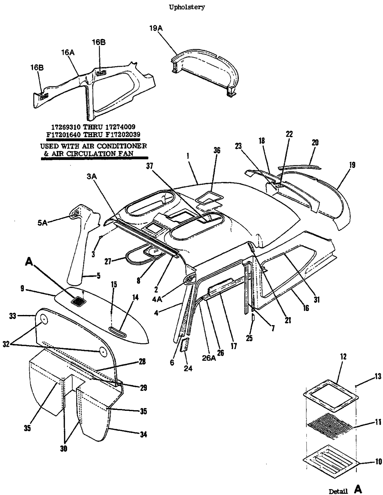
172 SERIAL 17263459 THRU 17274009 F172 SERIAL F17201235 THRU F17202039 Figure 50. Cabin Top & Firewall Upholstery Installation
