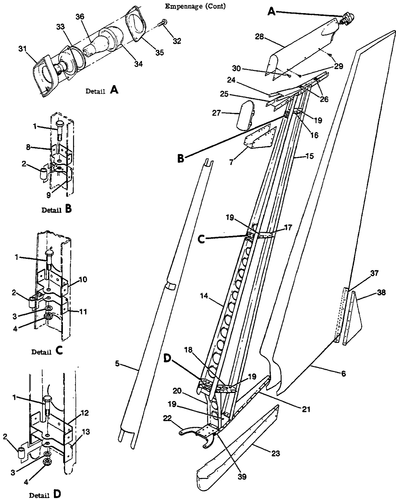
Figure 17A. Rudder Assembly
