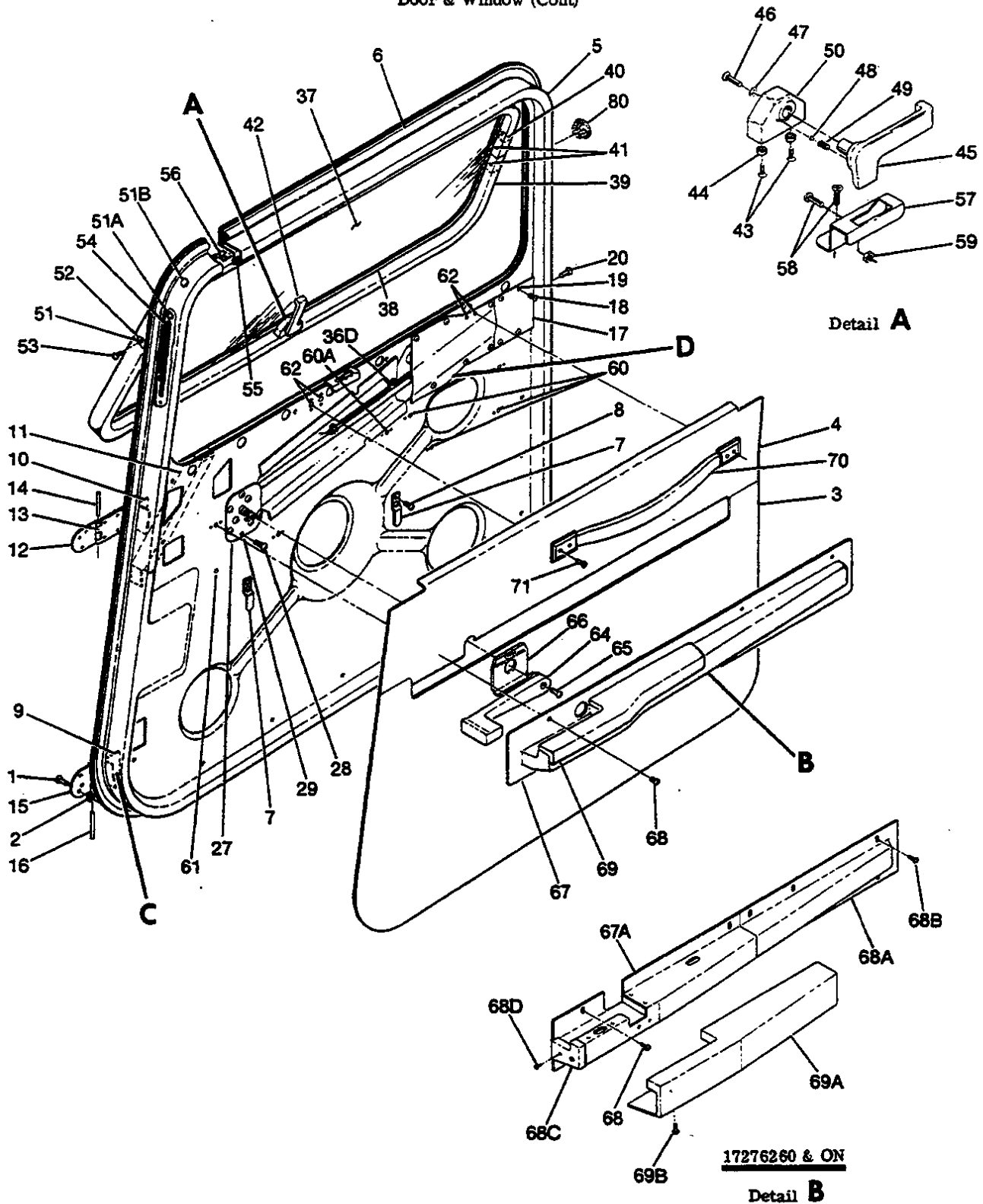
Figure 47B. (Sheet 1 of 2) RH Cabin Door Installation (Openable Window)
