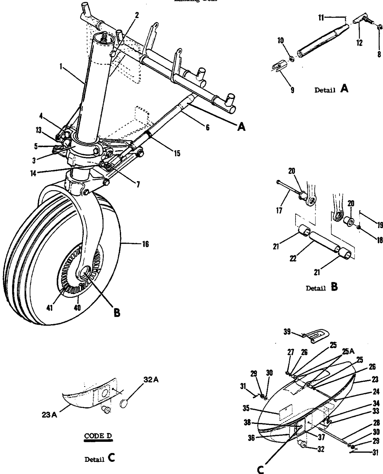
Landing Gear
