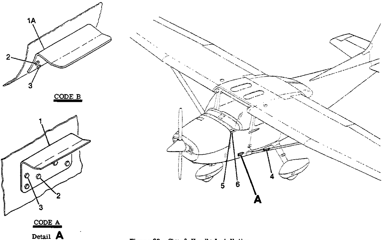
Figure 63. Step & Handle Installation
