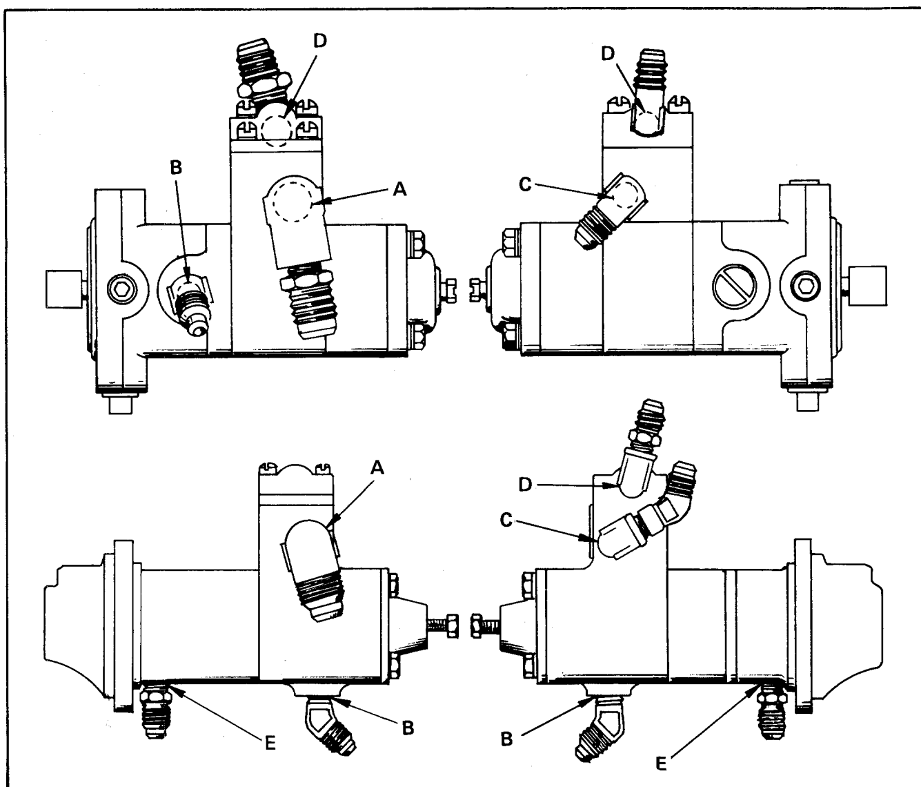
FIGURE 43. FUEL PUMP AND VAPOR SEPARATOR FITTING LOCATIONS
