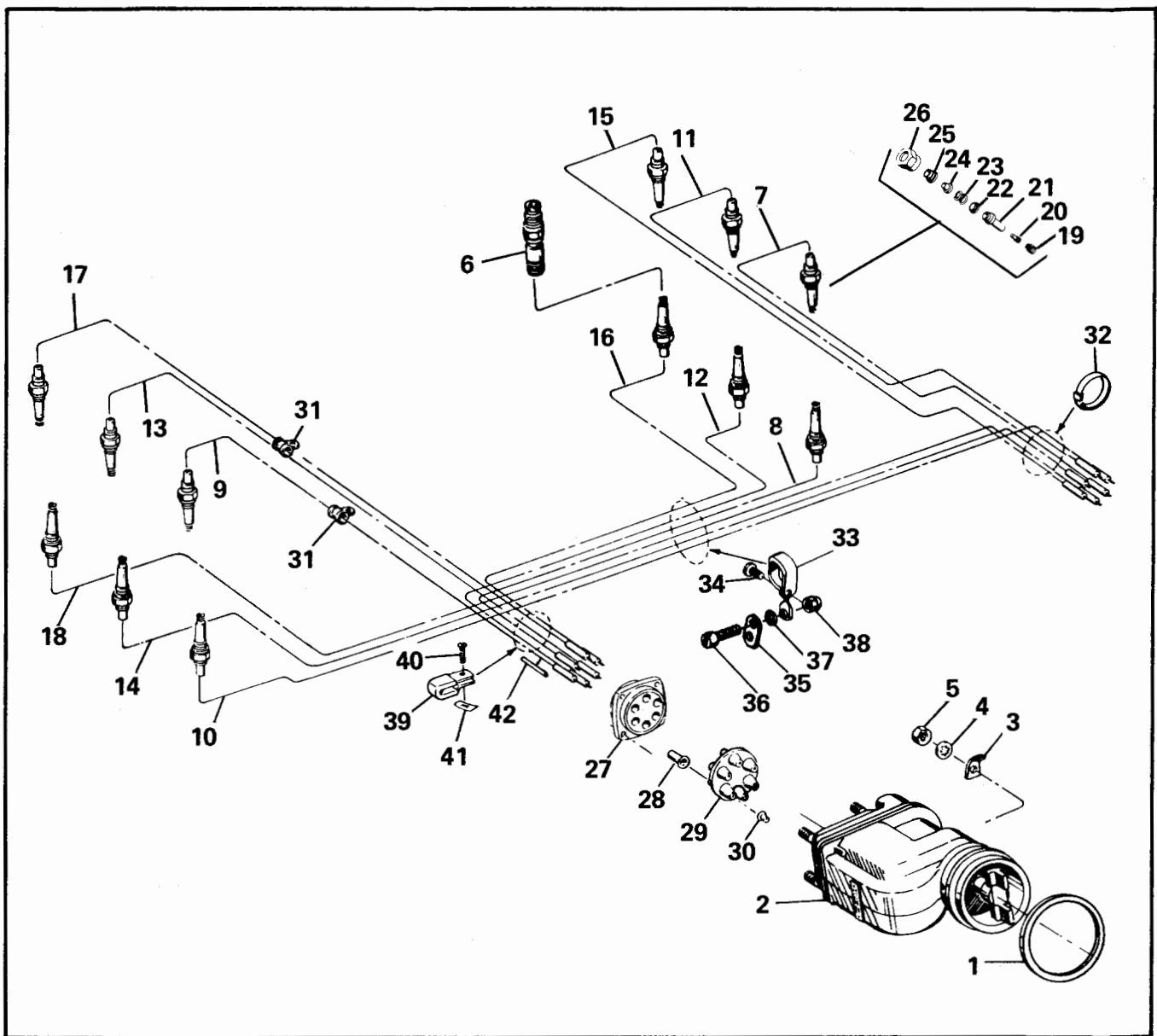
FIGURE 53. IGNITION SYSTEM
