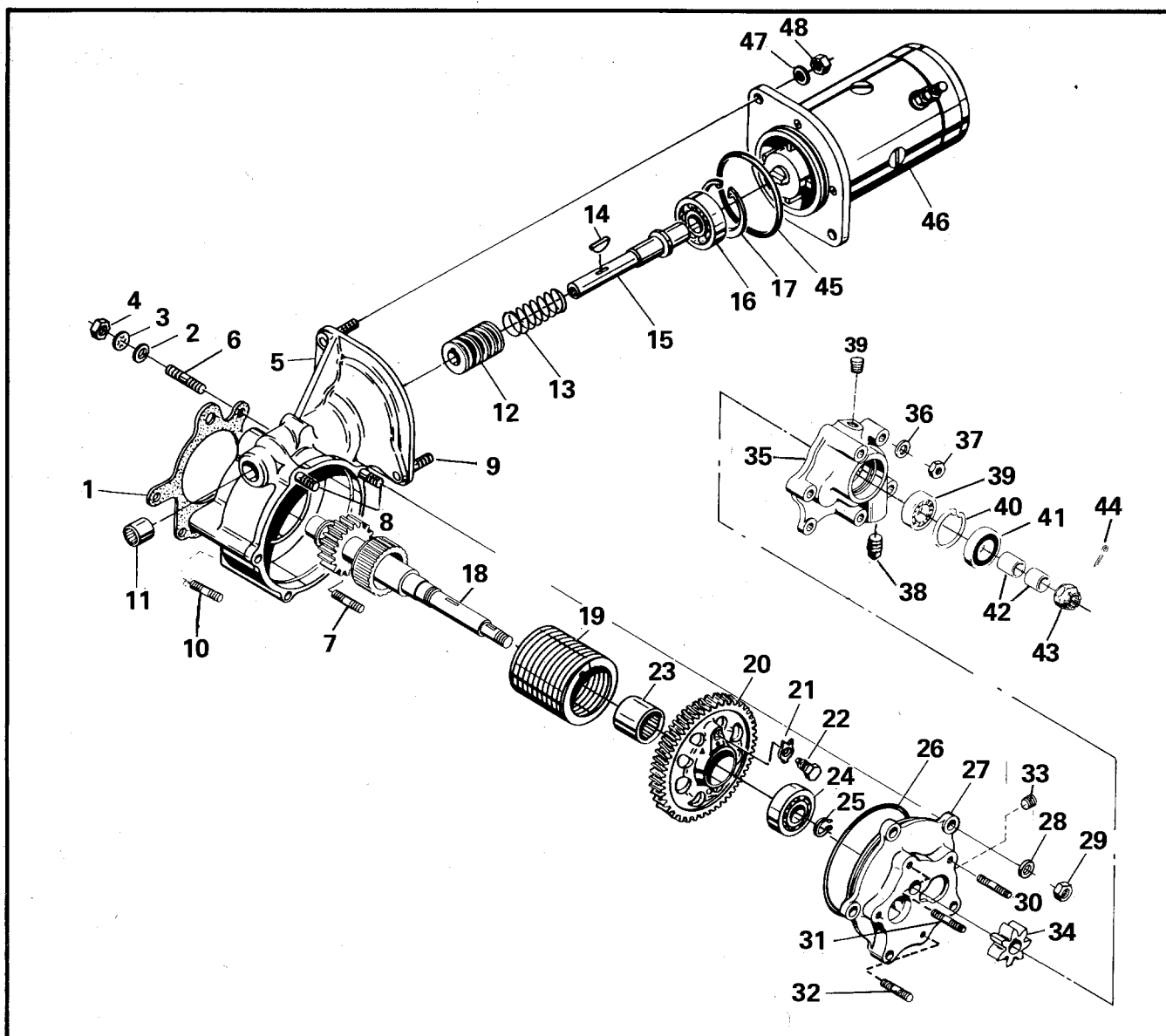
FIGURE 65. STARTER AND STARTER ADAPTER ASSEMBLY
