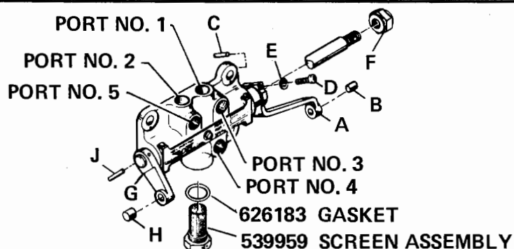
FIGURE 46. FUEL CONTROL FITTING LOCATIONS
