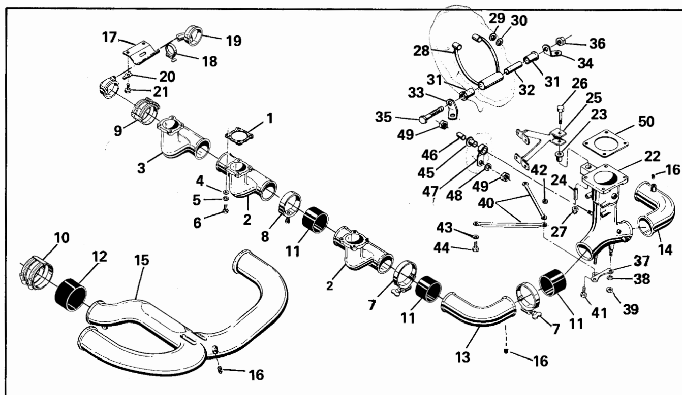
FIGURE 30. INDUCTION SYSTEM
