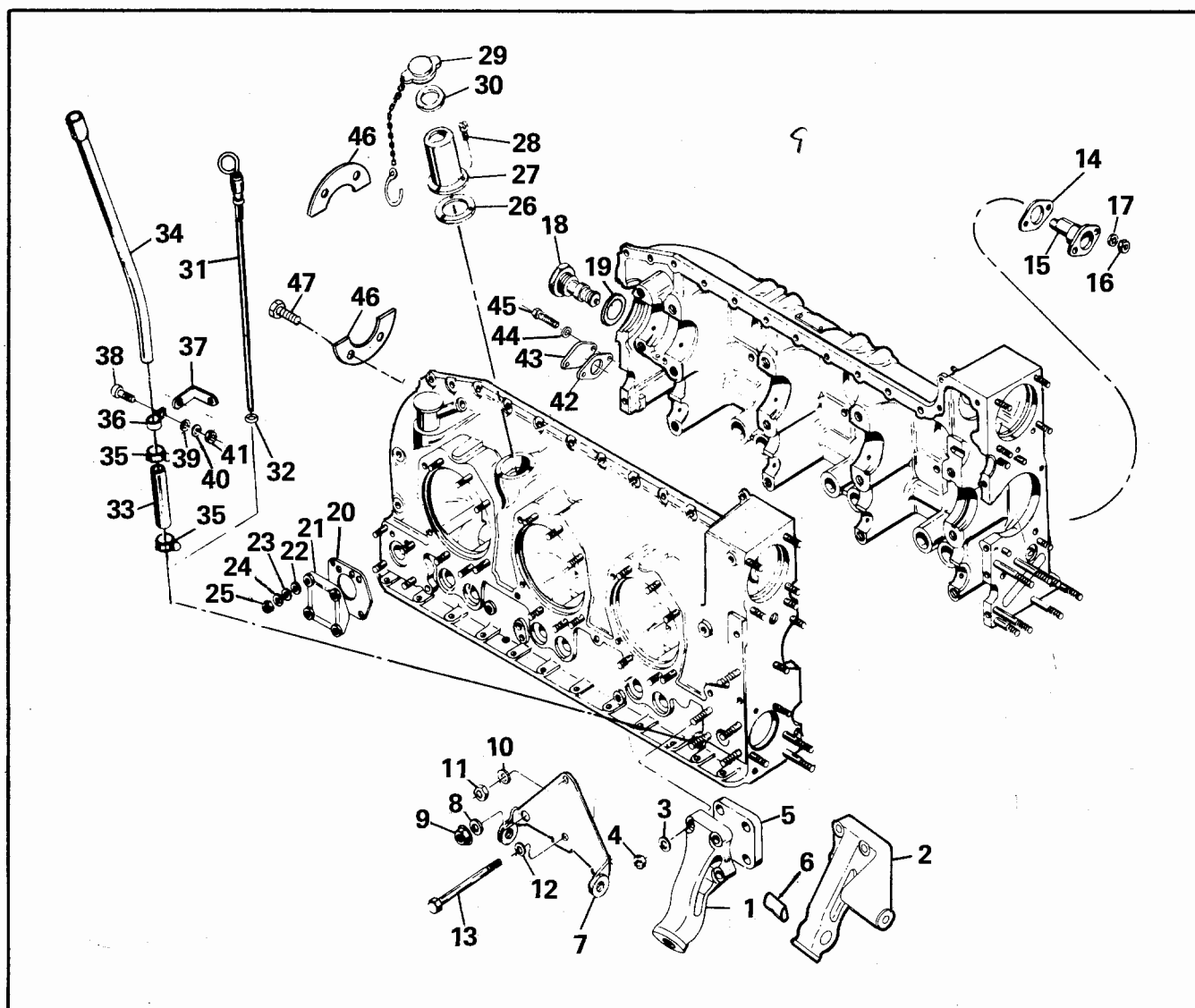
FIGURE 3. CRANKCASE ASSOCIATED PARTS
