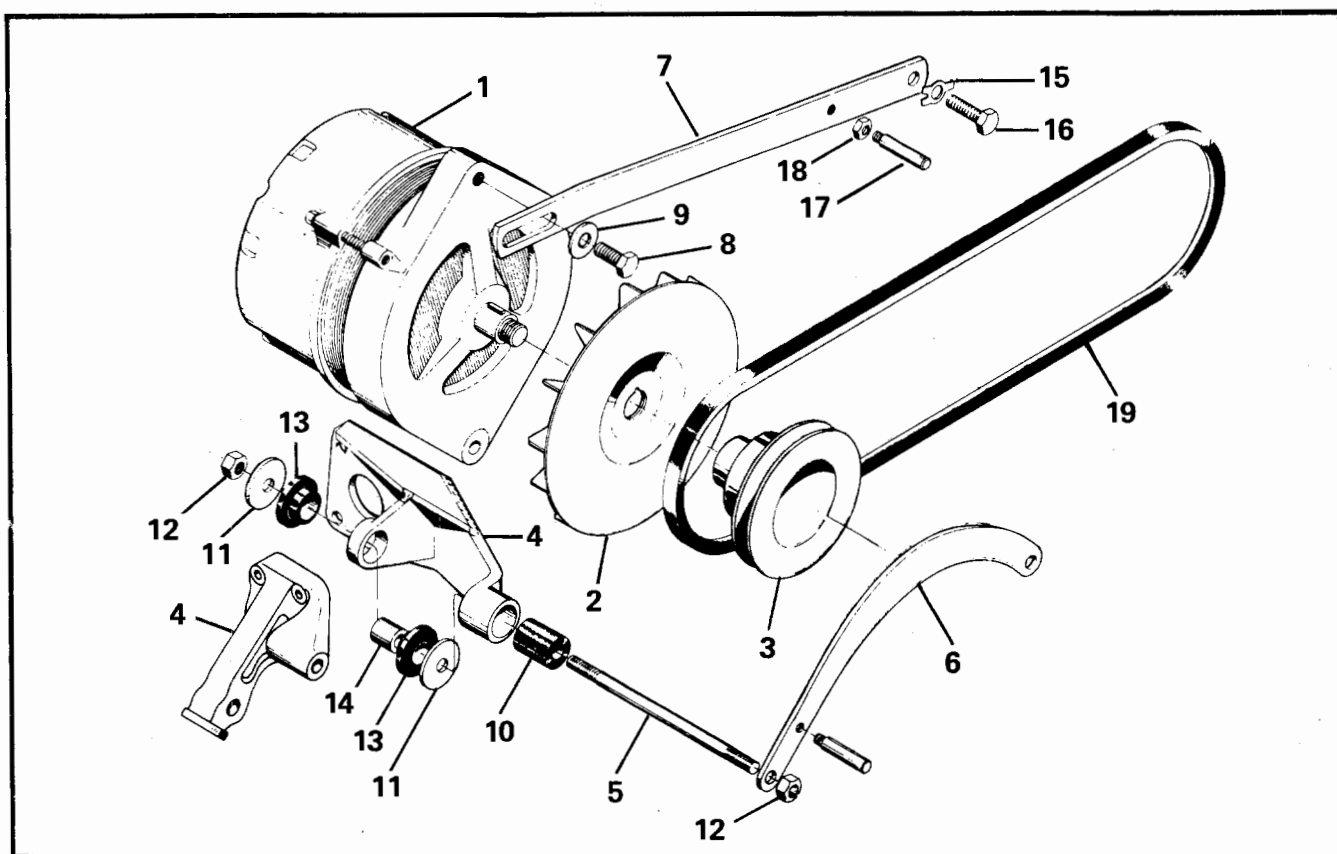
FIGURE 63. ALTERNATOR
