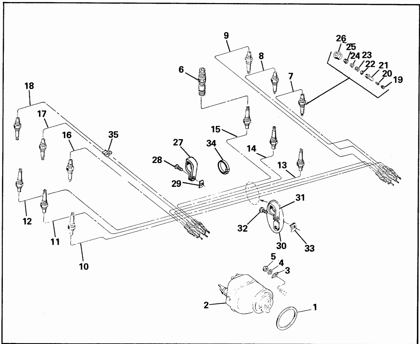
FIGURE 51. IGNITION SYSTEM
