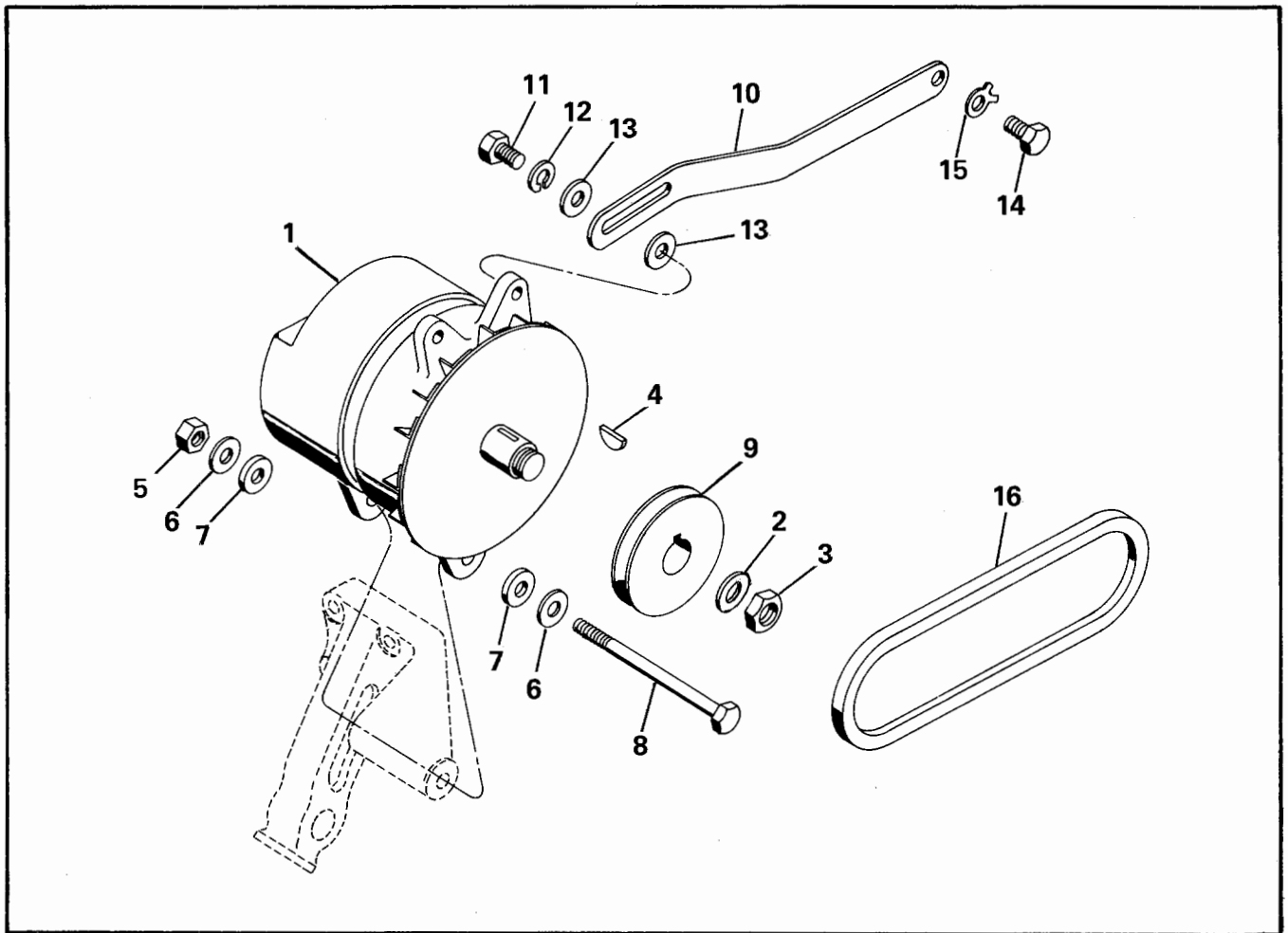
FIGURE 23. ALTERNATOR ASSEMBLY
