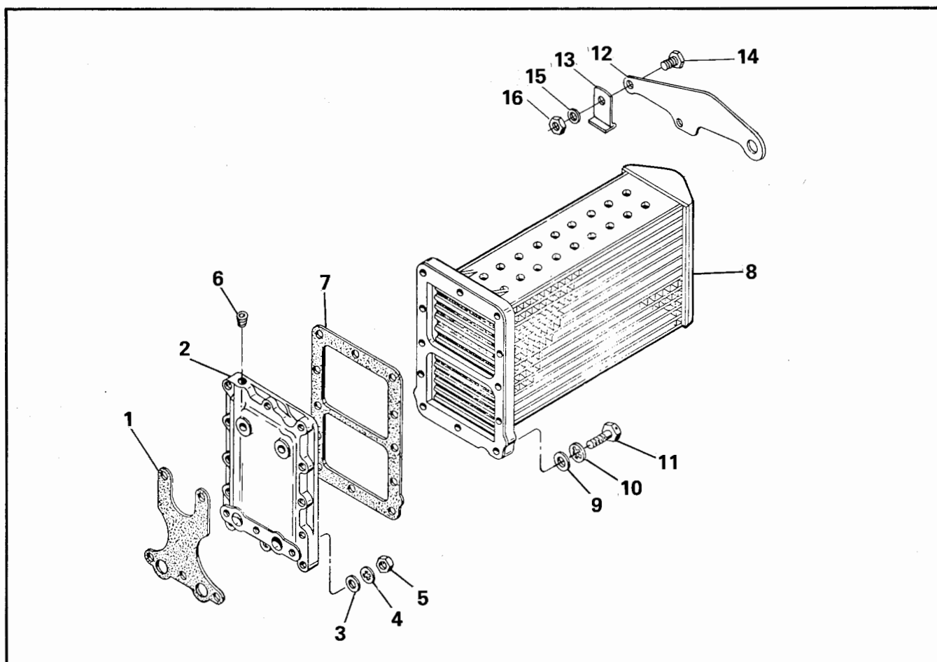
FIGURE 24. OIL COOLER
