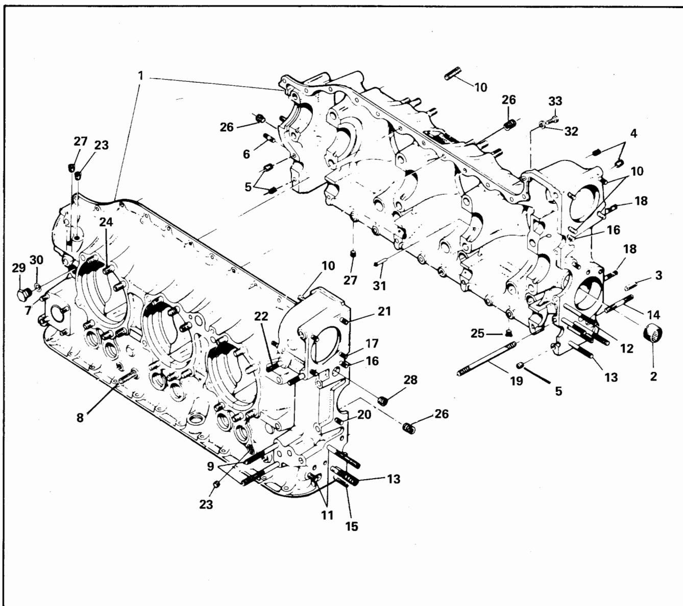
FIGURE 5. CRANKCASE STUDDING ASSEMBLY
