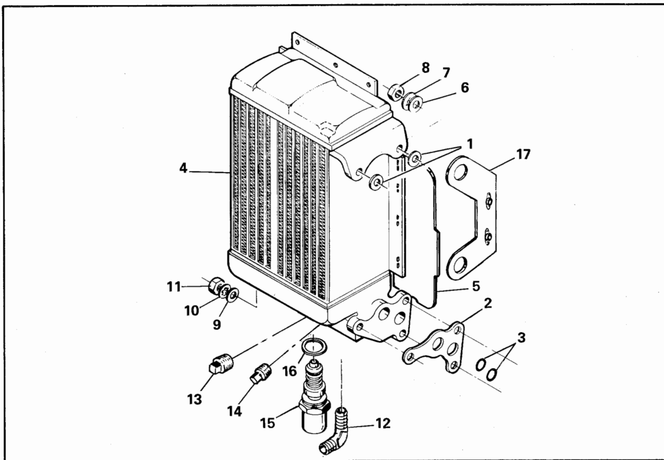
FIGURE 25. OIL COOLER
