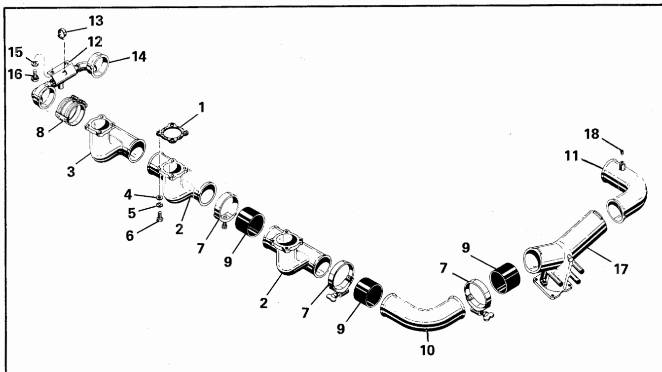
FIGURE 29. INDUCTION SYSTEM
