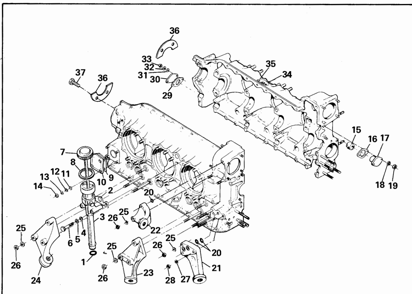
FIGURE 7. CRANKCASE ASSOCIATED PARTS
