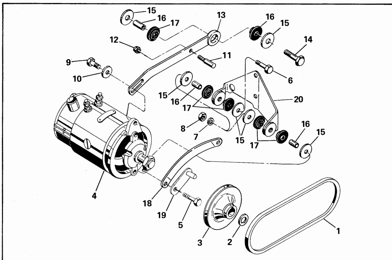
FIGURE 20. GENERATOR ASSEMBLY
