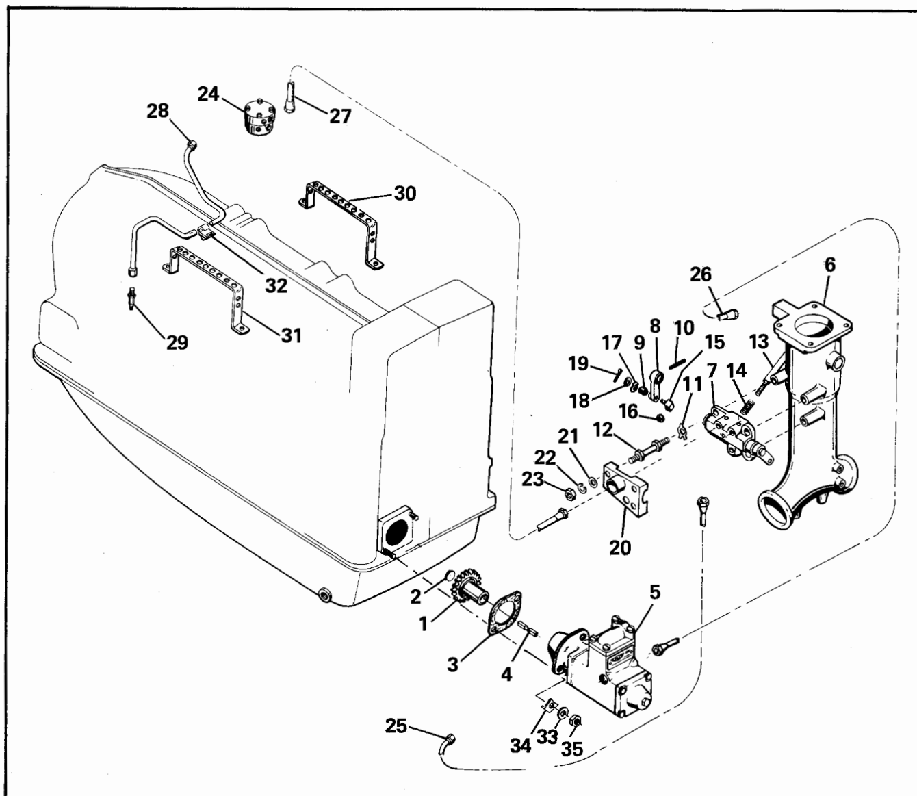
FIGURE 33. FUEL INJECTION SYSTEM
