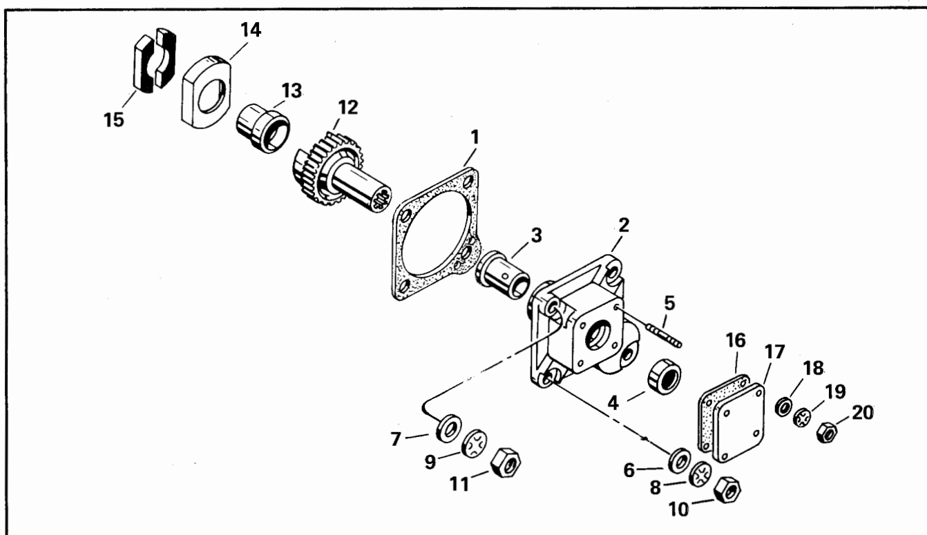
FIGURE 50. MAGNETO AND ACCESSORY DRIVE ASSEMBLY
