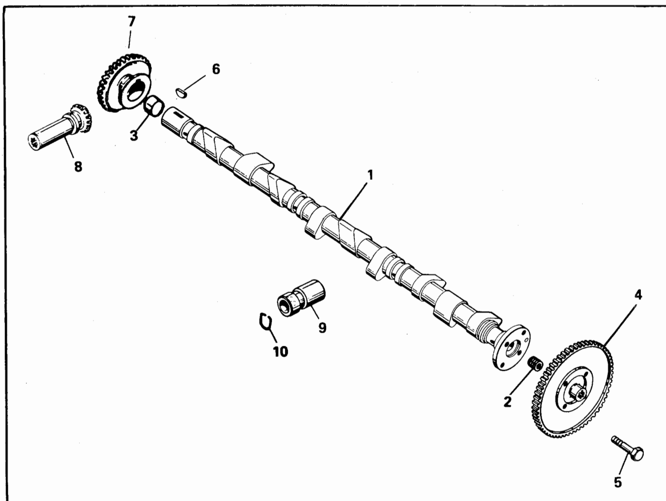
FIGURE 12. CAMSHAFT GROUP
