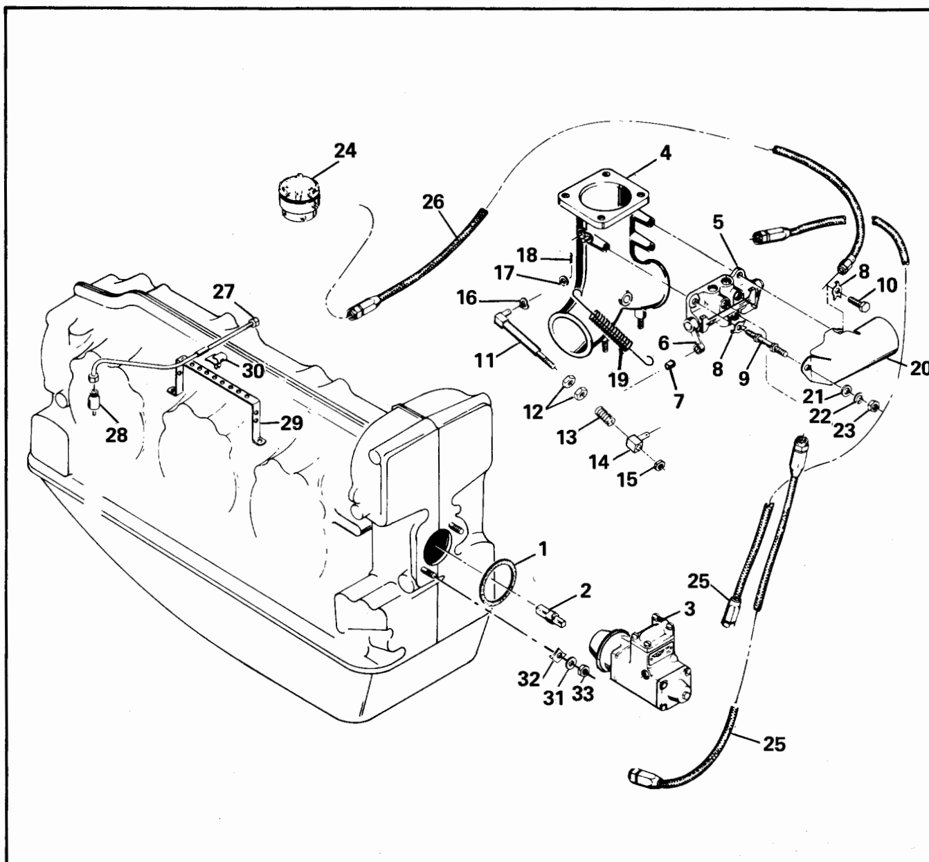
FIGURE 36. FUEL INJECTION SYSTEM
