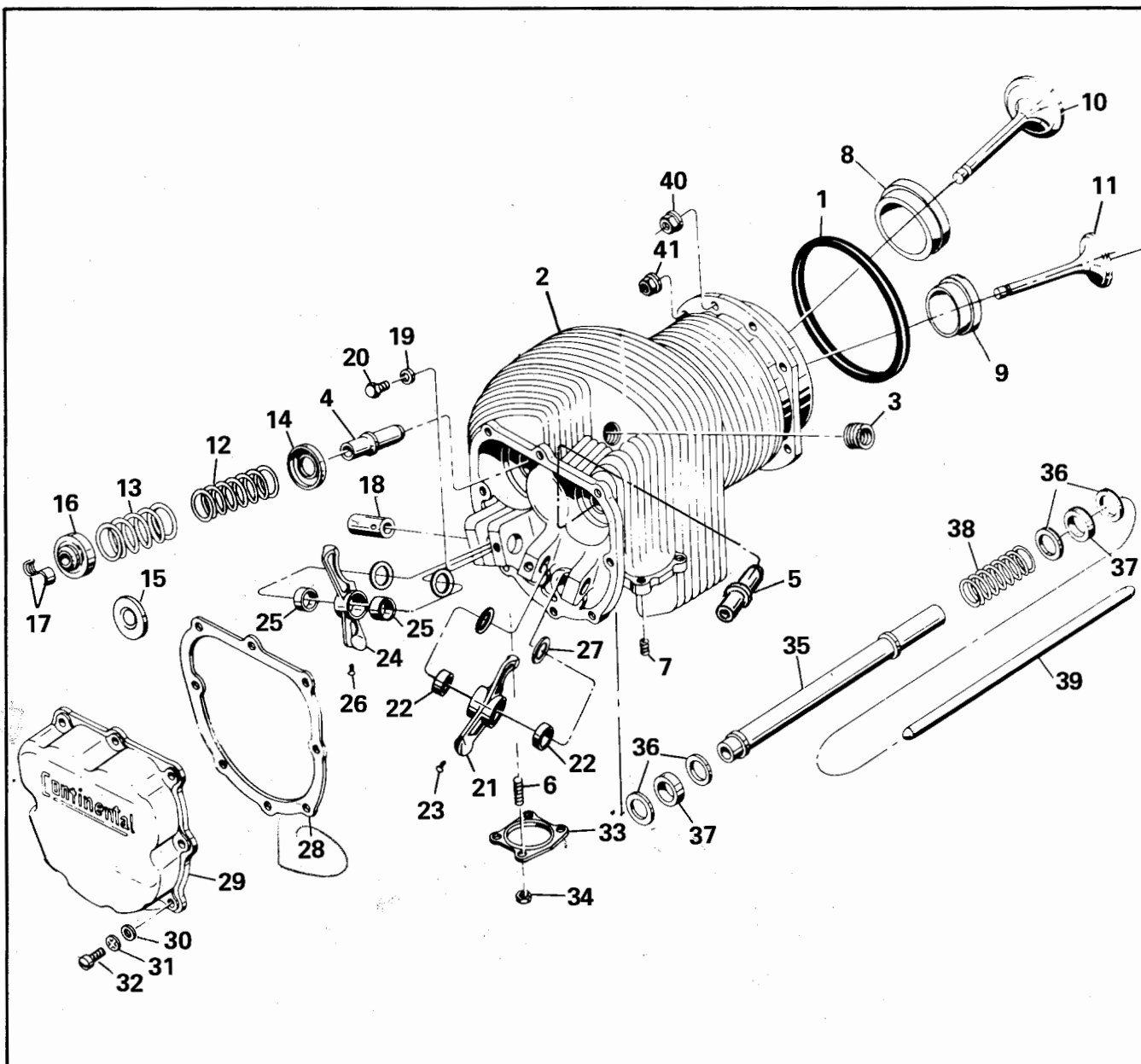
FIGURE 15. CYLINDER ASSEMBLY
