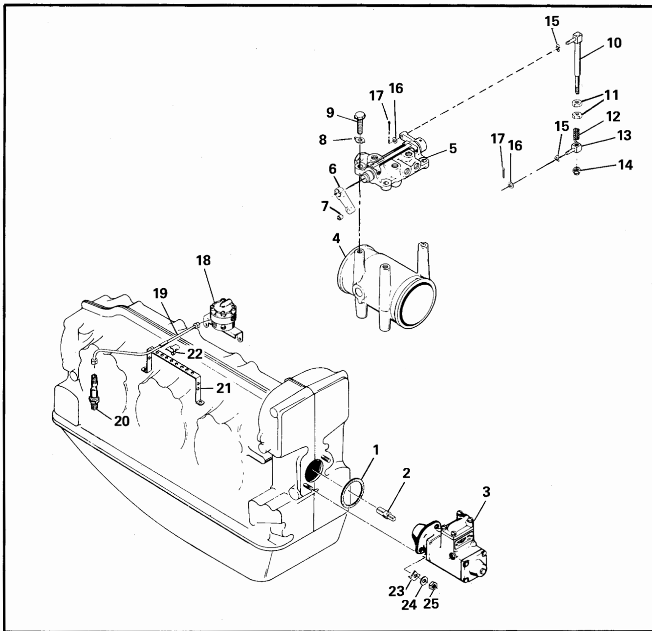
FIGURE 39. FUEL INJECTION SYSTEM
