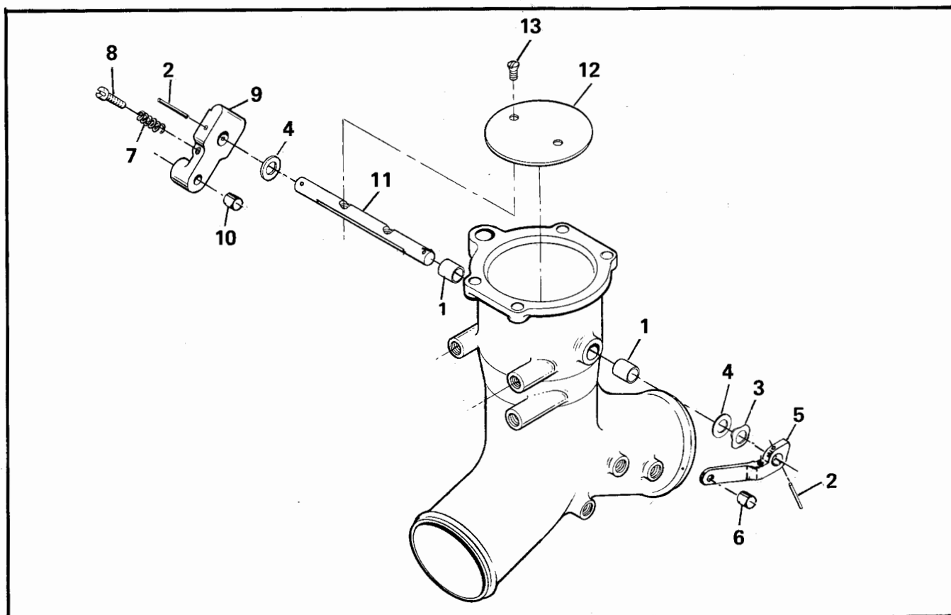
FIGURE 47. THROTTLE AND CONTROL ASSEMBLY
