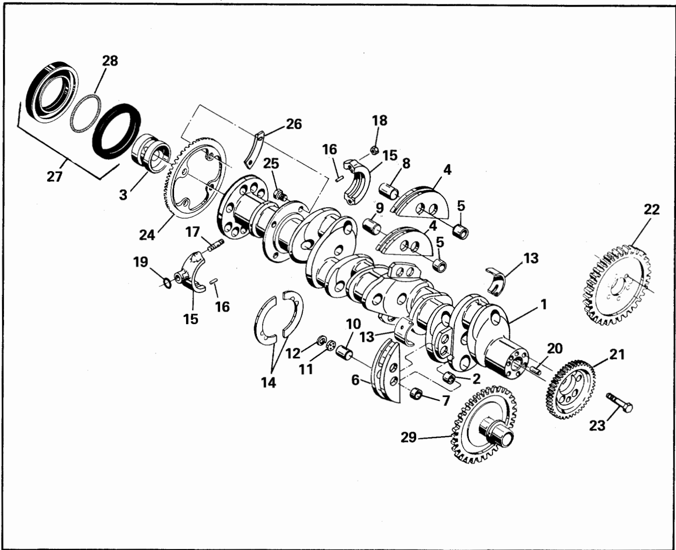
FIGURE 9. CRANKSHAFT GROUP
