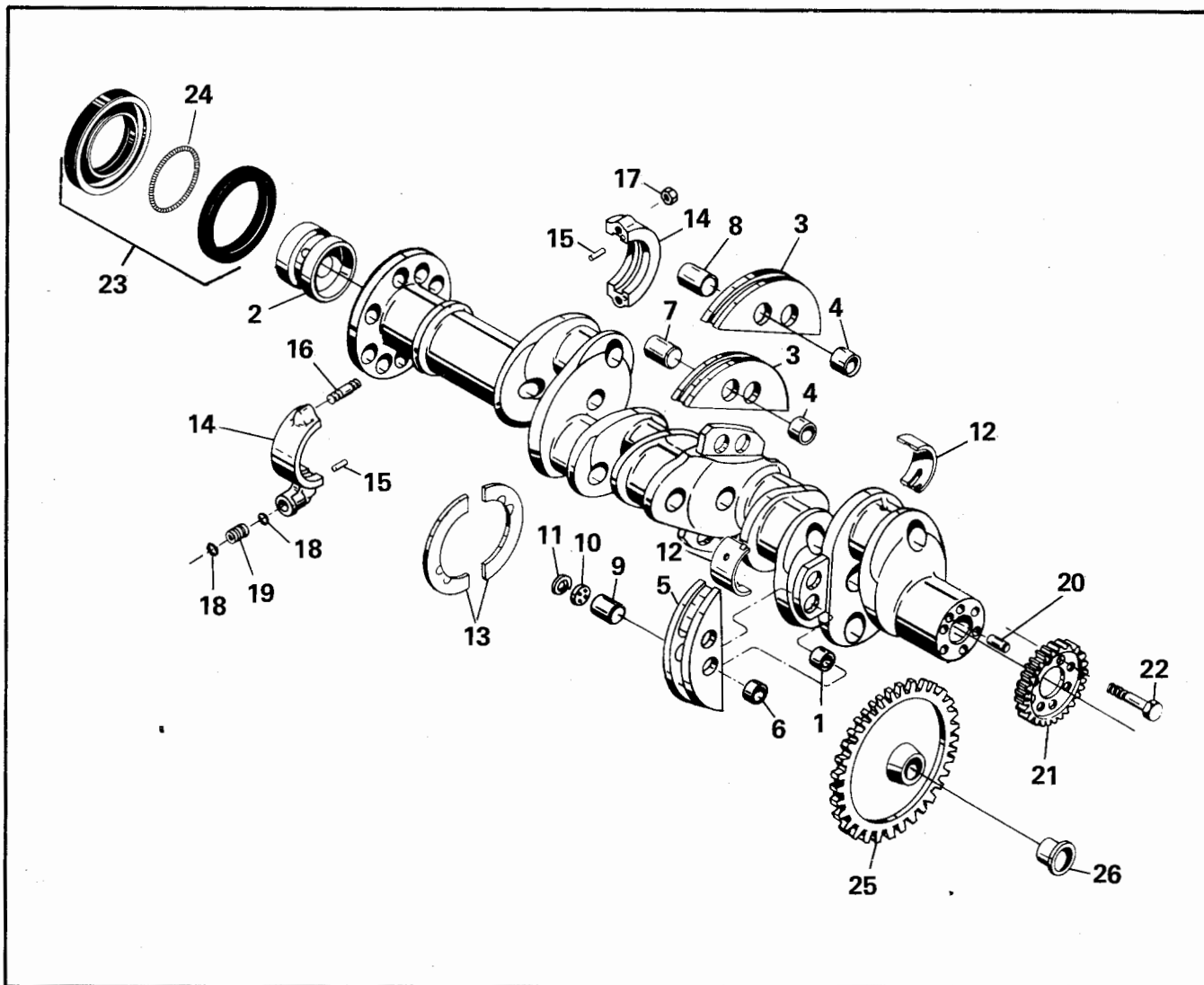
FIGURE 8. CRANKSHAFT GROUP
