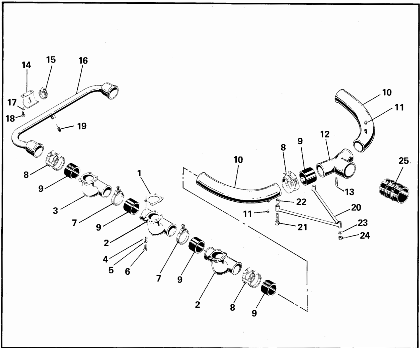
FIGURE 31. INDUCTION SYSTEM
