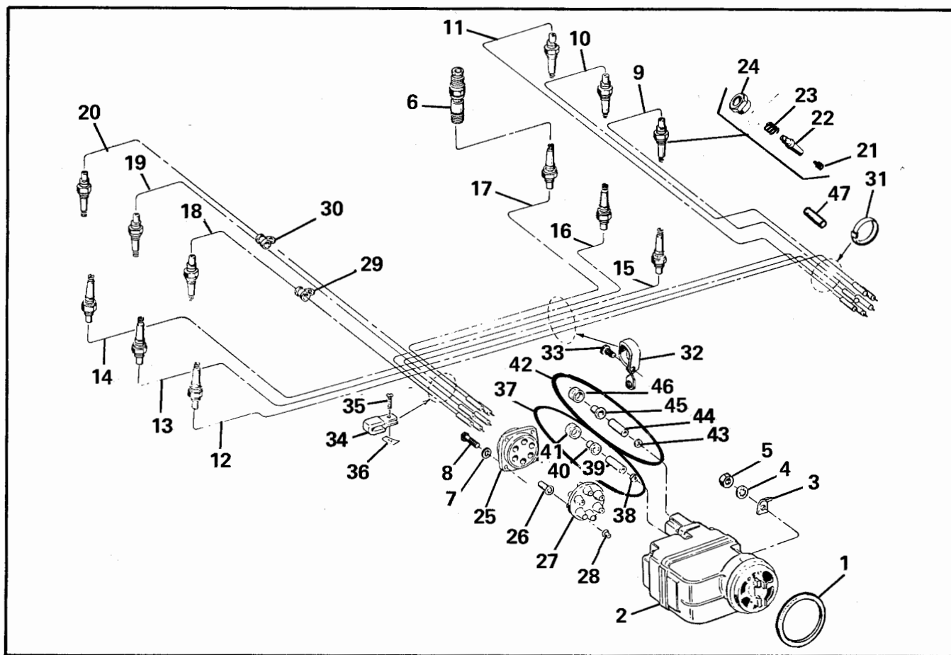
FIGURE 52. IGNITION SYSTEM
