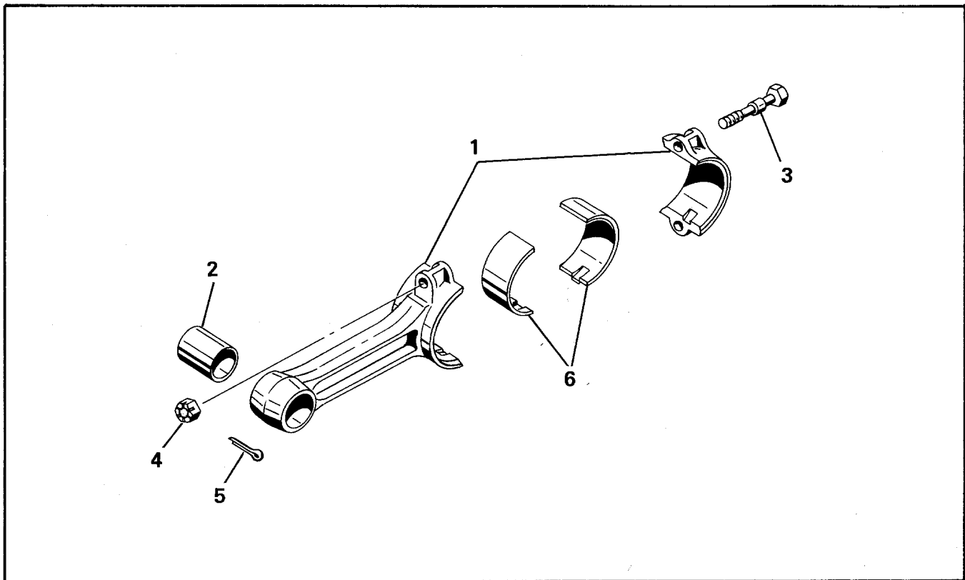
FIGURE 13. CONNECTING ROD ASSEMBLY
