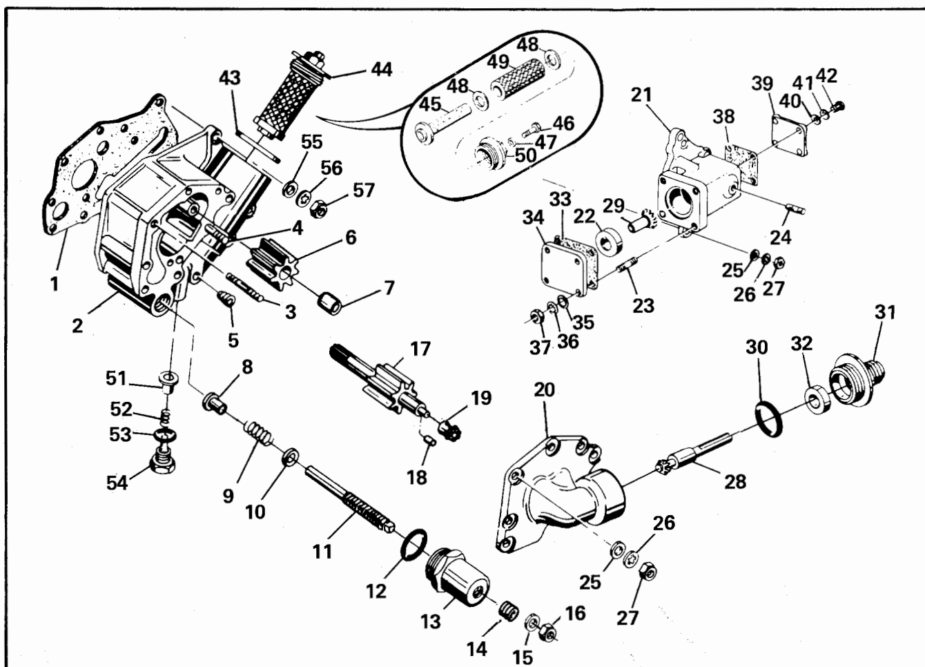
FIGURE 16. OIL PUMP ASSEMBLY (INTEGRAL TYPE OIL SCREEN)
