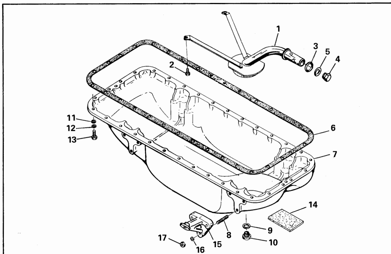
FIGURE 27. OIL SUMP
