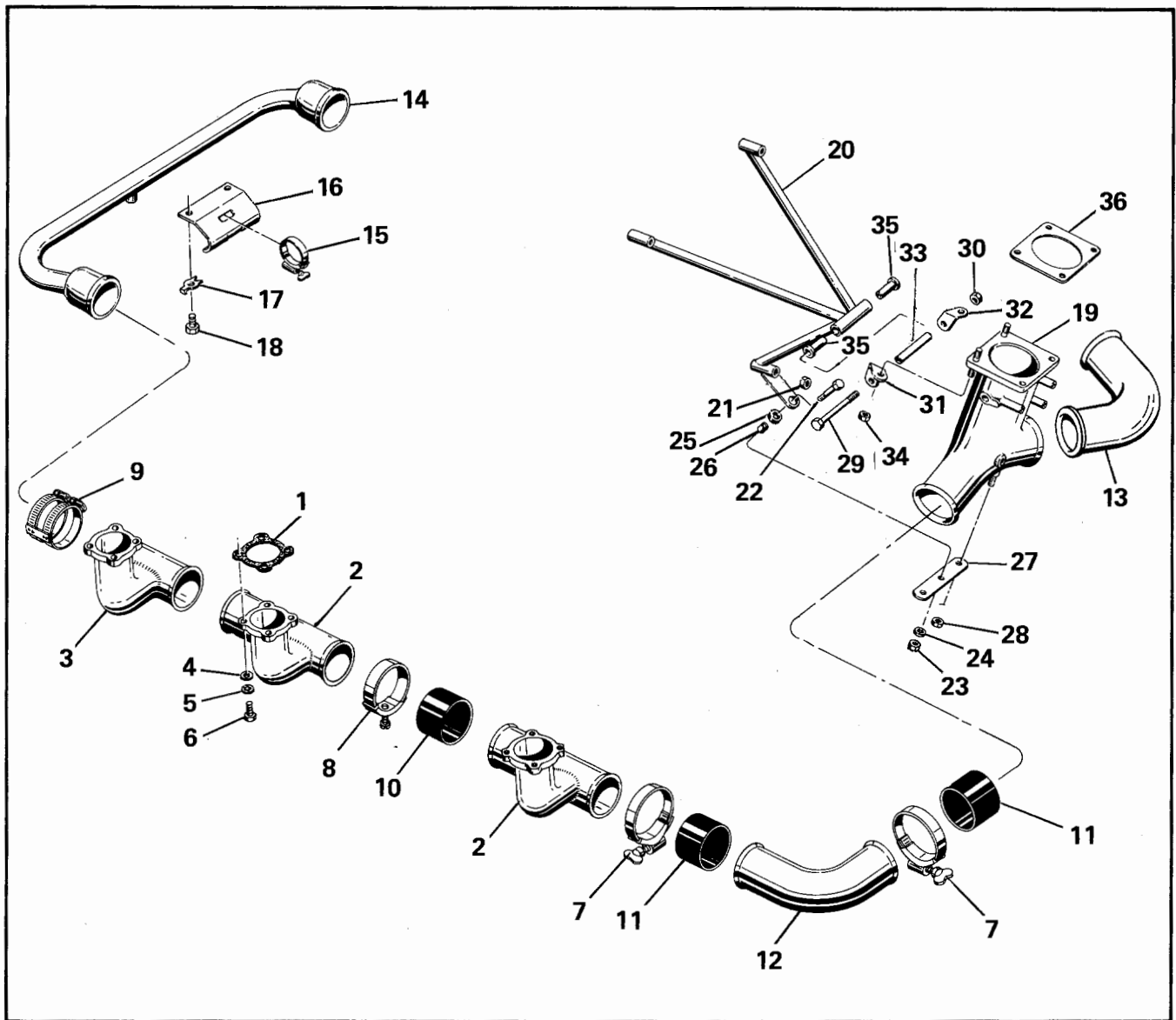
FIGURE 32. INDUCTION SYSTEM
