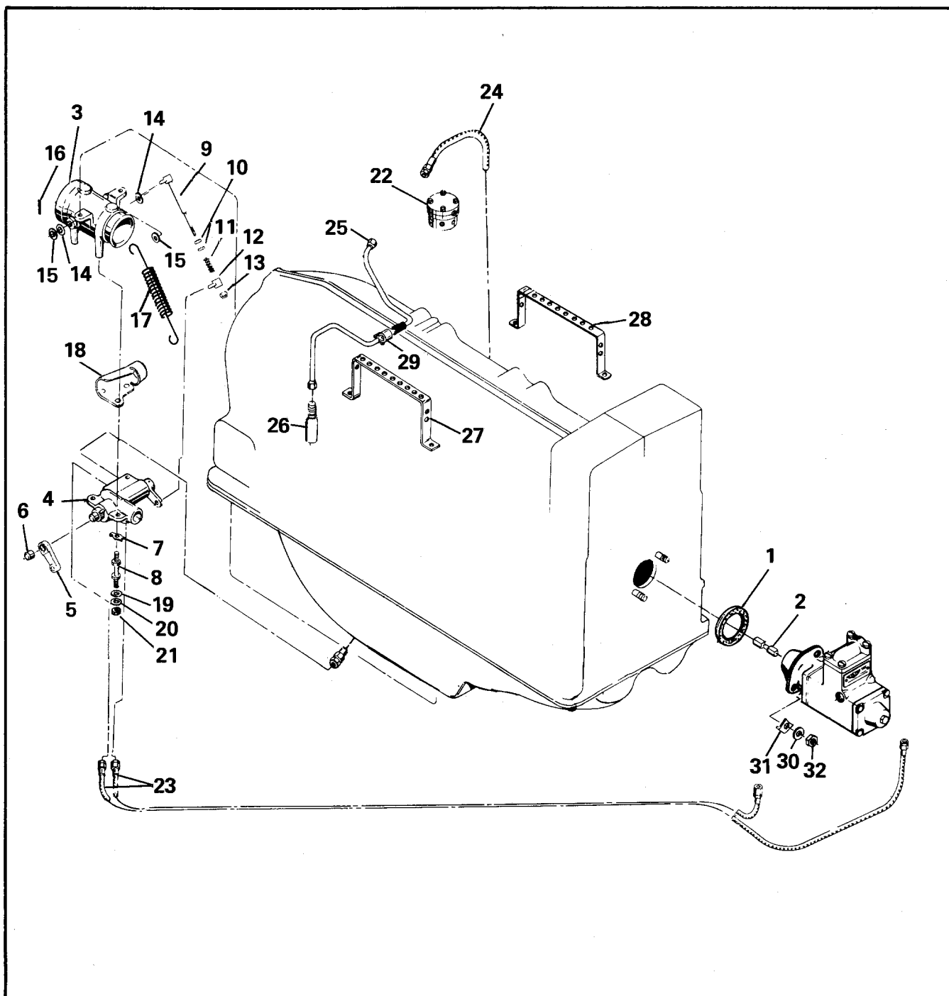
FIGURE 35. FUEL INJECTION SYSTEM
