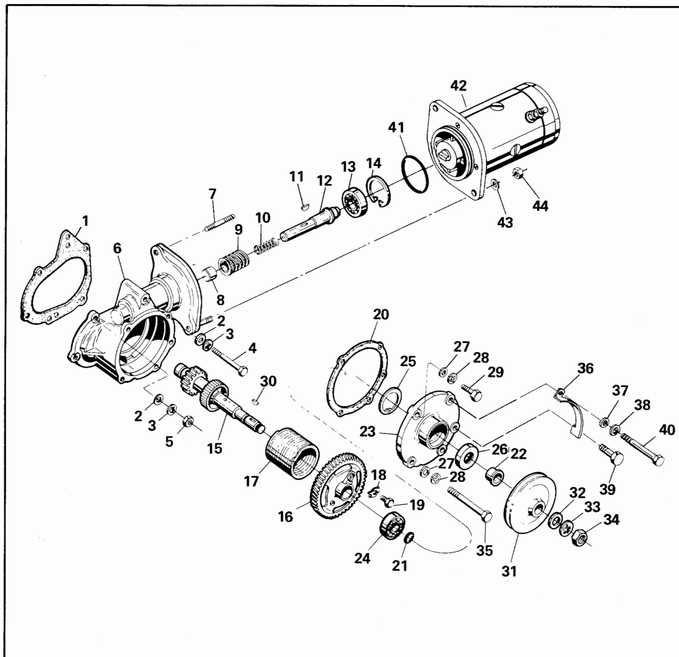
FIGURE 18. STARTER AND STARTER ADAPTER ASSEMBLY
