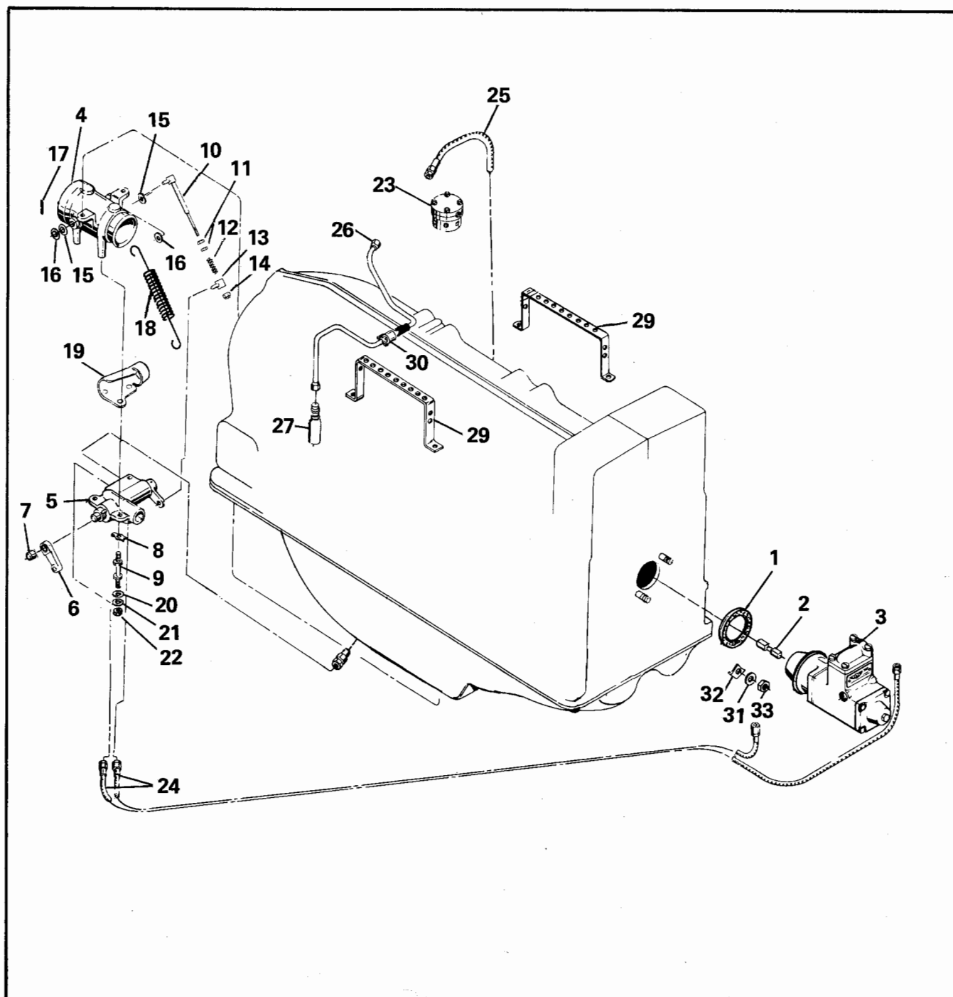
FIGURE 34. FUEL INJECTION SYSTEM
