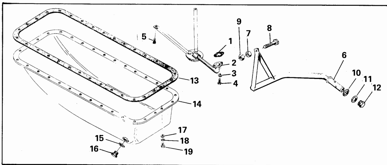
FIGURE 26. OIL SUMP
