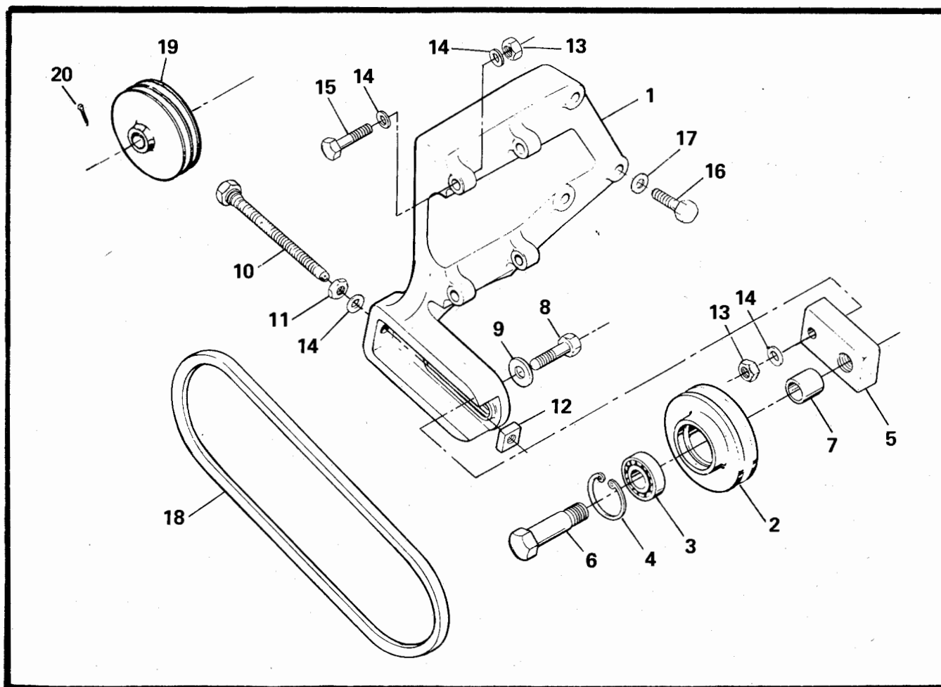
FIGURE 66. FREON COMPRESSOR BRACKET ASSEMBLY
