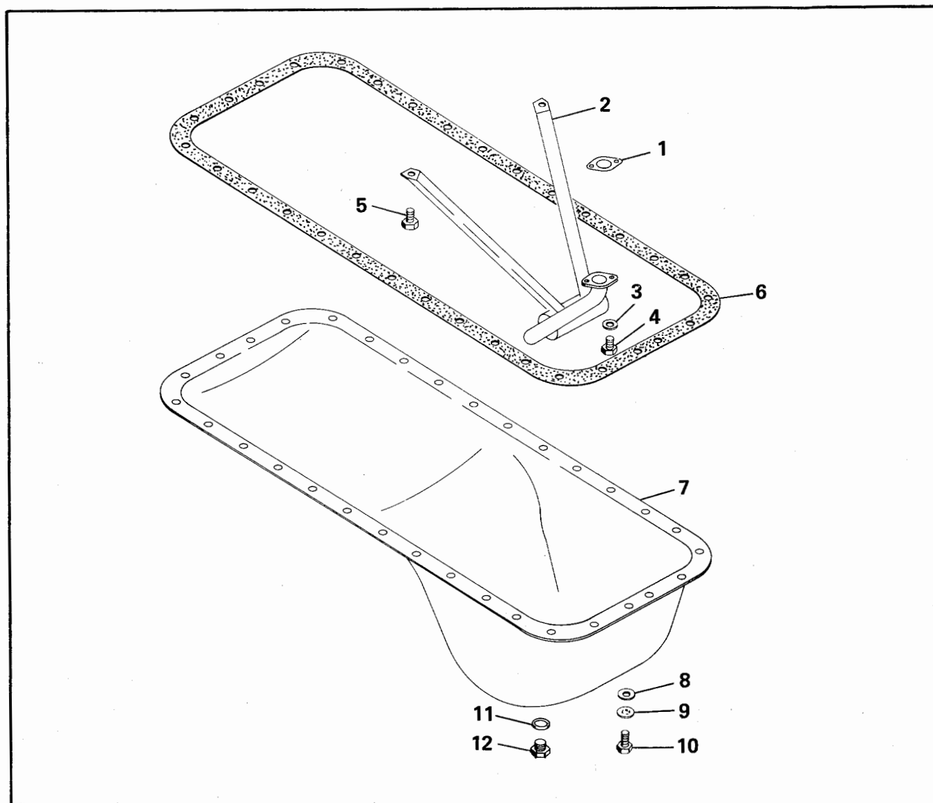
FIGURE 28. OIL SUMP
