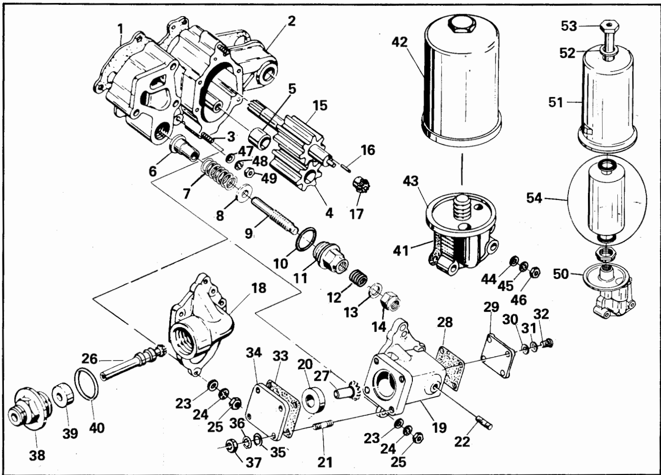
FIGURE 17. OIL PUMP ASSEMBLY (FULL FLOW TYPE FILTER)
