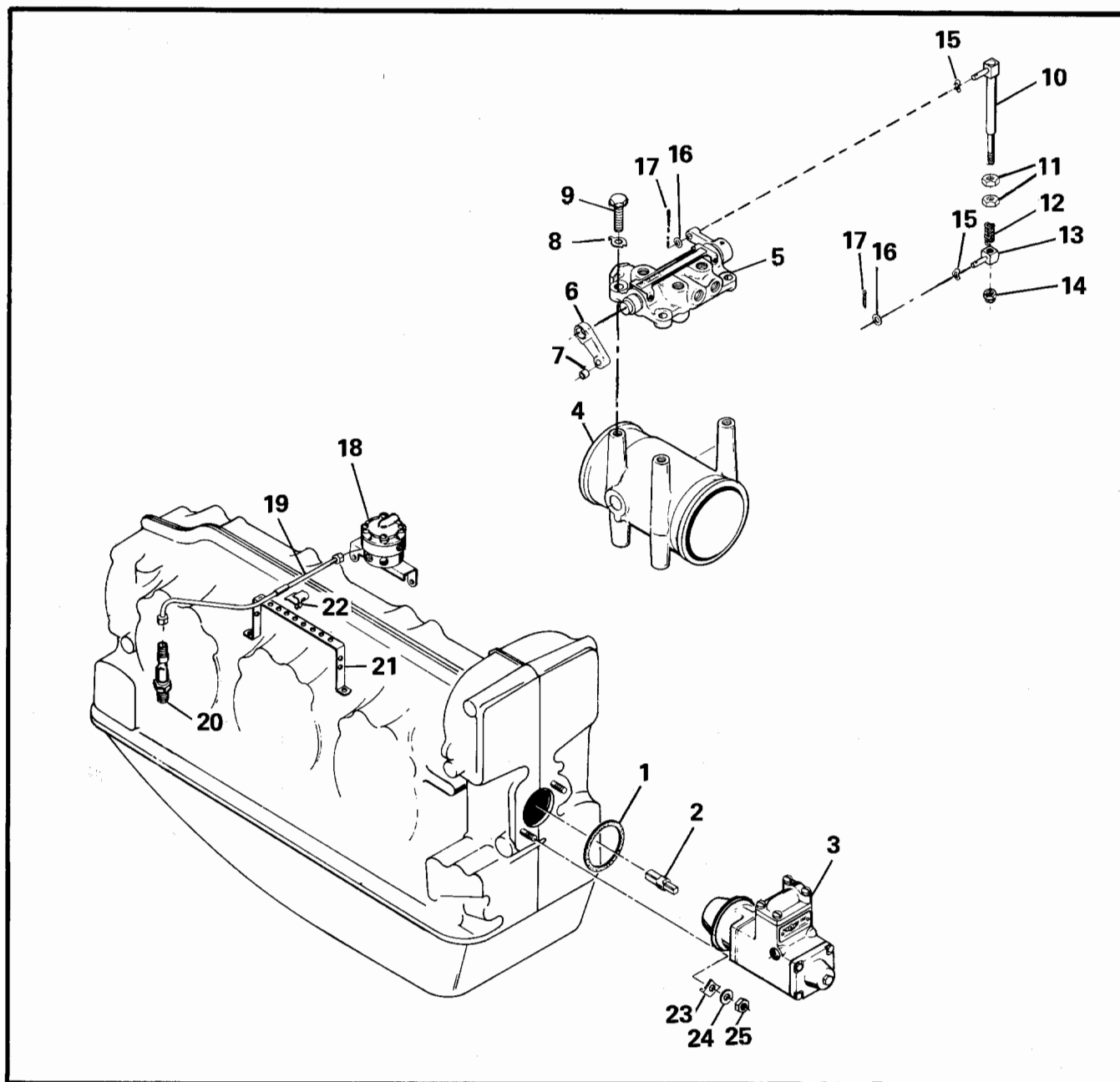
FIGURE 38. FUEL INJECTION SYSTEM
