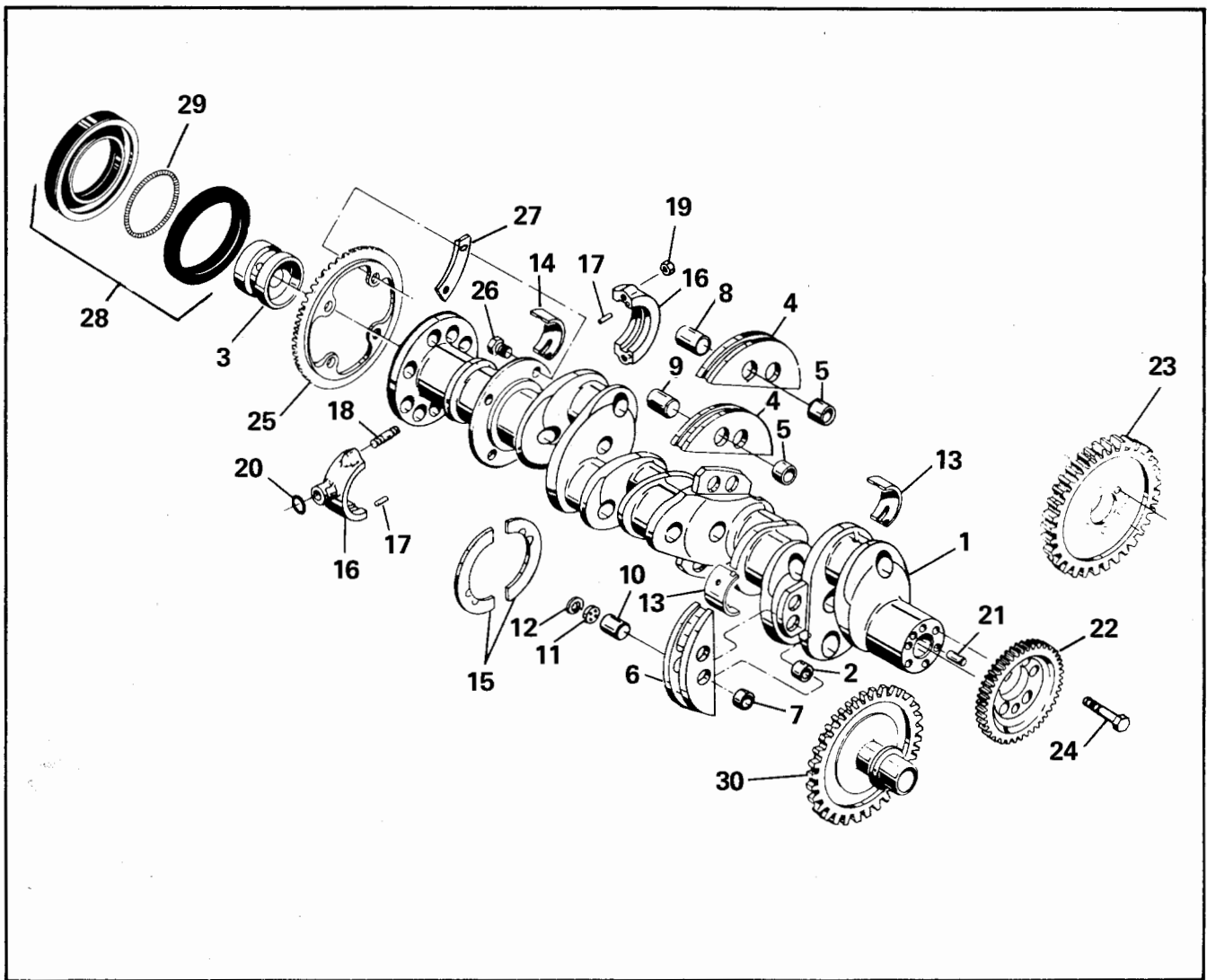
FIGURE 10. CRANKSHAFT GROUP
