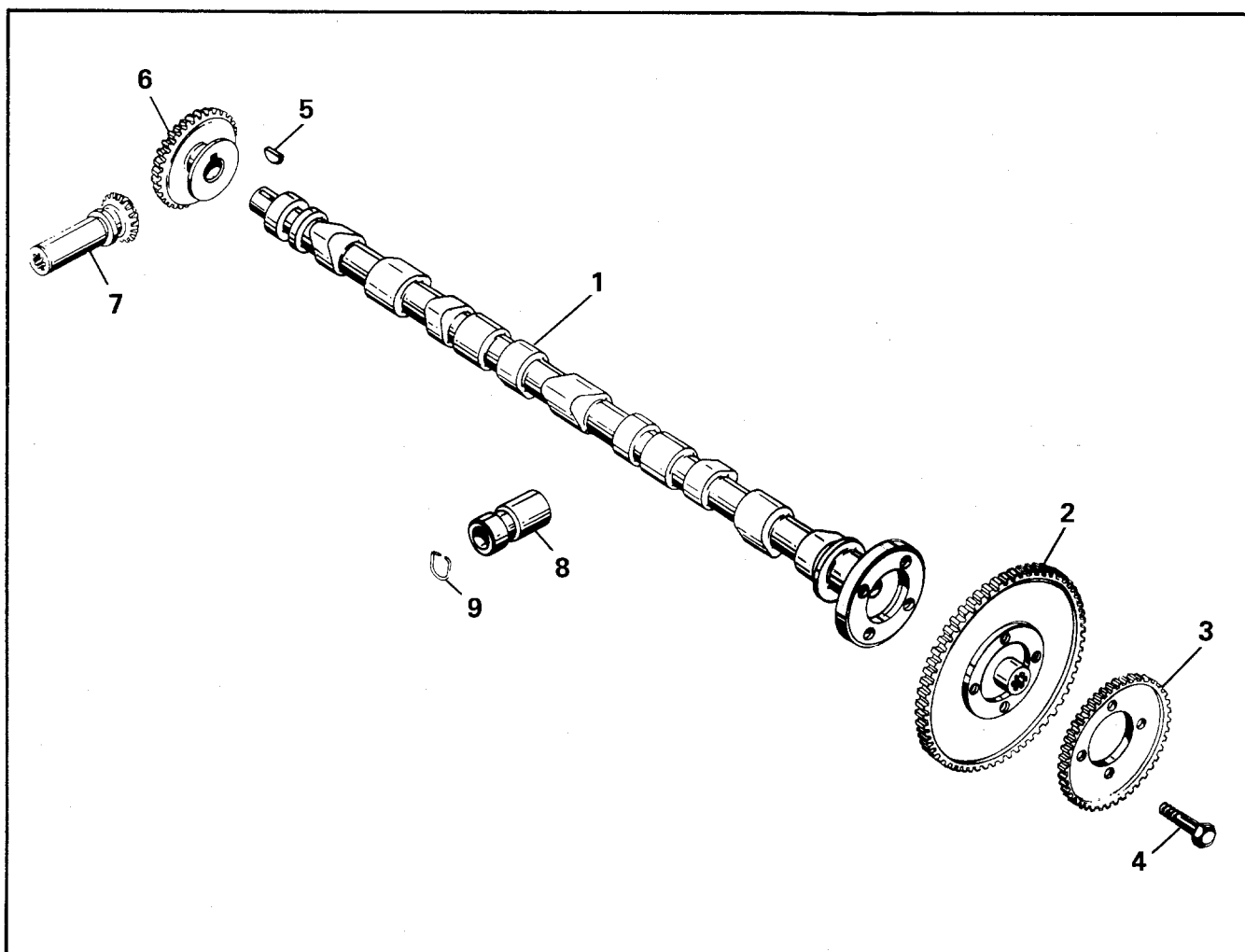
FIGURE 11. CAMSHAFT GROUP
