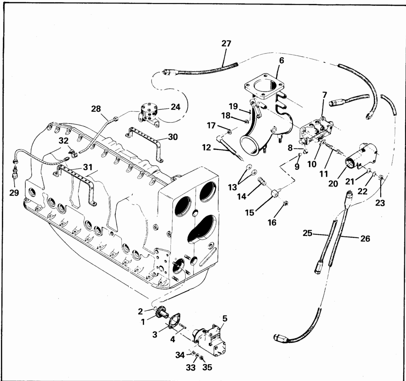
FIGURE 41. FUEL INJECTION SYSTEM
