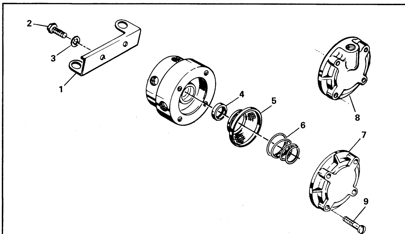
FIGURE 44. FUEL MANIFOLD VALVE ASSEMBLY
