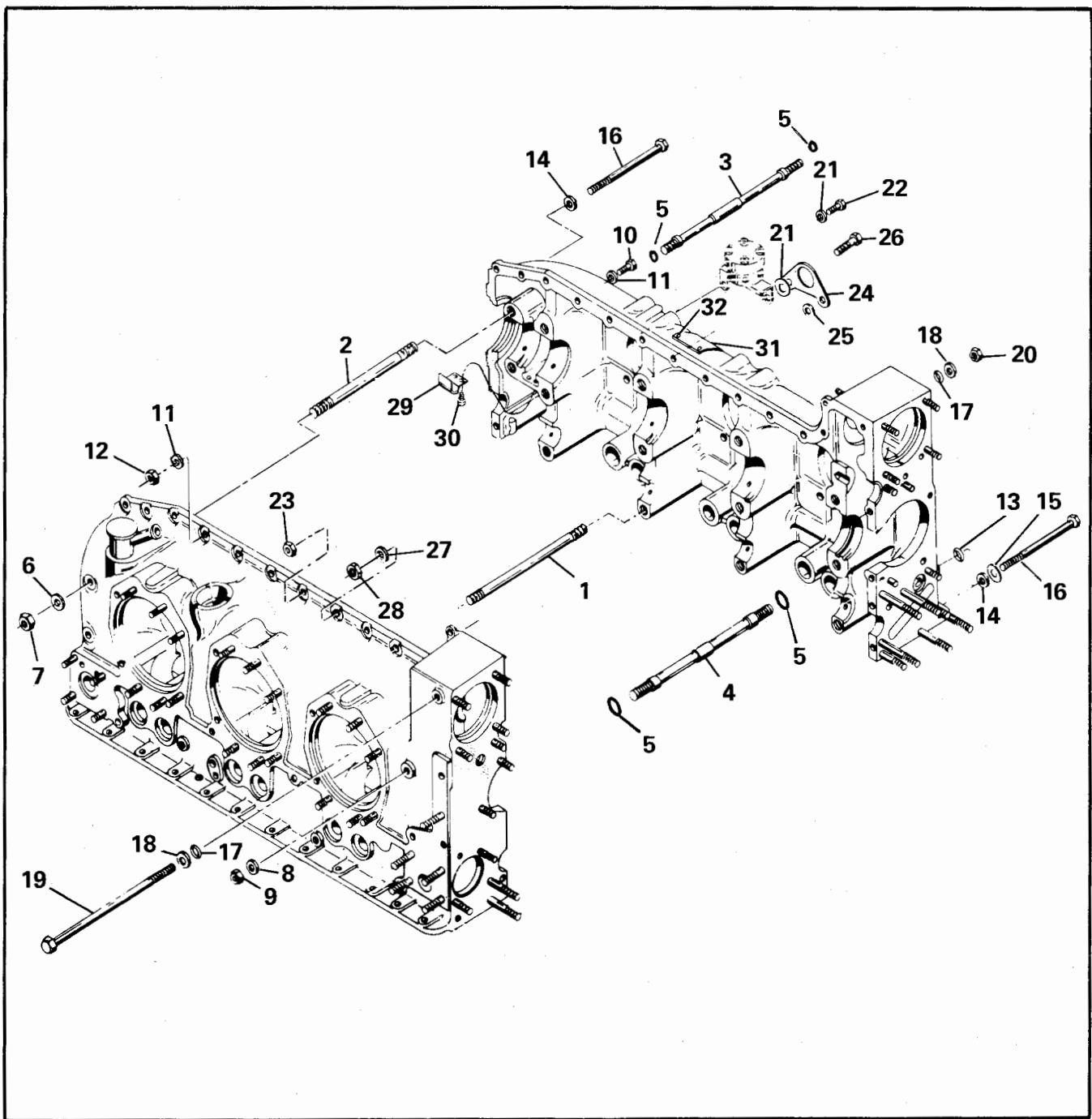
FIGURE 2. CRANKCASE ATTACHING PARTS
