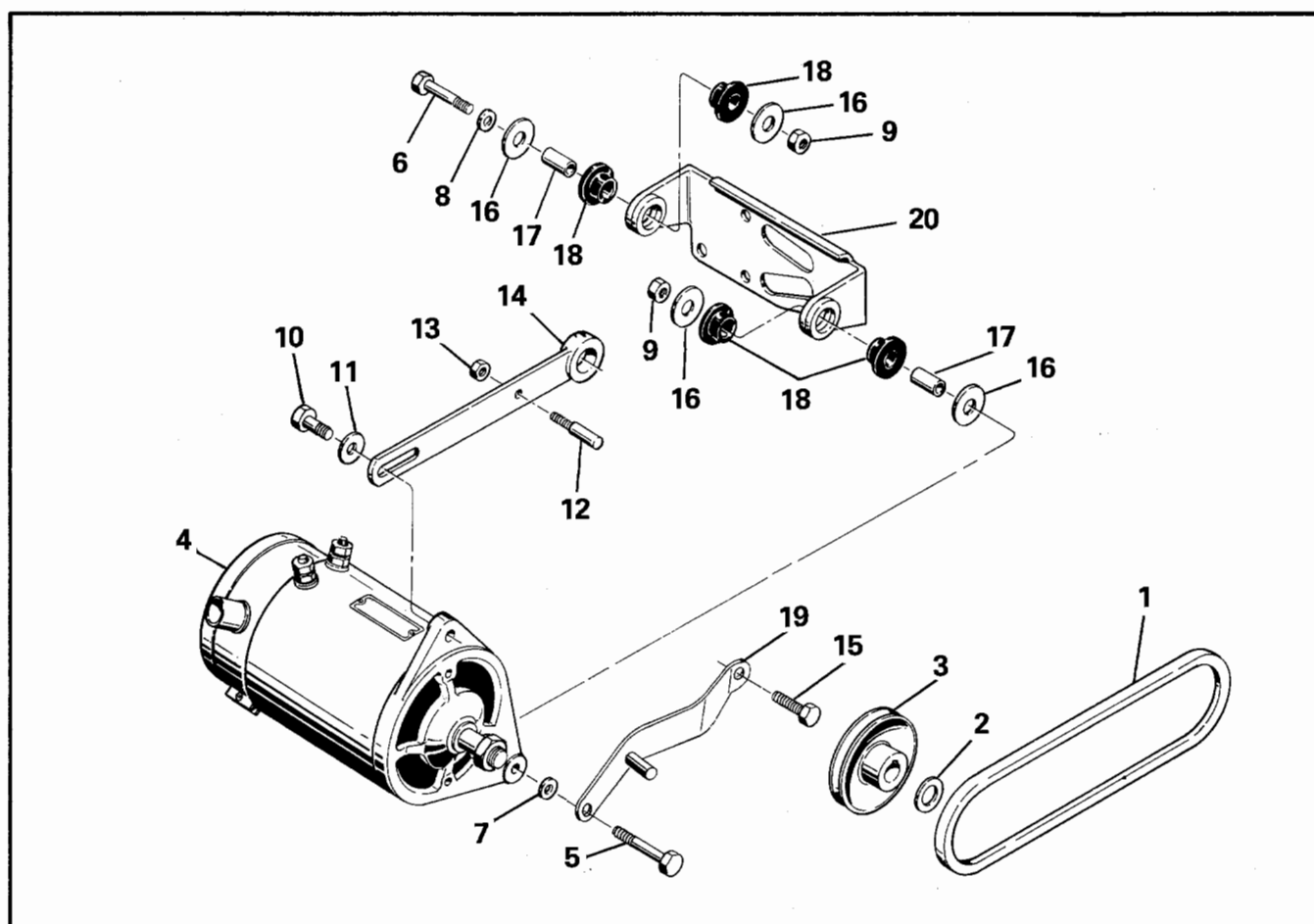
FIGURE 22. GENERATOR ASSEMBLY
