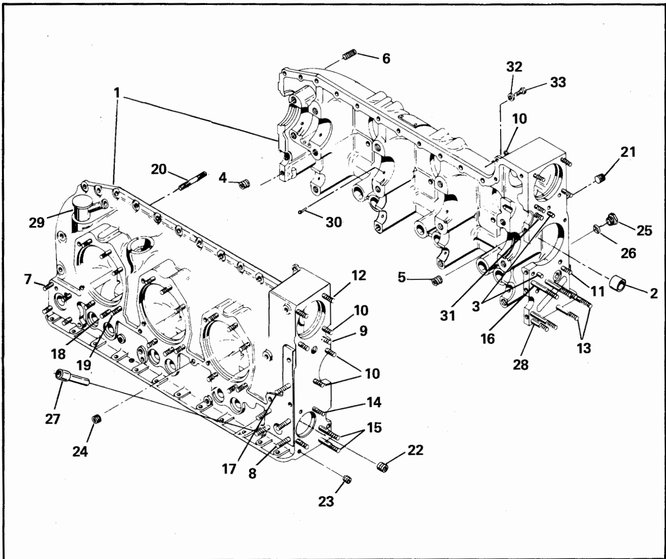
FIGURE 1. CRANKCASE STUDDING ASSEMBLY
