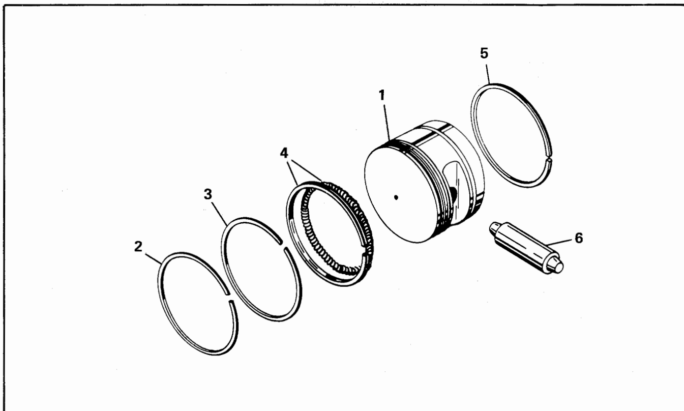
FIGURE 14. PISTON AND PIN ASSEMBLY
