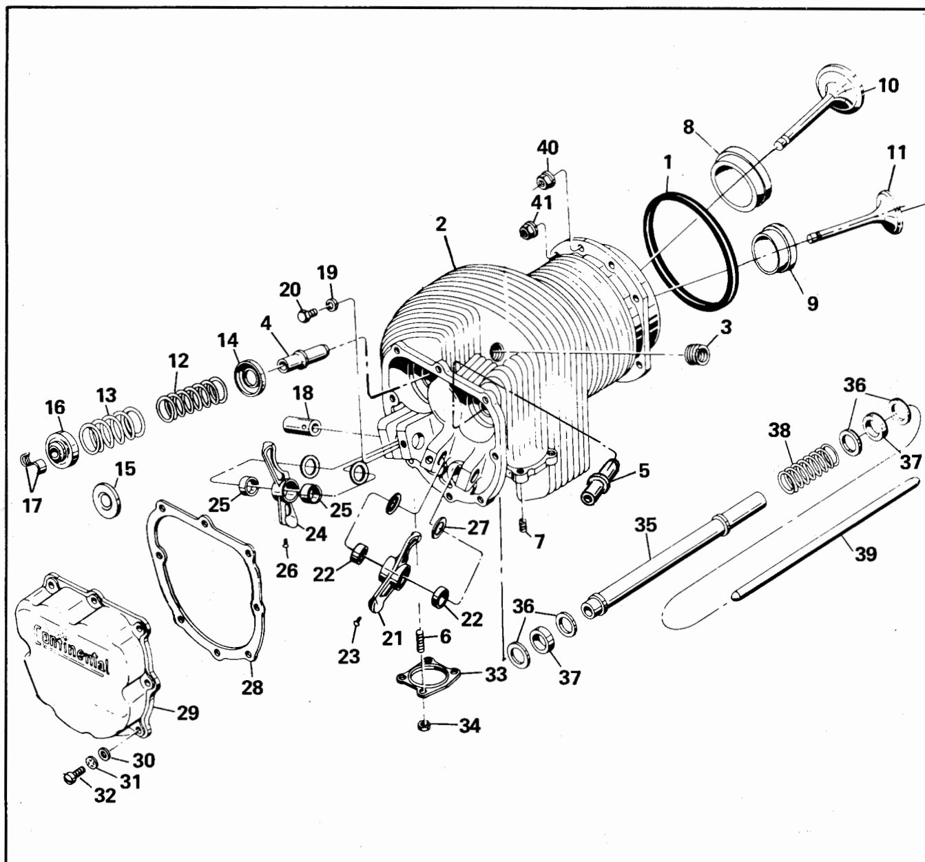
FIGURE 64. CYLINDER ASSEMBLY
