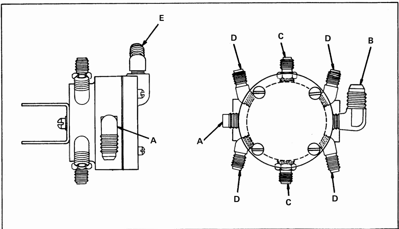
FIGURE 45. FUEL MANIFOLD VALVE FITTING LOCATIONS
