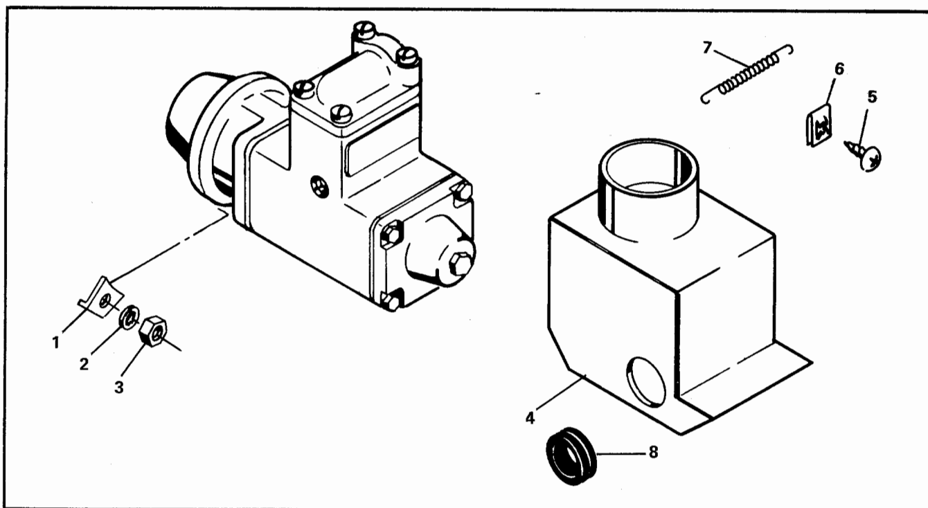
FIGURE 42. FUEL PUMP AND VAPOR SEPARATOR ASSEMBLY
