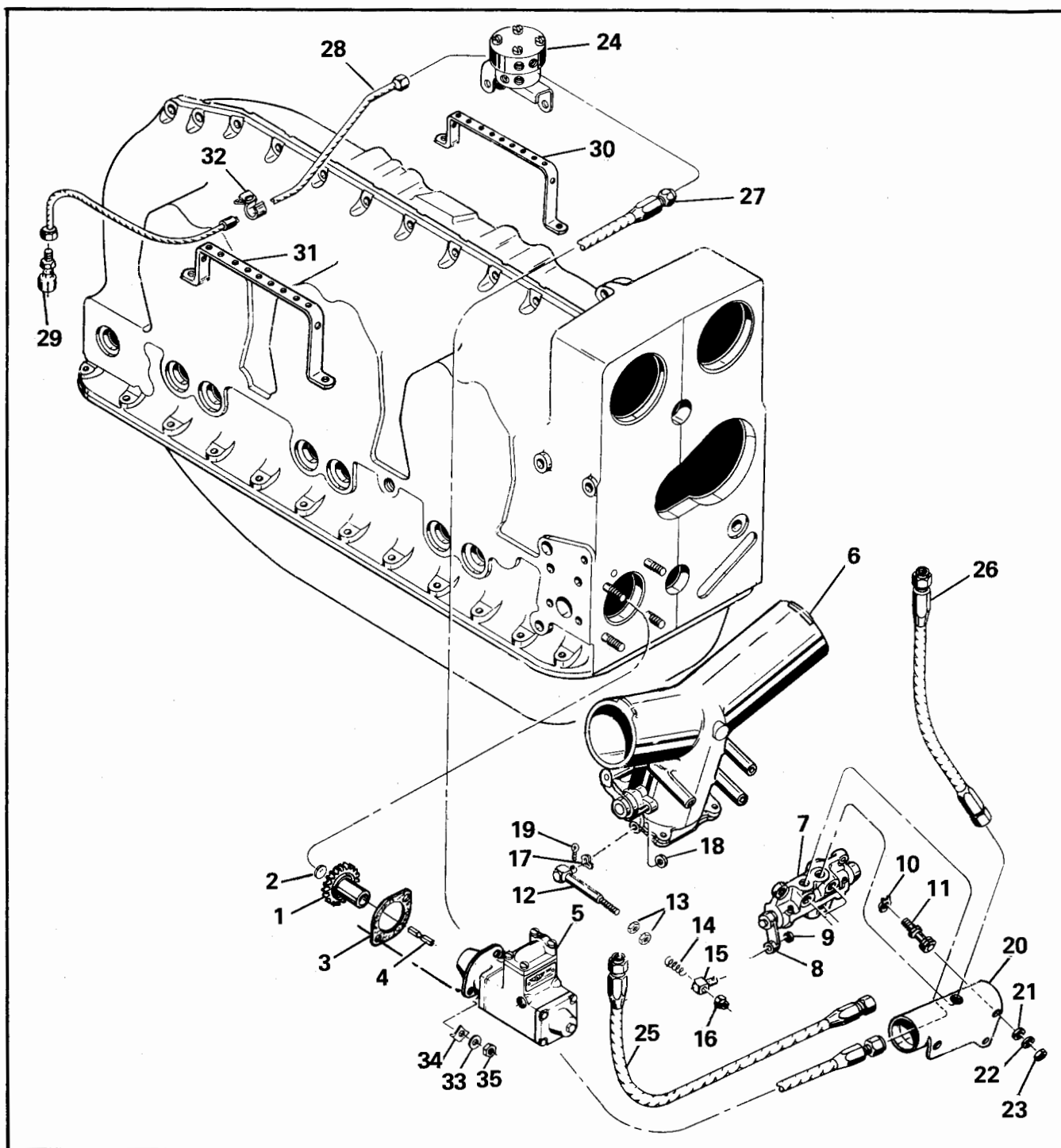
FIGURE 40. FUEL INJECTION SYSTEM
