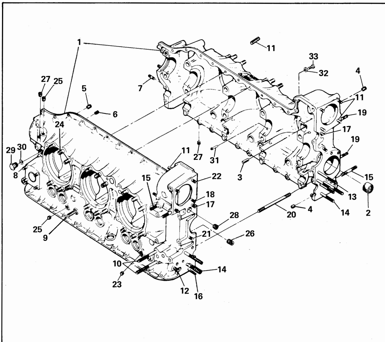
FIGURE 4. CRANKCASE STUDDING ASSEMBLY
