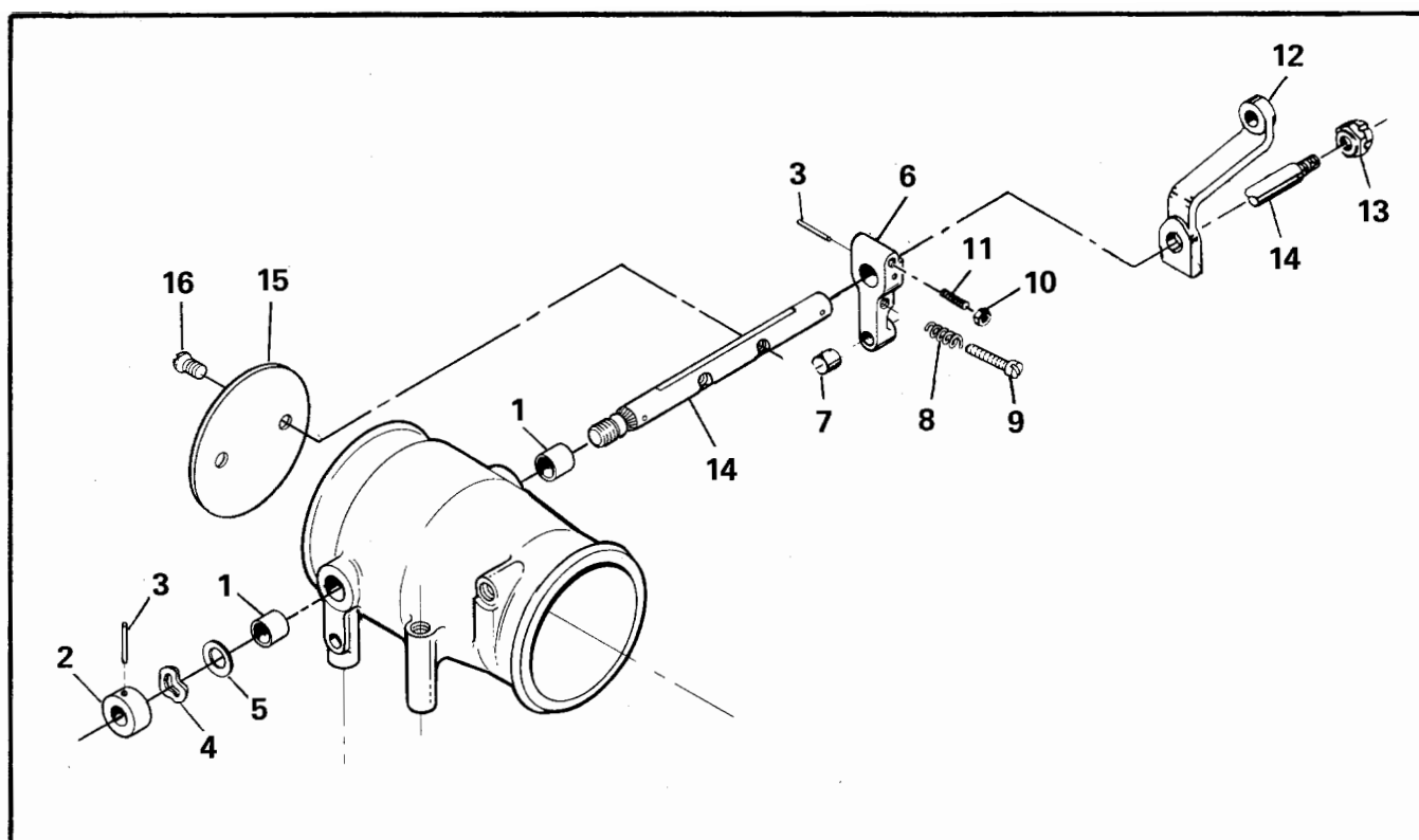
FIGURE 49. THROTTLE AND CONTROL ASSEMBLY
