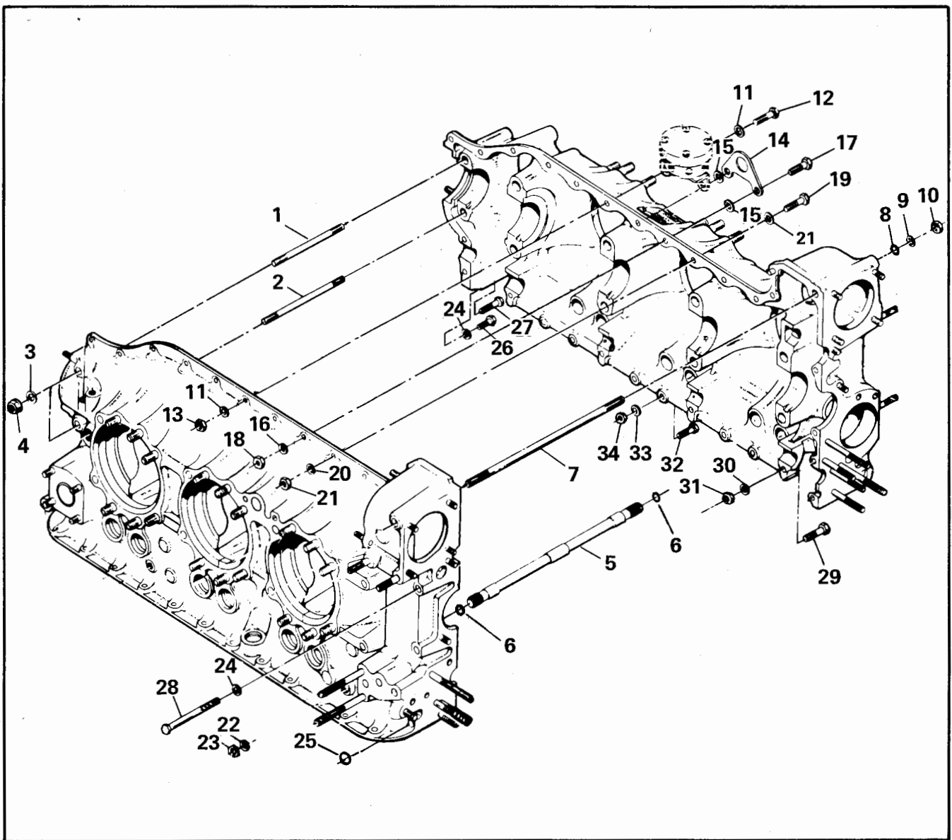
FIGURE 6. CRANKCASE ATTACHING PARTS
