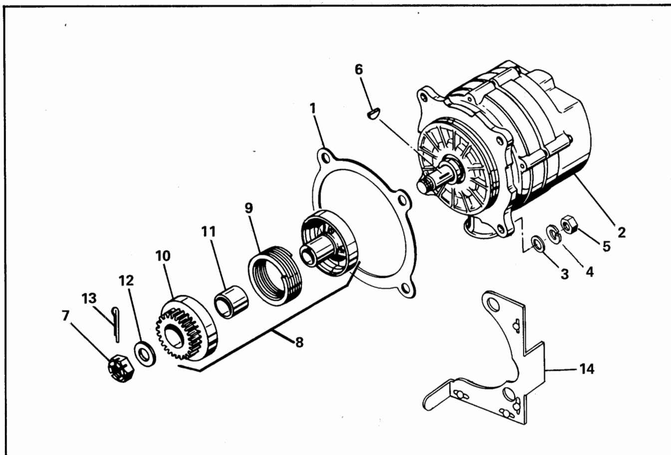
FIGURE 21. ALTERNATOR ASSEMBLY
