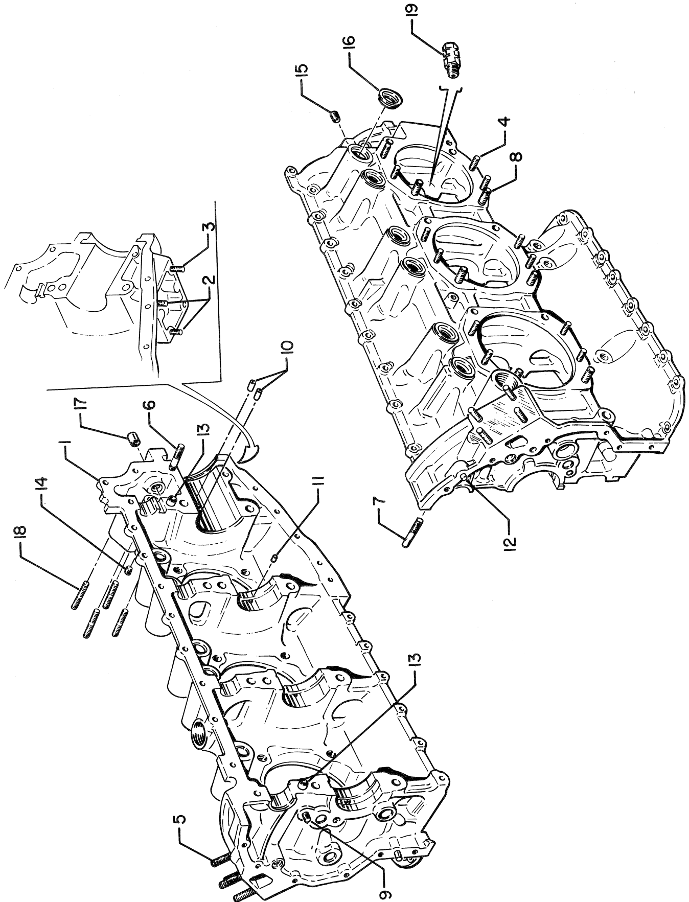
Figure 1 - Crankcase Assembly
