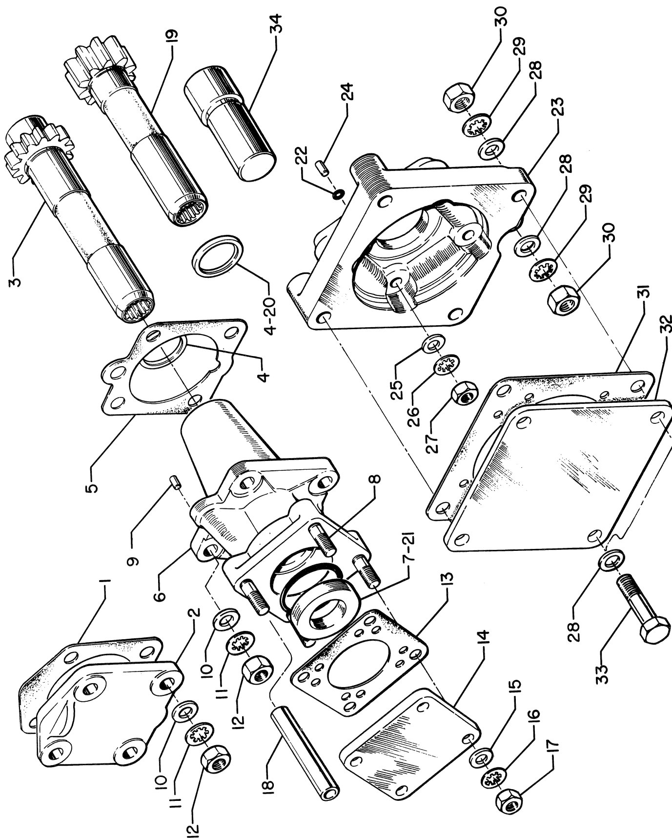
Figure 12 - Hydraulic Pump Drive and Covers
