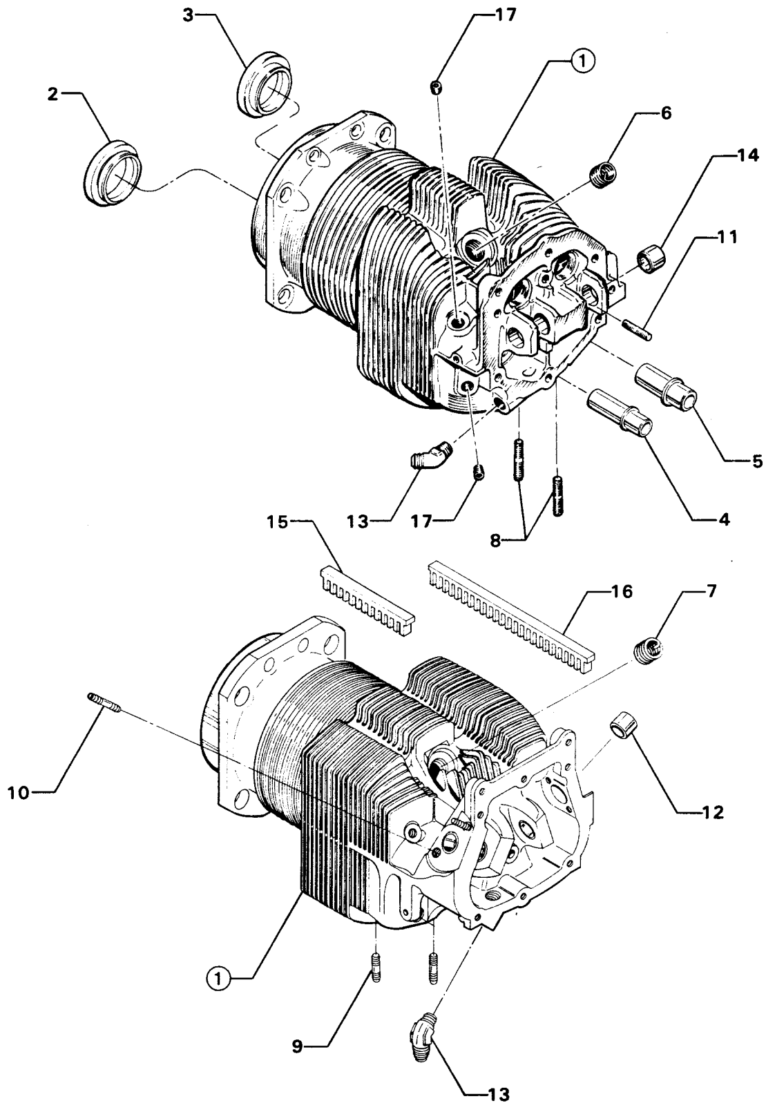
Figure 18. CYLINDER ASSEMBLY
