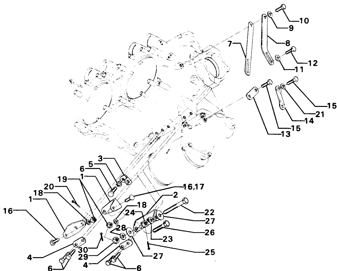
Figure 30. ALTERNATOR AND GENERATOR MOUNTING BRACKETS
