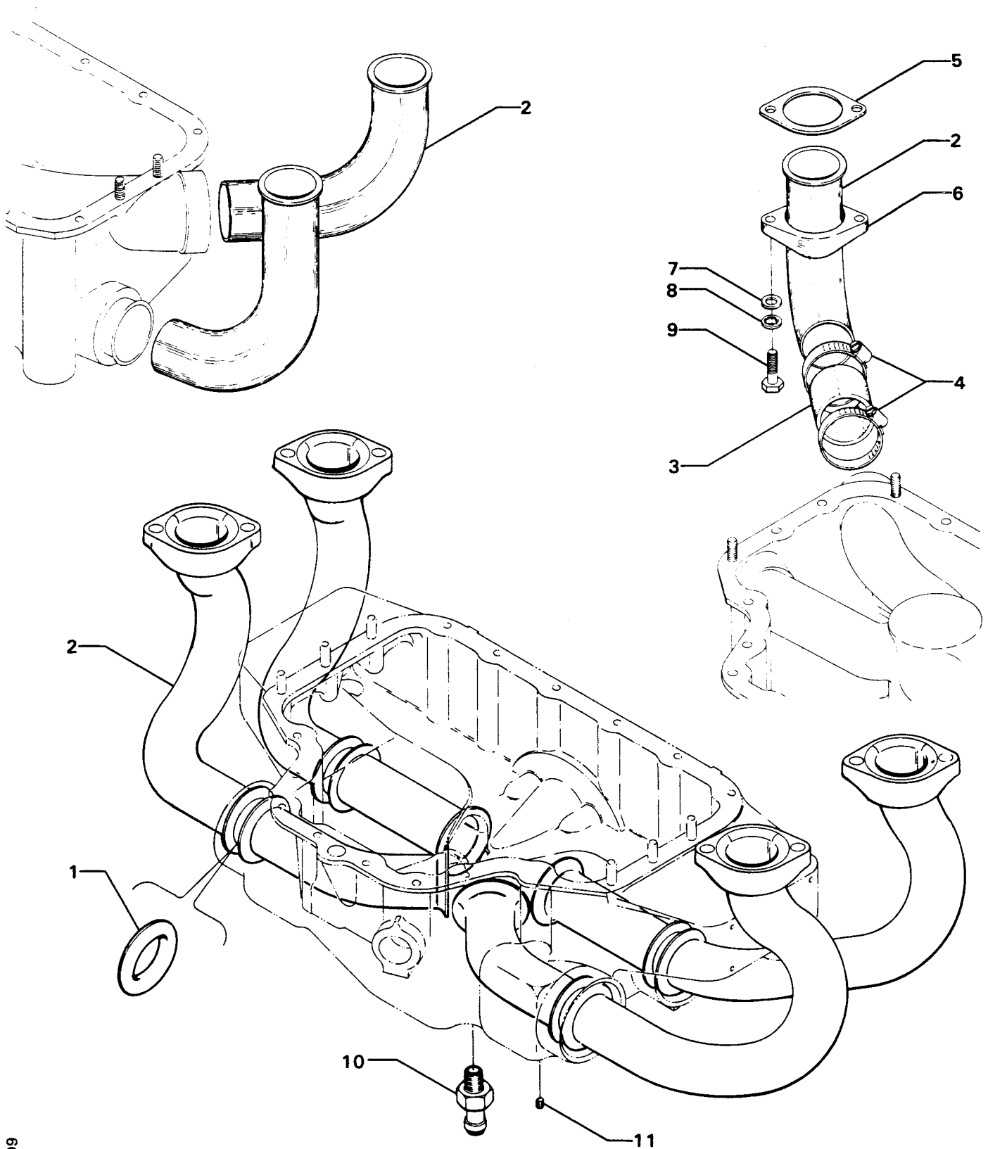
Figure 36. INTAKE PIPES
