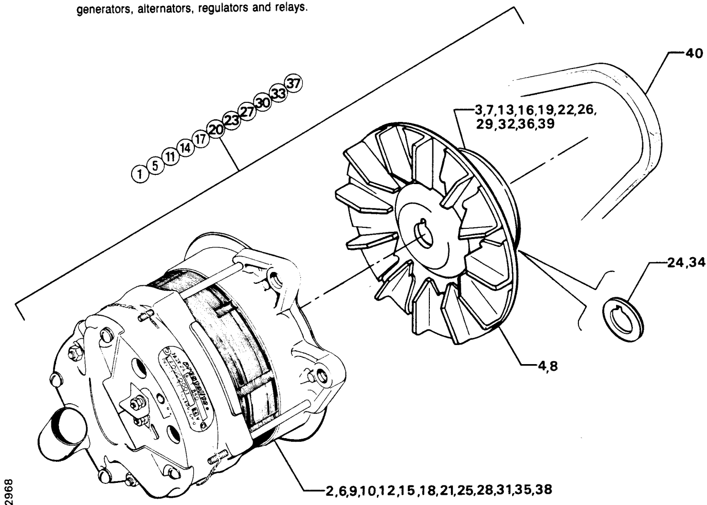
Figure 32. ALTERNATOR ASSEMBLY AND BELT
