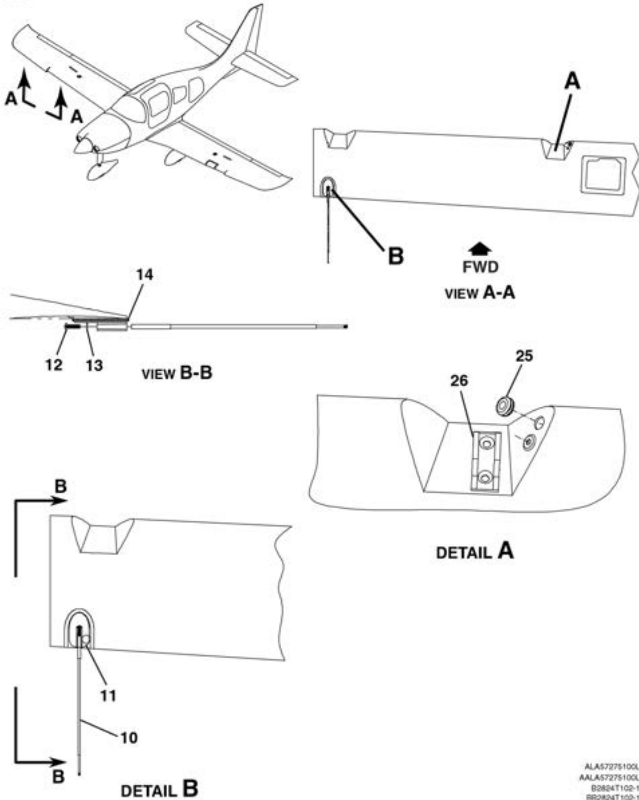
AILERON ASSEMBLY FIGURE 17 (SHEET 1)
