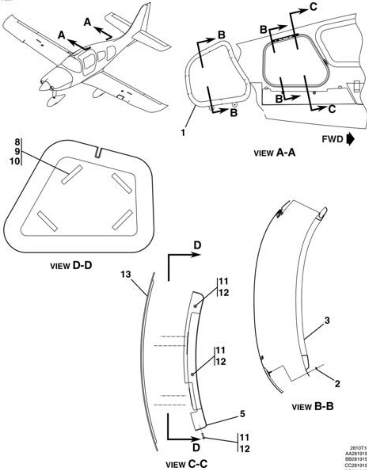
BAGGAGE DOOR PANEL FIGURE 18 (SHEET 1)
