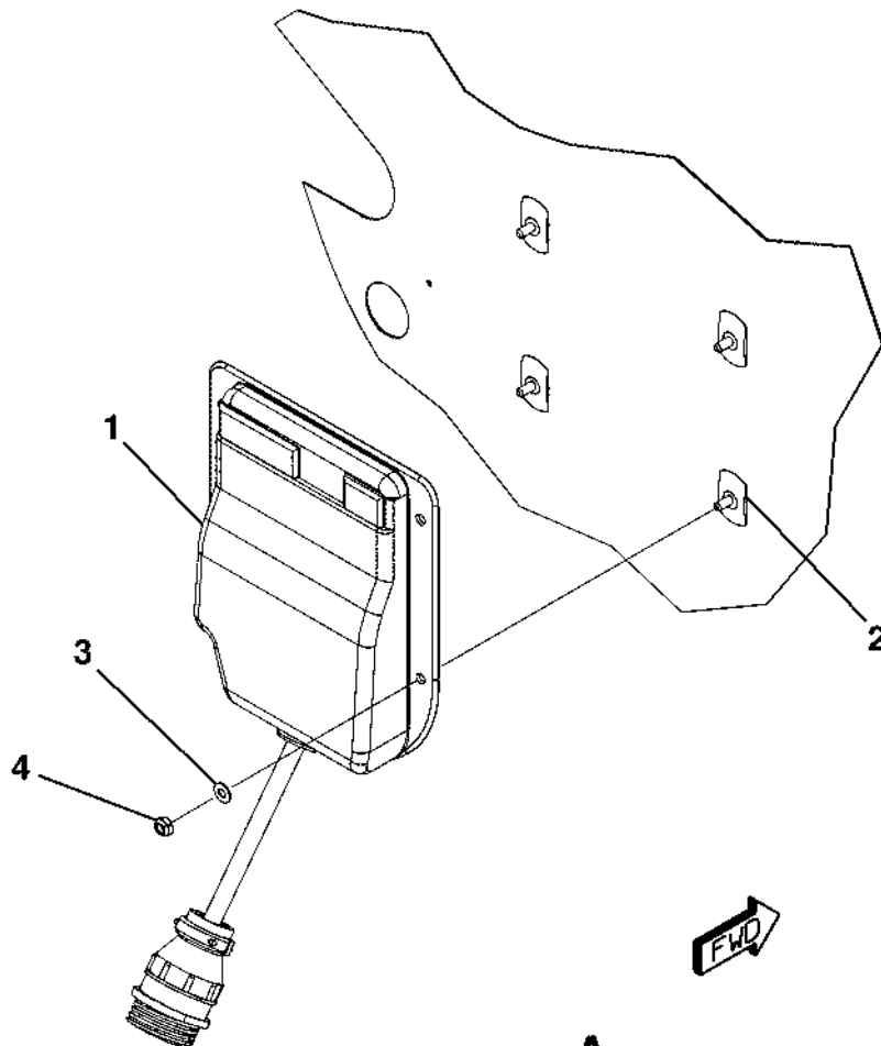
ELECTRONIC CONTROL UNIT MODULE FIGURE 05 (SHEET 1)
