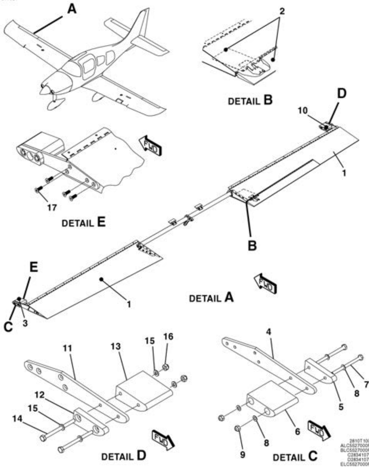
HORIZONTAL FLIGHT CONTROL ASSEMBLY FIGURE 03 (SHEET 1)
