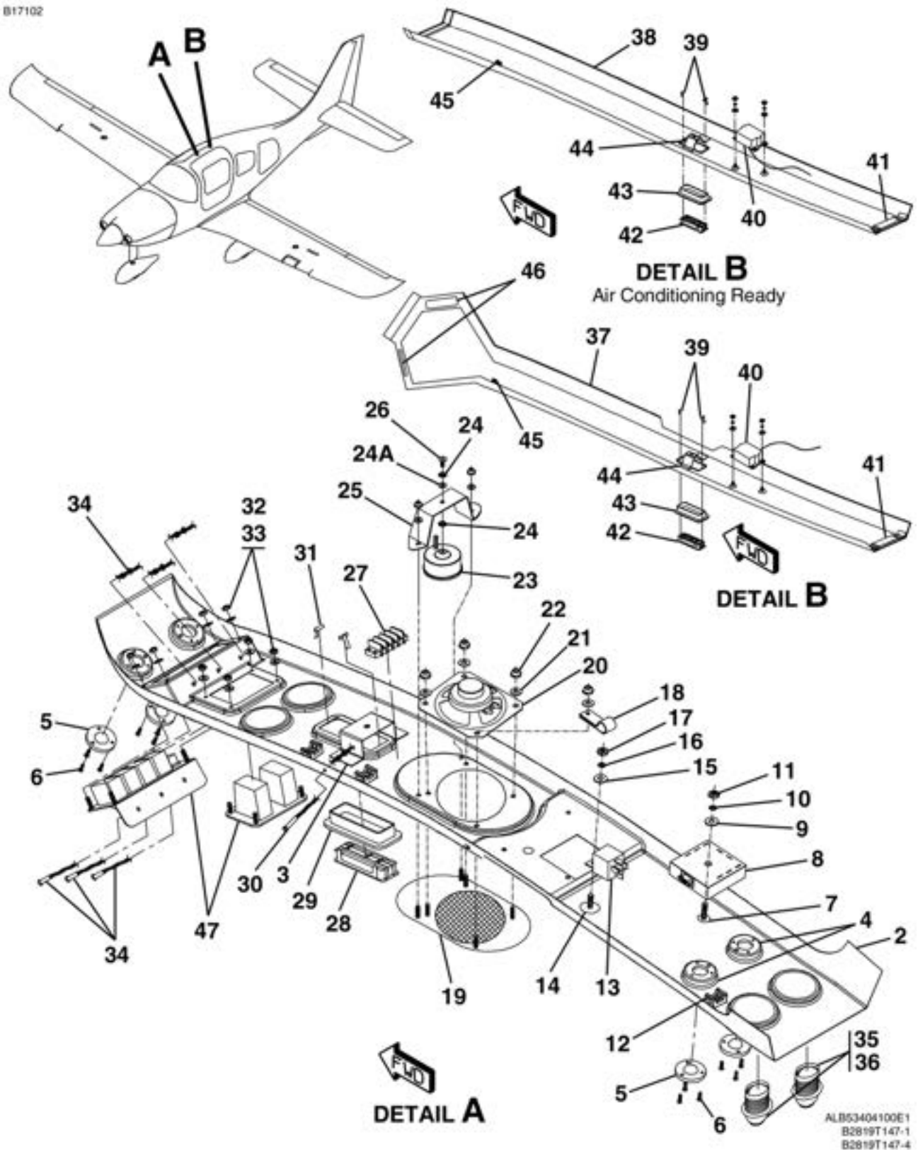
INTERIOR LIGHTING AND SPEAKER INSTALLATION FIGURE 01 (SHEET 1)
