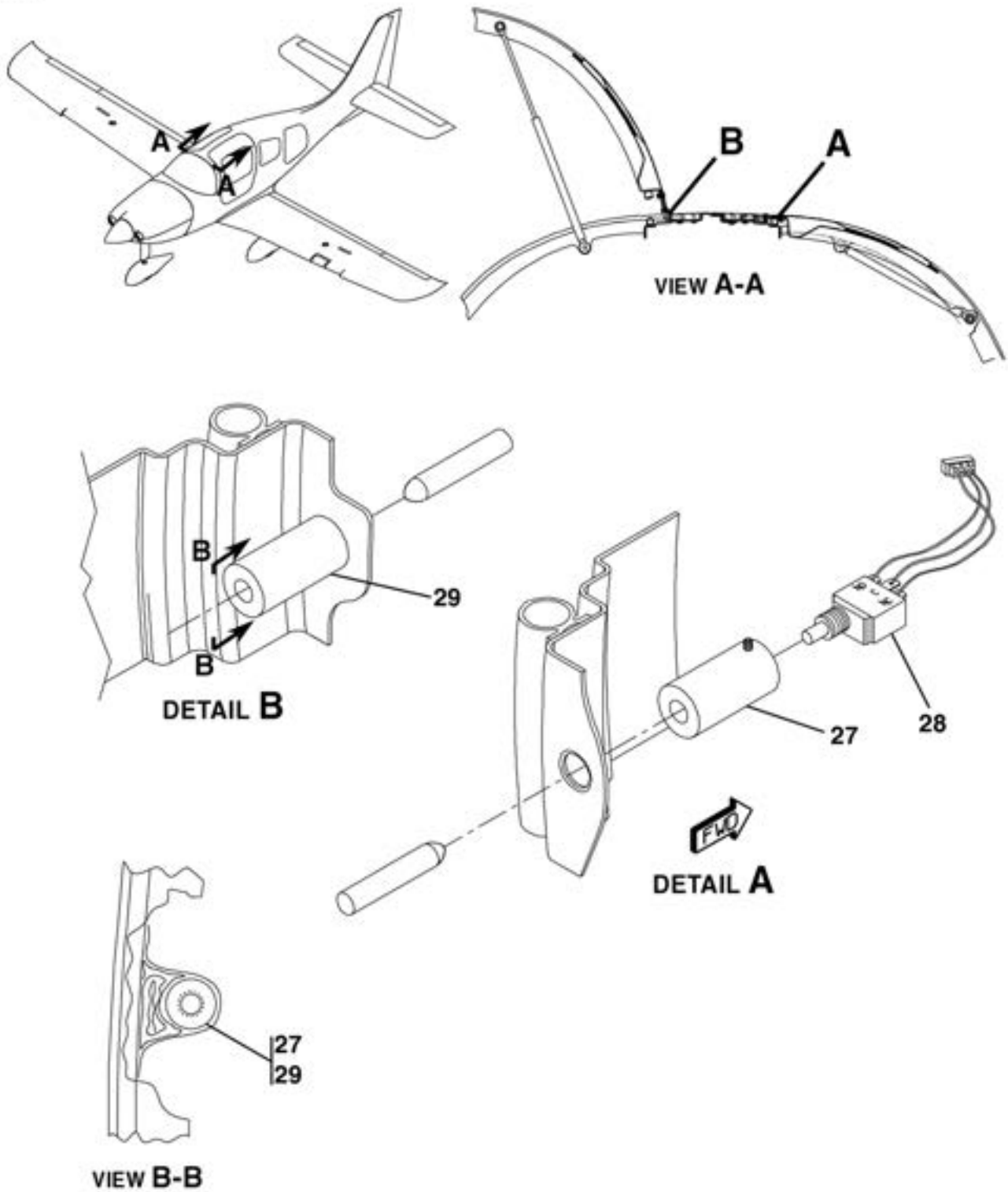
CABIN AND BAGGAGE DOOR INSTALLATION FIGURE 01 (SHEET 3)
