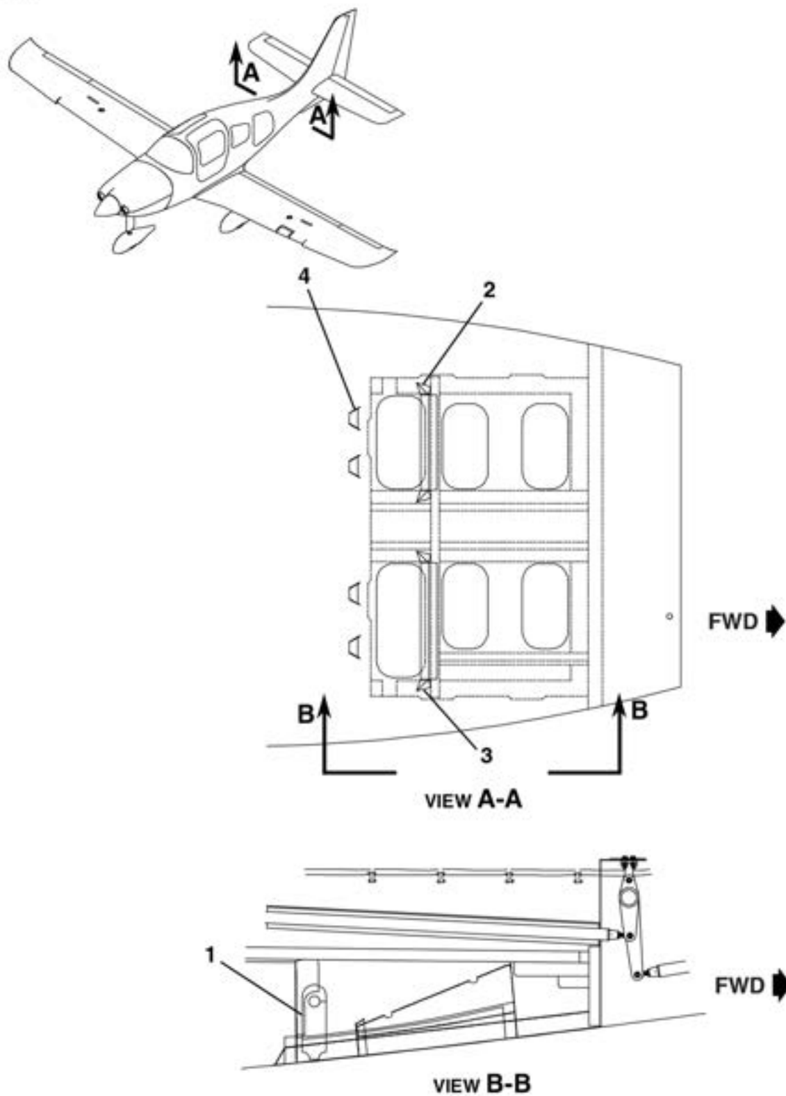
FUSELAGE MODIFICATION INSTALLATION - AIR CONDITIONING FIGURE 08 (SHEET 1)
