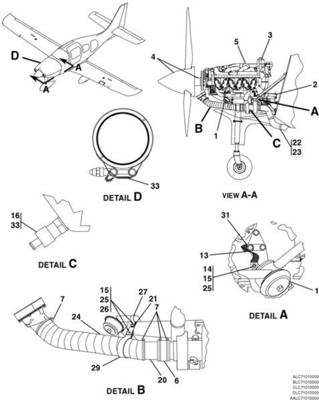
POWERPLANT ASSEMBLY FIGURE 01 (SHEET 1)
