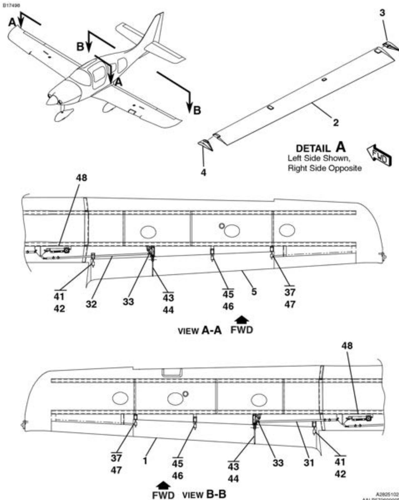
FLAP ASSEMBLY FIGURE 18 (SHEET 1)
