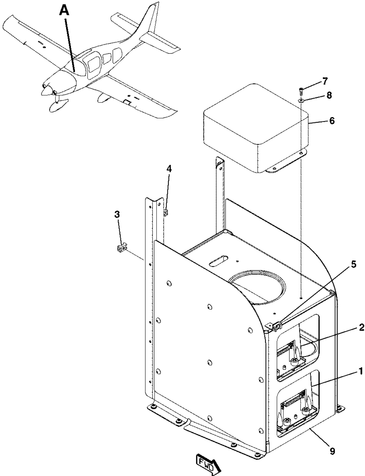
ATTITUDE HEADING REFERENCE SYSTEM (AHRS) INSTALLATION FIGURE 09 (SHEET 1)
