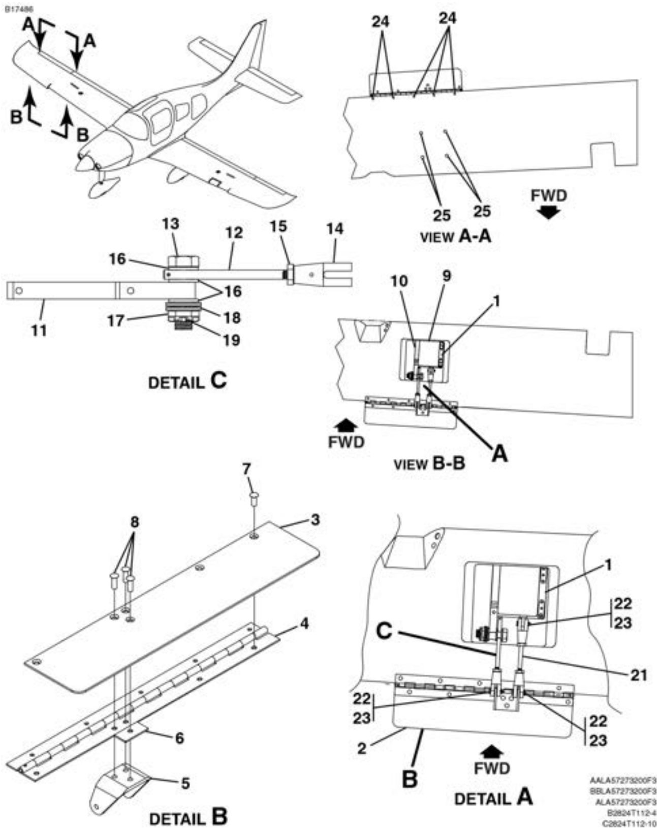
TRIM ASSEMBLY - AILERON FIGURE 12 (SHEET 1)
