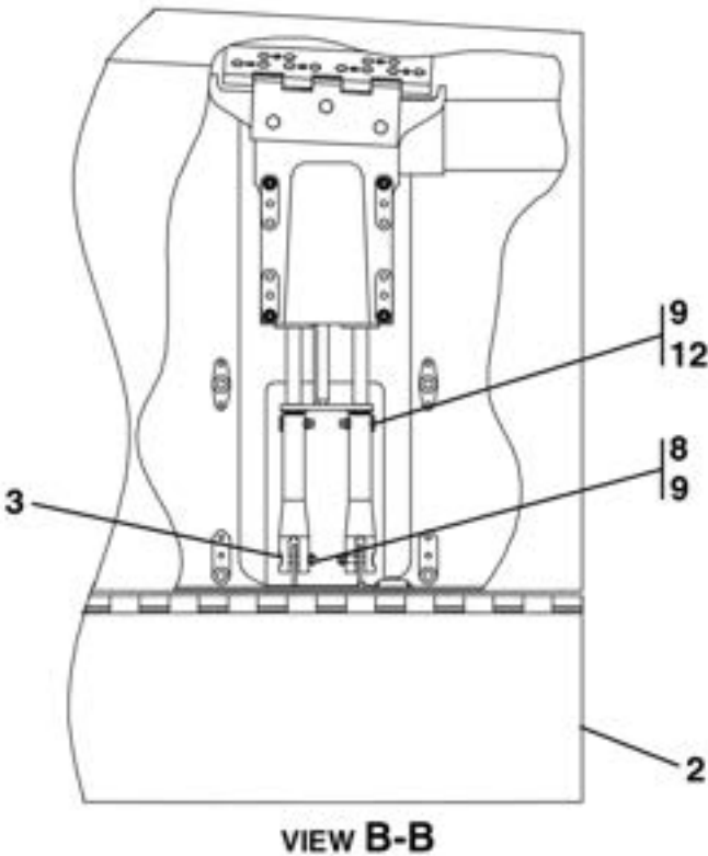
ELEVATOR TRIM TAB ASSEMBLY FIGURE 06 (SHEET 1)
