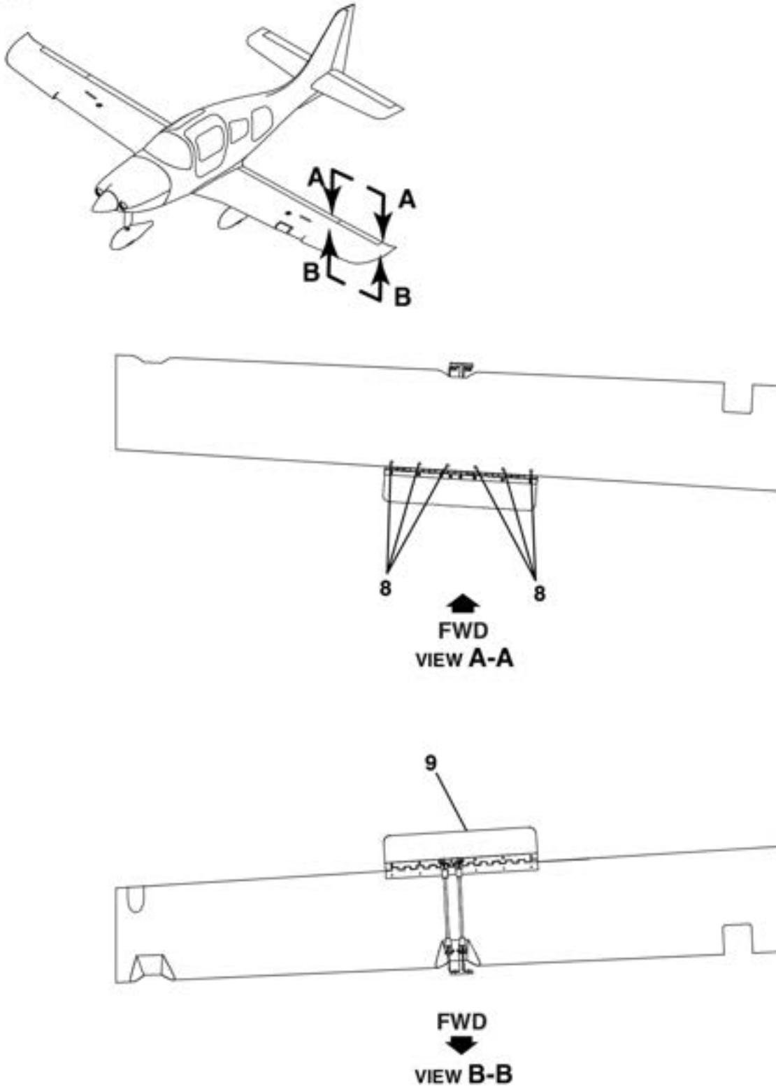
SERVO TAB ASSEMBLY - AILERON FIGURE 13 (SHEET 1)
