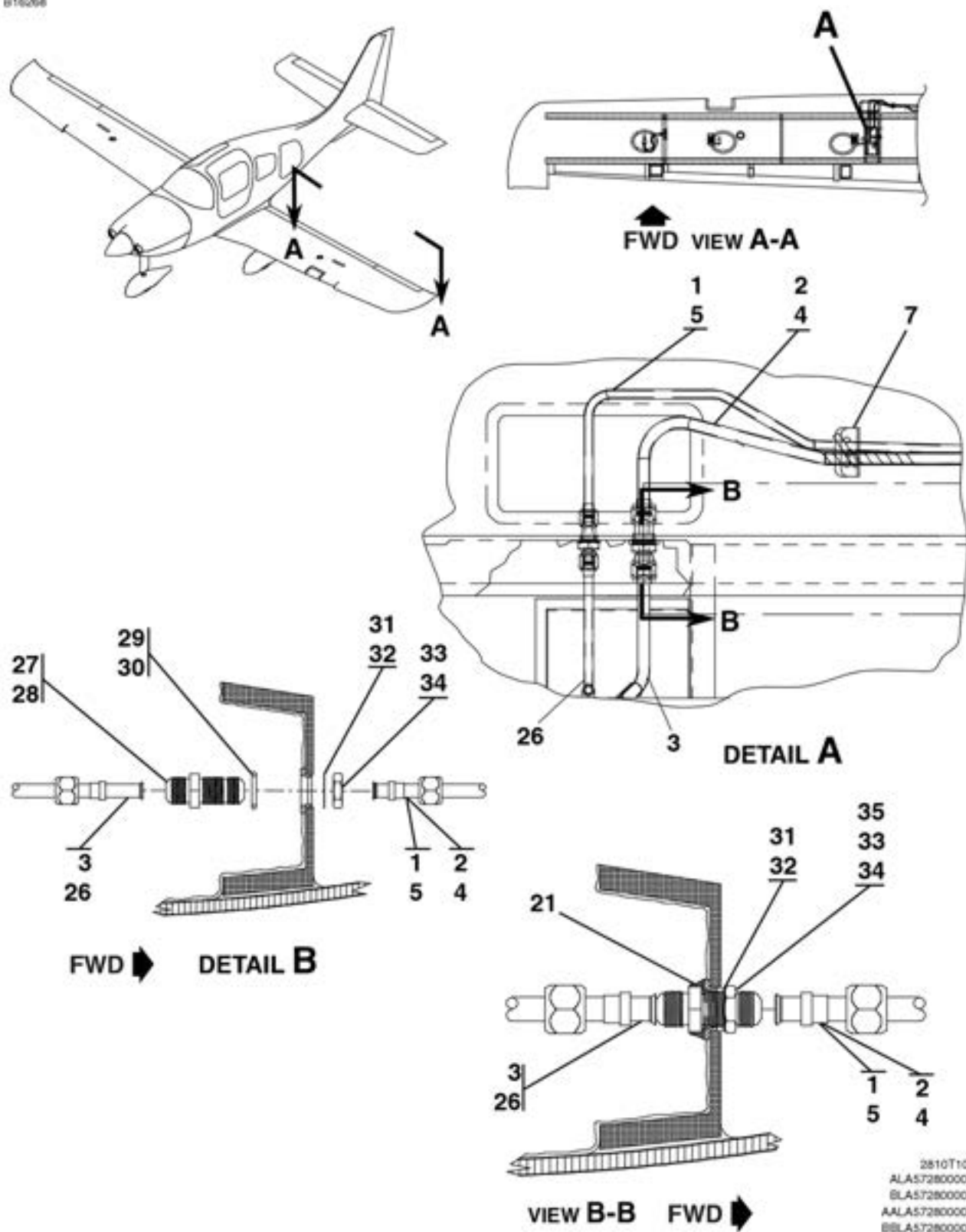
FUEL SYSTEM - WING ASSEMBLY FIGURE 04 (SHEET 5)
