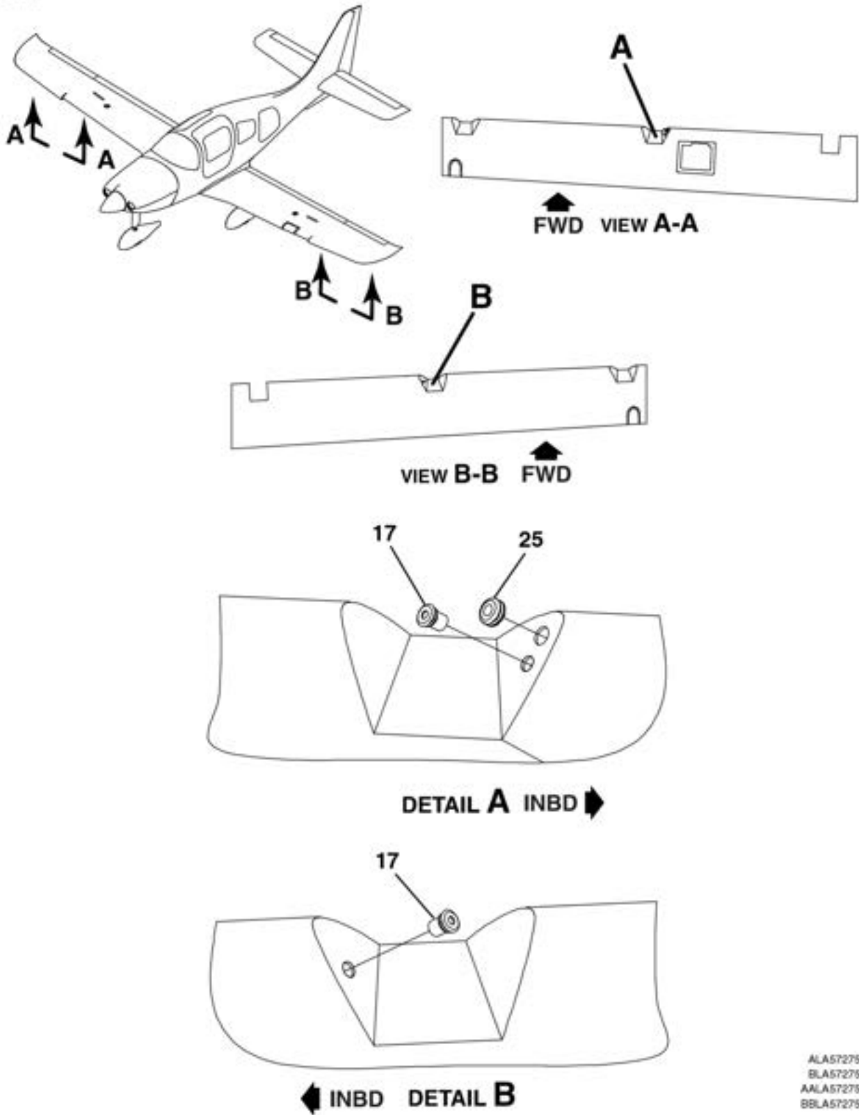
AILERON ASSEMBLY FIGURE 17 (SHEET 4)
