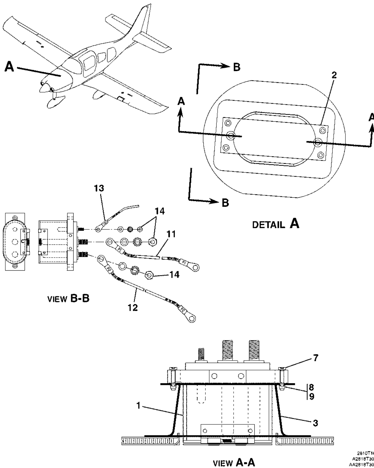
EXTERNAL POWER RECEPTACLE INSTALLATION FIGURE 07 (SHEET 1)
