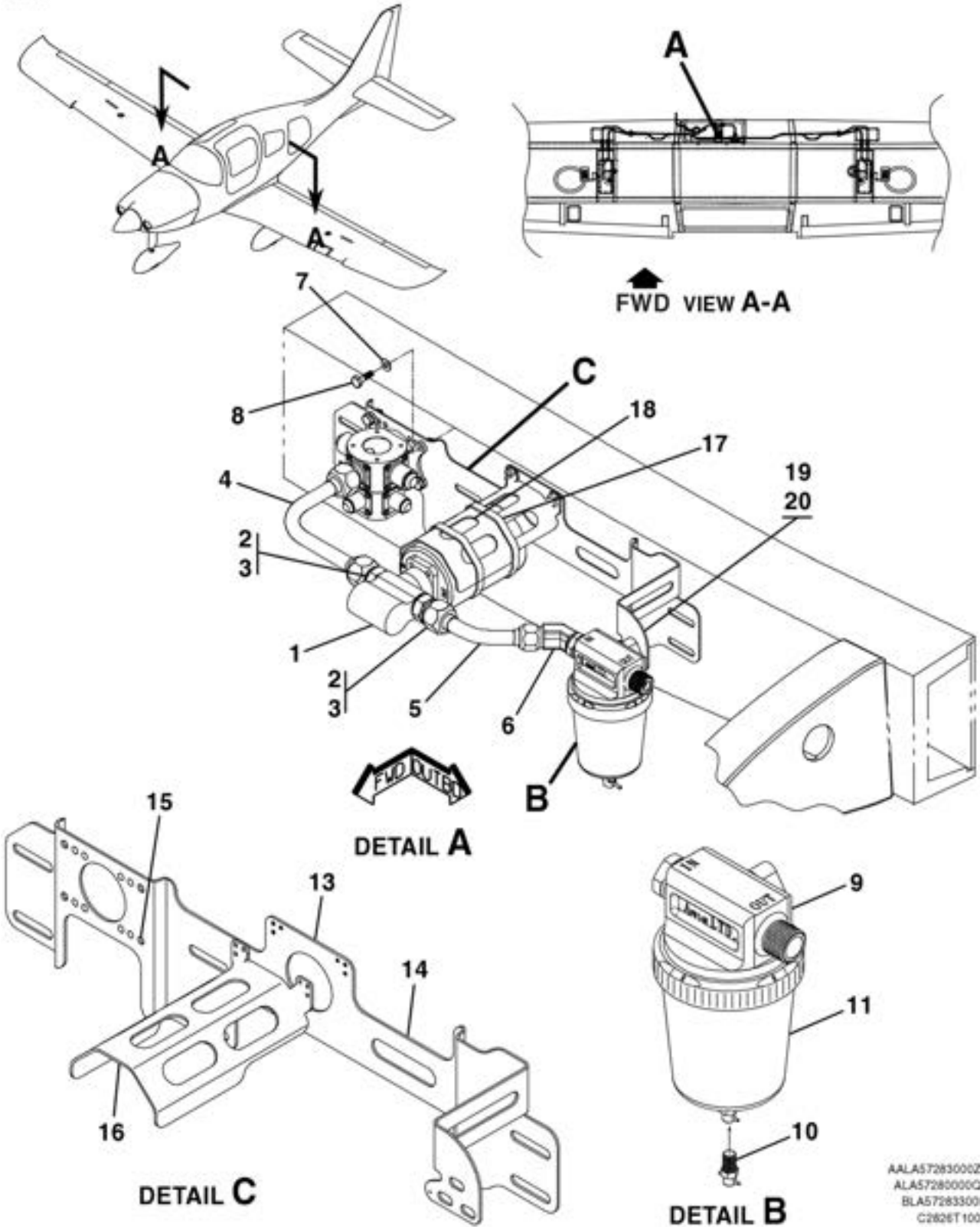
FUEL MODULE - SELECTOR, PUMP, STRAINER ASSEMBLY FIGURE 05 (SHEET 1)
