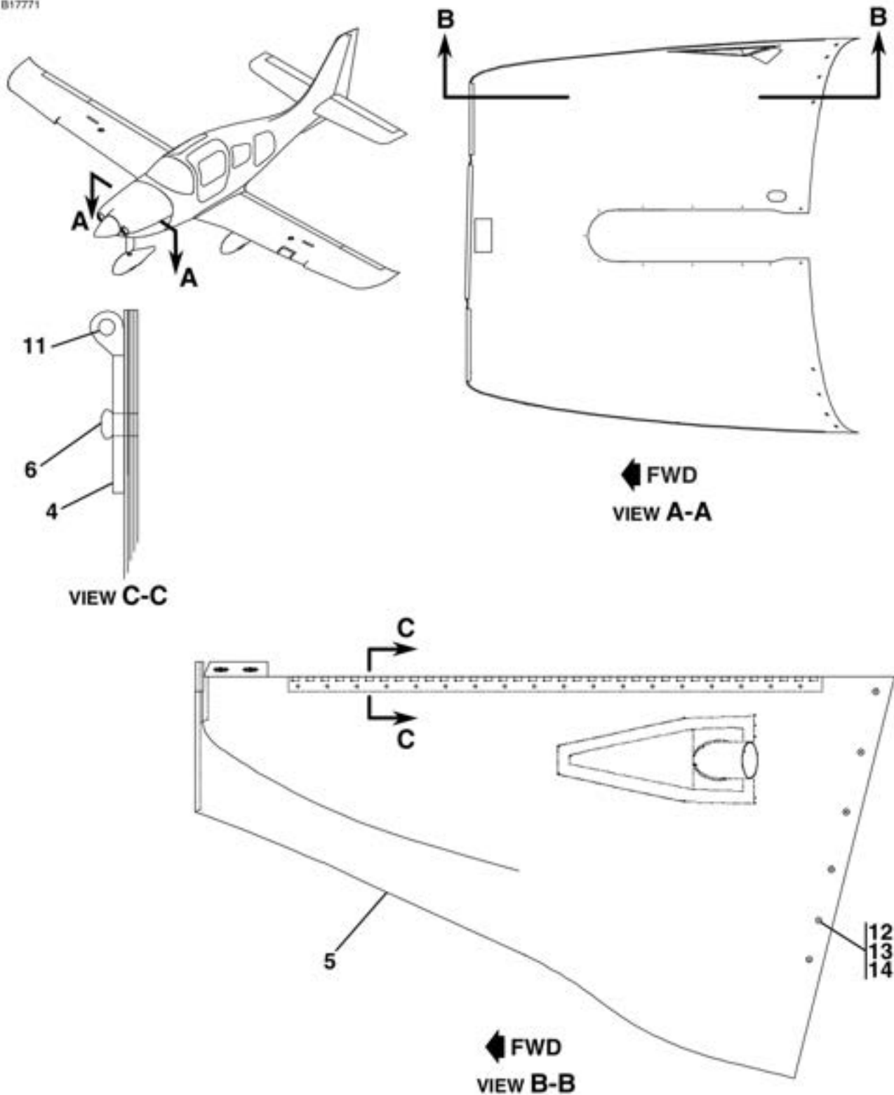
LOWER COWL ASSEMBLY FIGURE 06 (SHEET 2)
