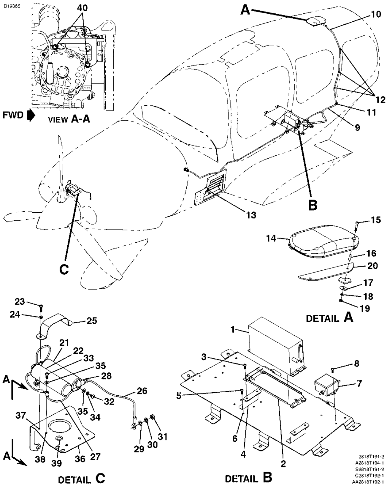
LIGHTNING DETECTION SYSTEM INSTALLATION FIGURE 17 (SHEET 1)
