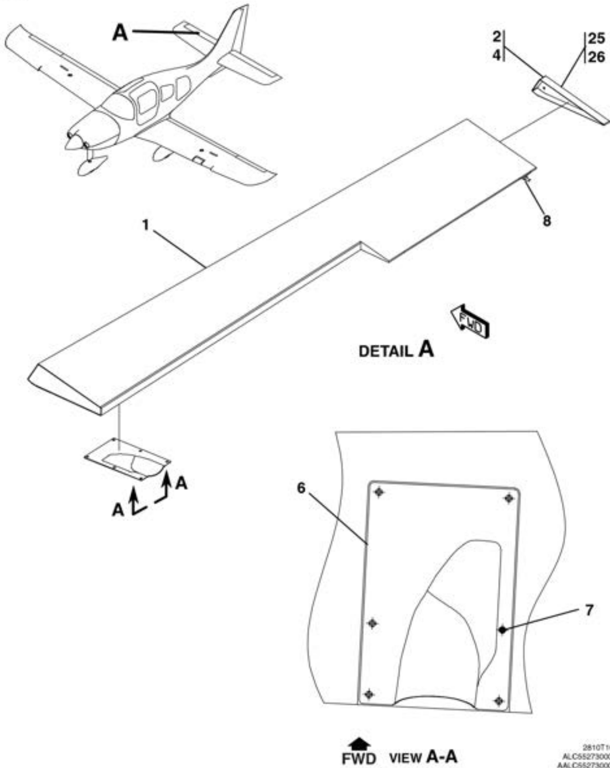
ELEVATOR ASSEMBLY FIGURE 04 (SHEET 1)
