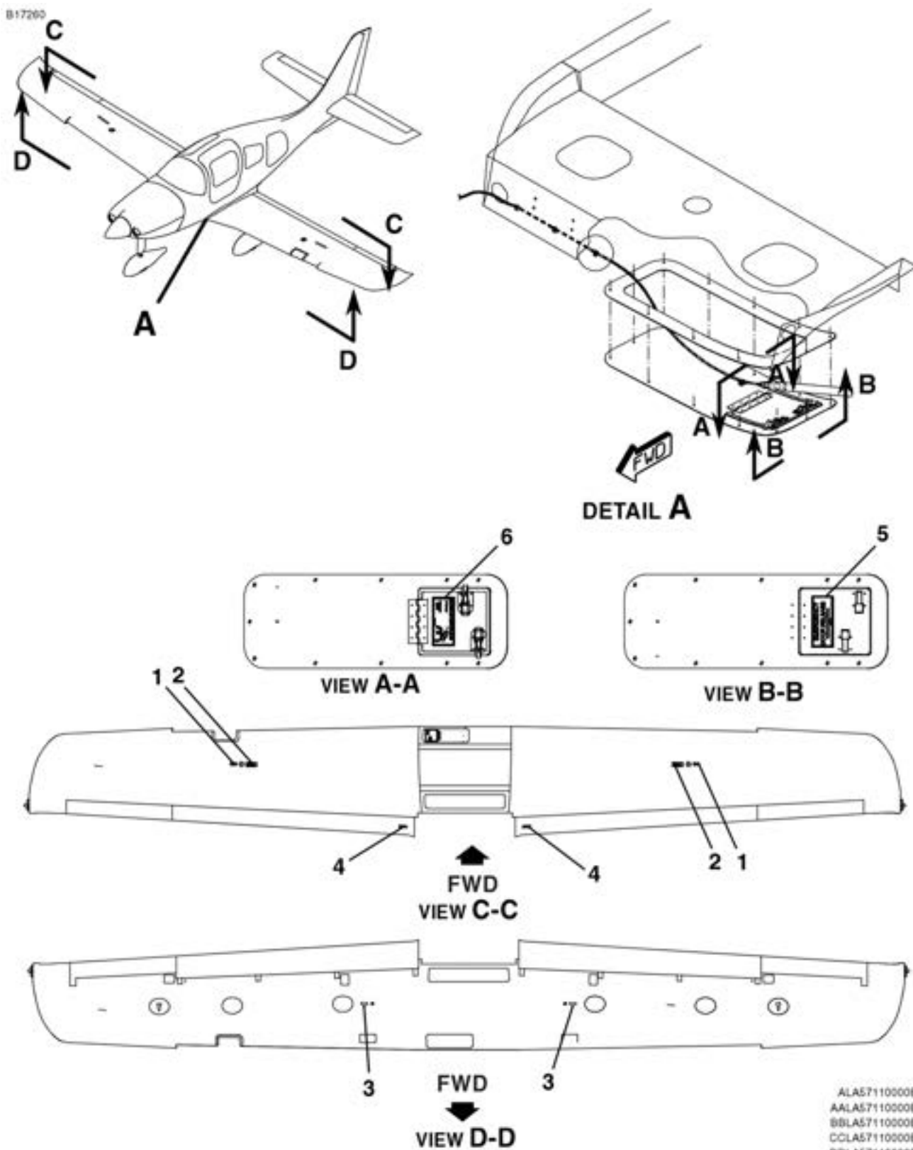
EXTERIOR PLACARDS AND MARKINGS - WING FIGURE 03 (SHEET 1)
