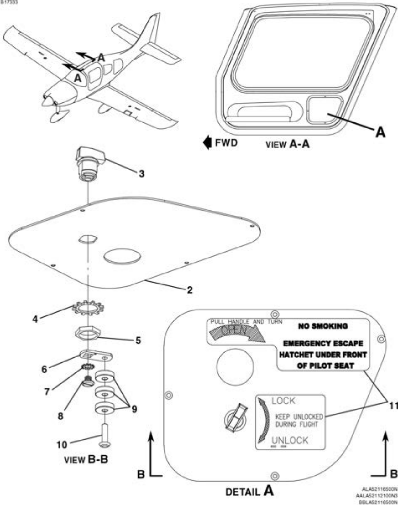
RIGHT CABIN DOOR ACCESS PANEL ASSY FIGURE 06 (SHEET 1)
