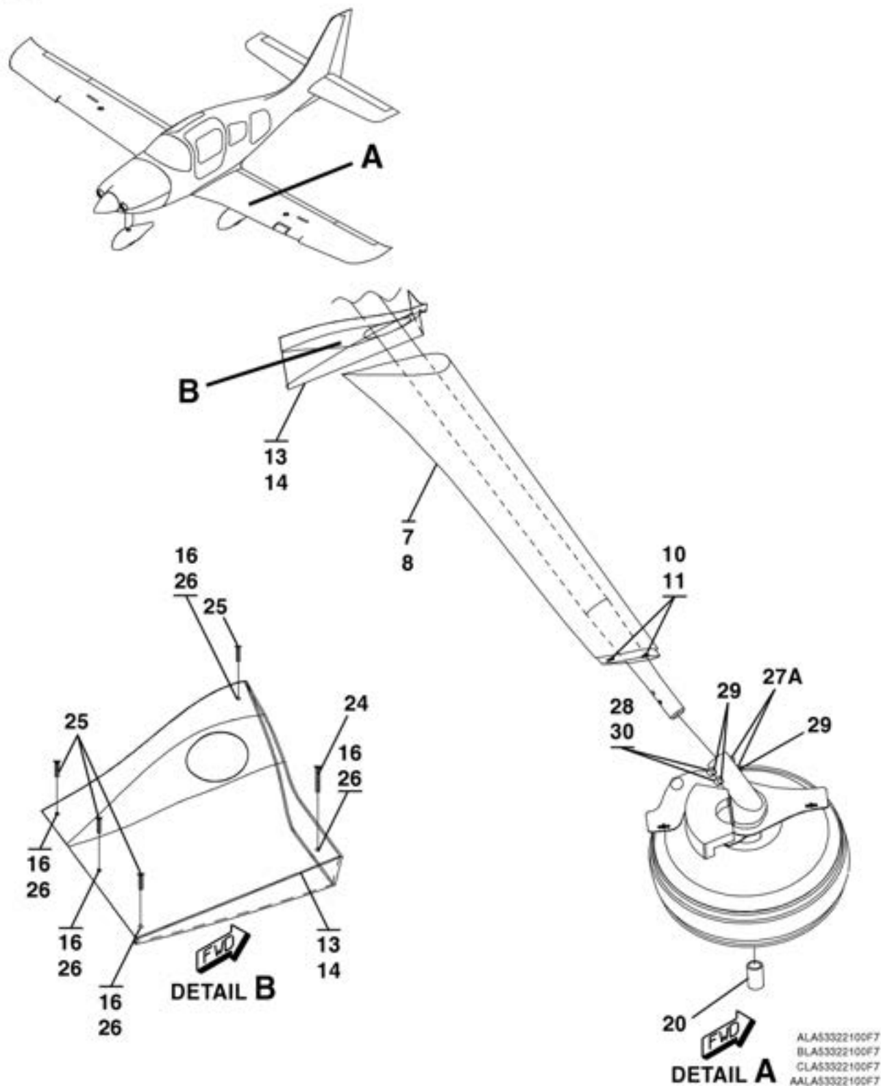
WHEEL PANT ASSEMBLY FIGURE 03 (SHEET 1)
