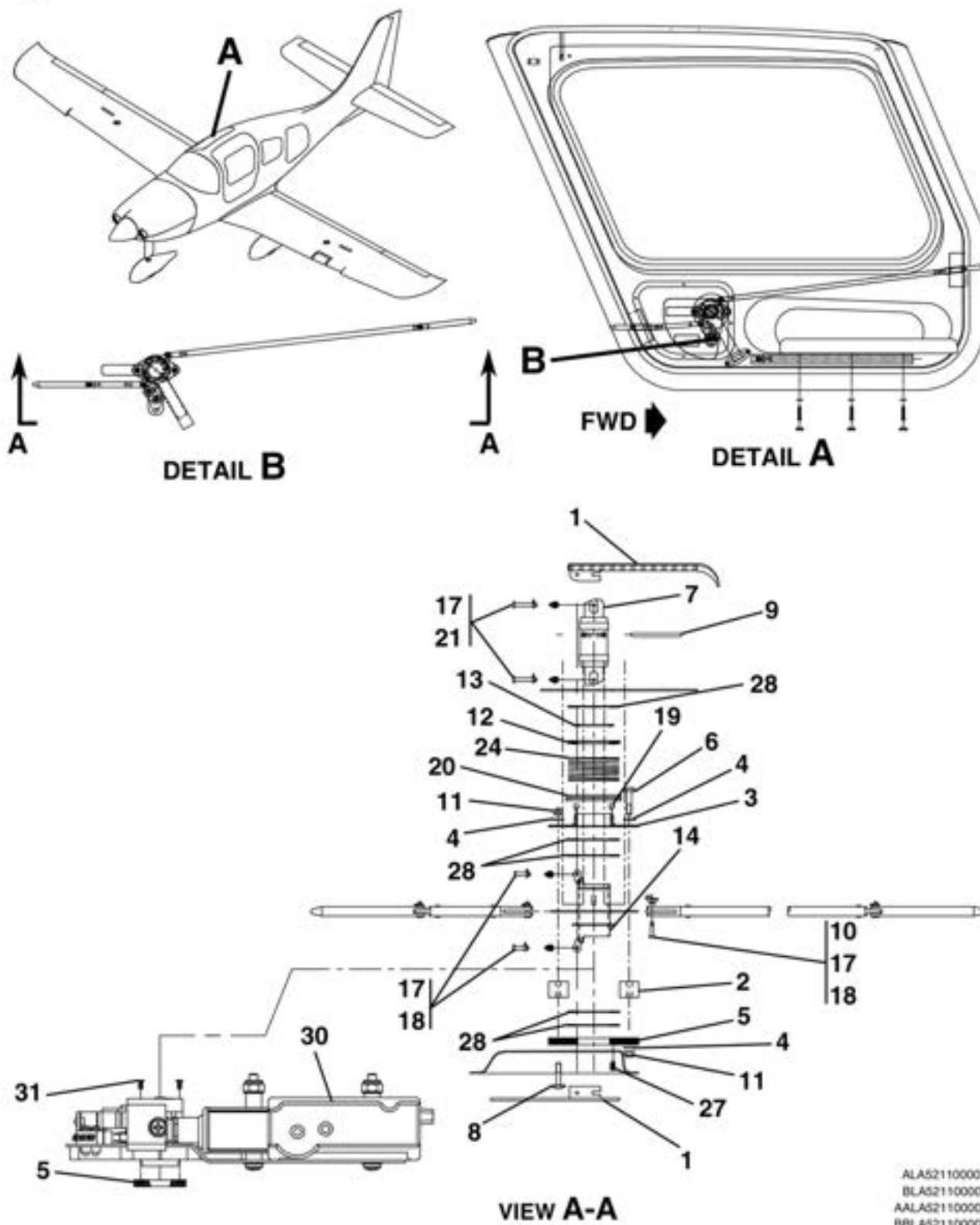
LEFT CABIN DOOR LATCH ASSEMBLY FIGURE 04 (SHEET 2)
