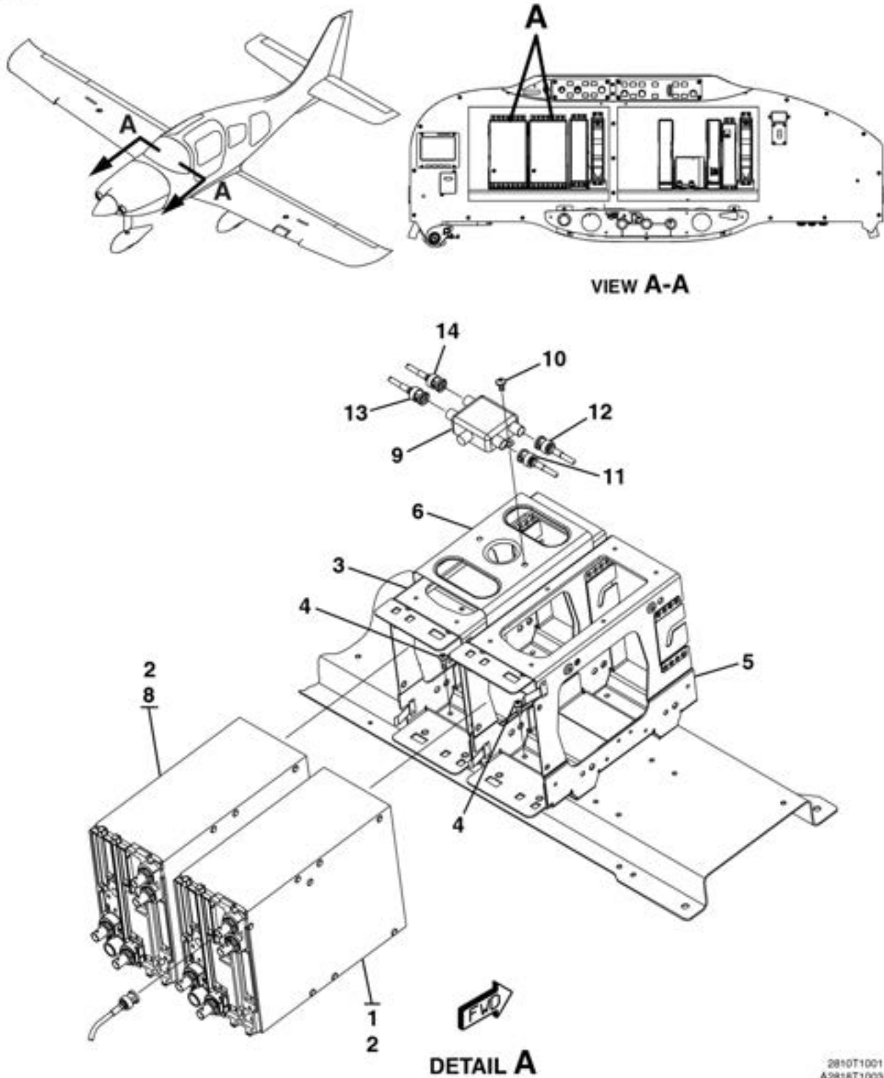
AVIONICS AND NAVIGATION EQUIPMENT - GIA 63W INTEGRATED AVIONICS UNITS INSTALLATION FIGURE 04 (SHEET 1)
