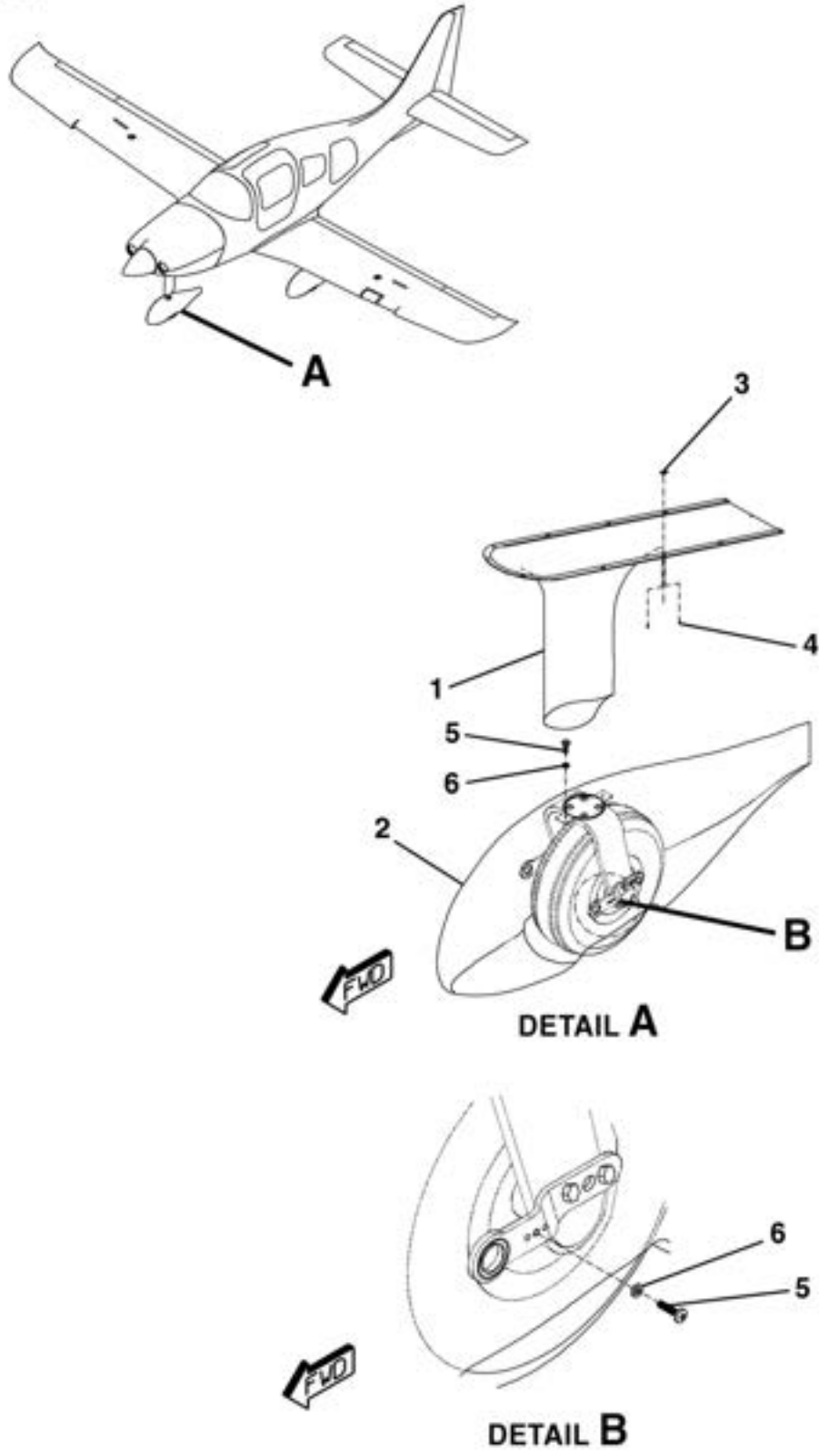
FAIRING AND PANT ASSEMBLY - NOSE GEAR FIGURE 08 (SHEET 1)
