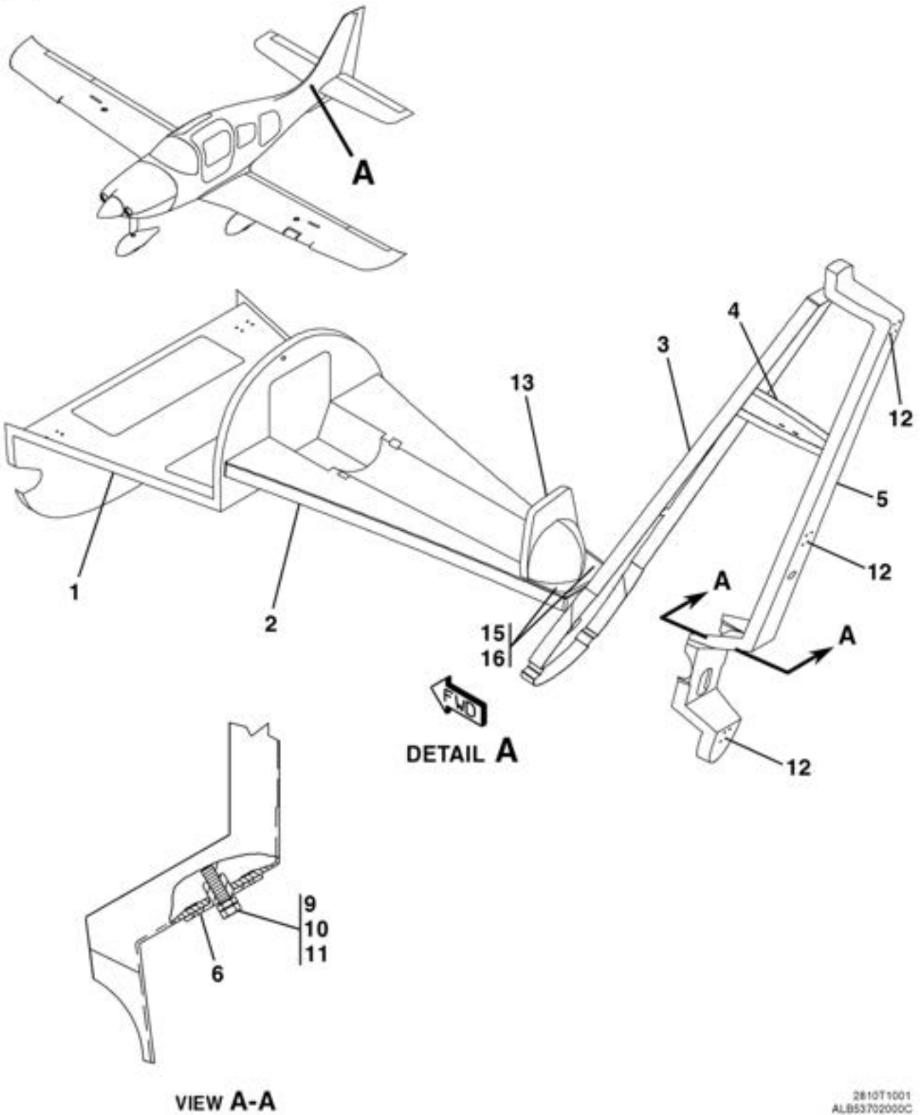
AFT FUSELAGE STRUCTURE ASSEMBLY FIGURE 03 (SHEET 1)
