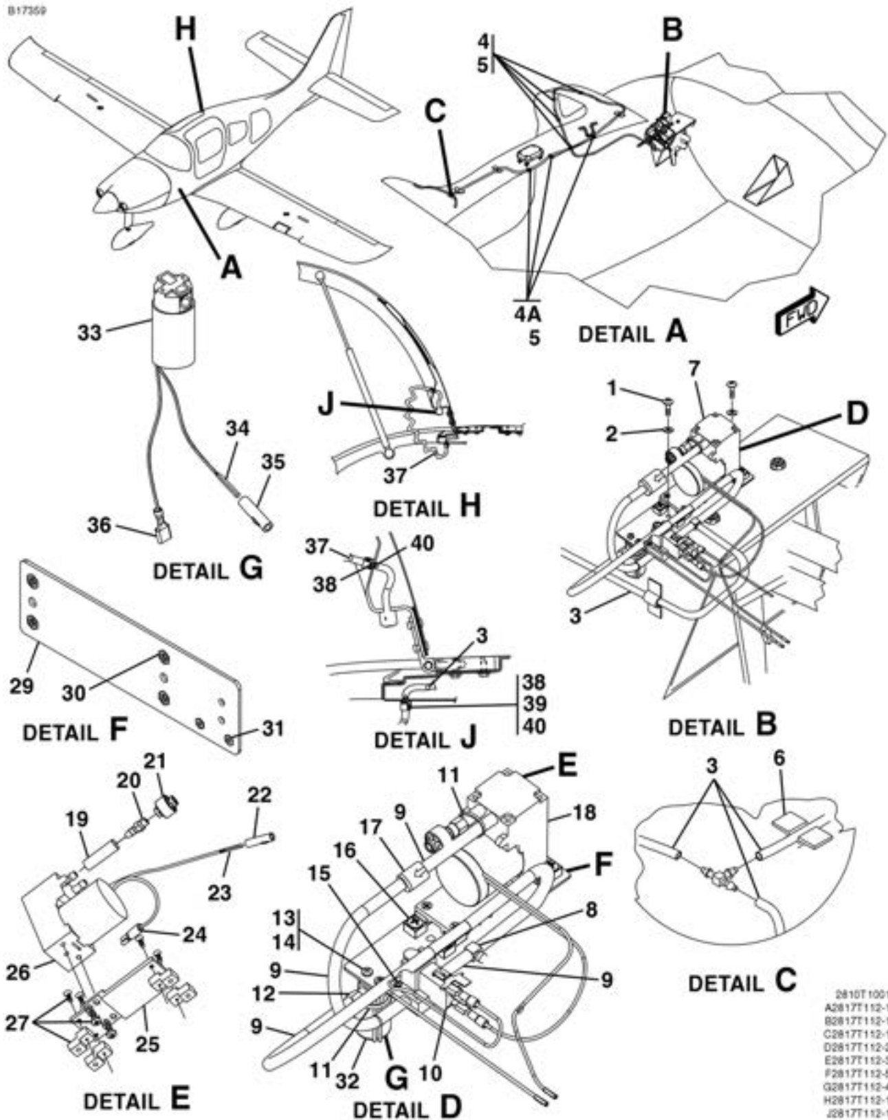
DOOR SEAL SYSTEM FIGURE 09 (SHEET 1)
