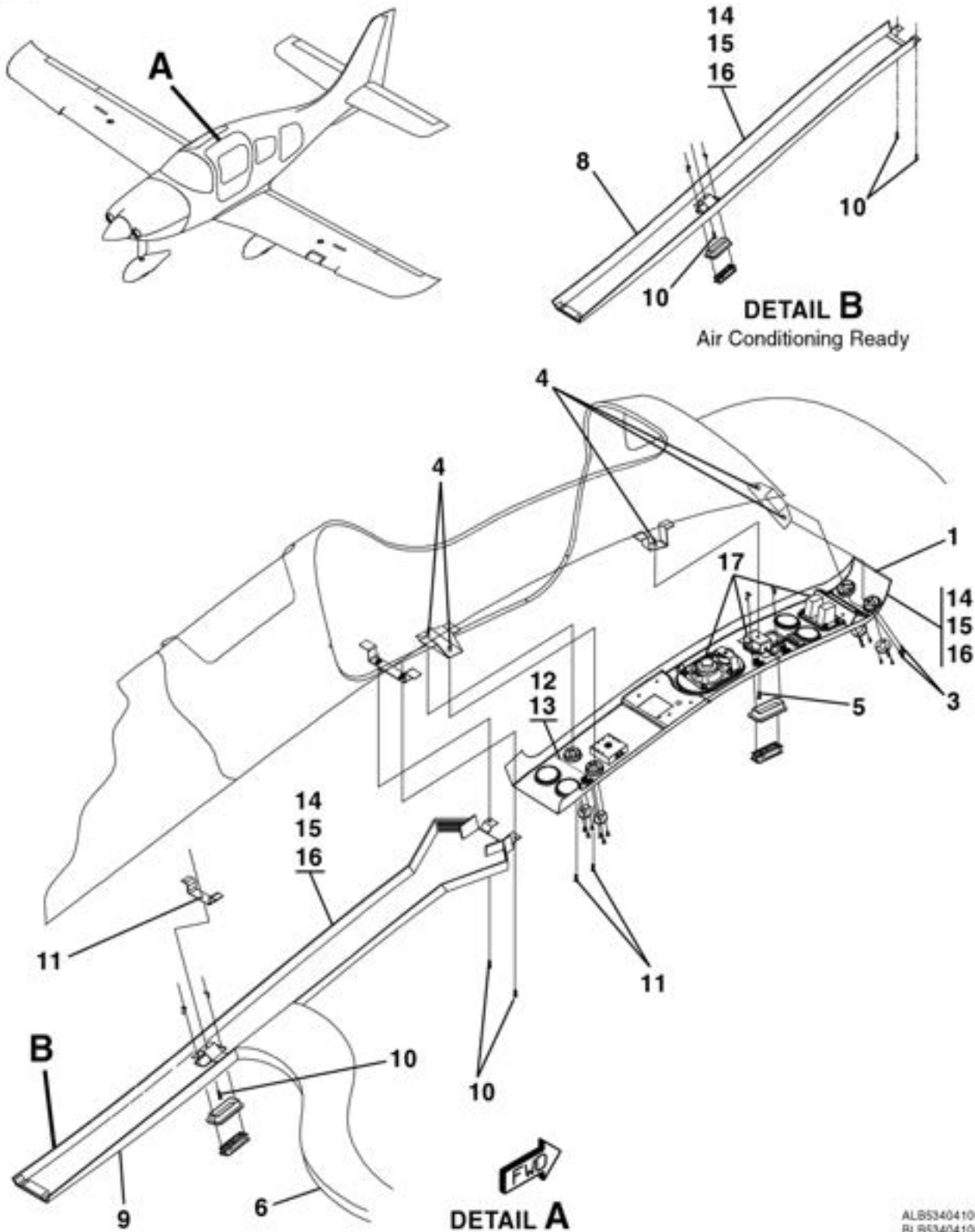
OVERHEAD CONSOLE PANEL INSTALLATION FIGURE 10 (SHEET 1)
