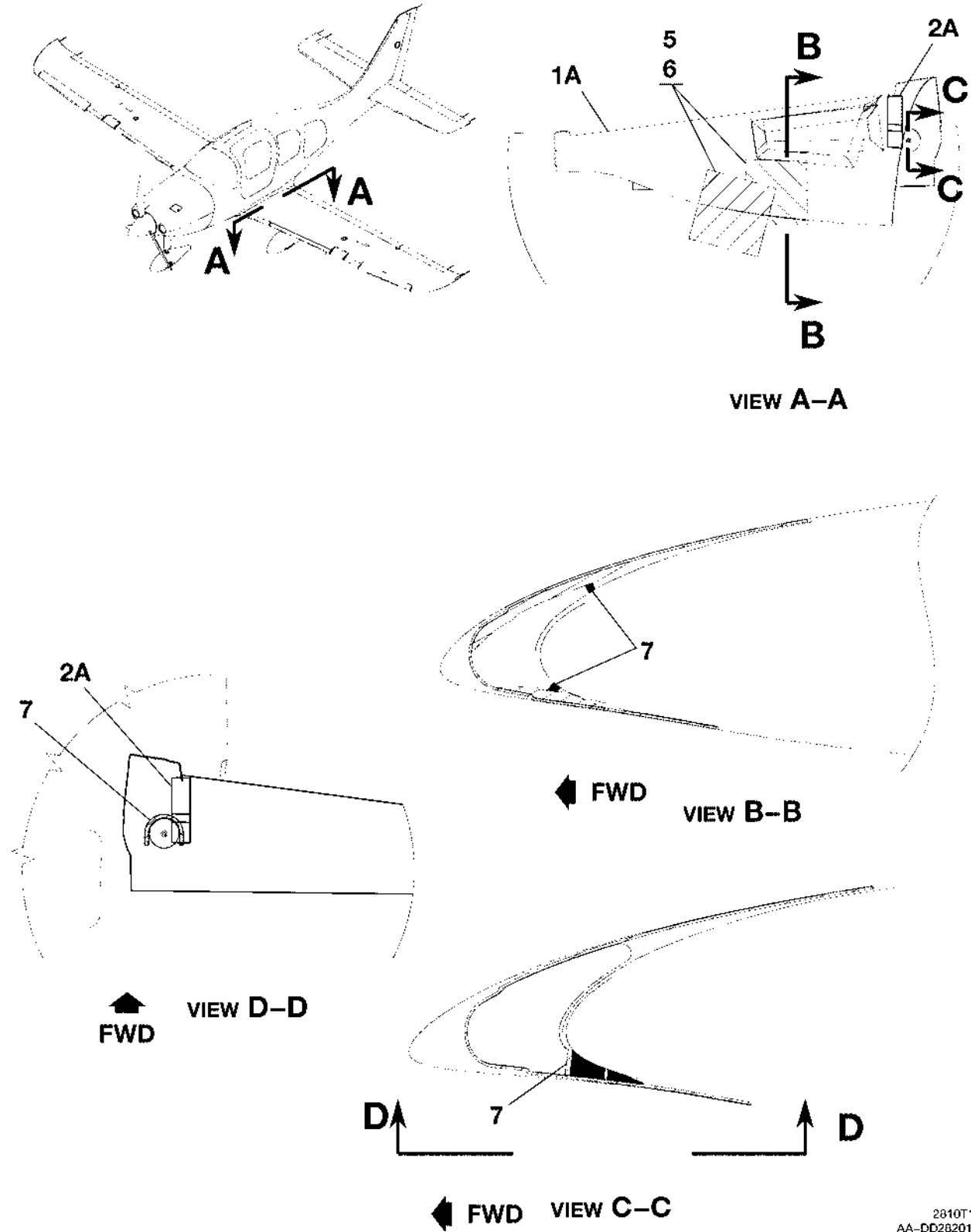
STRAKE INSTALLATION FIGURE 07 (SHEET 2)
