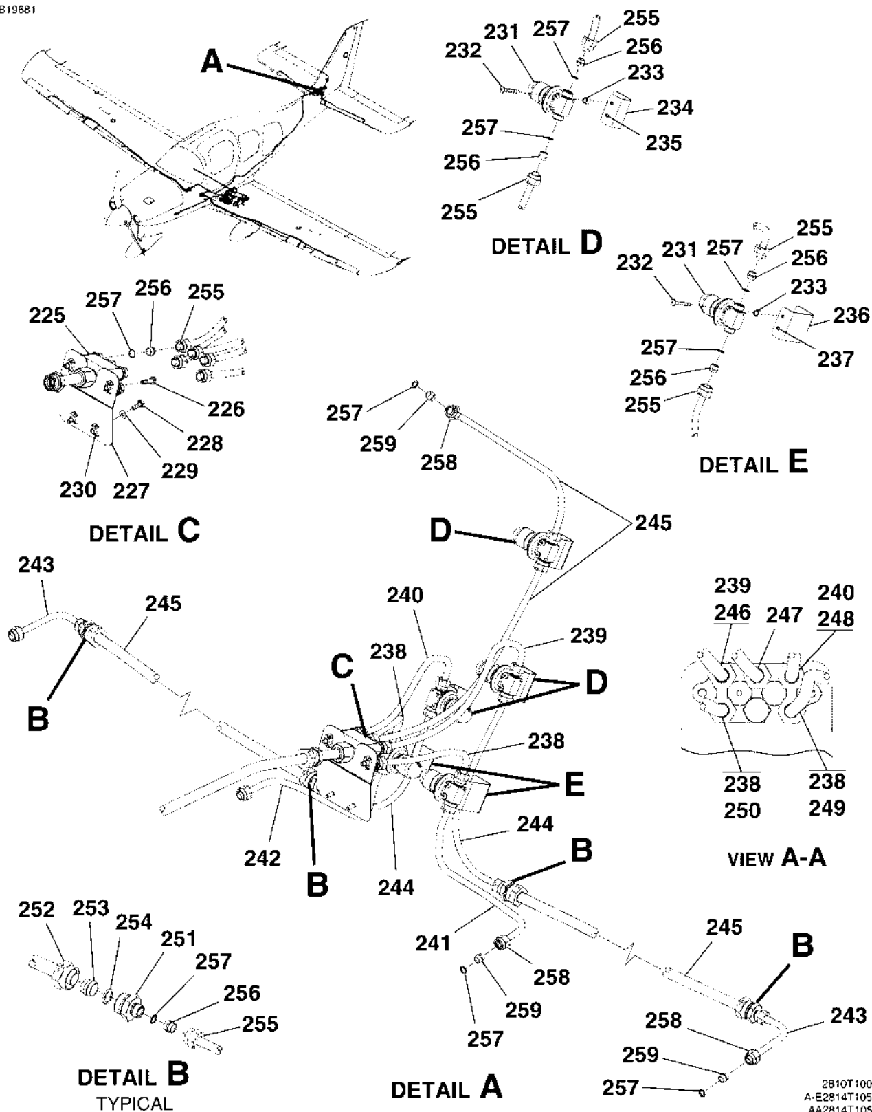
TKS SYSTEM - PLUMBING INSTALLATION FIGURE 05A (SHEET 4)
