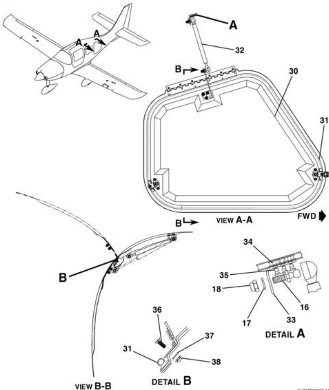
CABIN AND BAGGAGE DOOR INSTALLATION FIGURE 01 (SHEET 5)
