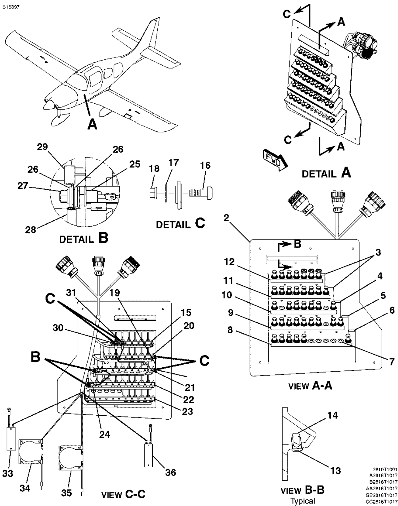
CIRCUIT BREAKER PANEL ASSEMBLY FIGURE 04 (SHEET 1)
