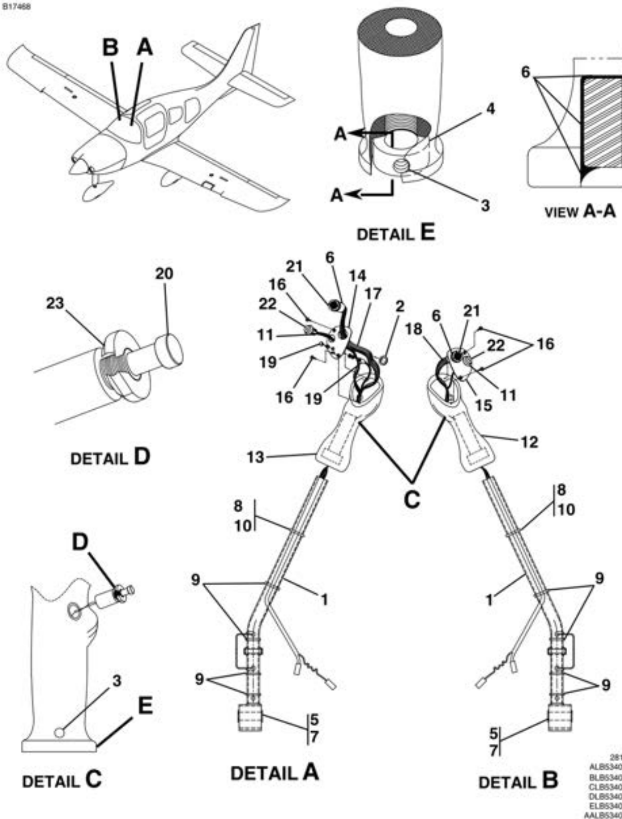
CONTROL STICK ASSEMBLY FIGURE 02 (SHEET 1)
