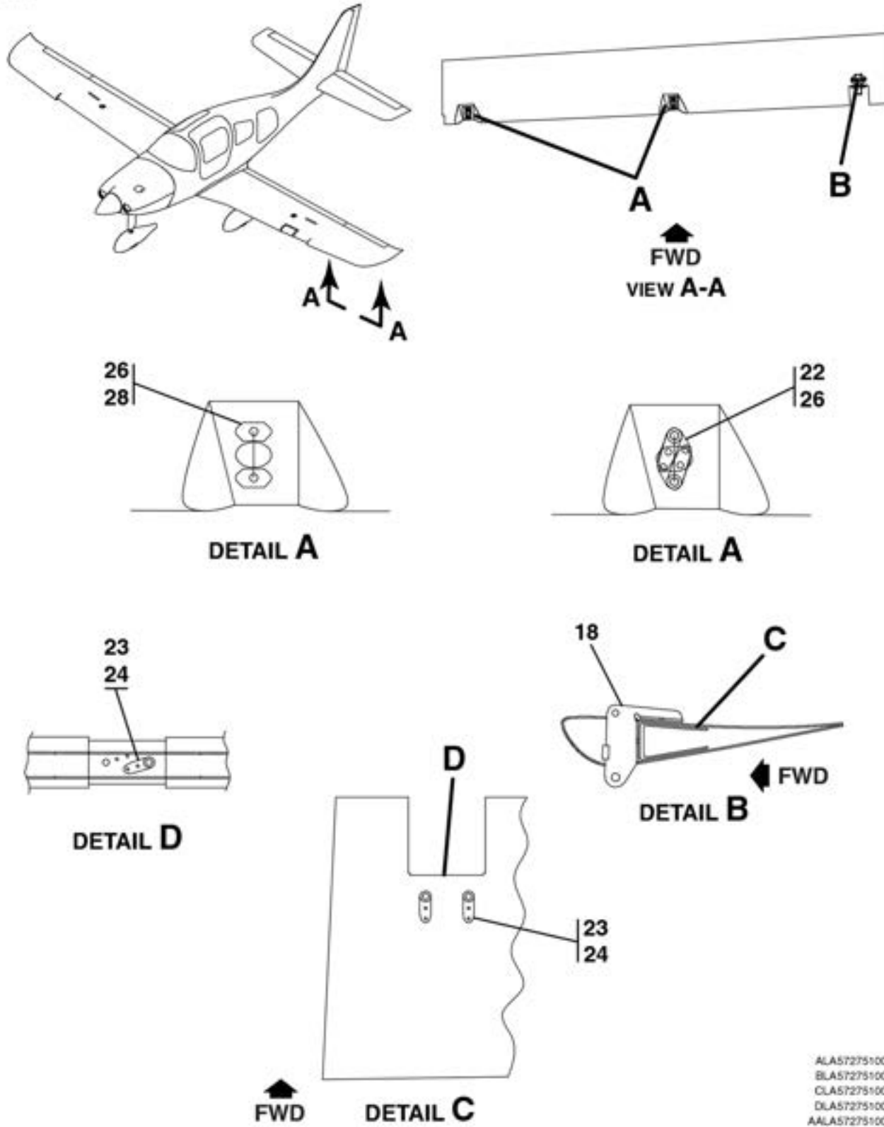
AILERON ASSEMBLY FIGURE 17 (SHEET 5)
