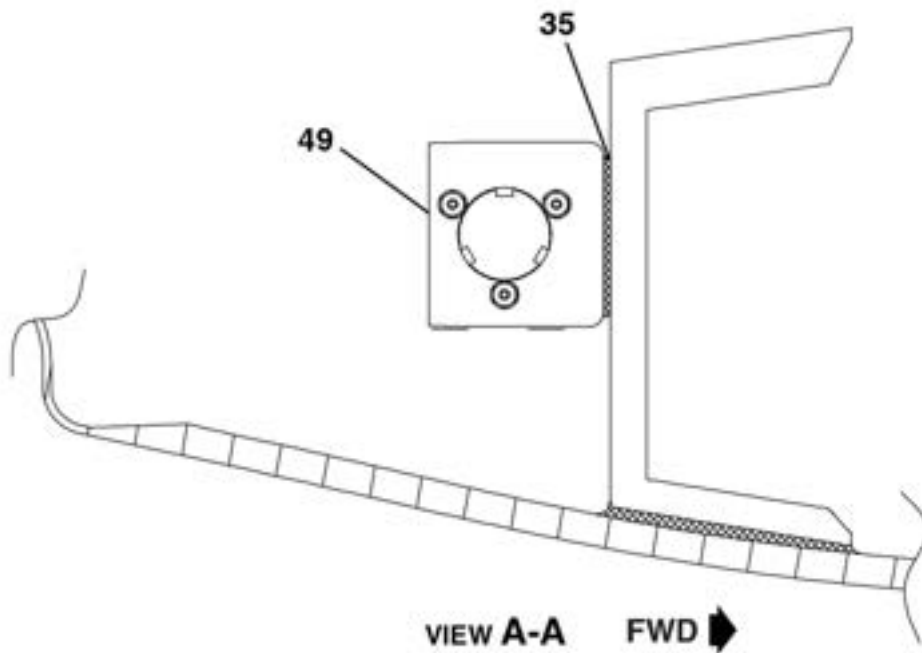
AILERON INSTALLATION FIGURE 10 (SHEET 7)
