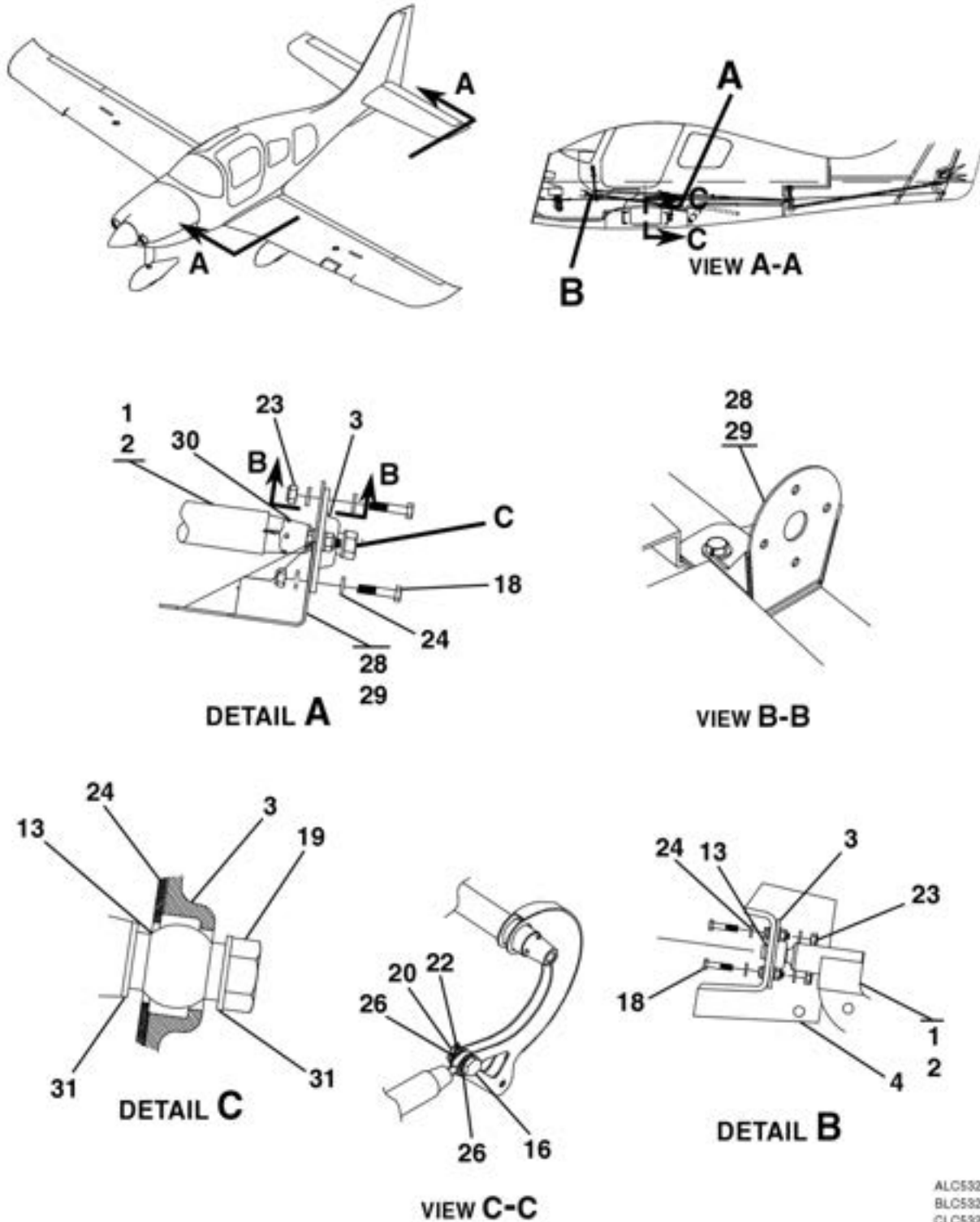
FUSELAGE CONTROL SYSTEM ASSEMBLY FIGURE 01 (SHEET 3)
