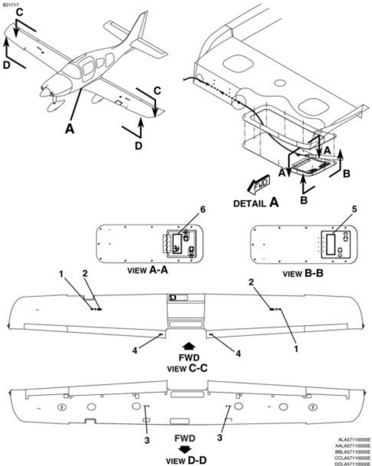
EXTERIOR PLACARDS AND MARKINGS - WING - ARGENTINA FIGURE 03C (SHEET 1)
