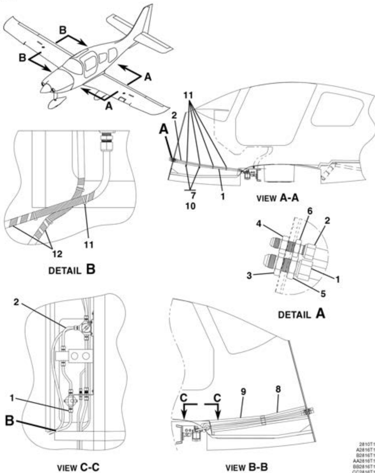
FUEL LINES ASSEMBLY - FUSELAGE FIGURE 03 (SHEET 1)
