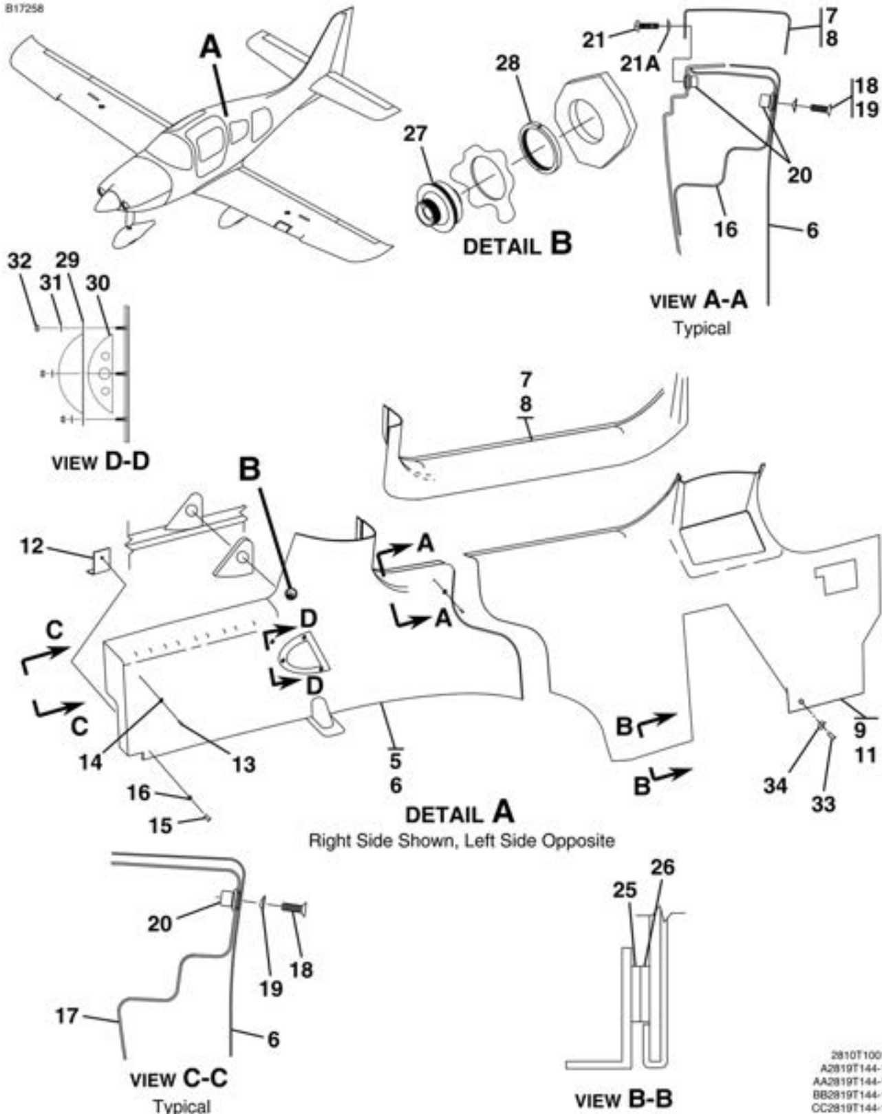
INTERIOR PANELS INSTALLATION - FOWARD AND MID CABIN FIGURE 07 (SHEET 2)
