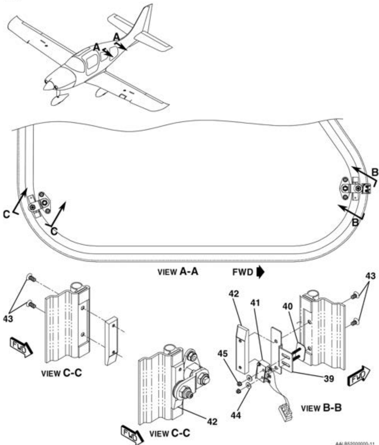
CABIN AND BAGGAGE DOOR INSTALLATION FIGURE 01 (SHEET 6)
