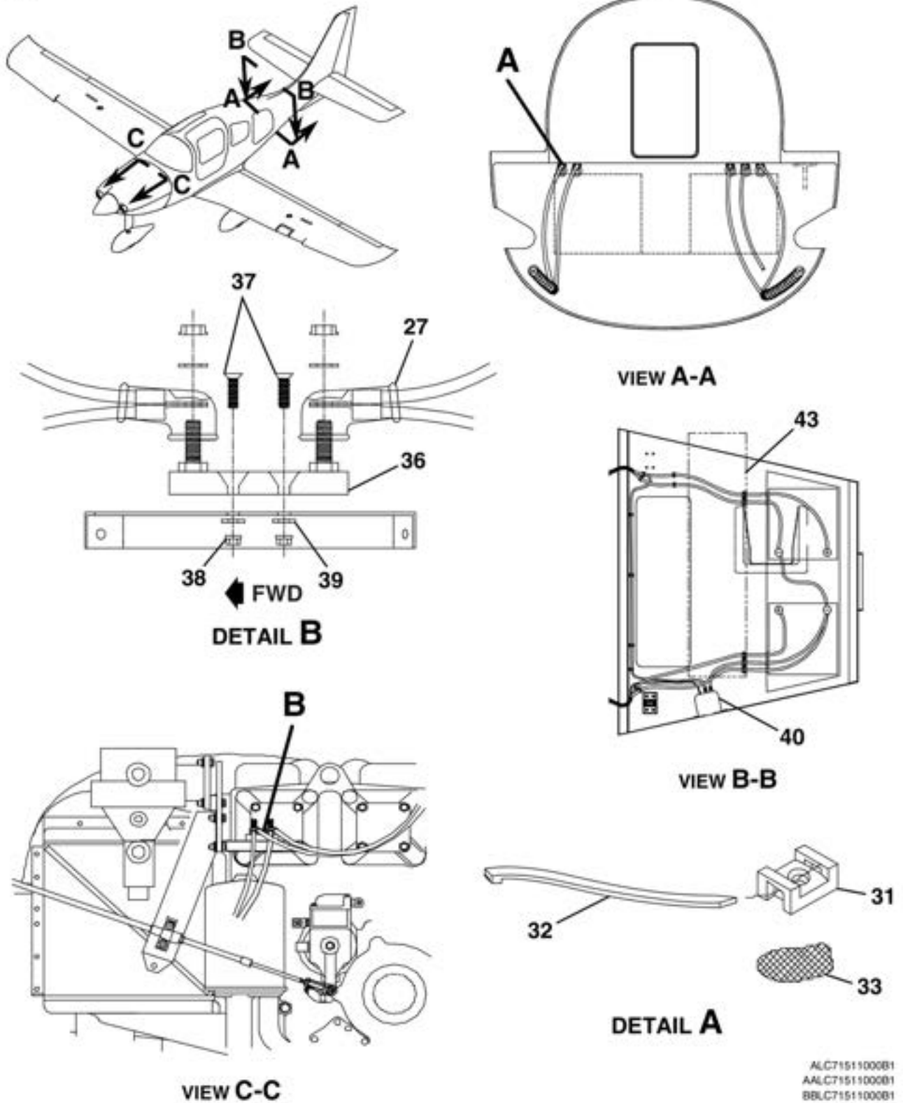
BATTERY INSTALLATION FIGURE 06 (SHEET 3)
