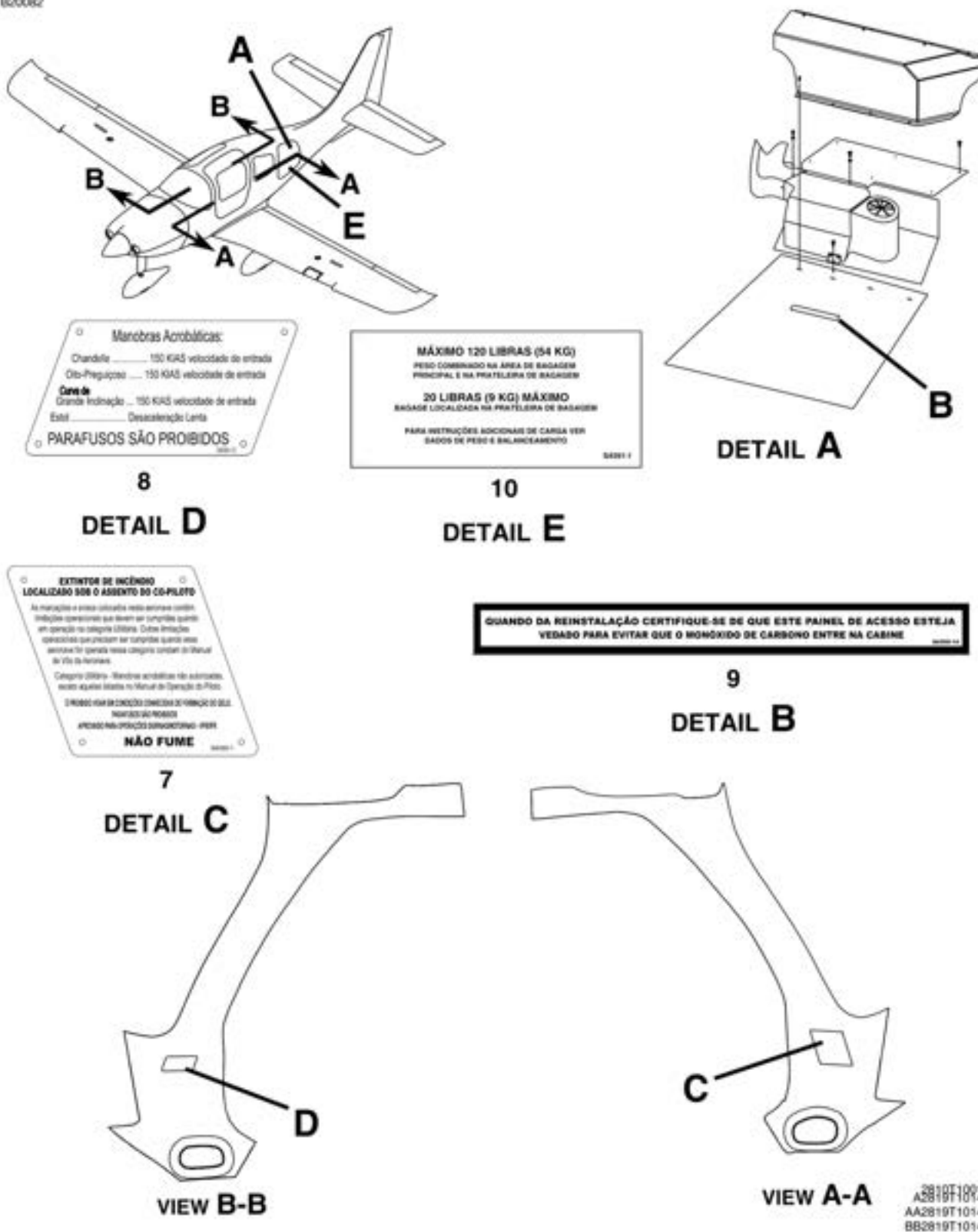
INTERIOR PLACARDS AND MARKINGS - FUSELAGE - BRAZIL FIGURE 01A (SHEET 2)
