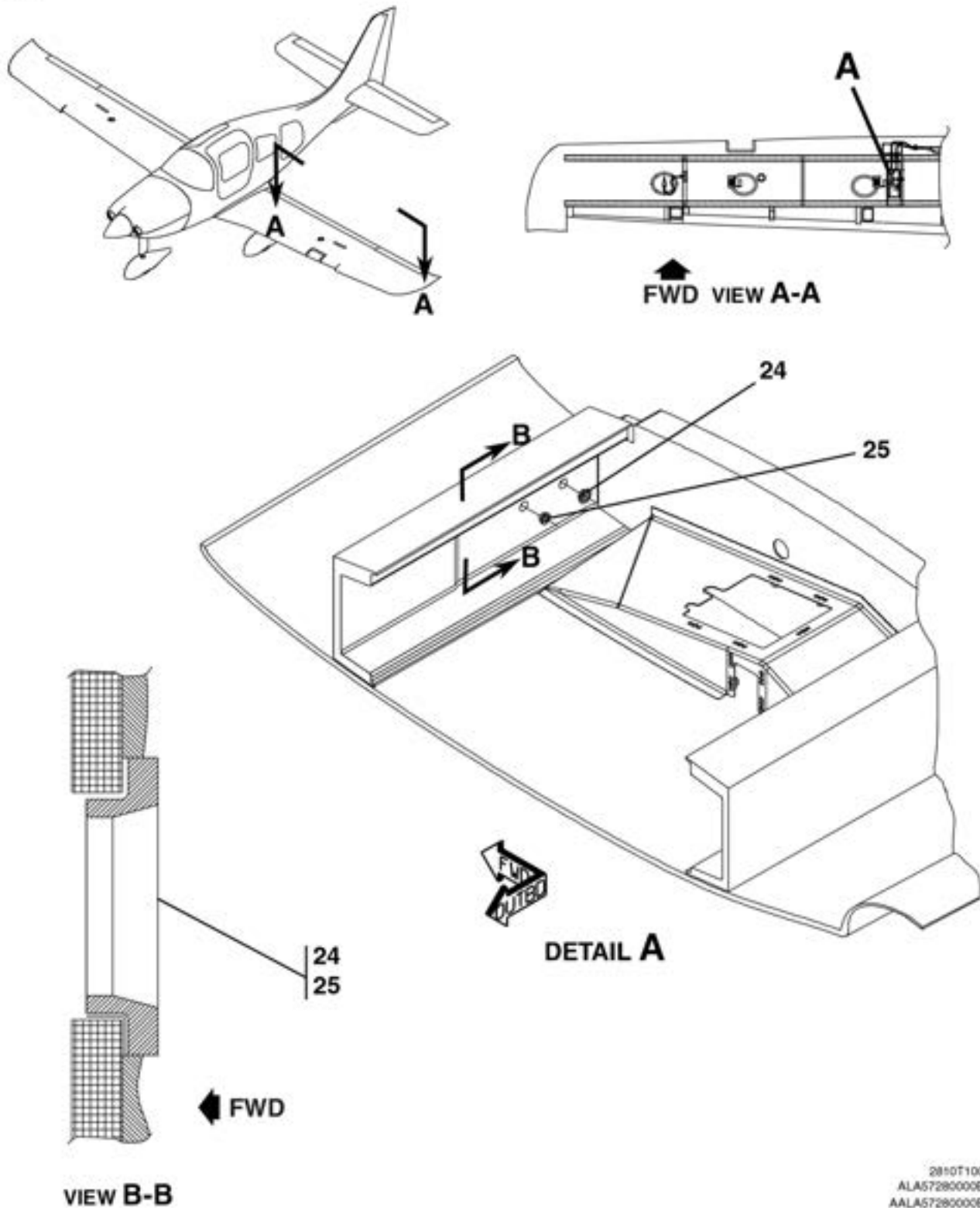
FUEL SYSTEM - WING ASSEMBLY FIGURE 04 (SHEET 4)
