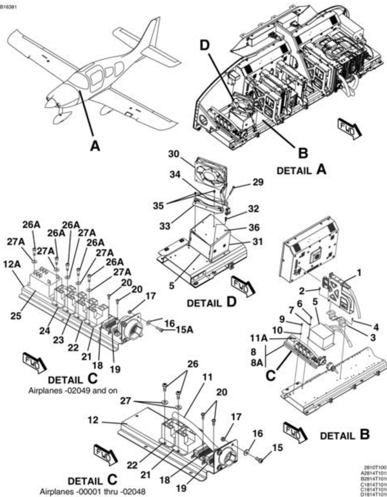
AVIONICS AND NAVIGATION EQUIPMENT - CHIPS MODULE, SMALL PARTS MODULE, & AUXILLARY RELAY INSTALLATION FIGURE 07 (SHEET 1)
