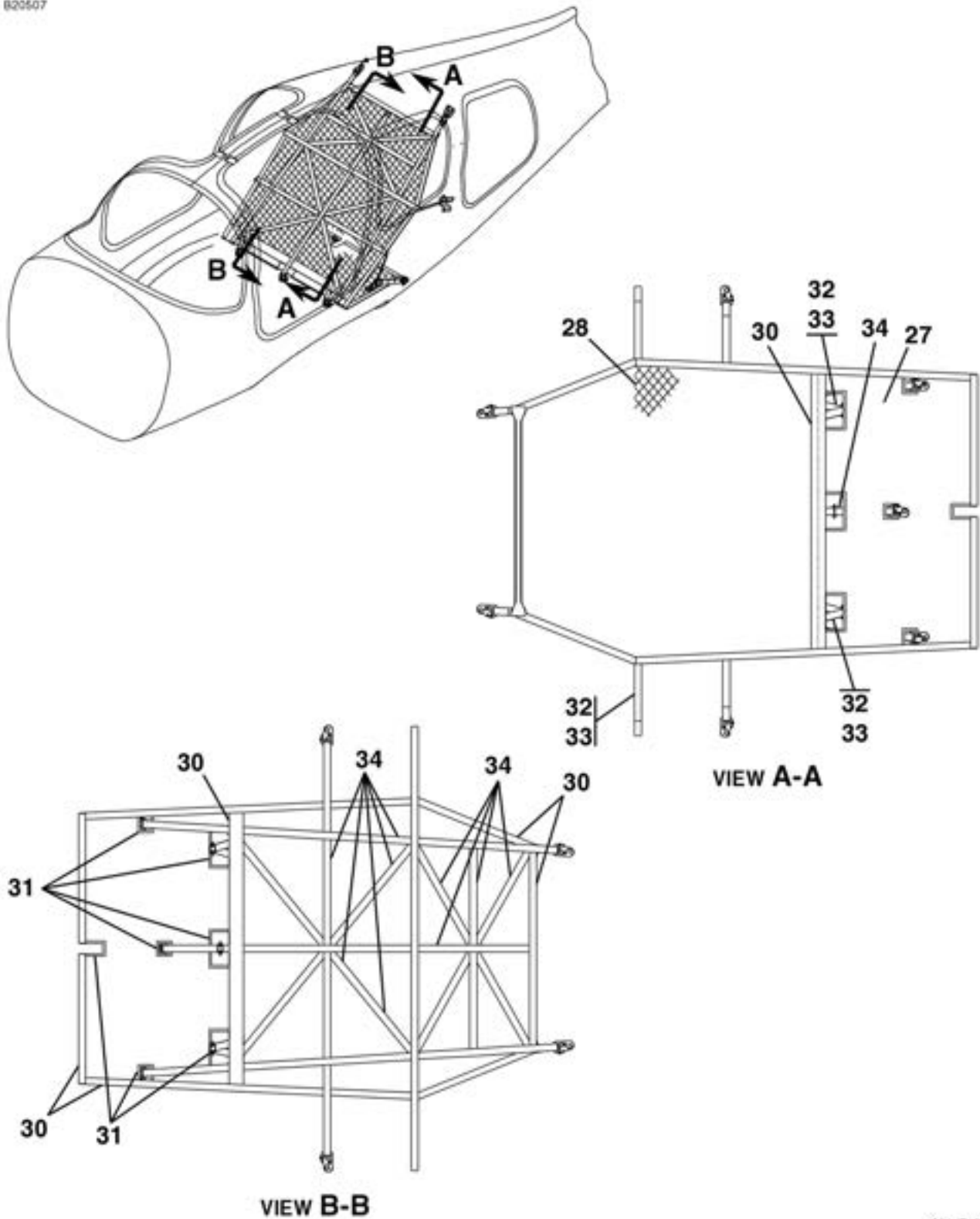
CARGO BARRIER NET INSTALLATION FIGURE 09 (SHEET 2)
