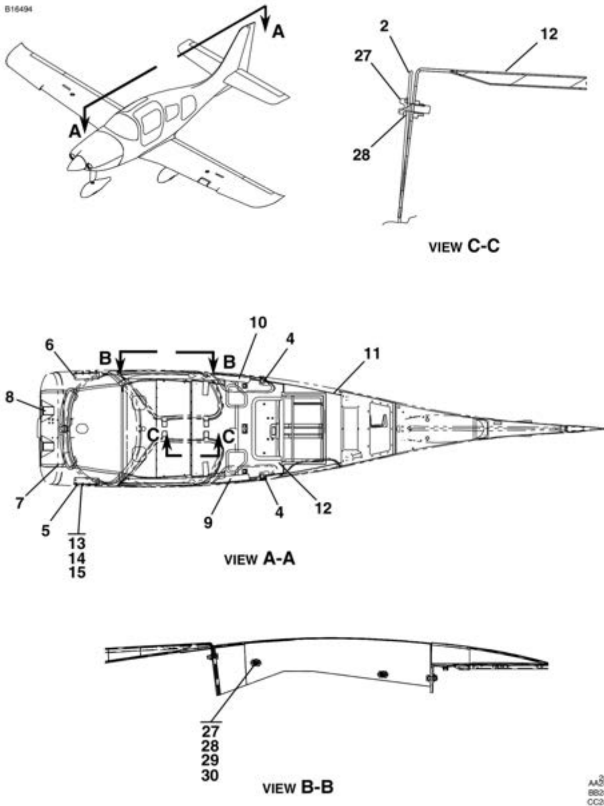
FUSELAGE STRUCTURE ASSEMBLY FIGURE 01 (SHEET 3)
