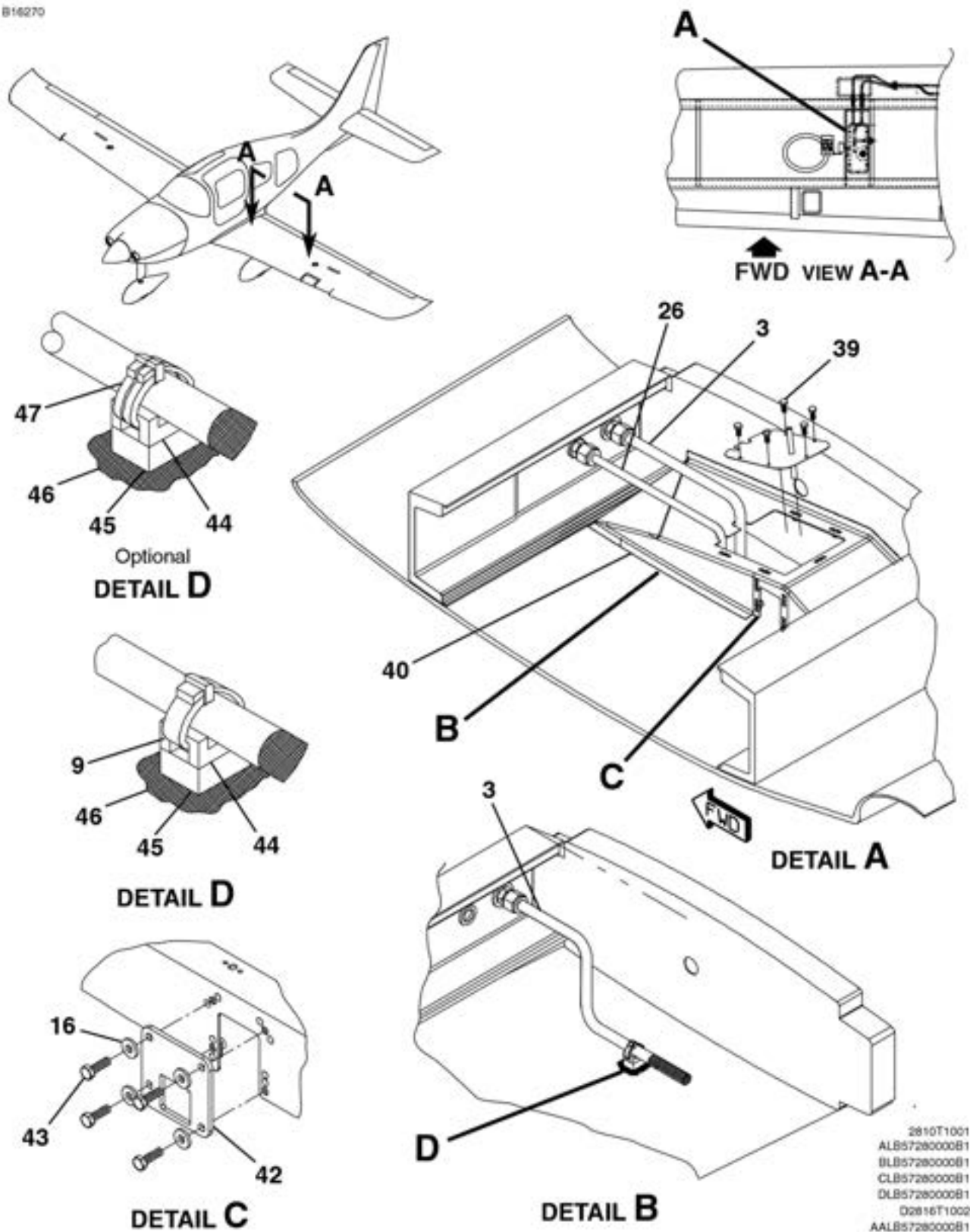
FUEL SYSTEM - WING ASSEMBLY FIGURE 04 (SHEET 7)
