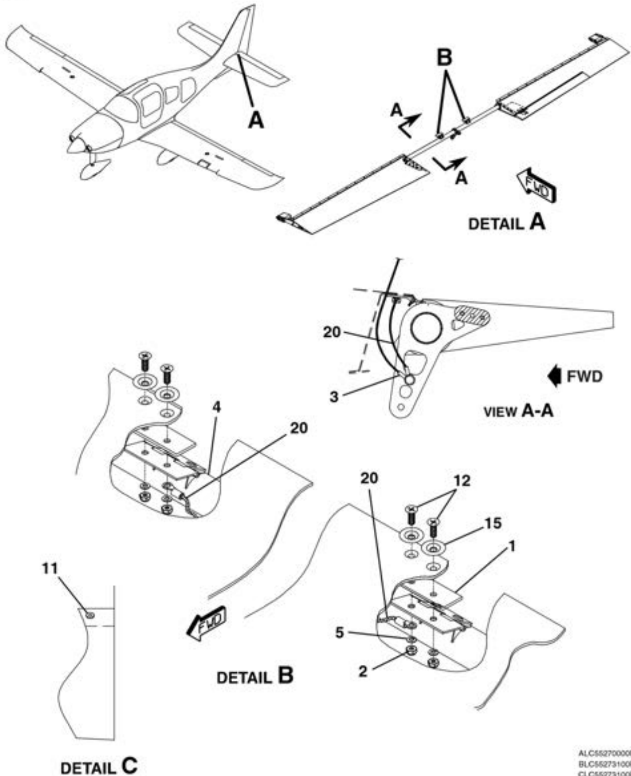
ELEVATOR ATTACH ASSEMBLY FIGURE 05 (SHEET 2)
