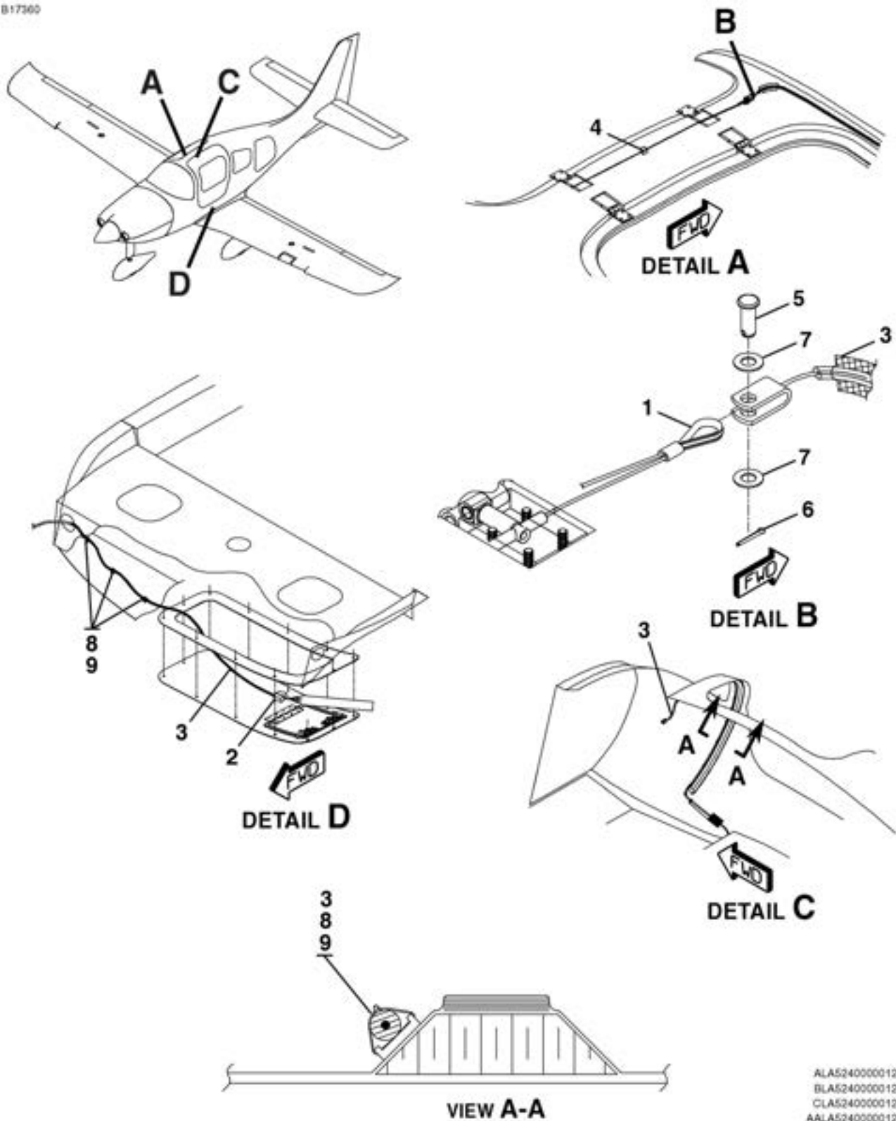
EMERGENCY DOOR RELEASE ASSEMBLY FIGURE 08 (SHEET 1)
