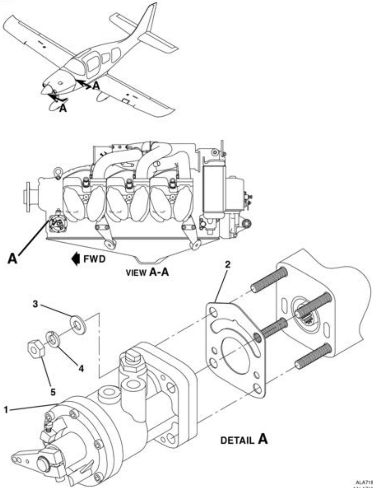
PROPELLER GOVERNOR ASSEMBLY FIGURE 02 (SHEET 1)
