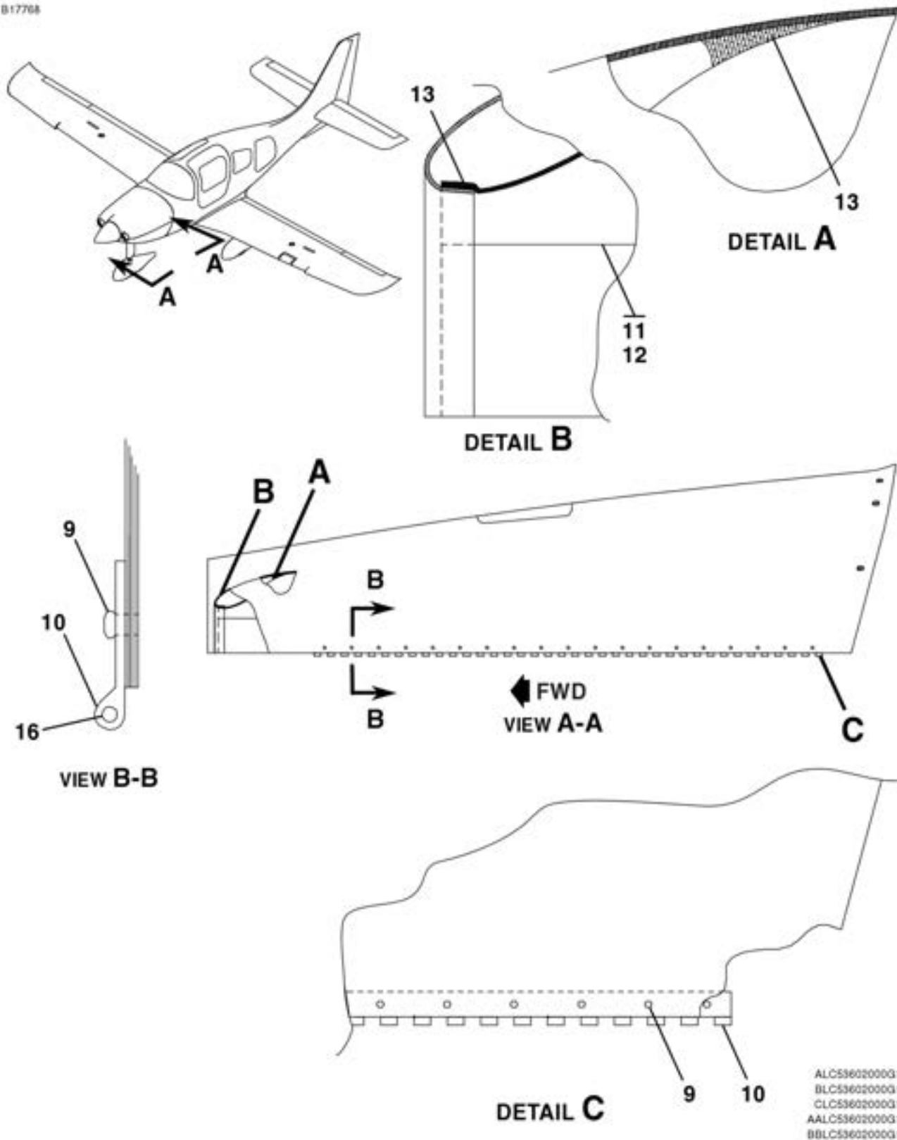
UPPER COWL ASSEMBLY FIGURE 05 (SHEET 1)
