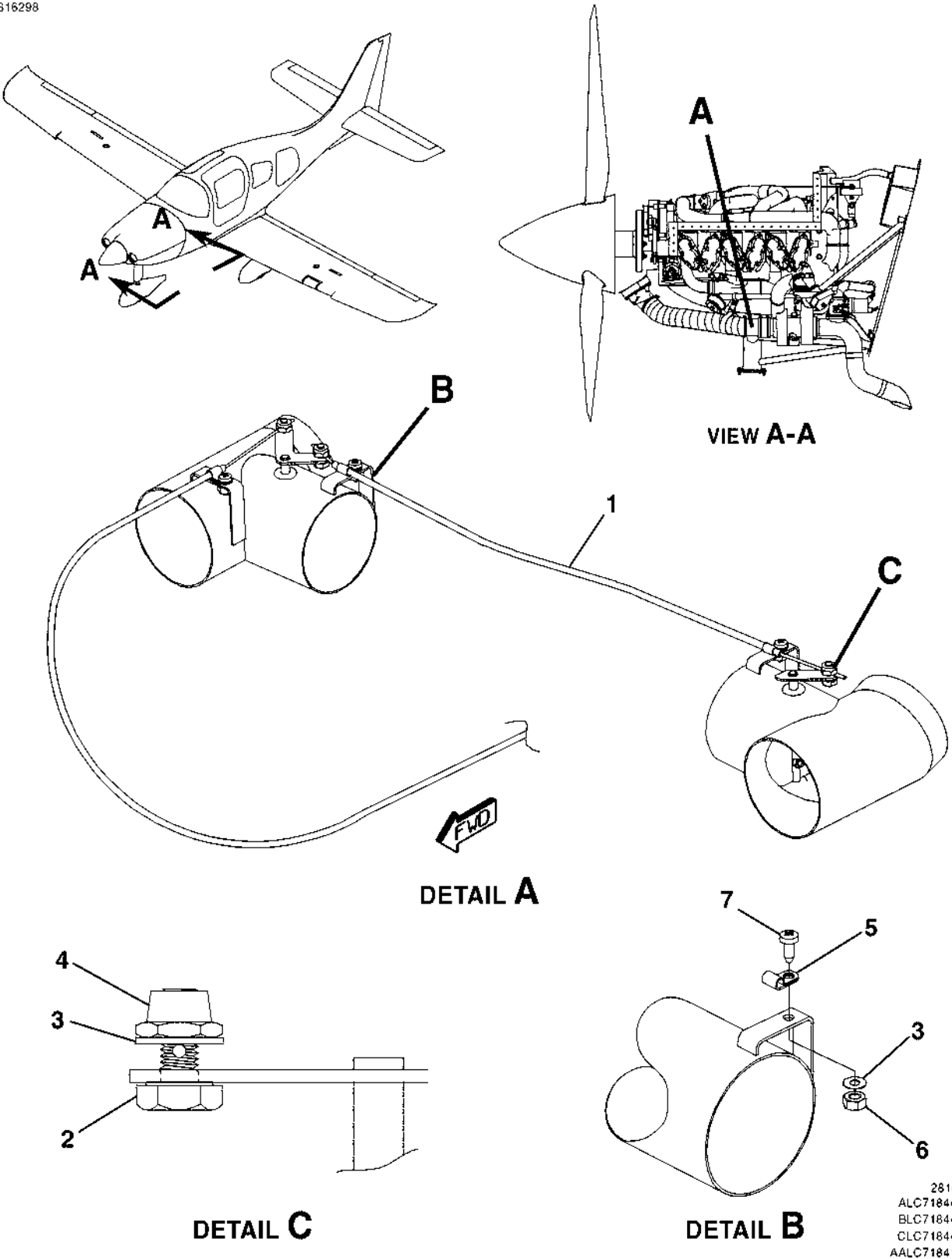
WARM AIR INDUCTION ASSEMBLY FIGURE 03 (SHEET 1)
