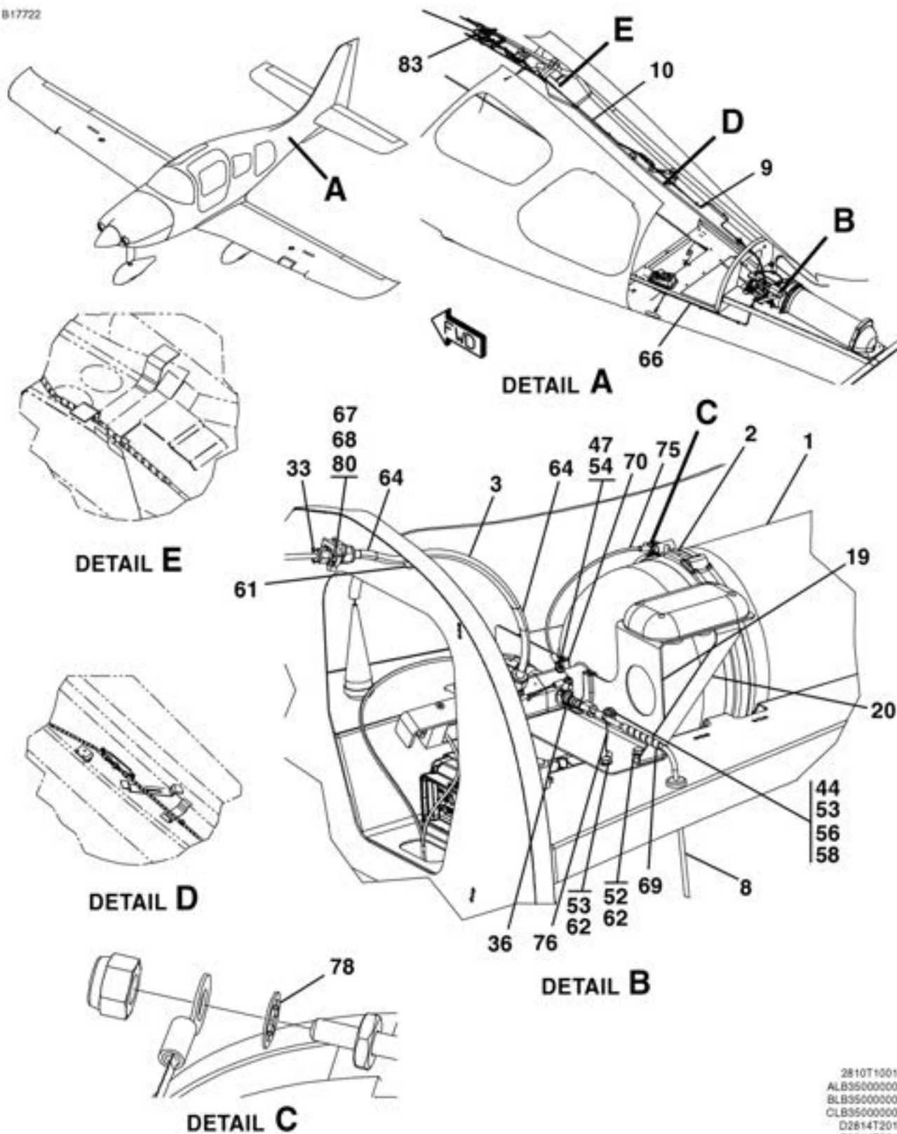
OXYGEN SYSTEM ASSEMBLY FIGURE 01 (SHEET 1)
