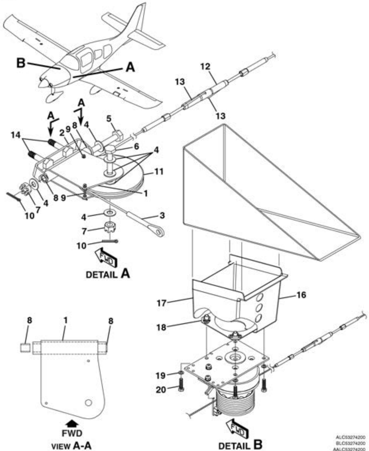
RUDDER PEDAL INTERCONNECT ASSEMBLY FIGURE 08 (SHEET 1)
