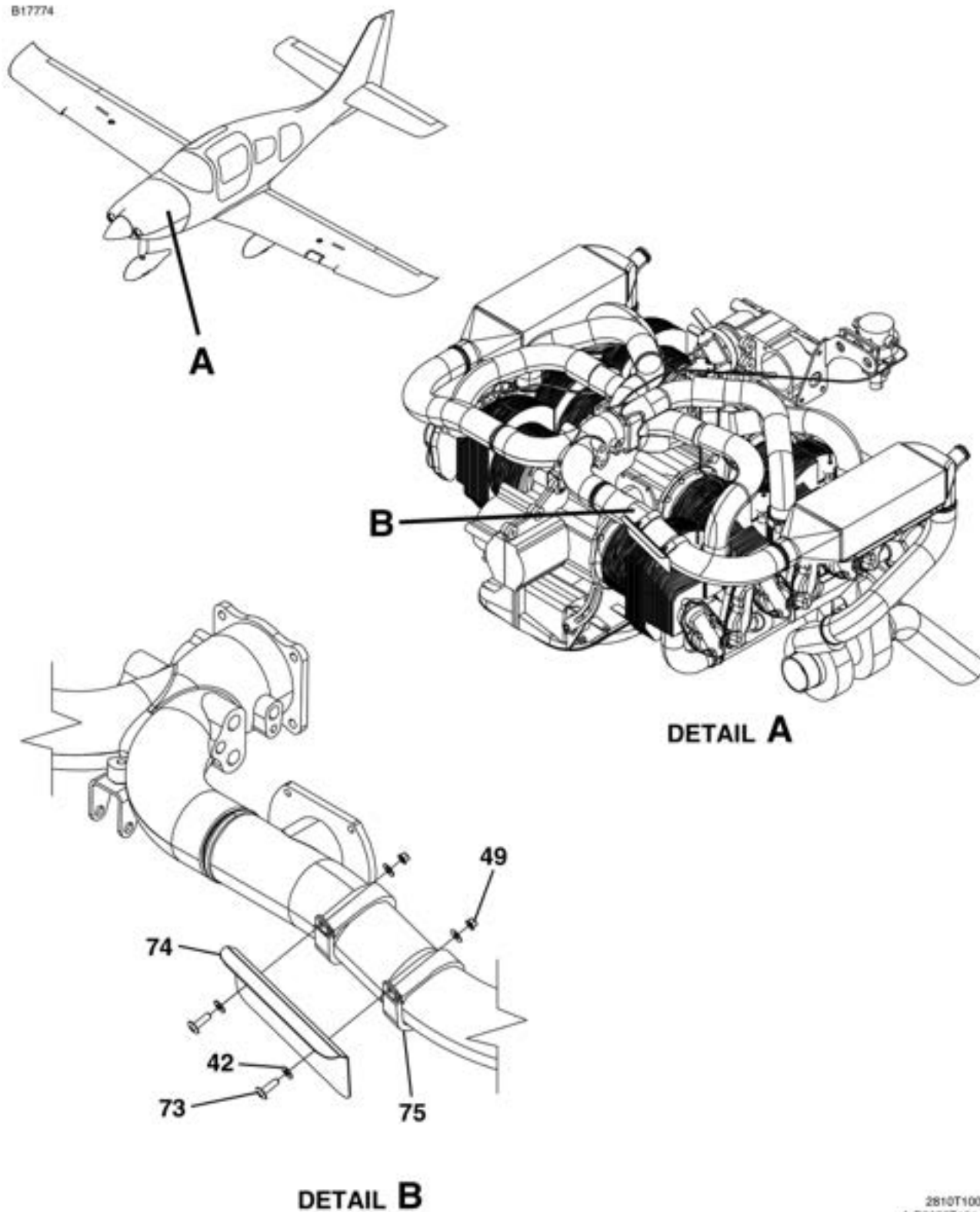
ENGINE BAFFLING ASSEMBLY FIGURE 07 (SHEET 3)
