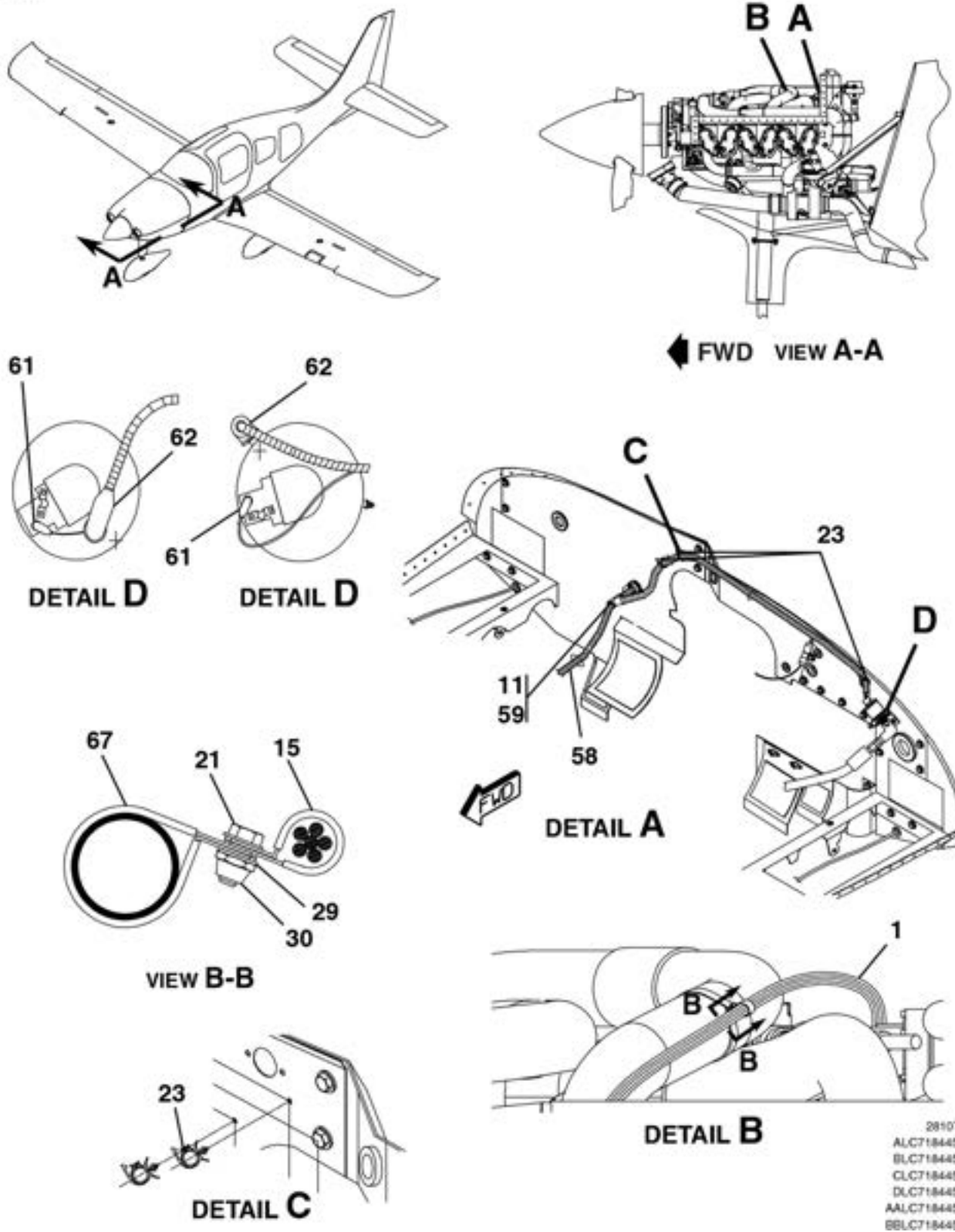
WIRING AND SENSORS ASSEMBLY FIGURE 02 (SHEET 1)
