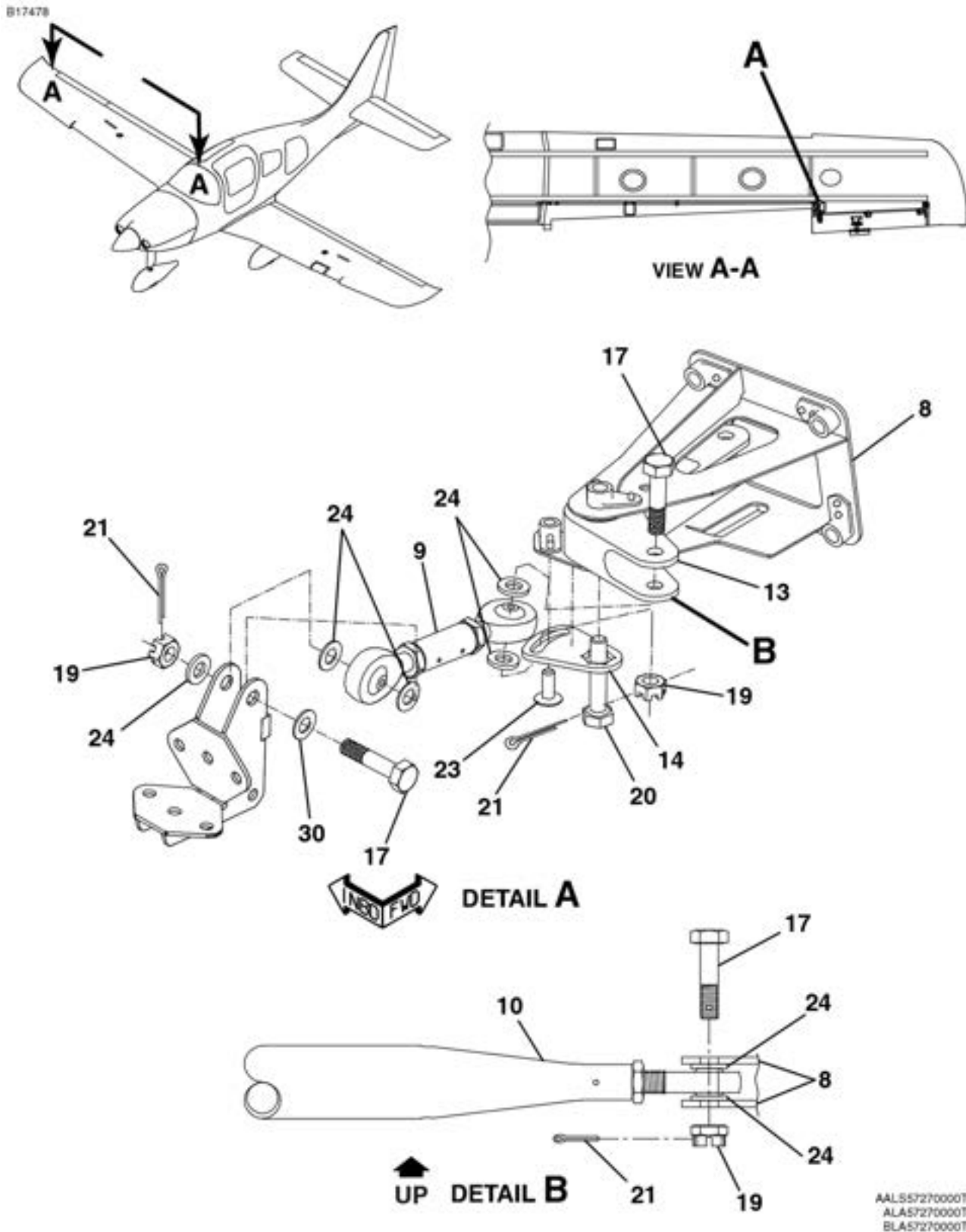
AILERON INSTALLATION FIGURE 10 (SHEET 2)
