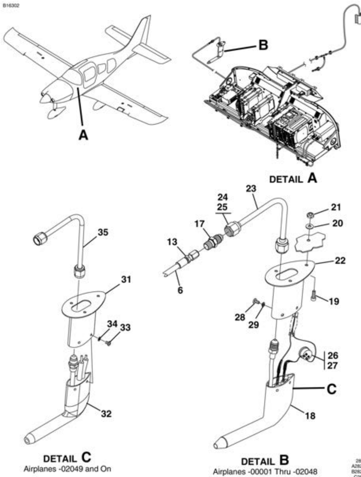
PITOT/STATIC INSTALLATION FIGURE 01 (SHEET 2)
