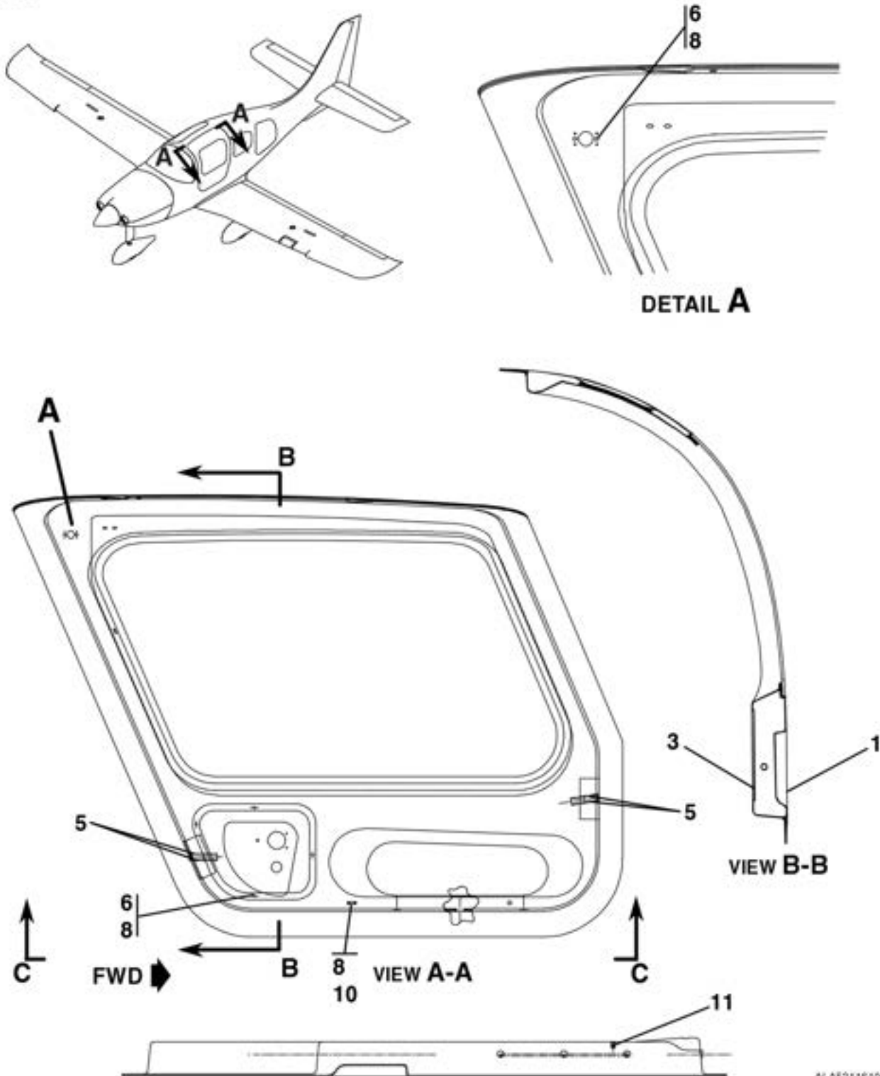
VIEW C-C Left Side Shown, Right Side Opposite CABIN DOOR STRUCTURE FIGURE 03 (SHEET 1)
