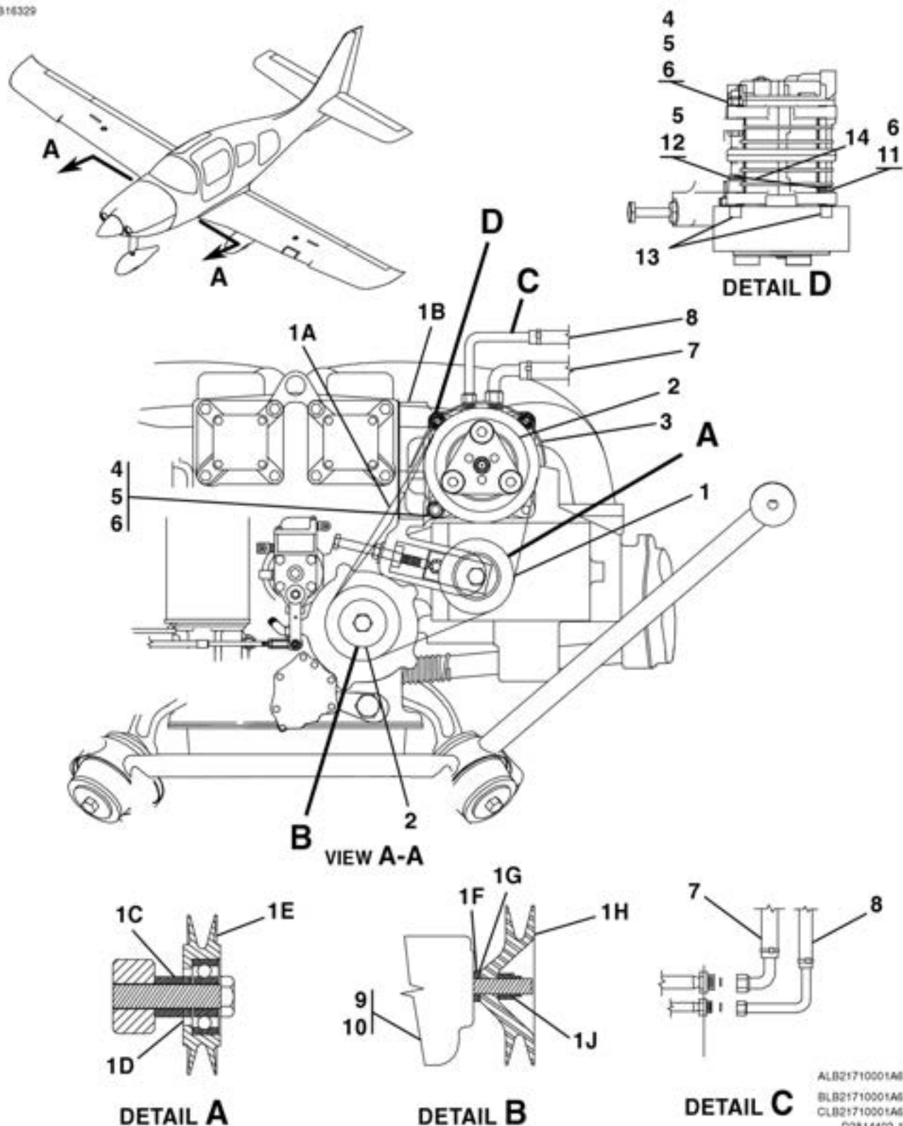
AIR CONDITIONING INSTALLATION ASSEMBLY - FIREWALL FORWARD FIGURE 06 (SHEET 1)
