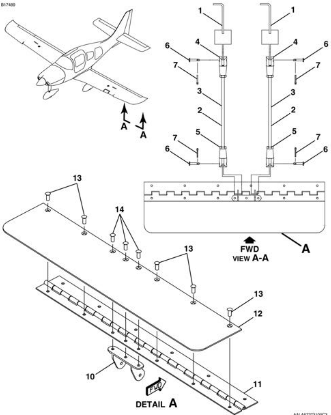
SERVO TAB ASSEMBLY - AILERON FIGURE 13 (SHEET 2)
