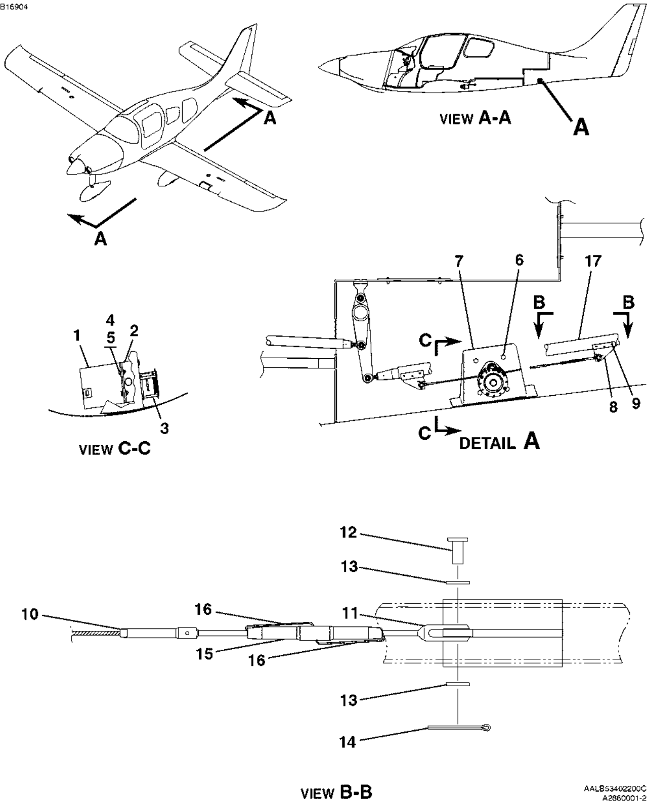
AUTOPILOT INSTALLATION - PITCH FIGURE 02 (SHEET 1)
