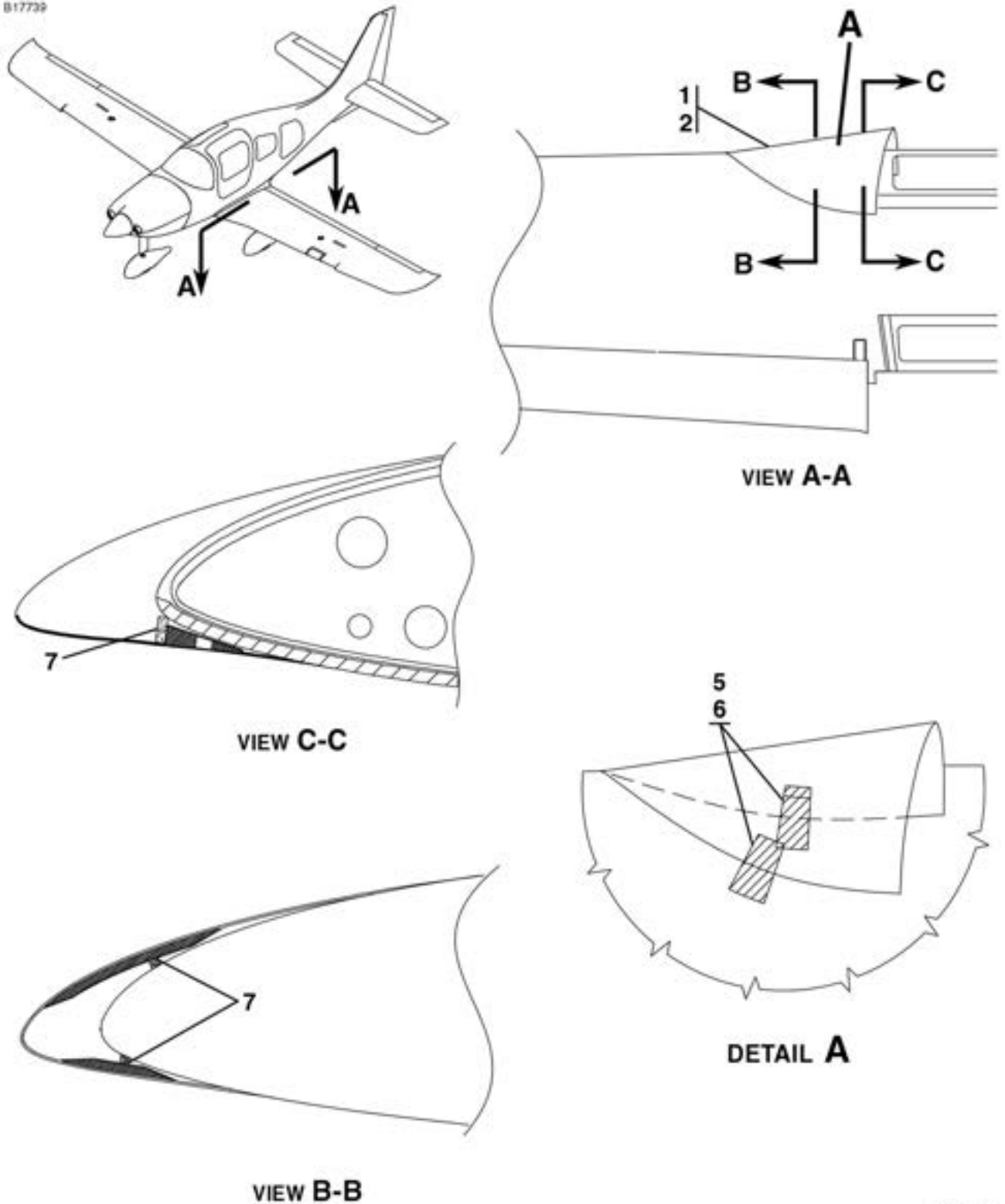
STRAKE INSTALLATION FIGURE 07 (SHEET 1)
