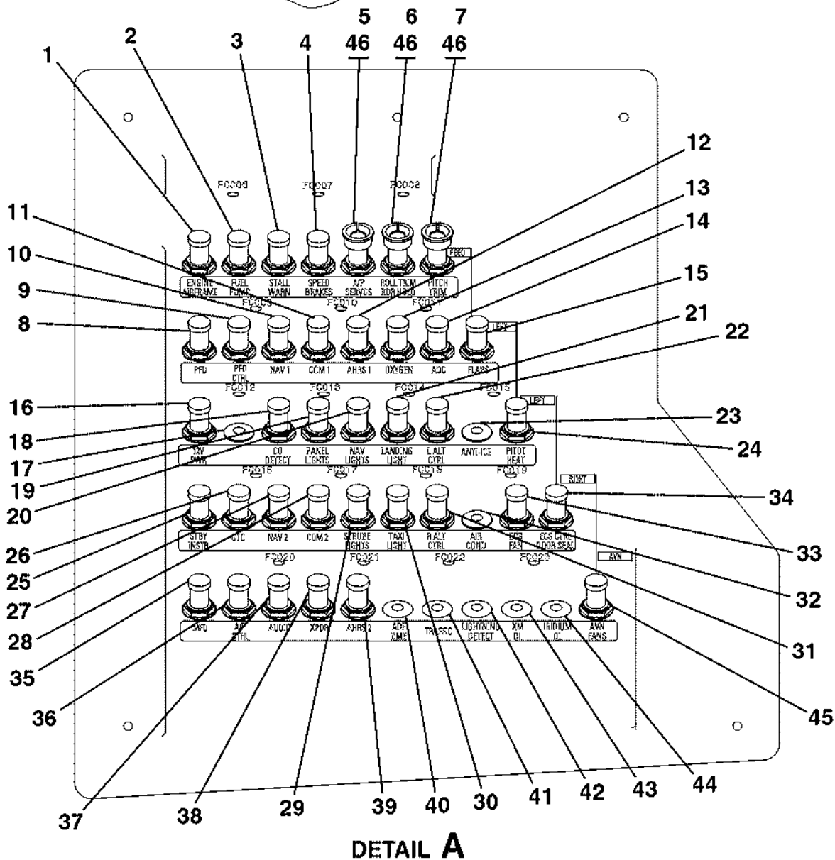
CIRCUIT BREAKER PANEL ASSEMBLY - CIRCUIT BREAKERS FIGURE 05 (SHEET 1)
