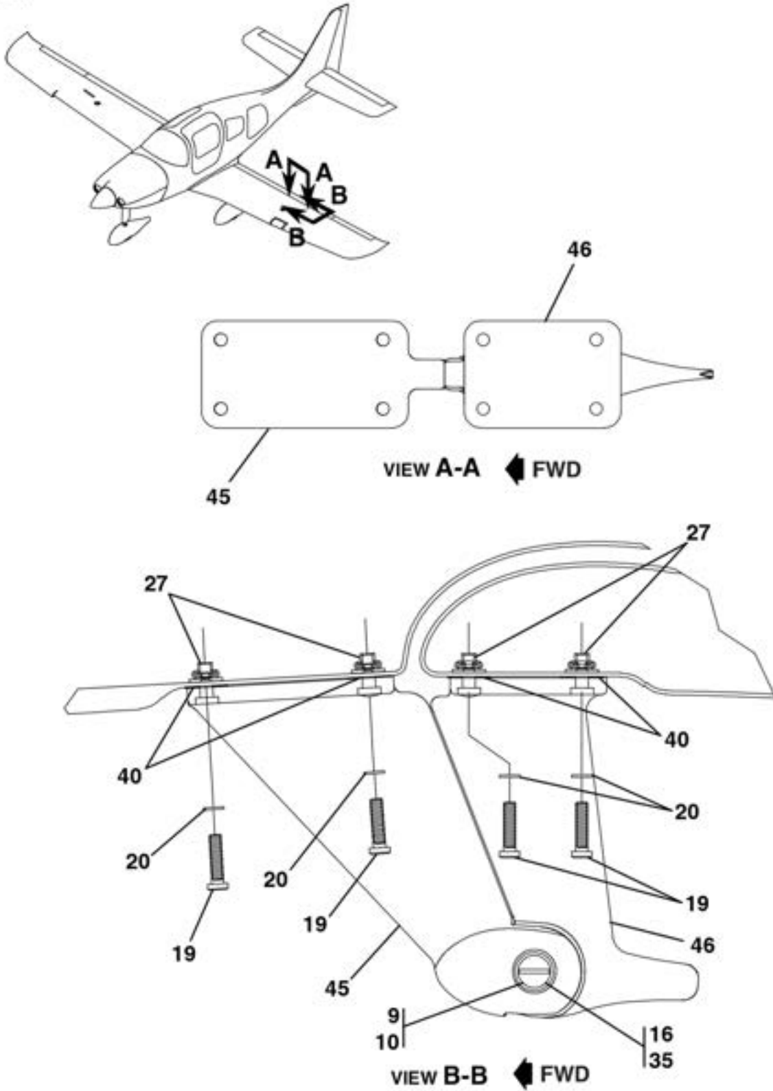
FLAP ASSEMBLY FIGURE 18 (SHEET 6)
