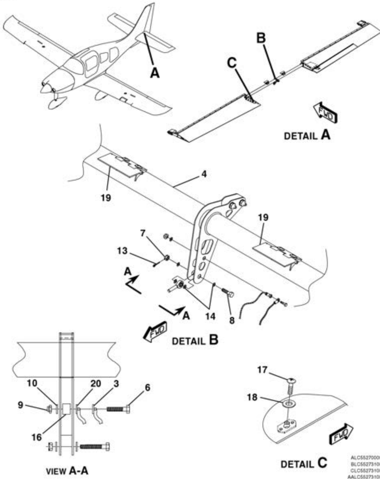
ELEVATOR ATTACH ASSEMBLY FIGURE 05 (SHEET 1)
