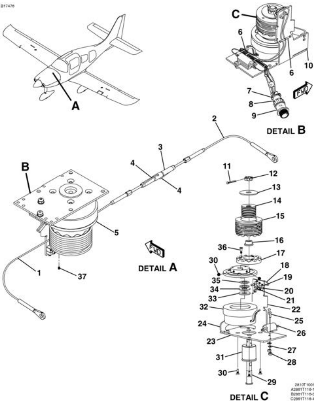
RUDDER HOLD BRAKE AND CABLES ASSEMBLY FIGURE 09 (SHEET 1)
