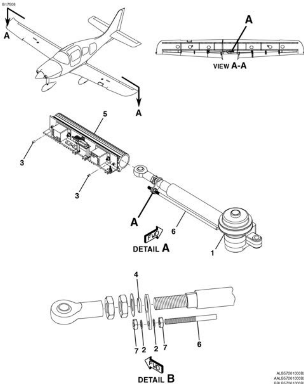
FLAP ACTUATOR ASSEMBLY FIGURE 20 (SHEET 1)
