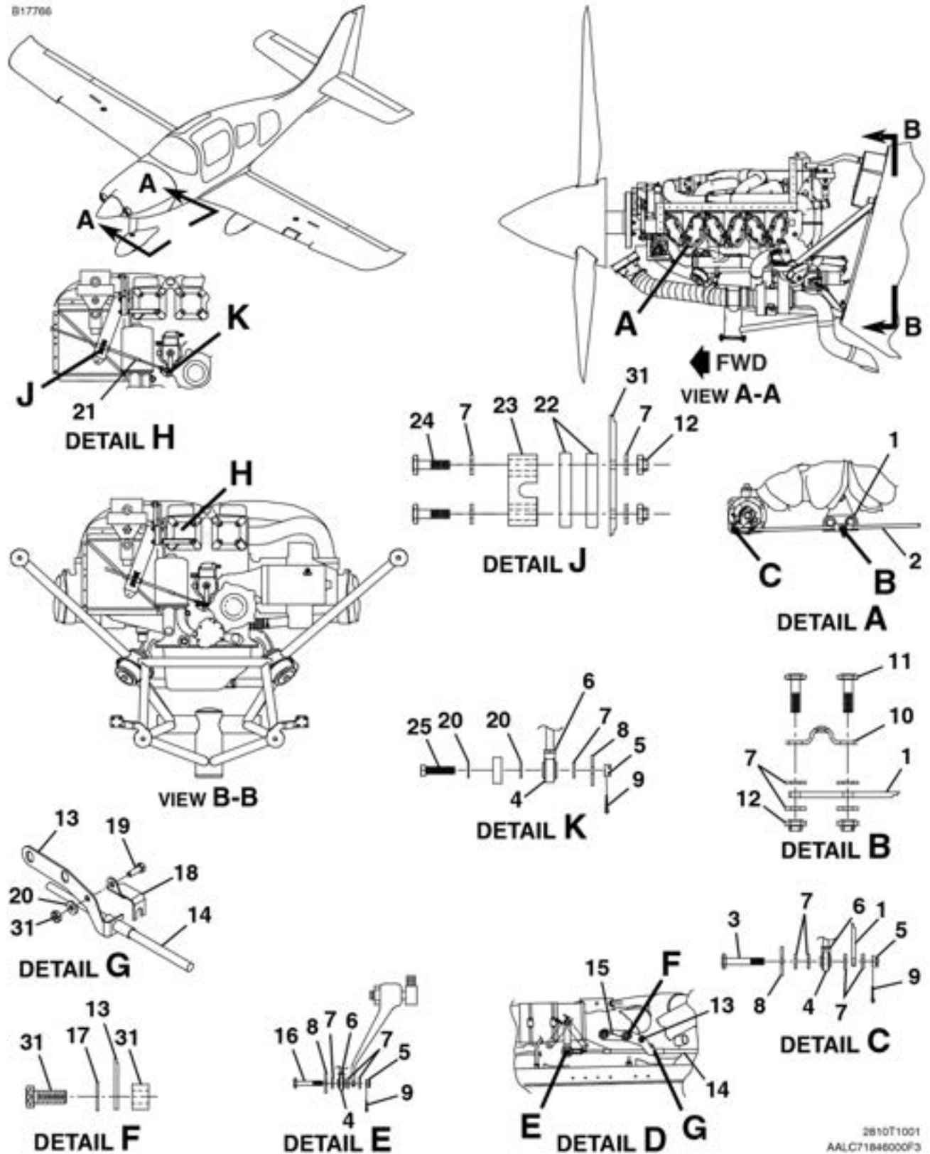
FORWARD ENGINE CONTROLS ASSEMBLY FIGURE 01 (SHEET 1)
