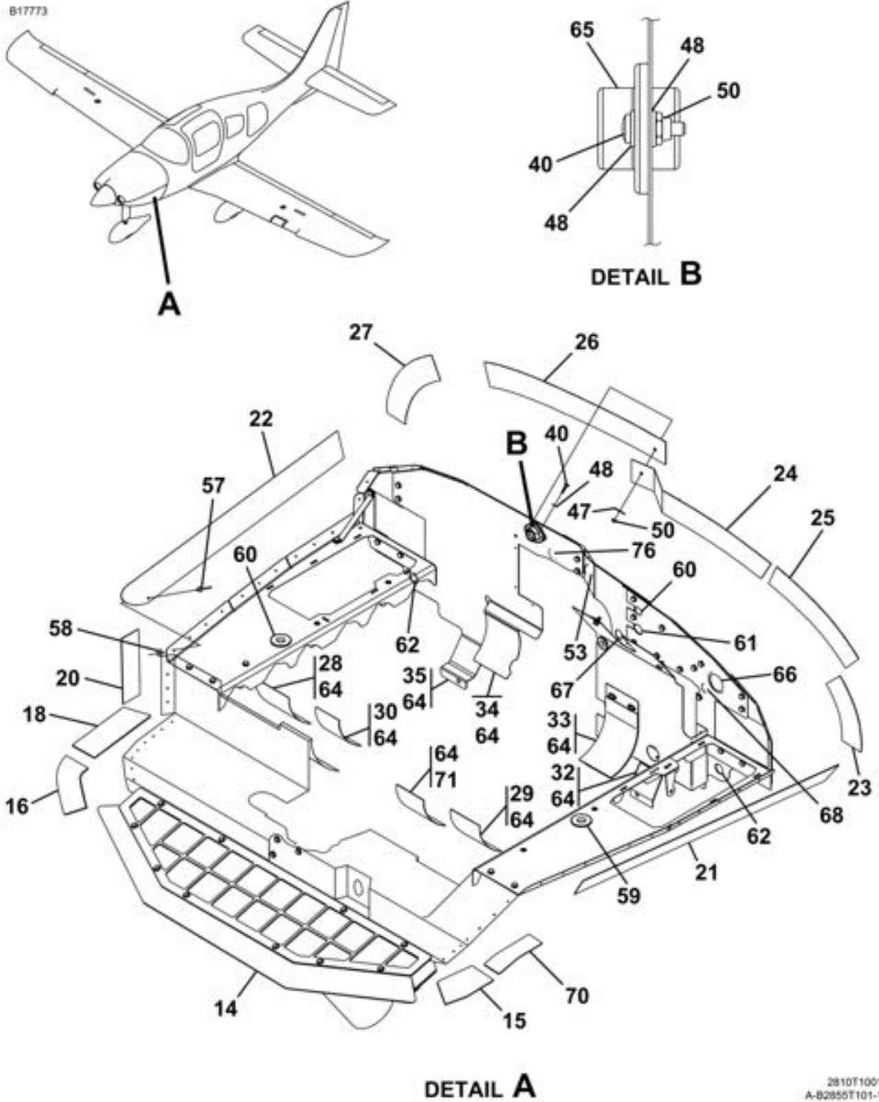
ENGINE BAFFLING ASSEMBLY FIGURE 07 (SHEET 2)
