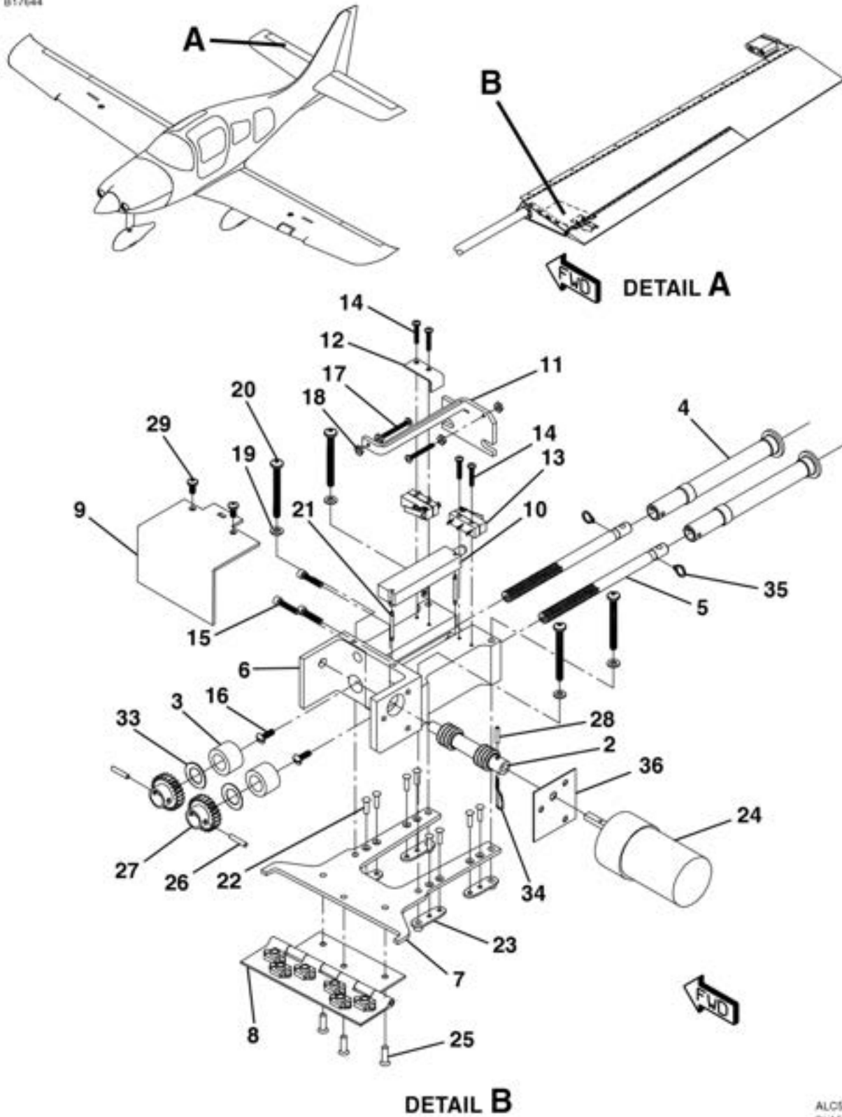
ELEVATOR TRIM ACTUATOR ASSEMBLY FIGURE 07 (SHEET 1)
