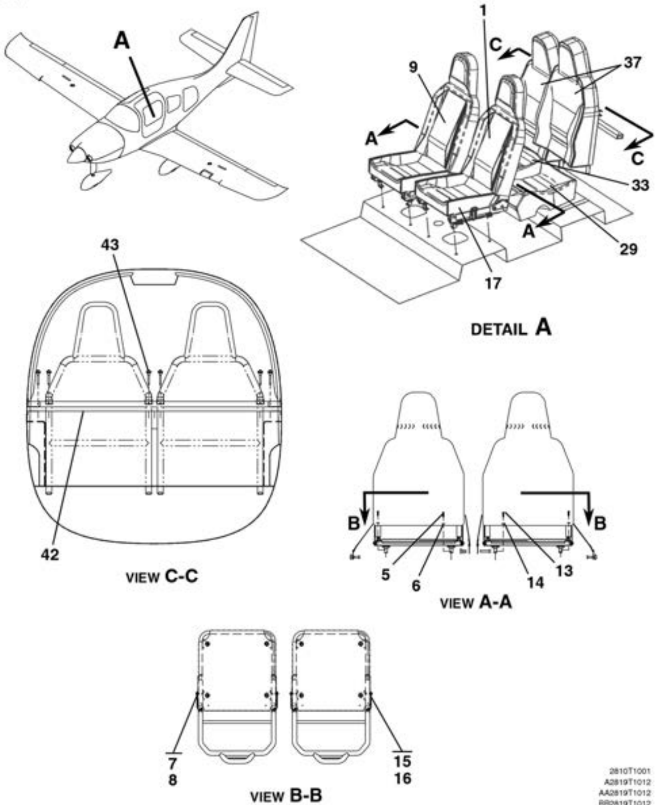
SEAT INSTALLATION FIGURE 01 (SHEET 1)
