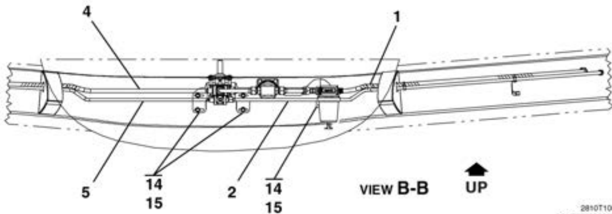
FUEL SYSTEM - WING ASSEMBLY FIGURE 04 (SHEET 2)
