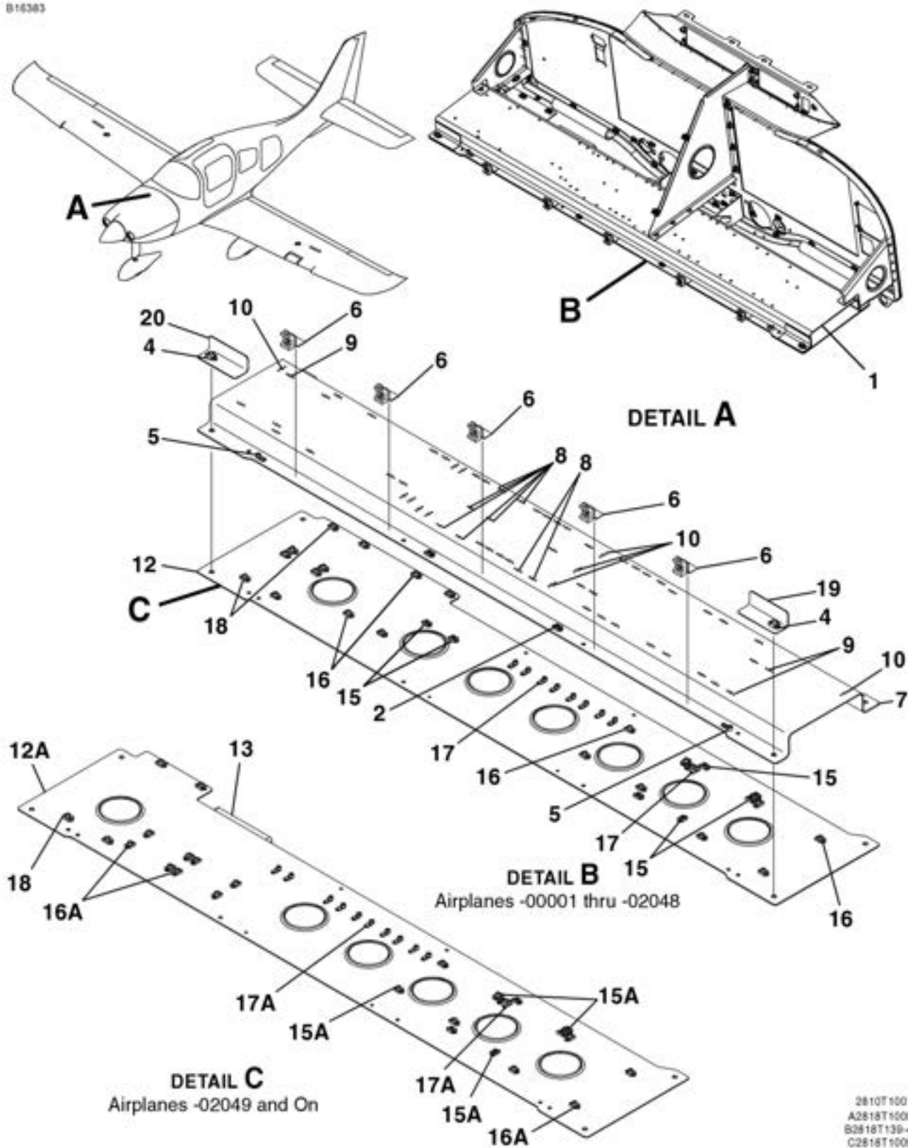
AVIONICS SHELF ASSEMBLY FIGURE 06 (SHEET 1)
