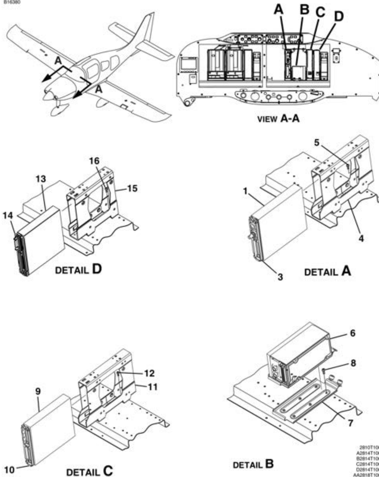
AVIONICS AND NAVIGATION EQUIPMENT - GDL 69A, GDC 74A, GEA 71, GMA 36, AND STALL WARNING COMPUTER INSTALLATION FIGURE 06 (SHEET 1)
