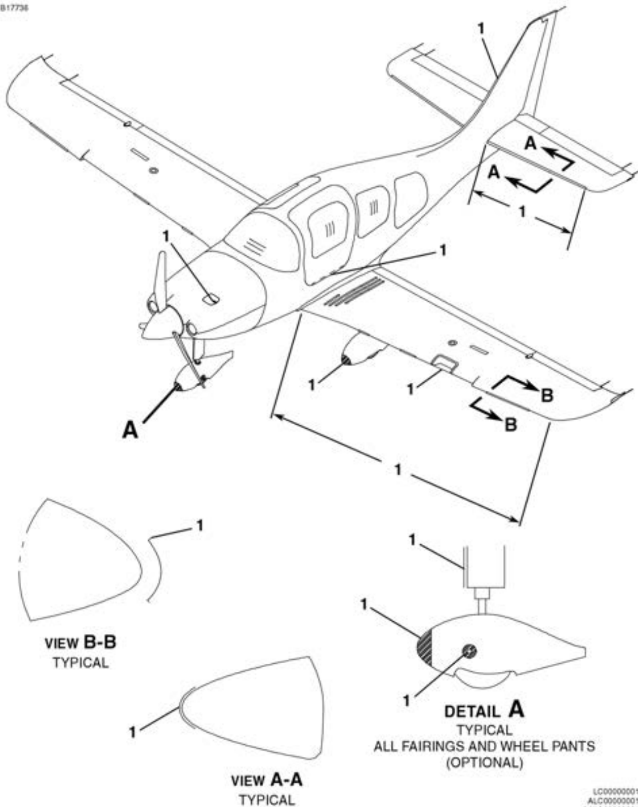
ANTI-CHAFE TAPE INSTALLATION FIGURE 04 (SHEET 1)
