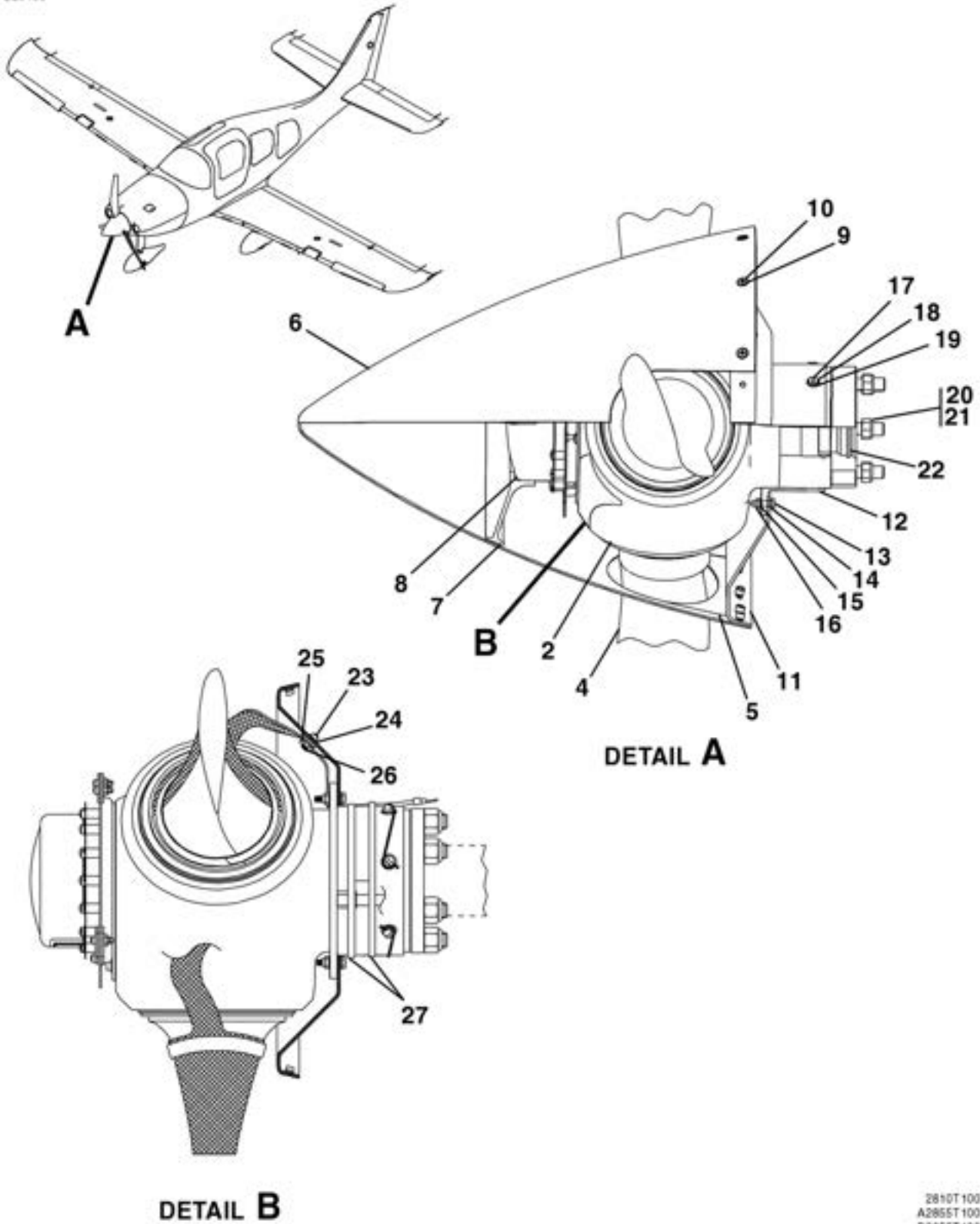
PROPELLER ASSEMBLY - MCCAULEY FIGURE 01A (SHEET 1)
