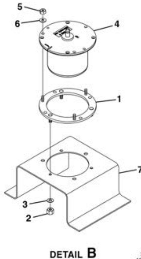
MAGNETOMETER INSTALLATION FIGURE 15 (SHEET 1)
