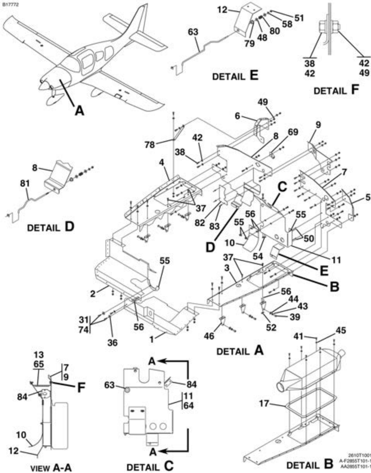
ENGINE BAFFLING ASSEMBLY FIGURE 07 (SHEET 1)
