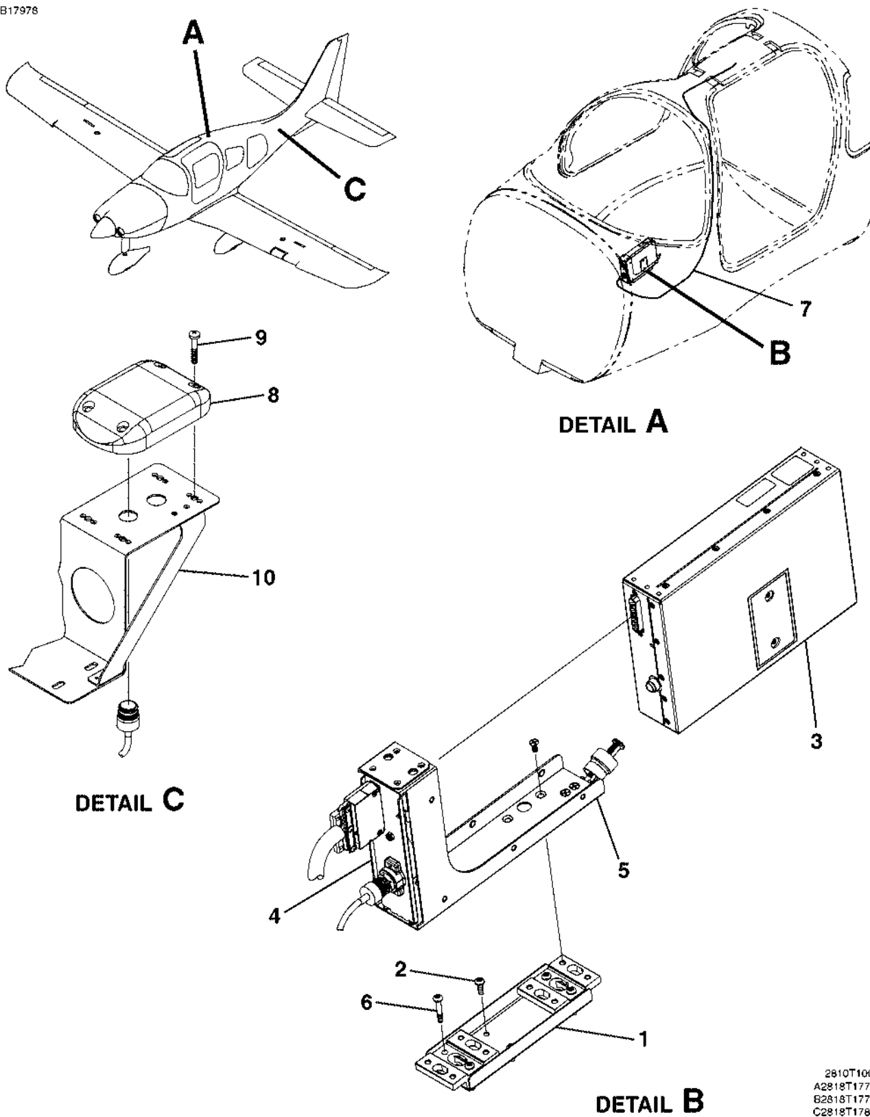
IRIDIUM SATELLITE DATALINK INSTALLATION FIGURE 16 (SHEET 1)
