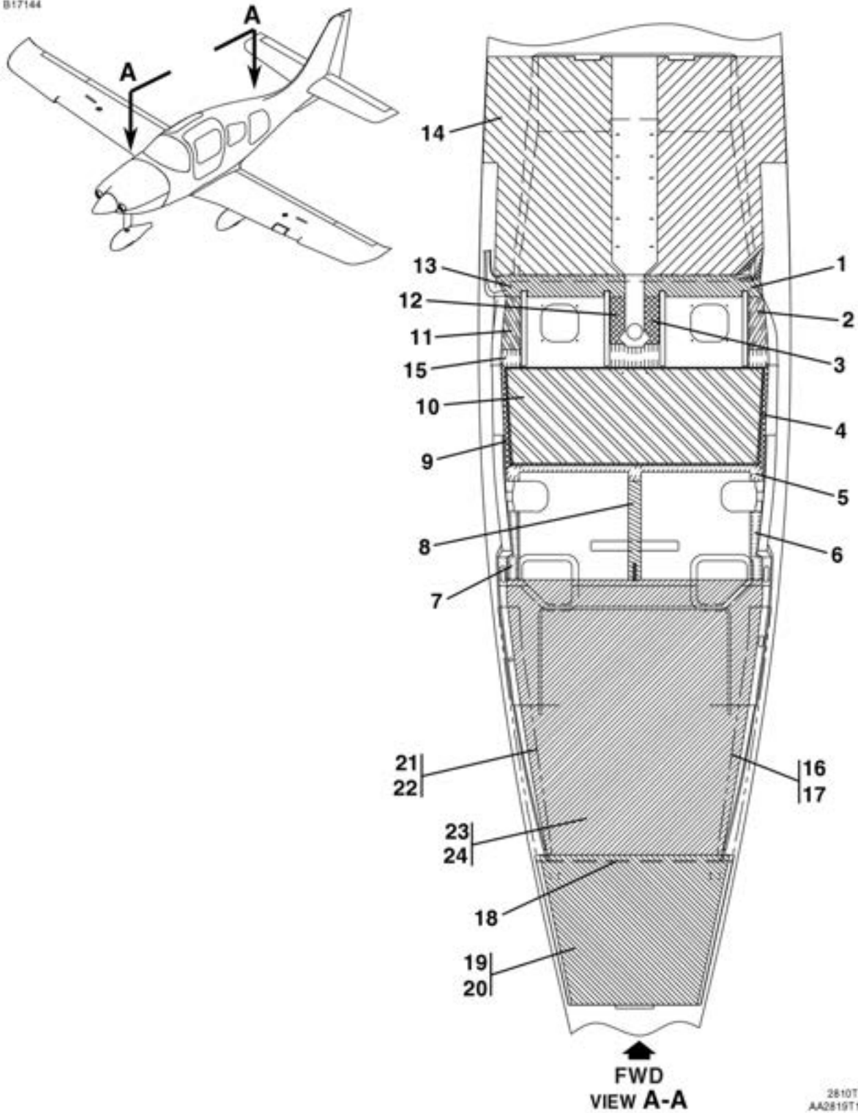
CARPET INSTALLATION FIGURE 17 (SHEET 1)
