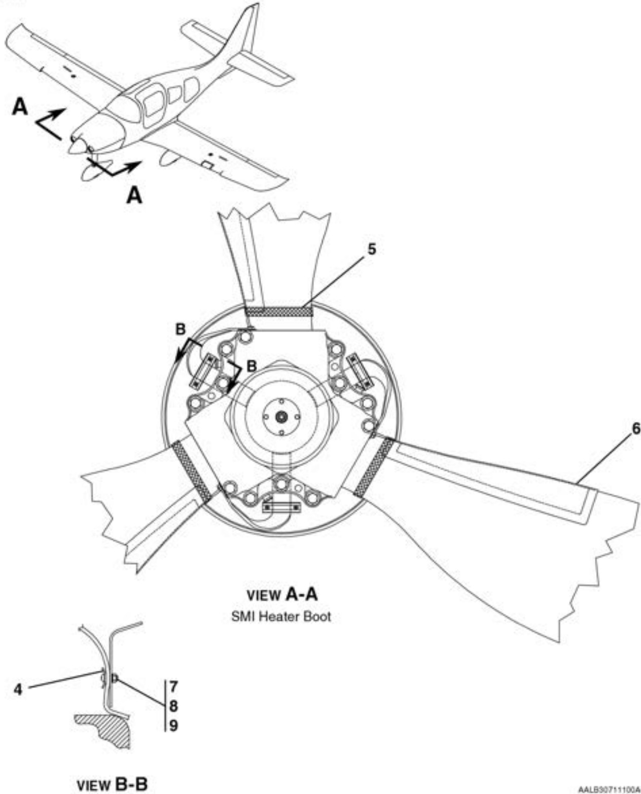
PROPELLER HEAT SYSTEM - BOOTED AND NON-BOOTED FIGURE 01 (SHEET 2)
