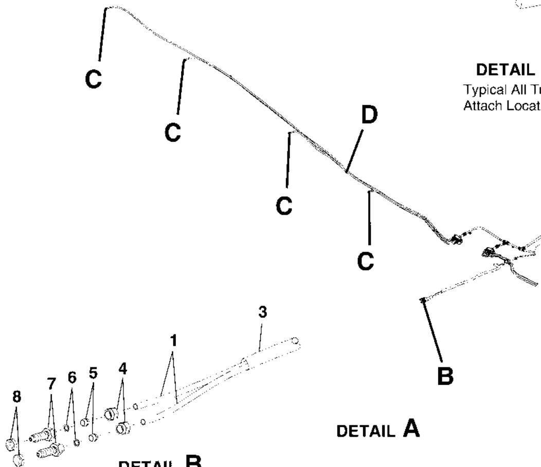
TKS SYSTEM - PLUMBING INSTALLATION FIGURE 05A (SHEET 1)
