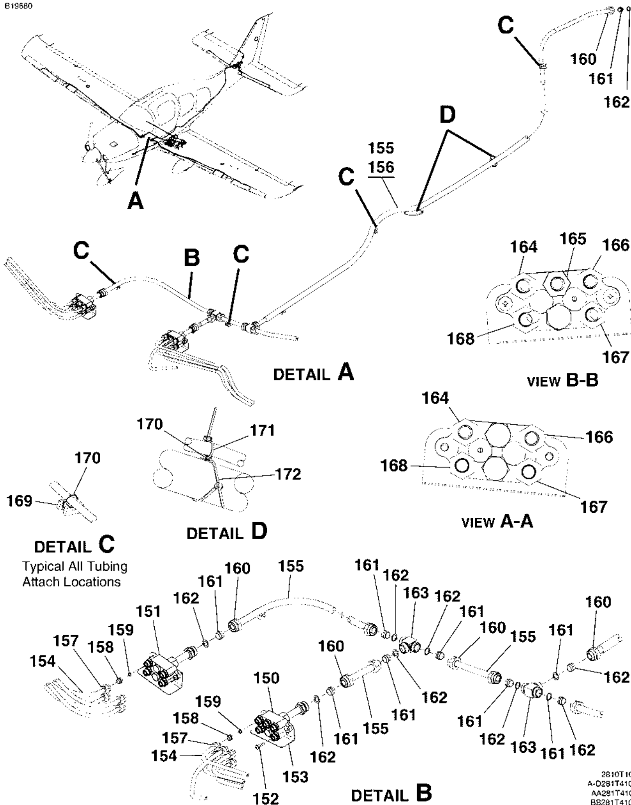
TKS SYSTEM - PLUMBING INSTALLATION FIGURE 05A (SHEET 3)
