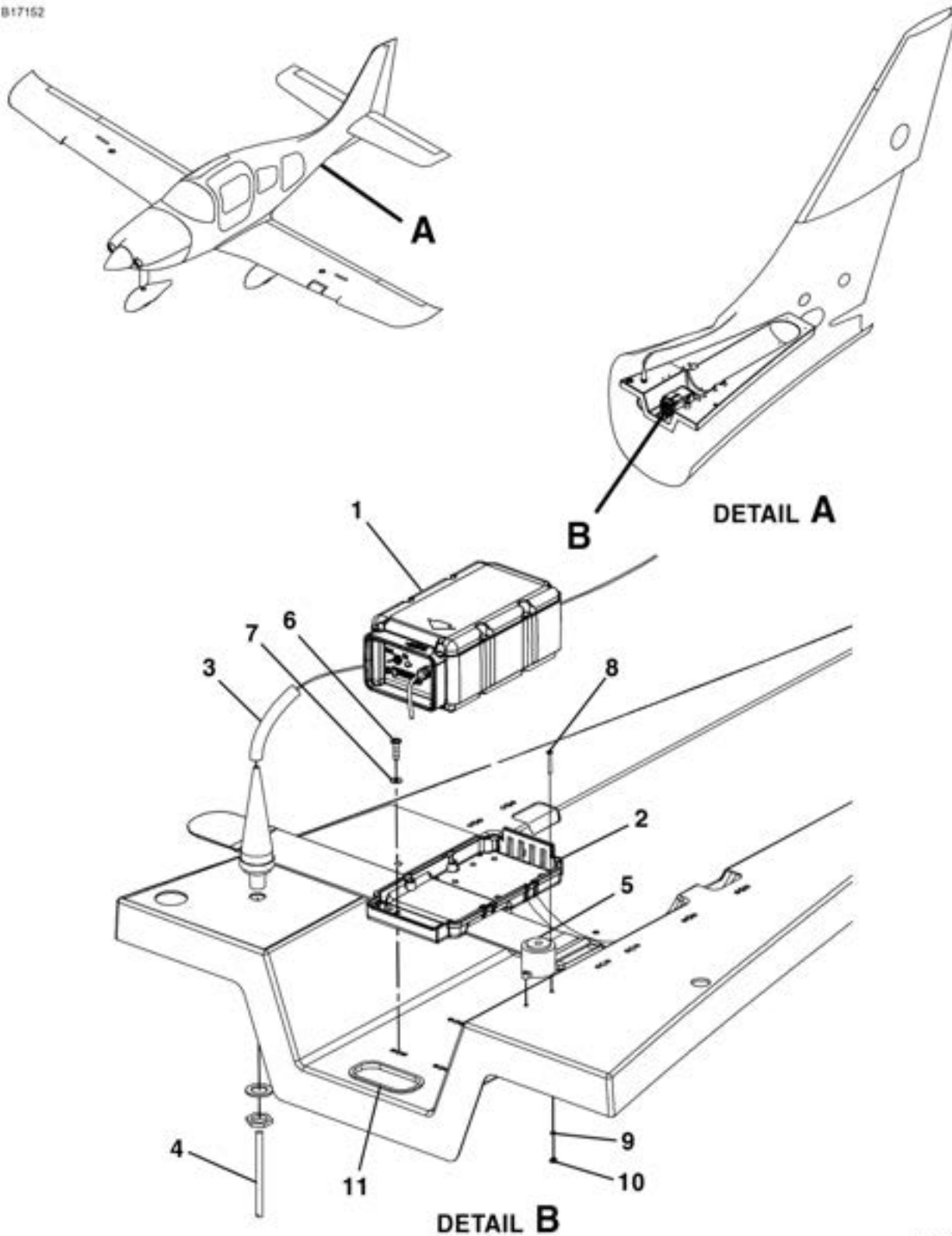
EMERGENCY LOCATOR TRANSMITTER SYSTEM FIGURE 20 (SHEET 1)
