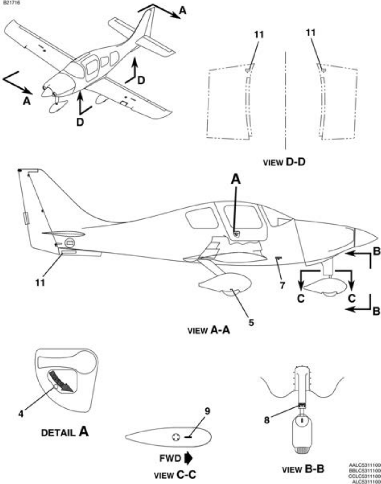
EXTERIOR PLACARDS AND MARKINGS - FUSELAGE - ARGENTINA FIGURE 02C (SHEET 2)
