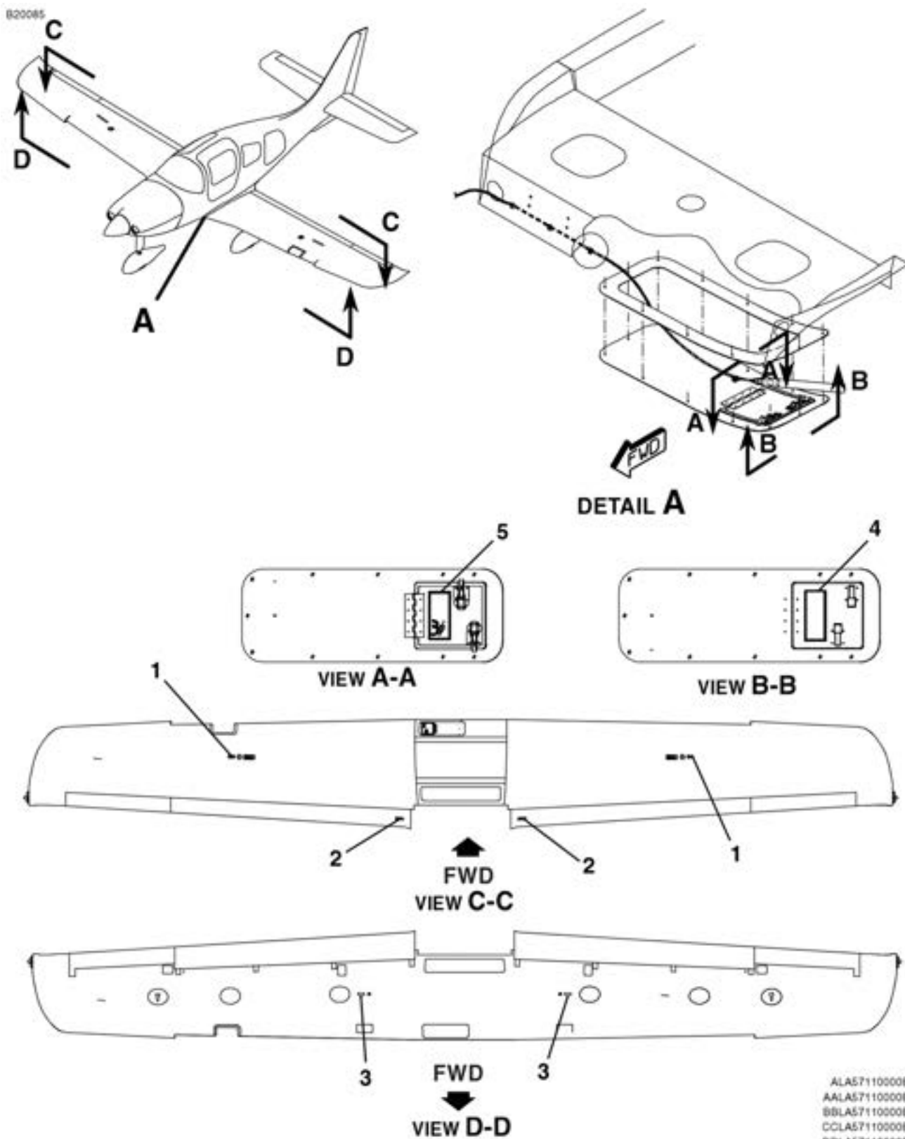
EXTERIOR PLACARDS AND MARKINGS - WING - BRAZIL FIGURE 03A (SHEET 1)
