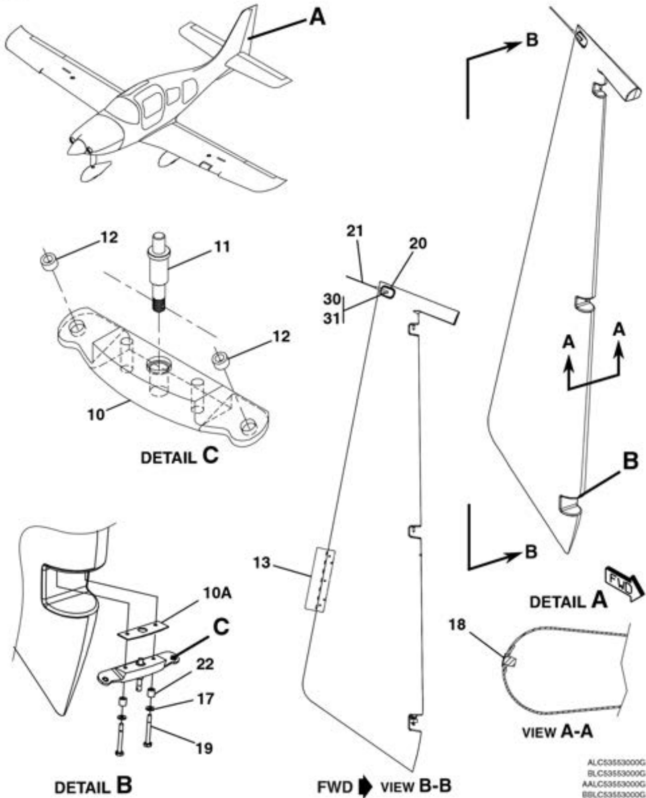
RUDDER ASSEMBLY FIGURE 12 (SHEET 2)
