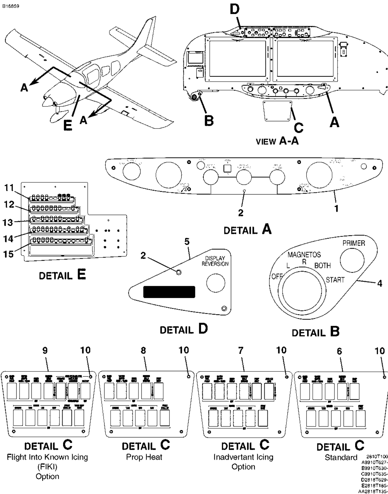
INTERIOR LIGHTING - LIGHT EMITTING DIODE (LED) PANELS FIGURE 02 (SHEET 1)
