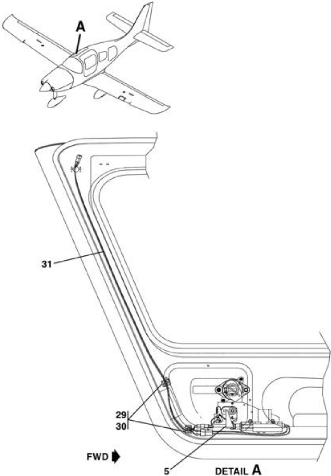
CABIN DOOR ASSEMBLY FIGURE 02 (SHEET 2)
