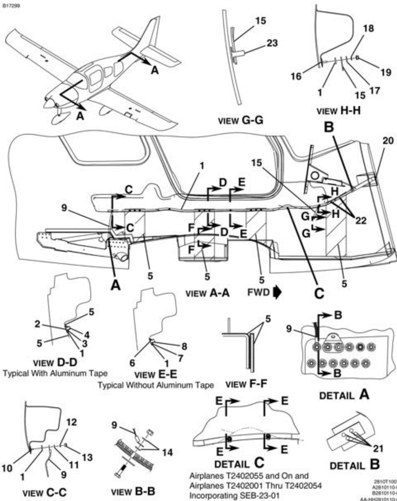
LIGHTNING PROTECTION ASSEMBLY FIGURE 01 (SHEET 1)
