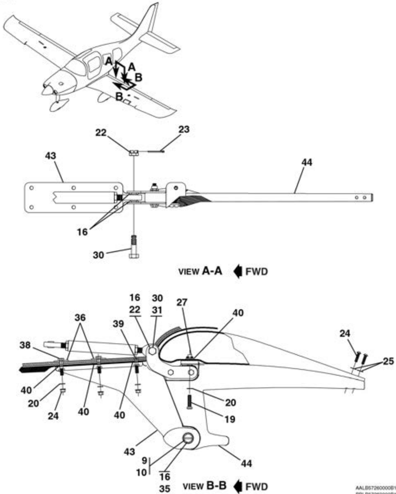
FLAP ASSEMBLY FIGURE 18 (SHEET 5)
