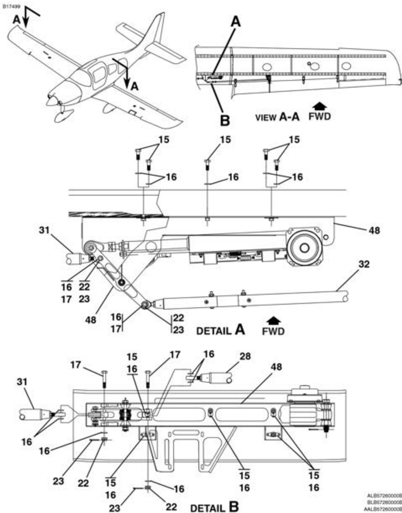
FLAP ASSEMBLY FIGURE 18 (SHEET 2)
