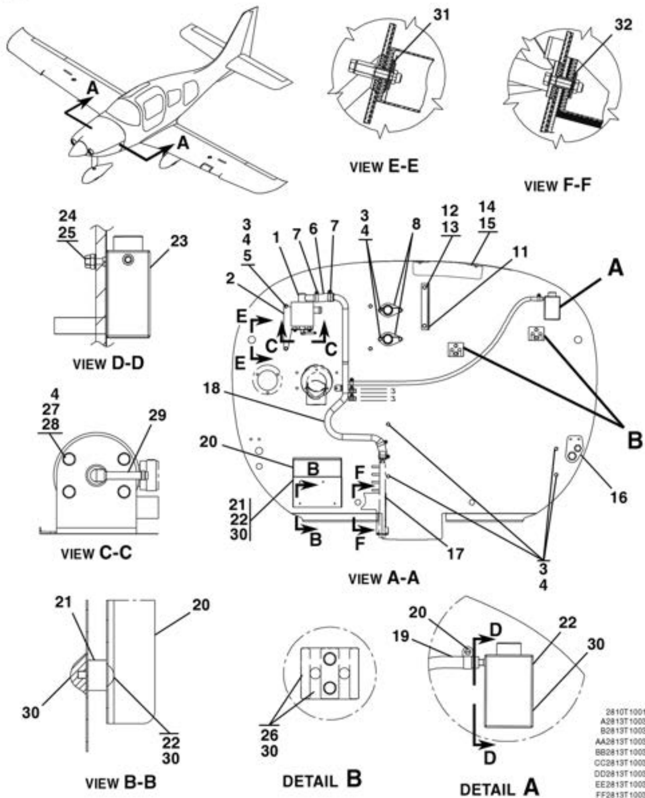
FIREWALL ASSEMBLY FIGURE 11 (SHEET 1)
