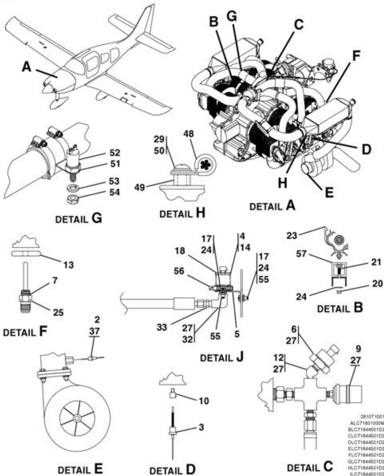
WIRING AND SENSORS ASSEMBLY FIGURE 02 (SHEET 2)
