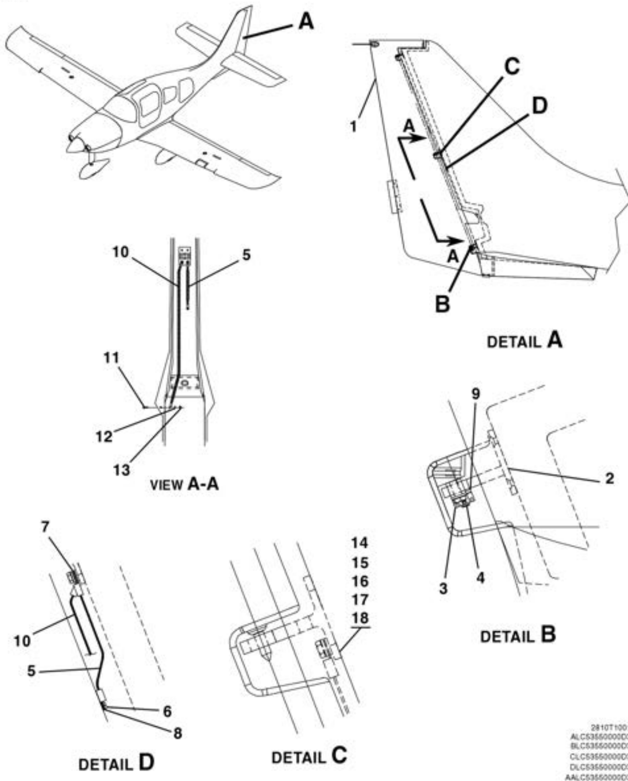
RUDDER INSTALLATION FIGURE 10 (SHEET 1)
