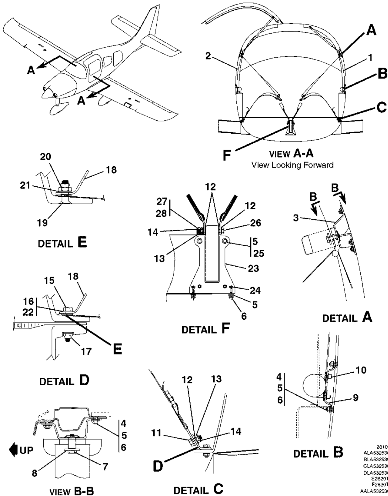
SEAT BELT INSTALLATION - FRONT FIGURE 02 (SHEET 1)
