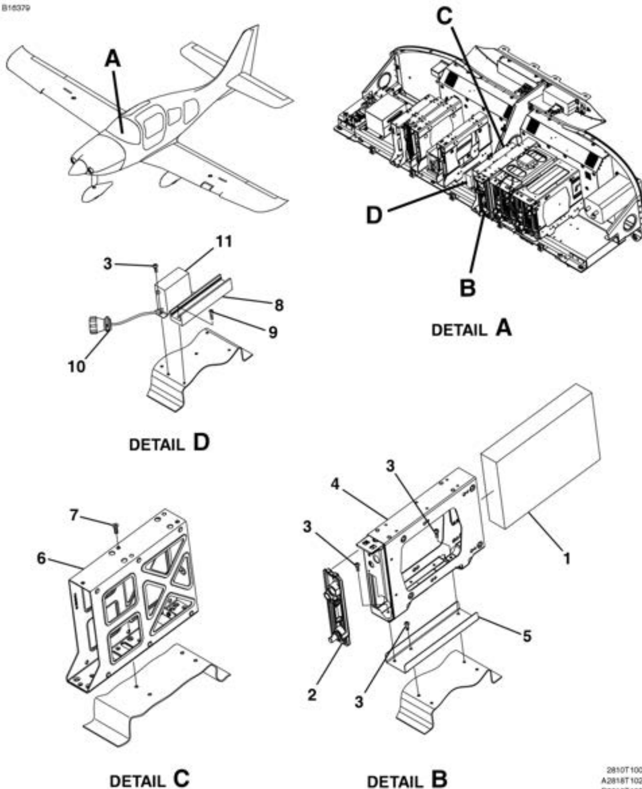
AVIONICS AND NAVIGATION EQUIPMENT - GTX 33D, CHIPS MODULE, & PROP HEAT TIMER INSTALLATION FIGURE 05 (SHEET 1)
