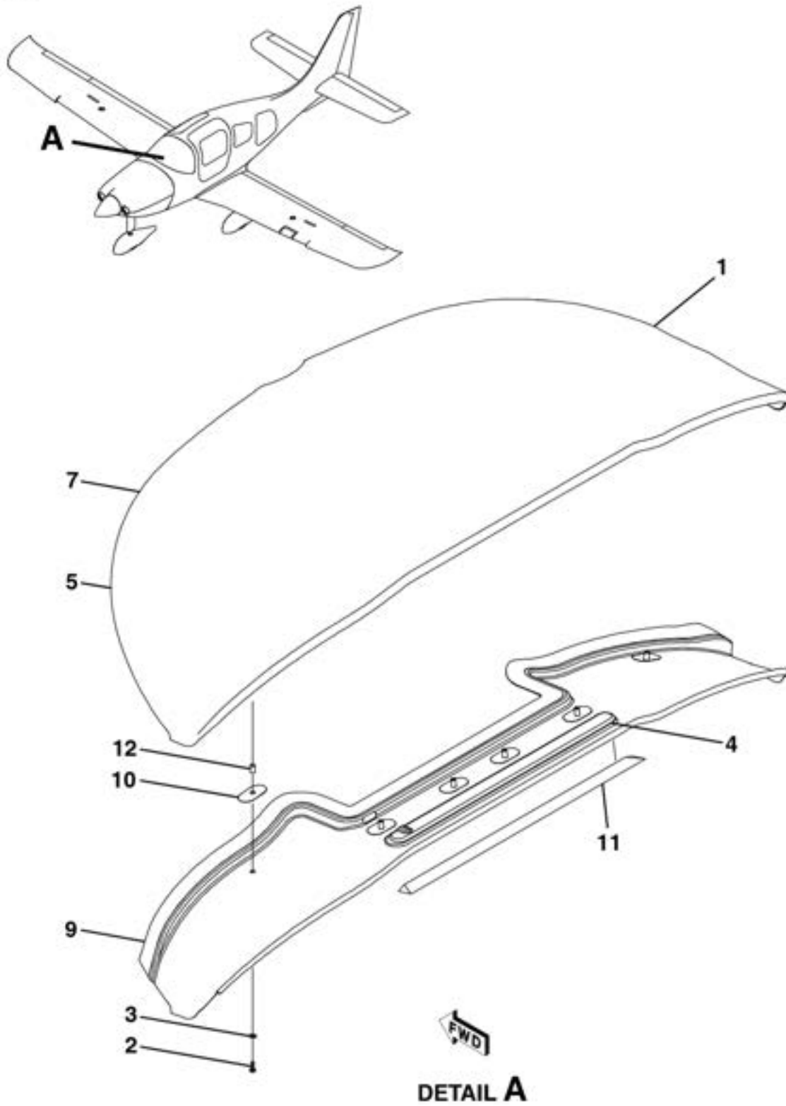
GLARESHIELD ASSEMBLY FIGURE 12 (SHEET 1)
