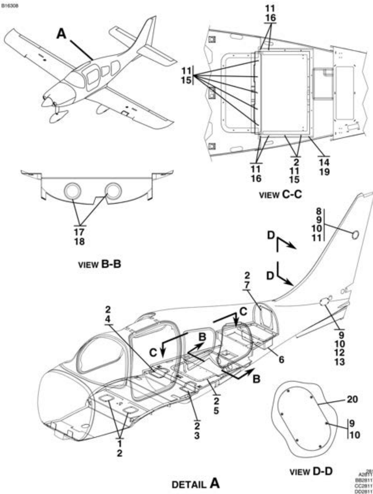
FUSELAGE ACCESS PANELS FIGURE 02 (SHEET 1)
