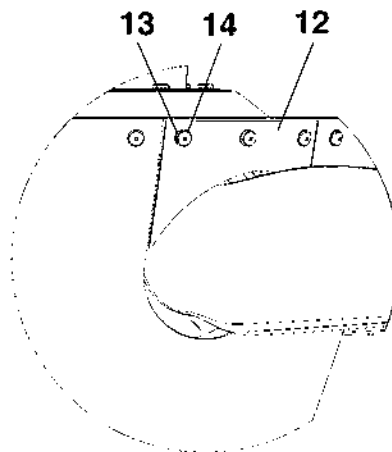
PROPELLER ASSEMBLY - TKS SYSTEM FIGURE 01B (SHEET 1)
