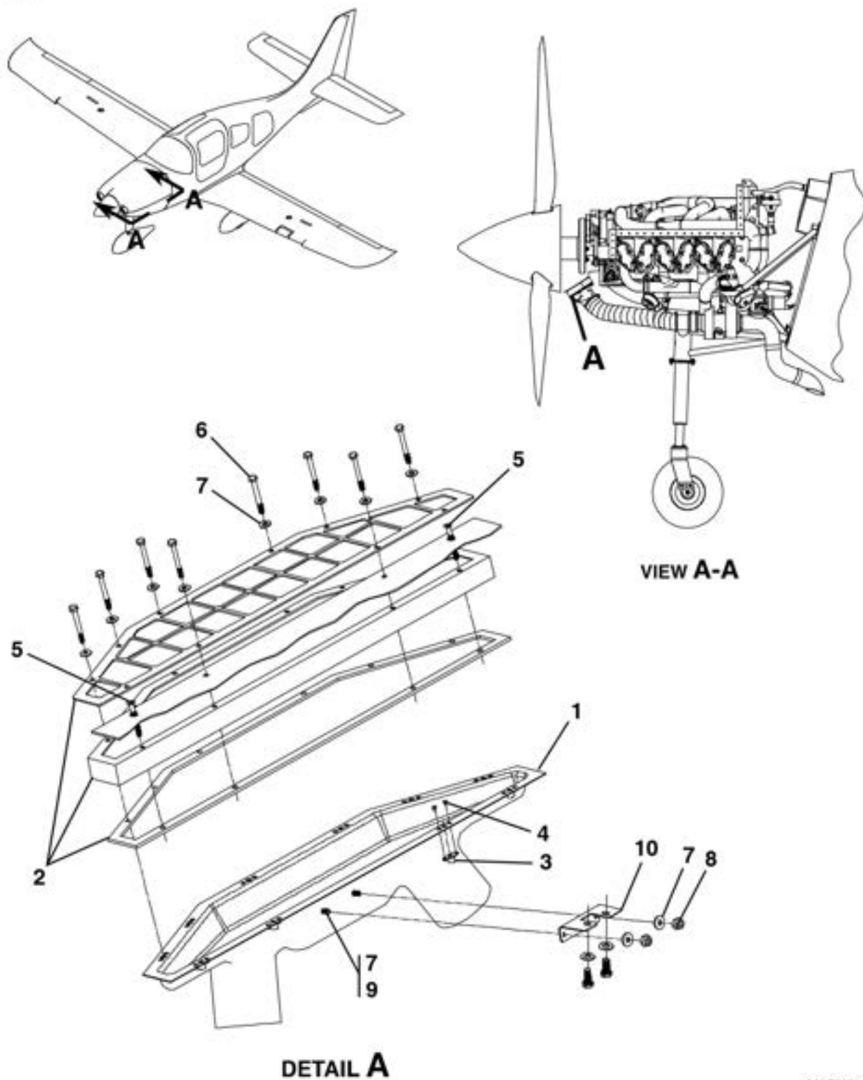
AIR FILTER ASSEMBLY FIGURE 08 (SHEET 1)
