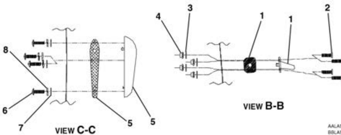
WING ANTENNAS INSTALLATION FIGURE 03 (SHEET 1)
