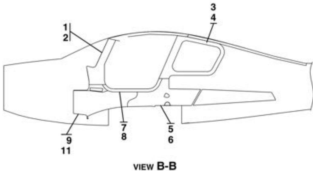
INTERIOR PANELS INSTALLATION - FOWARD AND MID CABIN FIGURE 07 (SHEET 1)
