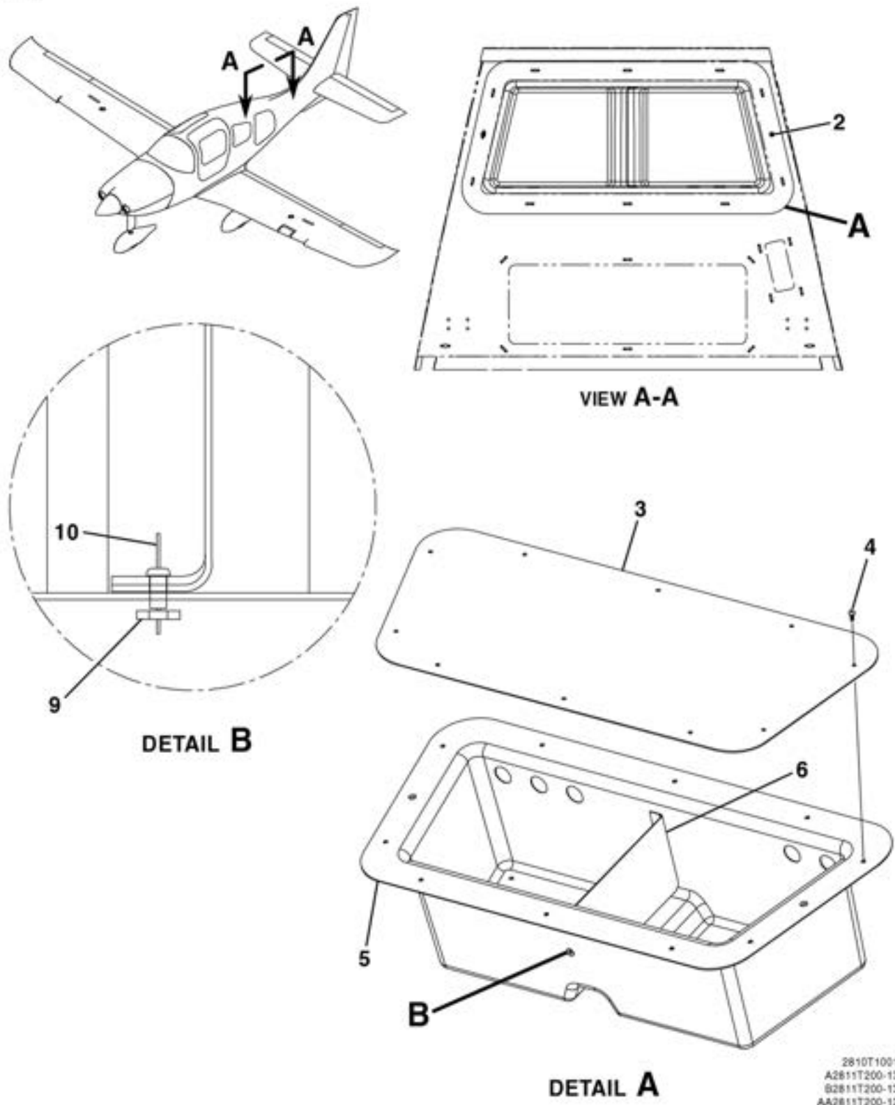
BATTERY BOX FIGURE 10 (SHEET 1)
