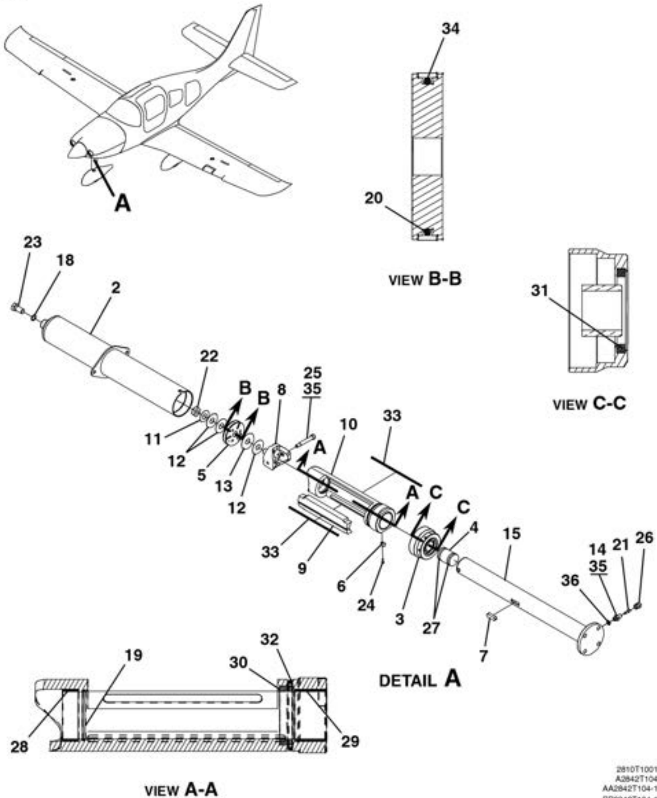
STRUT ASSEMBLY FIGURE 09 (SHEET 1)
