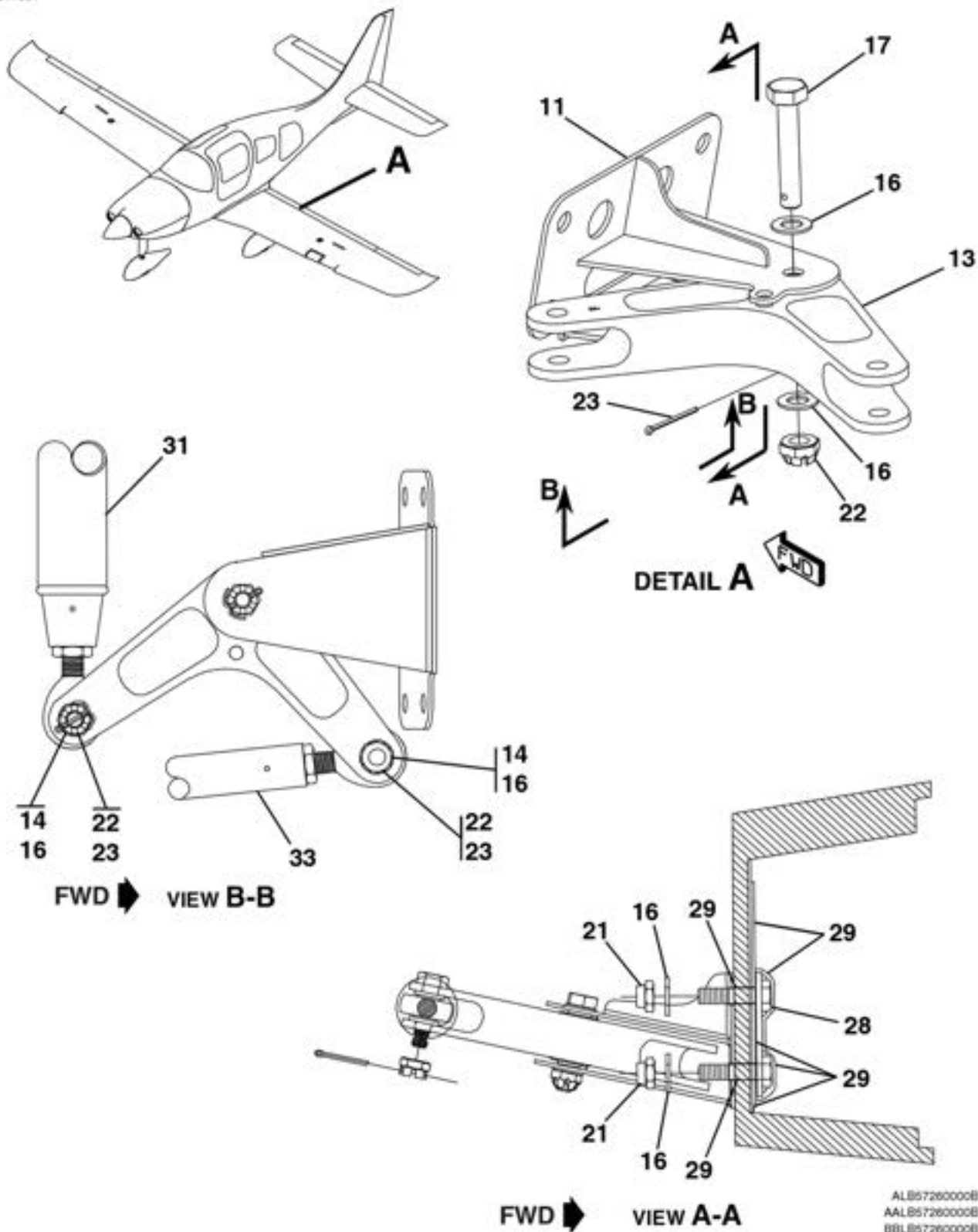
FLAP ASSEMBLY FIGURE 18 (SHEET 4)
