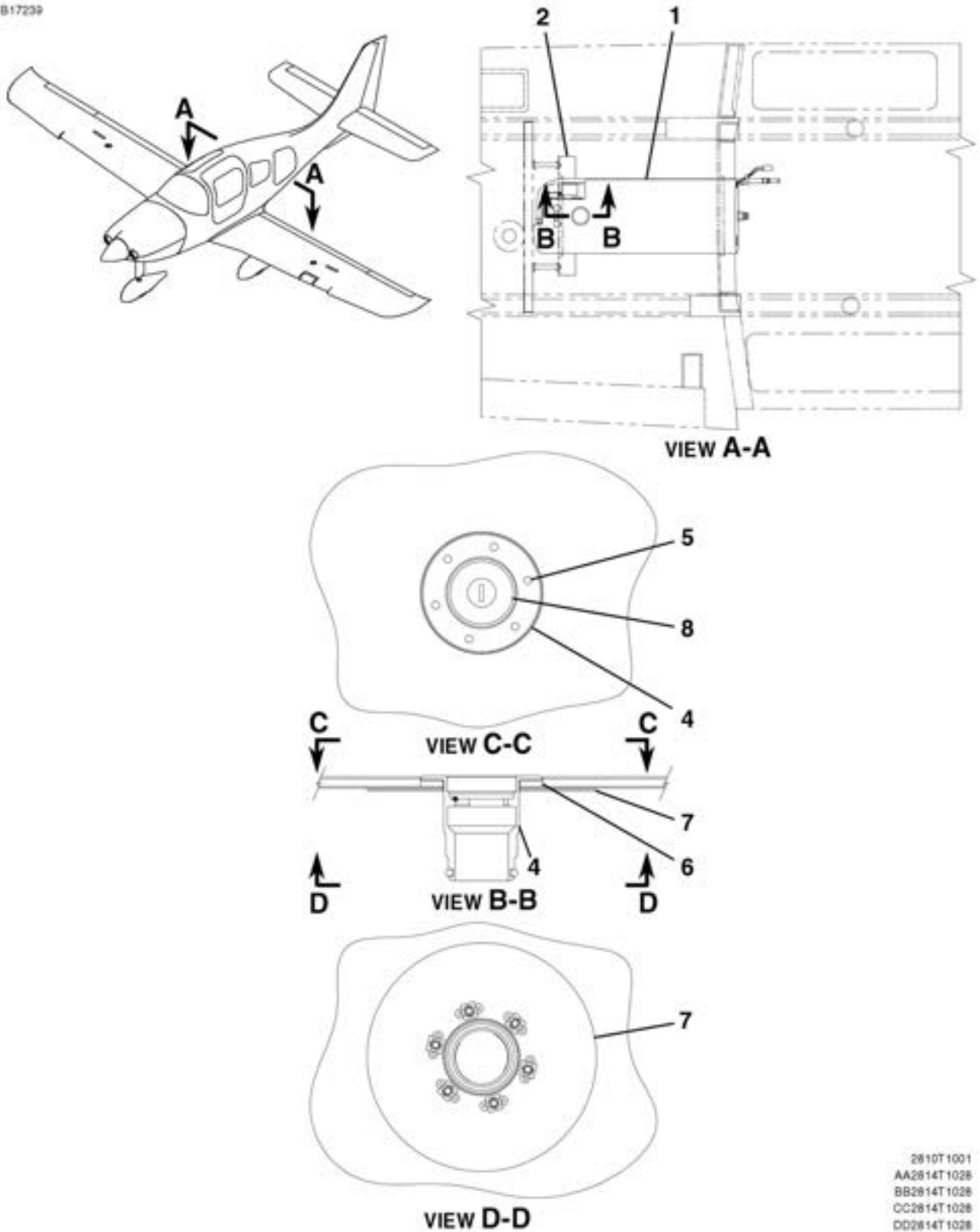
INADVERTANT ICING SYSTEM - FLUID TANK, RIB, AND FILLER INSTALLATION FIGURE 03 (SHEET 1)
