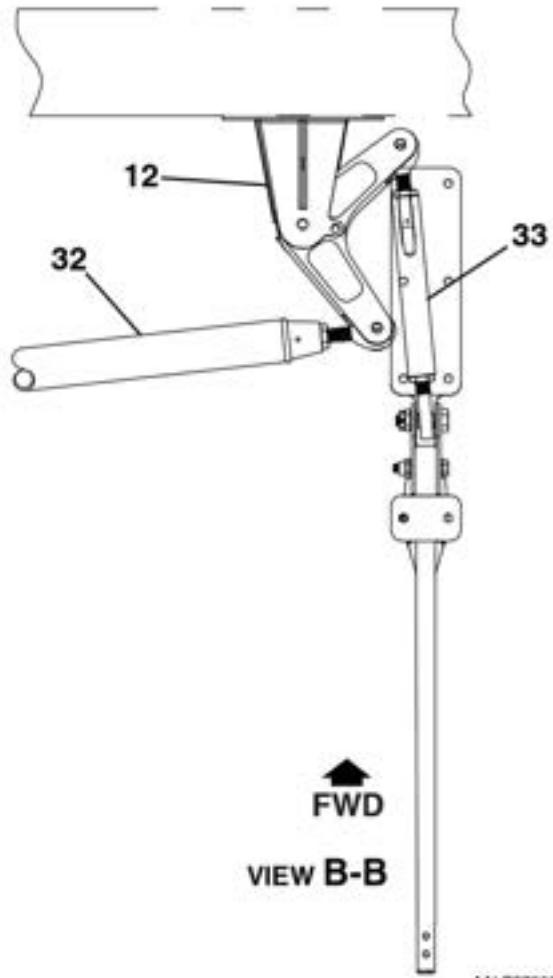
FLAP ASSEMBLY FIGURE 18 (SHEET 3)
