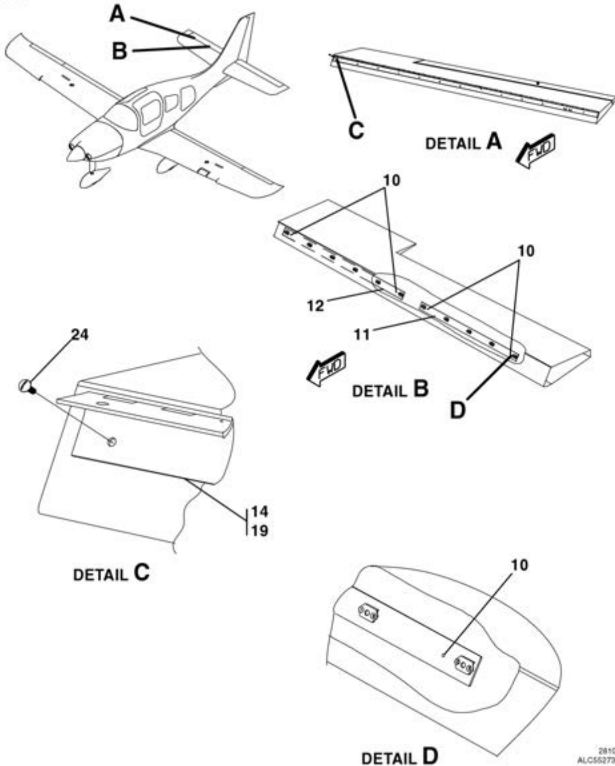
ELEVATOR ASSEMBLY FIGURE 04 (SHEET 3)
