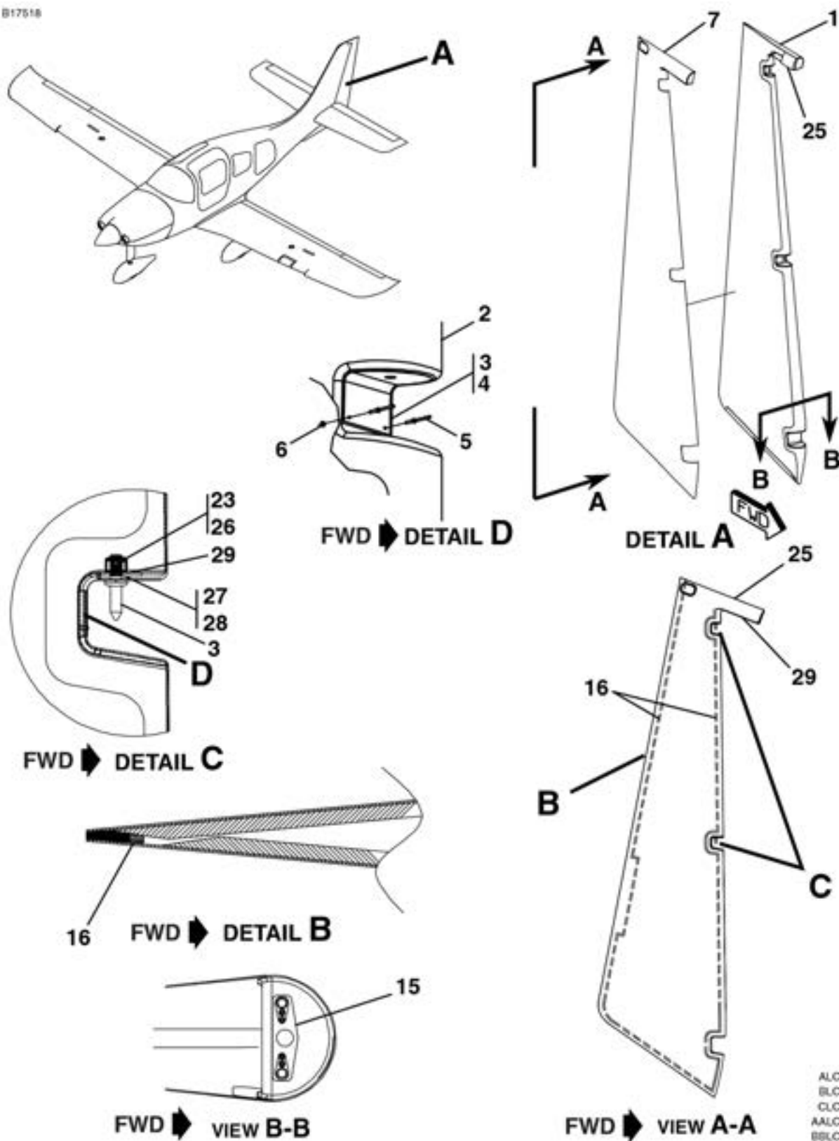
RUDDER ASSEMBLY FIGURE 12 (SHEET 1)
