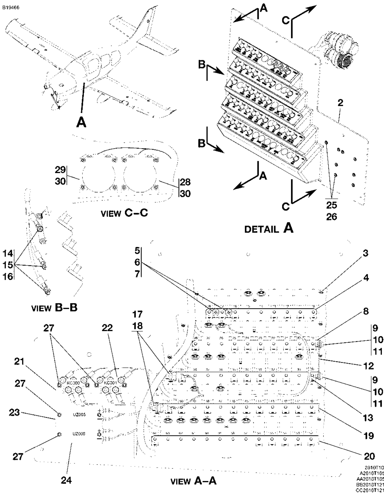
CIRCUIT BREAKER PANEL ASSEMBLY FIGURE 04A (SHEET 1)
