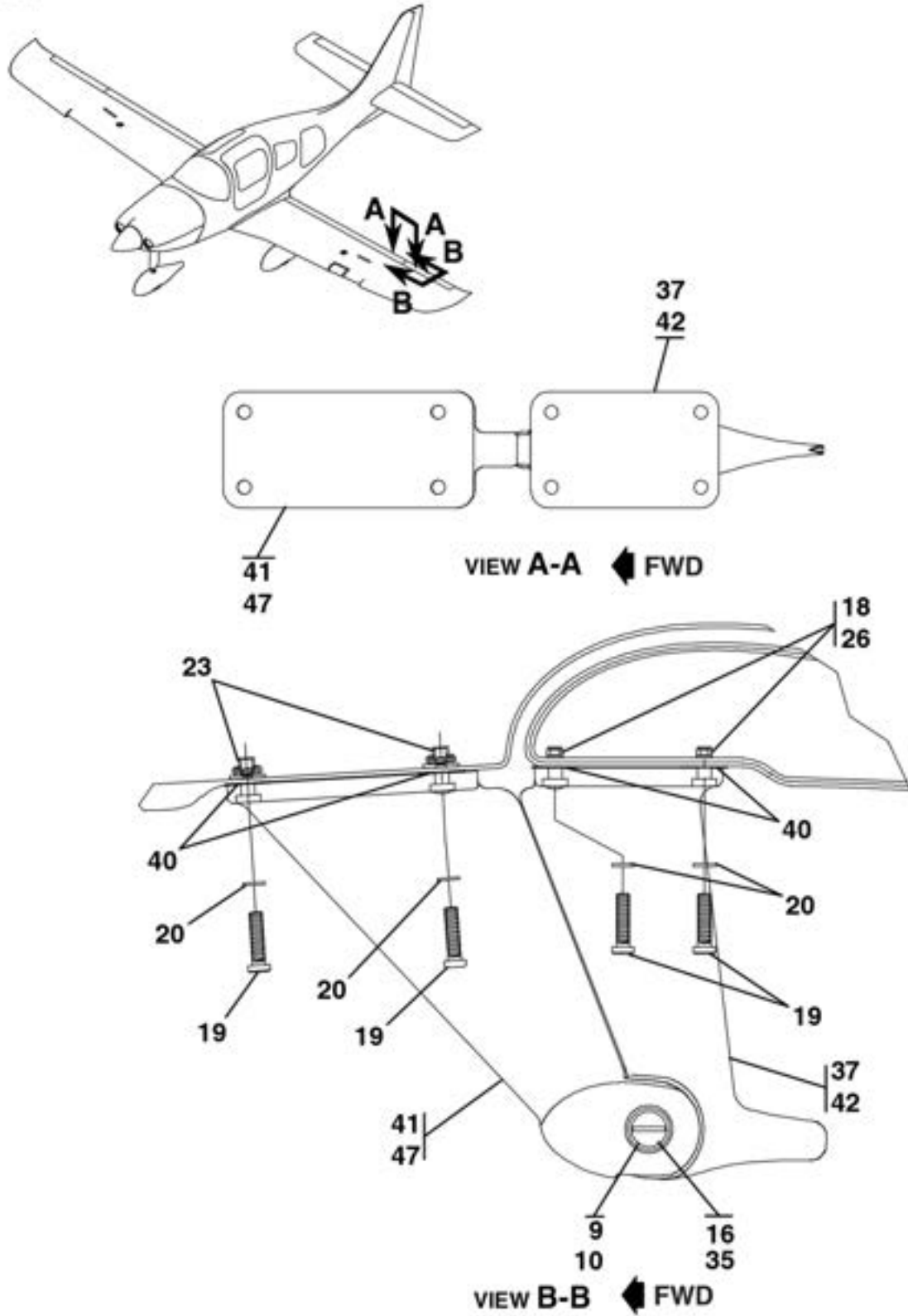
FLAP ASSEMBLY FIGURE 18 (SHEET 7)
