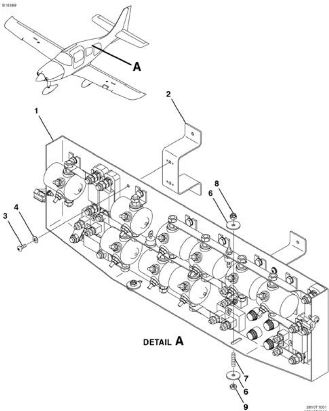
POWER RELAY PANEL INSTALLATION FIGURE 01 (SHEET 1)
