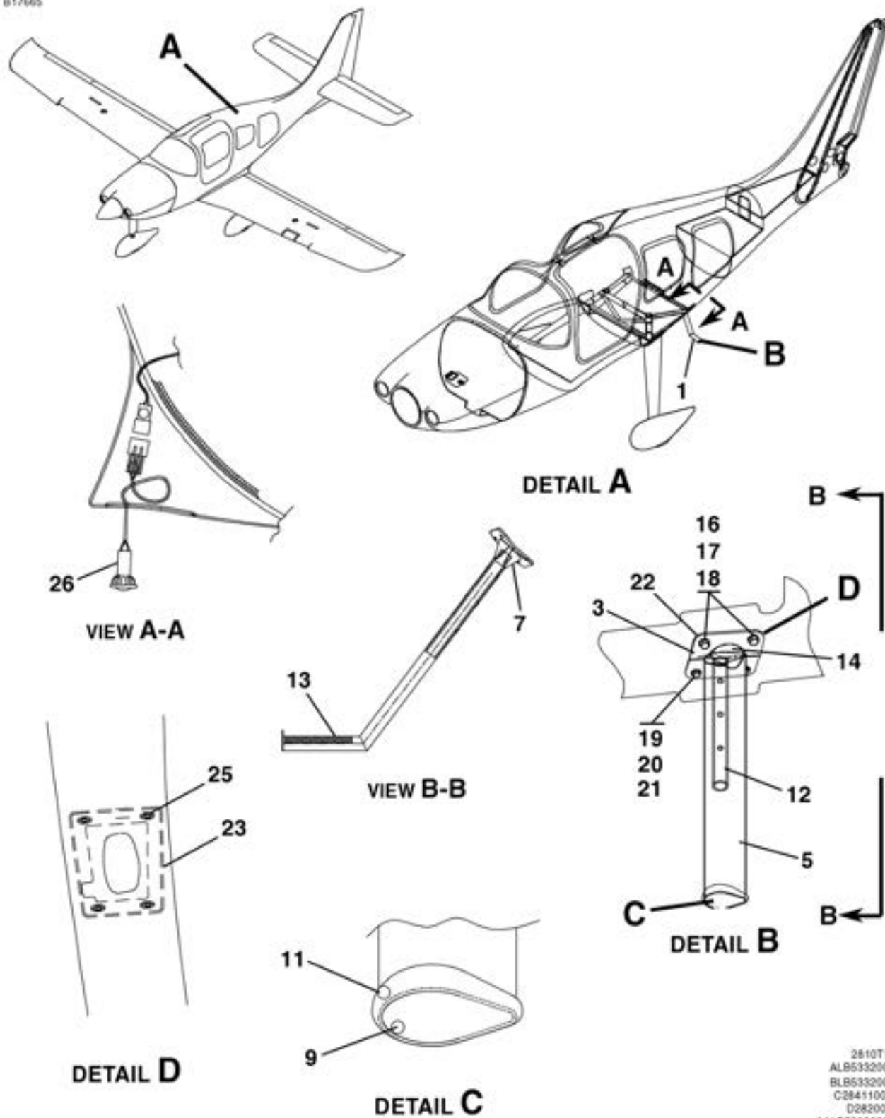
CABIN STEP AND LIGHT ASSEMBLY FIGURE 11 (SHEET 1)
