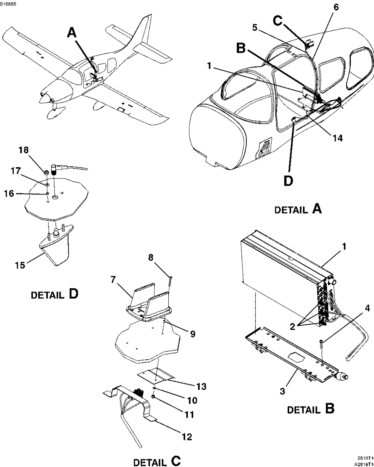
TRAFFIC ADVISORY SYSTEM FIGURE 13 (SHEET 1)
