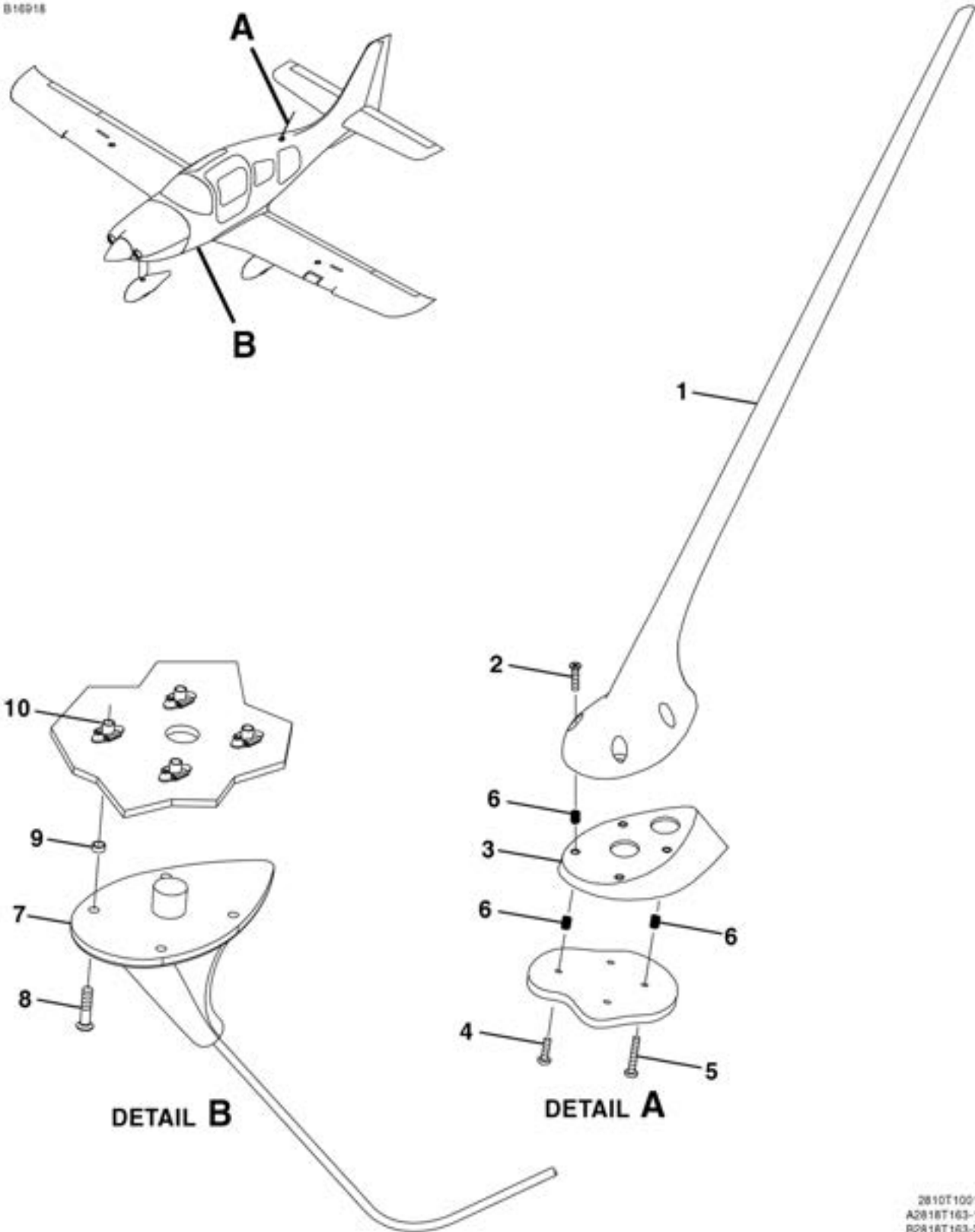
ANTENNA INSTALLATION - COM AND GPS FIGURE 02 (SHEET 1)
