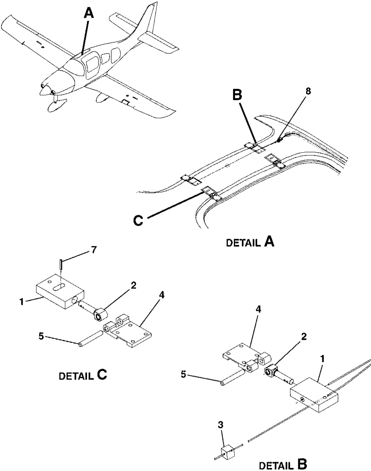
CABIN AND BAGGAGE DOOR INSTALLATION FIGURE 01 (SHEET 1)
