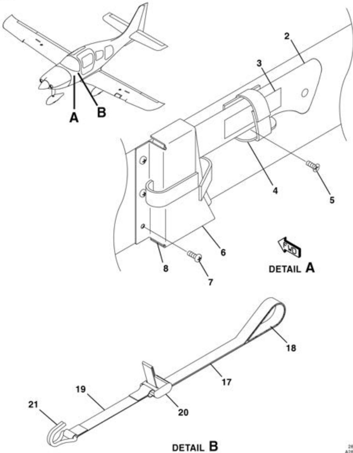
CABIN AND MISCELLANEOUS EQUIPMENT FIGURE 22 (SHEET 1)
