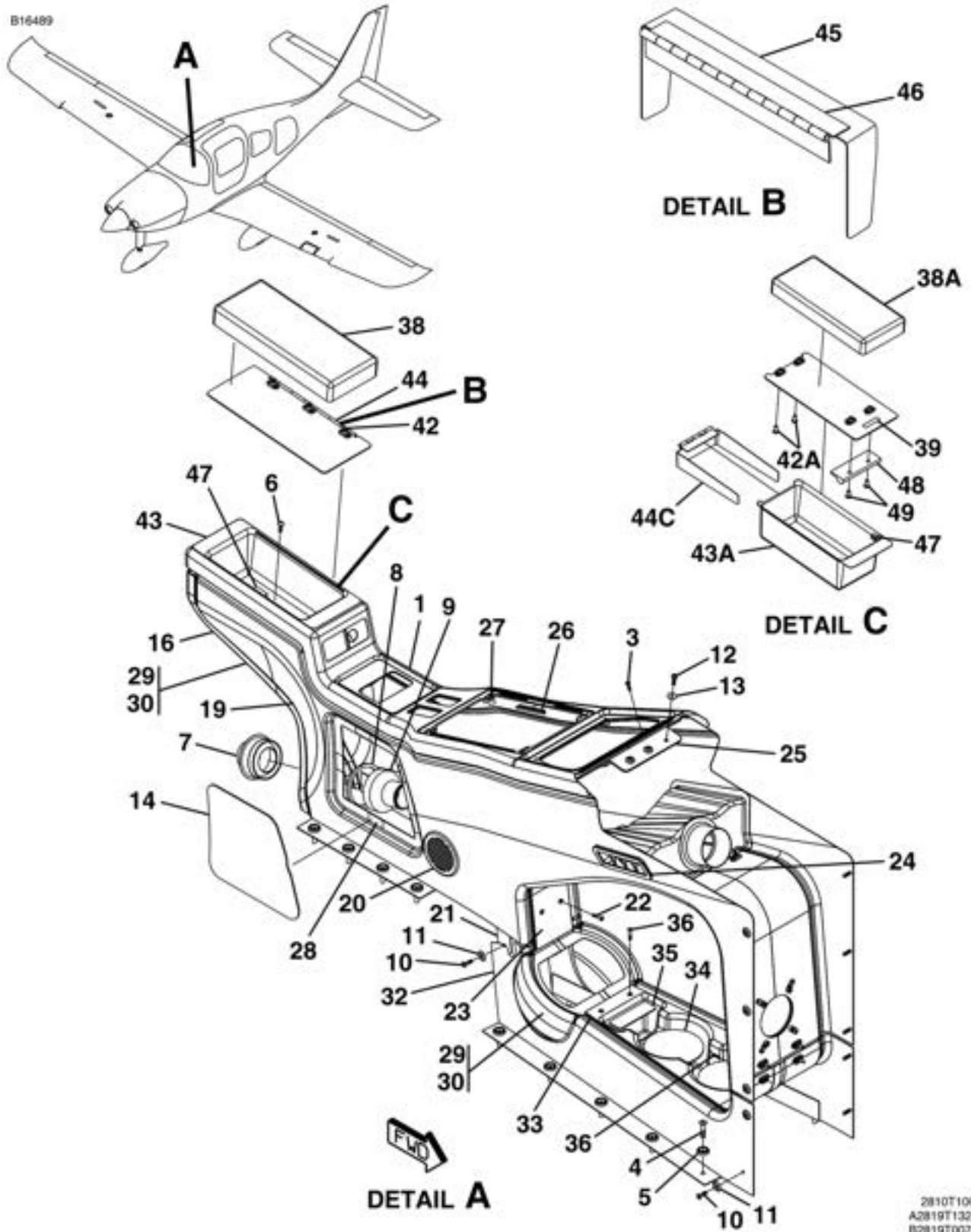
CENTER CONSOLE FIGURE 08 (SHEET 1)
