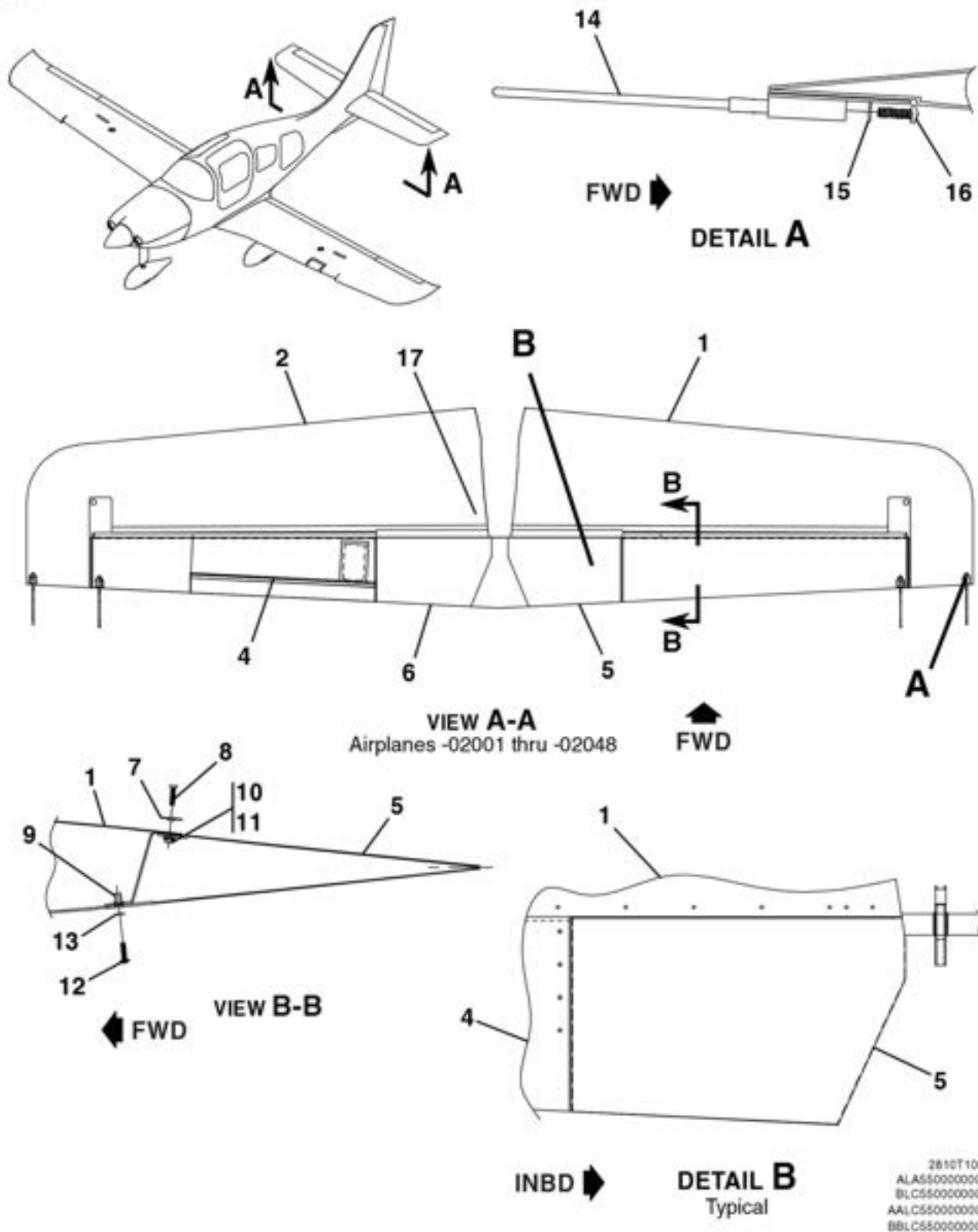
HORIZONTAL STABILIZER ASSEMBLY FIGURE 02 (SHEET 1)
