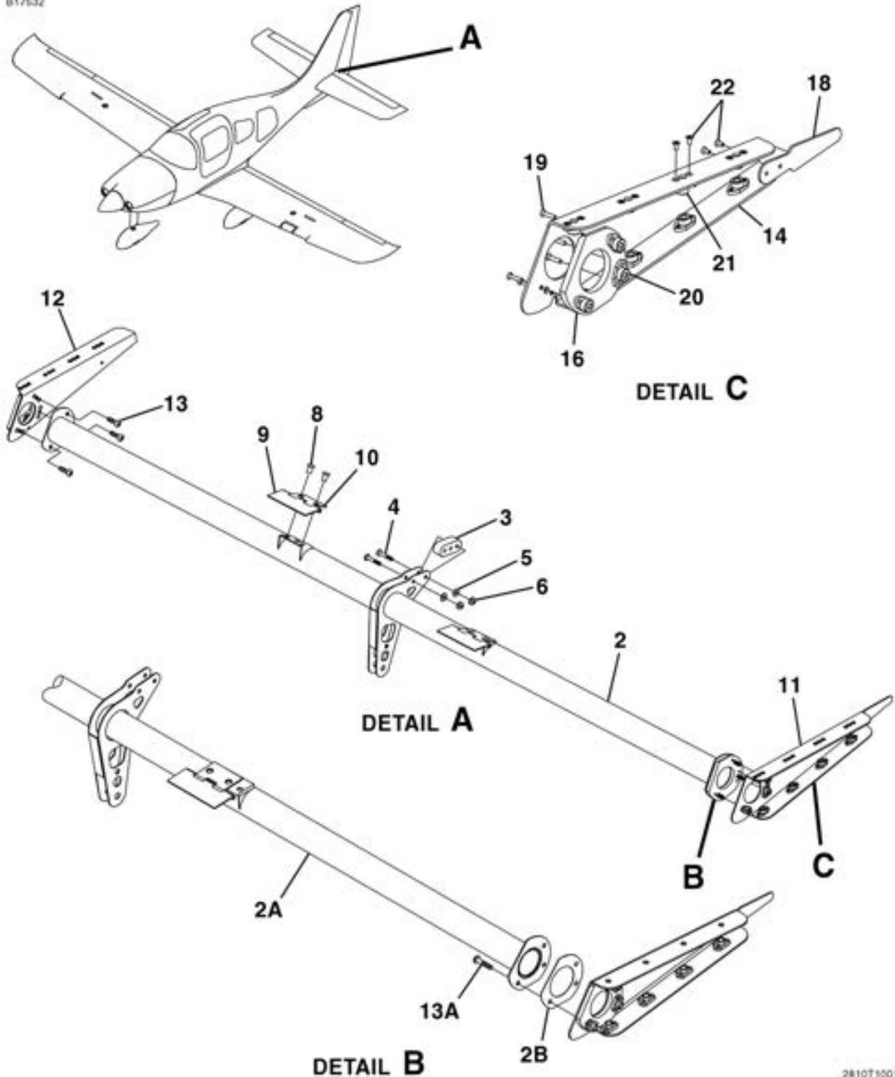
ELEVATOR TORQUE TUBE ASSEMBLY FIGURE 09 (SHEET 1)
