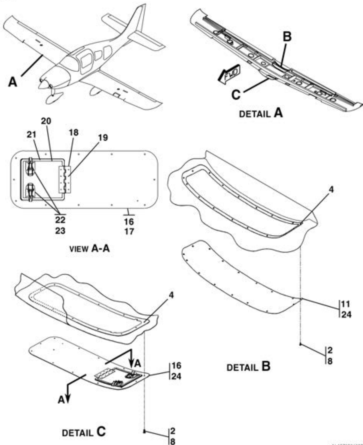
WING ACCESS PANEL ASSEMBLY FIGURE 03 (SHEET 3)
