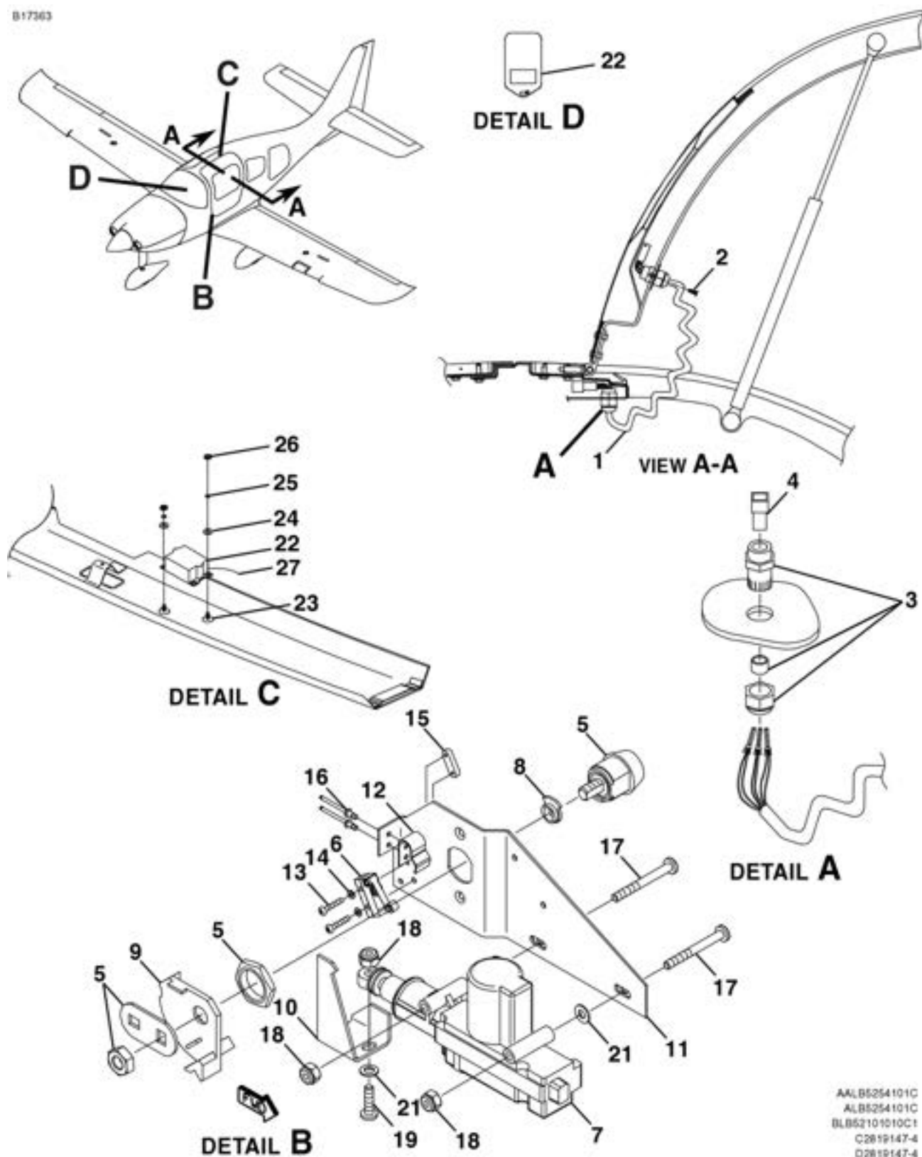
REMOTE KEYLESS ENTRY SYSTEM FIGURE 10 (SHEET 1)
