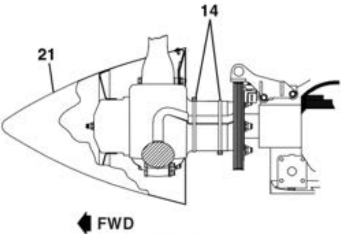
VIEW A-A SMR Heater Boot Lead Secure - Booted and Unbooted
