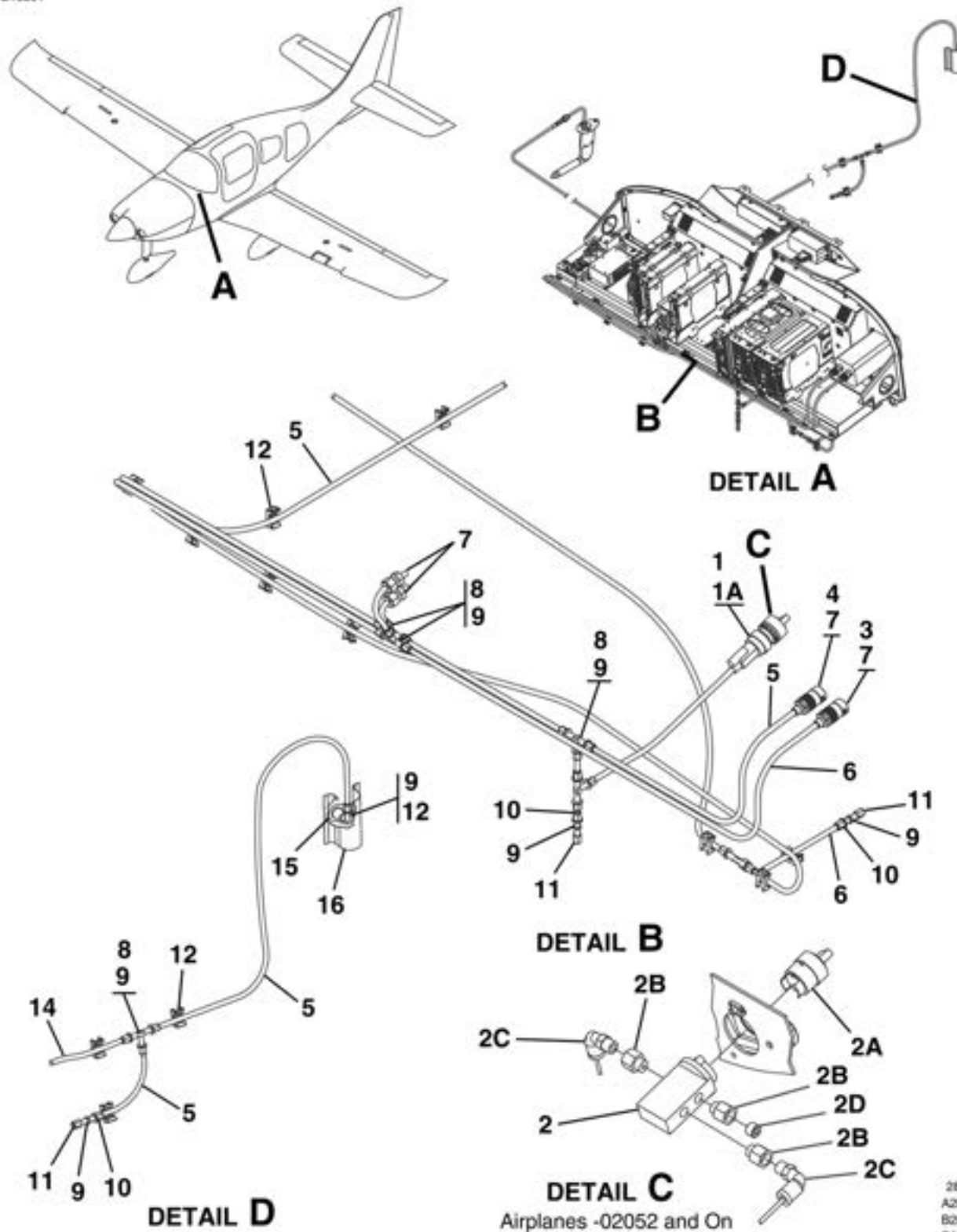
PITOT/STATIC INSTALLATION FIGURE 01 (SHEET 1)
