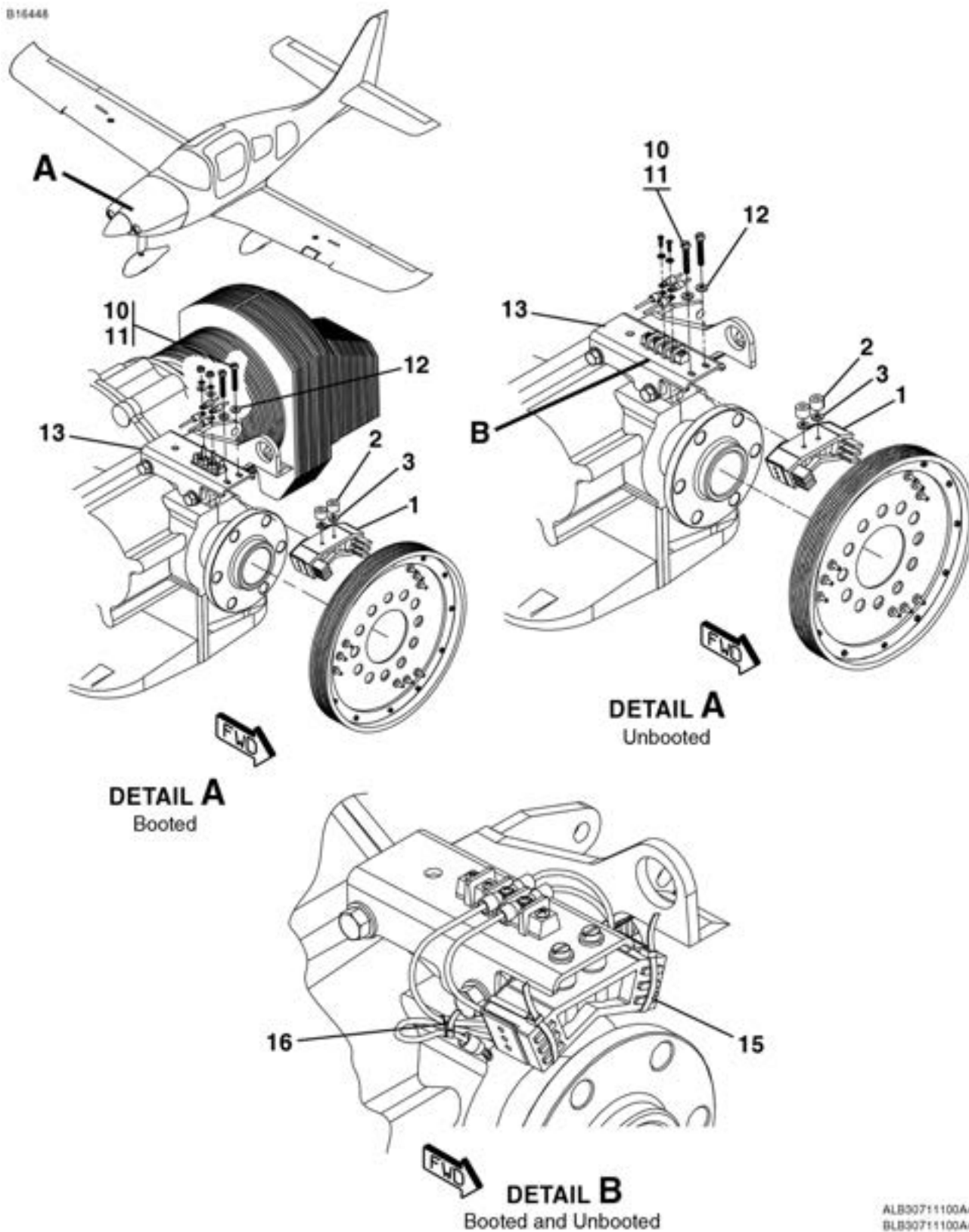
PROPELLER HEAT SYSTEM - BOOTED AND NON-BOOTED FIGURE 01 (SHEET 1)
