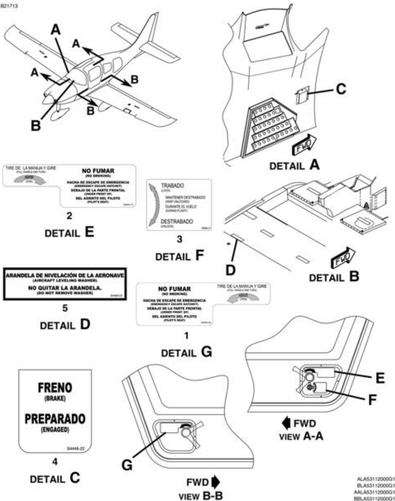
INTERIOR PLACARDS AND MARKINGS - FUSELAGE - ARGENTINA FIGURE 01C (SHEET 1)
