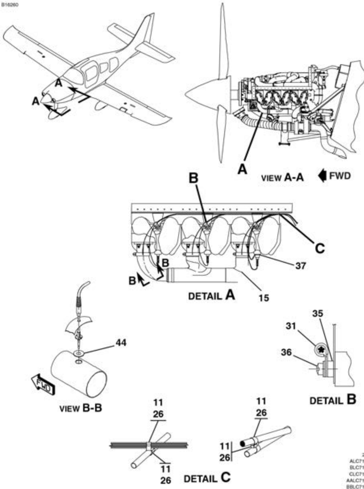
WIRING AND SENSORS ASSEMBLY FIGURE 02 (SHEET 3)
