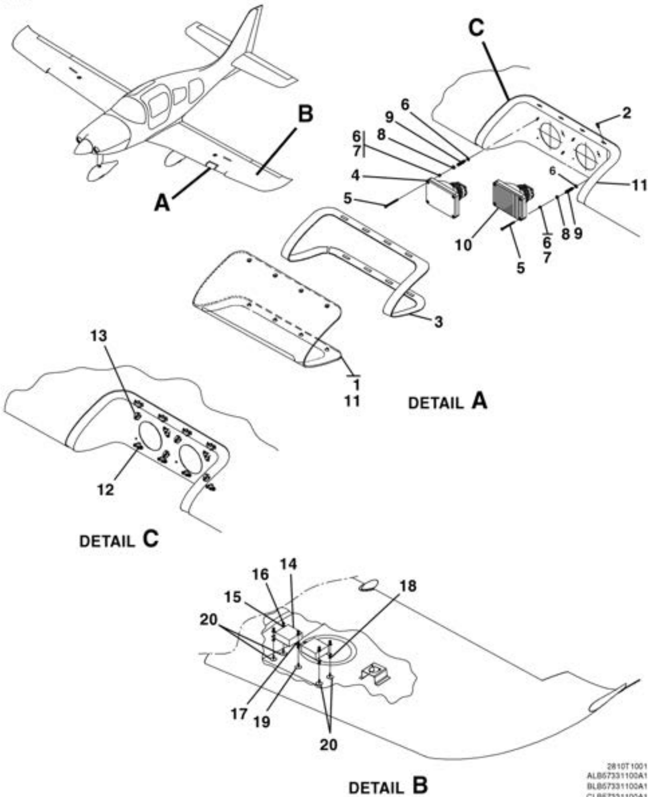
LANDING/TAXI LIGHT ASSEMBLY FIGURE 03 (SHEET 1)
