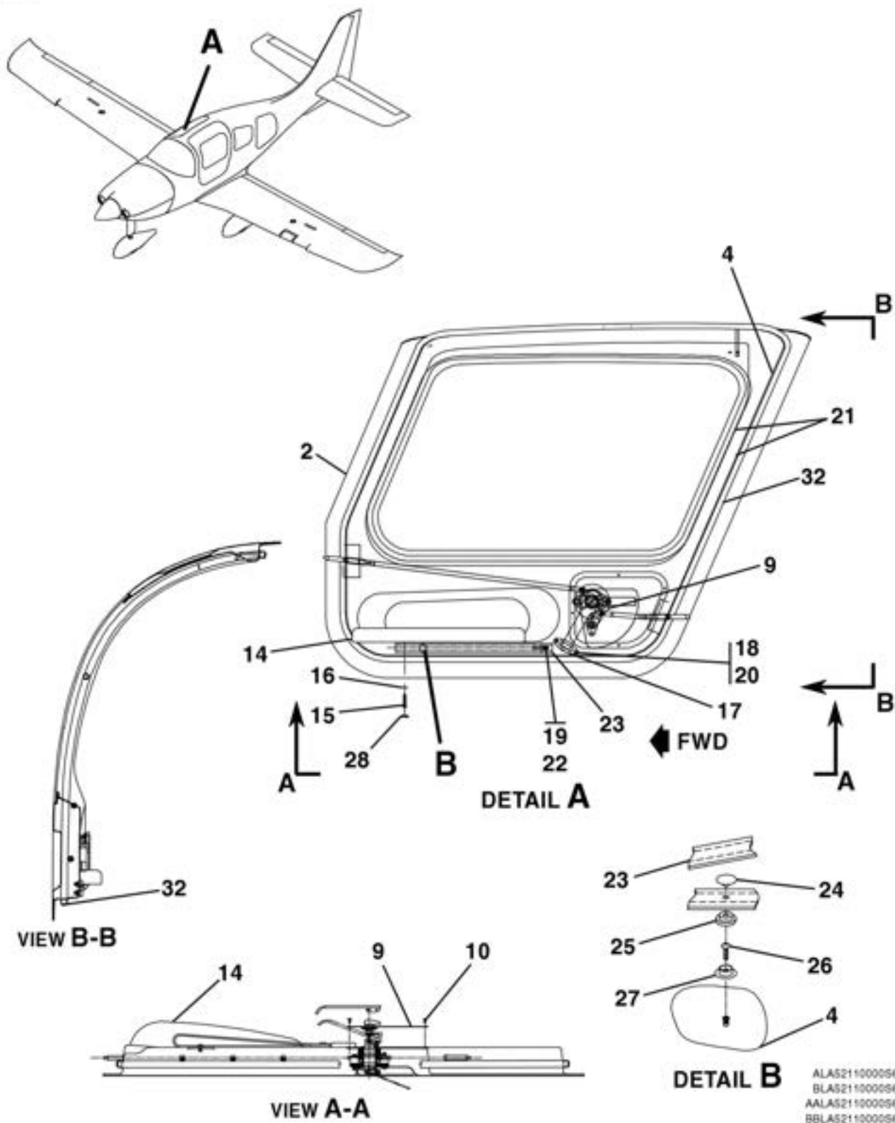
CABIN DOOR ASSEMBLY FIGURE 02 (SHEET 3)
