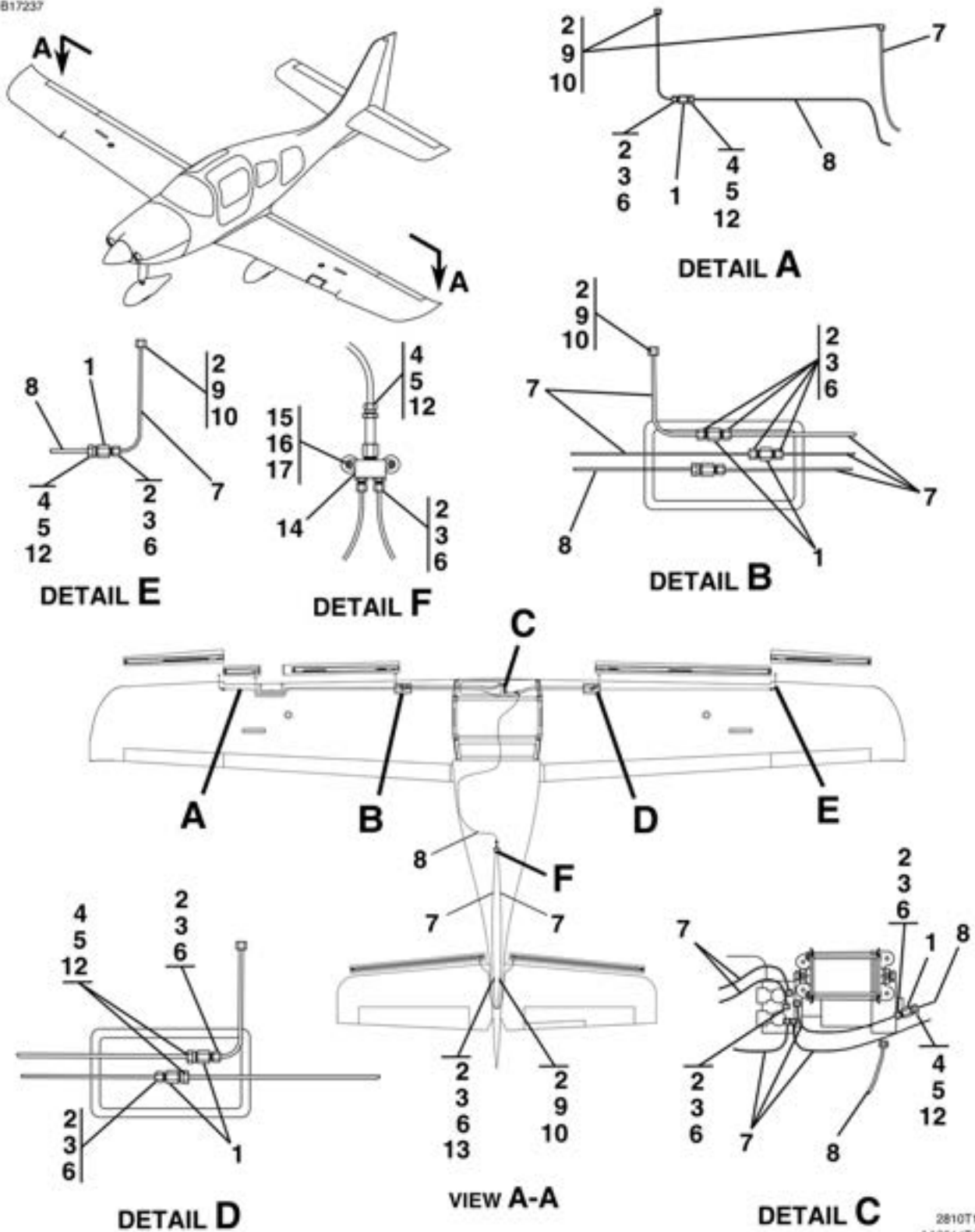
INADVERTANT ICING SYSTEM - WING RIB AND PLUMBING INSTALLATION FIGURE 05 (SHEET 1)
