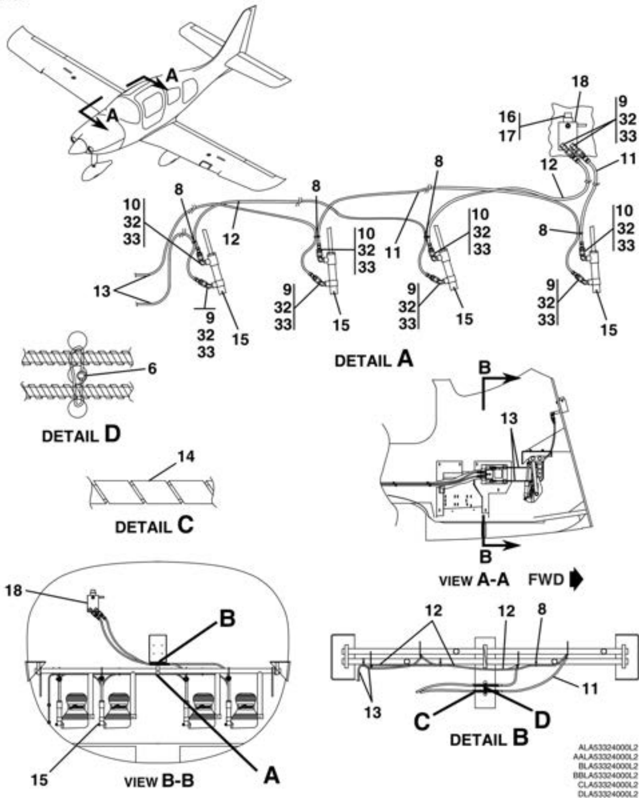
BRAKE SYSTEM ASSEMBLY FIGURE 05 (SHEET 3)
