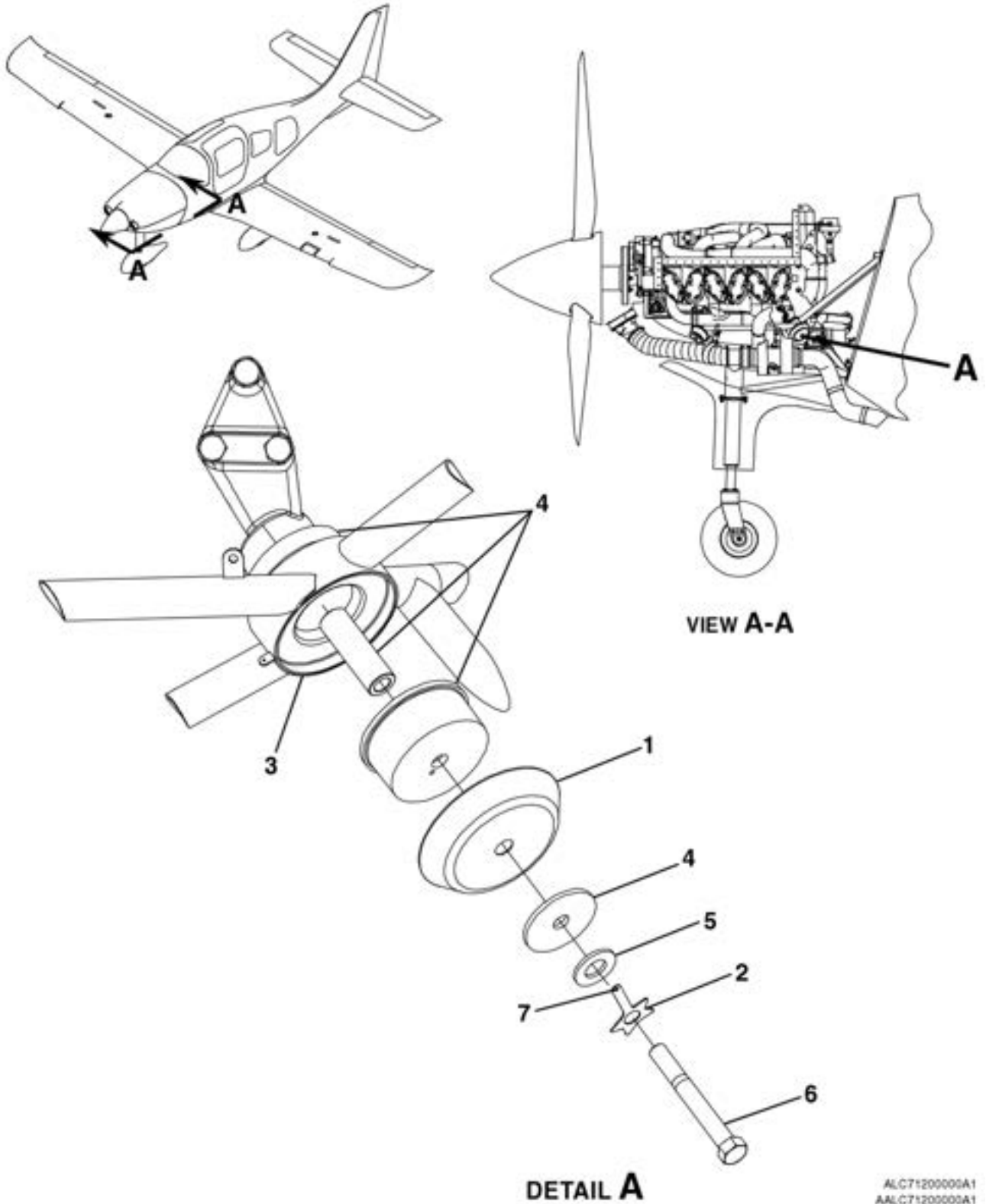
ISOLATOR ASSEMBLY FIGURE 04 (SHEET 1)
