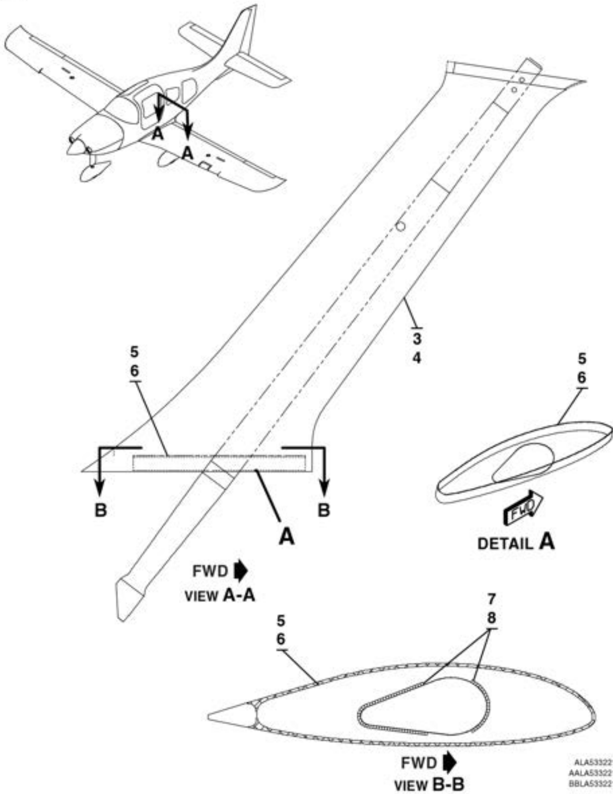
MAIN GEAR FAIRING ASSEMBLY FIGURE 04 (SHEET 1)
