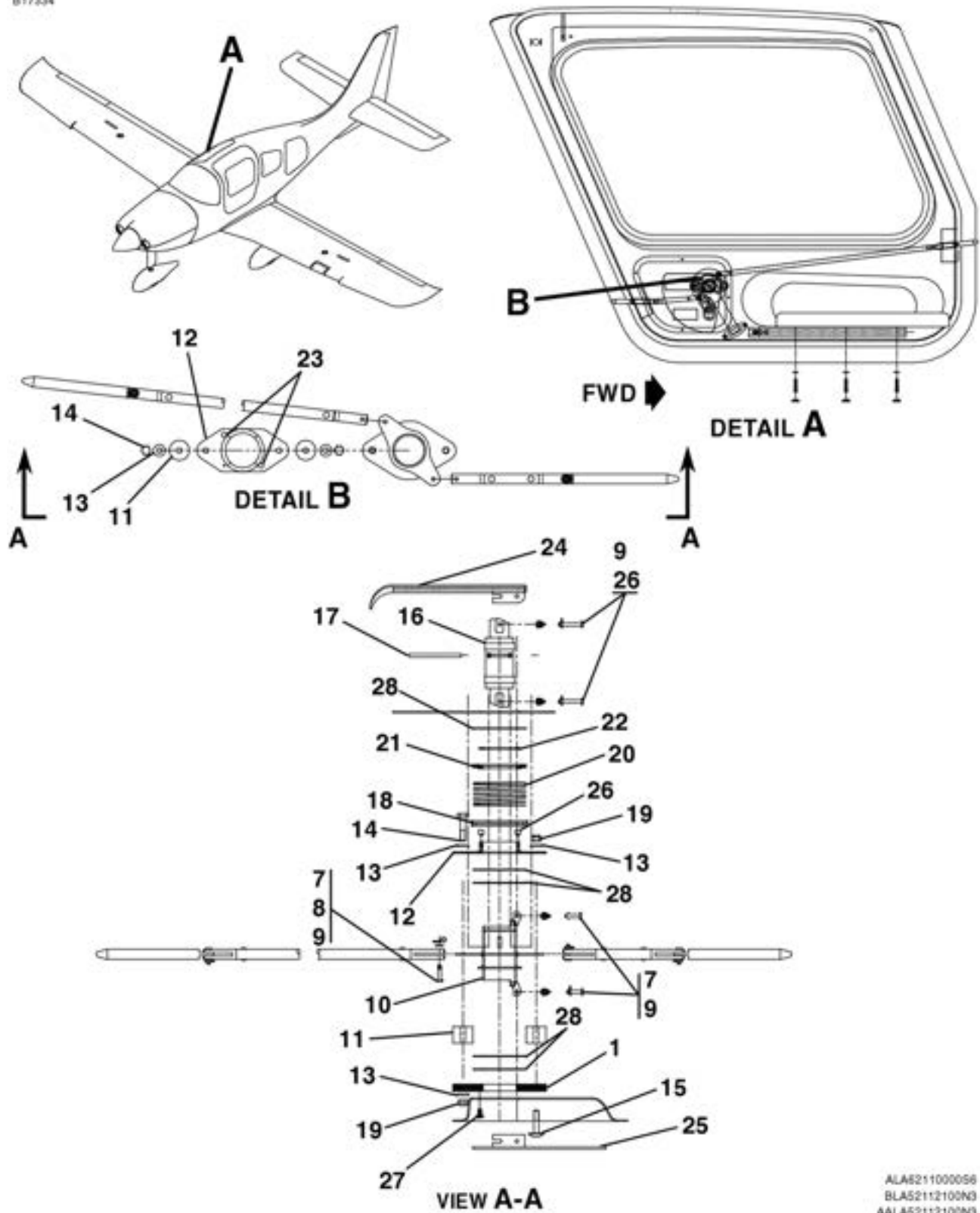
RIGHT CABIN DOOR LATCH ASSEMBLY FIGURE 05 (SHEET 1)
