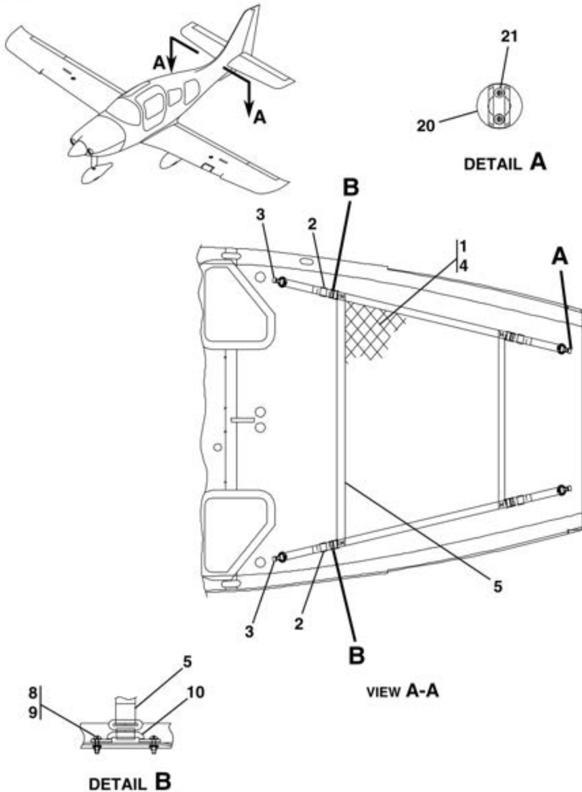
BAGGAGE NET INSTALLATION FIGURE 21 (SHEET 1)
