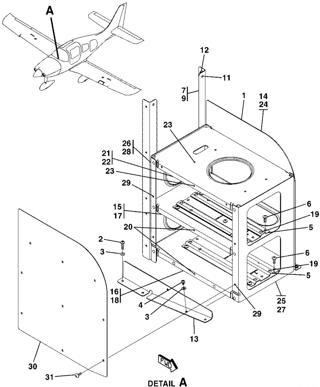
ATTITUDE HEADING REFERENCE SYSTEM (AHRS) STRUCTURE INSTALLATION FIGURE 07 (SHEET 1)
