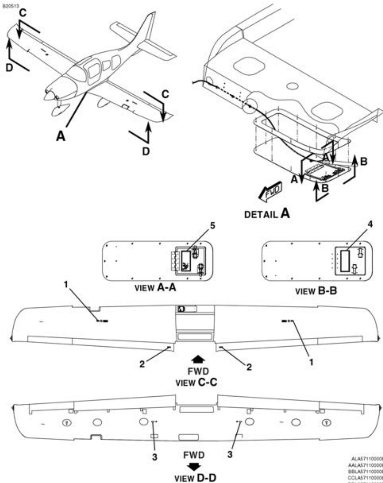
EXTERIOR PLACARDS AND MARKINGS - WING - MEXICO FIGURE 03B (SHEET 1)
