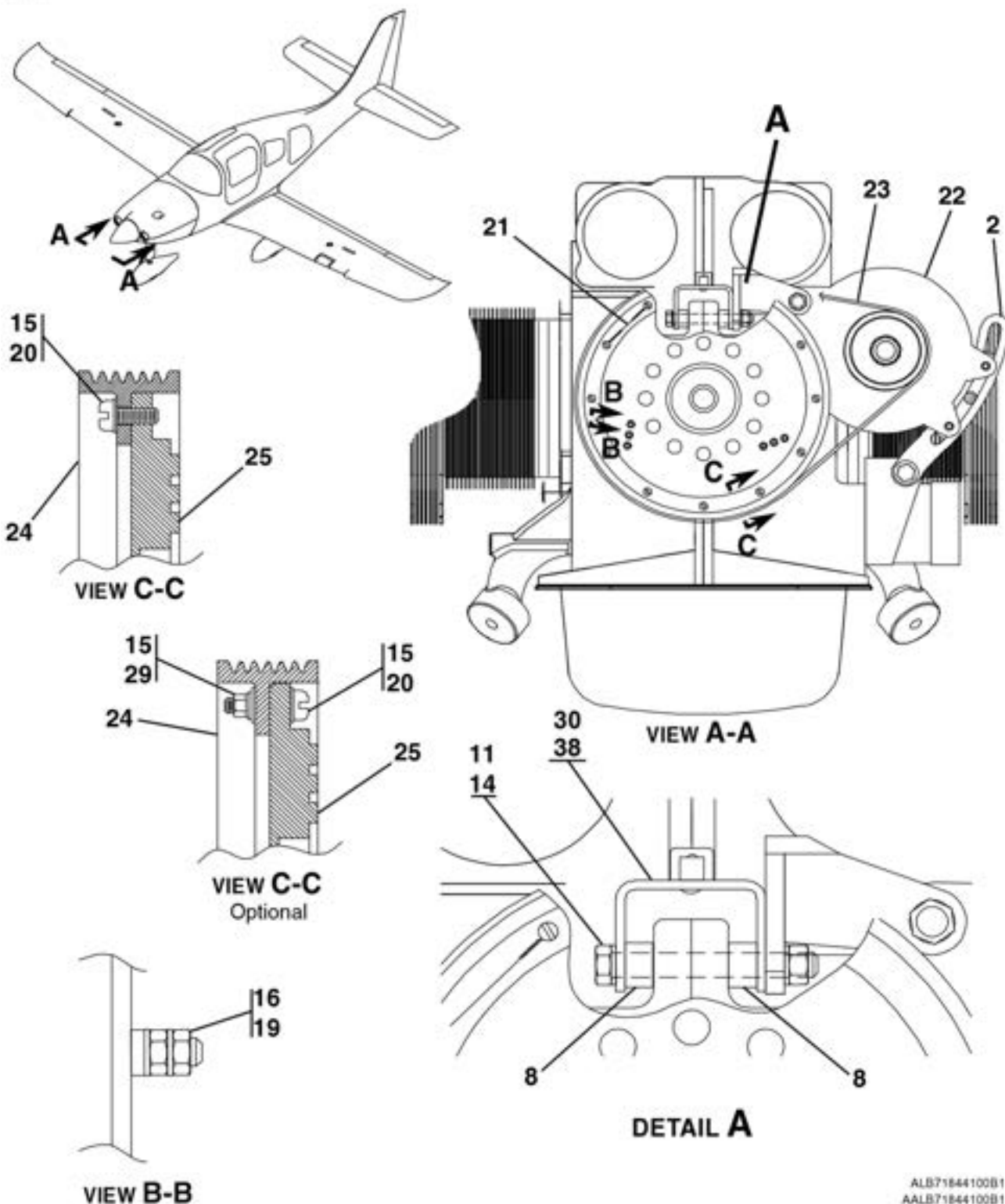
ALTERNATOR INSTALLATION FIGURE 09 (SHEET 1)
