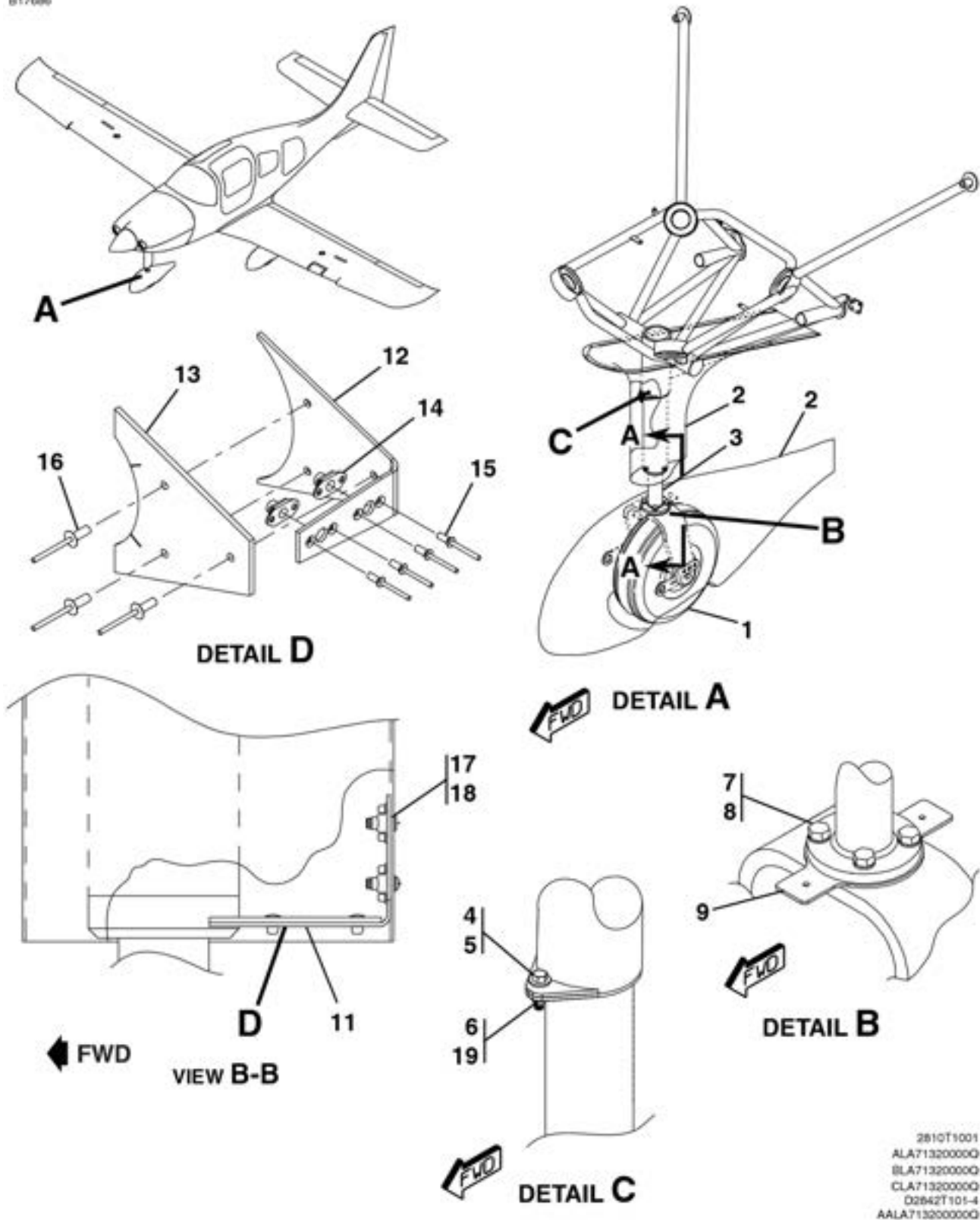
NOSE GEAR ASSEMBLY FIGURE 06 (SHEET 1)
