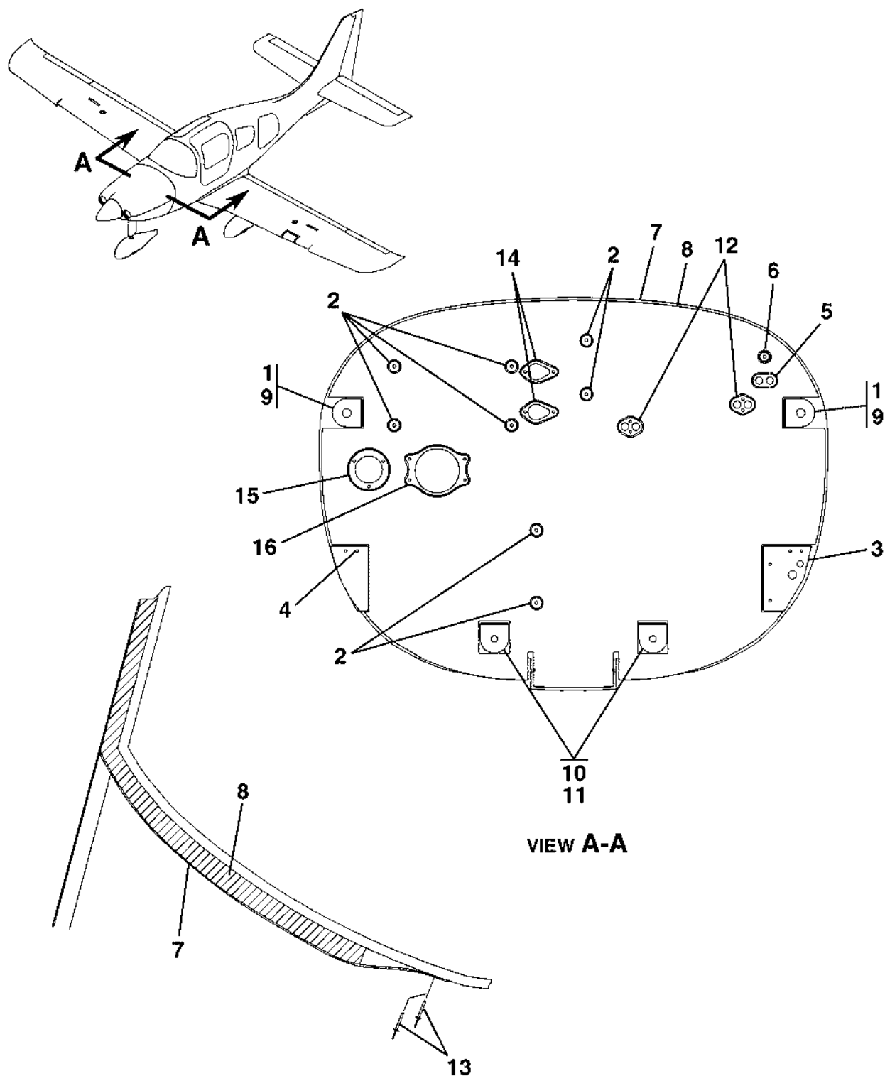
PHENOLIC SPACER ASSEMBLY FIGURE 12 (SHEET 1)
