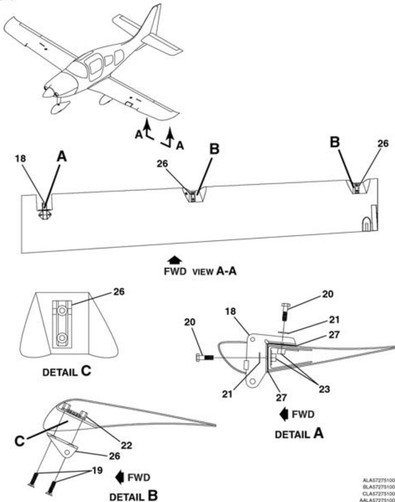
AILERON ASSEMBLY FIGURE 17 (SHEET 2)
