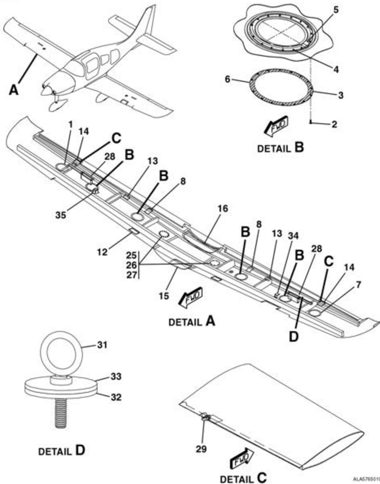
WING ACCESS PANEL ASSEMBLY FIGURE 03 (SHEET 1)
