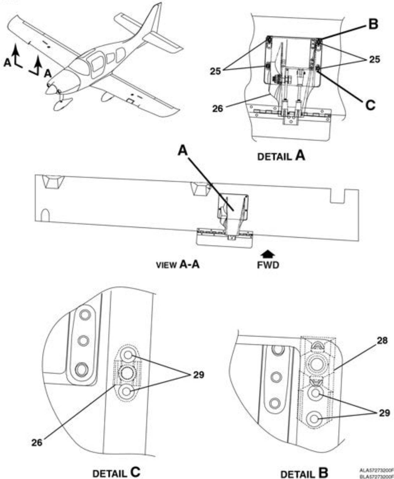
TRIM ASSEMBLY - AILERON FIGURE 12 (SHEET 2)
