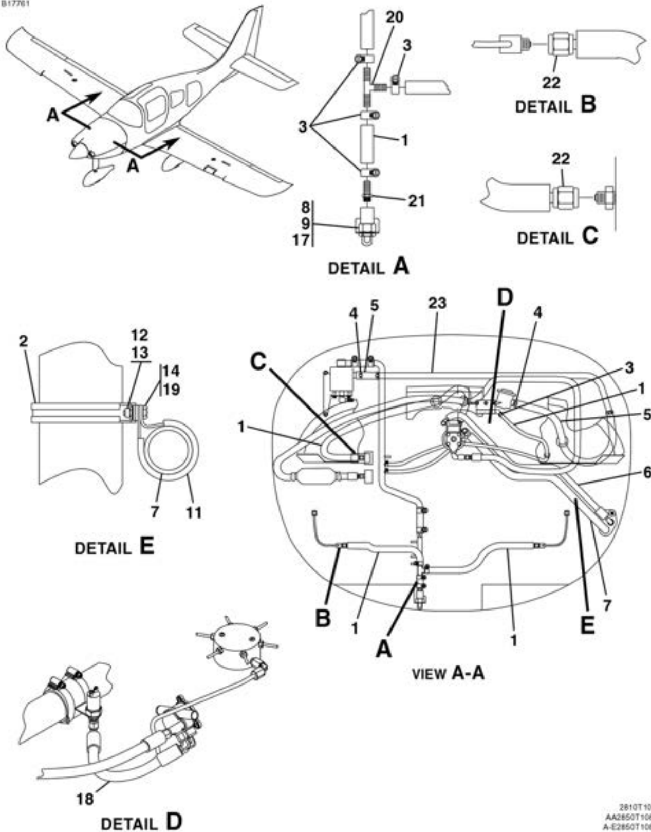
ENGINE FUEL SYSTEMS ASSEMBLY FIGURE 01 (SHEET 1)
