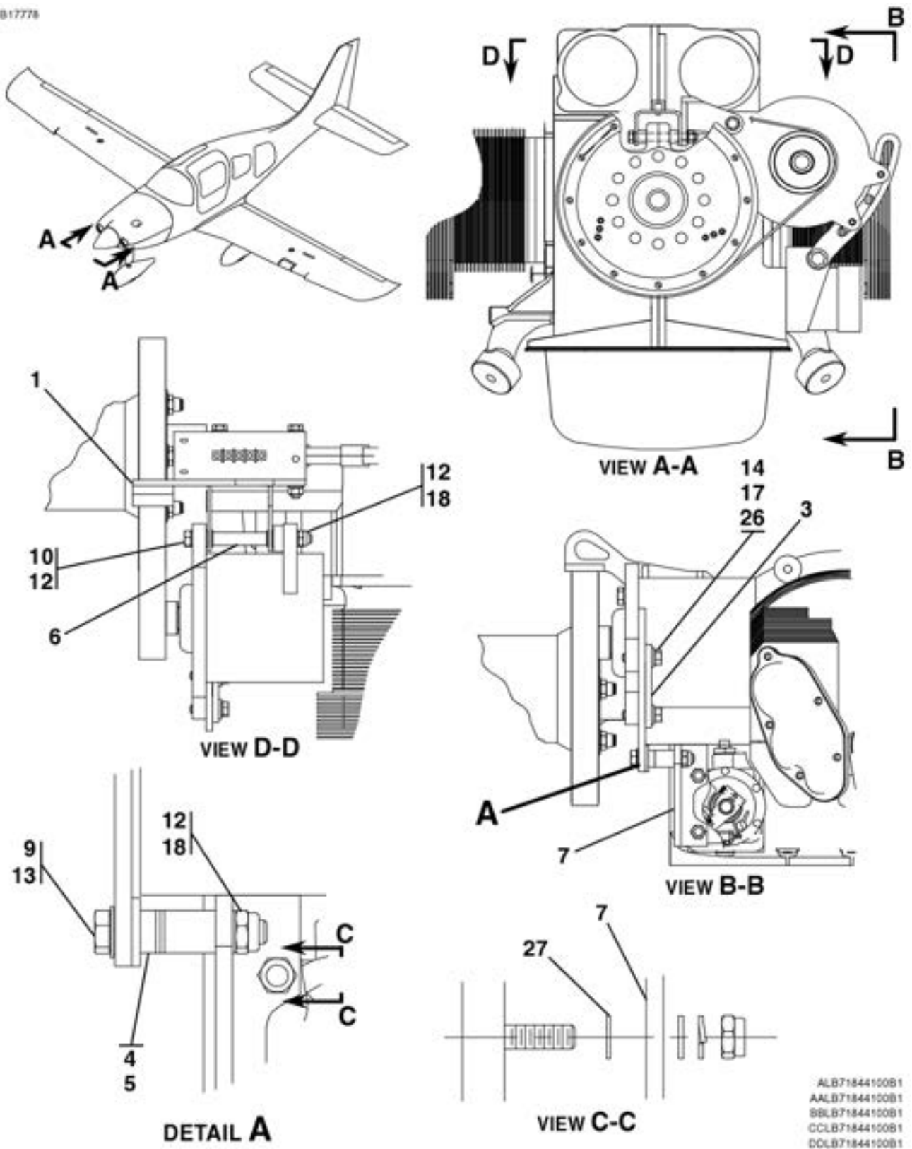
ALTERNATOR INSTALLATION FIGURE 09 (SHEET 2)
