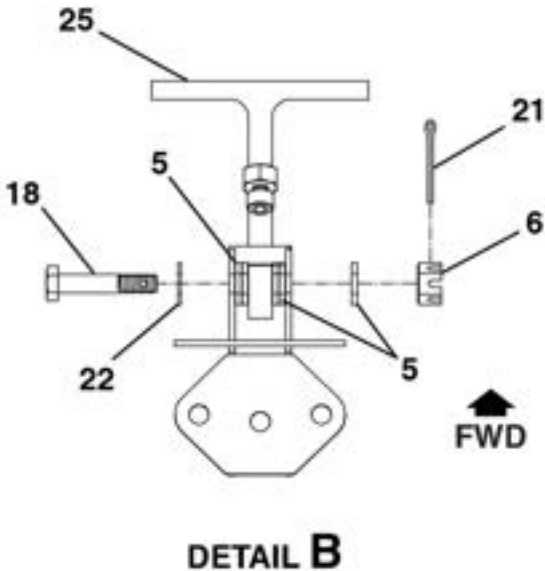
AILERON INSTALLATION FIGURE 10 (SHEET 5)
