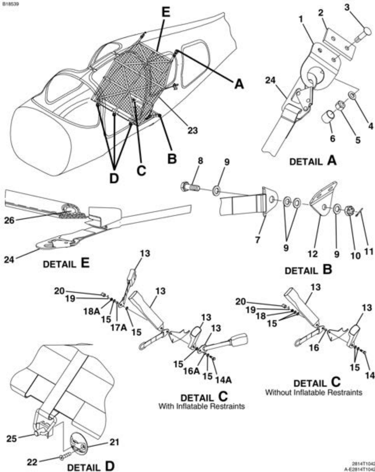
CARGO BARRIER NET INSTALLATION FIGURE 09 (SHEET 1)
