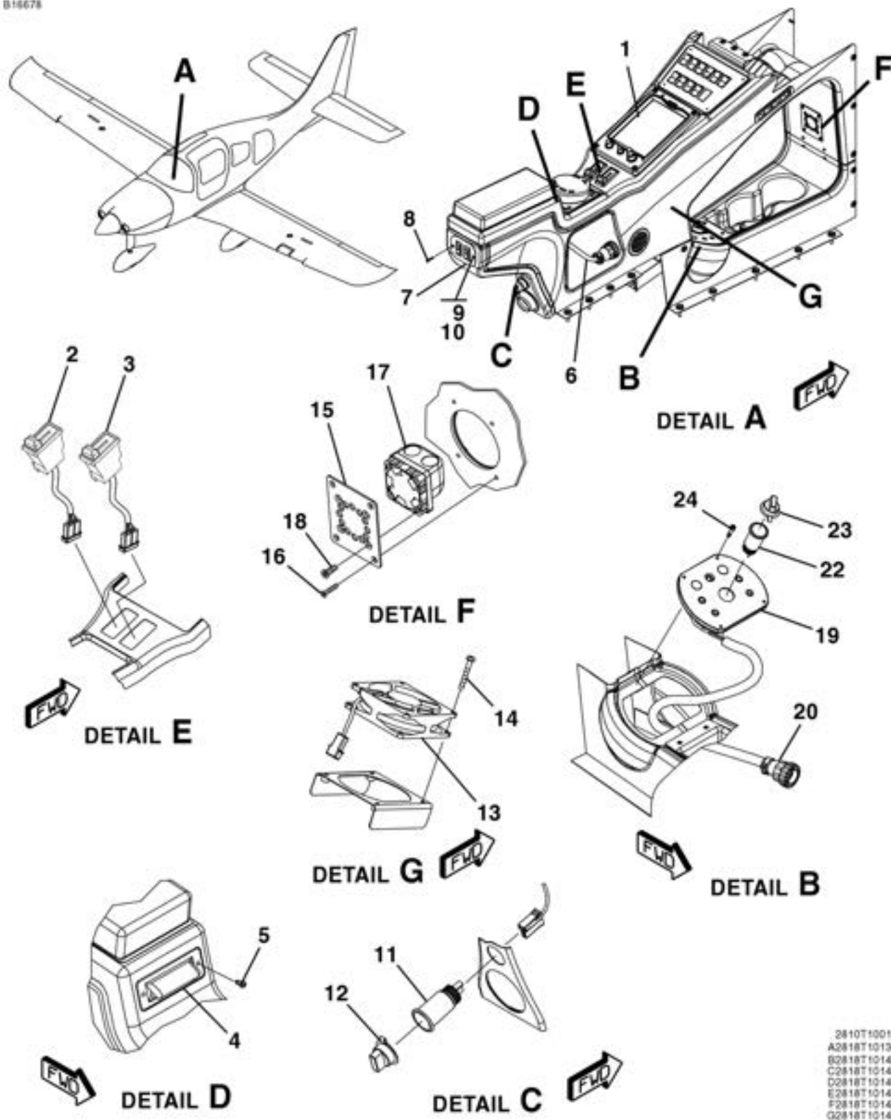
PEDESTAL EQUIPMENT FIGURE 03 (SHEET 1)
