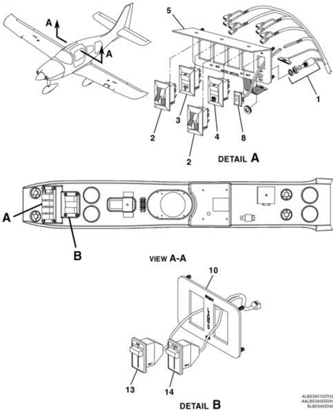
OVERHEAD CONSOLE MASTER SWITCH PANELS FIGURE 02 (SHEET 1)
