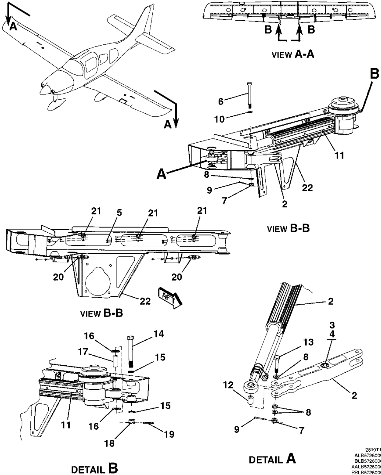
CENTRAL BELL CRANK ASSEMBLY - FLAP FIGURE 19 (SHEET 1)
