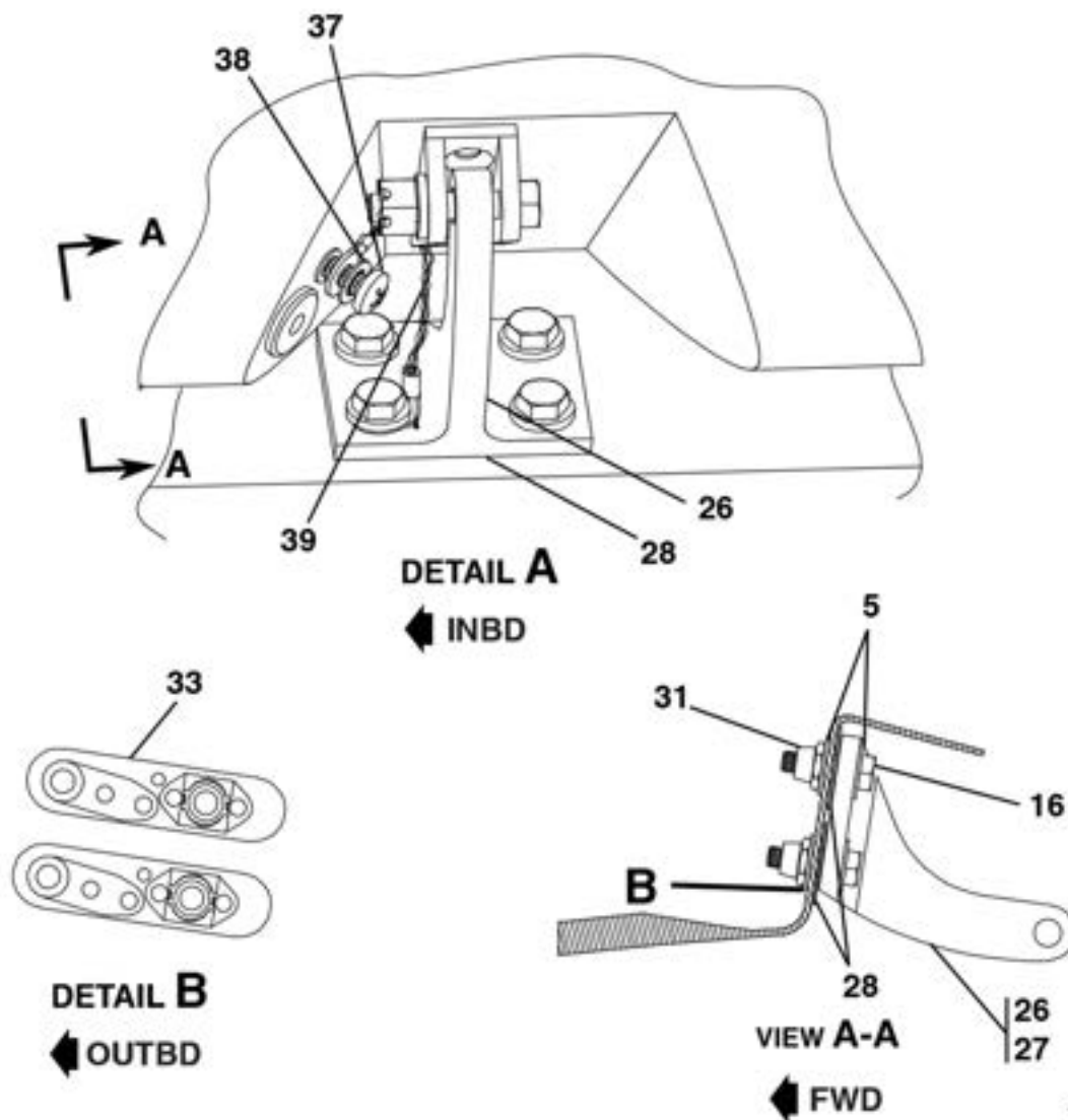
AILERON INSTALLATION FIGURE 10 (SHEET 4)
