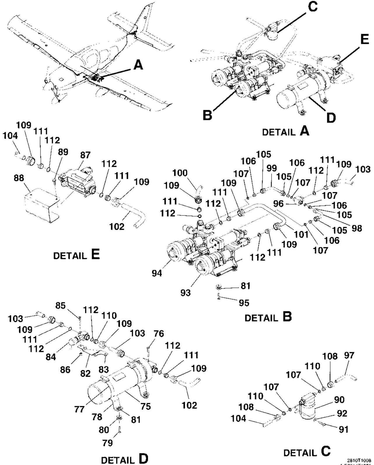
TKS SYSTEM - PLUMBING INSTALLATION FIGURE 05A (SHEET 2)
