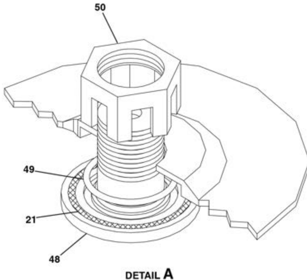
FUEL SYSTEM - WING ASSEMBLY FIGURE 04 (SHEET 8)
