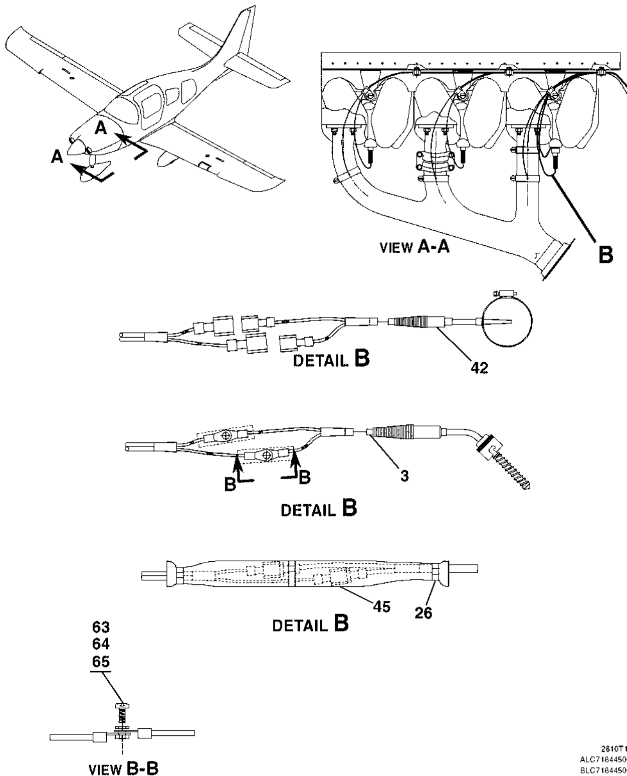
WIRING AND SENSORS ASSEMBLY FIGURE 02 (SHEET 5)
