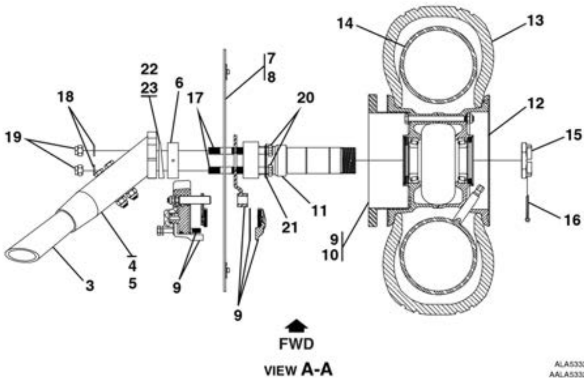
MAIN GEAR ASSEMBLY FIGURE 02 (SHEET 1)
