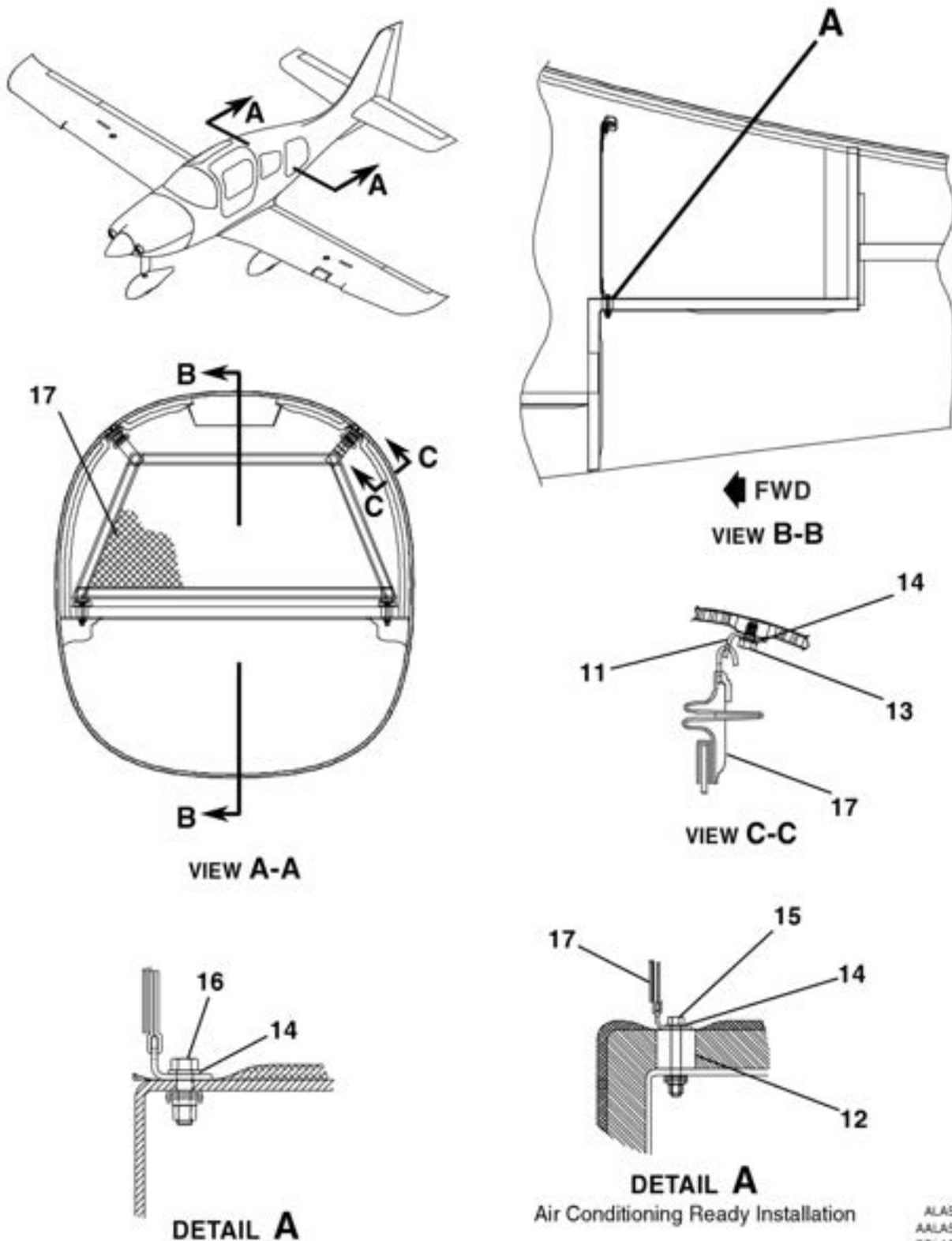
BAGGAGE NET INSTALLATION FIGURE 21 (SHEET 2)
