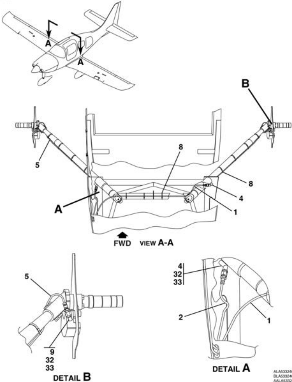
BRAKE SYSTEM ASSEMBLY FIGURE 05 (SHEET 2)
