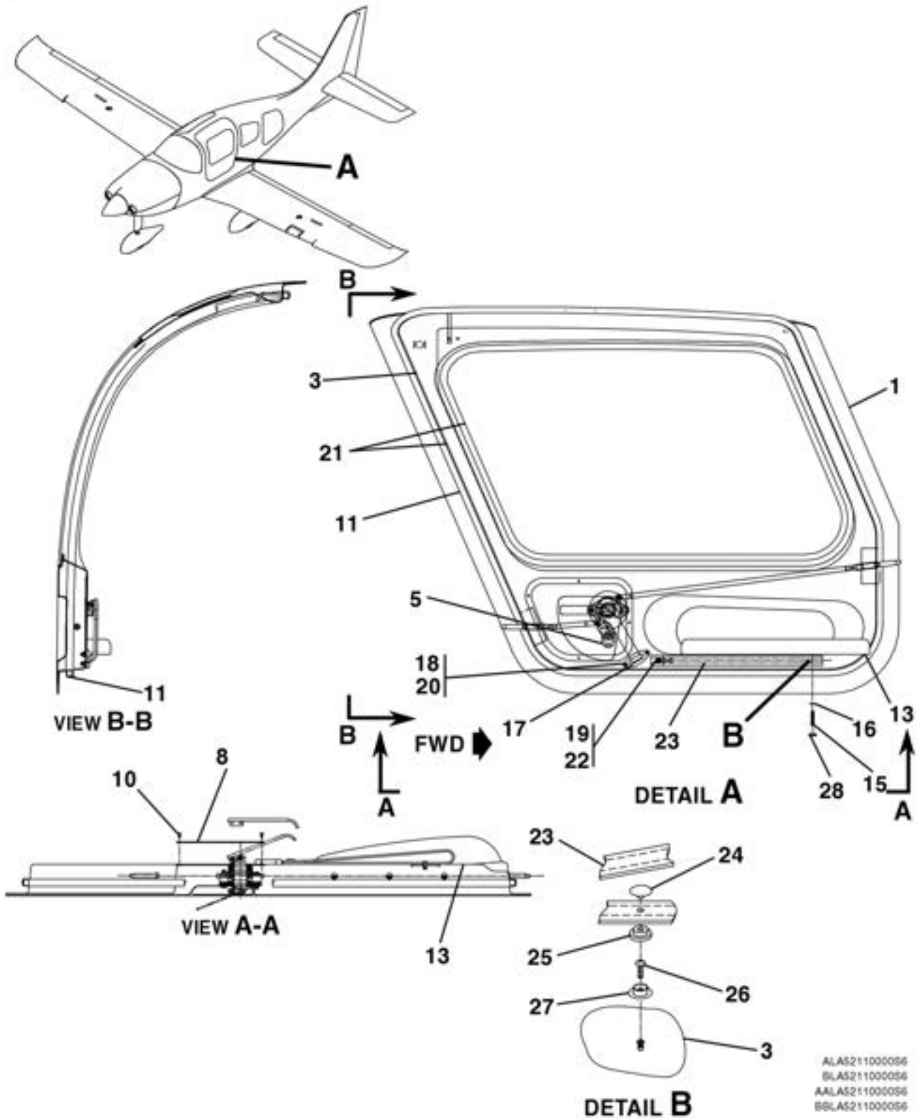
CABIN DOOR ASSEMBLY FIGURE 02 (SHEET 1)
