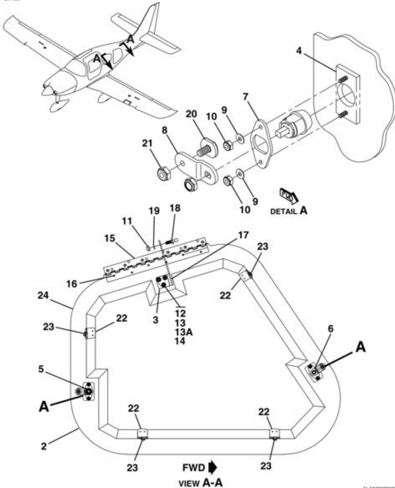
BAGGAGE DOOR ASSEMBLY FIGURE 07 (SHEET 1)
