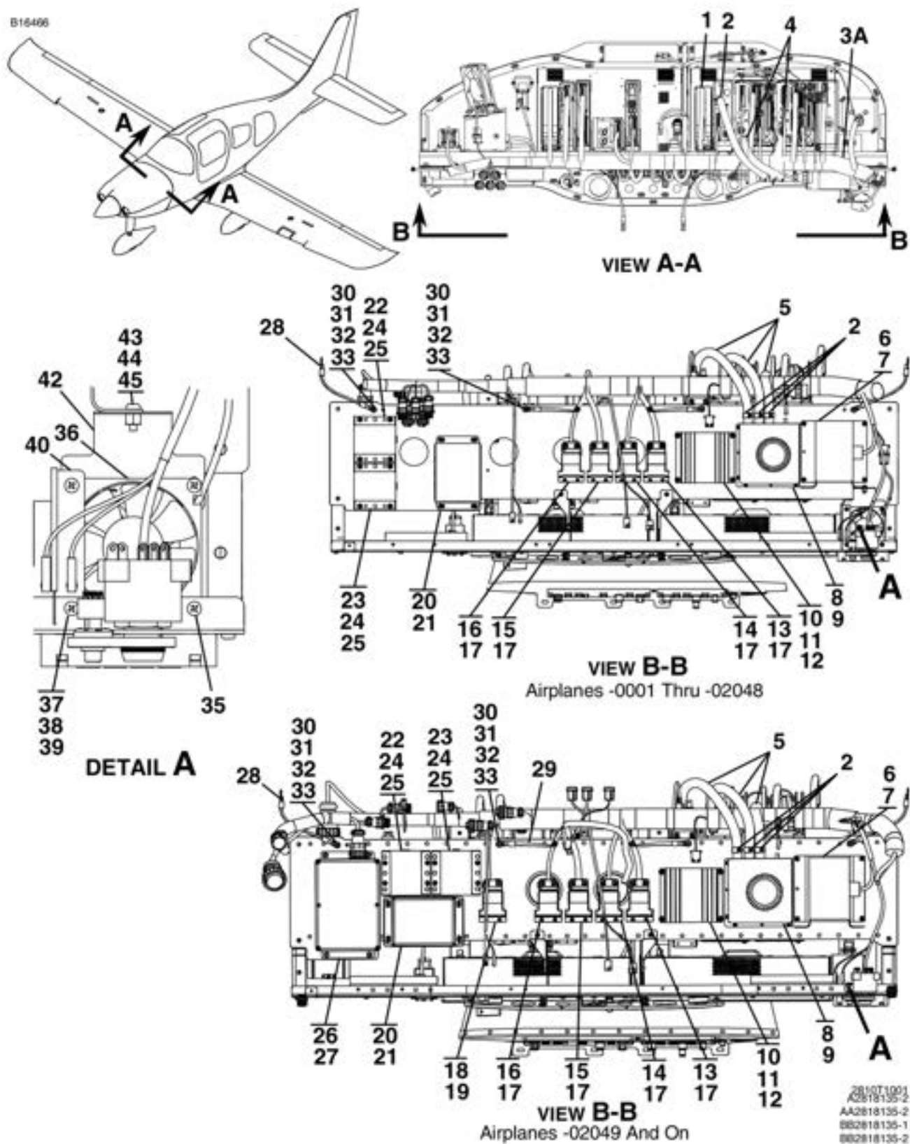
AVIONICS AND NAVIGATION EQUIPMENT - AVIONICS SHELF HARNESS AND EQUIPMENT FIGURE 08 (SHEET 1)
