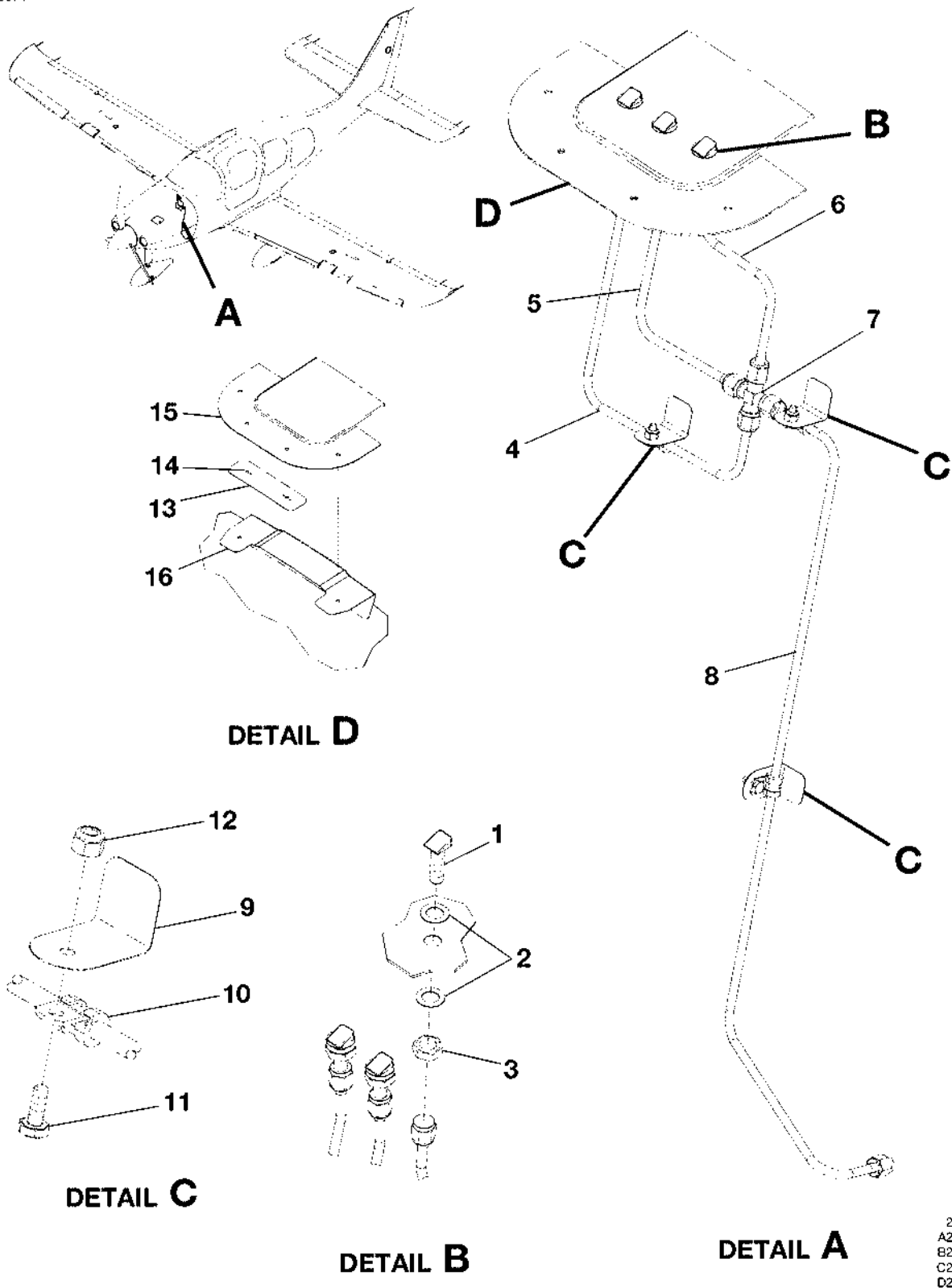
TKS SYSTEM - WINDSHIELD NOZZLE INSTALLATION FIGURE 06 (SHEET 1)
