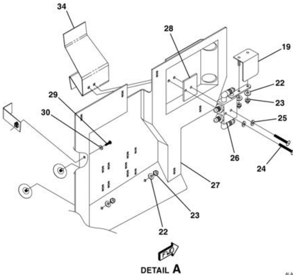
BRAKE SYSTEM ASSEMBLY FIGURE 05 (SHEET 4)
