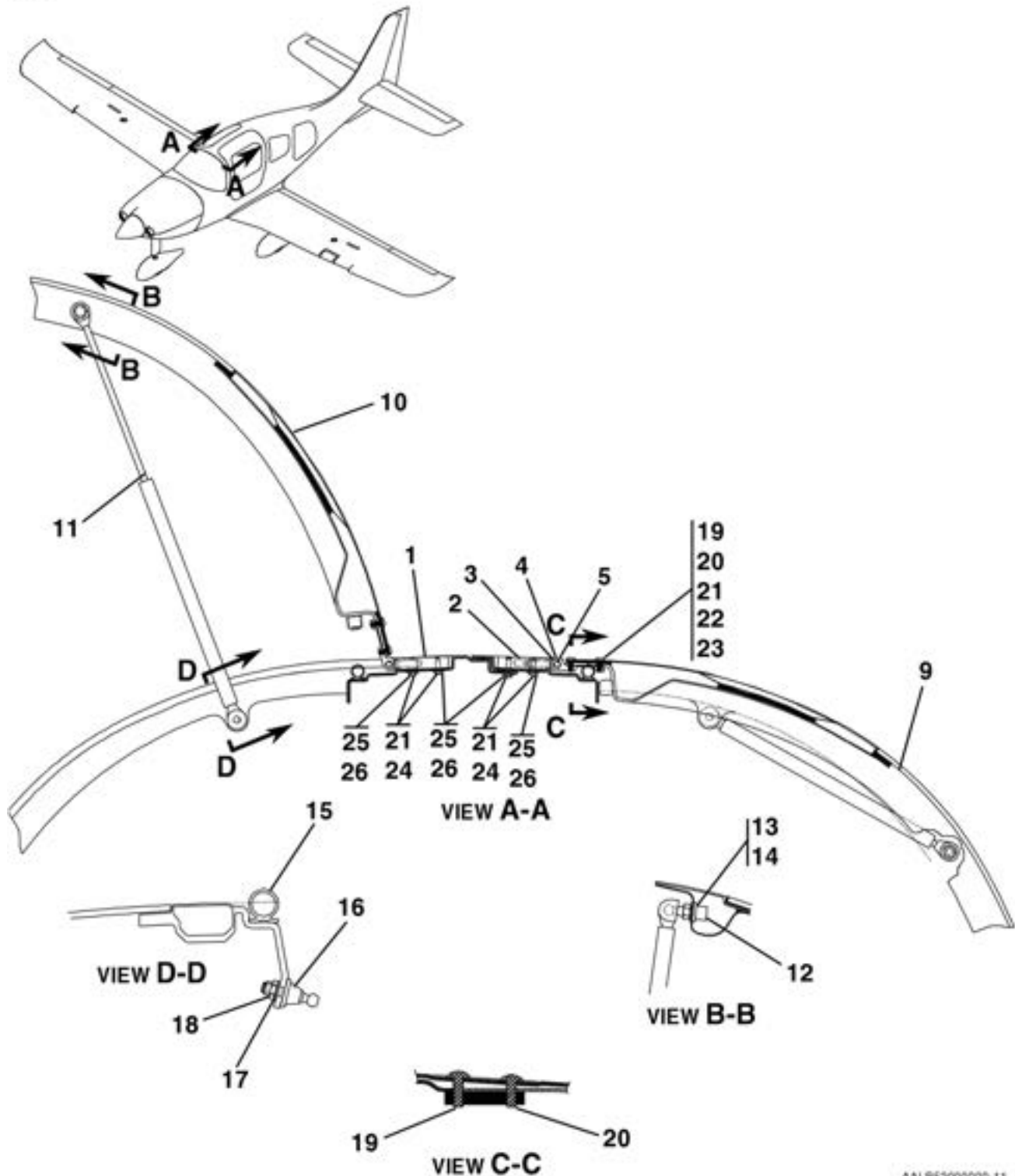
CABIN AND BAGGAGE DOOR INSTALLATION FIGURE 01 (SHEET 2)
