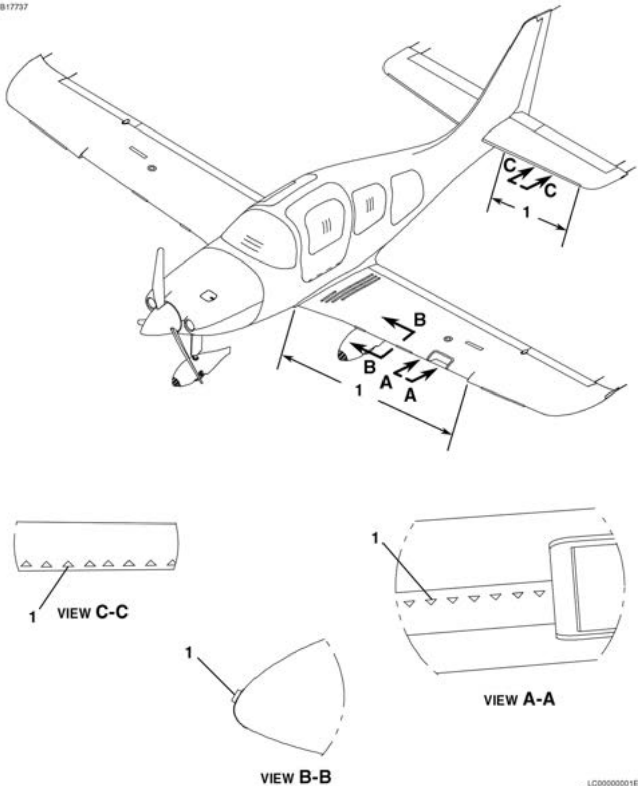
TURBULATOR TRIANGLES INSTALLATION FIGURE 05 (SHEET 1)
