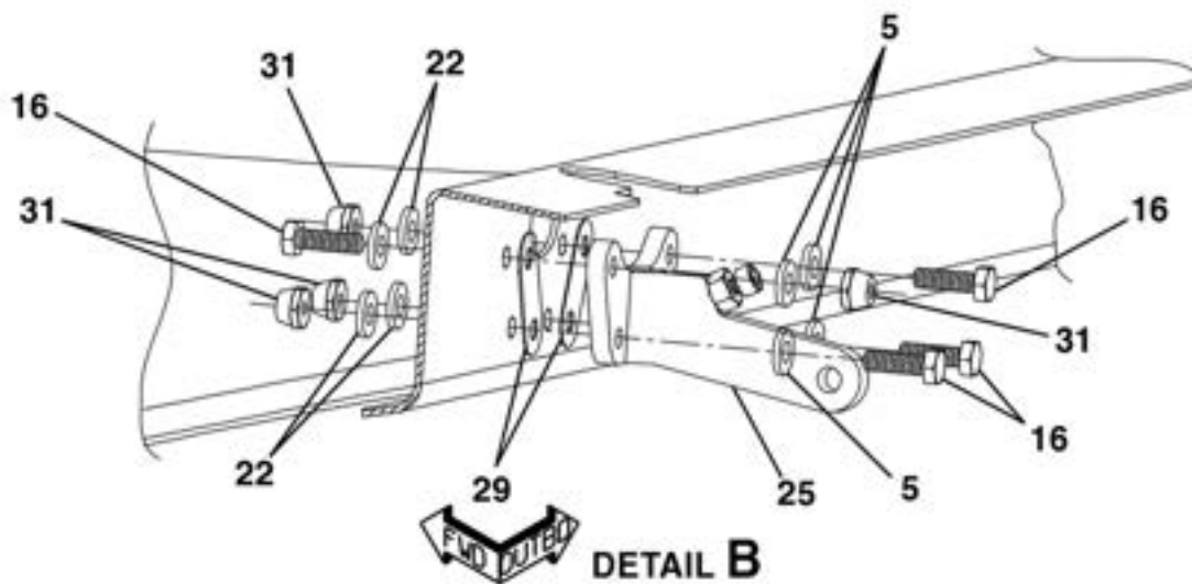
AILERON INSTALLATION FIGURE 10 (SHEET 3)
