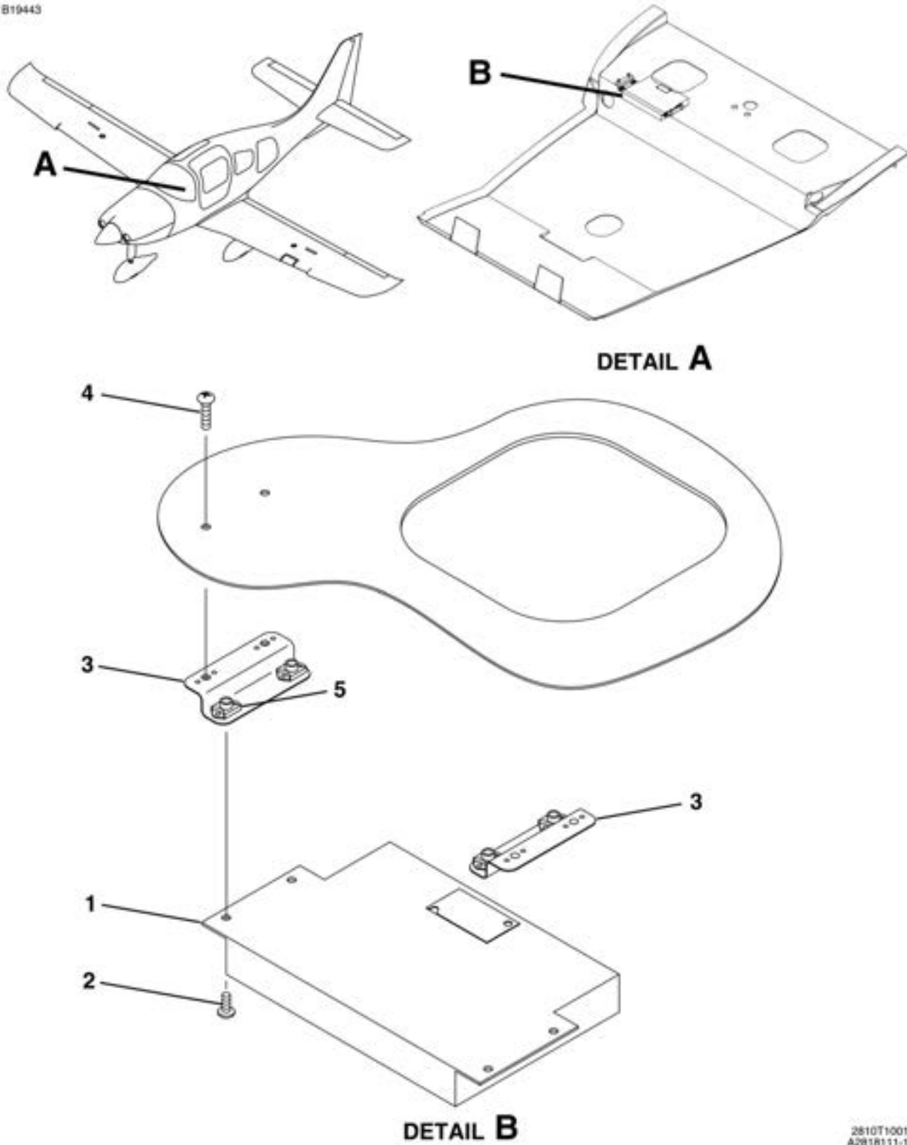
STALL COMPUTER INSTALLATION FIGURE 18 (SHEET 1)
