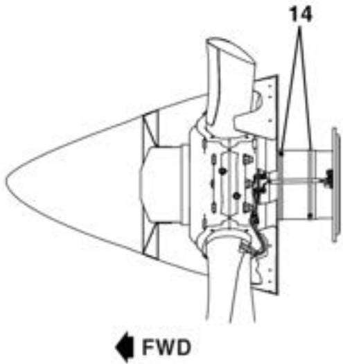
VIEW A-A Hartzell Heater Boot Lead Secure - Booted and Unbooted
