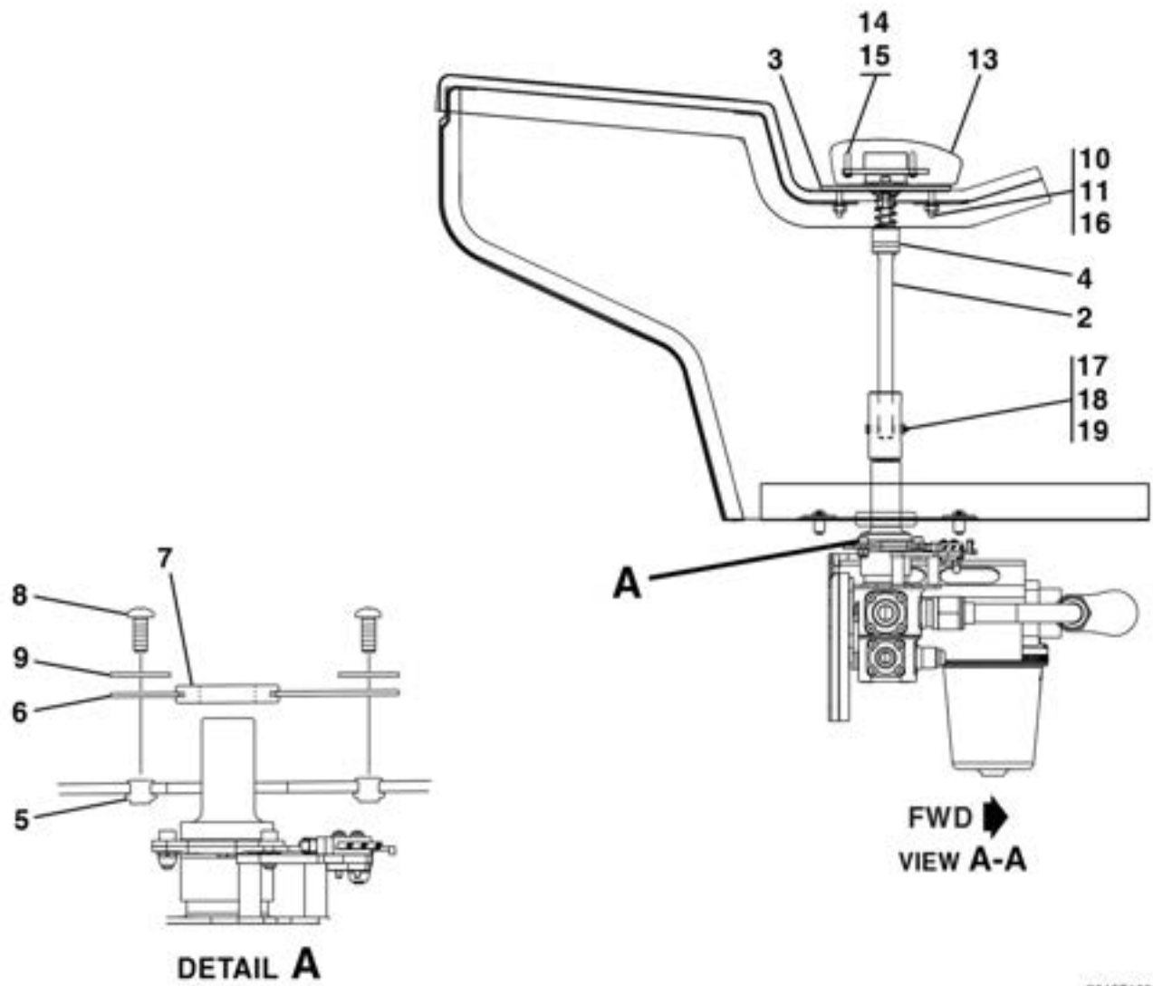
FUEL SYSTEM ASSMBLY - FUSELAGE FIGURE 01 (SHEET 1)
