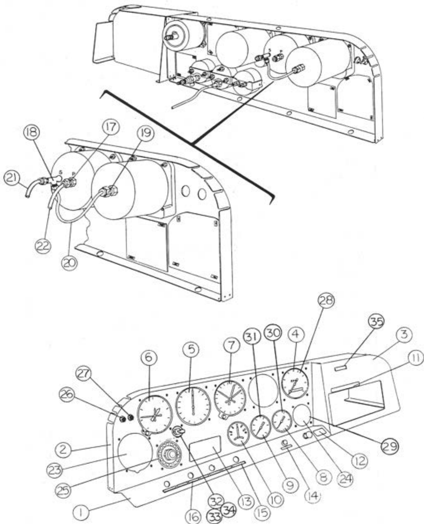
FIGURE 12 INSTALLATION - INSTRUMENTS (LOW PANEL) PRE 1978 MODELS
