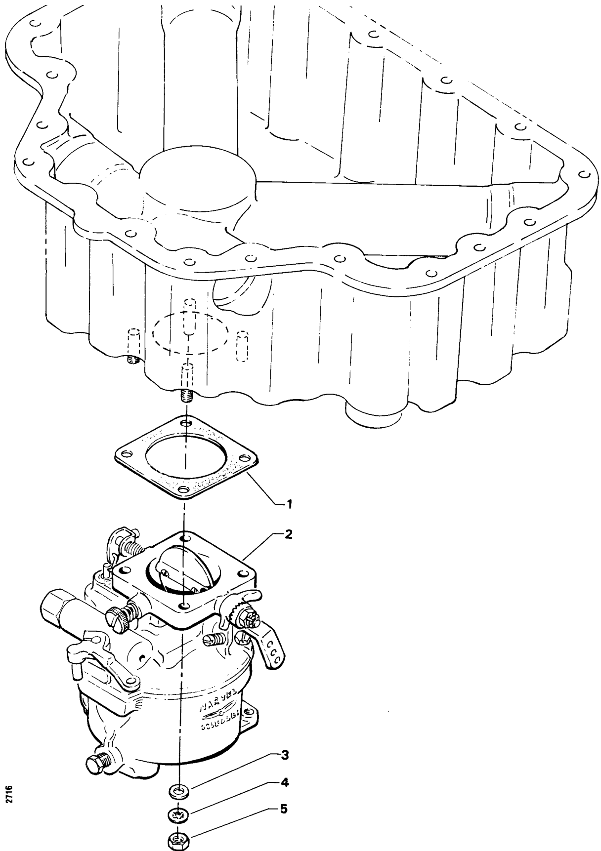
Figure 30. Carburetor Assembly
