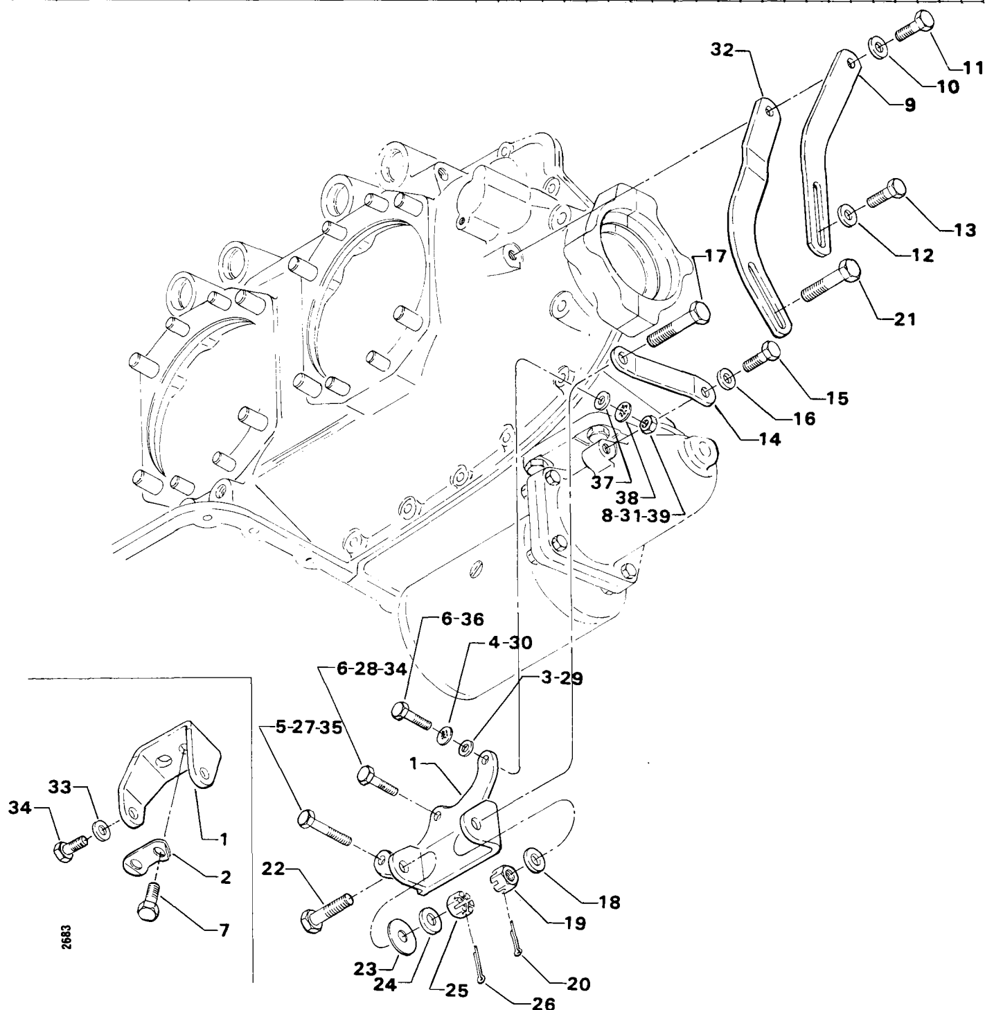
Figure 25. Alternator Mounting and Attaching Parts
