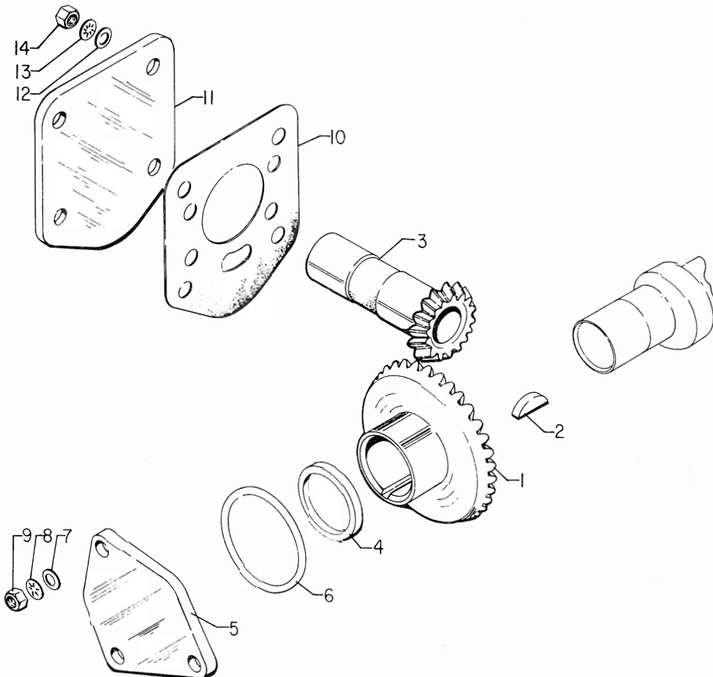
Figure 5. Propeller Governor Drive
