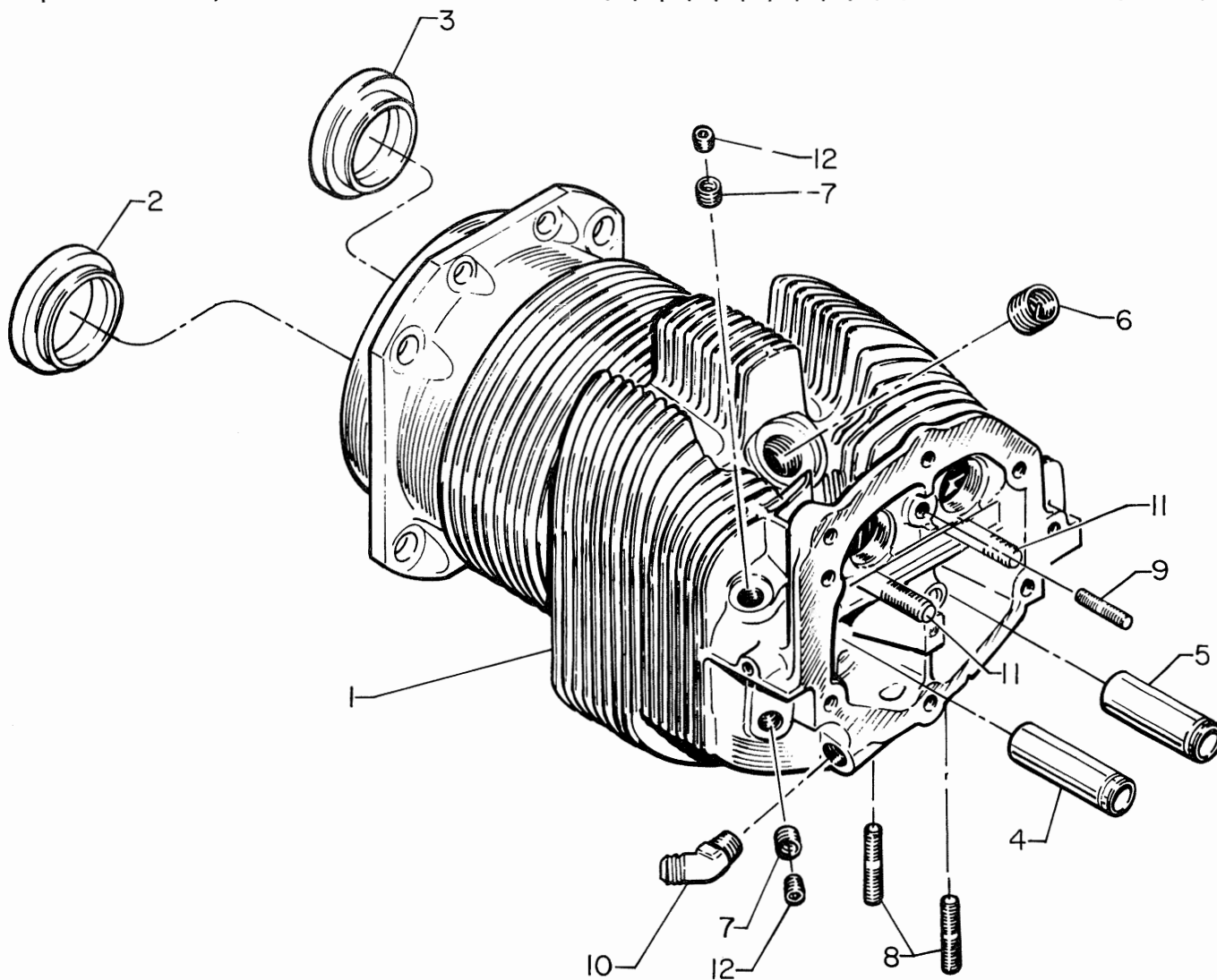
Figure 10. Cylinder Assembly
