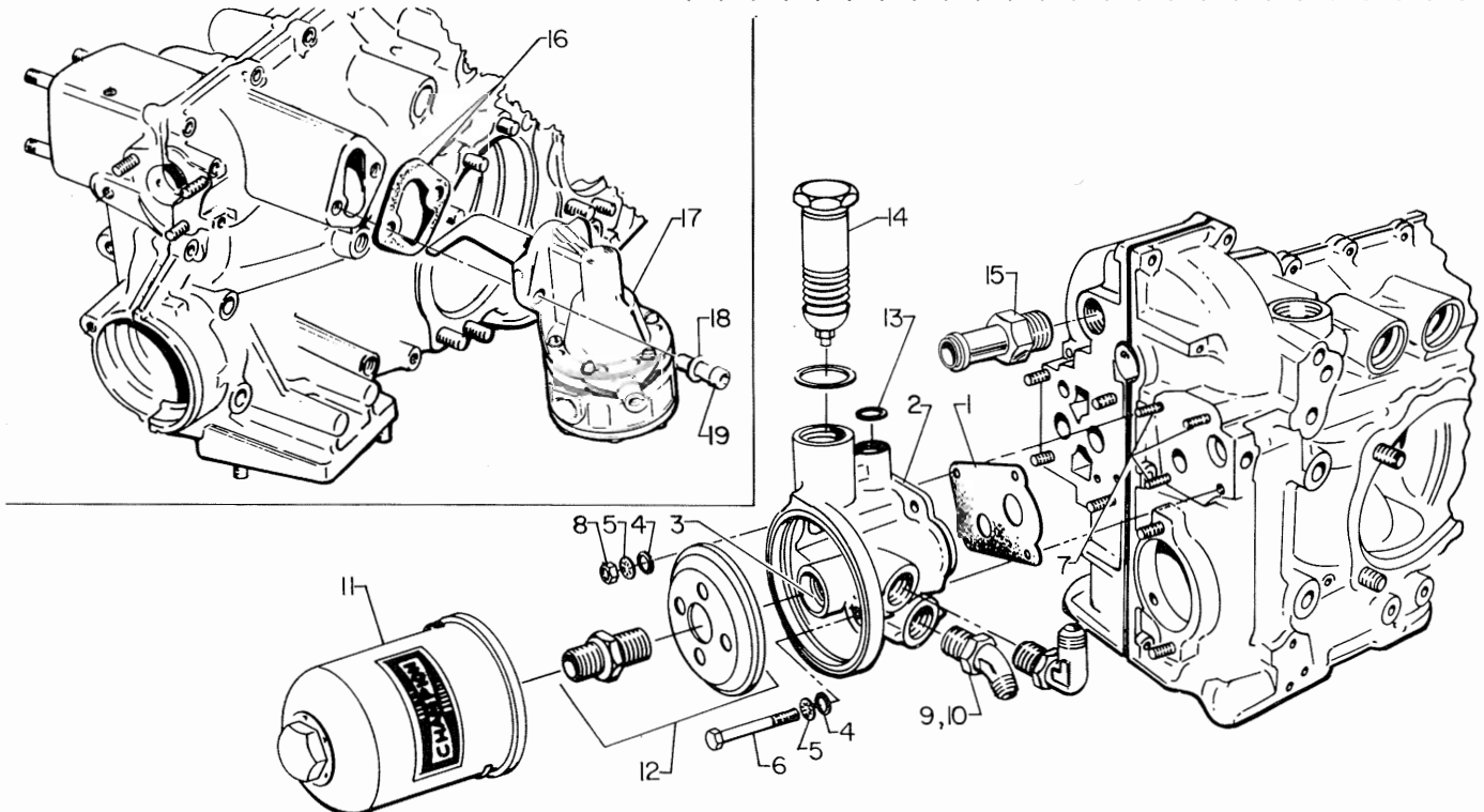
Figure 8. Oil Filter and Fuel Pump
