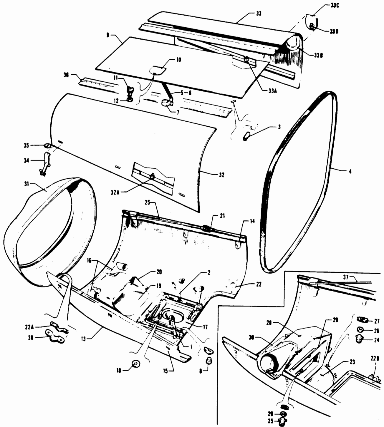
Figure 25. Engine Cowl Installation (PA-24-180 and PA-24-250 - Serial Nos. 24-1 and up) (PA-24-260 - Serial Nos. 24-3642, 24-4000 to 24-4782, 24-4784 to 24-4803 inclusive)
