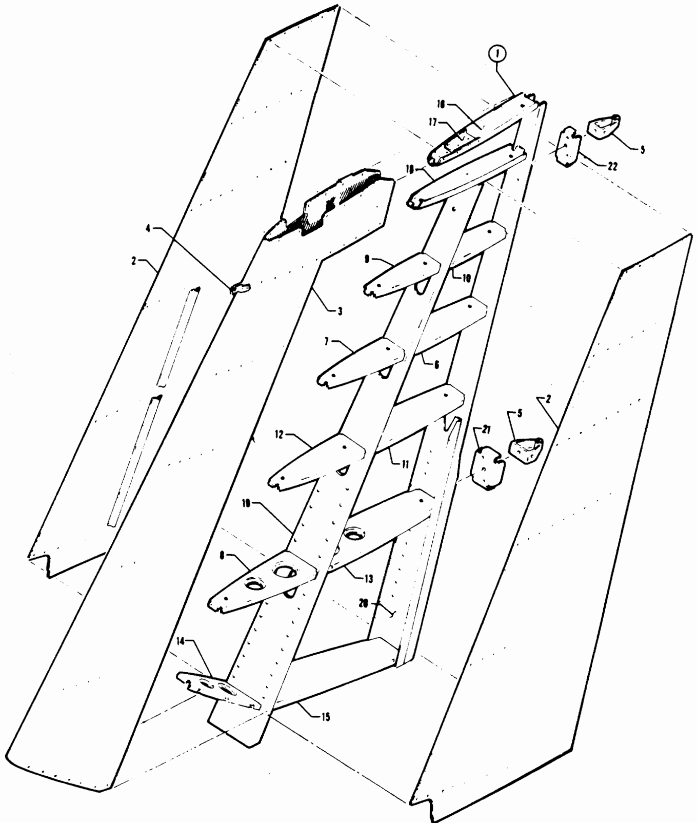
Figure 23G. Fin Assembly "400"
