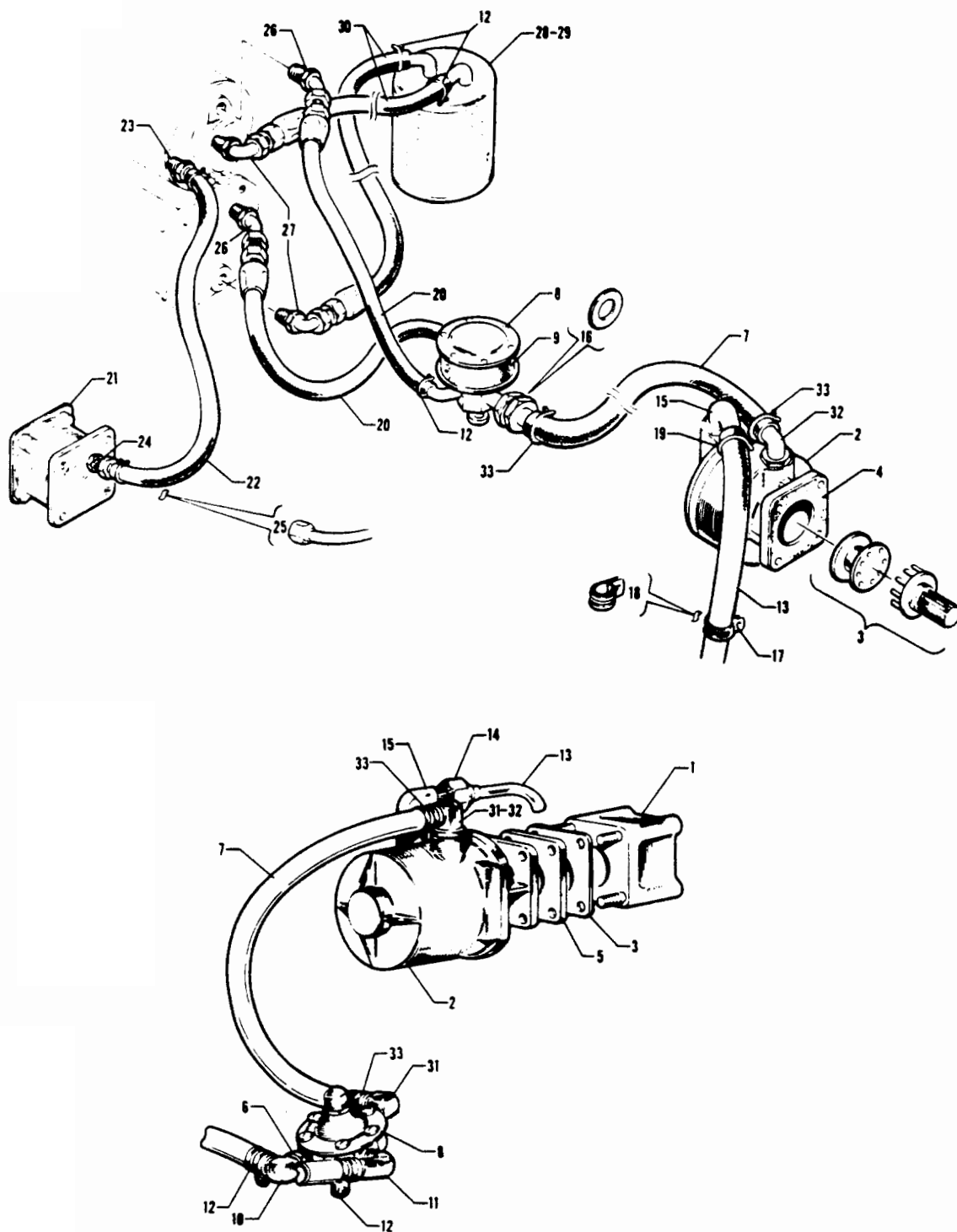
Figure 14A. Vacuum System Installation (Dry Vacuum Pump) (Serial Nos. 24-2176, 24-2177, 24-2179 to 24-2184 incl., 24-2186 to 24-2202 incl., 24-2204 to 24-2218 incl., 24-2222, 24-2299 and up, and 26-2 and up.)
