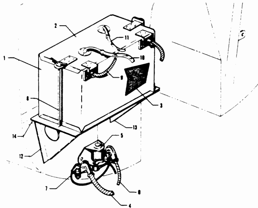
Figure 32C. Battery Box Installation (Serial Nos. 24-4247, 24-4300 and up)
