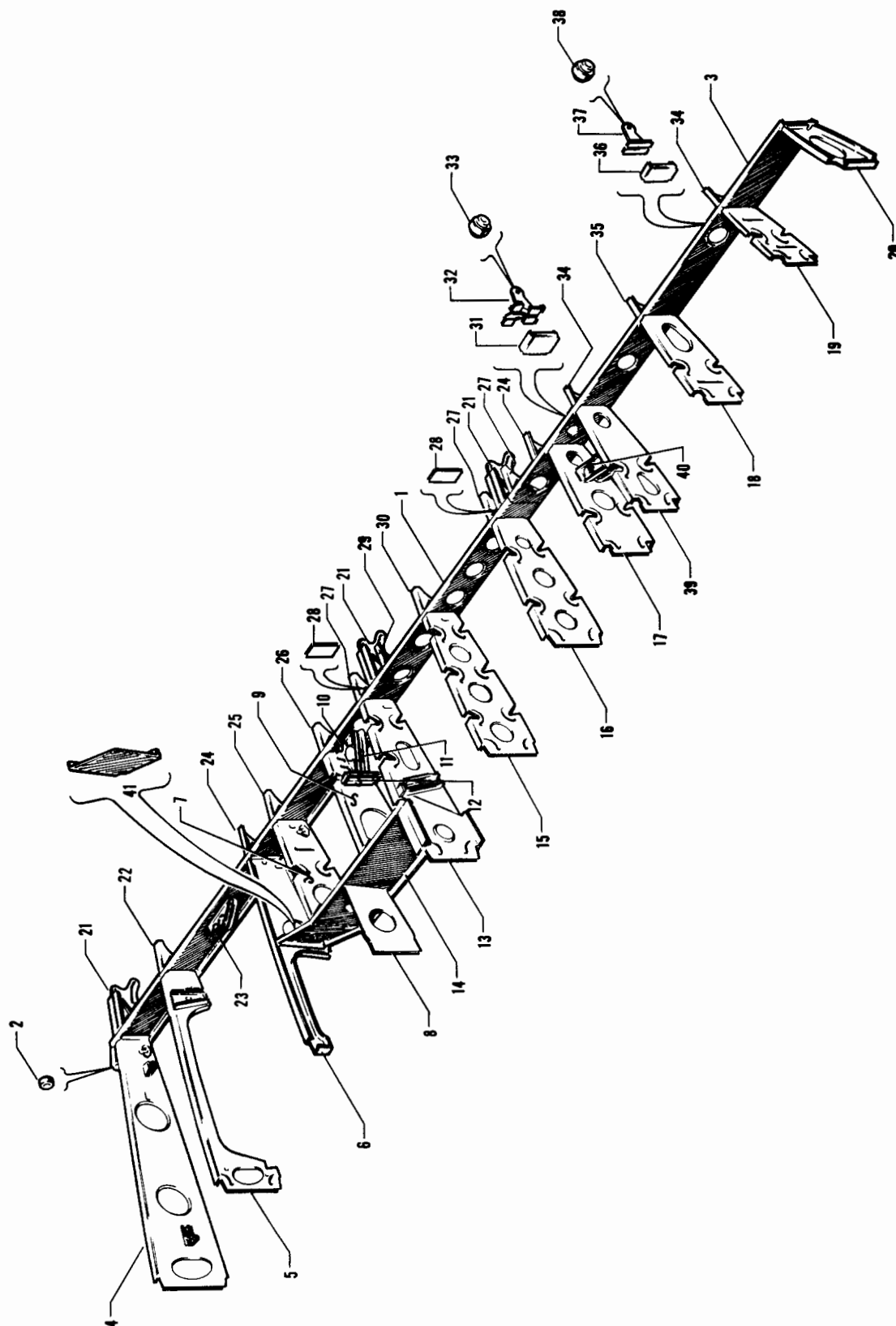
Figure 3B. Wing Construction Rear Spar Section (Serial Nos. 24-2844 and up, 26-2 and up)
