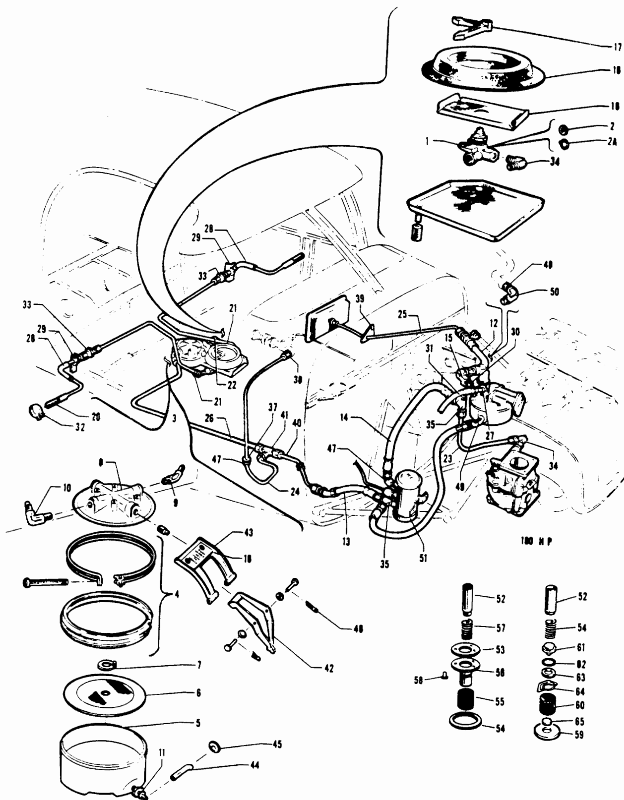
Figure 30A. Fuel System Installation "180" (Serial Nos. 24-2175, 24-2299 and up)
