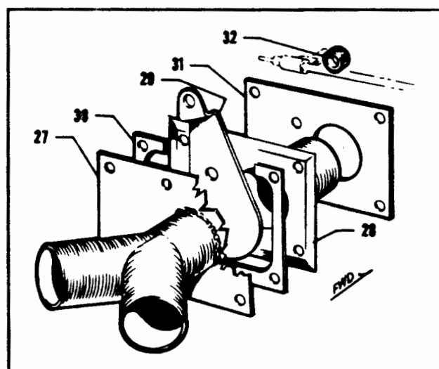
Figure 13. Cabin Heat, Defroster and Fresh Air Systems (Serial Nos. 24-1 to 24-1251 inclusive)
