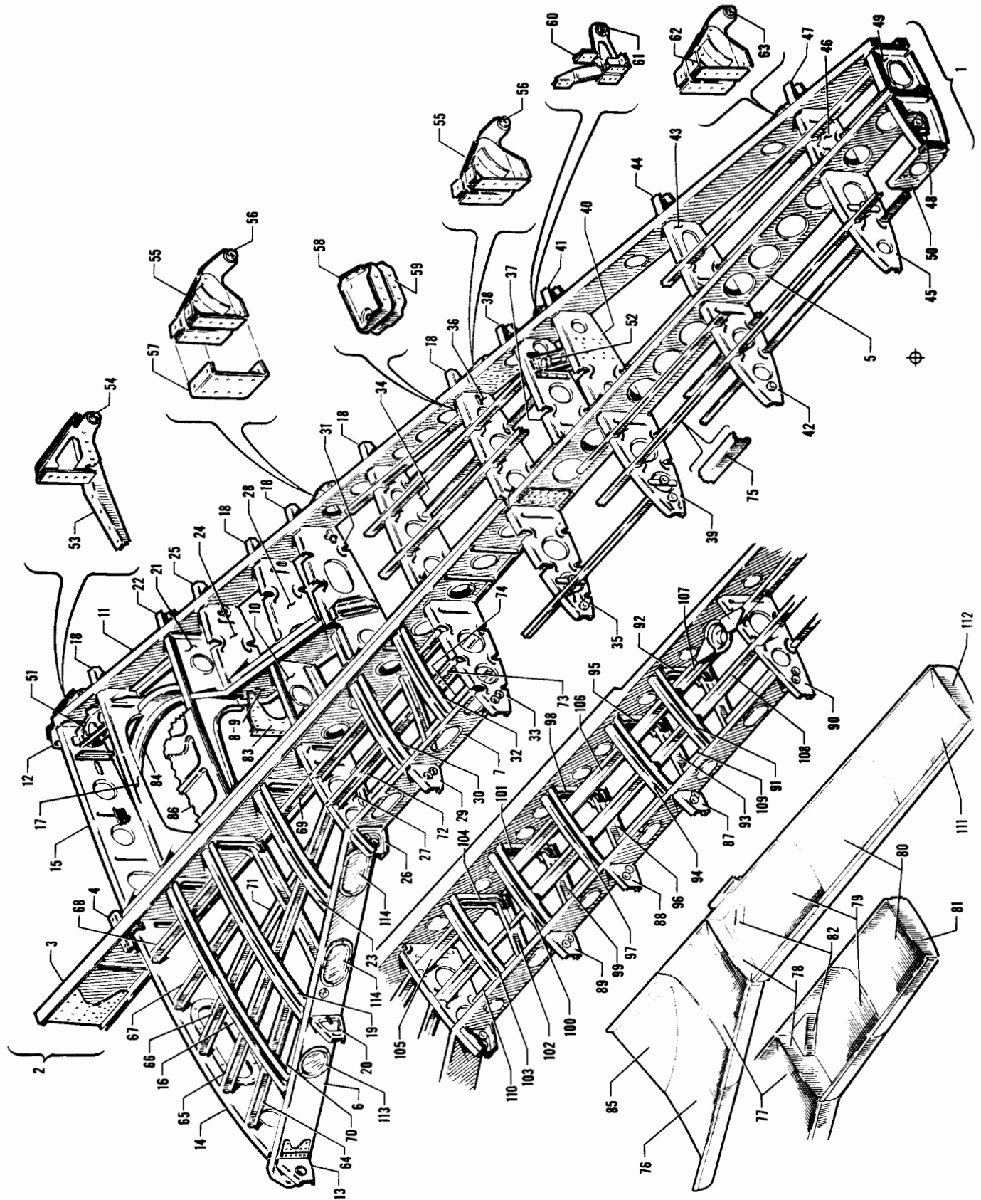
Figure 3A. Wing Construction (Wing Panels 22181, 22701 and 22700)
