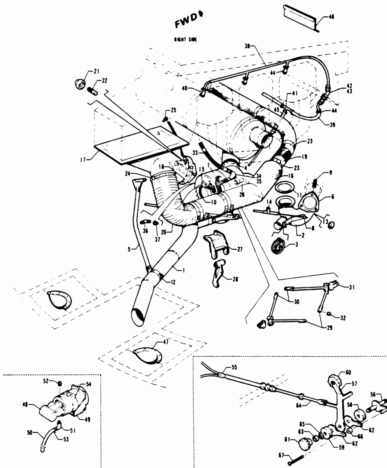
Figure 24H. Rajay Turbocharger Components
