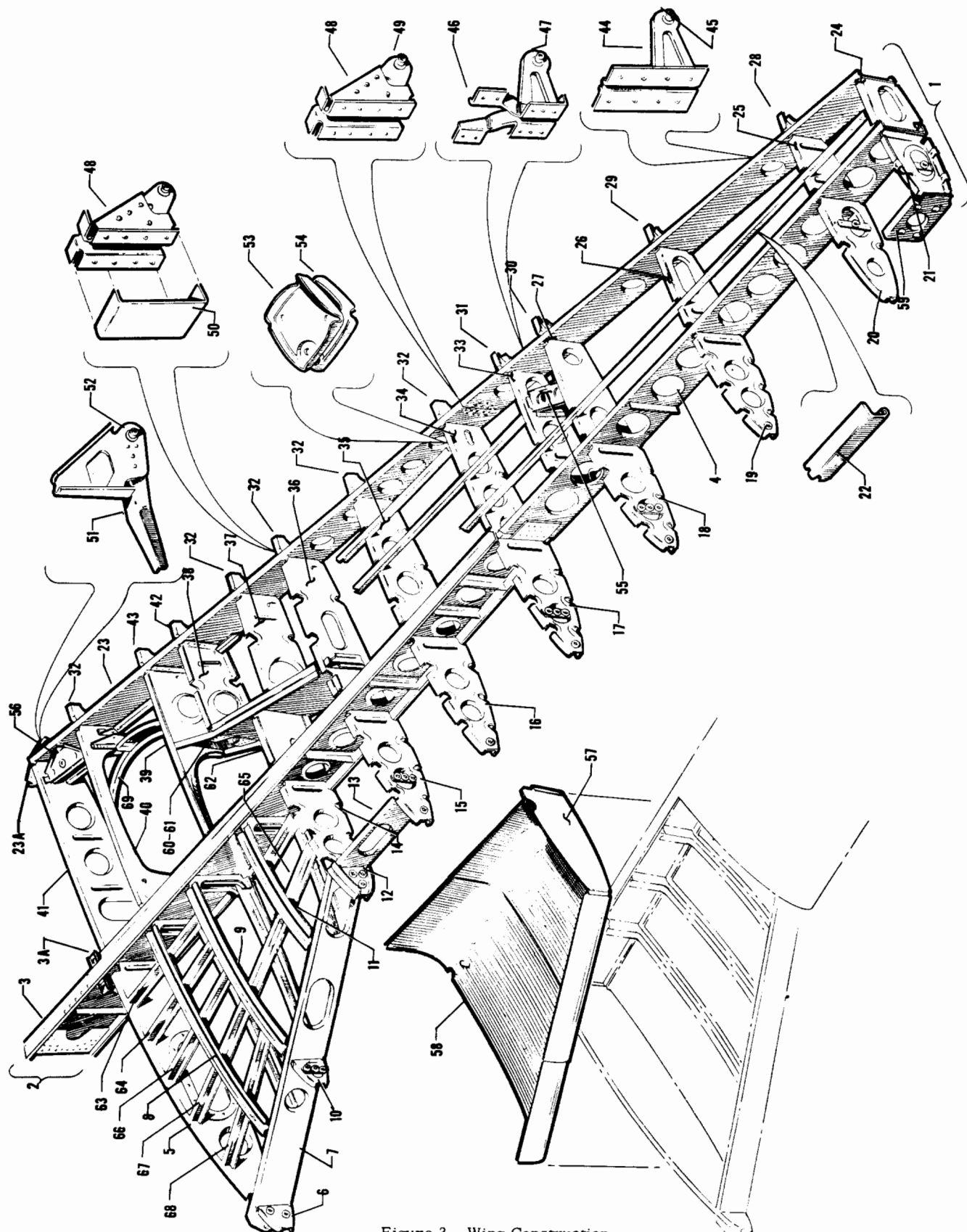
Figure 3. Wing Construction (Wing Panel 20377 Only)
