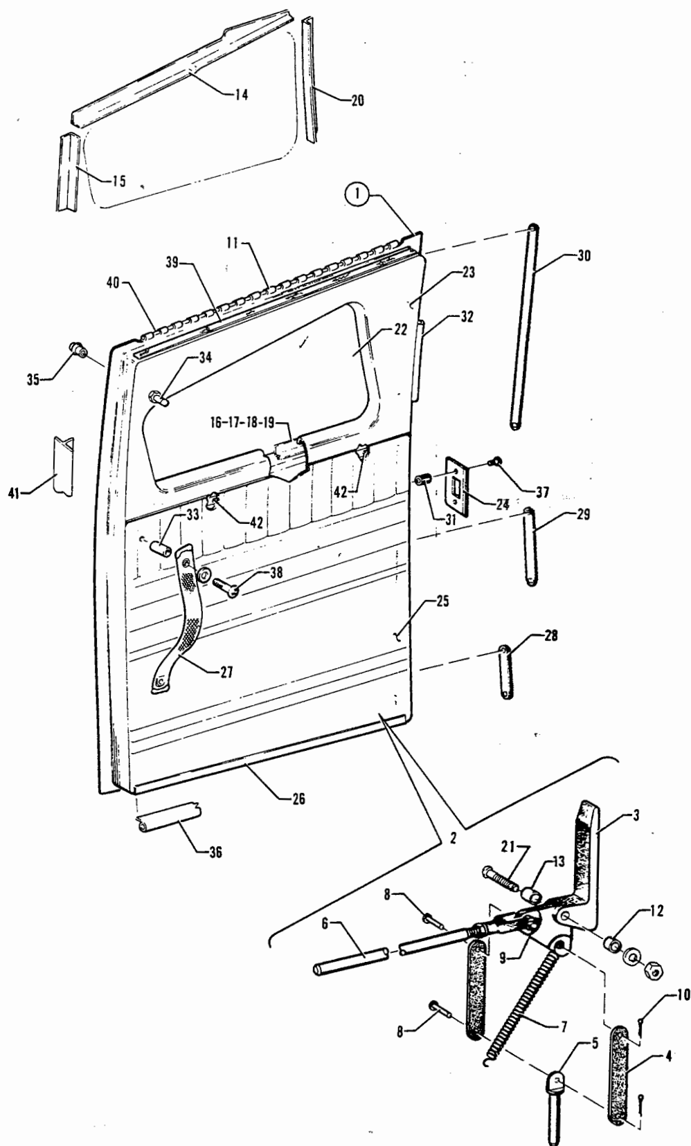
Figure 17. Fuselage Aft Cargo Door
