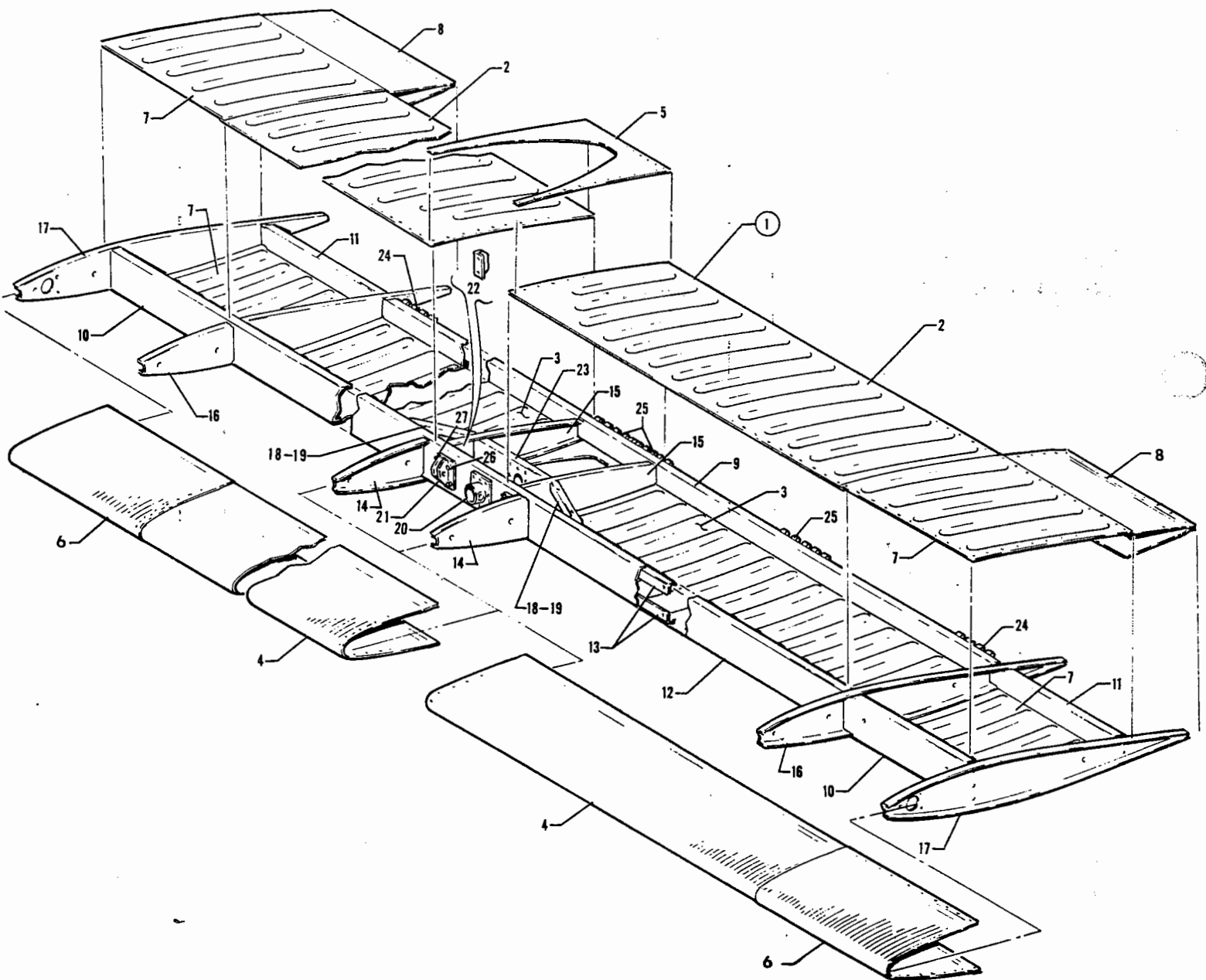
Figure 20. Stabilator Assembly
