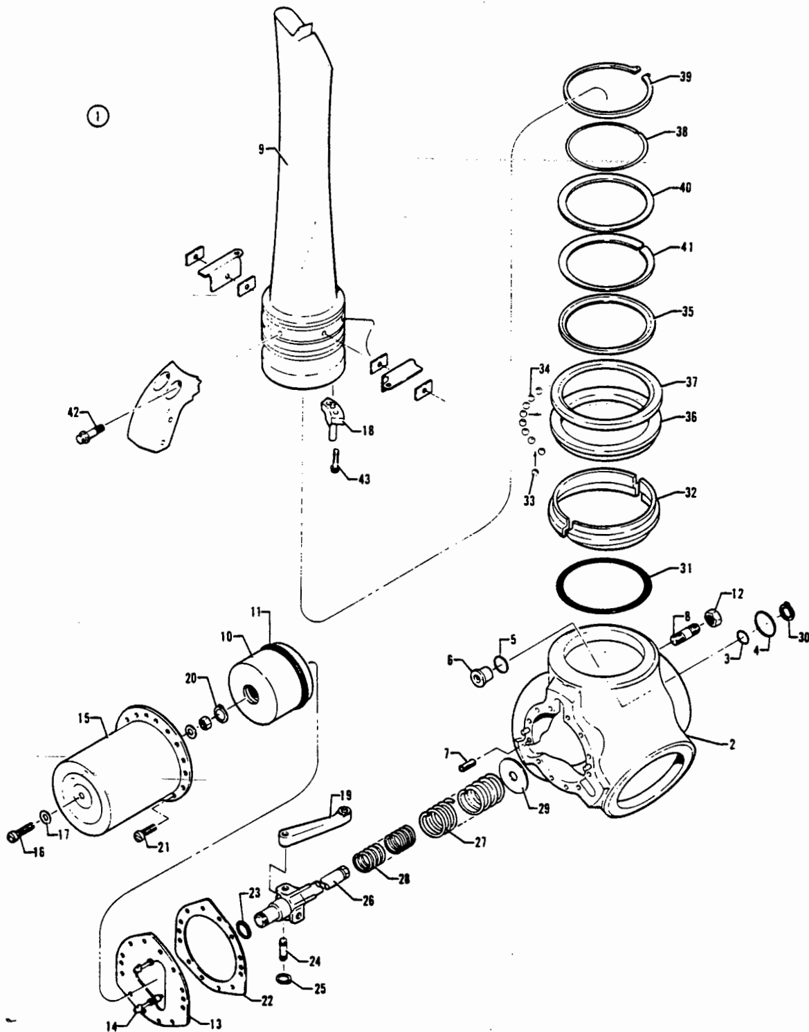
Figure 54B. Three Blade Propeller Assembly (McCauley) (Serial Nos. 34-7970001 and up)
