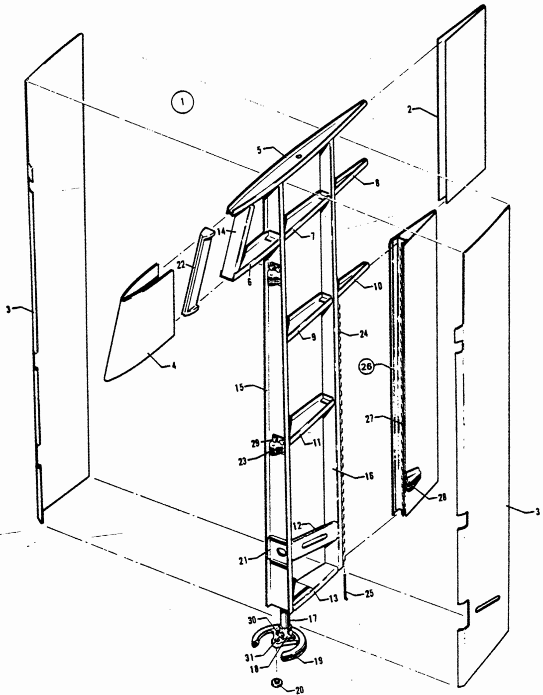
Figure 41. Rudder Assembly
