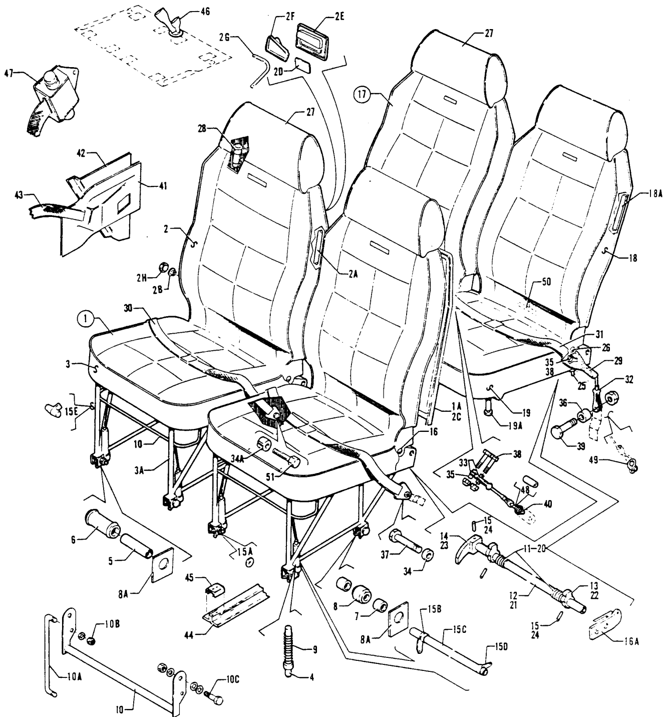
Figure 28A. Seats Installation (PA-28-140 - Serial Nos. 28-7125001and up) (PA-28-180 - Serial Nos. 28-7105001and up) (PA-28R-180 - Serial Nos. 28R-7130001and up) (PA-28R-200 - Serial Nos. 28R-7135001and up) (PA-28R-235 - Serial Nos. 28R-7110001and up)
