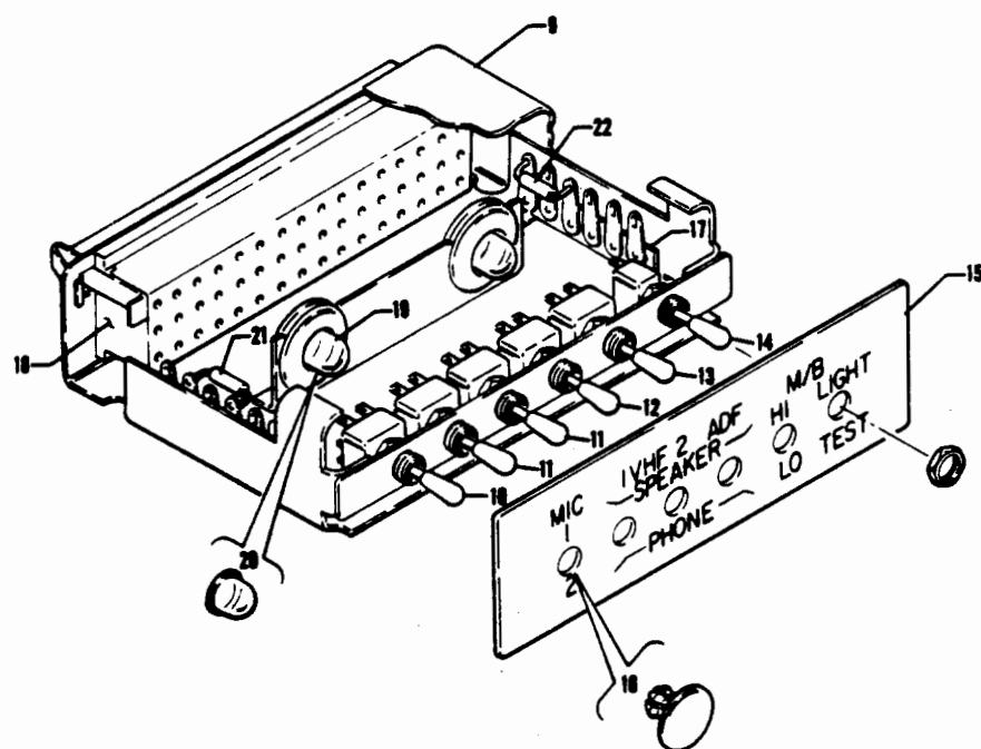
Figure 95. Radio Junction Boxes (PA-28-140 - Serial Nos. 28-25000 and up) (PA-28-180 - Serial Nos. 28-4378 and up) (PA-28R-180 - Serial Nos. 28R-30006 to 28R-30481 inclusive, 28R-30483 and up) (PA-28-235 - Serial Nos. 28-11040 and up) (PA-28R-200 - Serial Nos. 28R-30482, 28R-35001 and up)
