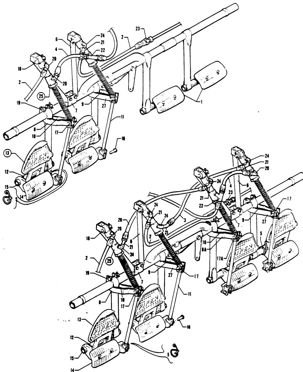
Figure 48. Toe Brake Installation
