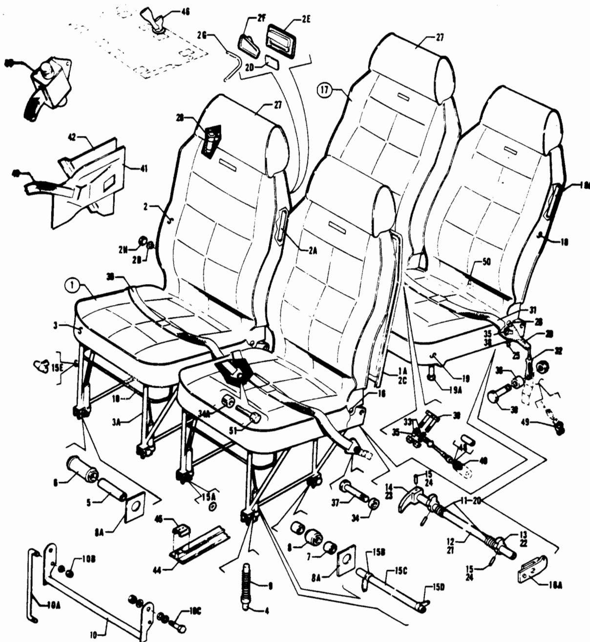
Figure 28A. Seats Installation
