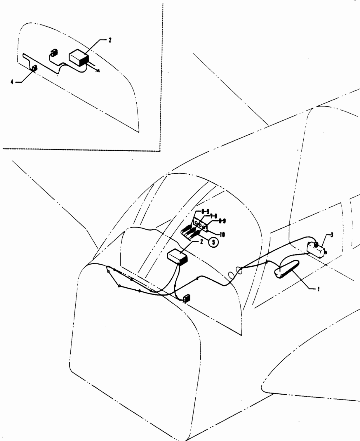
Figure 94. Piper PM-1 Marker Beacon Installation (PA-28-140 - Serial Nos. 28-25000 to 28-7425454 inclusive) (PA-28-150-160-180 - Serial Nos. 28-1761 to 28-7406290 inclusive) (PA-28-235 - Serial Nos. 28-10487 to 28-7410120 inclusive) (PA-28R-180 - Serial Nos. 28R-30005 to 28R-30481 inclusive, 28R-30483 to 28R-7130019 inclusive) (PA-28R-200 - Serial Nos. 28R-30482, 28R-35001 to 28R-7435331 inclusive)
