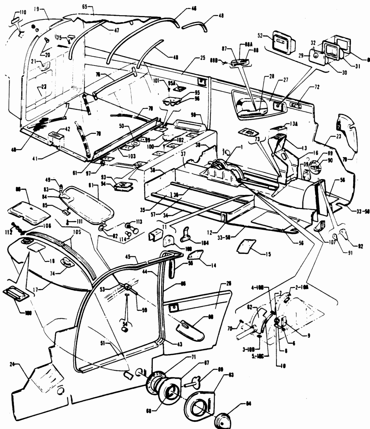
Figure 27. Cockpit Finishing Installation (PA-28-180 - Serial Nos. 28-4378 and up) (PA-28R-180 - Serial Nos. 28R-30005 to 28R-30482 inclusive, 28R-30483 and up) (PA-28R-200 - Serial Nos. 28R-30482, 28R-35001 and up)
