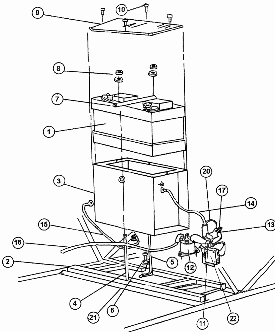
FIGURE 15 INSTALLATION - BATTERY
