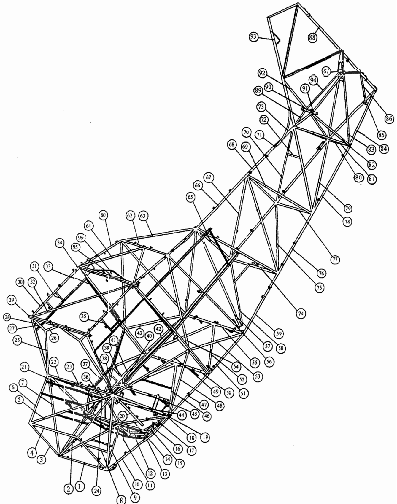
FIGURE 2 ASSEMBLY - FUSELAGE FRAME TUBES
