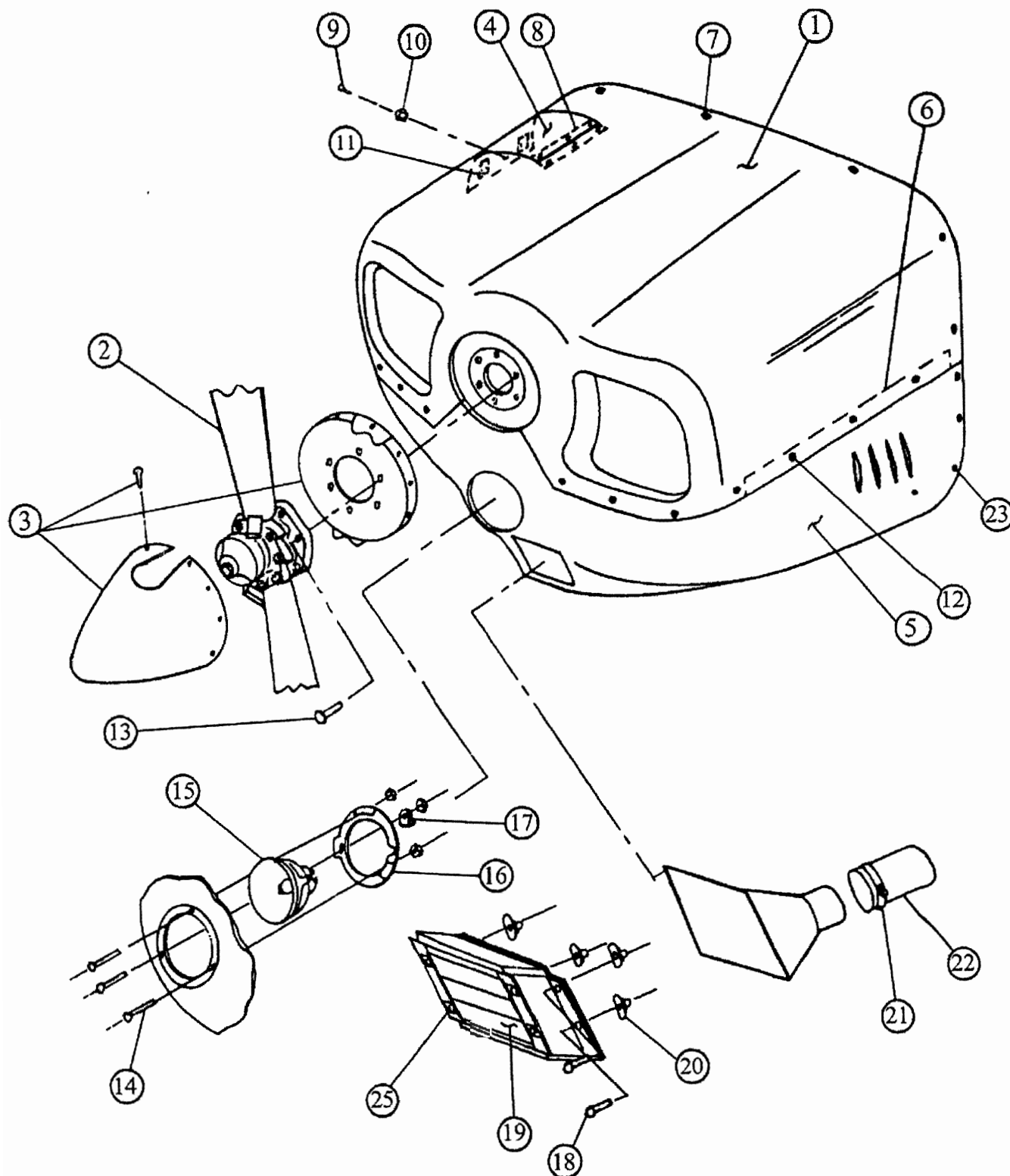
FIGURE 33 INSTALLATION - COWLING AND PROPELLER 180 HP CONSTANT SPEED
