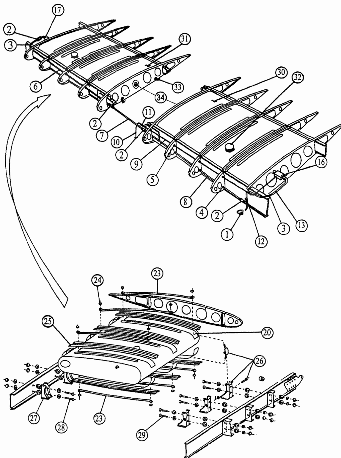
FIGURE 20 INSTALLATION – FUEL TANK AND FUEL VENT
