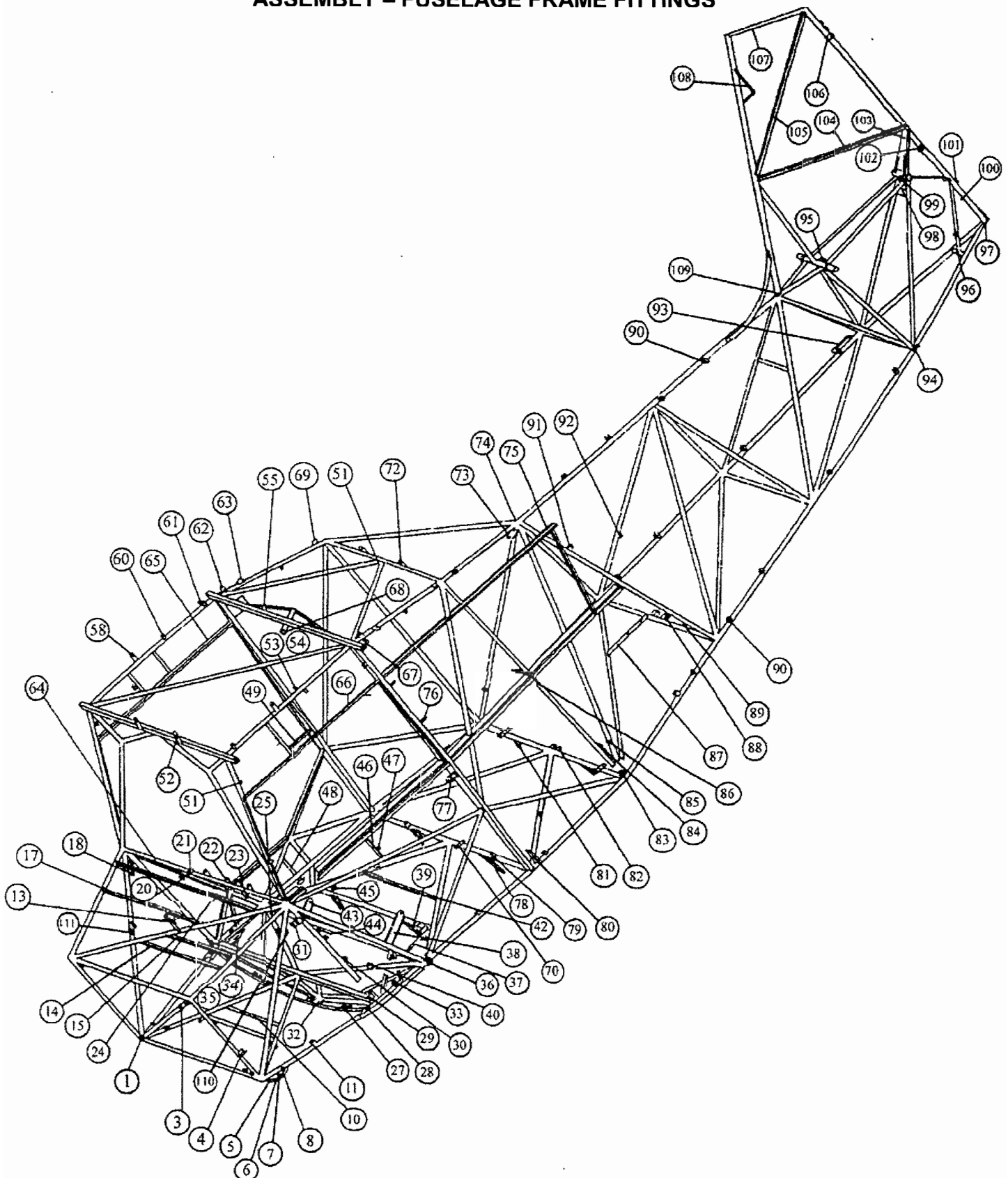
FIGURE 3 ASSEMBLY – FUSELAGE FRAME FITTINGS
