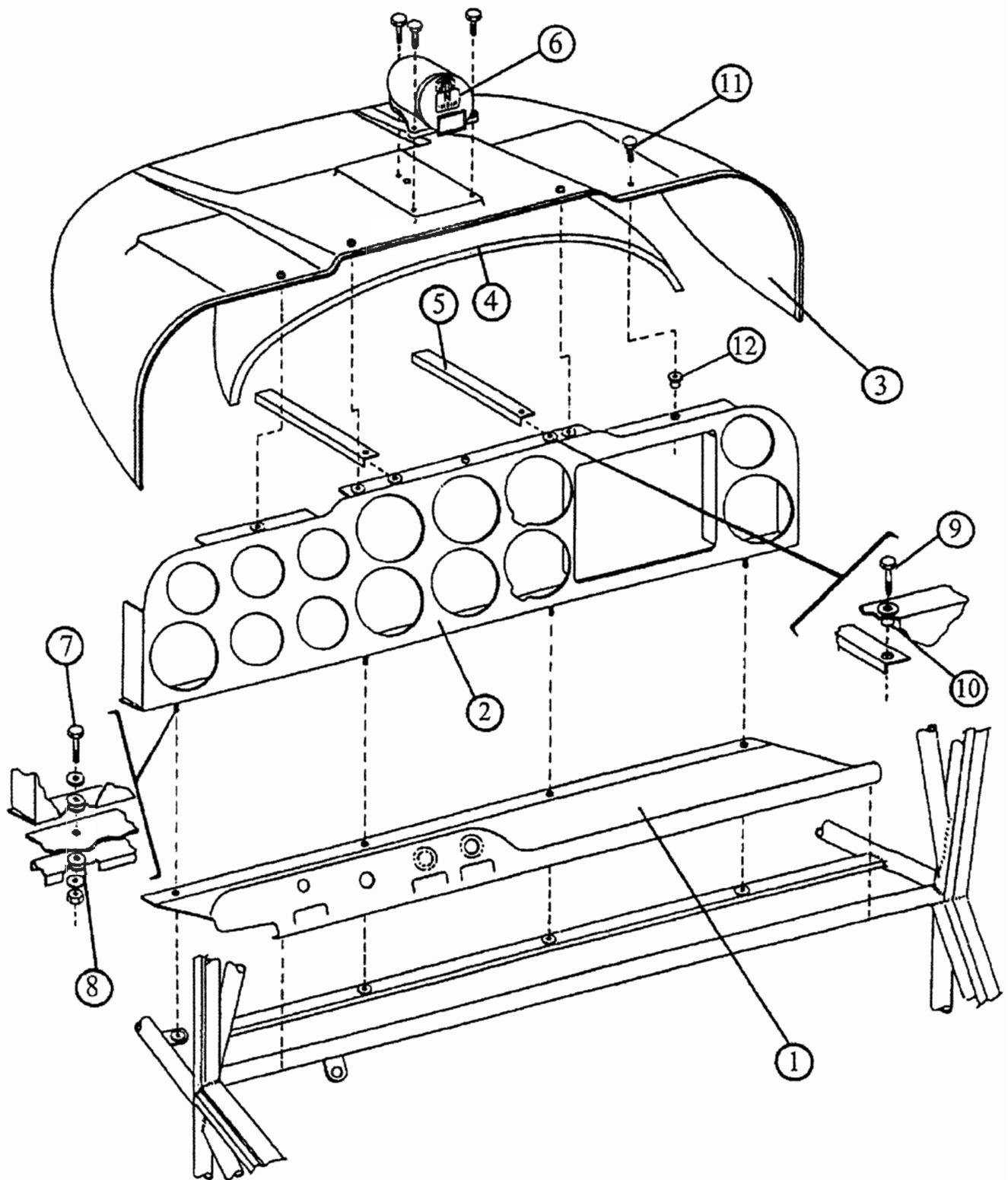
FIGURE 7 INSTALLATION - INSTRUMENT PANEL
