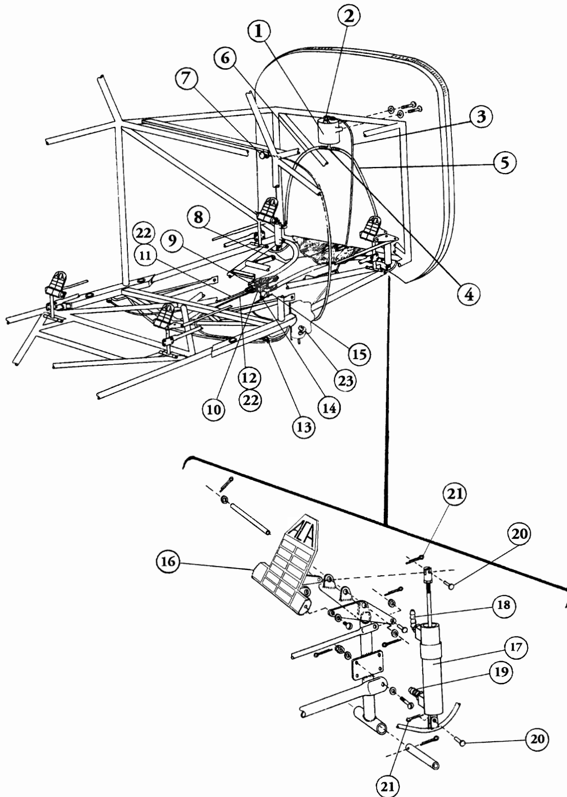
FIGURE 17 INSTALLATION - TOE BRAKE SYSTEM
