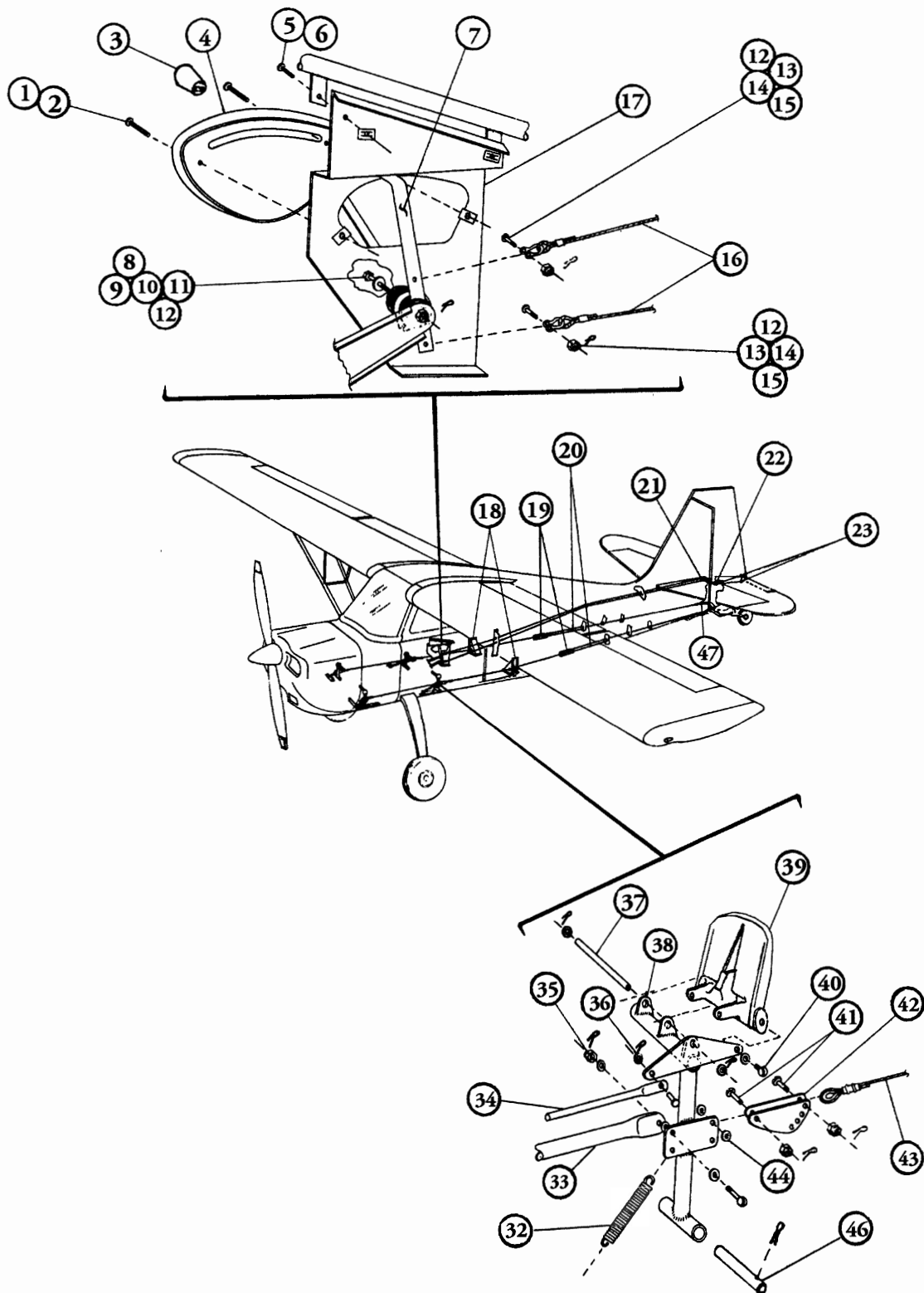
FIGURE 5 INSTALLATION – RUDDER AND TRIM CONTROLS
