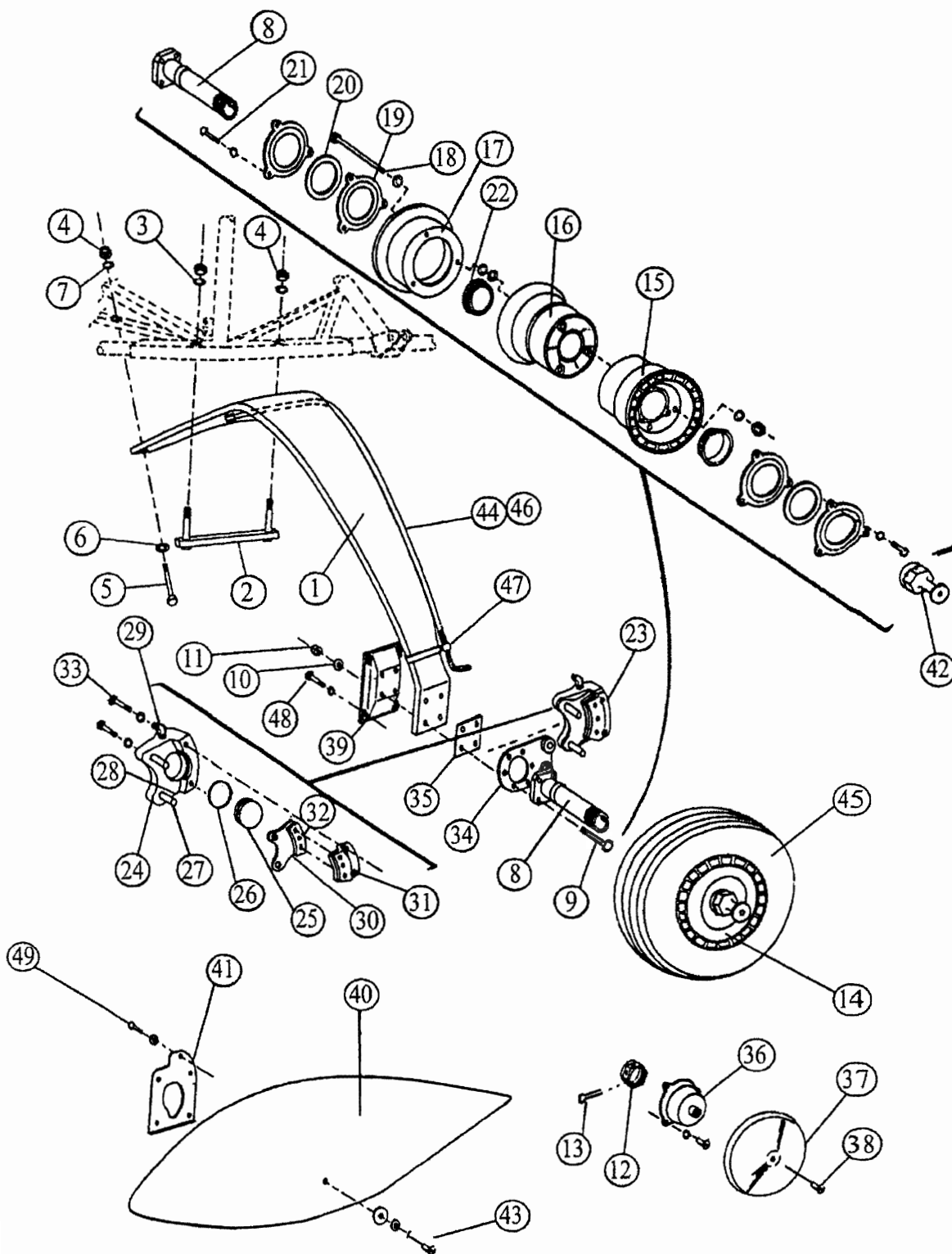
FIGURE 22 INSTALLATION - LANDING GEAR - CLEVELAND BRAKES
