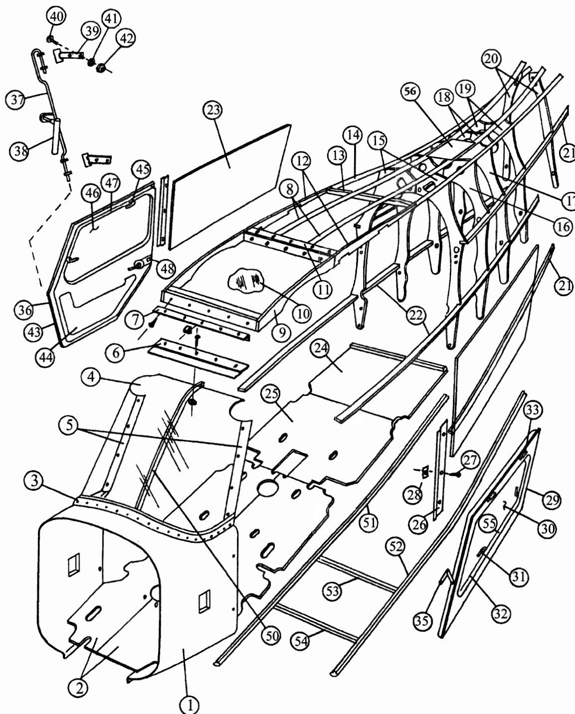
FIGURE 10 INSTALLATION – PRIMARY FUSELAGE EQUIPMENT
