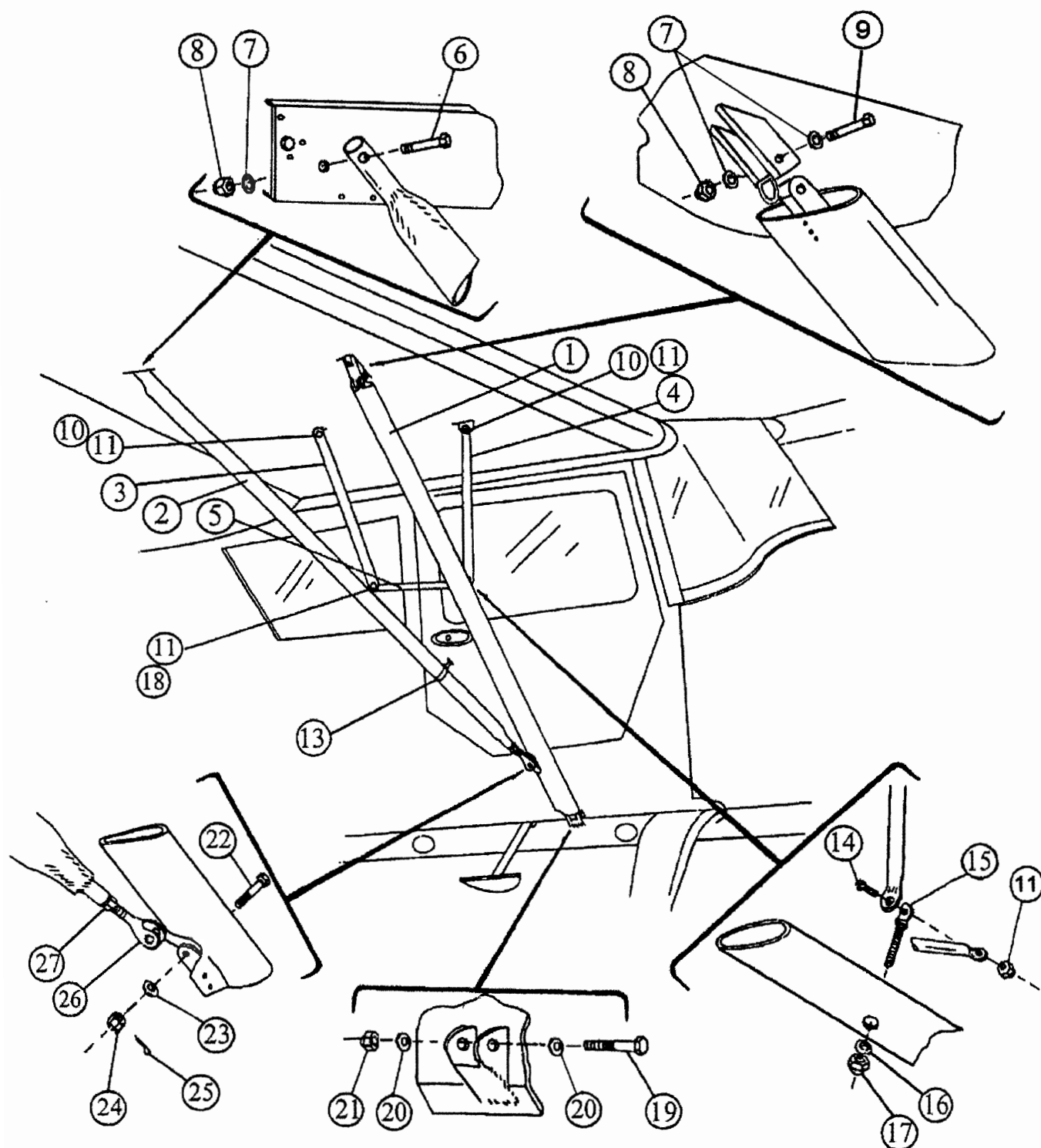
FIGURE 26 INSTALLATION - WING STRUTS
