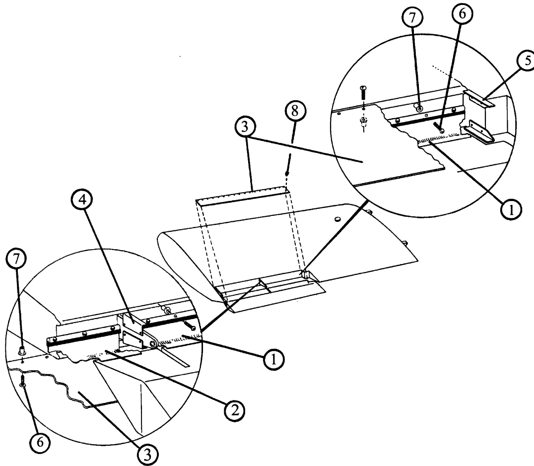
FIGURE 25 INSTALLATION – AILERON GAP COVERS AND SEALS
