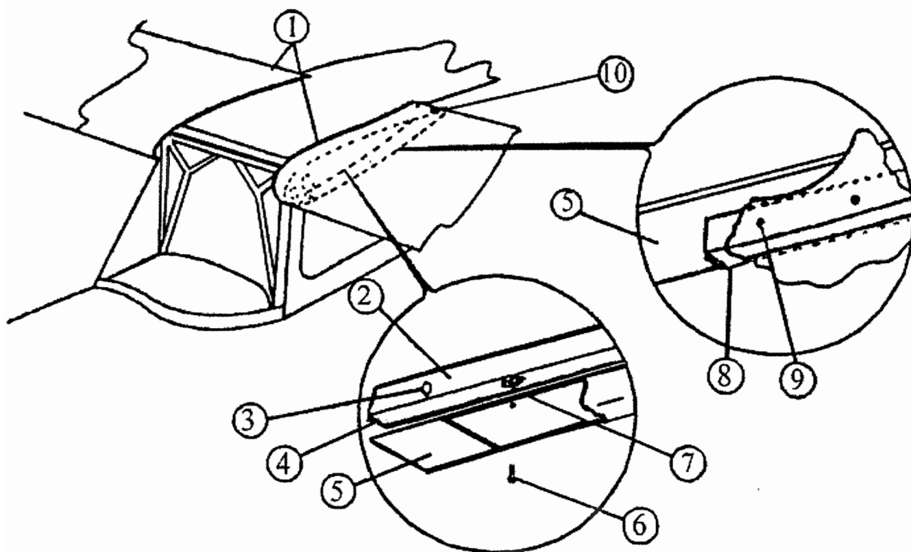
FIGURE 27 INSTALLATION - GAP COVERS
