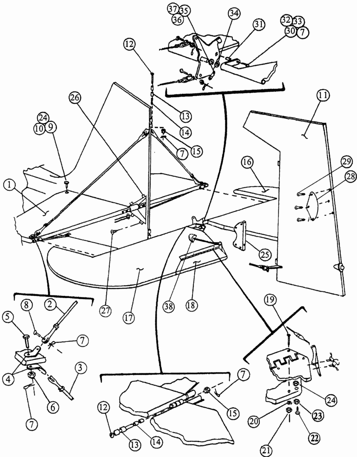
FIGURE 28 INSTALLATION - TAIL SURFACES
