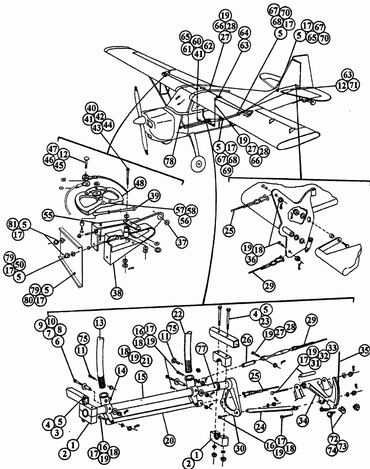
FIGURE 4 INSTALLATION - ELEVATOR AND AILERON CONTROLS
