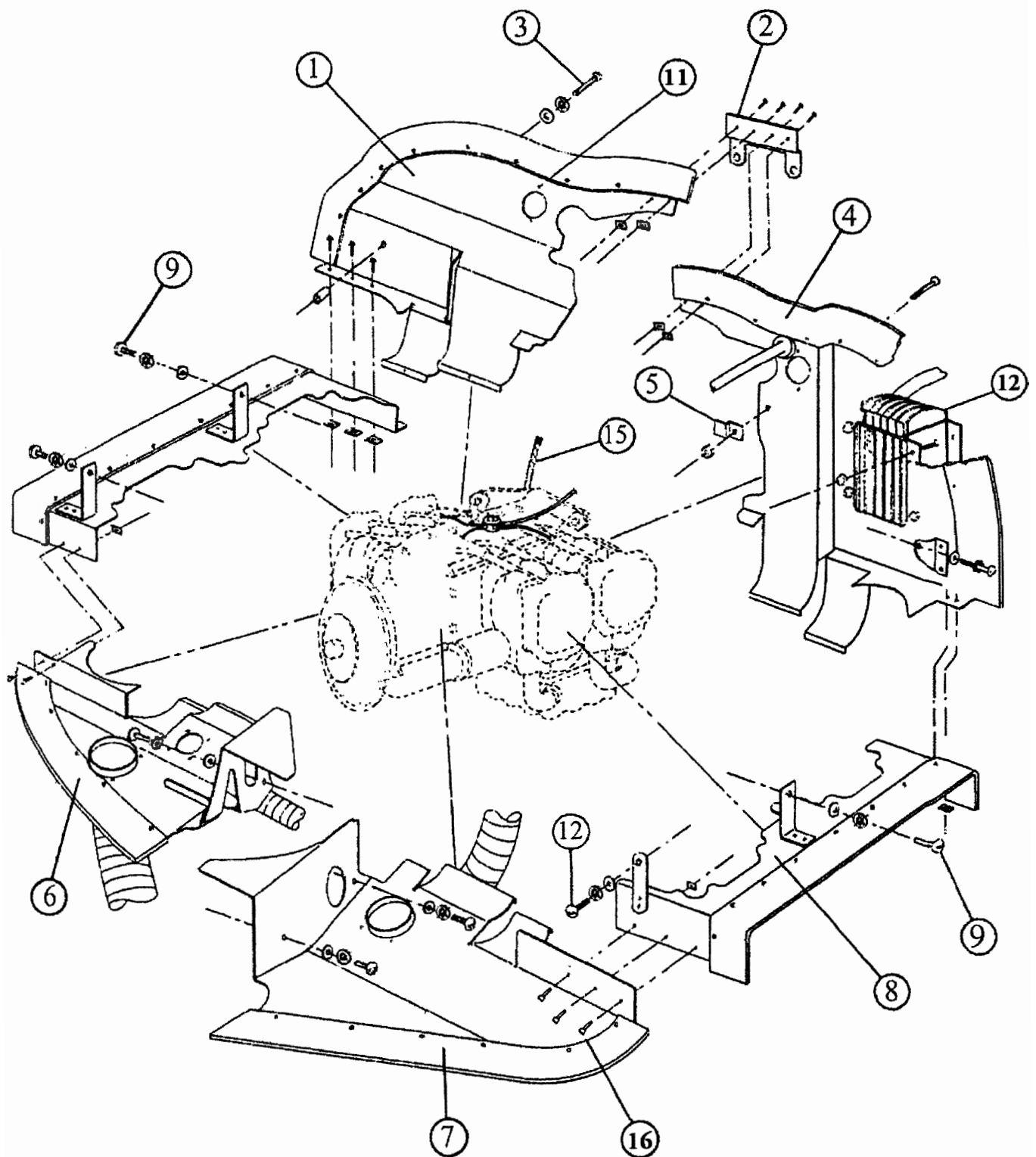
FIGURE 29 INSTALLATION – ENGINE Baffles AND OIL COOLER AEIO-360-H1A
