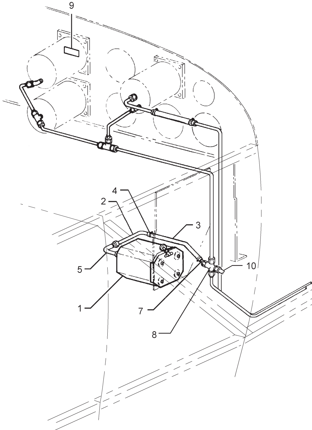
Figure 74. Encoder Installation (AR-850)(AK-350)
