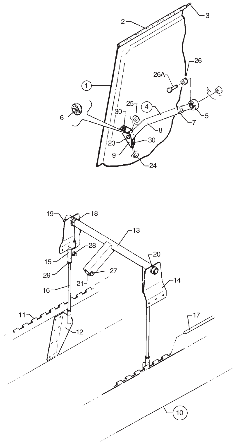
Figure 29. Landing Gear Door Installation
