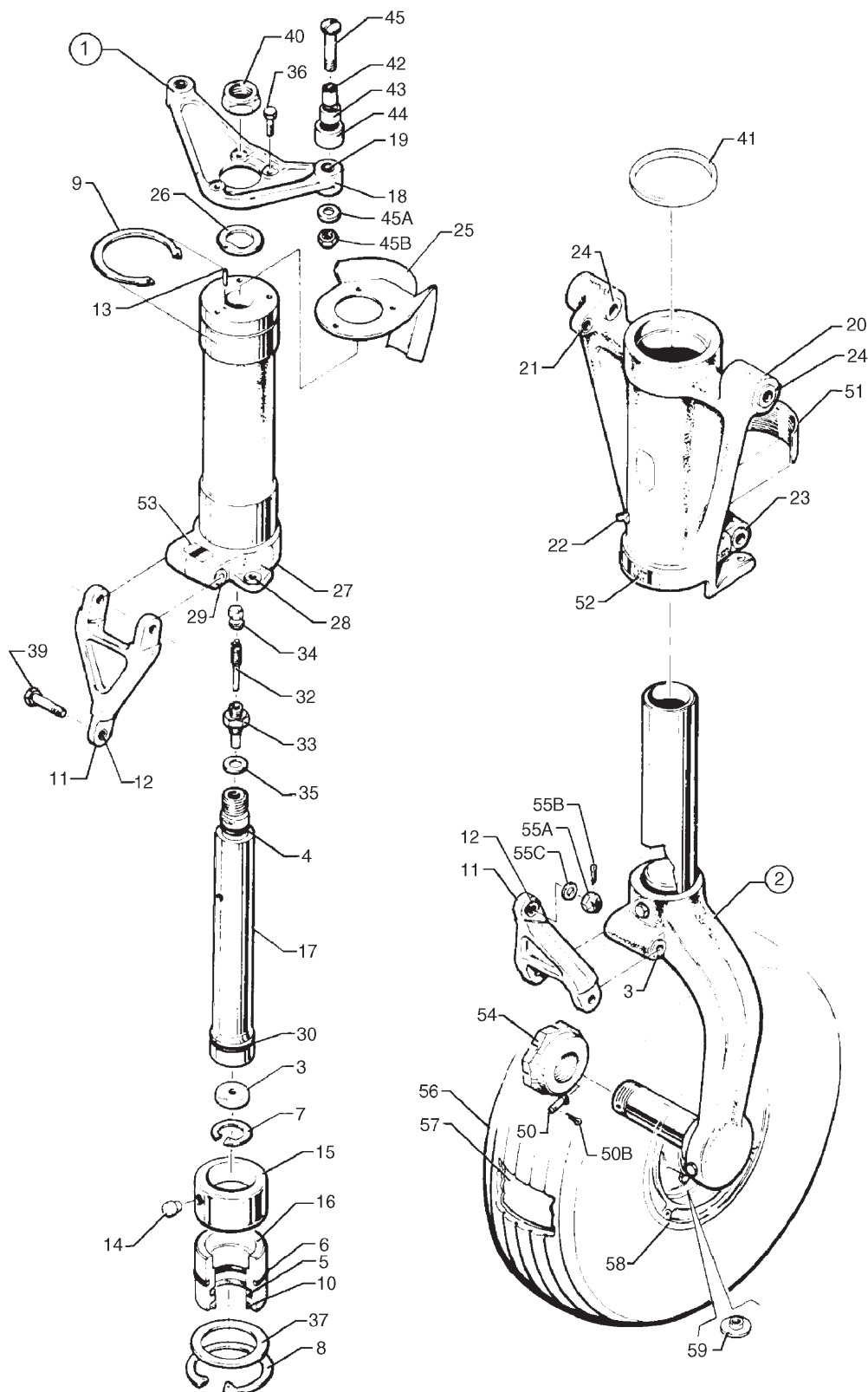
Figure 22. Nose Gear Assembly
