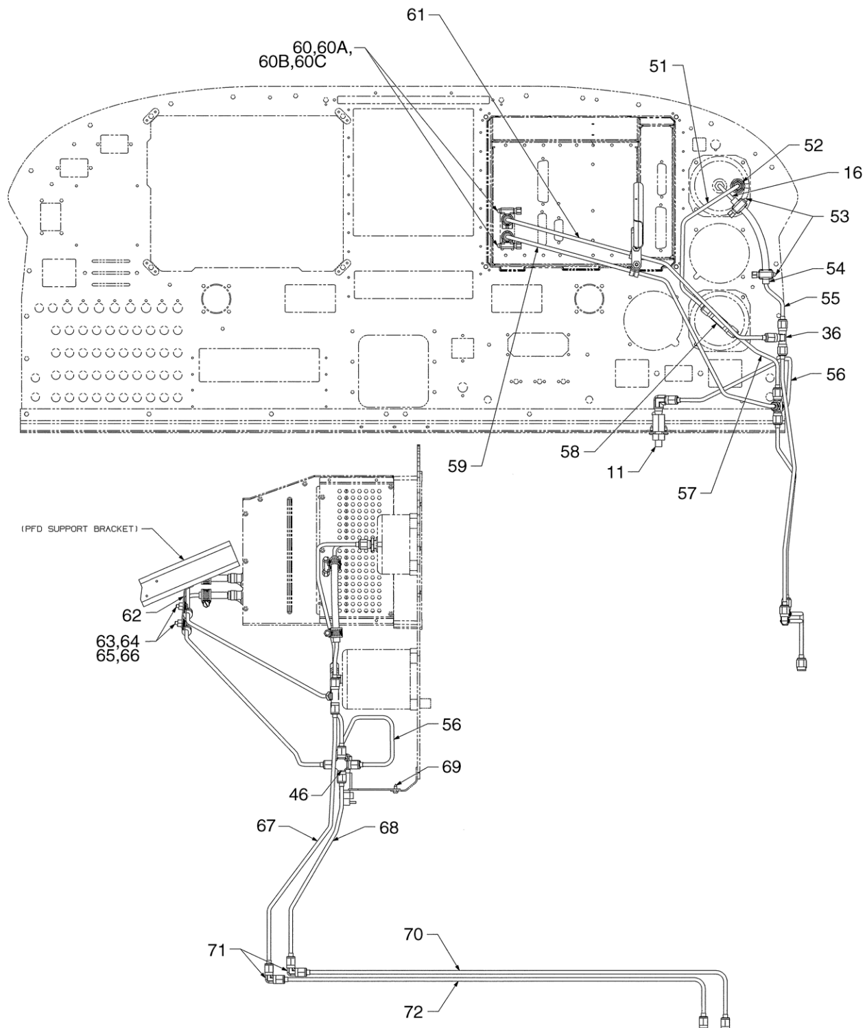
Figure 39. Pitot Static System Installation (with Entegra) (Sheet 2 of 2)
