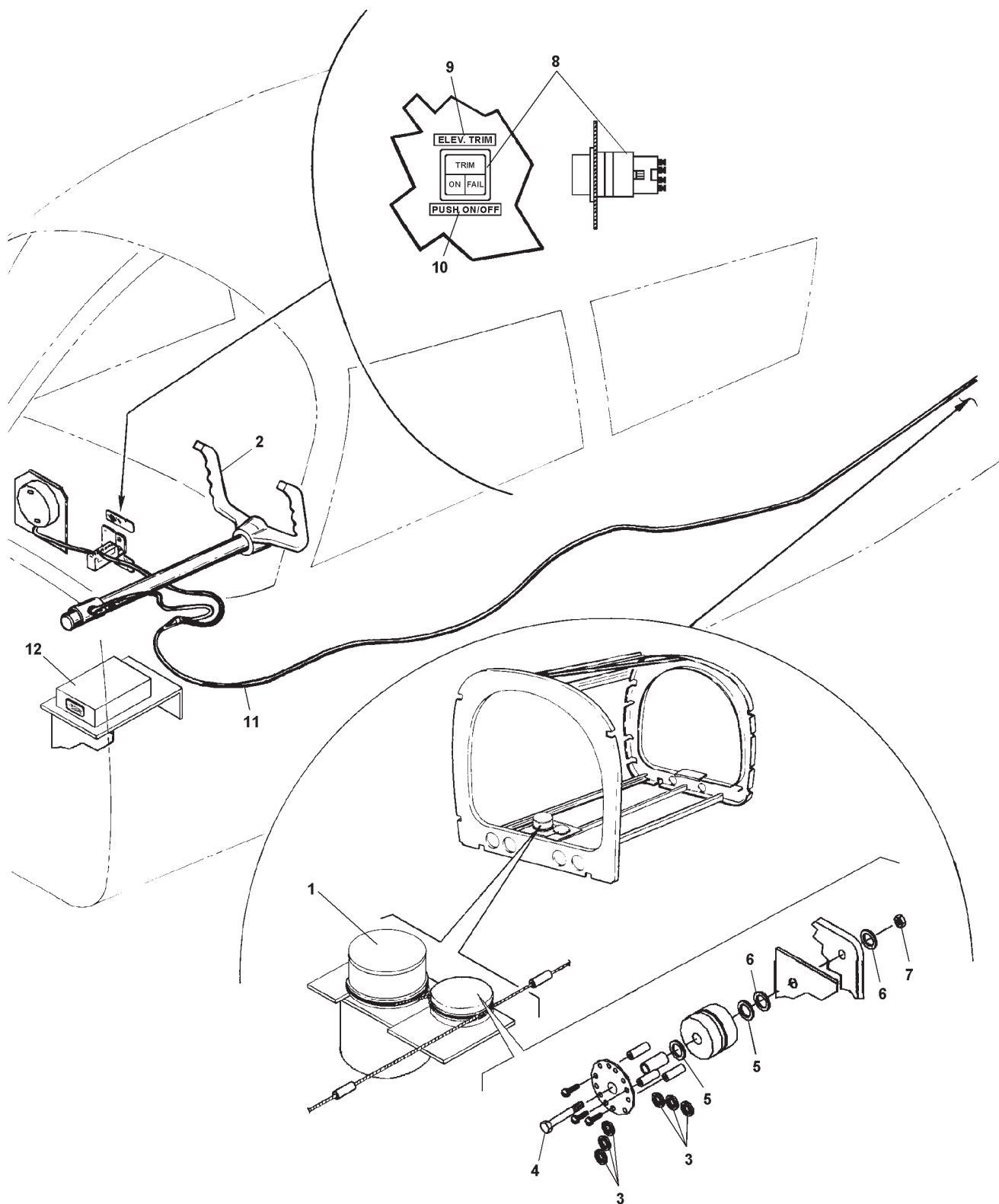
Figure 72. Manual Electric Trim Installation
