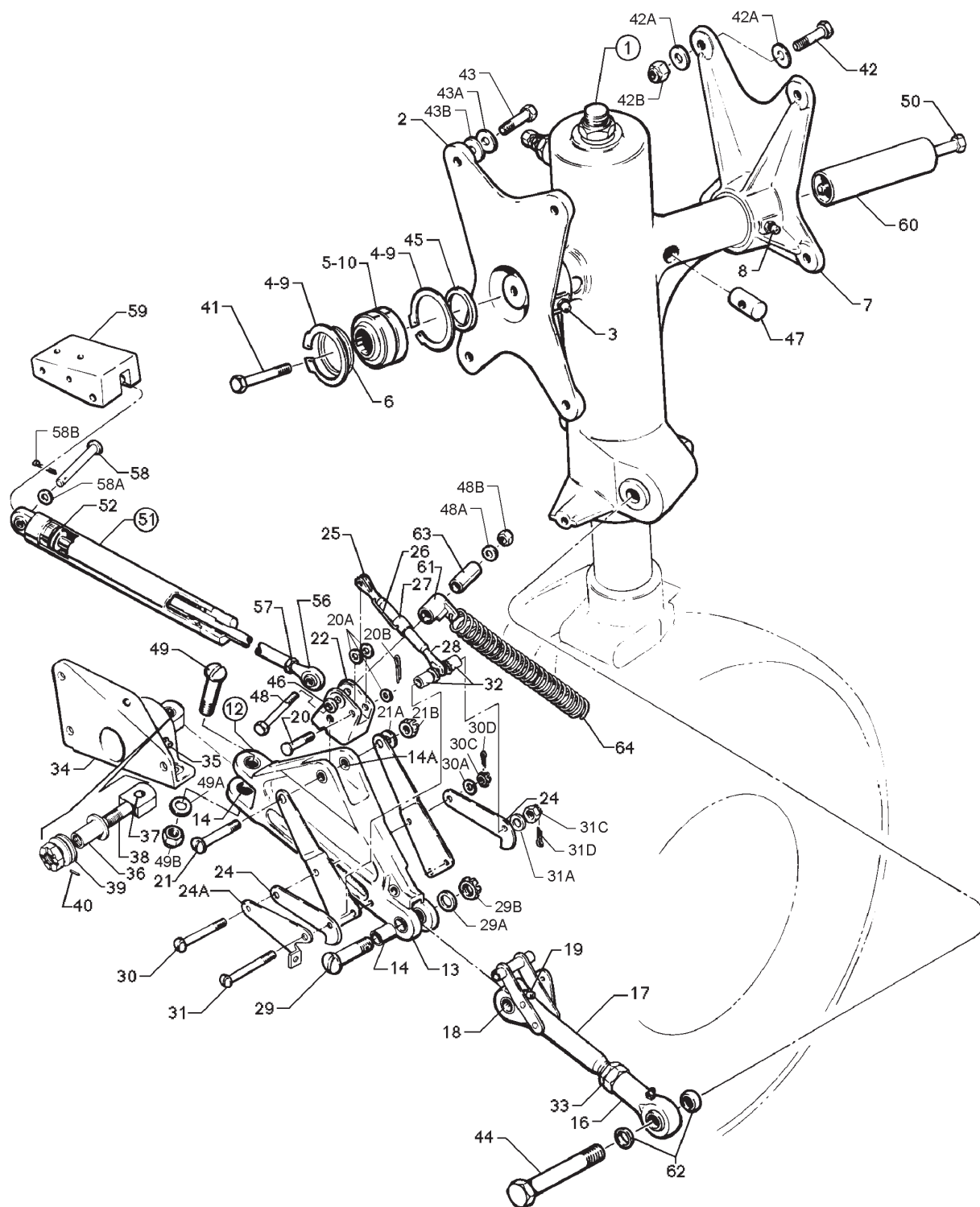
Figure 25. Main Gear Installation
