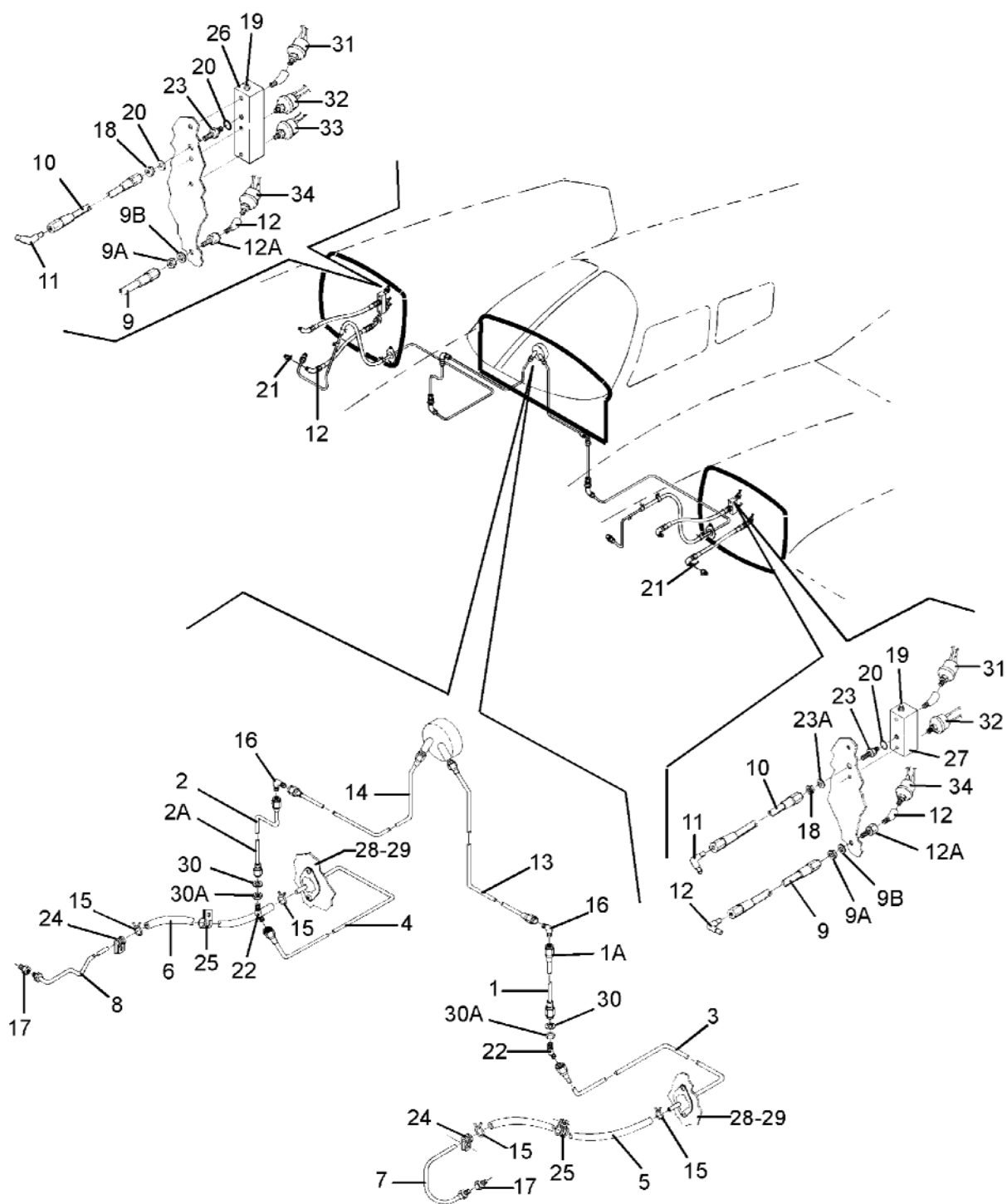
Figure 41. Engine Instrument Lines Installation
