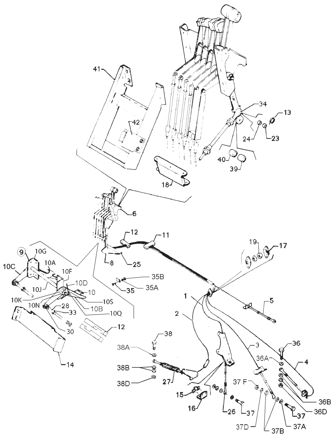
Figure 48. Engine Controls Installation
