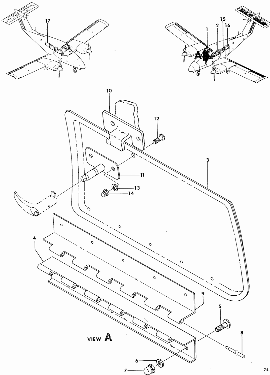
FIGURE 10-01.CABIN WINDOW INSTALLATION
