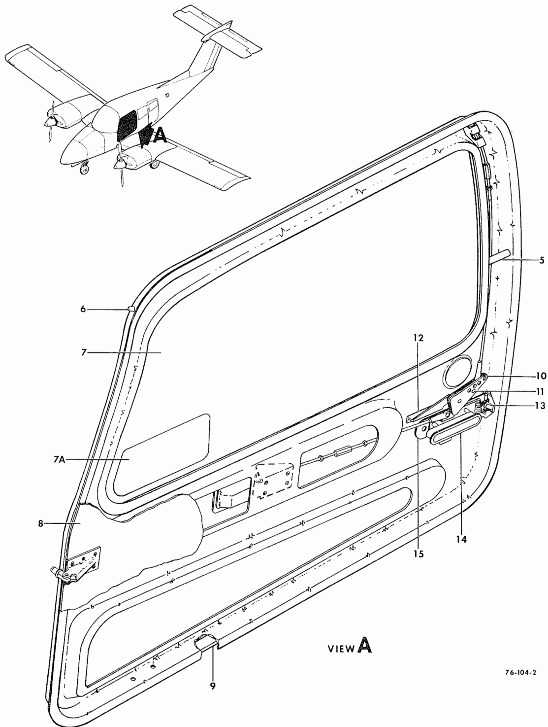
FIGURE 10-01.CABIN DOOR /SHEET 2 OF 3 SHEETS/
