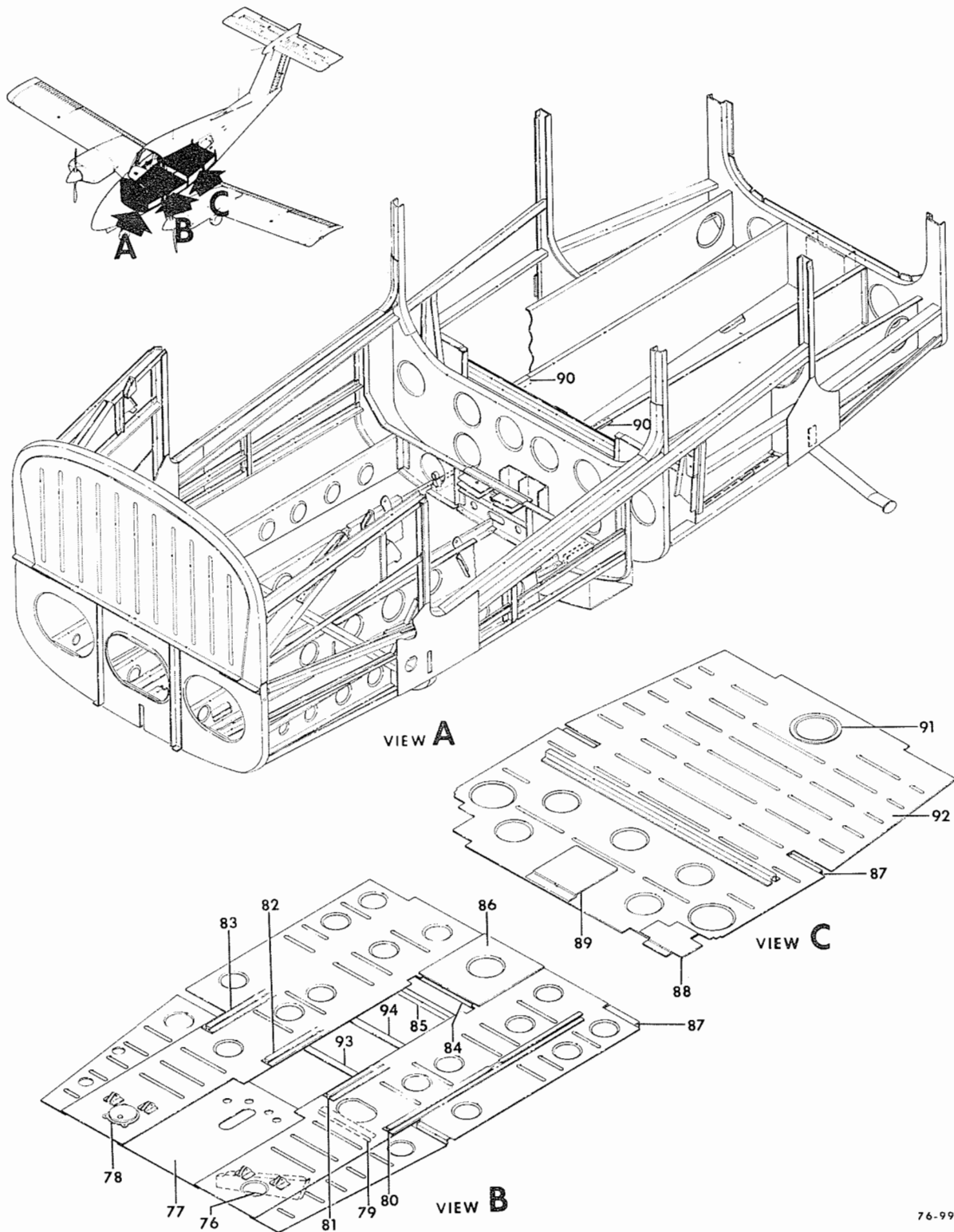
FIGURE 12-01. LOWER CABIN STRUCTURE /SHEET 4 OF 4 SHEETS/
