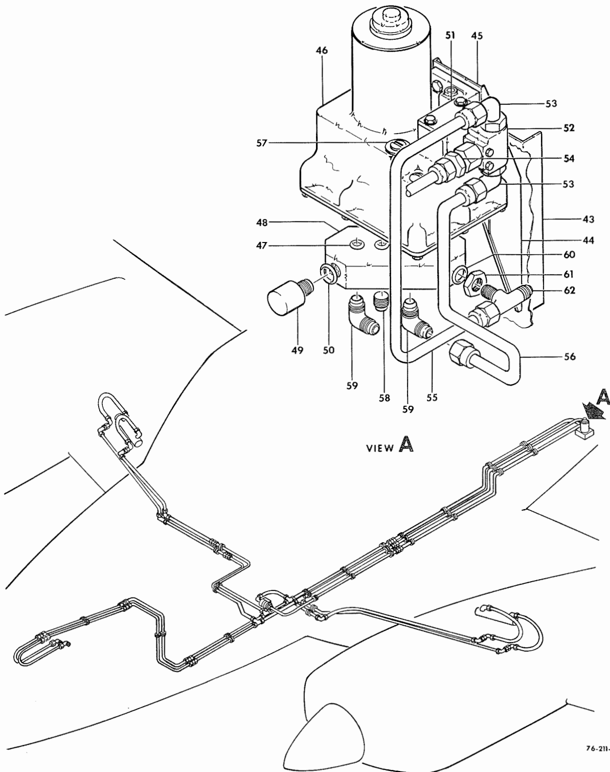
FIGURE 30-01. LANDING GEAR EXTENSION & RETRACT /SHEET 3 OF 3 SHEETS/
