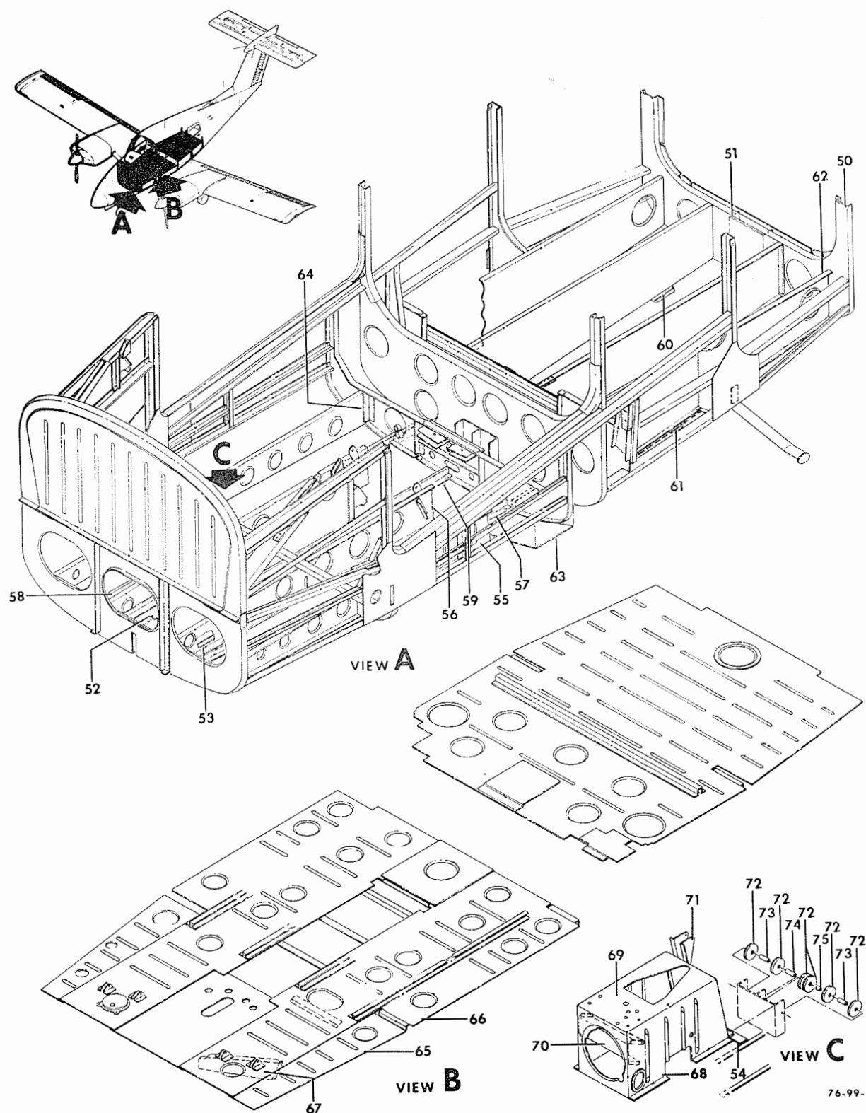
FIGURE 12-01. LOWER FUSELAGE STRUCTURE /SHEET 3 OF 4 SHEETS/
