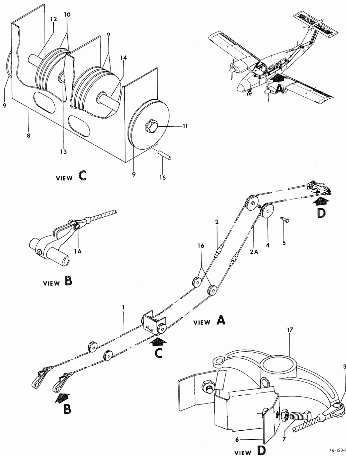
FIGURE 20-01. RUDDER CONTROLS
