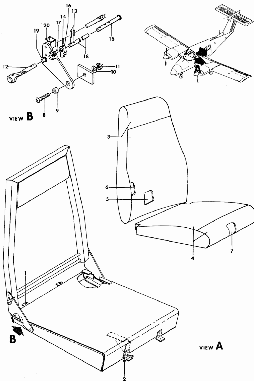
FIGURE 21-01. PASSENGER SPLIT SEATS /SHEET 1 OF 2 SHEETS/
