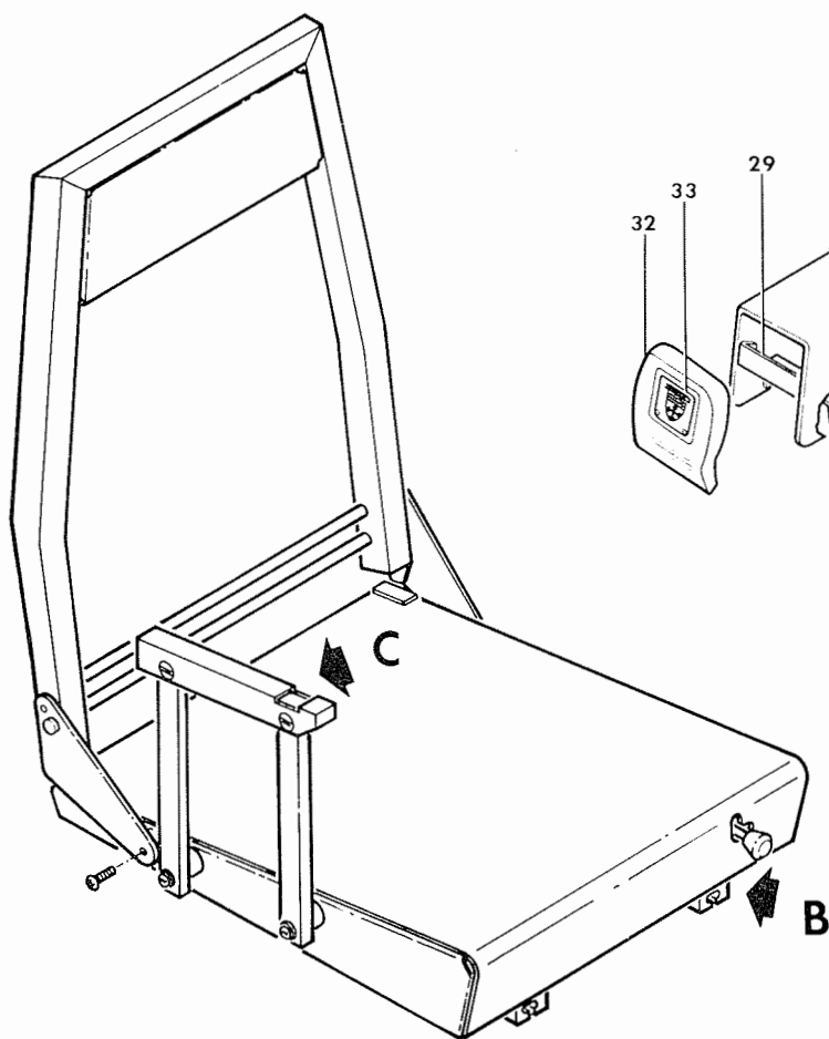
VIEW A
