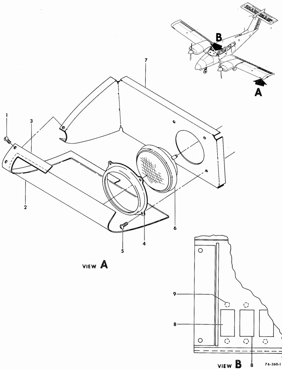
FIGURE 40-01.LANDING AND TAXI LIGHTS
