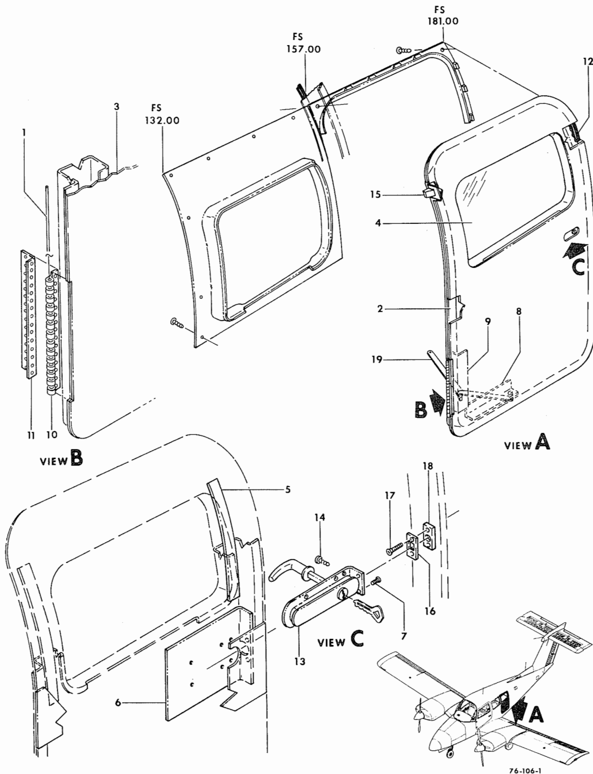
FIGURE 30-01.BAGGAGE DOOR
