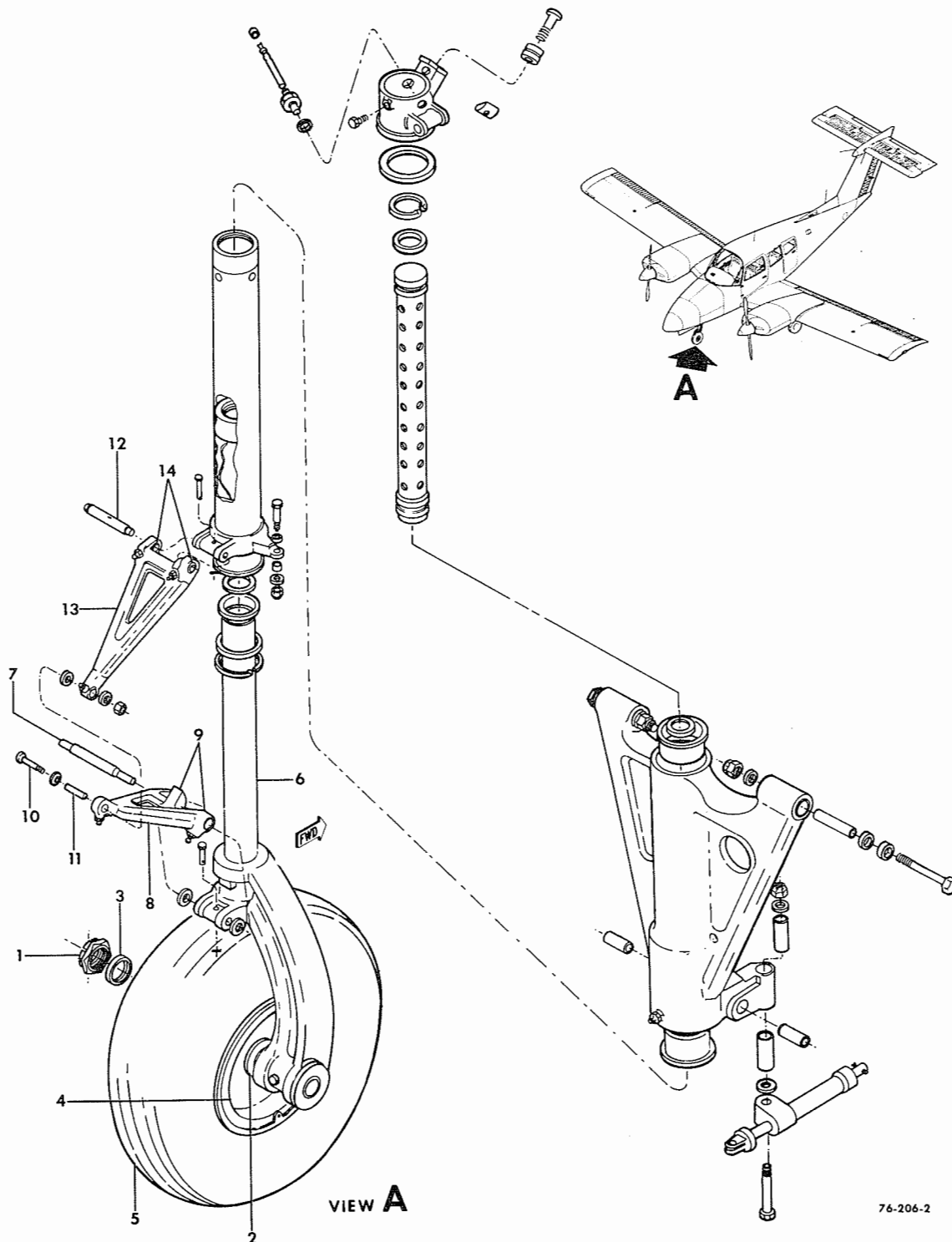
FIGURE 20-10. NOSE LANDING GEAR ASSEMBLY /SHEET 1 OF 2 SHEETS/
