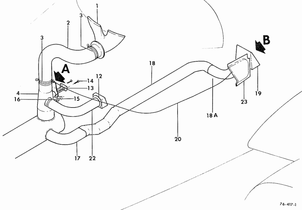
FIGURE 20-01.CABIN HEAT DUCTS
