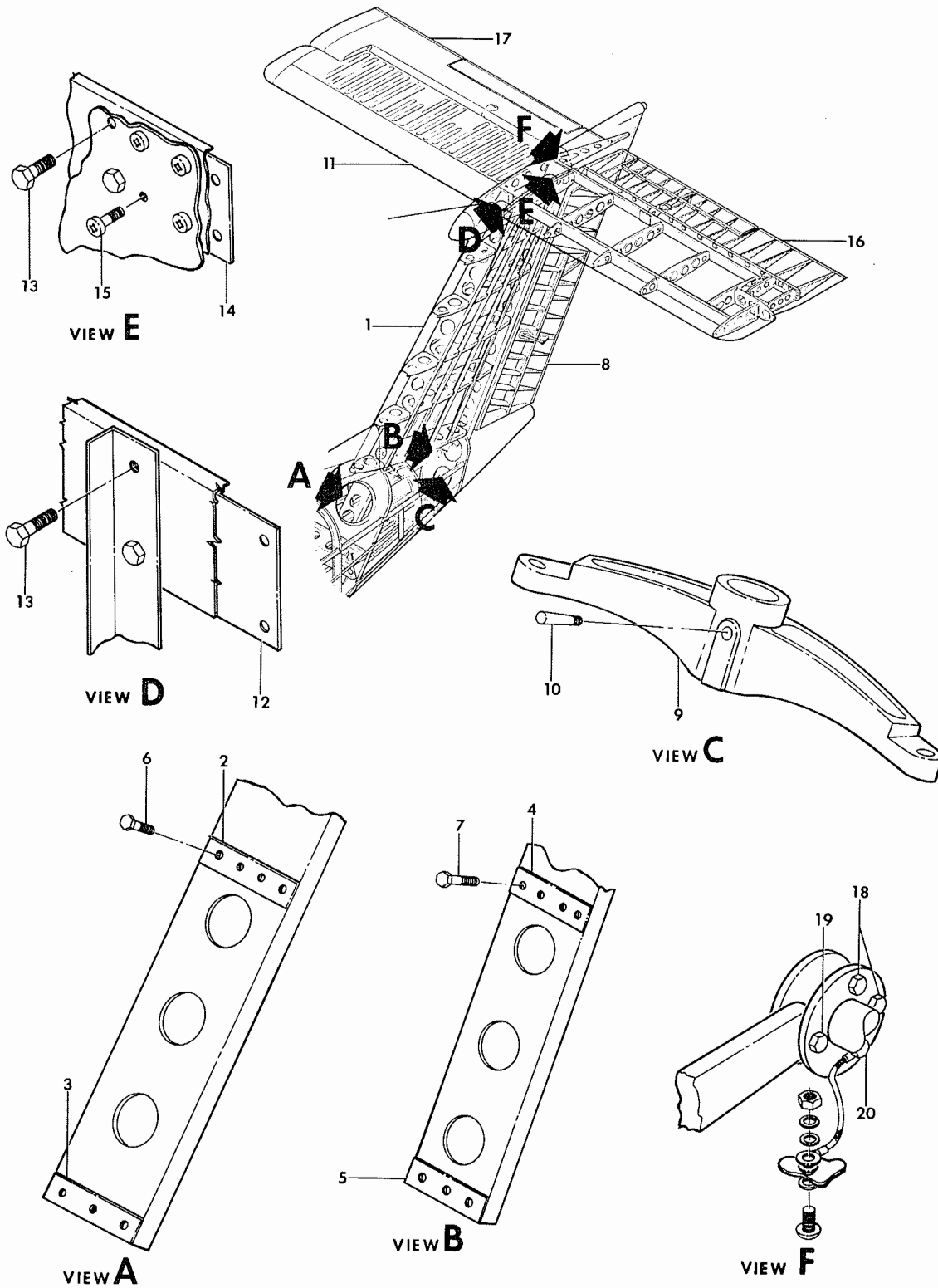
FIGURE 00-01. EMPENNAGE INSTALLATION /SHEET 1 OF 2 SHEETS/
