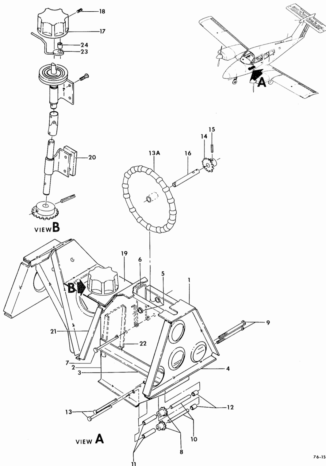
FIGURE 25-01. TRIM TAB CONTROLS /SHEET 1 OF 3 SHEETS/
