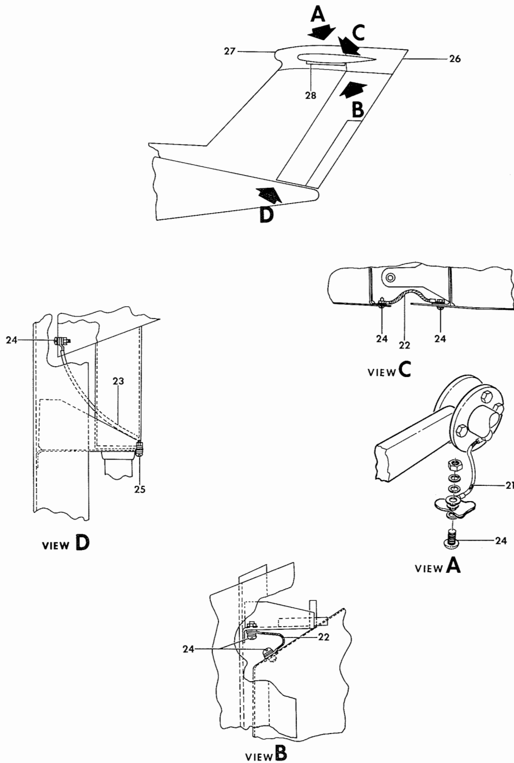
FIGURE 00-01. EMPENNAGE INSTALLATION /SHEET 2 OF 2 SHEETS/
