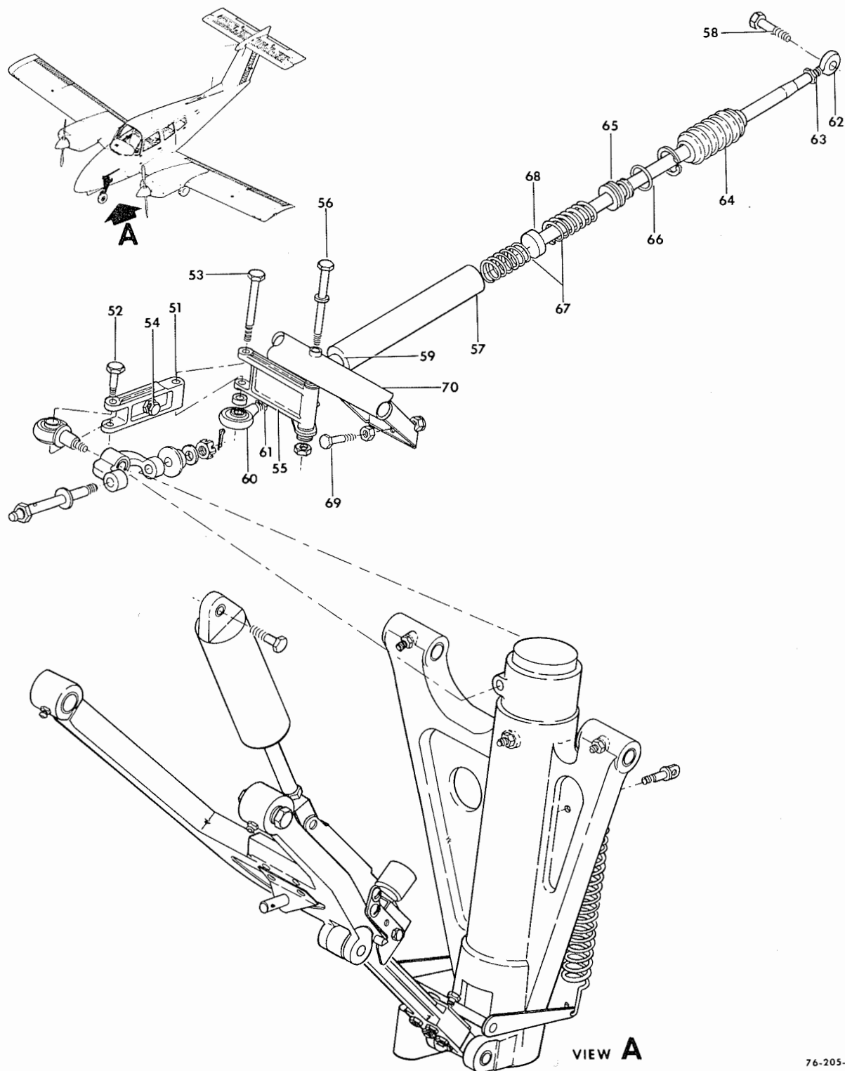
FIGURE 20-01, NOSE LANDING GEAR INSTALLATION /SHEET 4 OF 4 SHEETS/
