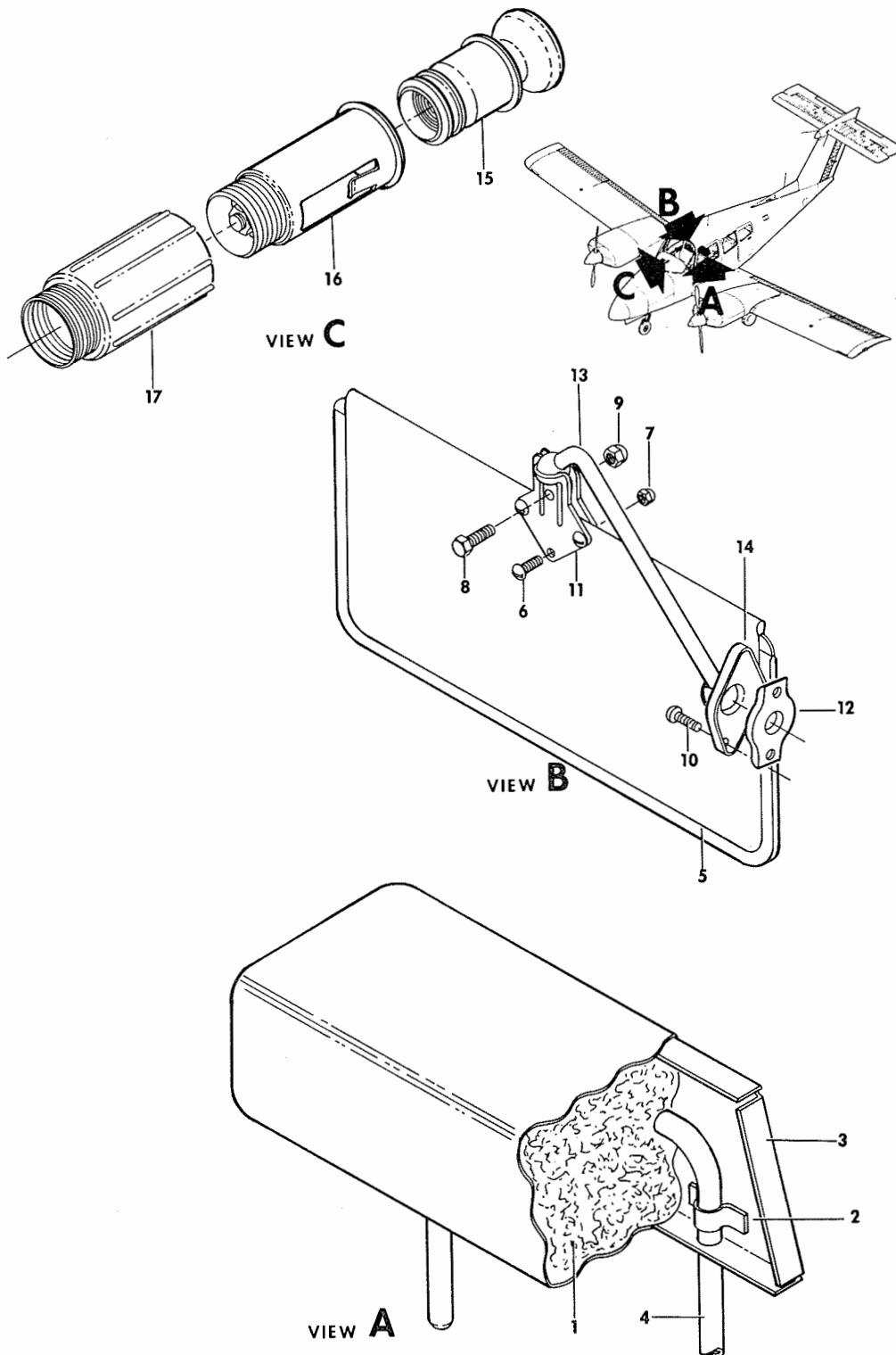
FIGURE 11-01.CABIN FURNISHINGS /SHEET 1 OF 2 SHEETS/
