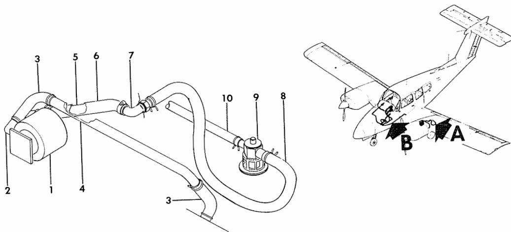
VIEW A
