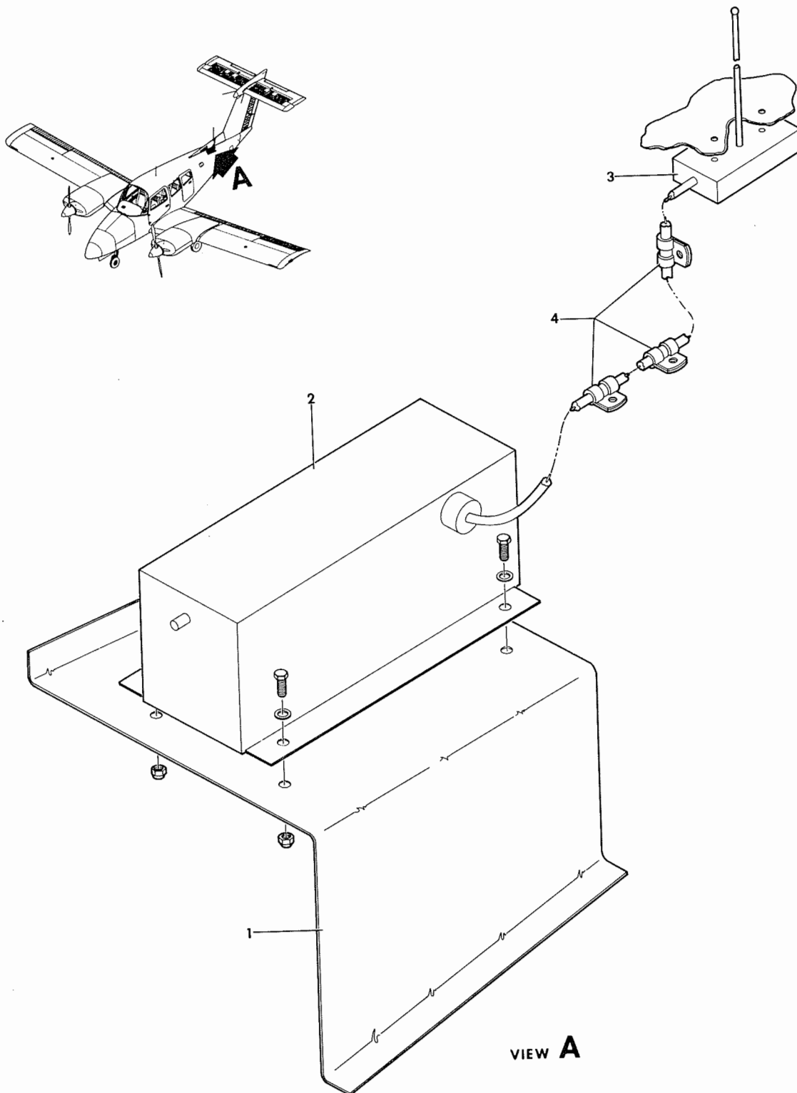
FIGURE 60-01. EMERGENCY LOCATOR TRANSMITTER
