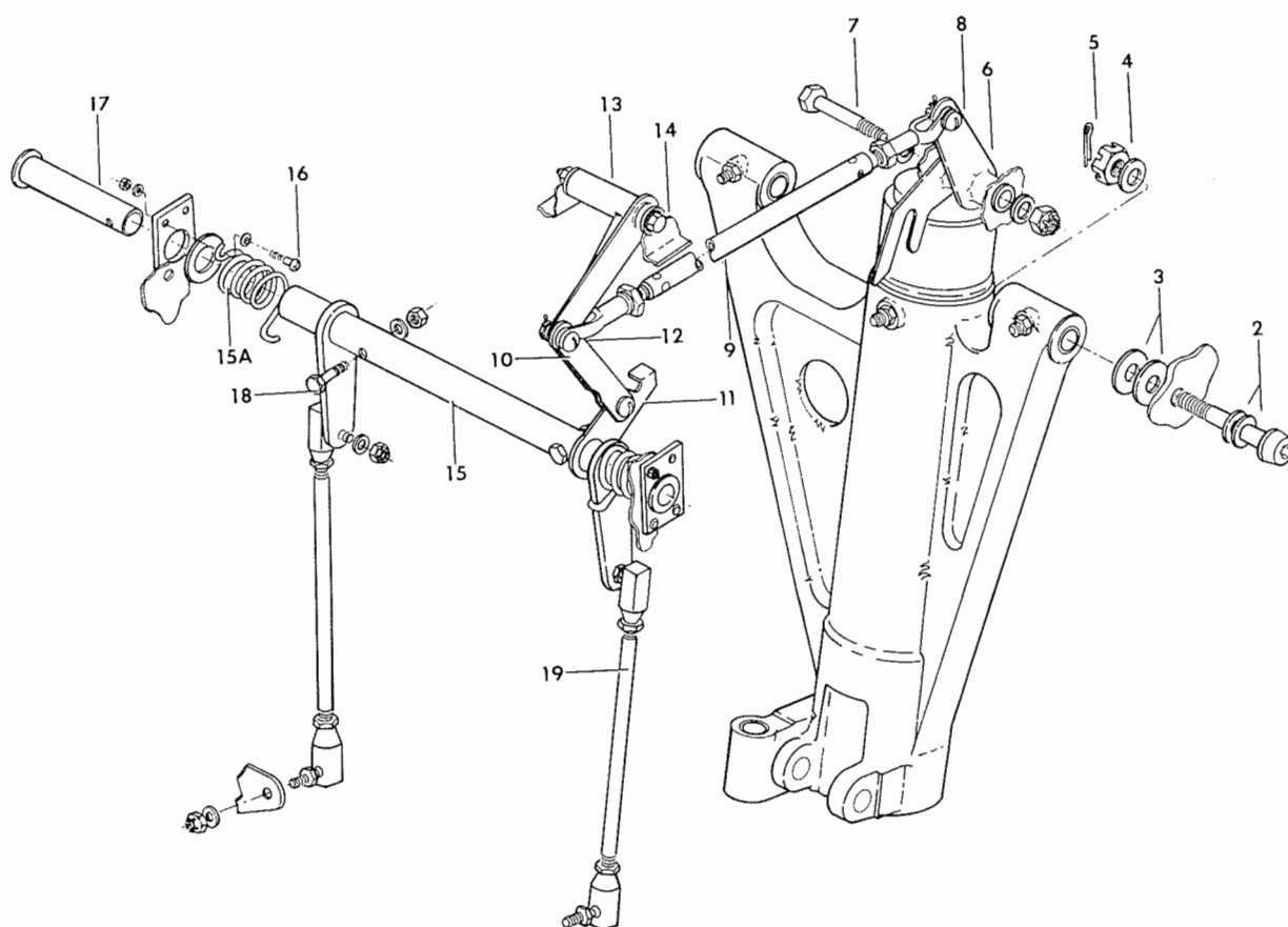
VIEW A
