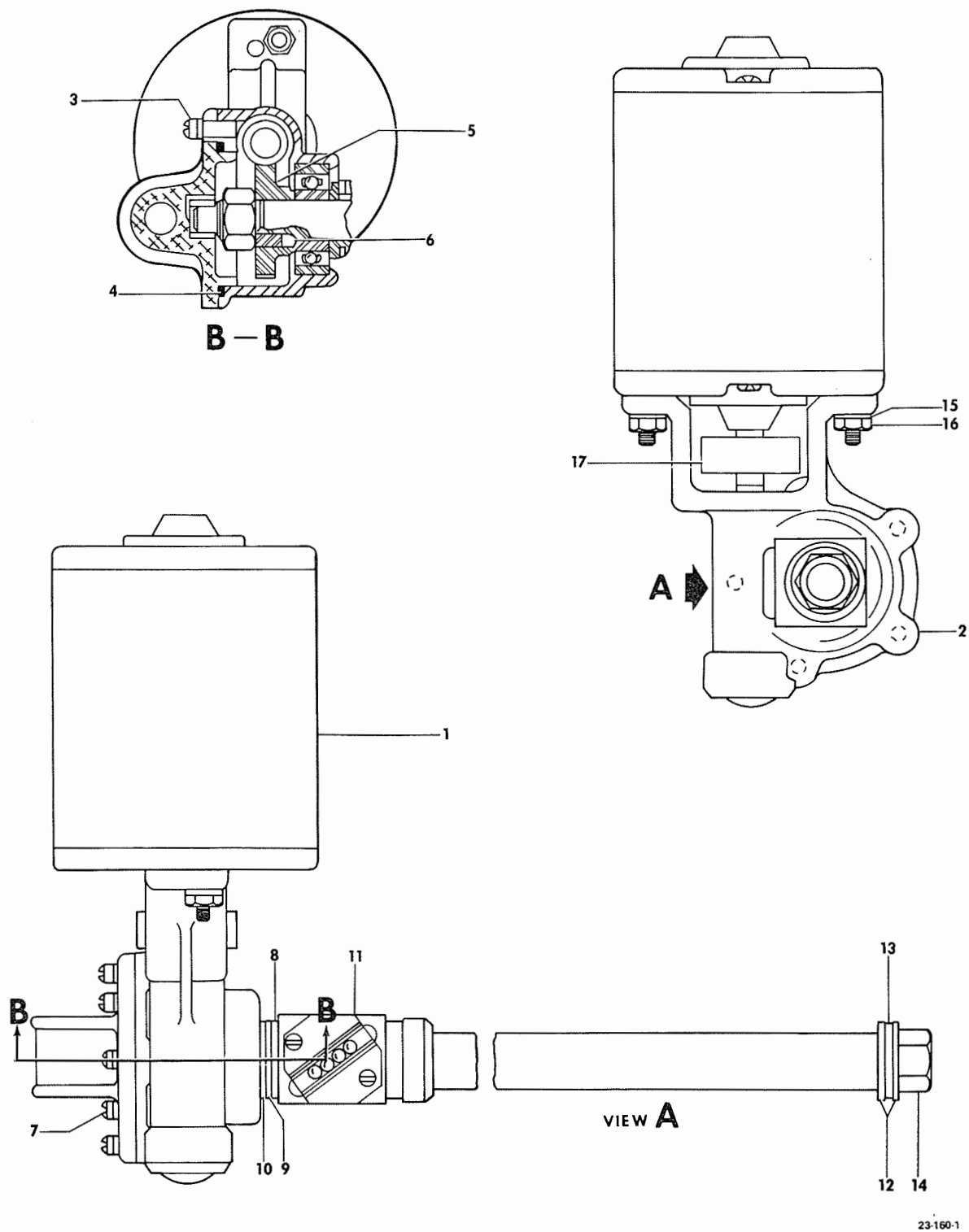
FIGURE 50-10. FLAP MOTOR & GEARBOX
