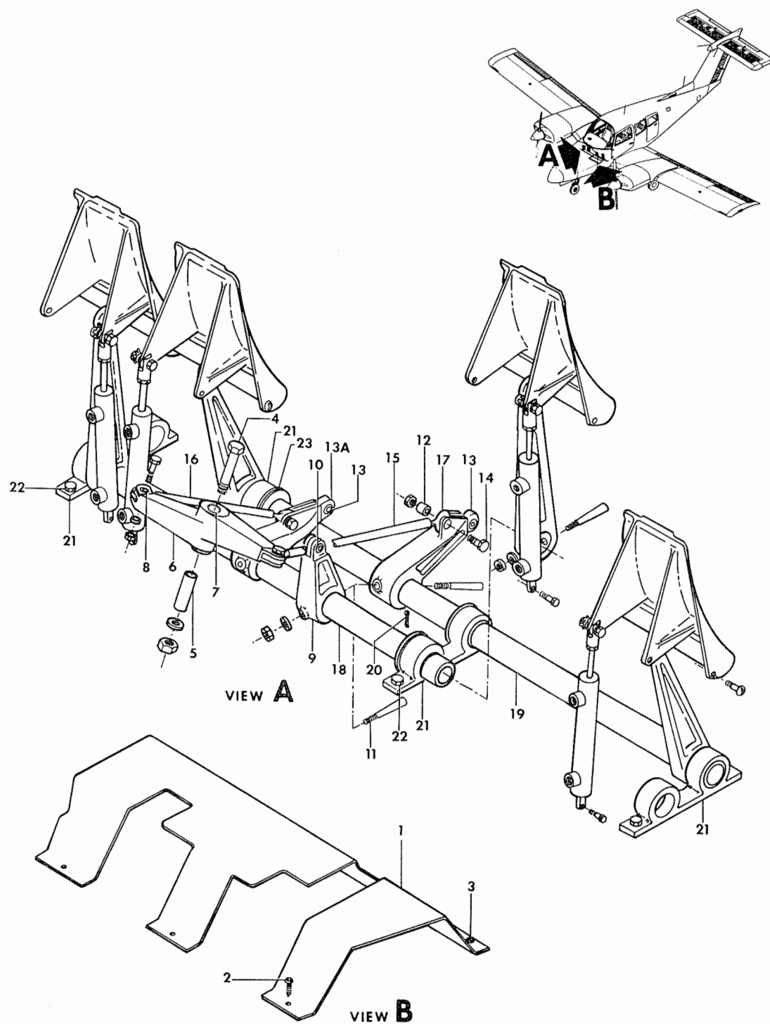
FIGURE 20-30. RUDDER PEDALS /SHEET 1 OF 2 SHEETS/
