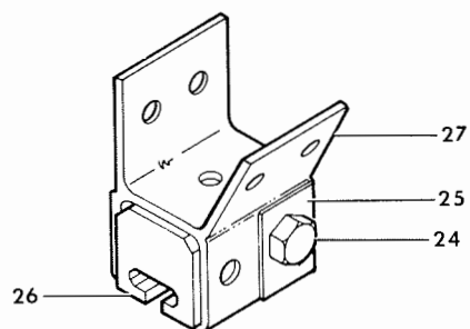
VIEW B
