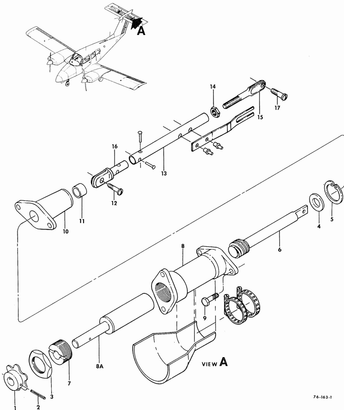
FIGURE 30-10.ELEVATOR TAB ACTUATOR
