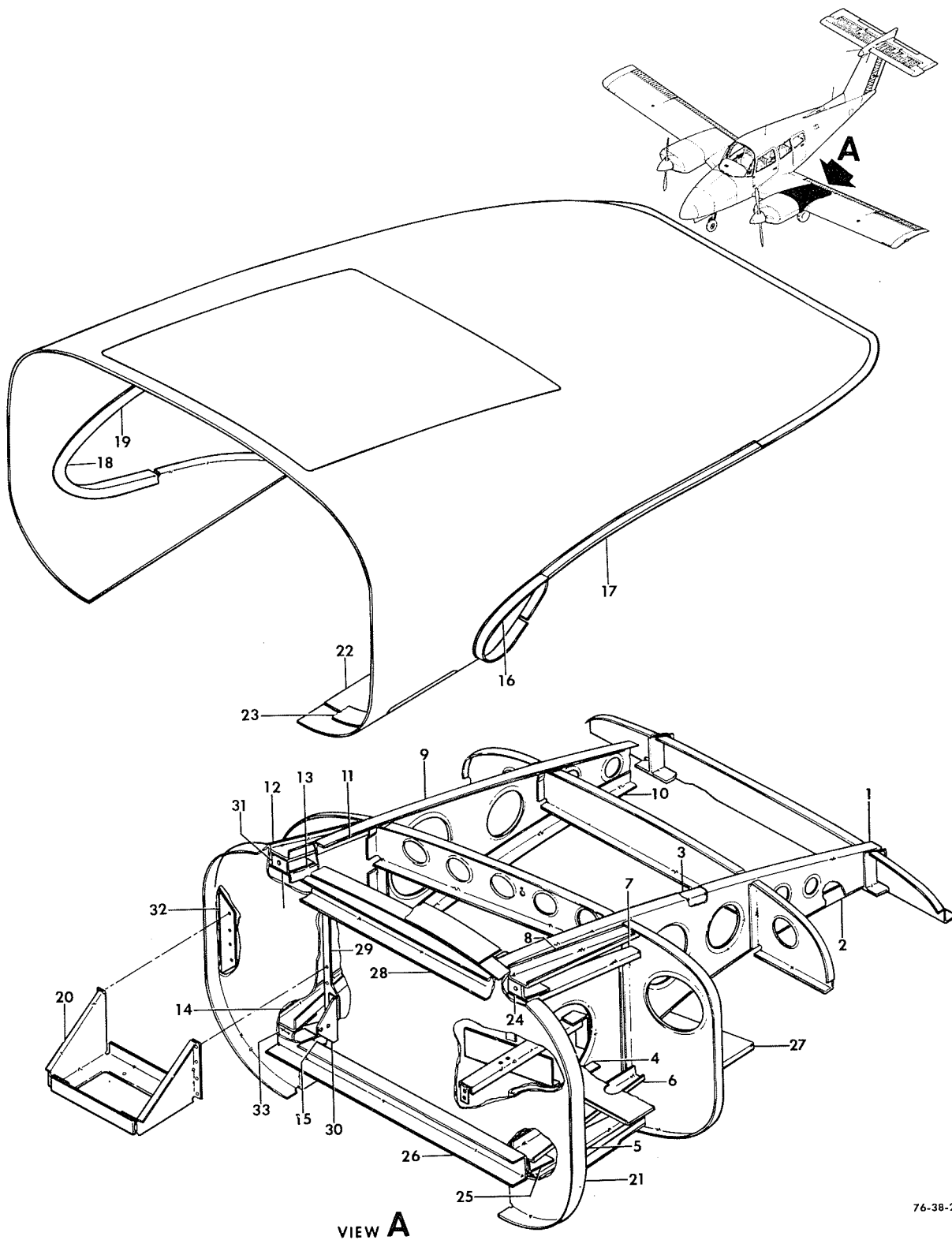
FIGURE 10-01. NACELLE INSTALLATION /SHEET 1 OF 2 SHEETS/
