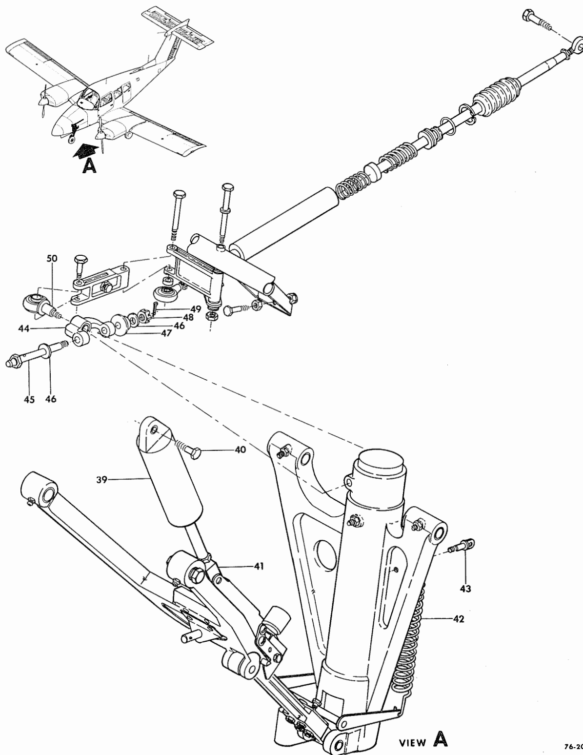
FIGURE 20-01. NOSE LANDING GEAR INSTALLATION /SHEET 3 OF 4 SHEETS/
