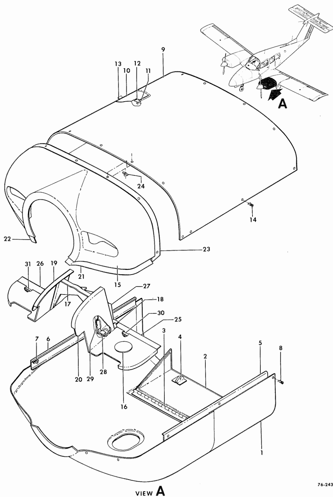
FIGURE 10-01.COWLING INSTALLATION
