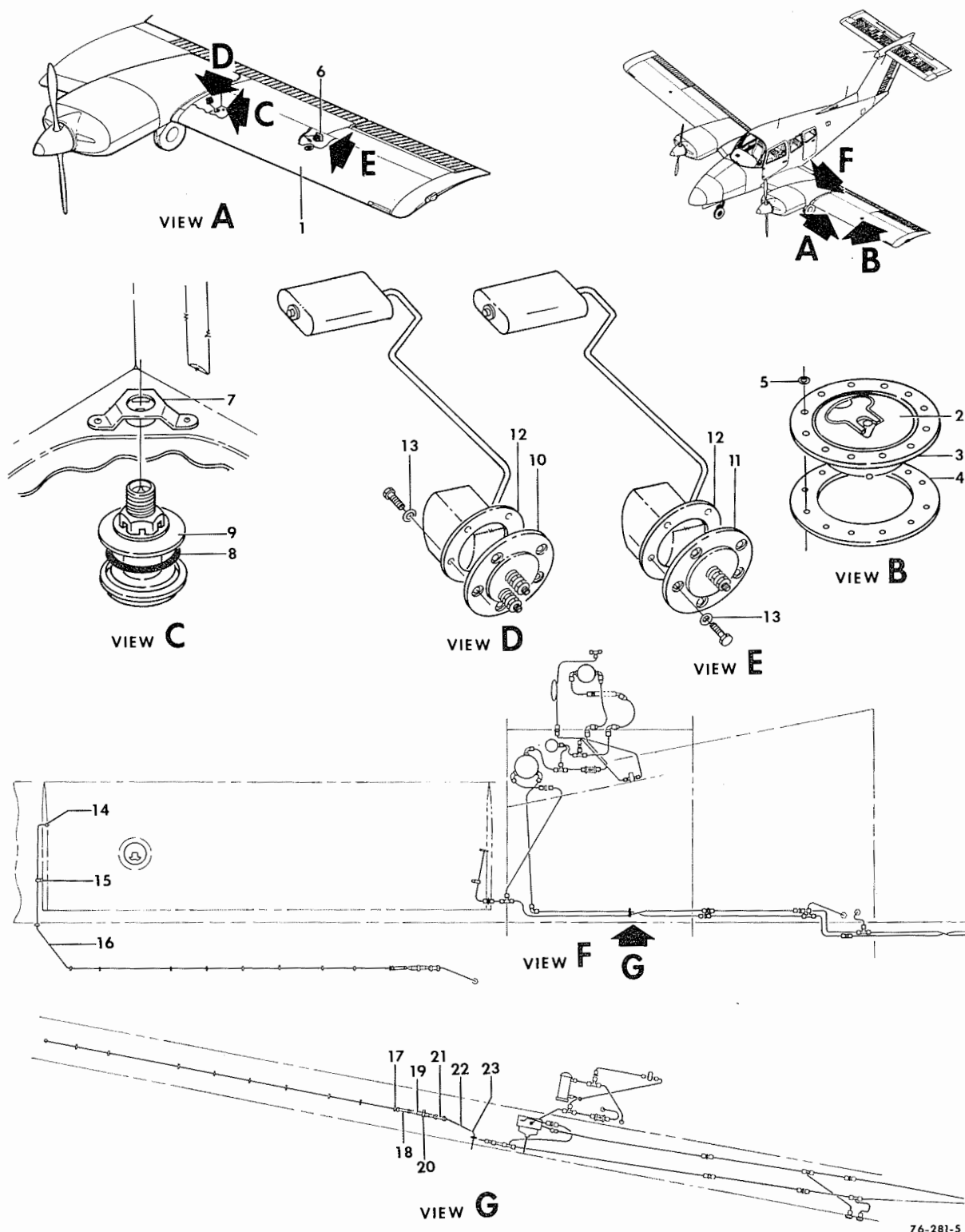
FIGURE 10-01.FUEL TANK & VENT SYSTEM
