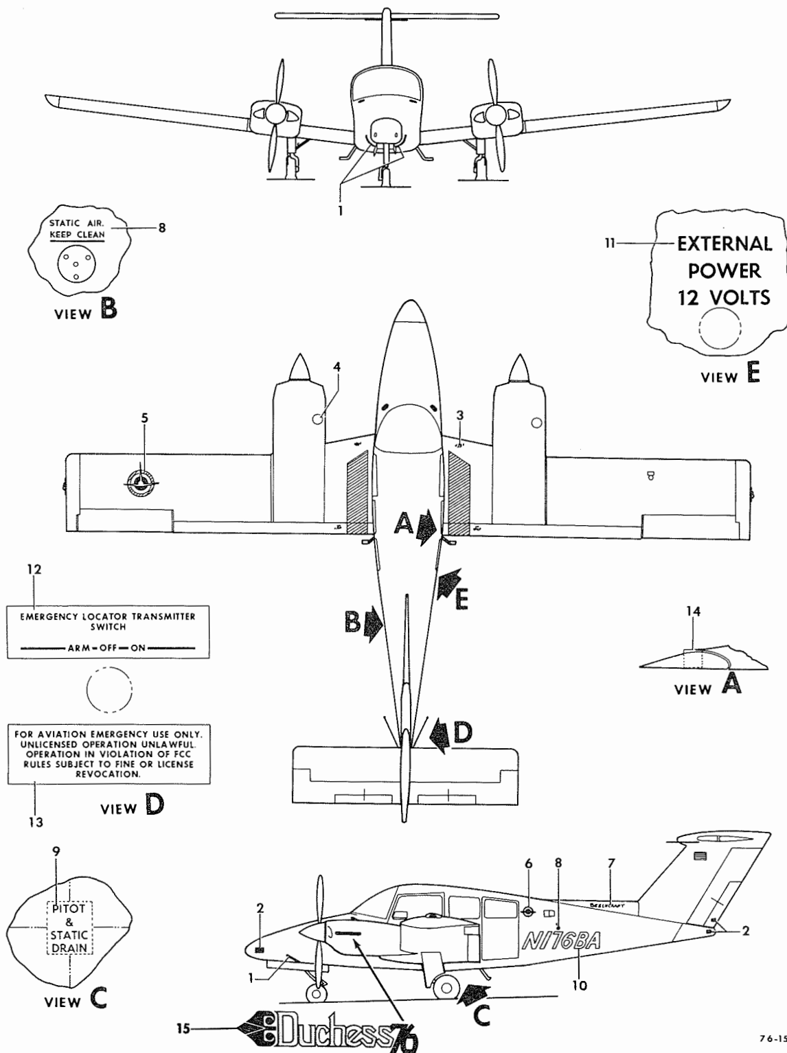
FIGURE 20-01. EXTERIOR PLACARDS AND MARKINGS
