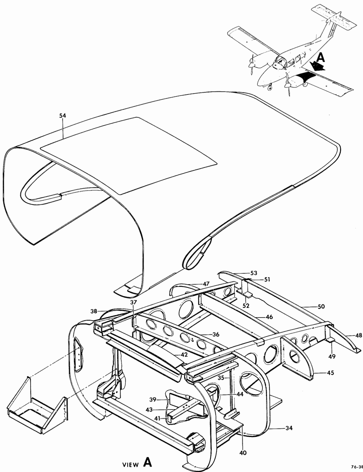
FIGURE 10-01. NACELLE INSTALLATION /SHEET 2 OF 2 SHEETS/
