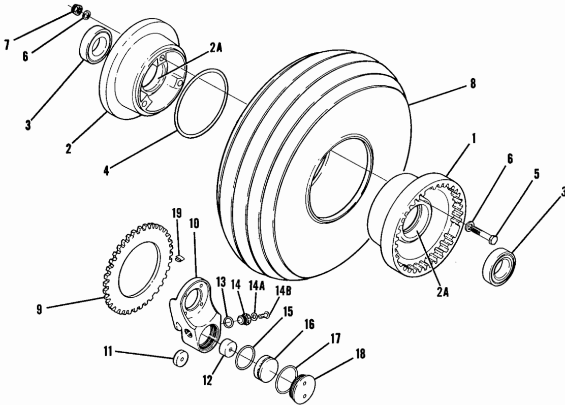
Figure 51. Main Landing Gear Wheel and Brake Assembly
