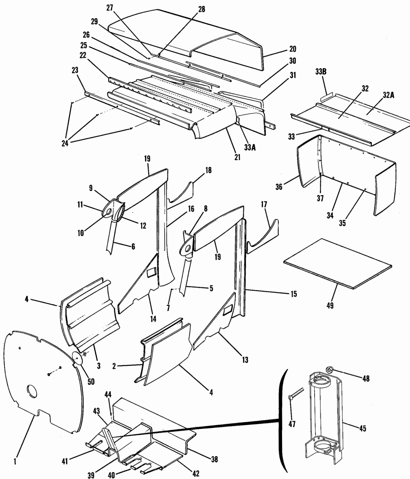
Figure 20. Upholstery Installation
