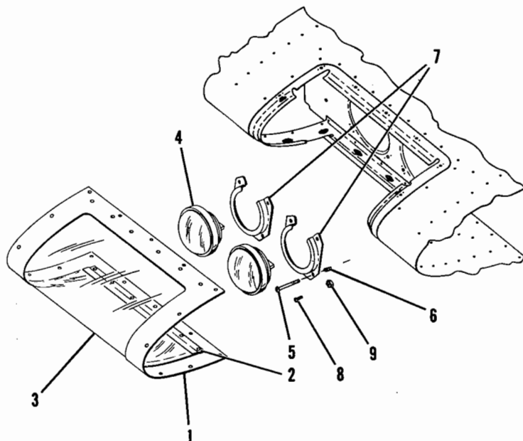
Figure 47. Landing Light Installation
