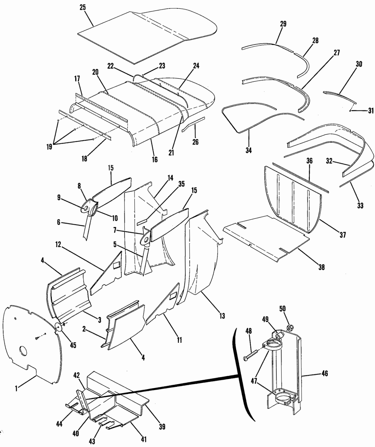
Figure 20A. Upholstery Installation
