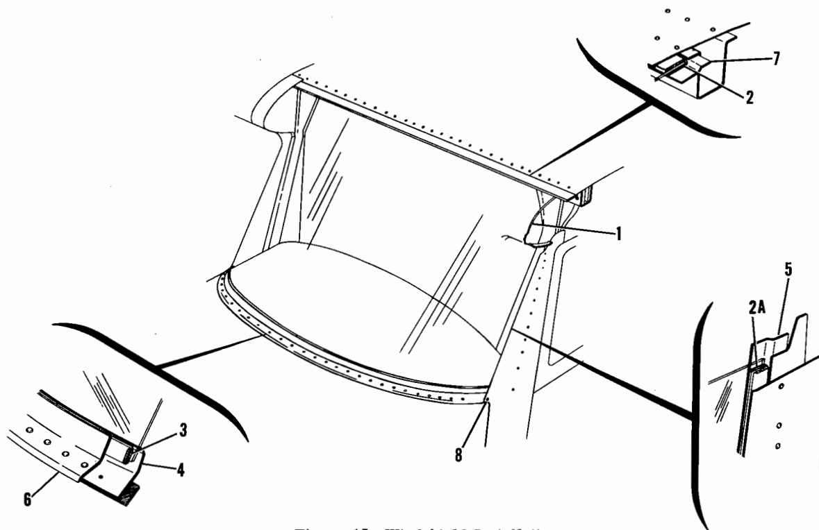
Figure 15. Windshield Installation
