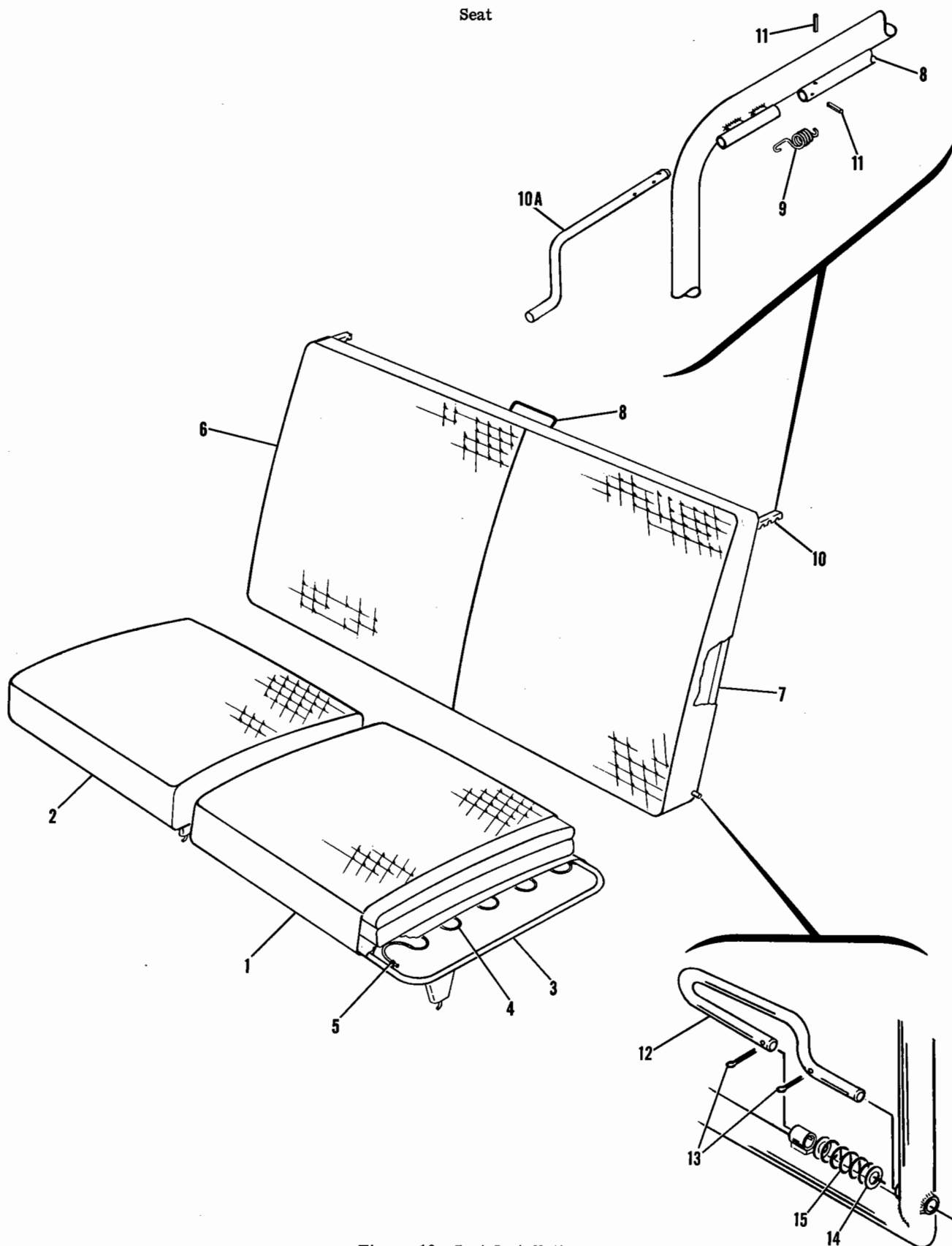
Figure 19. Seat Installation
