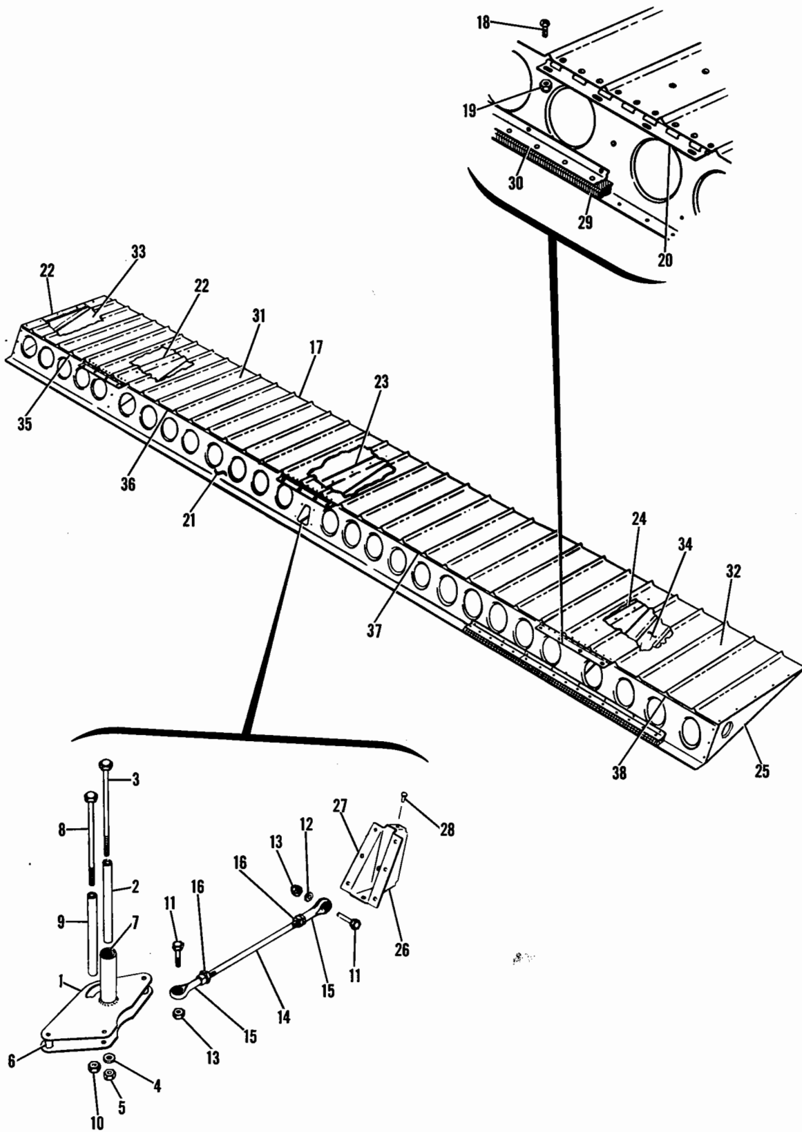
Figure 5. Aileron Installation
