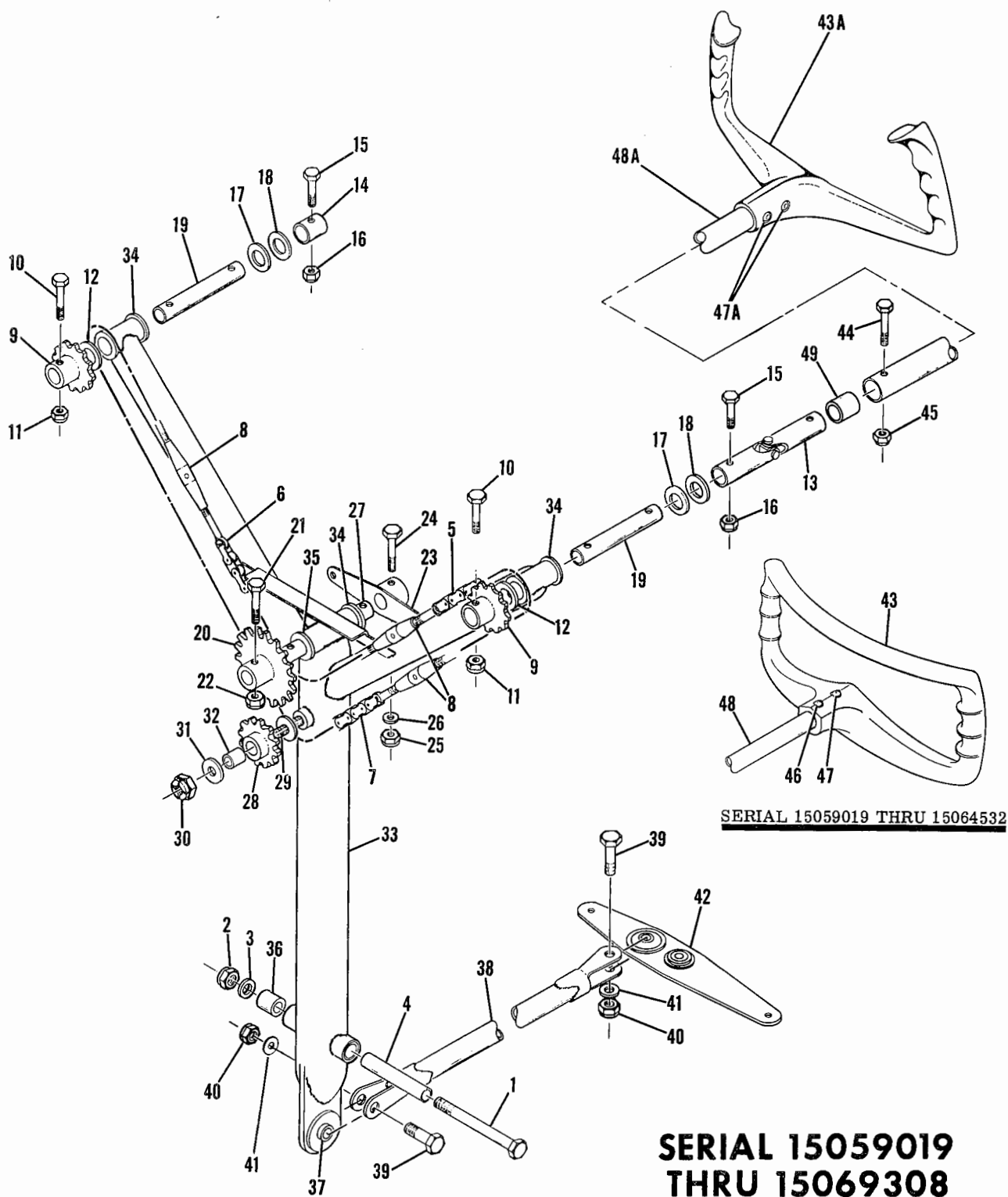
Figure 35A. Control Y Installation
