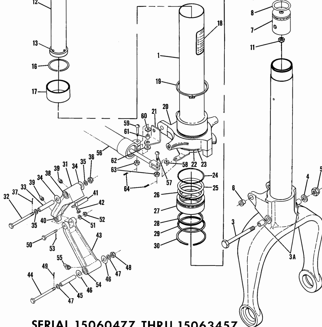
Figure 17B. Heavy Duty Nose Gear Strut Assembly
