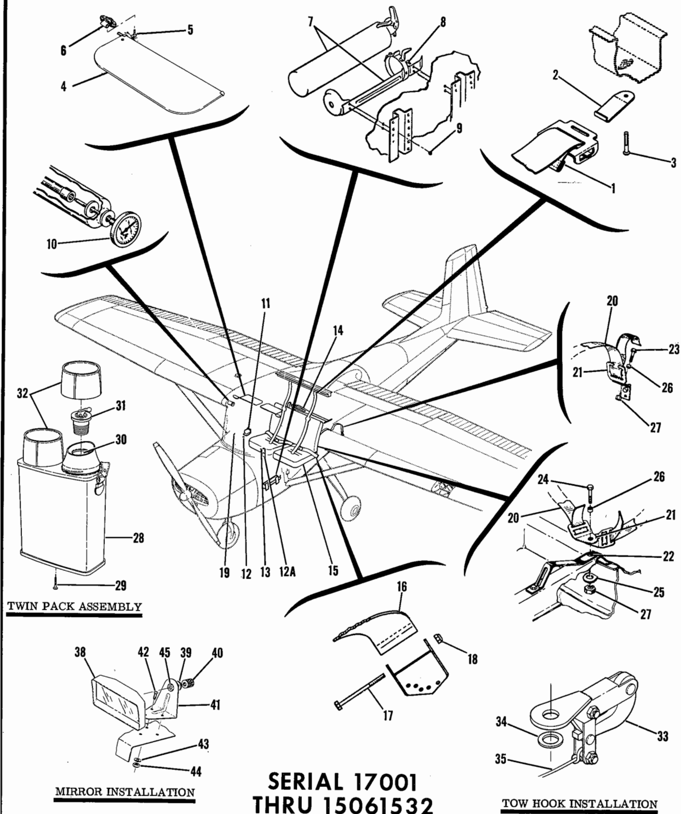
Figure 25. Fuselage Equipment Installation
