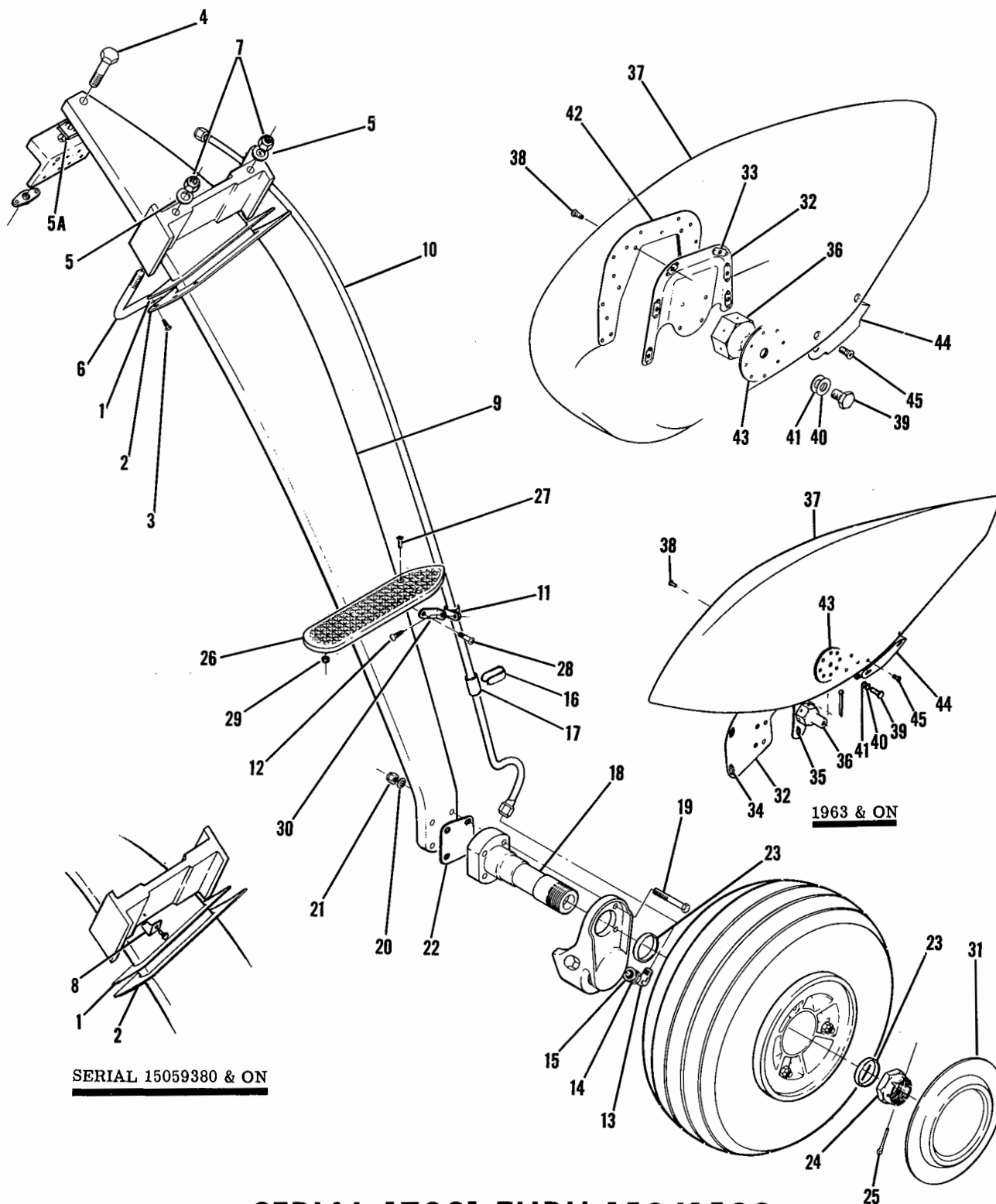
Figure 18. Main Landing Gear Installation
