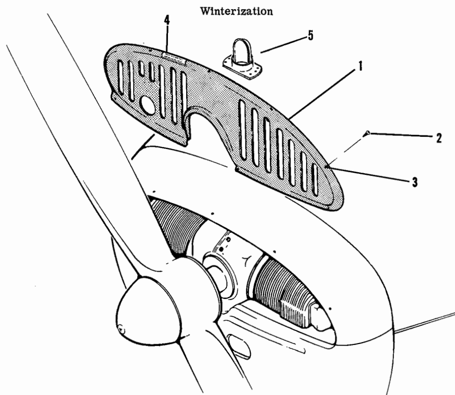
Figure 27. Engine Winterization Installation
