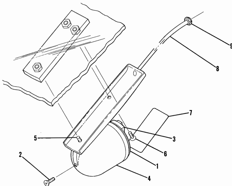
Figure 25B. Compass Installation
