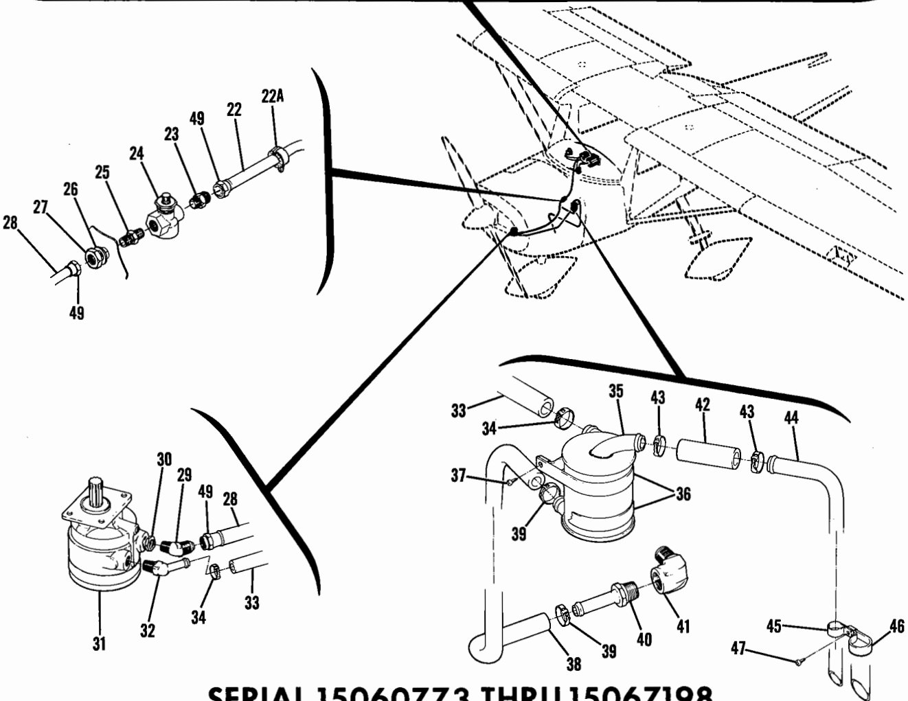
Figure 45B. Vacuum System Installation
