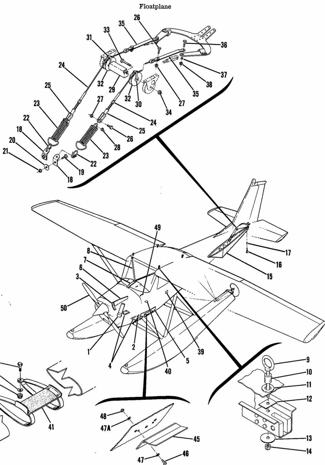
Figure 55. Floatplane Fittings Installation
