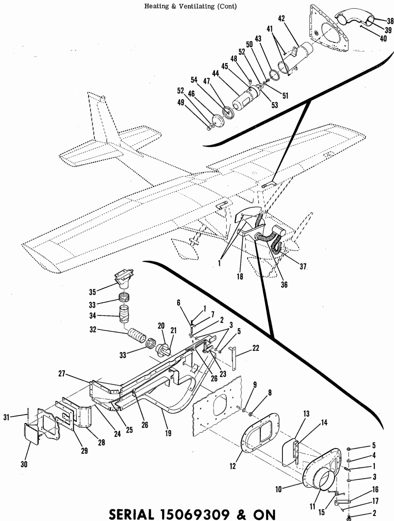
Figure 33B. Cabin Heating &amp; Ventilating System Installation
