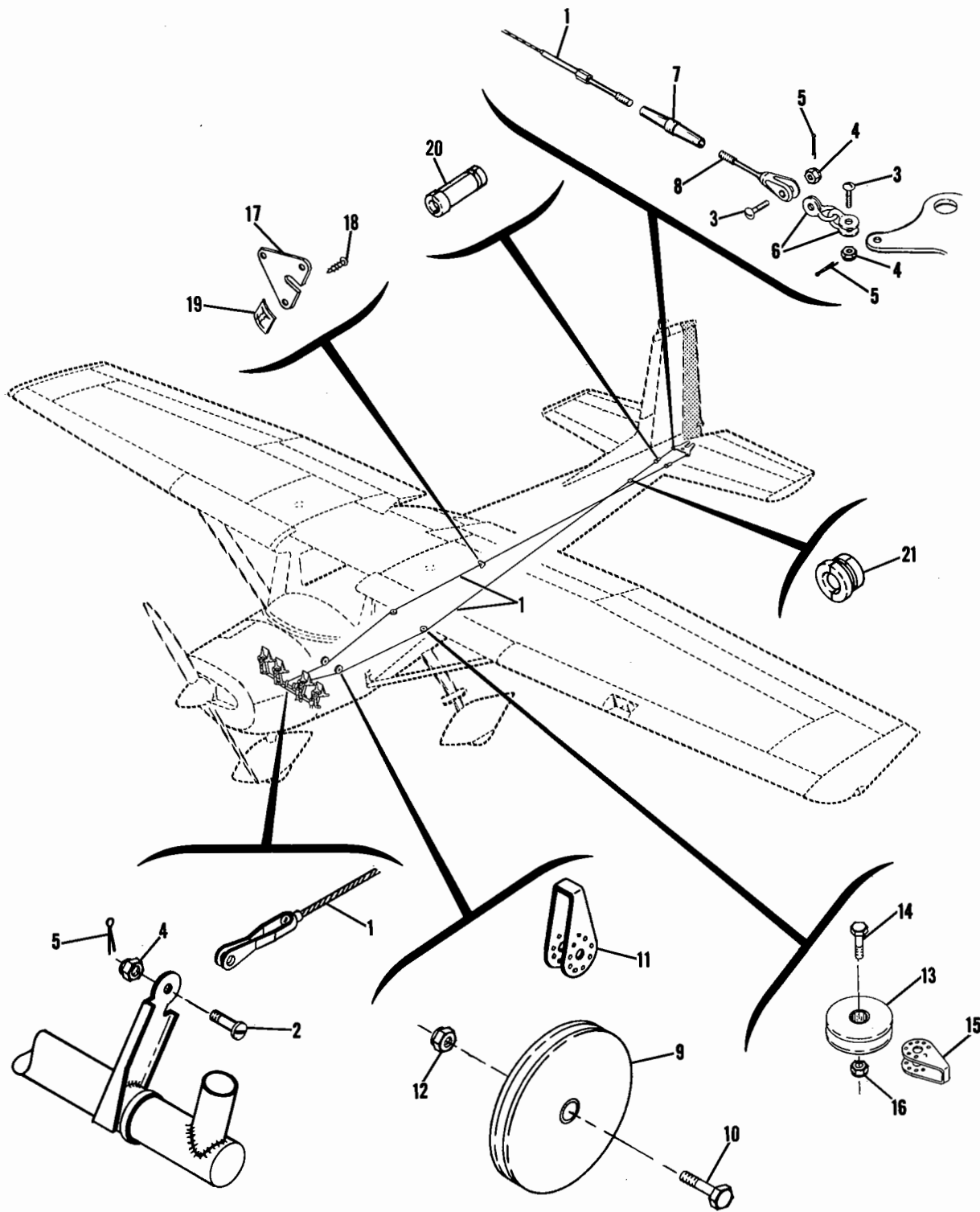
Figure 36. Rudder Control System Installation
