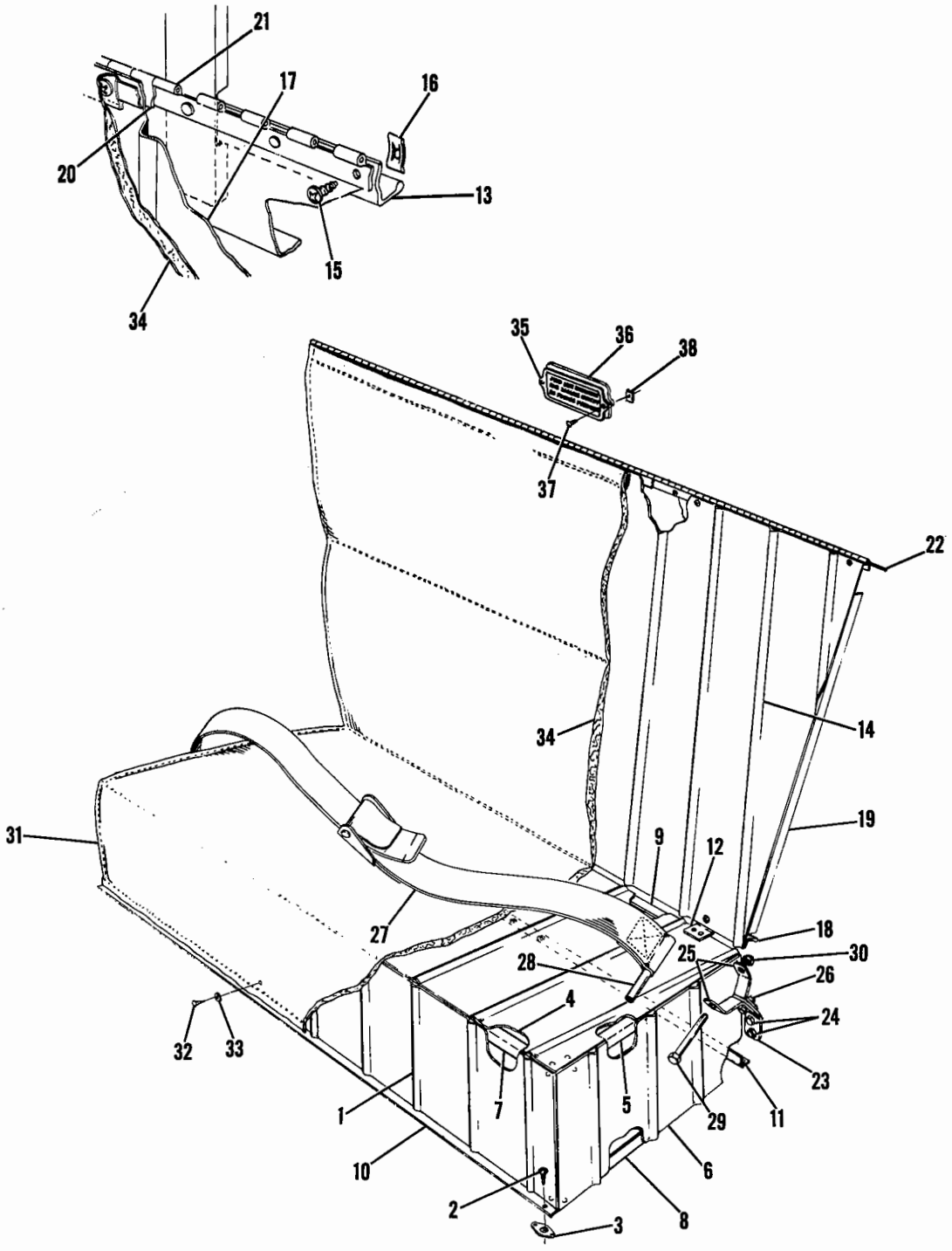
SERIAL 17001 THRU 15059350 Figure 19A. Child Seat Installation
