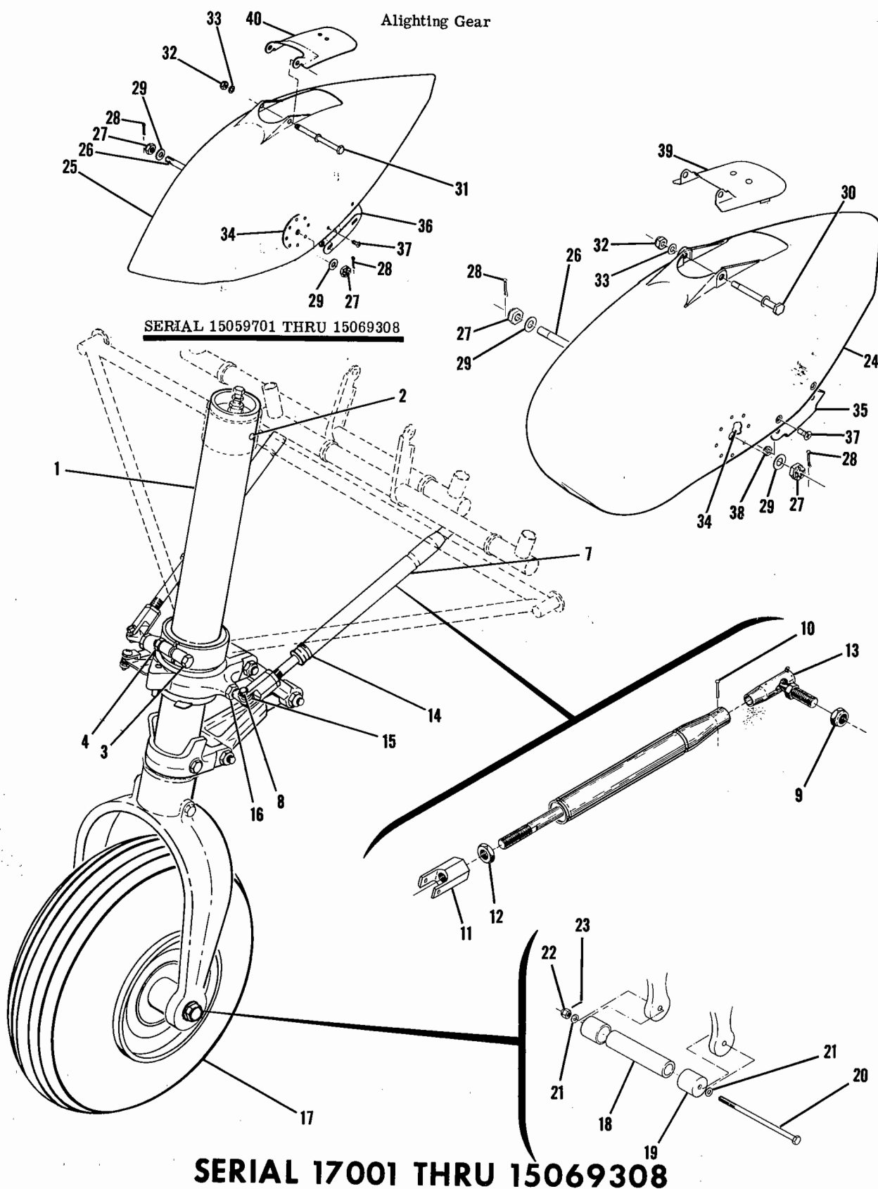
Figure 16. Nose Gear Installation
