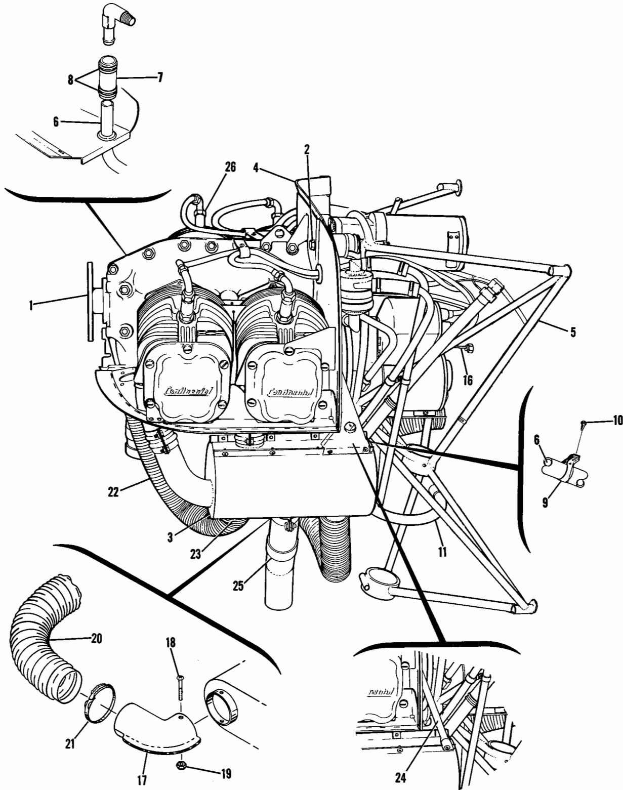
Figure 30. Engine Assembly
