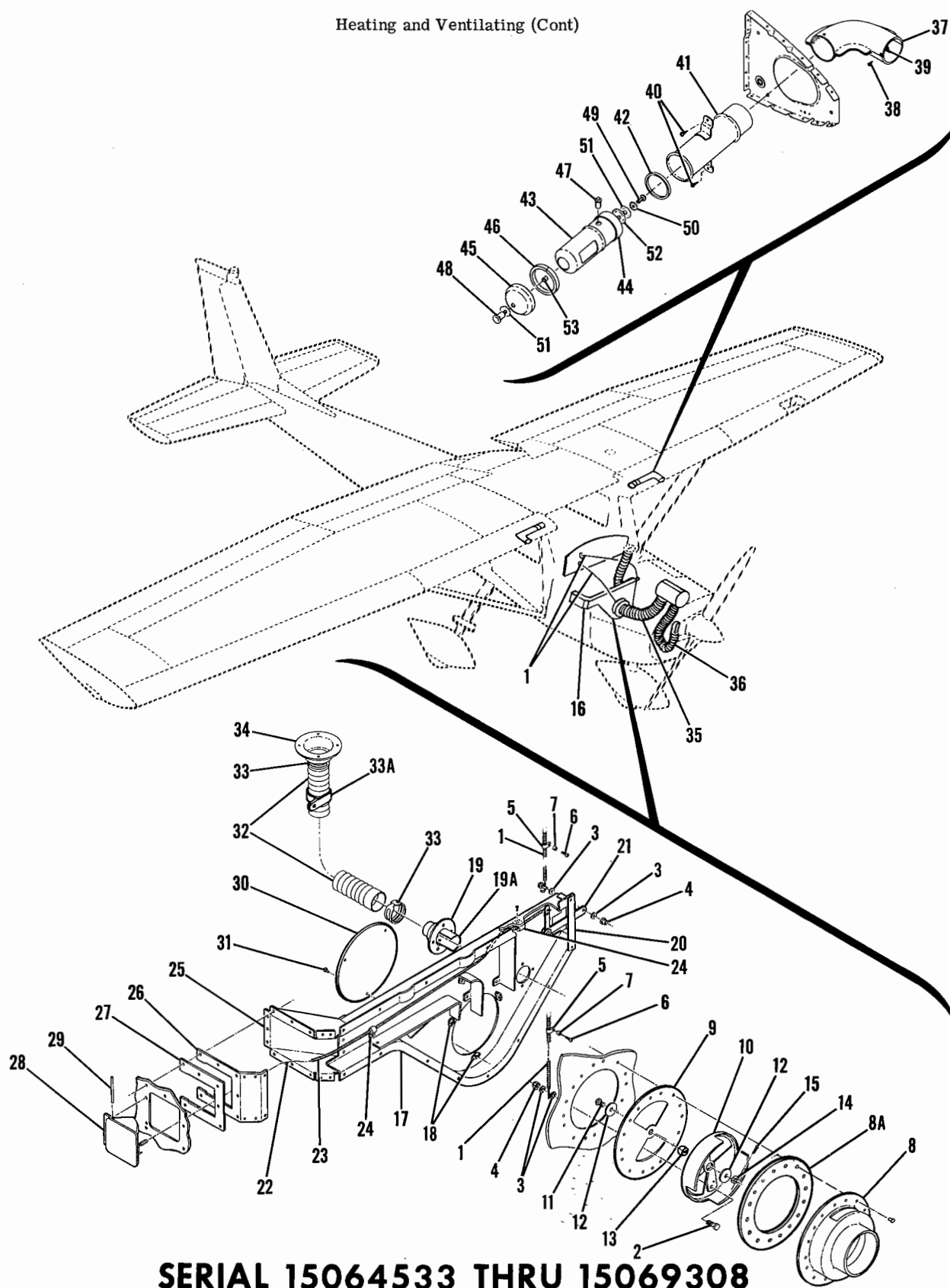
Figure 33A. Cabin Heating and Ventilating System Installation
