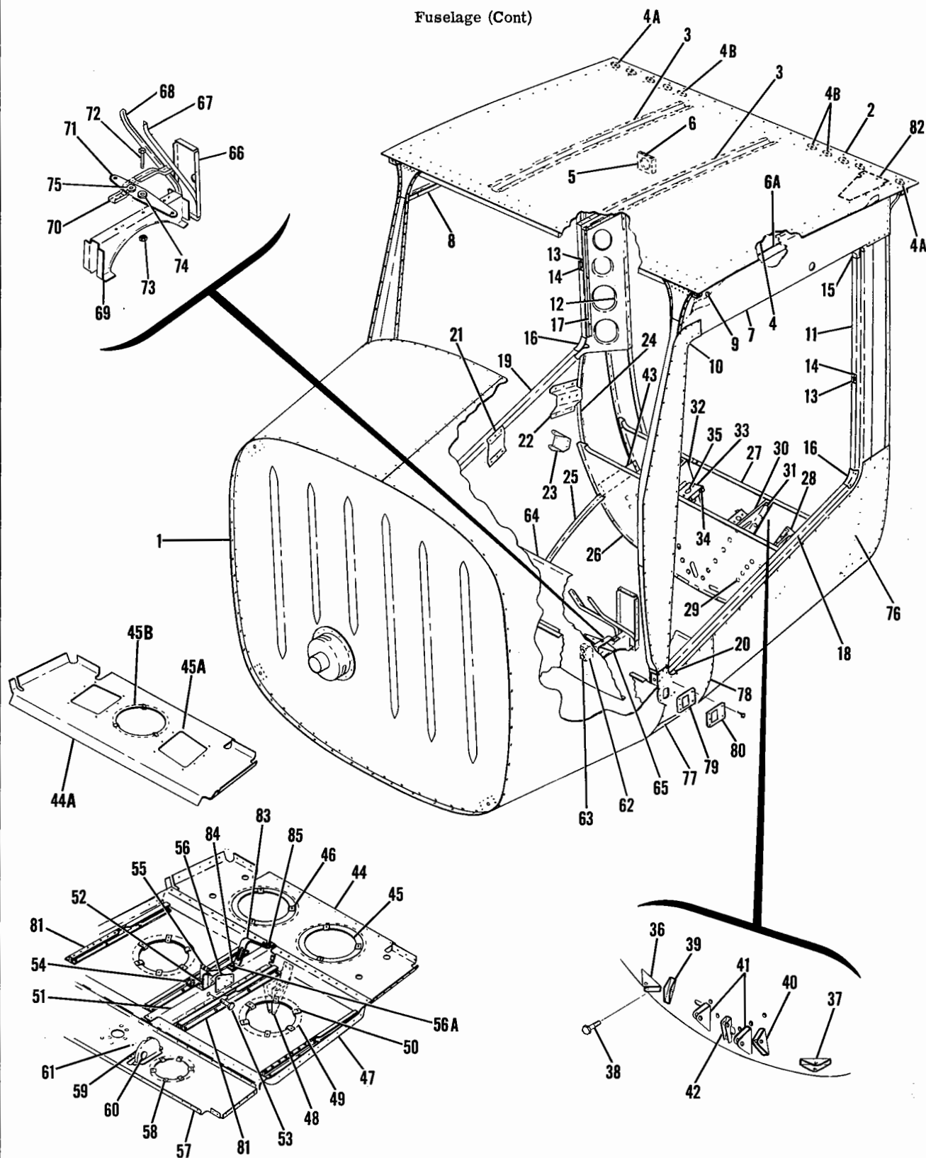
Figure 11. Fuselage Front and Center Section Assembly
