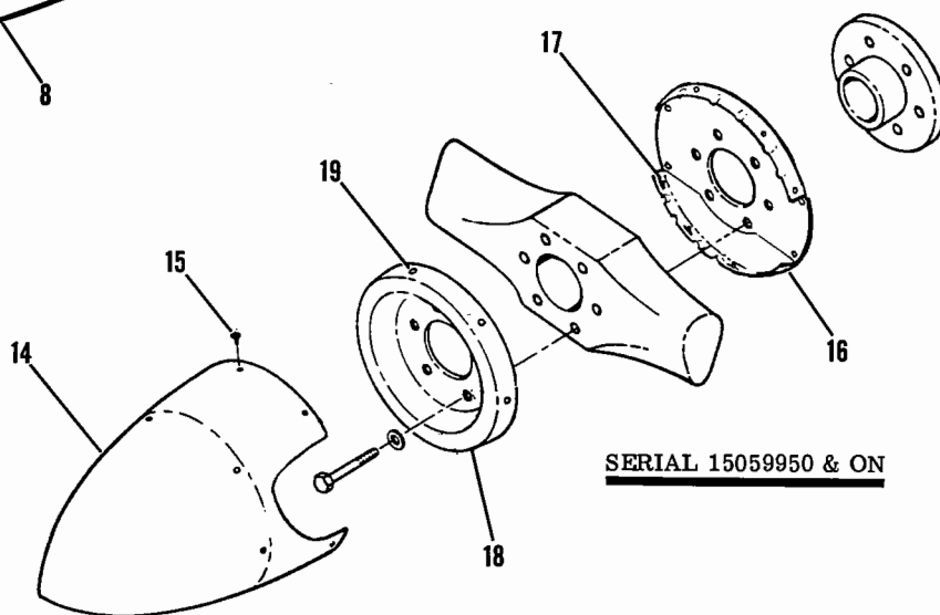
Figure 26. Propeller and Spinner Installation
