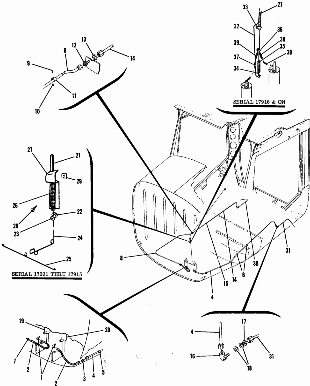
Figure 42. Brake System Installation
