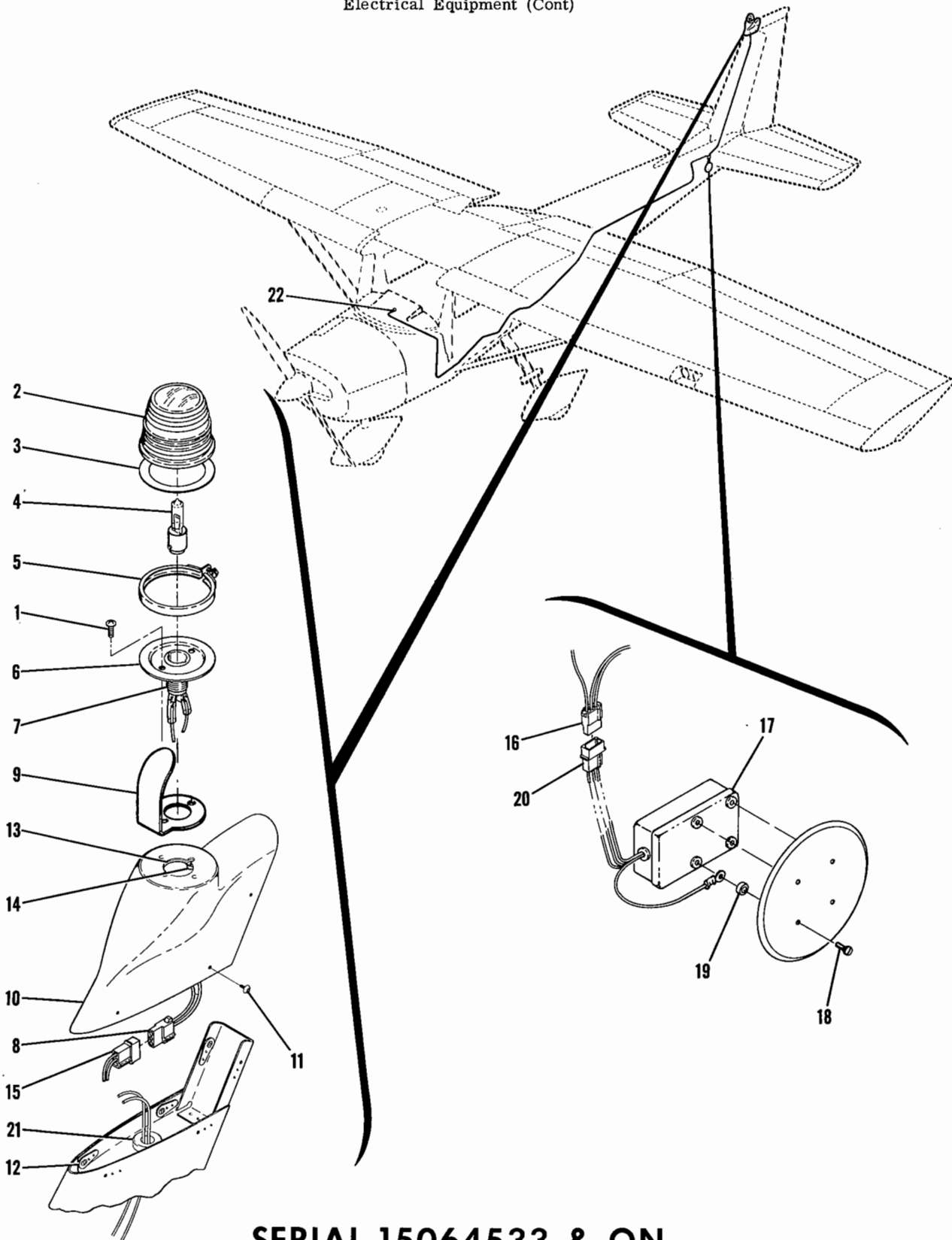
Figure 48A. Flashing Beacon Light Installation
