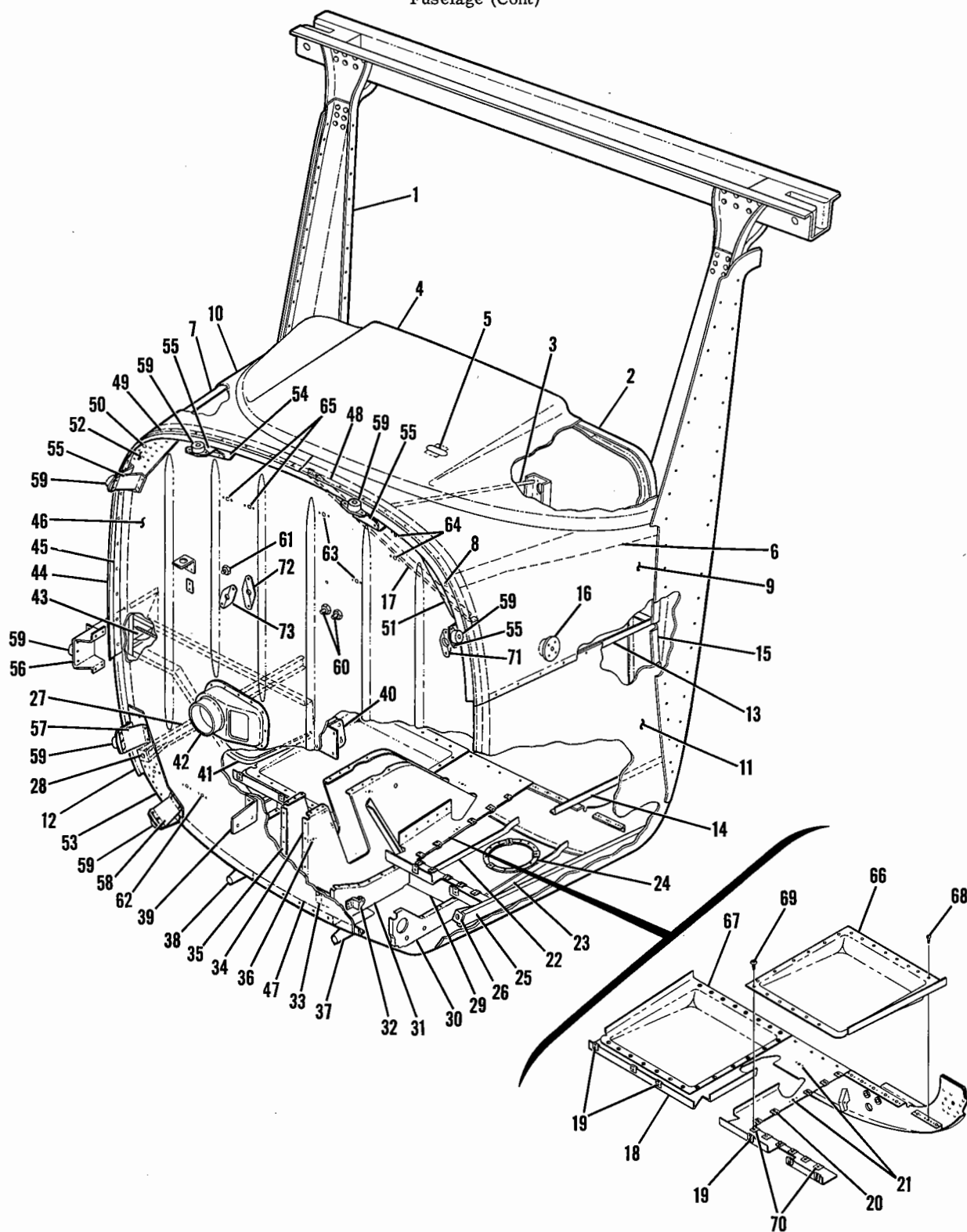
Figure 12C. Fuselage Front Section Assembly
