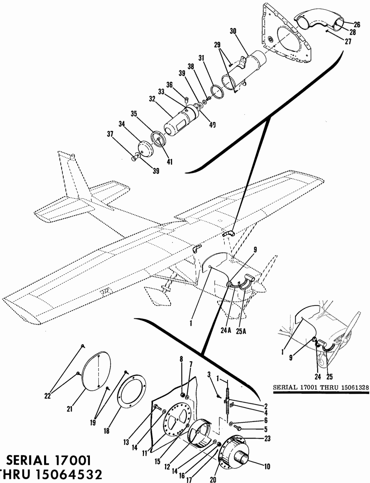
Figure 33. Cabin Heating and Ventilating System Installation
