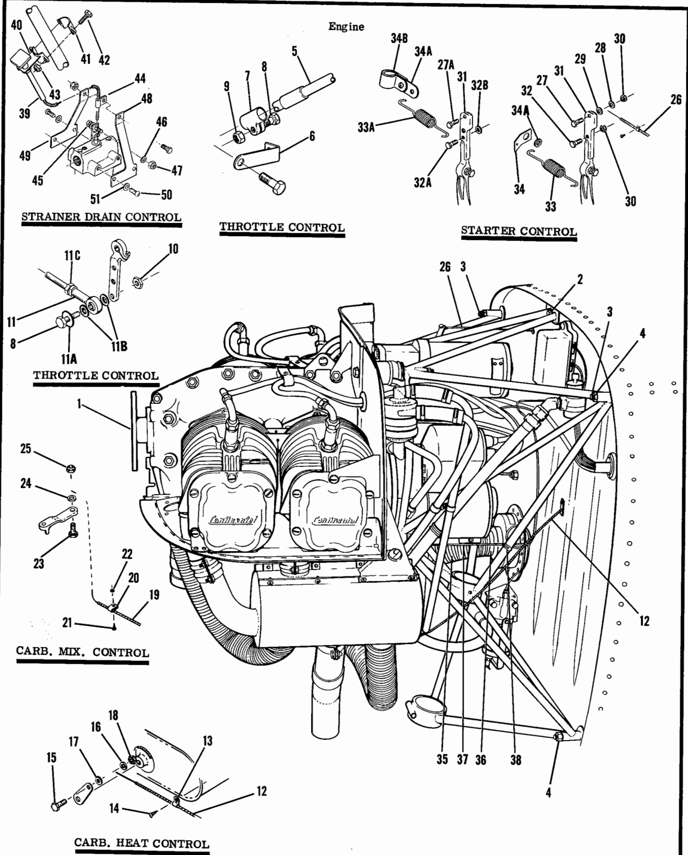
Figure 29. Engine Installation
