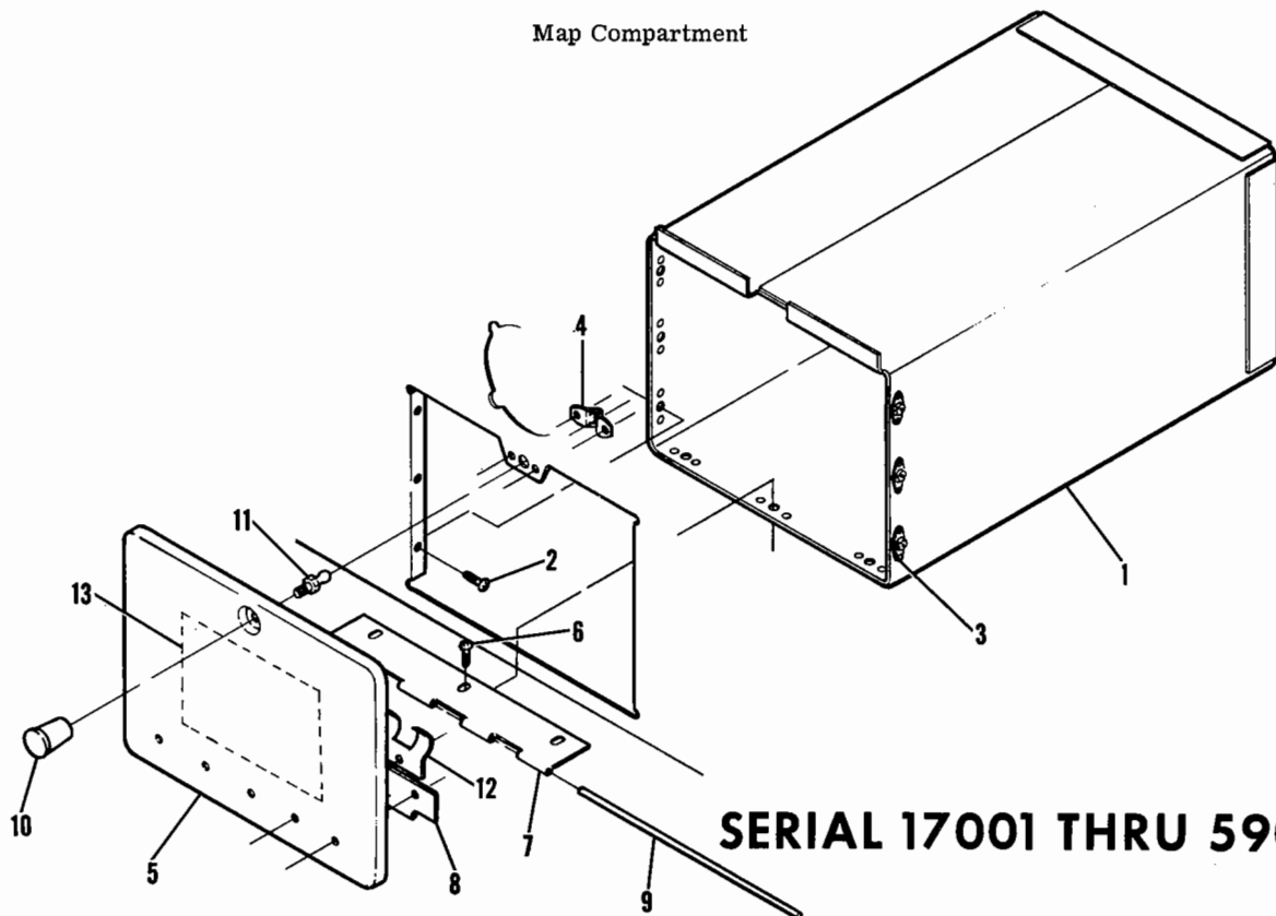
Figure 24. Glove Box Installation
