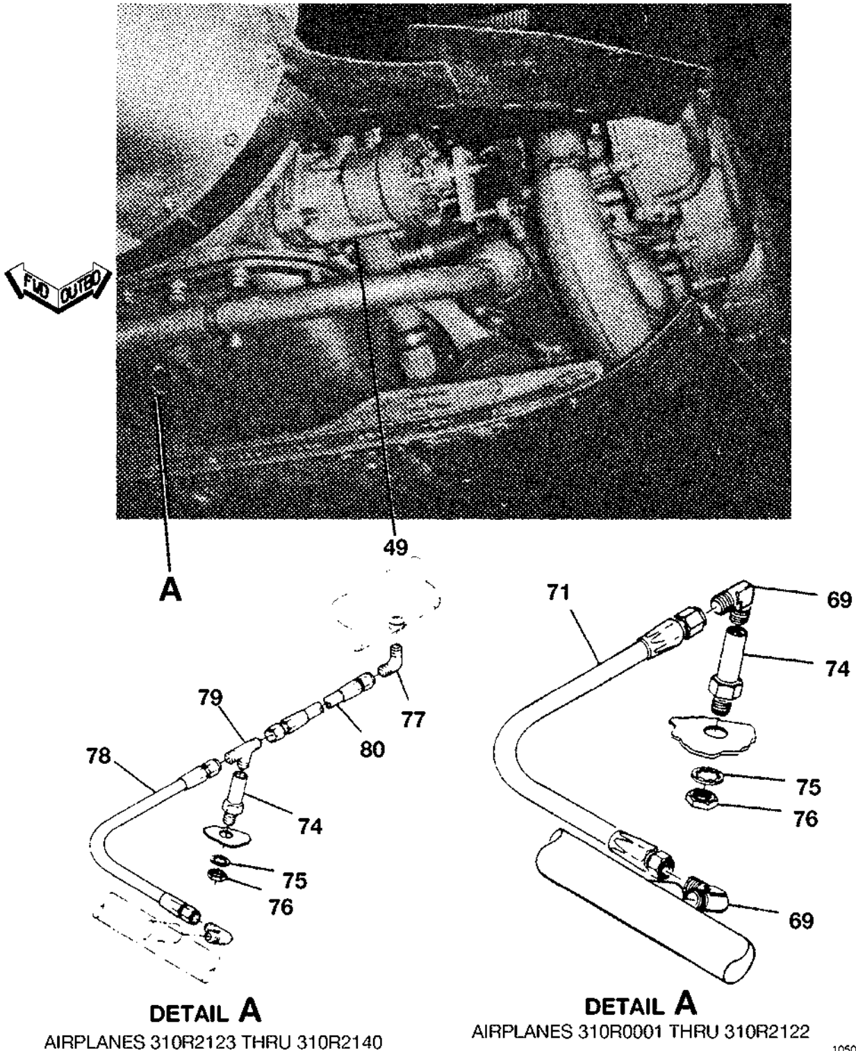
ENGINE ASSEMBLY AND ACCESSORIES INSTALLATION FIGURE 02 (SHEET 2)
