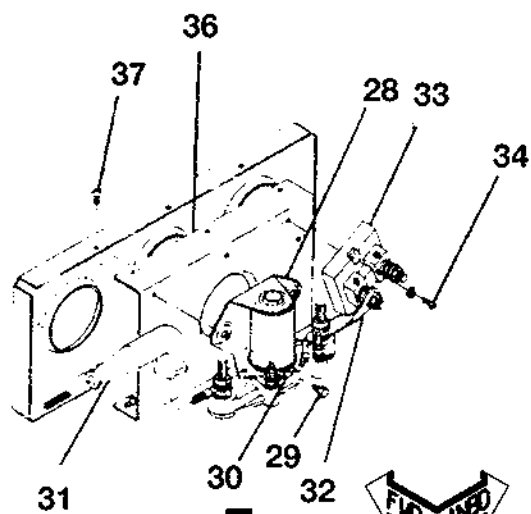
DETAIL E
