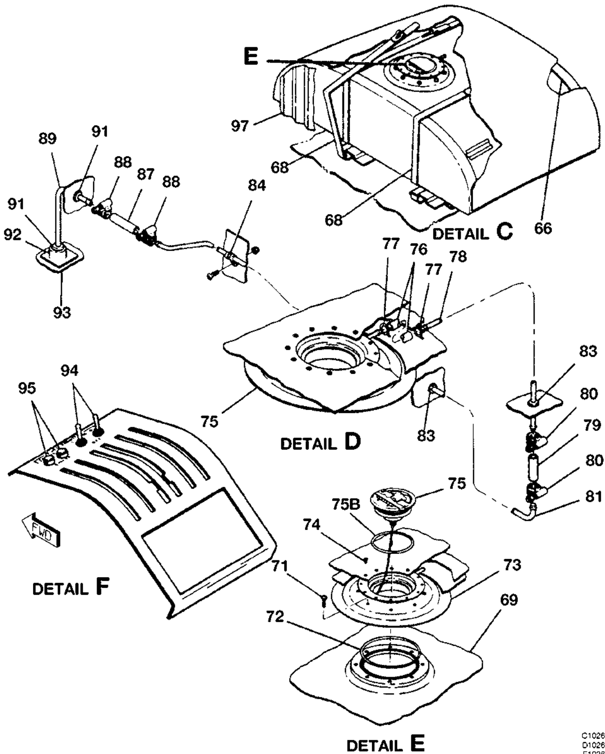
WING LOCKER FUEL SYSTEM FIGURE 02 (SHEET 2)
