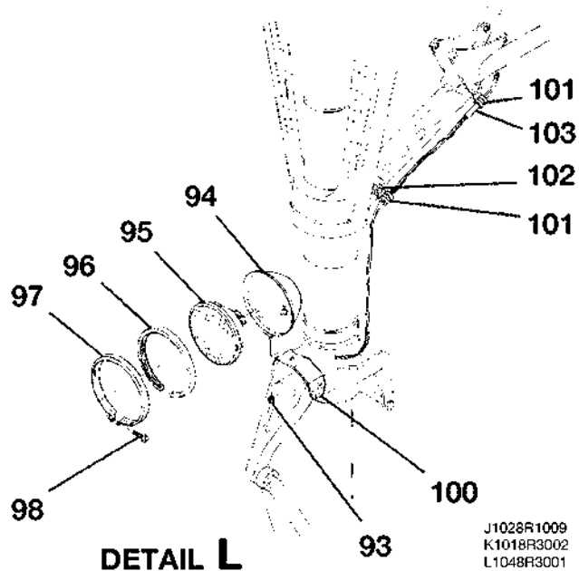
EXTERIOR LIGHTING INSTALLATION FIGURE 01 (SHEET 3)
