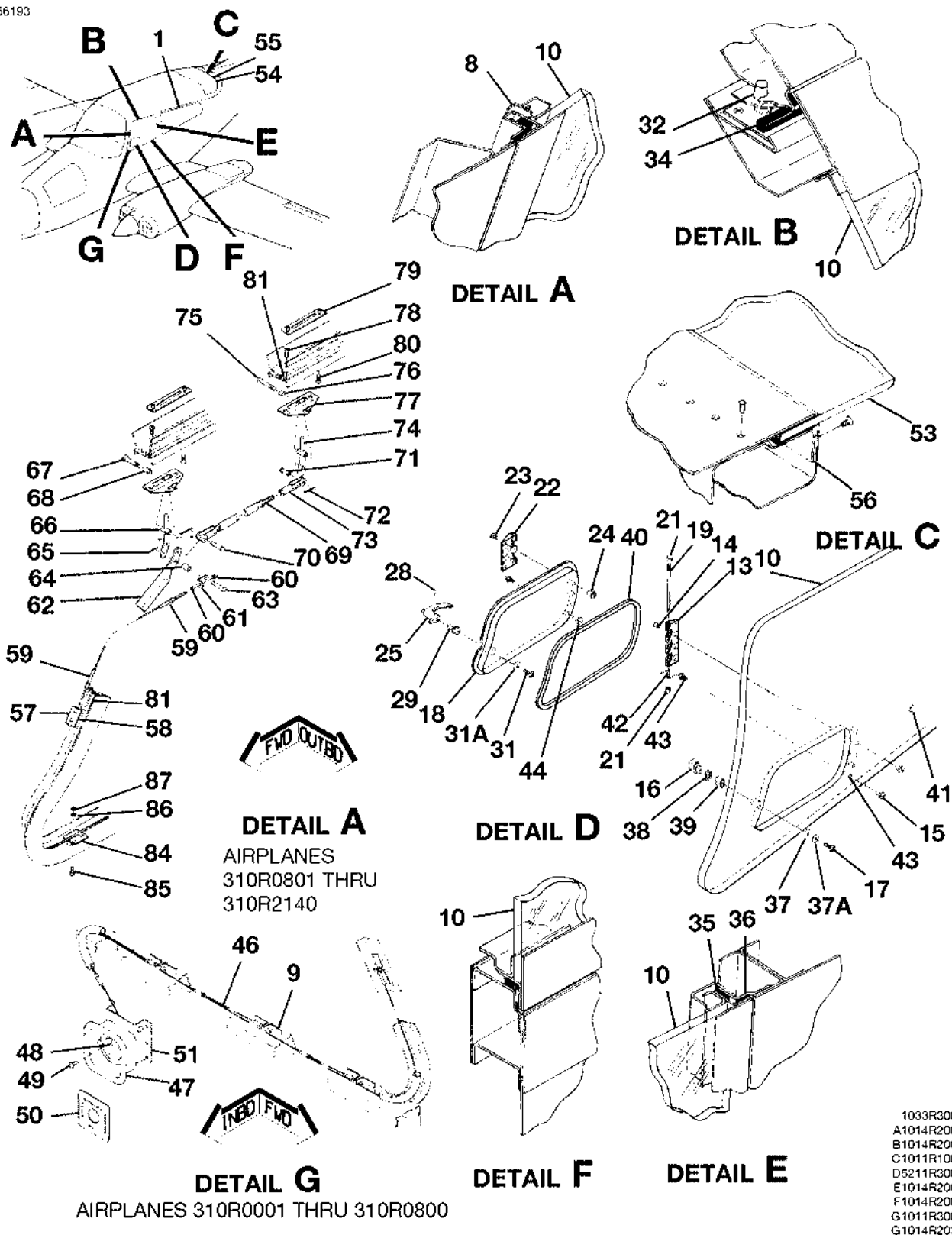
CABIN WINDOWS INSTALLATION FIGURE 02 (SHEET 1)
