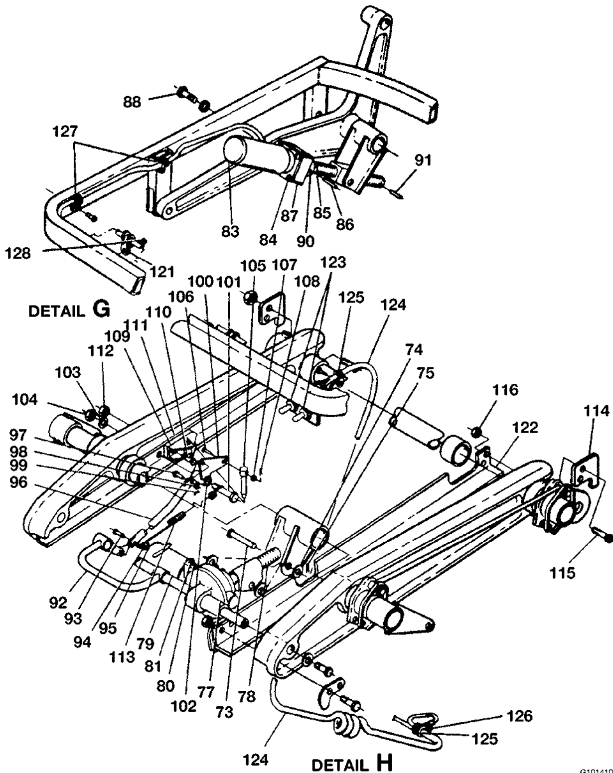
PILOT AND COPILOT ELECTRICALLY ADJUSTABLE SEAT INSTALLATION FIGURE 03 (SHEET 3)
