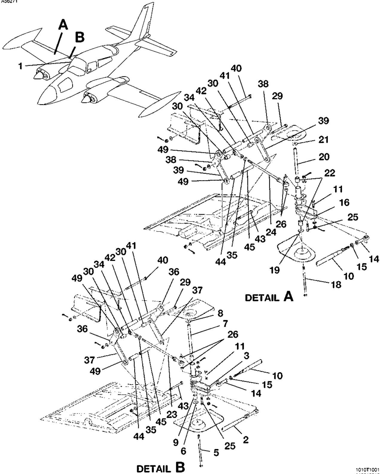
OUTBOARD FLAP CONTROL SYSTEM FIGURE 02 (SHEET 1)
