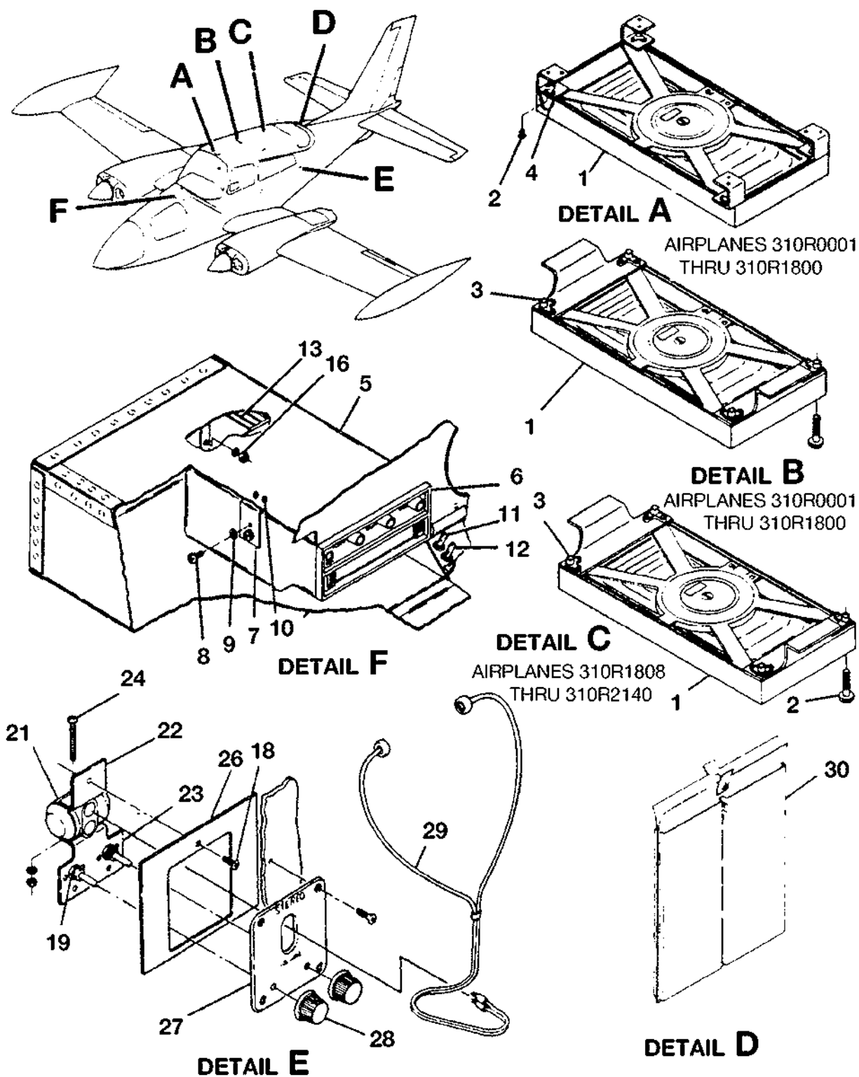
CABIN STEREO COMPONENTS FIGURE 01 (SHEET 1)
