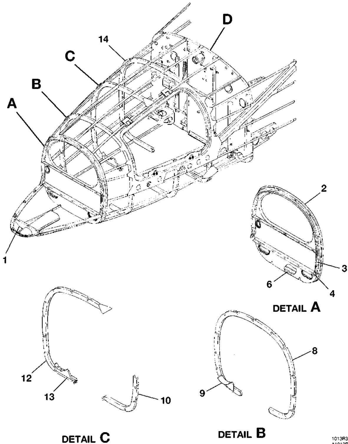
NOSE BULKHEADS INSTALLATION FIGURE 02 (SHEET 1)
