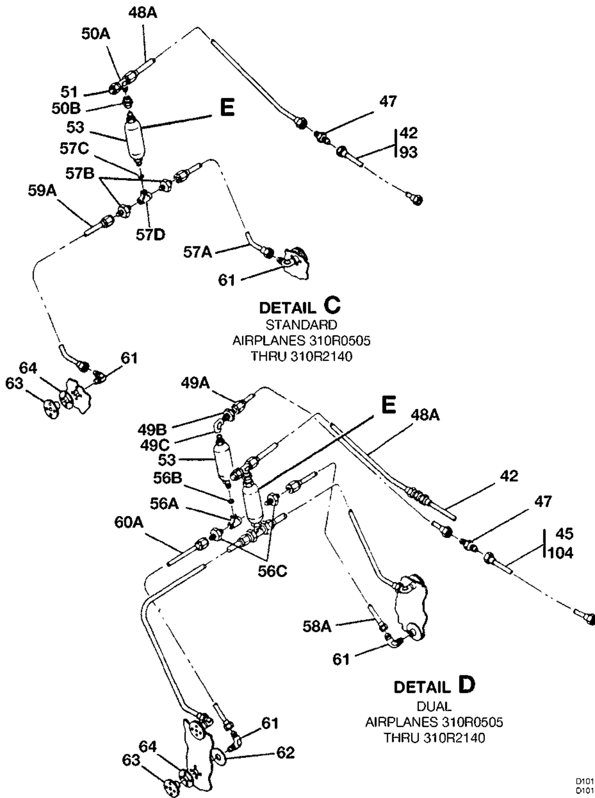
STATIC SYSTEM FIGURE 01 (SHEET 3)
