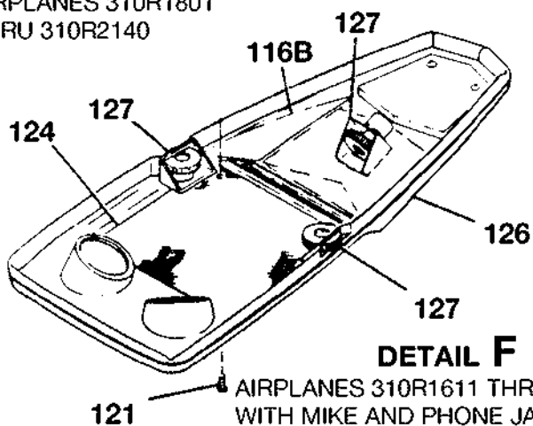
UPHOLSTERY TRIM INSTALLATION FIGURE 01 (SHEET 3)
