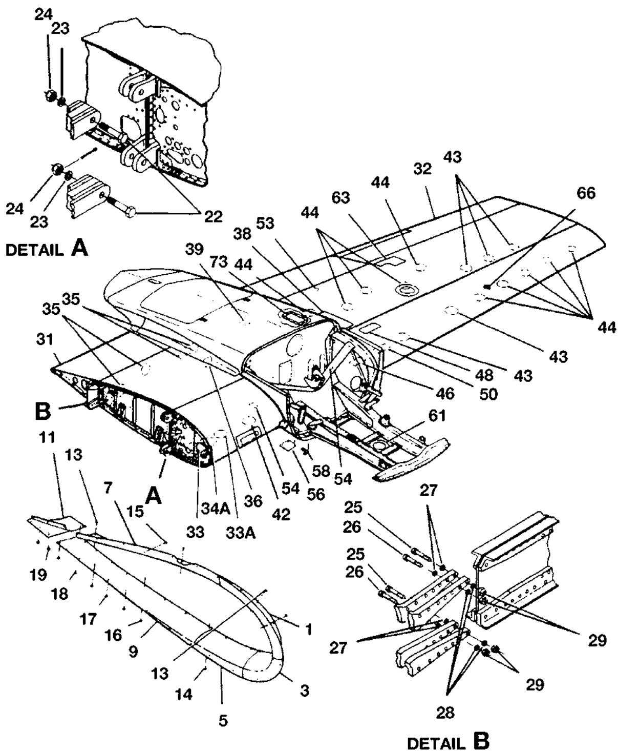
WING INSTALLATION FIGURE 01 (SHEET 1)
