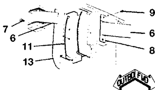
DETAIL A INERTIA REEL
