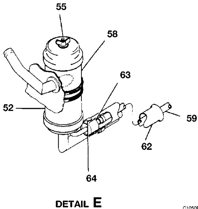
ENGINE ASSEMBLY AND ACCESSORIES INSTALLATION TURBO 310 FIGURE 03 (SHEET 2)
