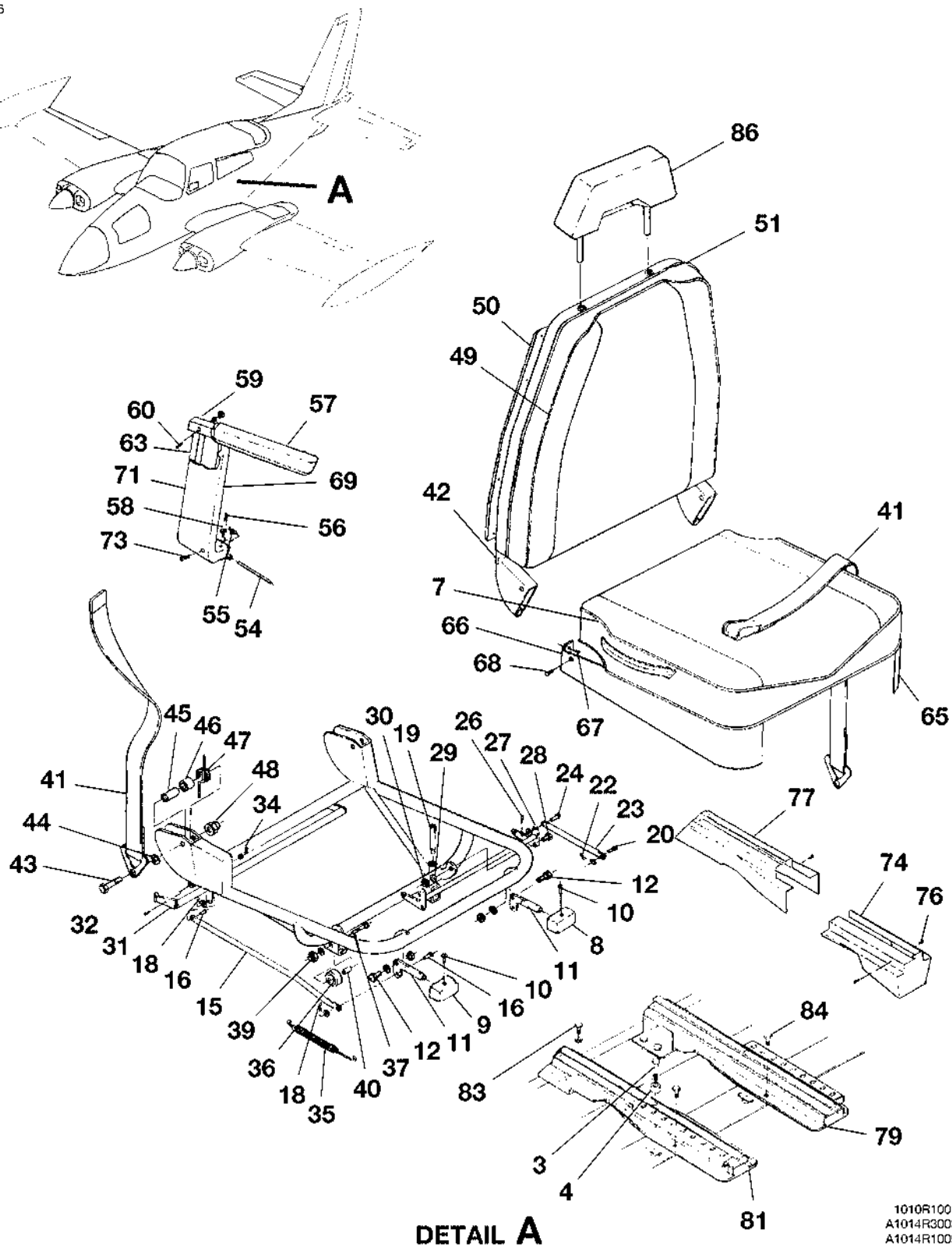
CENTER SINGLE SEAT INSTALLATION FIGURE 01 (SHEET 1)
