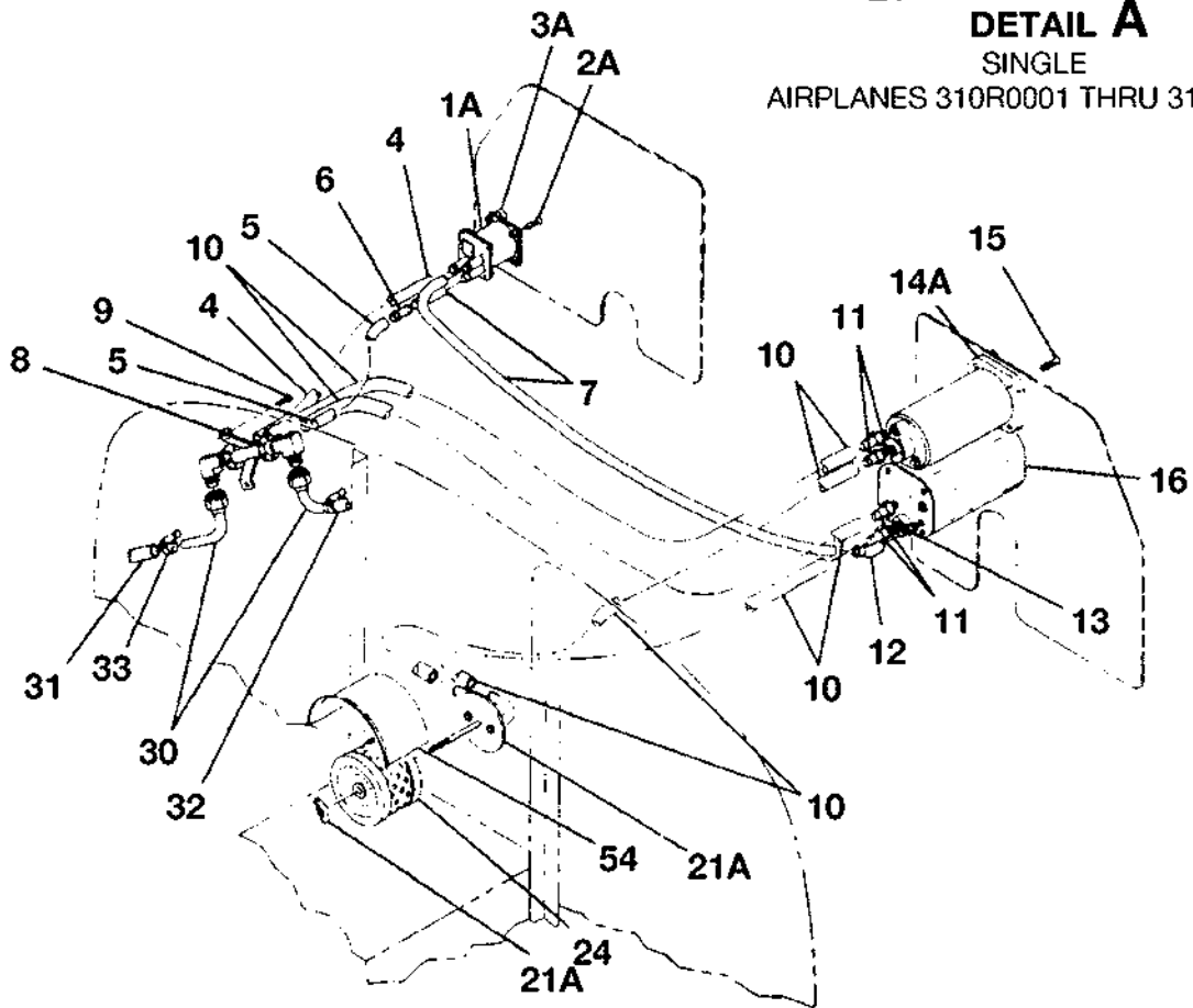
DETAIL A SINGLE AIRPLANES 310R0501 THRU 310R2140 VACUUM SYSTEM FIGURE 01 (SHEET 1)
