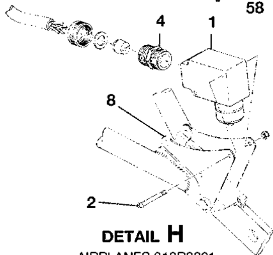
LANDING GEAR ELECTRICAL COMPONENTS FIGURE 01 (SHEET 2)
