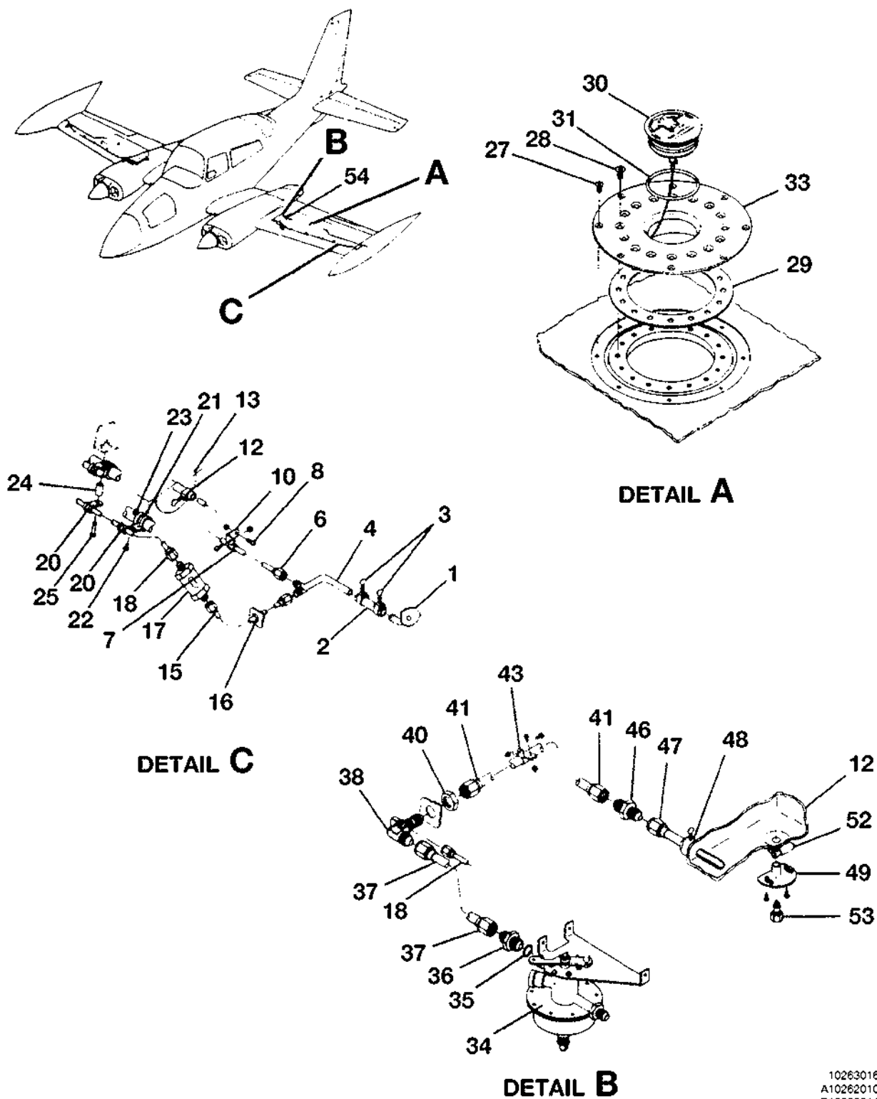
AUXILIARY FUEL SYSTEM COMPONENTS 40 GALLON FIGURE 01 (SHEET 1)
