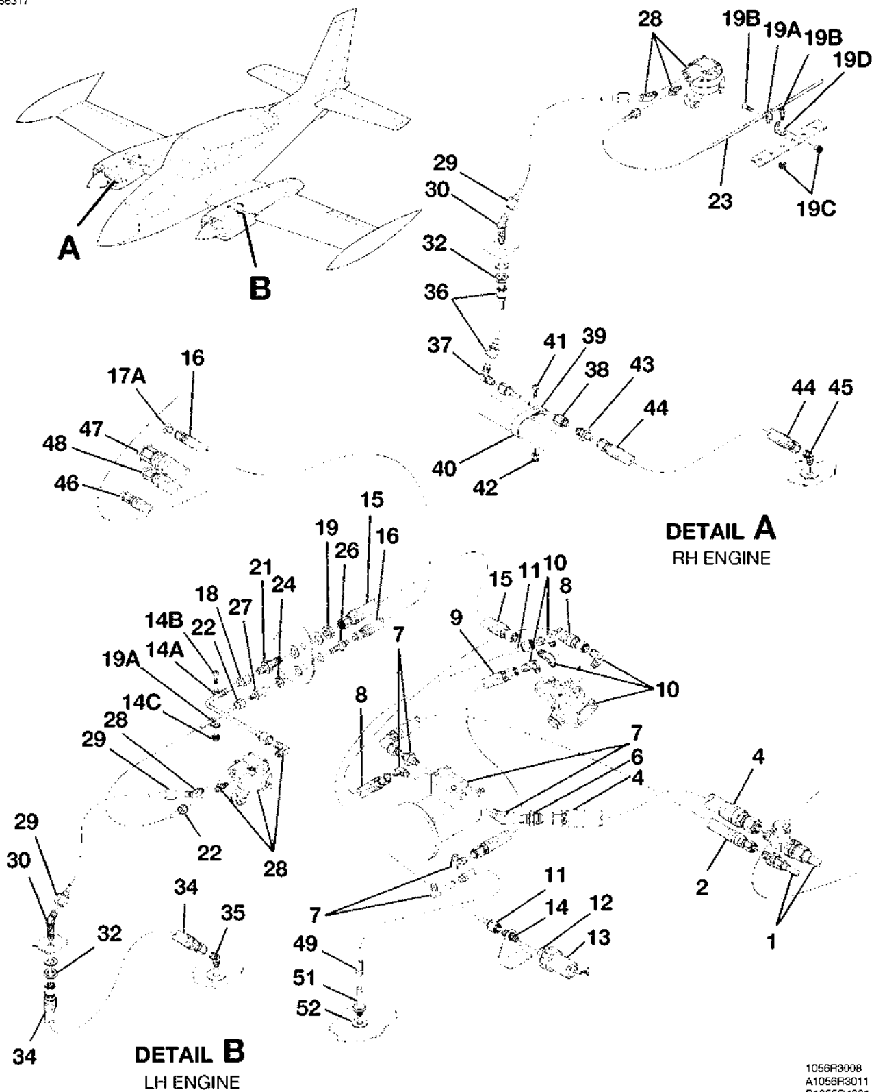
ENGINE COMPARTMENT FUEL SYSTEM COMPONENTS FIGURE 01 (SHEET 1)
