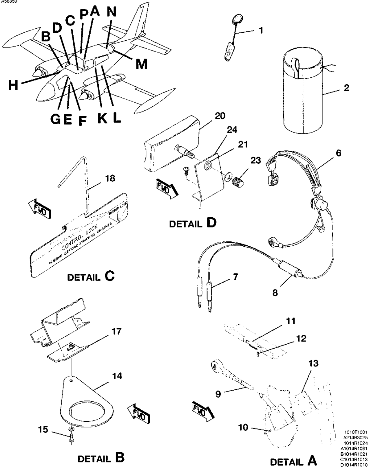
MISCELLANEOUS EQUIPMENT FIGURE 01 (SHEET 1)
