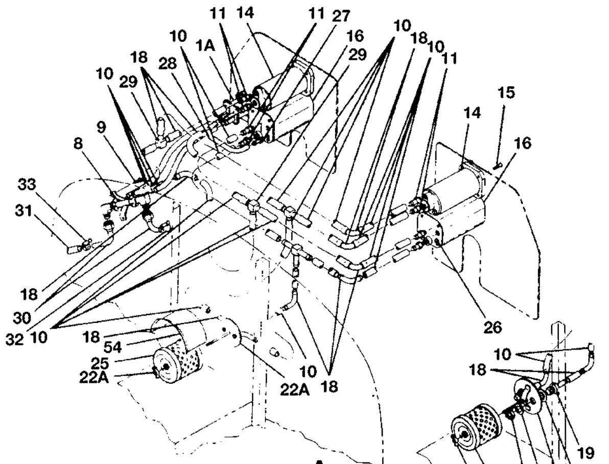
DETAIL A
