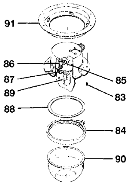
DETAIL K
