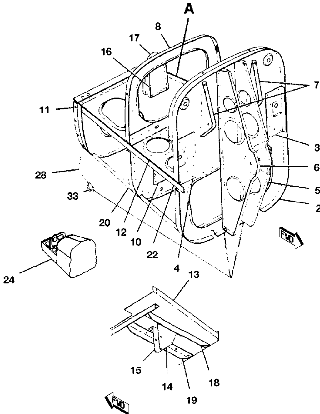
DETAIL A
