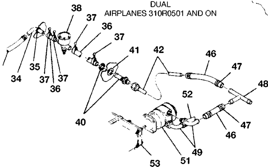
DETAIL B
