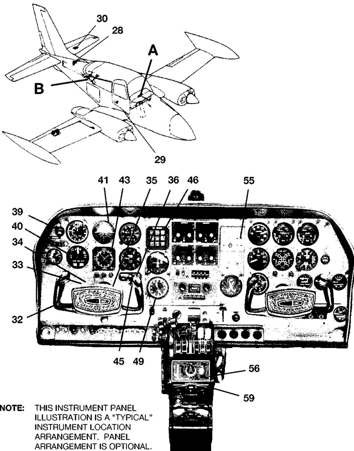
INTEGRATED FLIGHT CONTROL SYSTEM FIGURE 03 (SHEET 1)
