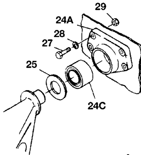
DETAIL A SMALL LUG (1.19 DIAMETER) TRUNNION
