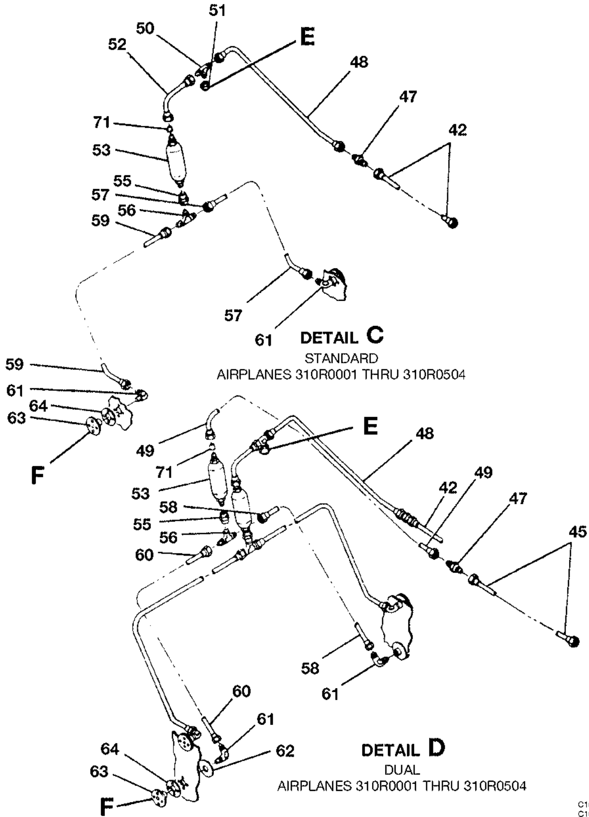
STATIC SYSTEM FIGURE 01 (SHEET 2)
