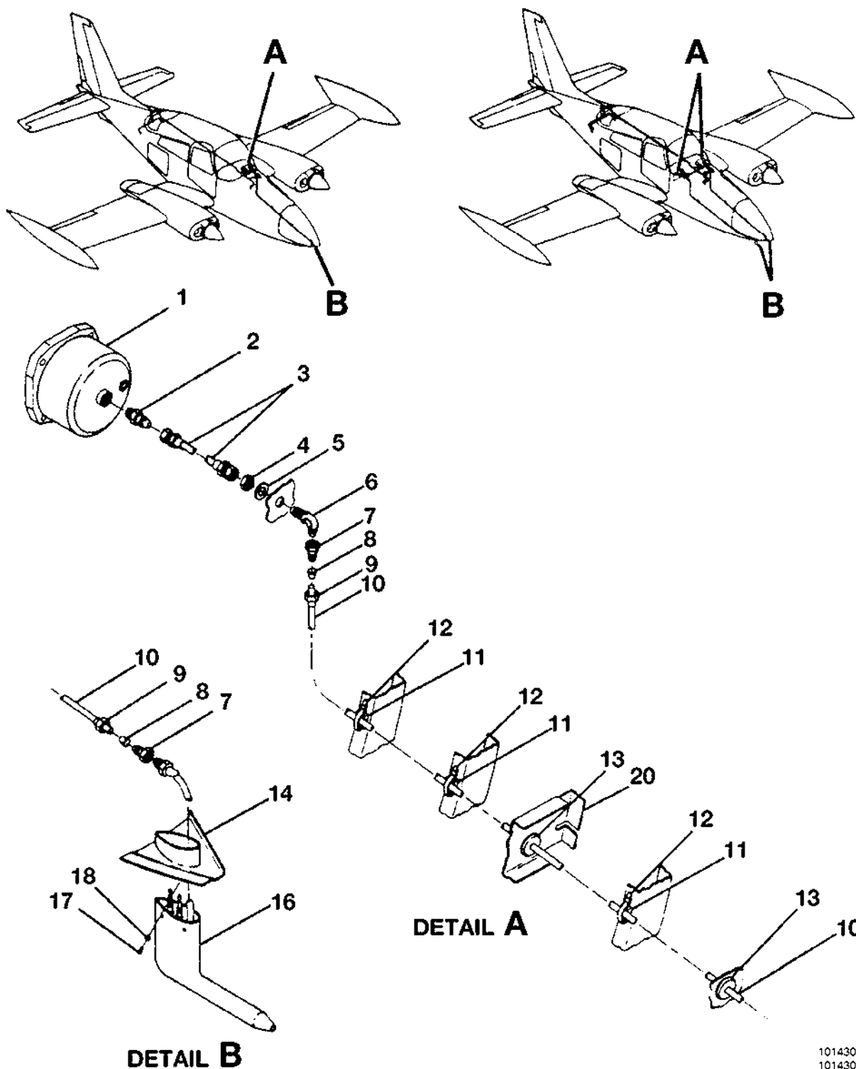
PITOT SYSTEM FIGURE 02 (SHEET 1)
